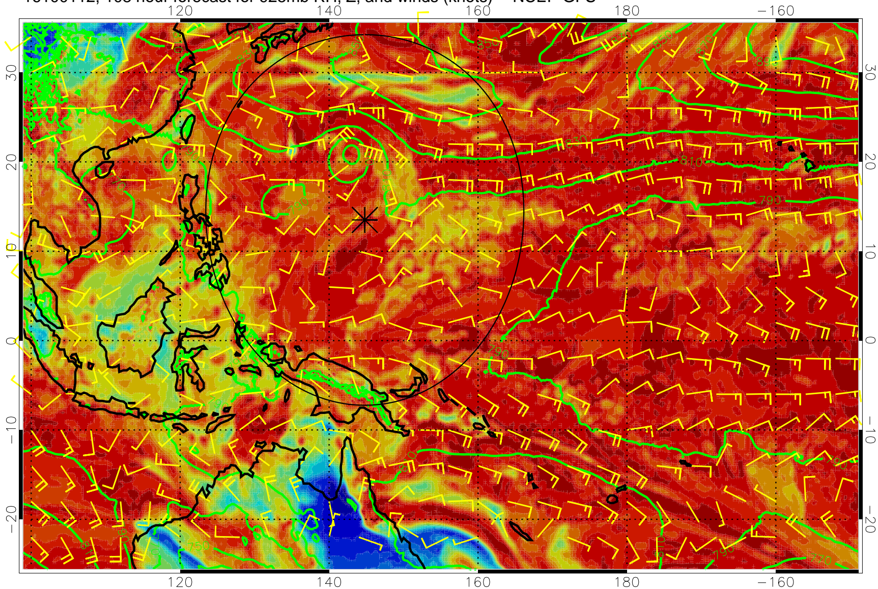
16100112, 108 hour forecast for 925mb RH, Z, and winds (knots) -- NCEP GFS
