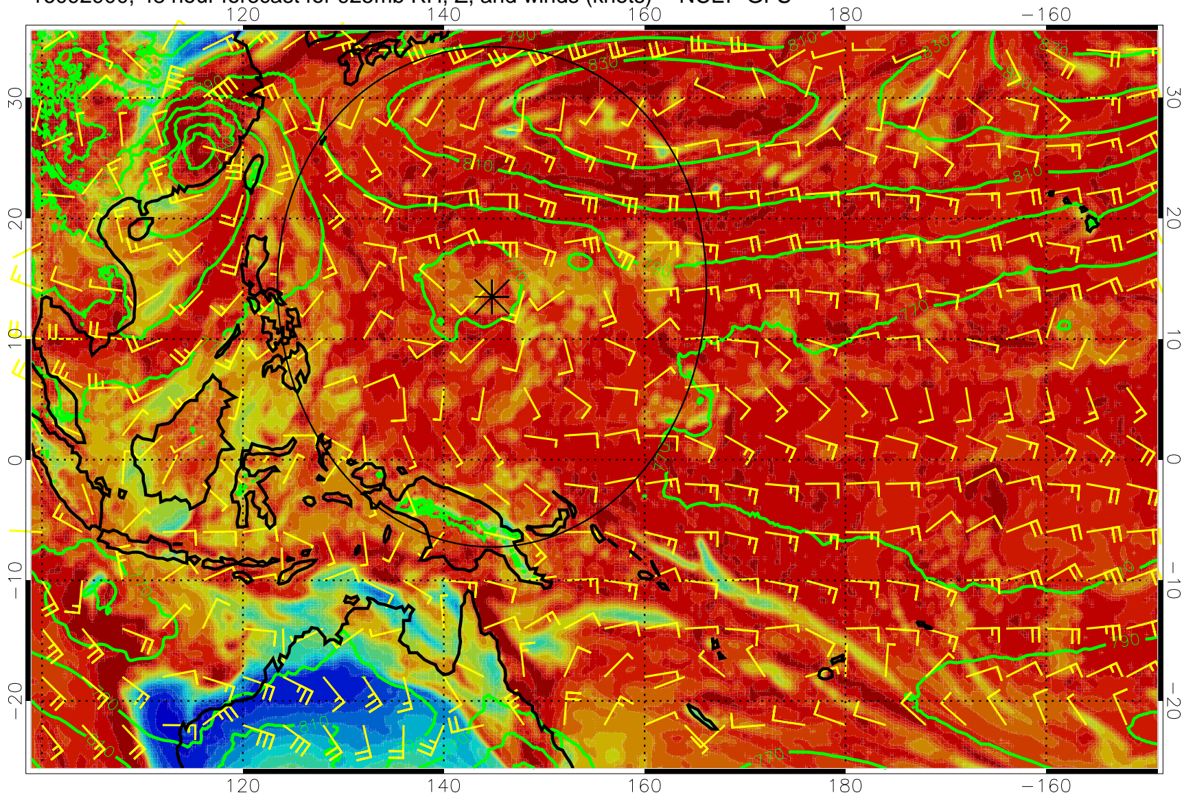
16092900, 48 hour forecast for 925mb RH, Z, and winds (knots) -- NCEP GFS
