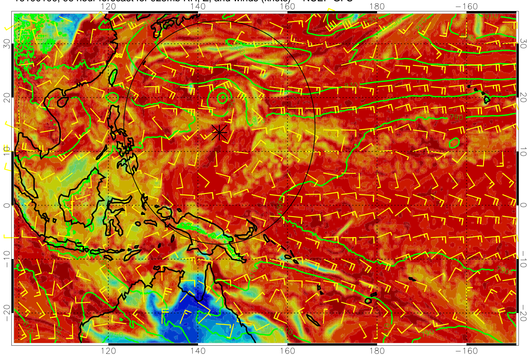
16100100, 96 hour forecast for 925mb RH, Z, and winds (knots) -- NCEP GFS
