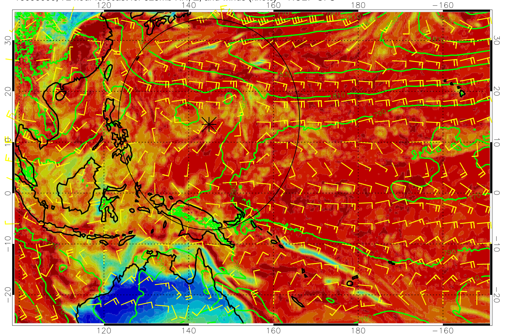
16093000, 72 hour forecast for 925mb RH, Z, and winds (knots) -- NCEP GFS
