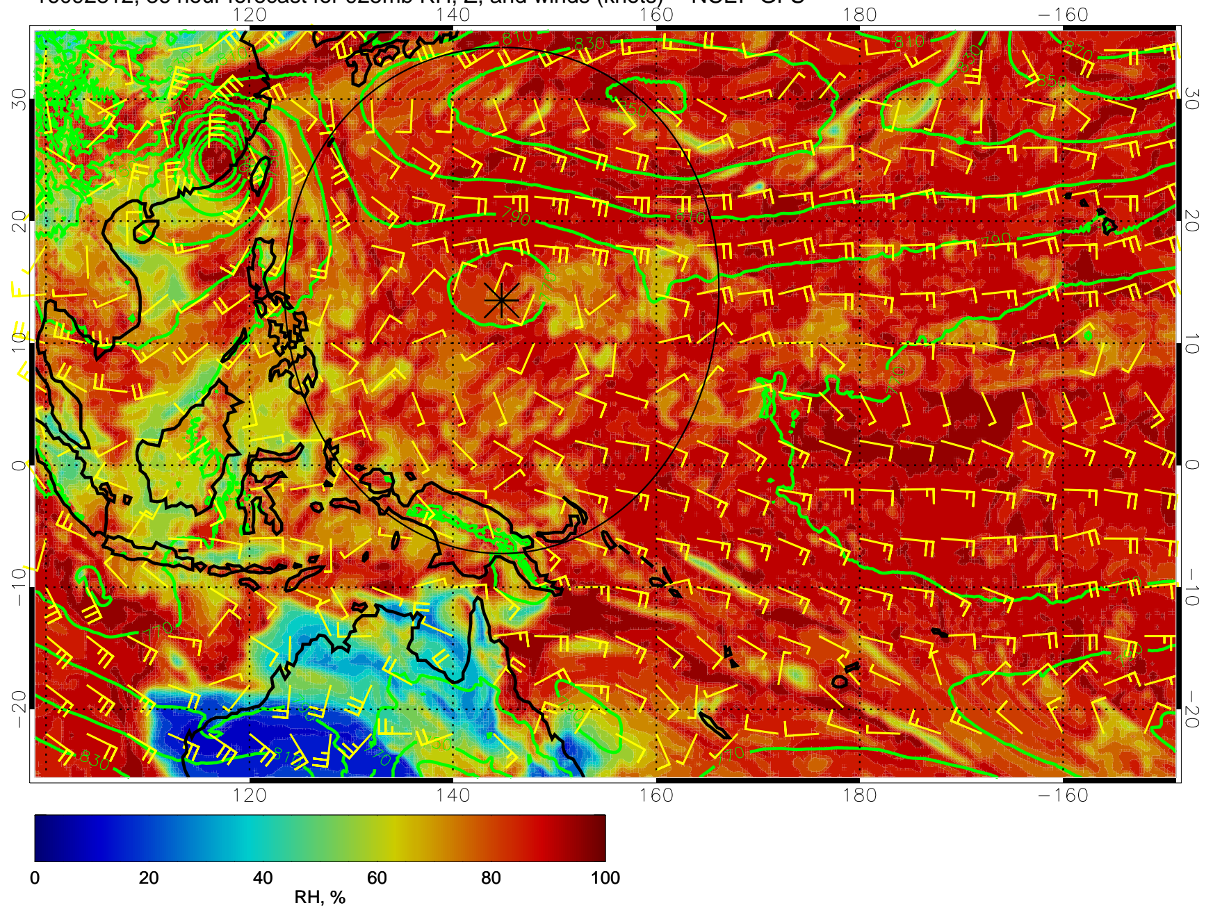
16092812, 36 hour forecast for 925mb RH, Z, and winds (knots) -- NCEP GFS
