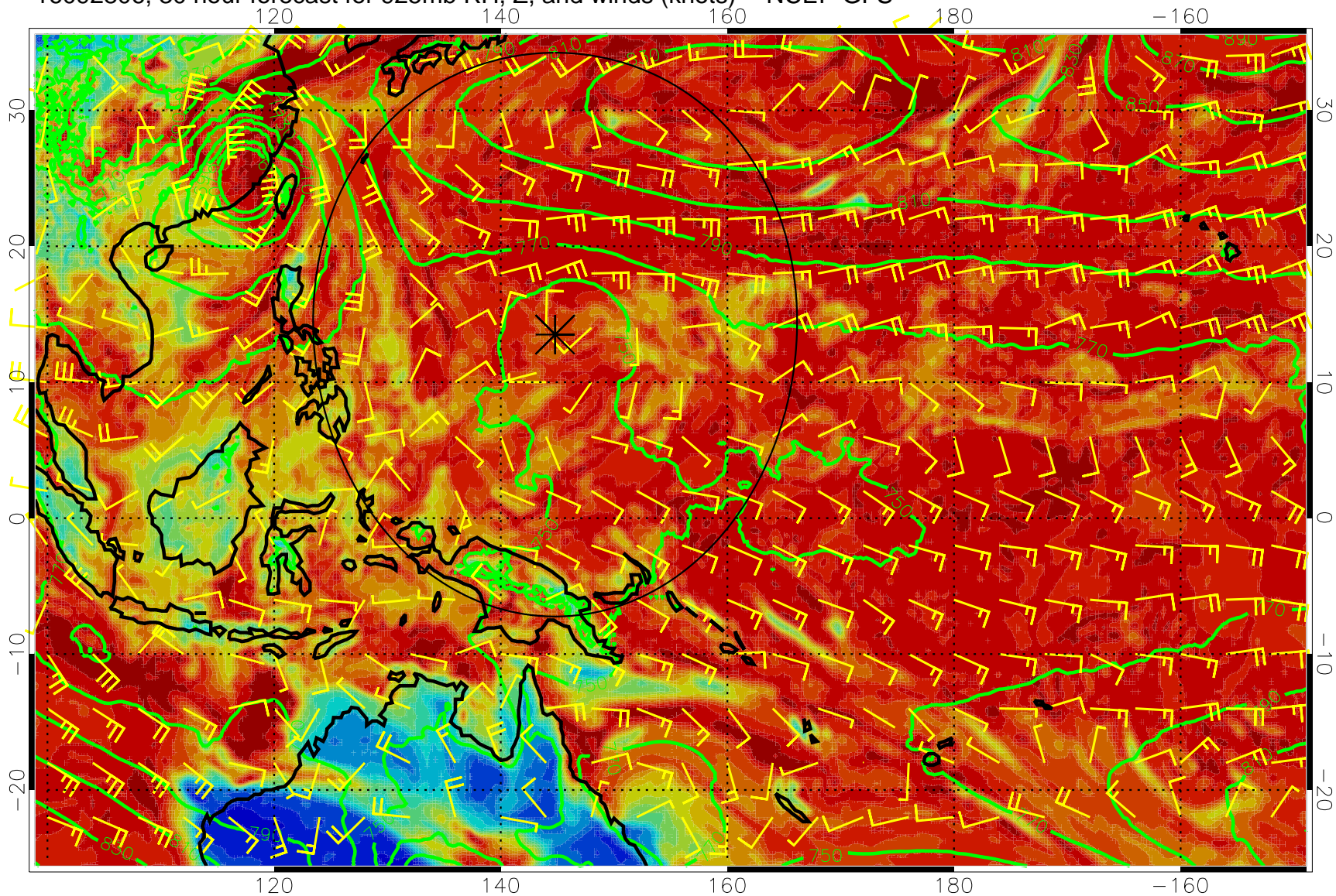
16092806, 30 hour forecast for 925mb RH, Z, and winds (knots) -- NCEP GFS
