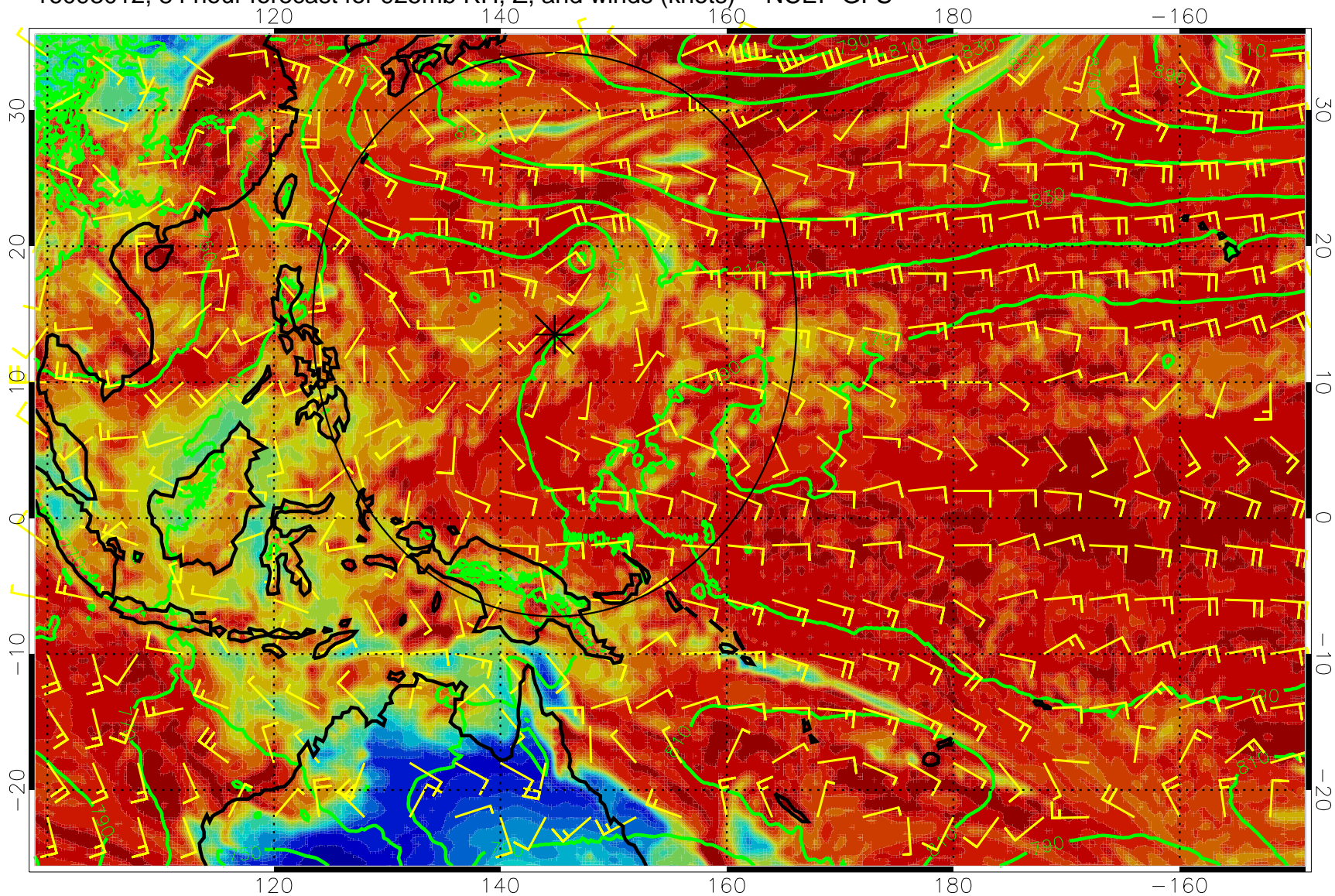
16093012, 84 hour forecast for 925mb RH, Z, and winds (knots) -- NCEP GFS
