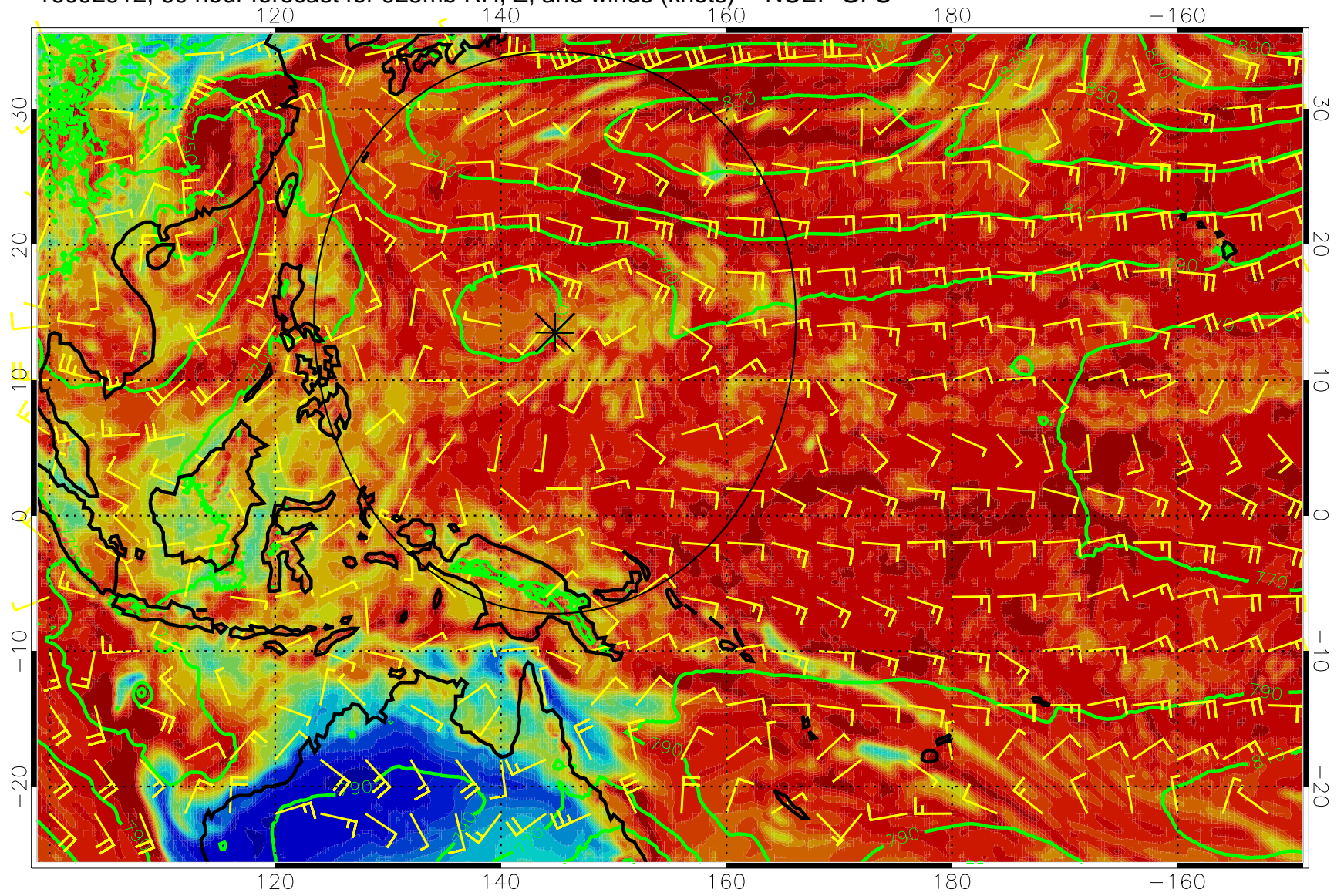
16092912, 60 hour forecast for 925mb RH, Z, and winds (knots) -- NCEP GFS
