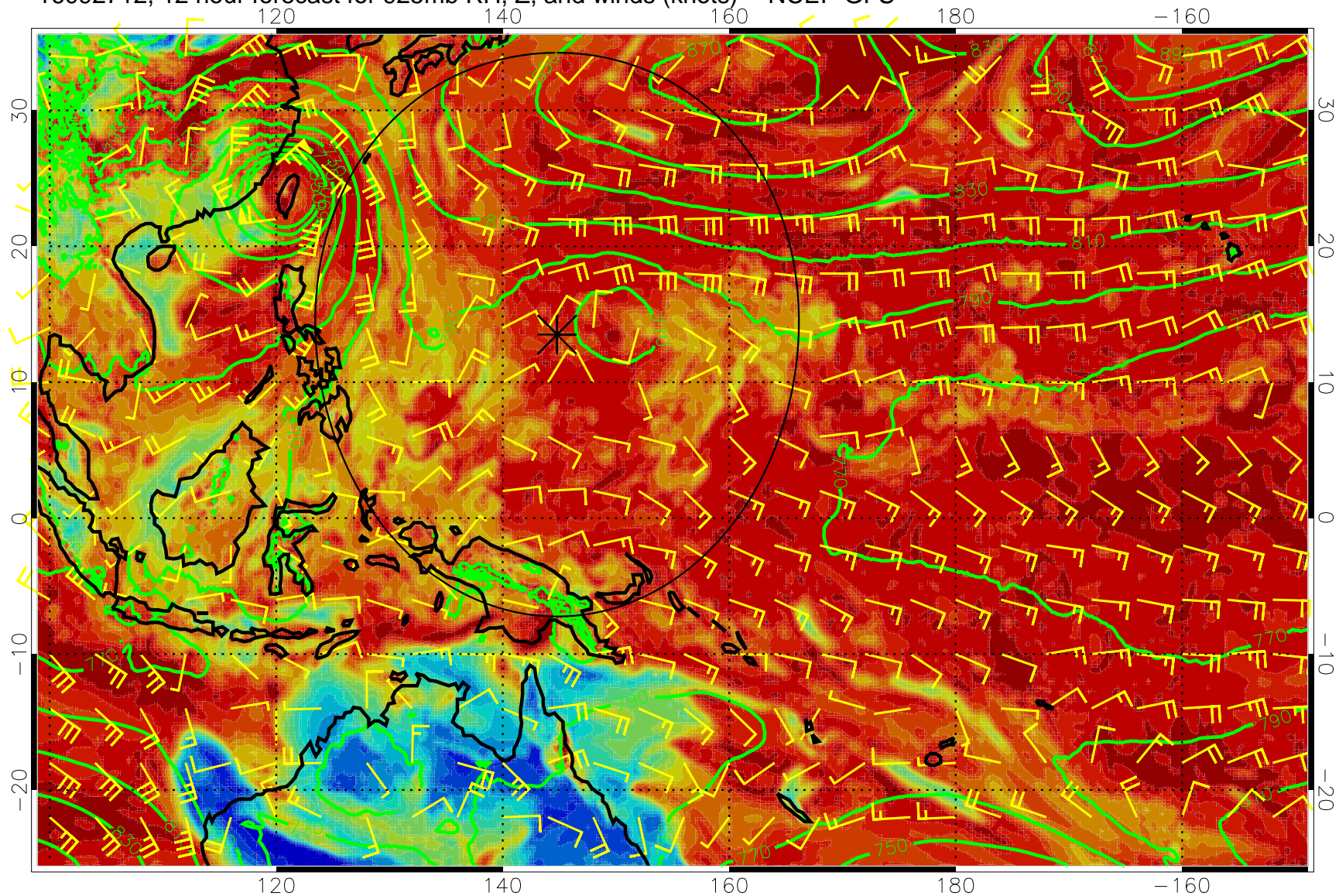
16092712, 12 hour forecast for 925mb RH, Z, and winds (knots) -- NCEP GFS
