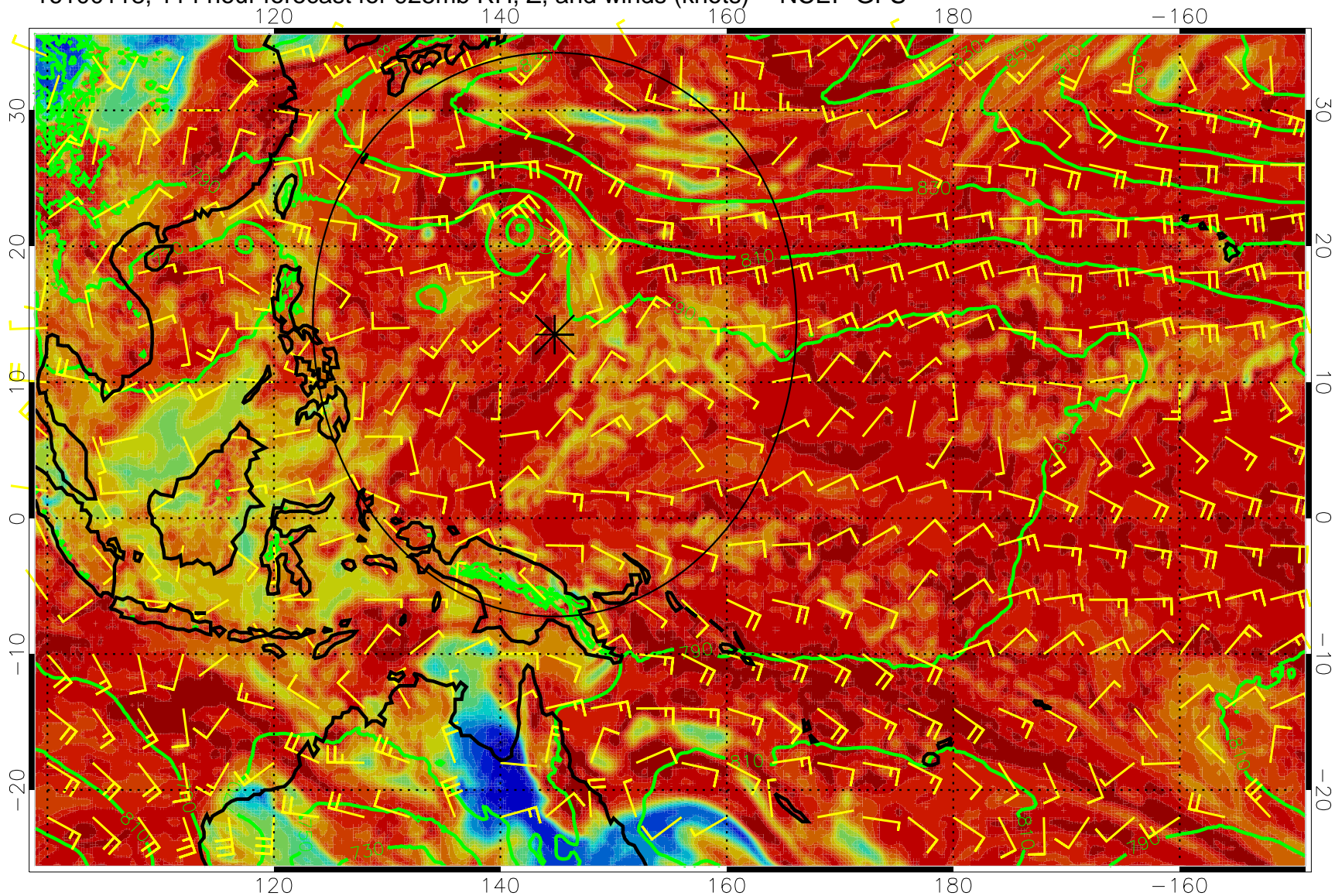
16100118, 114 hour forecast for 925mb RH, Z, and winds (knots) -- NCEP GFS
