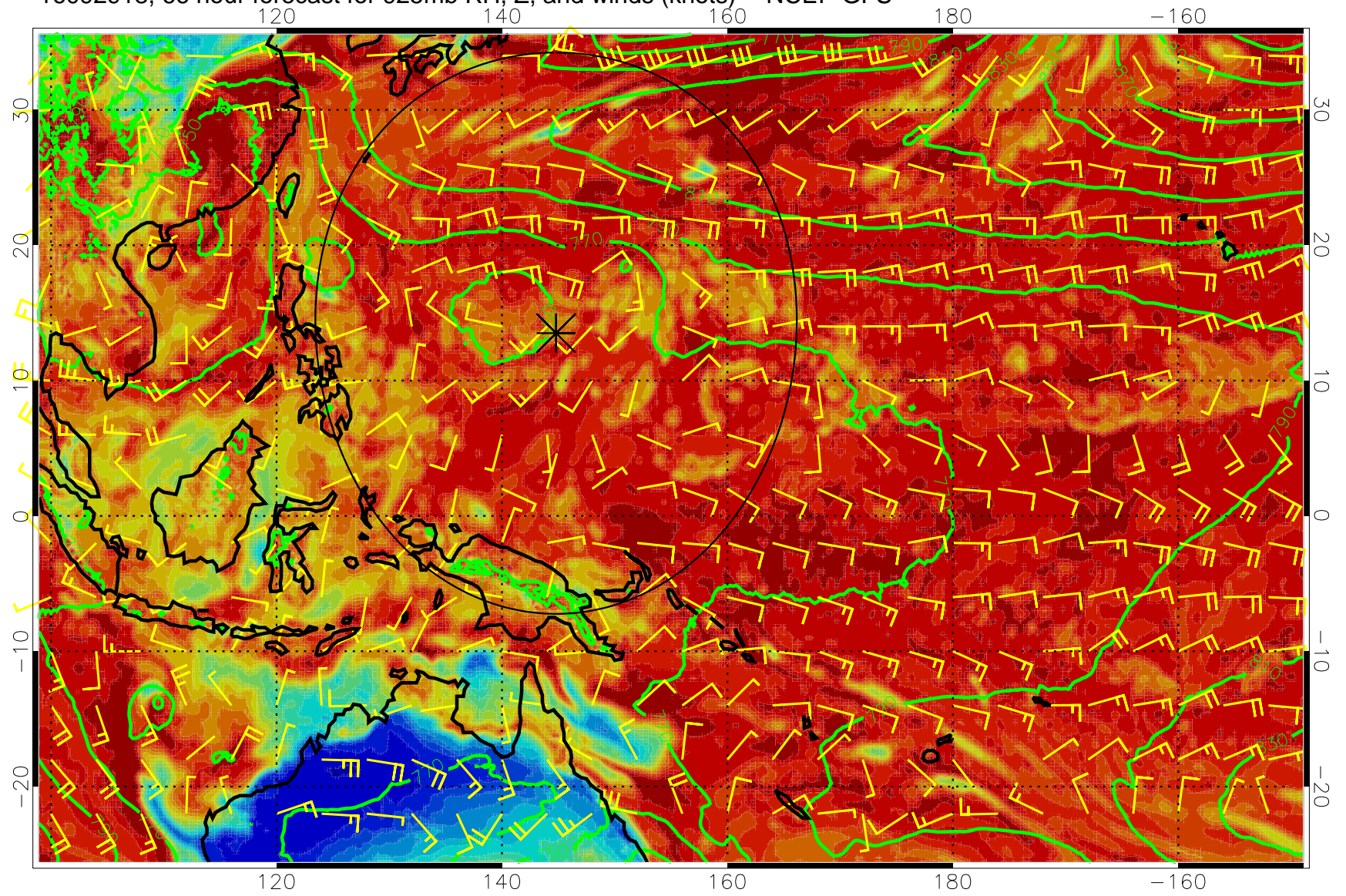
16092918, 66 hour forecast for 925mb RH, Z, and winds (knots) -- NCEP GFS
