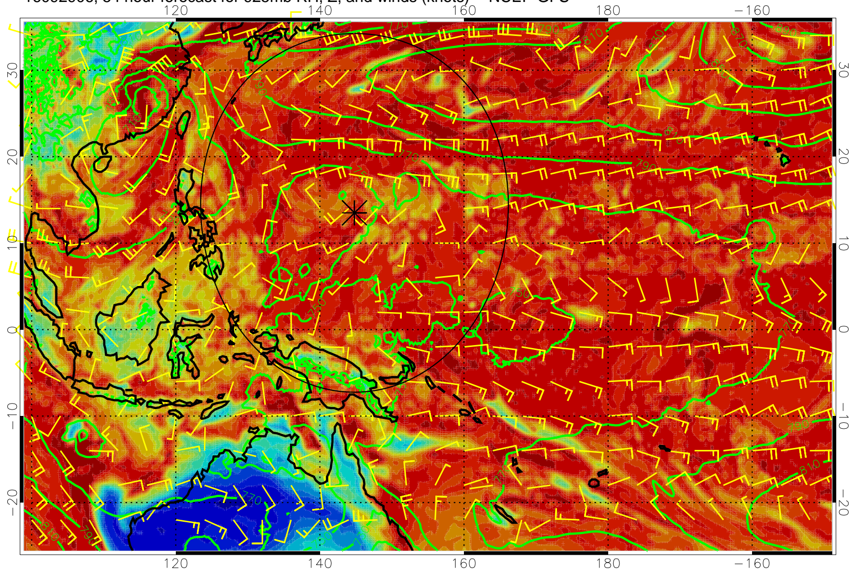
16092906, 54 hour forecast for 925mb RH, Z, and winds (knots) -- NCEP GFS
