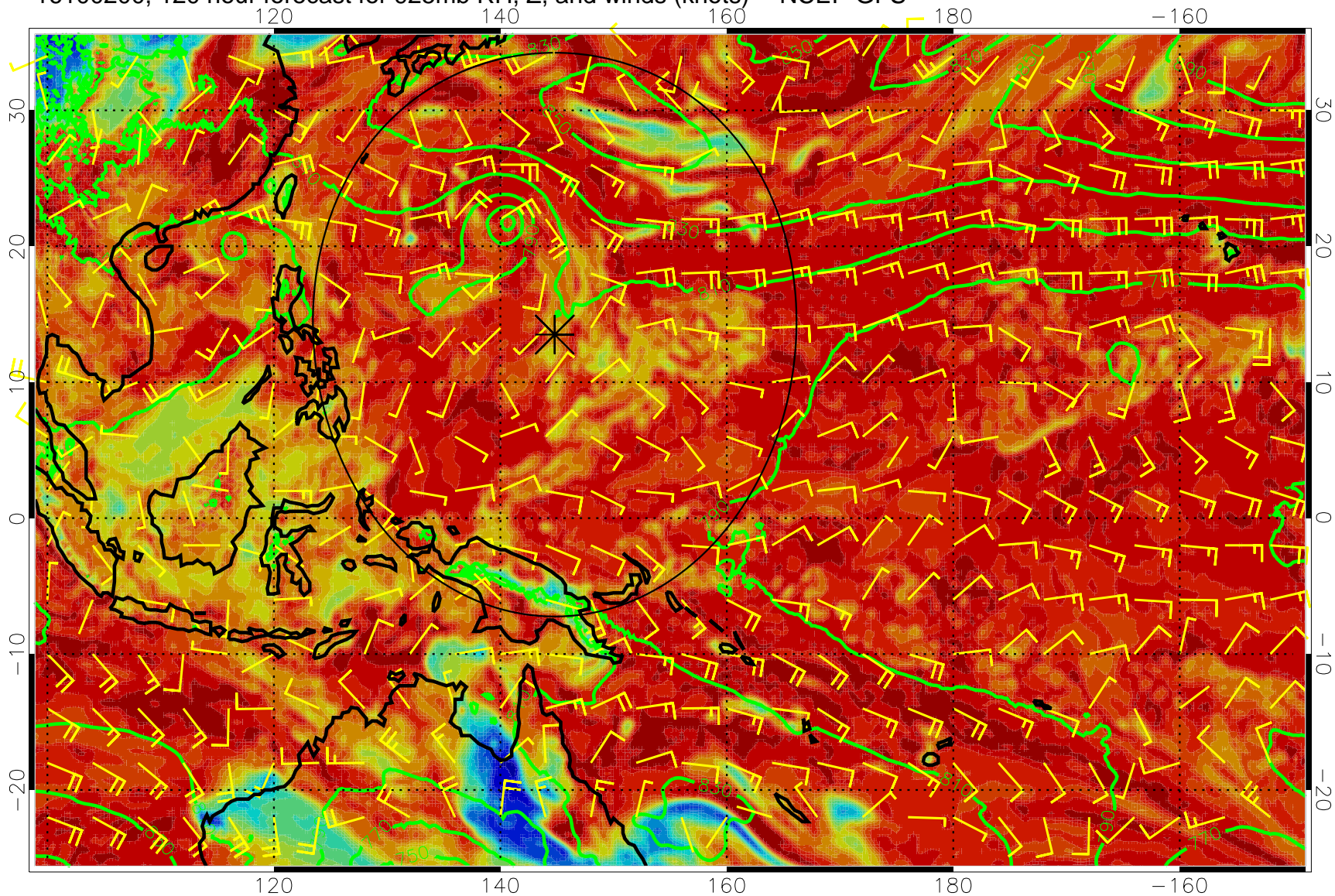
16100200, 120 hour forecast for 925mb RH, Z, and winds (knots) -- NCEP GFS
