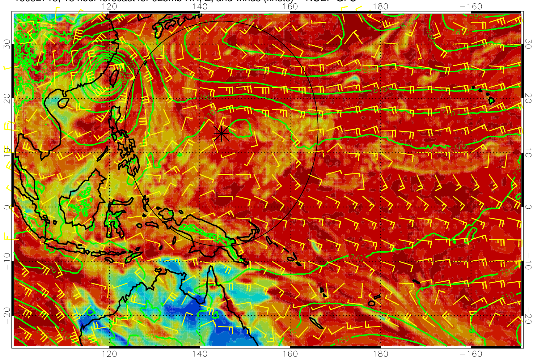
16092718, 18 hour forecast for 925mb RH, Z, and winds (knots) -- NCEP GFS
