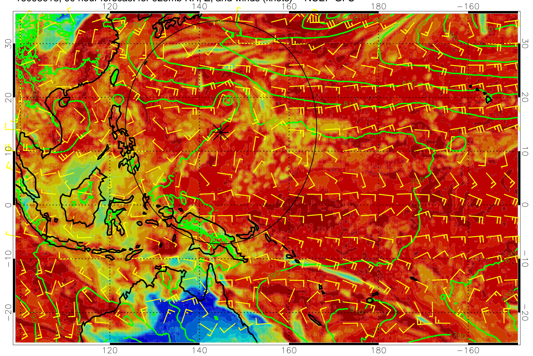
16093018, 90 hour forecast for 925mb RH, Z, and winds (knots) -- NCEP GFS
