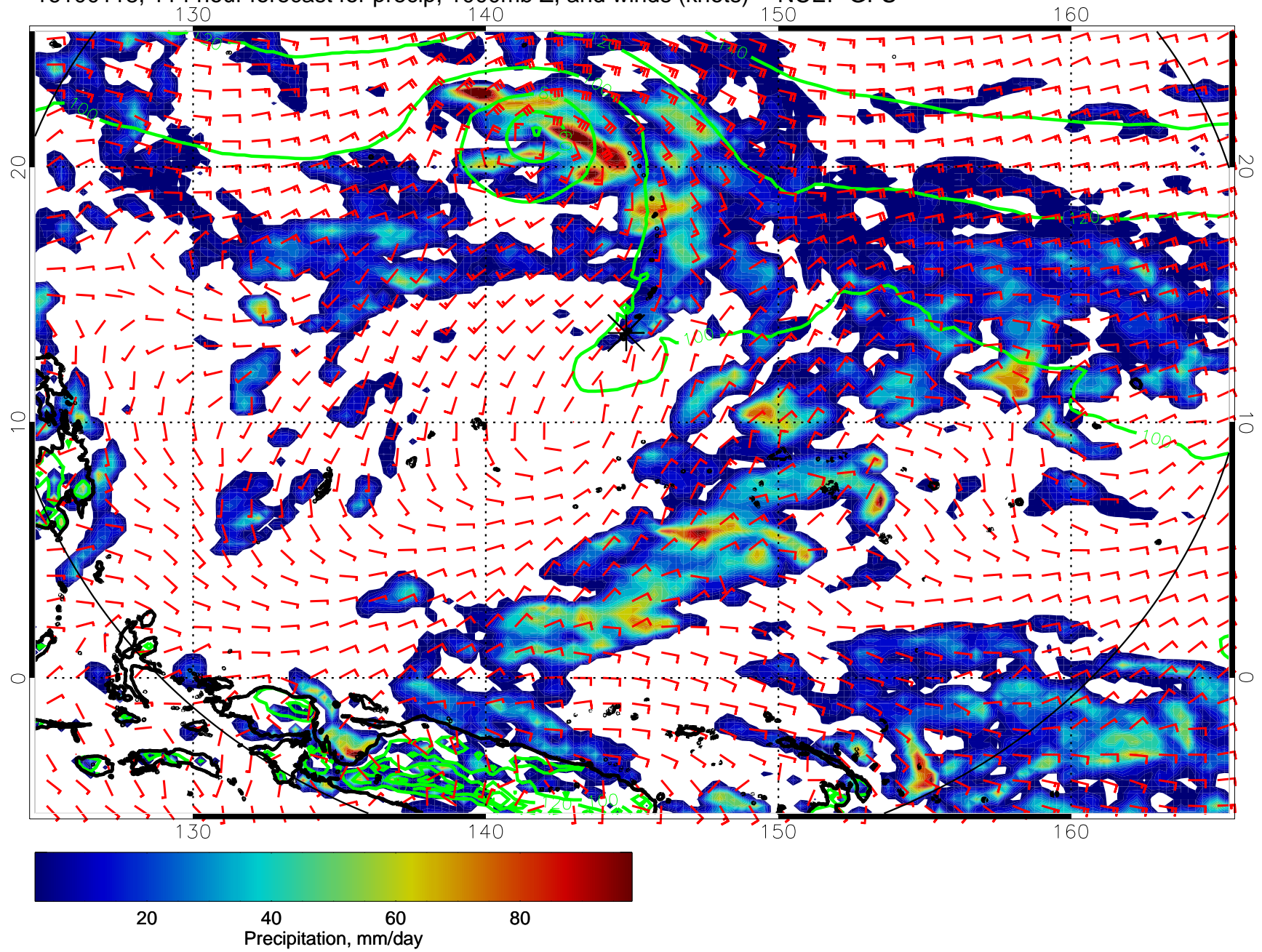
16100118, 114 hour forecast for precip, 1000mb Z, and winds (knots) -- NCEP GFS
