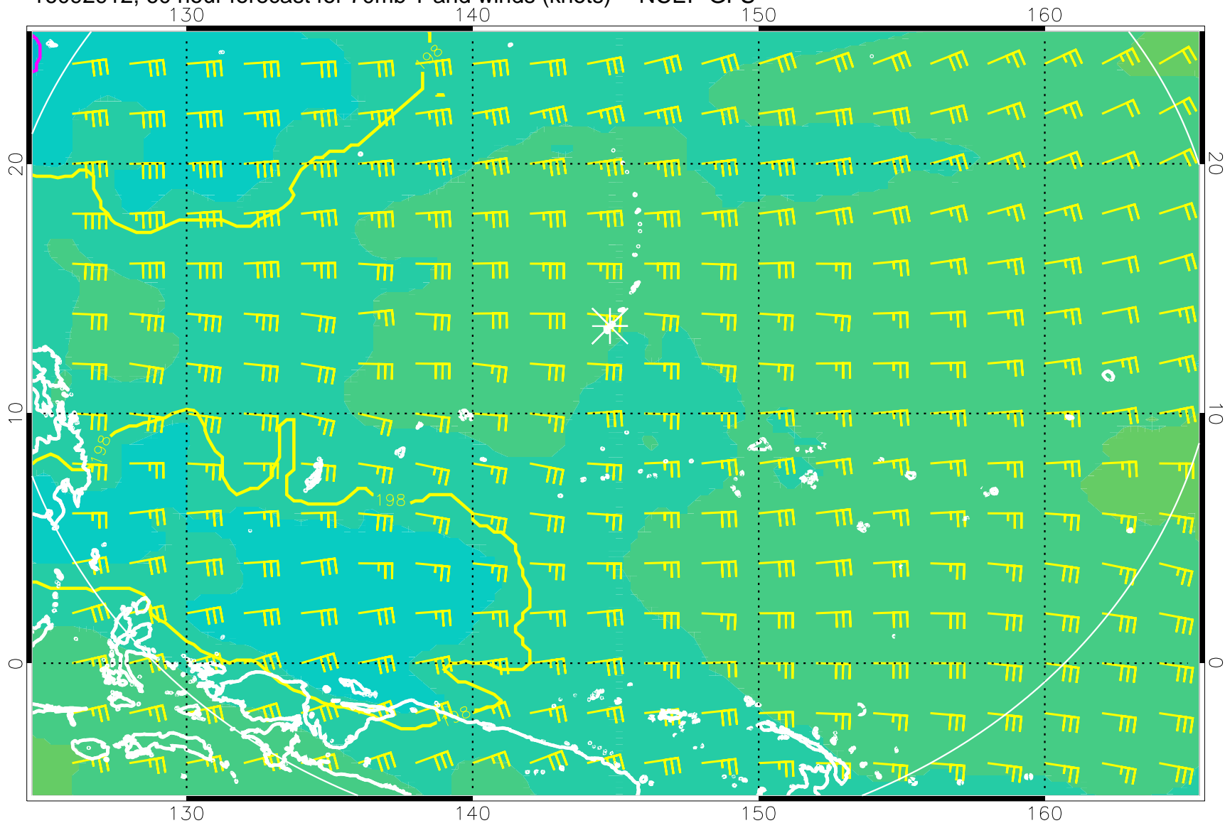
16092912, 60 hour forecast for 70mb T and winds (knots) -- NCEP GFS
