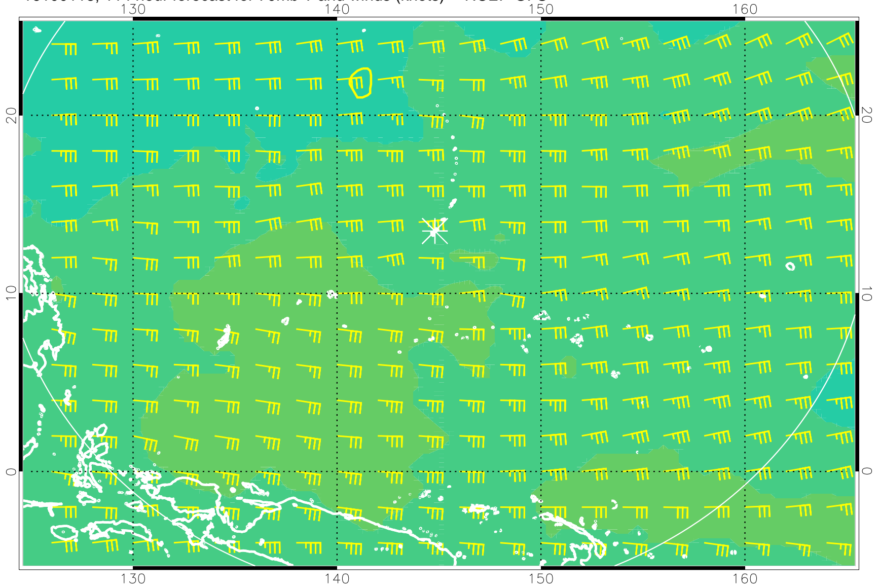
16100118, 114 hour forecast for 70mb T and winds (knots) -- NCEP GFS
