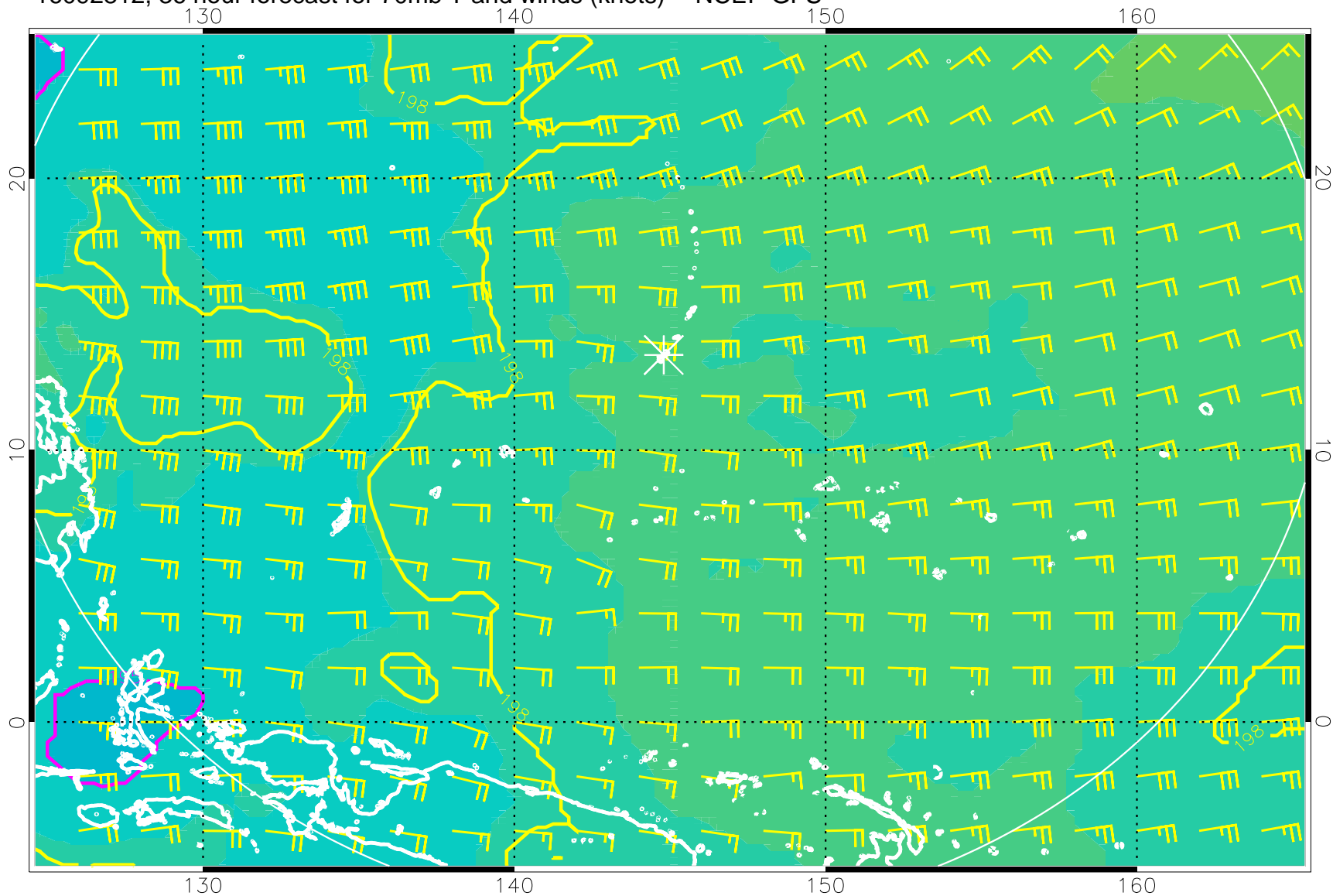
16092812, 36 hour forecast for 70mb T and winds (knots) -- NCEP GFS
