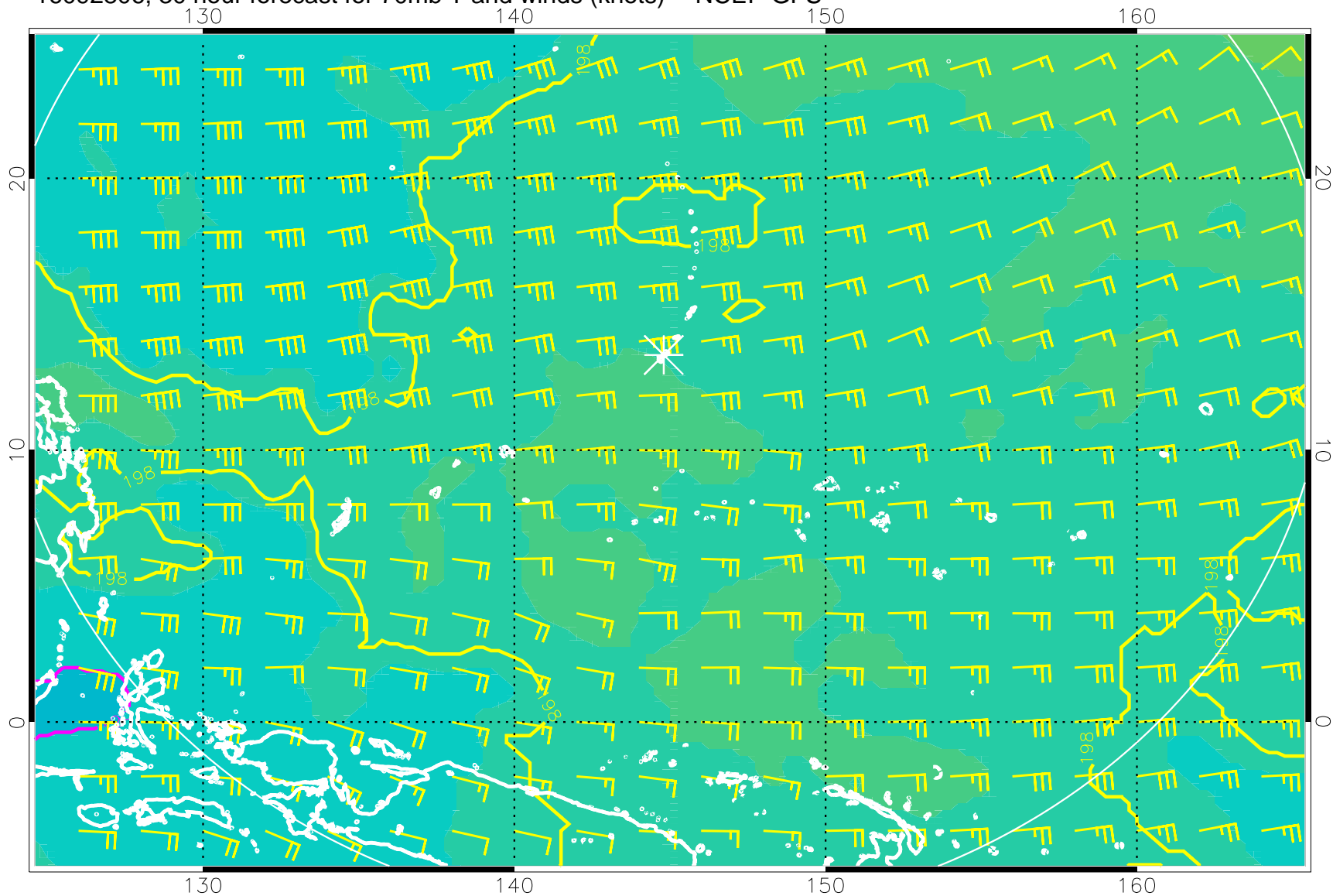
16092806, 30 hour forecast for 70mb T and winds (knots) -- NCEP GFS
