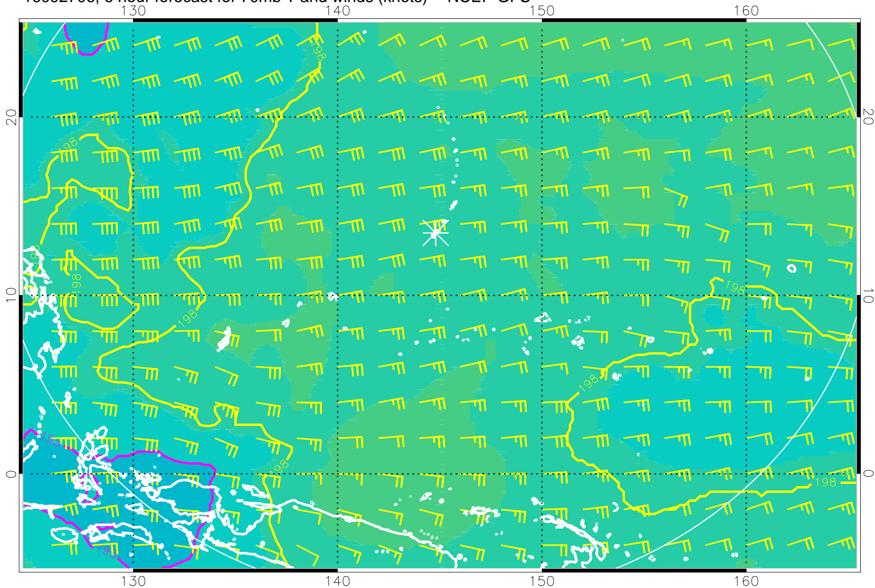
16092706, 6 hour forecast for 70mb T and winds (knots) -- NCEP GFS
