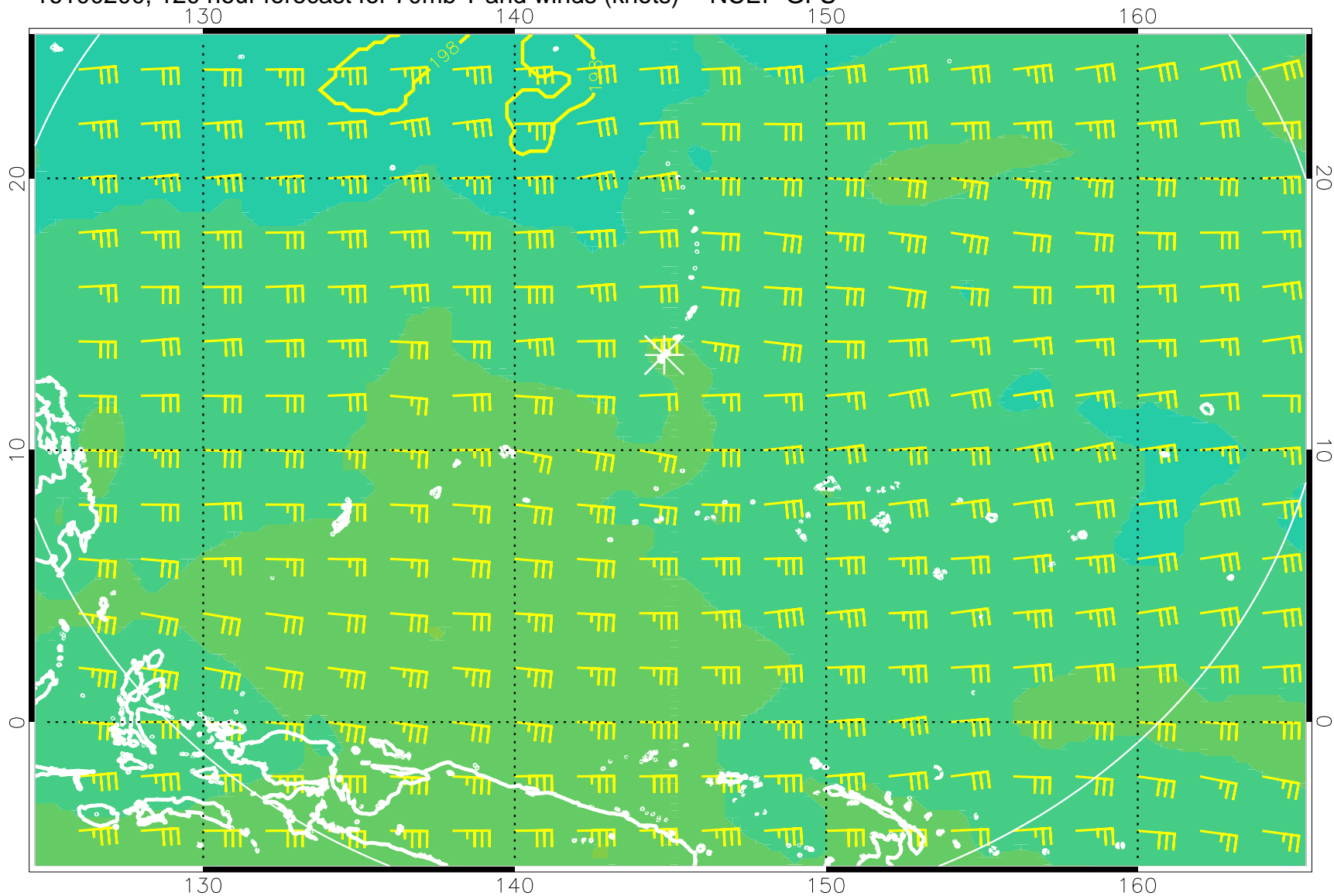
16100200, 120 hour forecast for 70mb T and winds (knots) -- NCEP GFS
