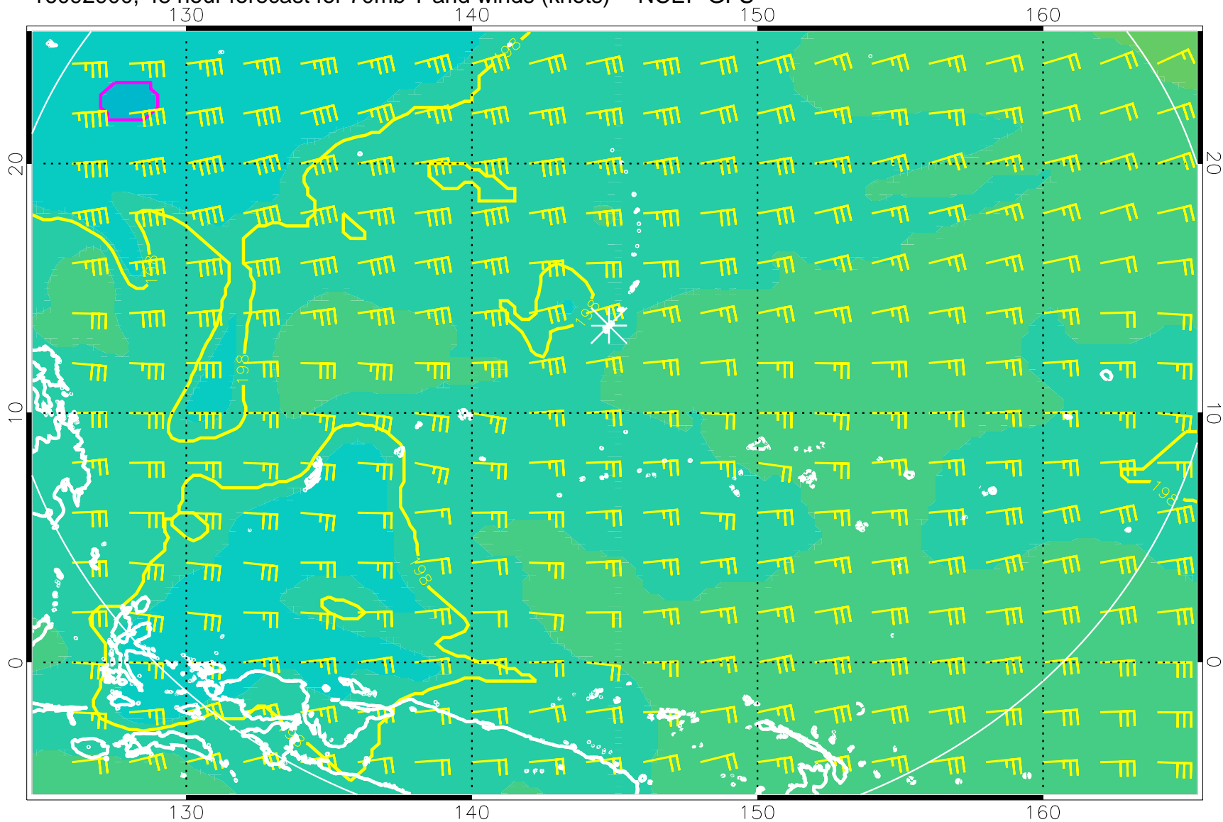
16092900, 48 hour forecast for 70mb T and winds (knots) -- NCEP GFS
