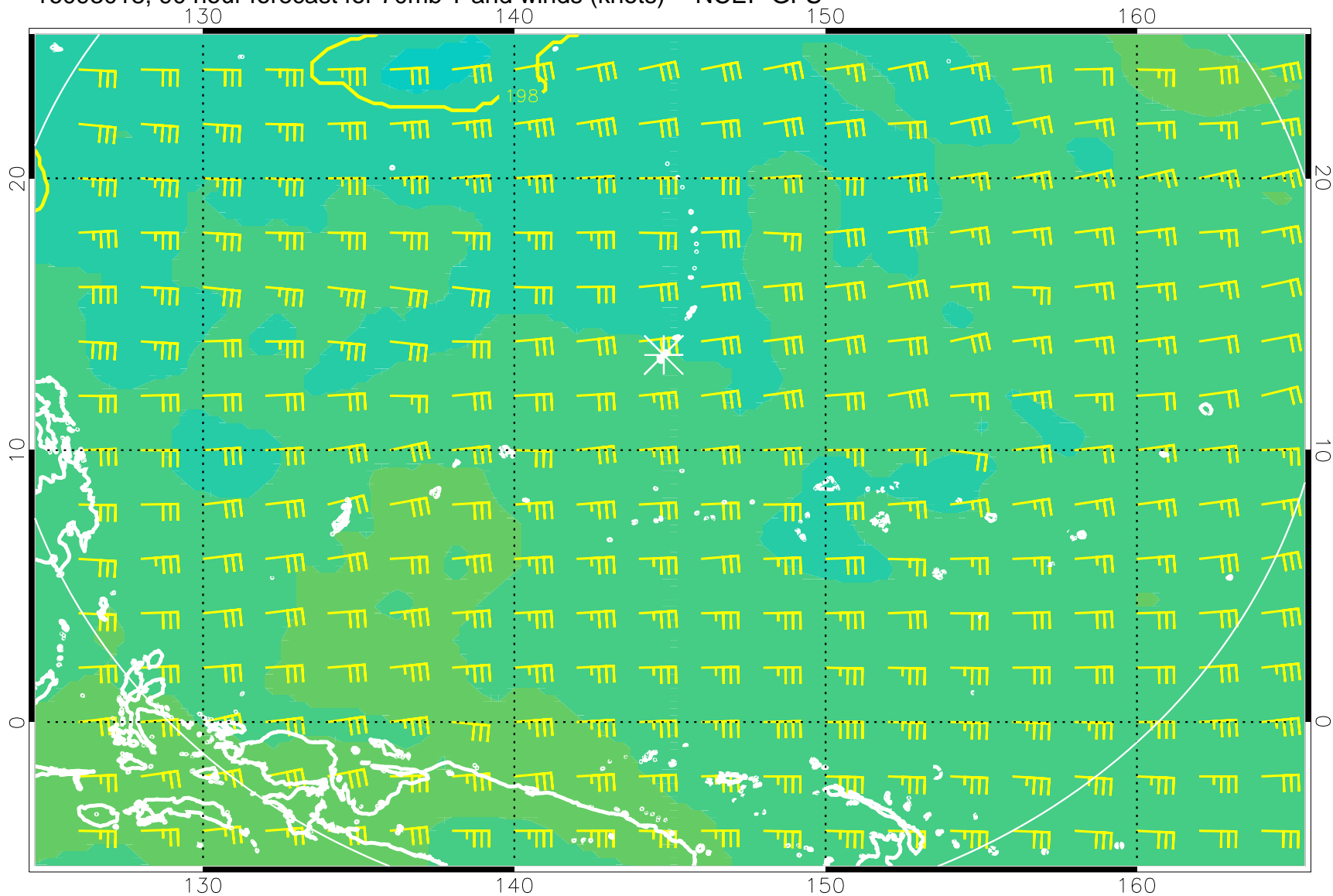
16093018, 90 hour forecast for 70mb T and winds (knots) -- NCEP GFS
