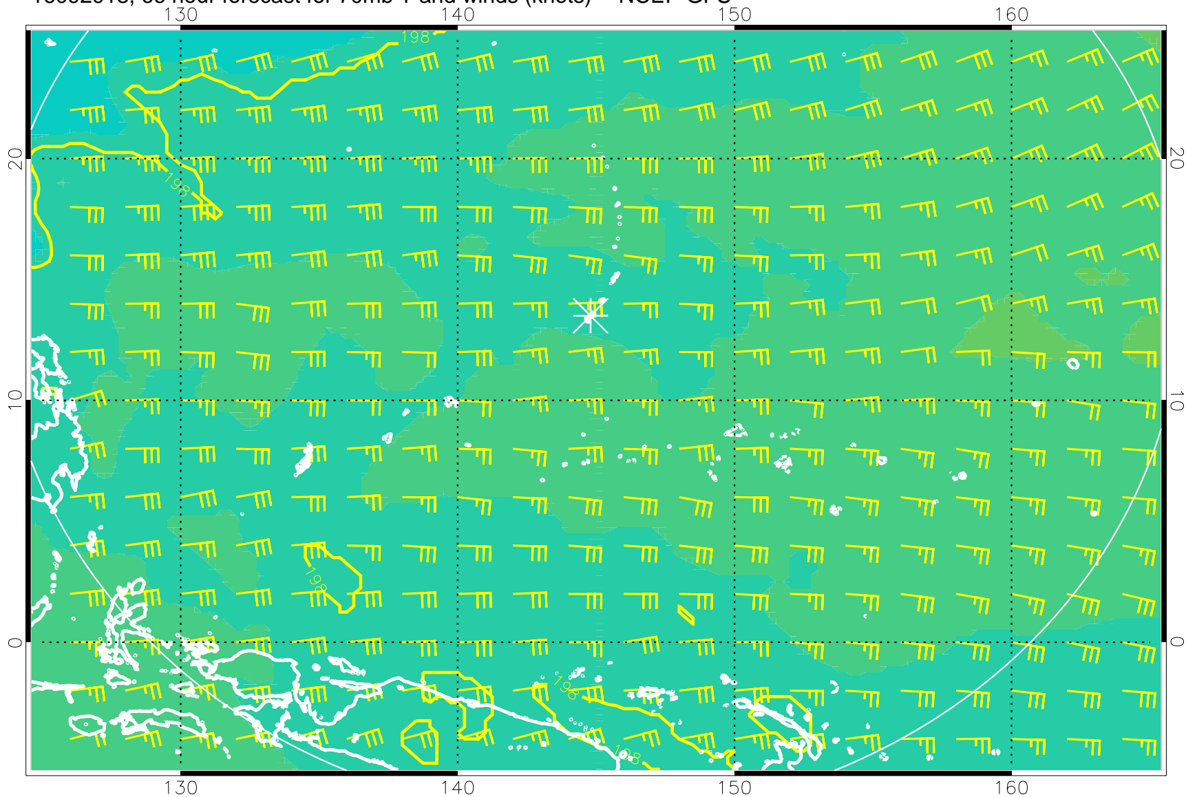
16092918, 66 hour forecast for 70mb T and winds (knots) -- NCEP GFS
