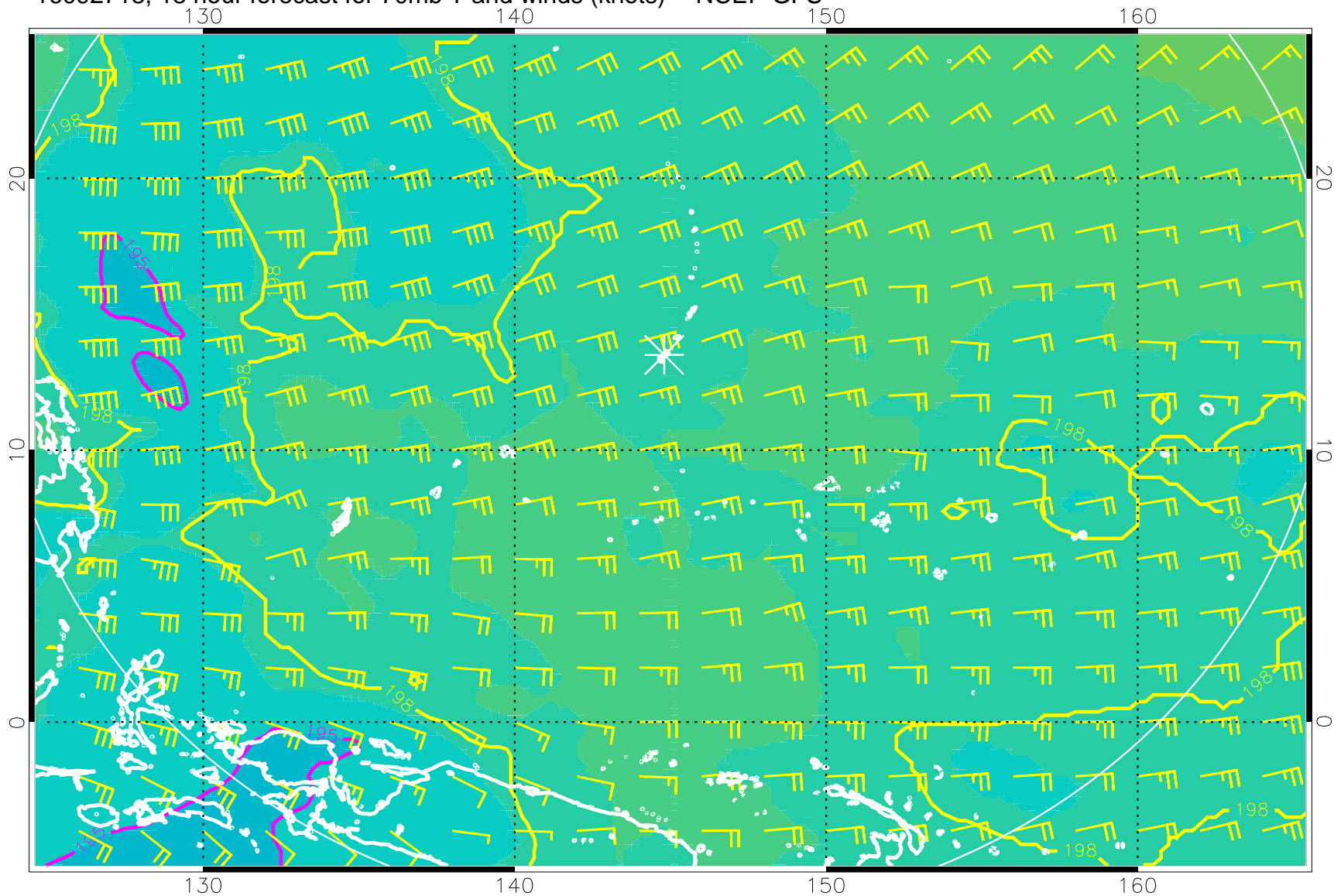
16092718, 18 hour forecast for 70mb T and winds (knots) -- NCEP GFS
