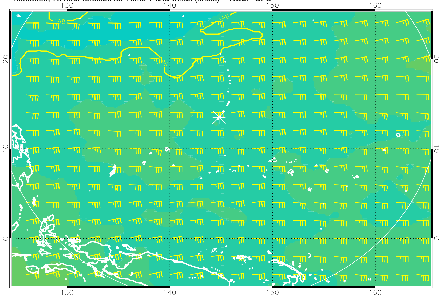
16093006, 78 hour forecast for 70mb T and winds (knots) -- NCEP GFS
