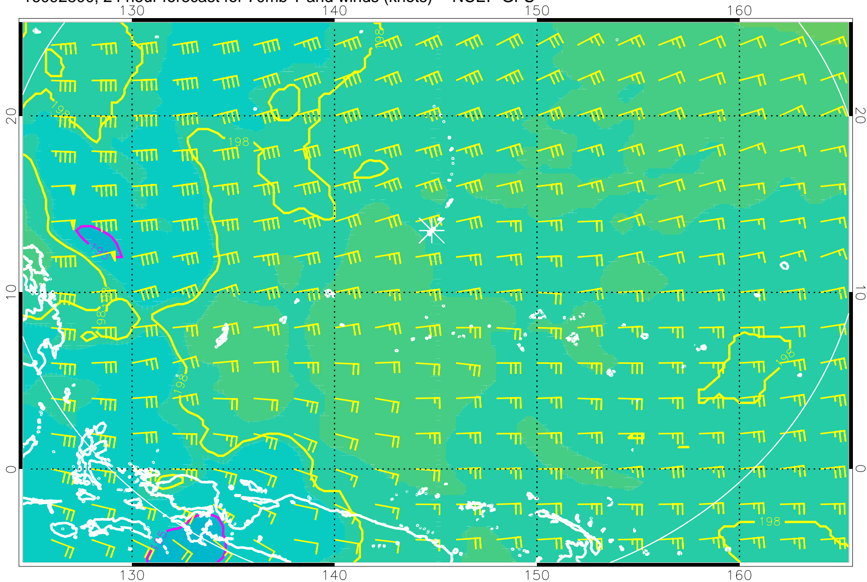
16092800, 24 hour forecast for 70mb T and winds (knots) -- NCEP GFS
