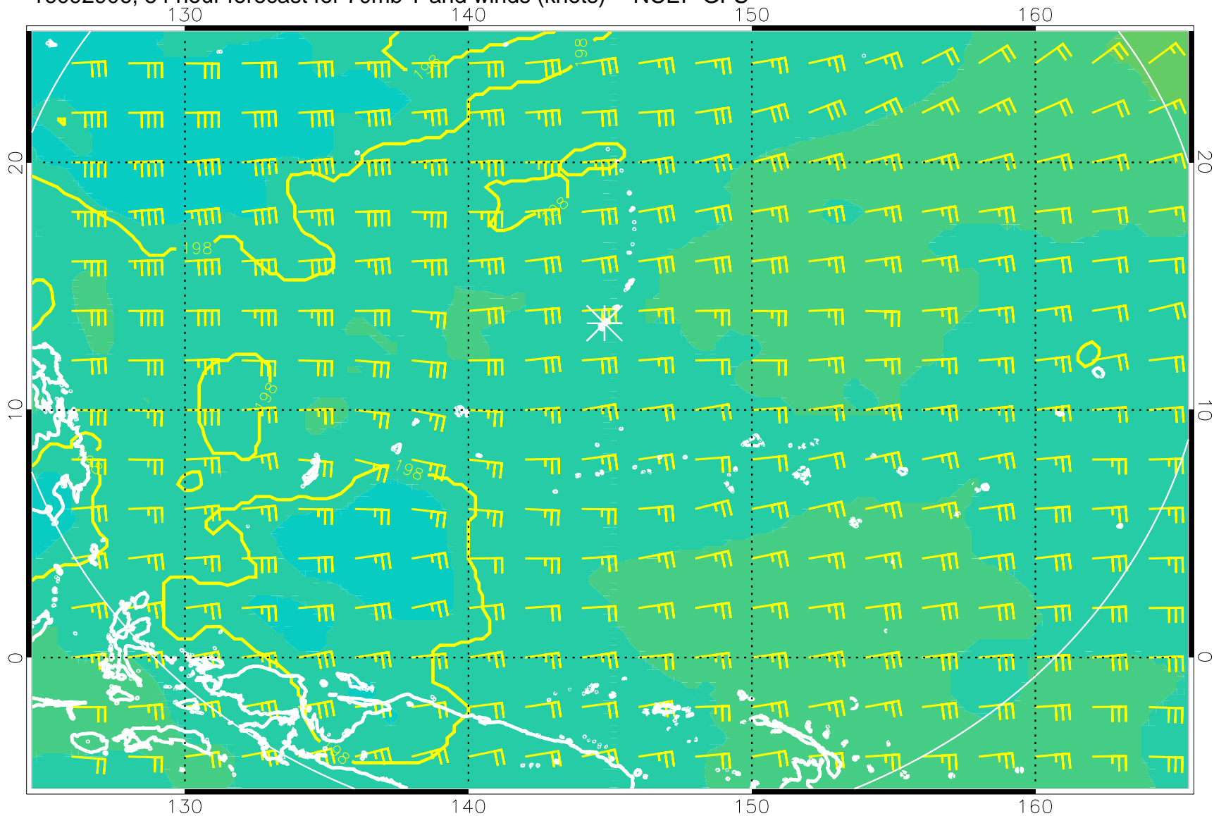
16092906, 54 hour forecast for 70mb T and winds (knots) -- NCEP GFS
