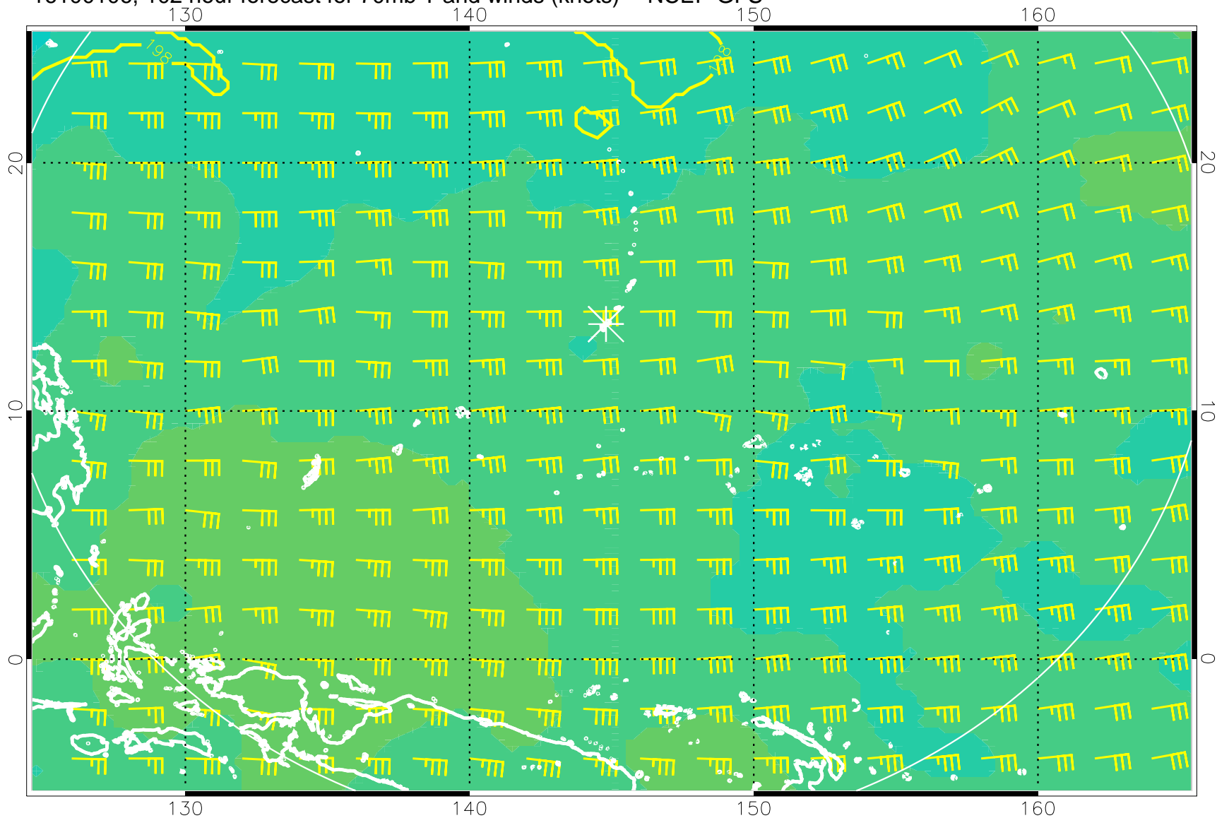
16100106, 102 hour forecast for 70mb T and winds (knots) -- NCEP GFS
