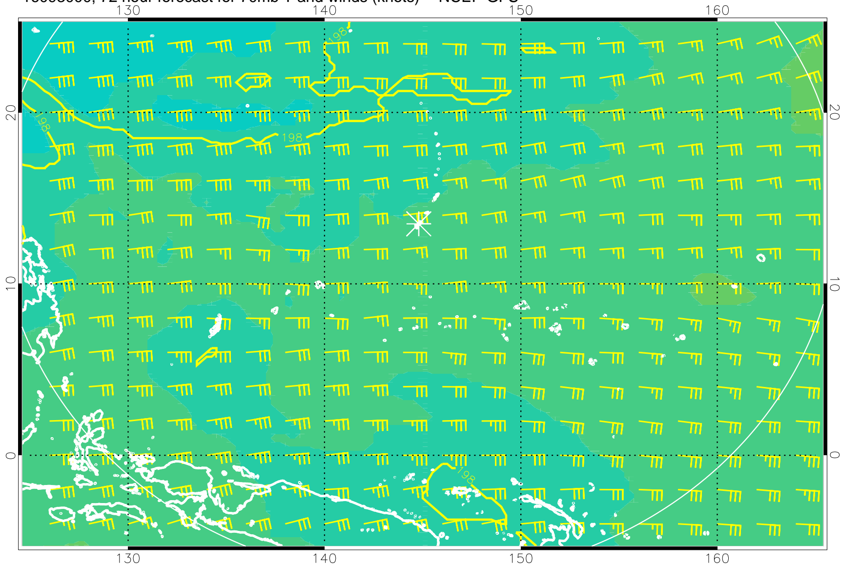
16093000, 72 hour forecast for 70mb T and winds (knots) -- NCEP GFS
