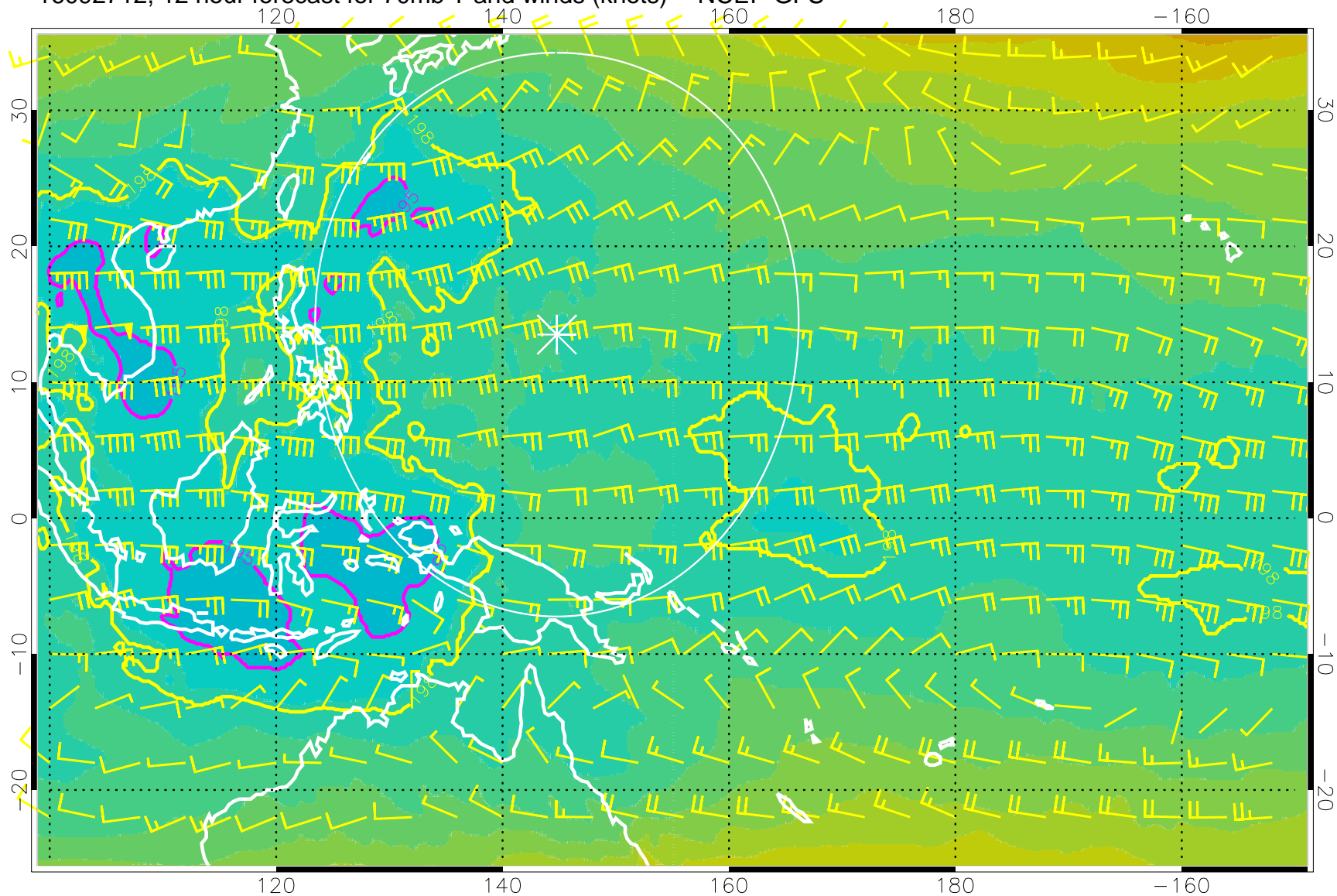
16092712, 12 hour forecast for 70mb T and winds (knots) -- NCEP GFS
