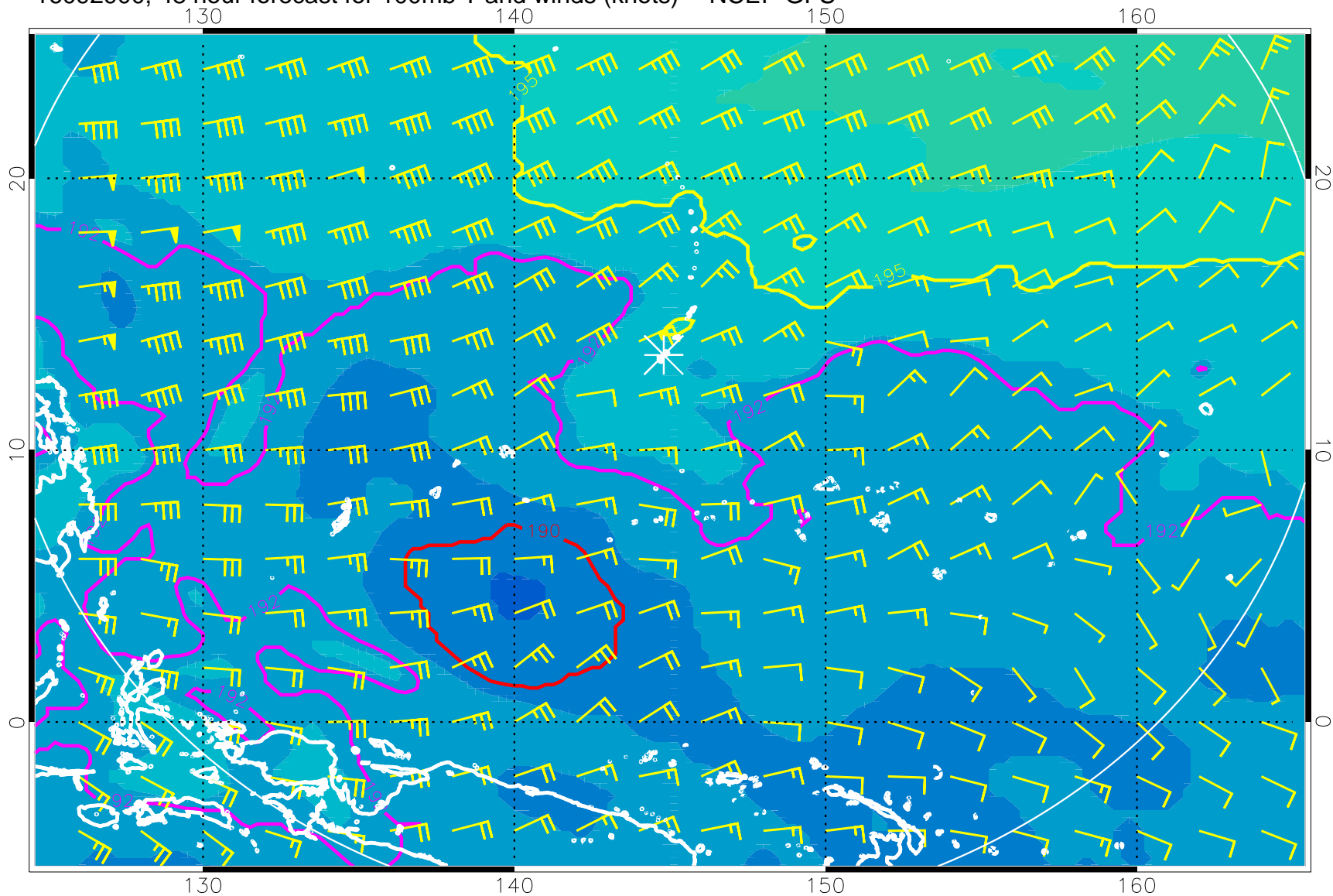
16092900, 48 hour forecast for 100mb T and winds (knots) -- NCEP GFS
