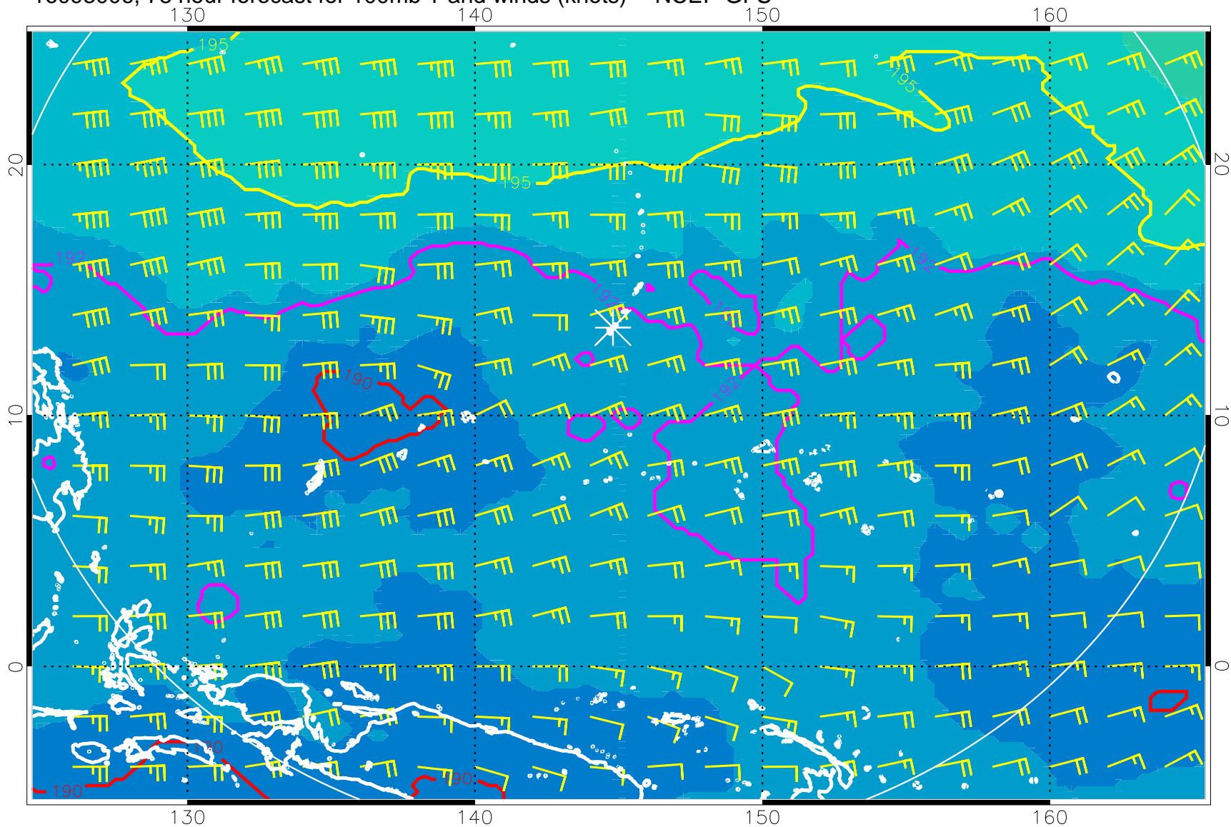
16093006, 78 hour forecast for 100mb T and winds (knots) -- NCEP GFS
