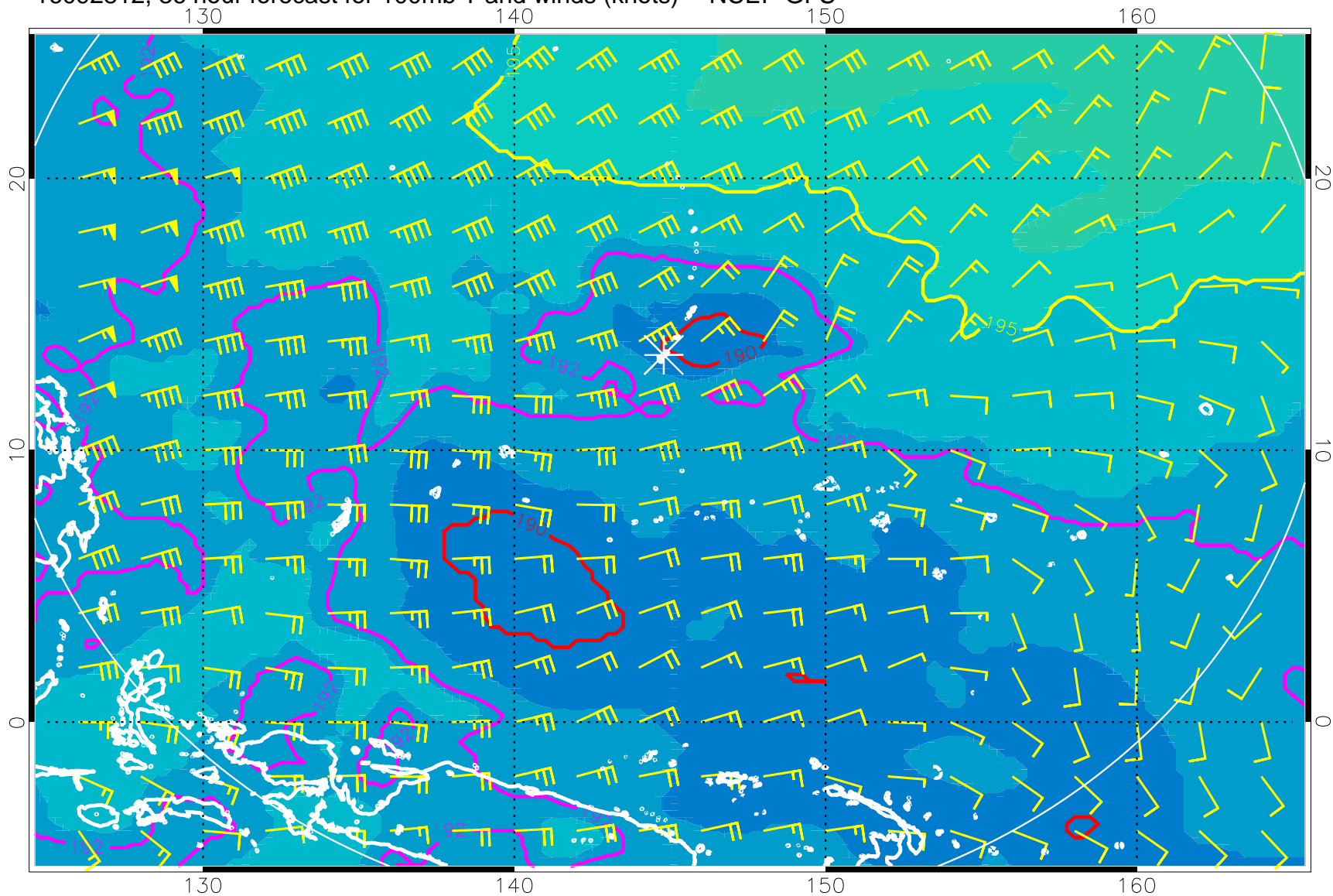
16092812, 36 hour forecast for 100mb T and winds (knots) -- NCEP GFS
