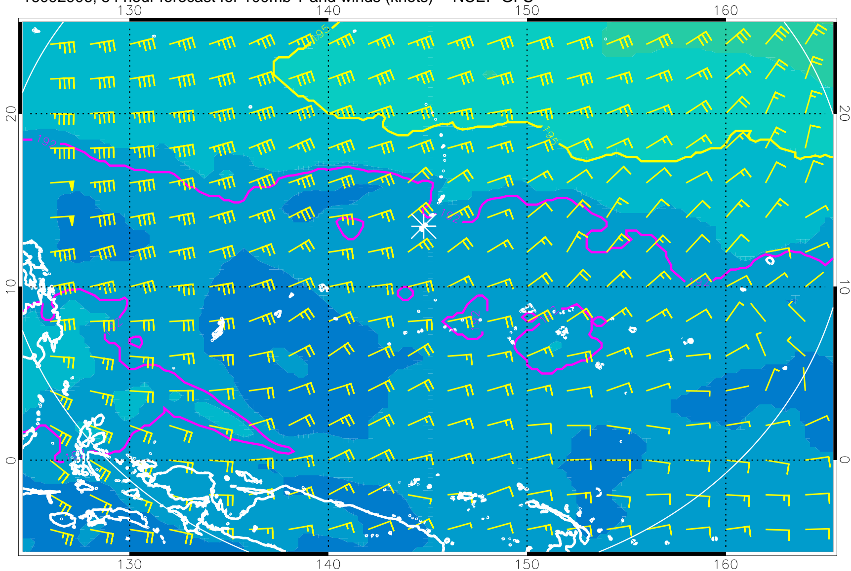
16092906, 54 hour forecast for 100mb T and winds (knots) -- NCEP GFS
