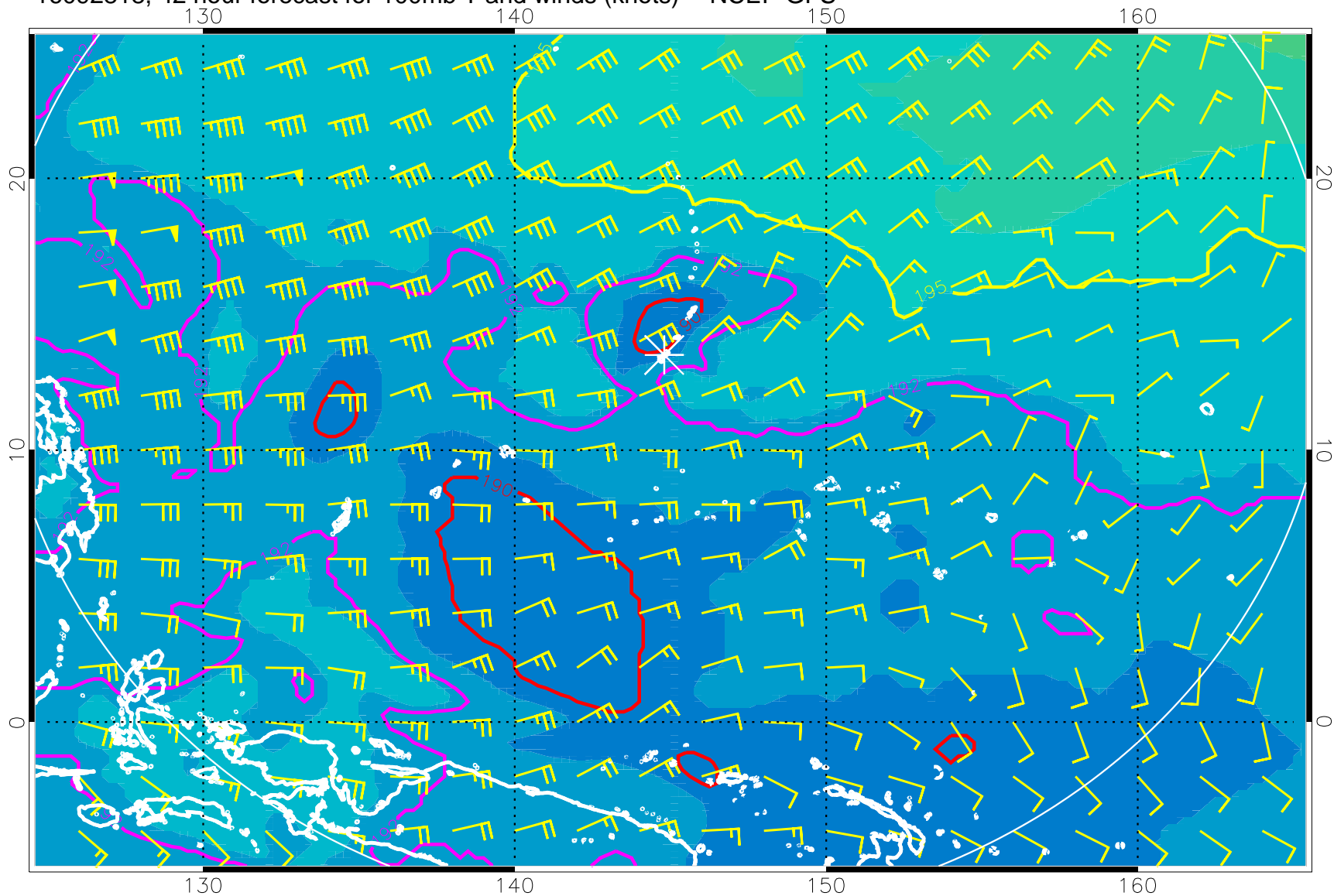
16092818, 42 hour forecast for 100mb T and winds (knots) -- NCEP GFS
