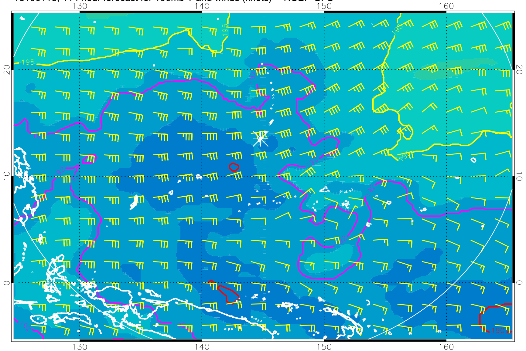
16100118, 114 hour forecast for 100mb T and winds (knots) -- NCEP GFS
