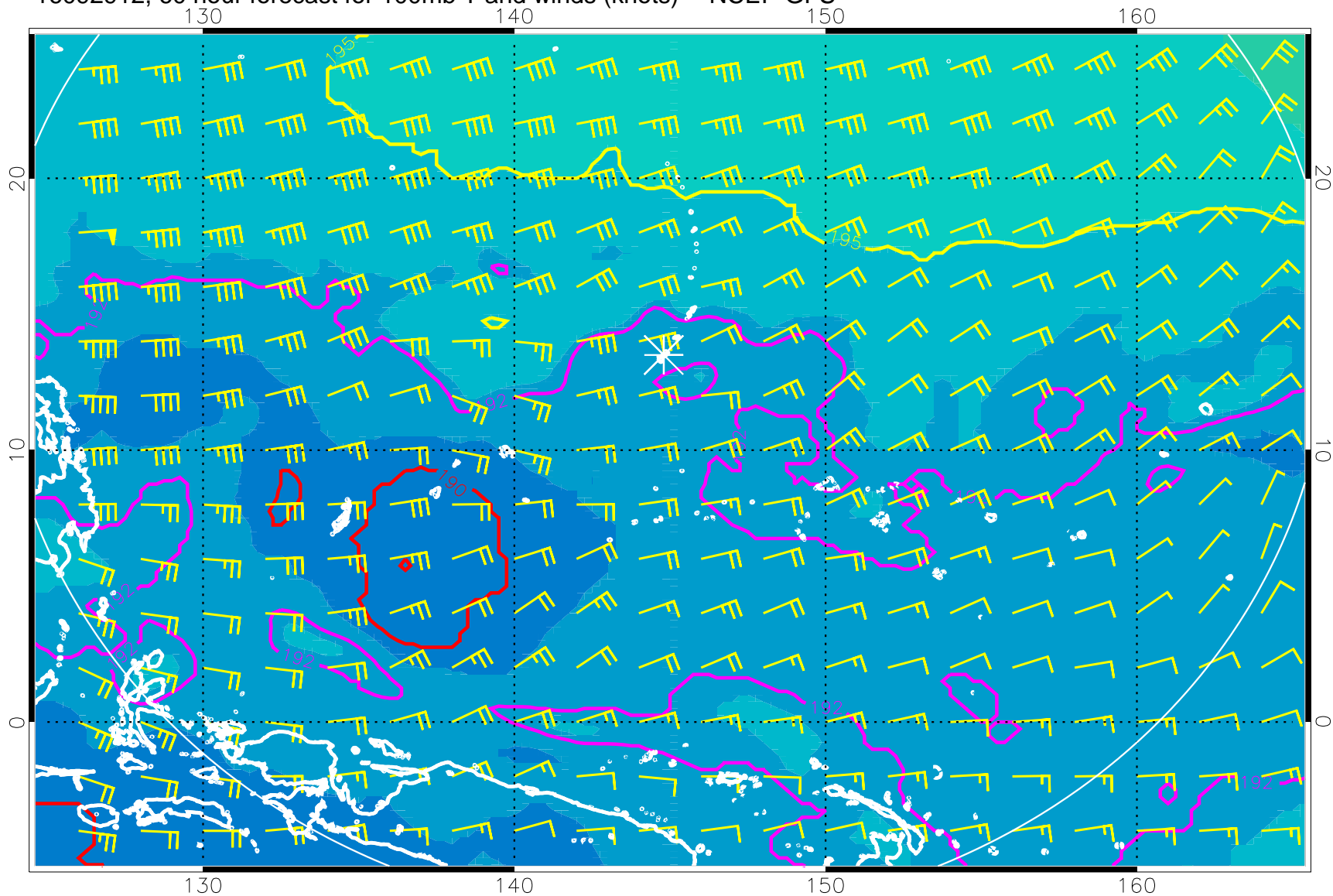
16092912, 60 hour forecast for 100mb T and winds (knots) -- NCEP GFS
