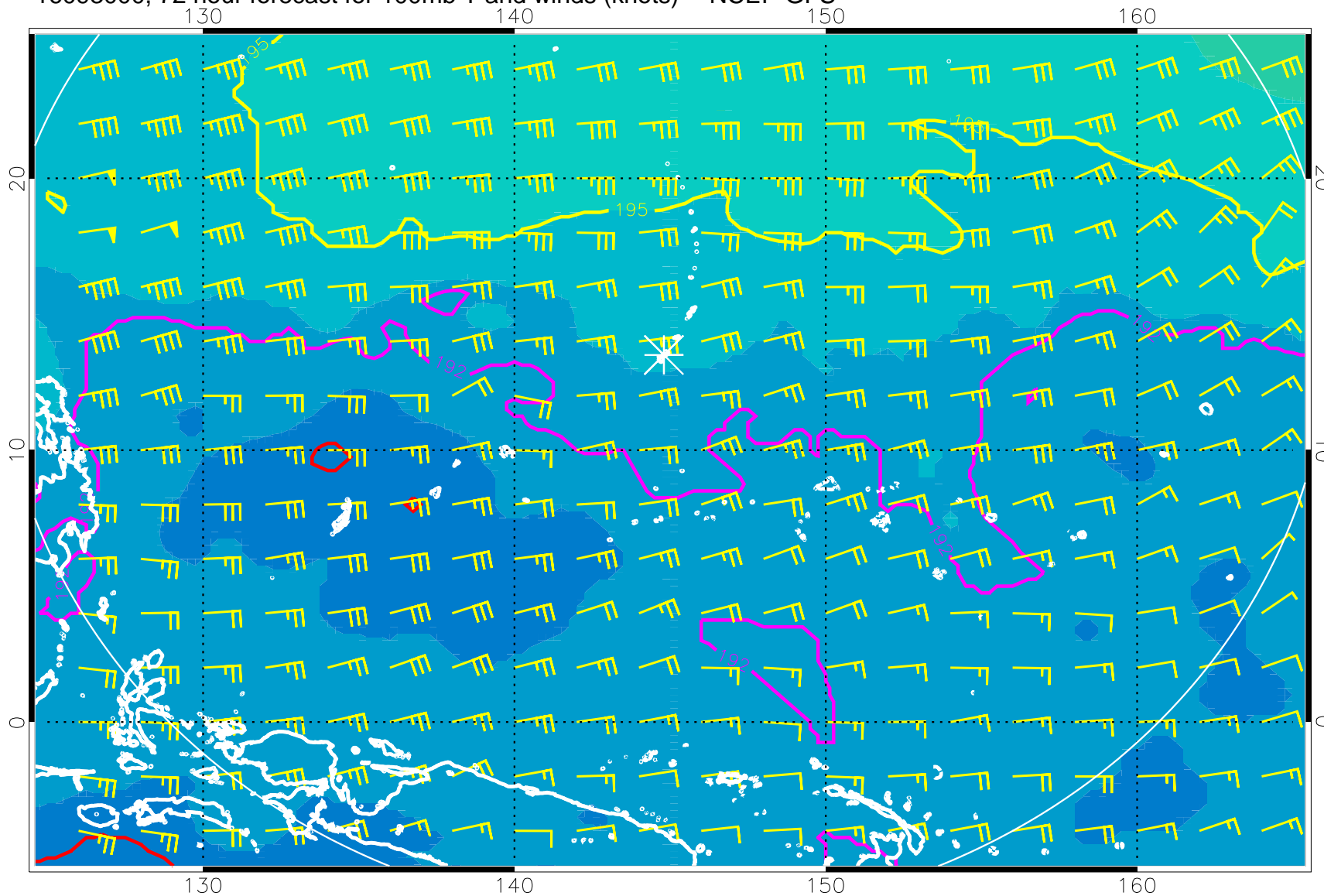
16093000, 72 hour forecast for 100mb T and winds (knots) -- NCEP GFS
