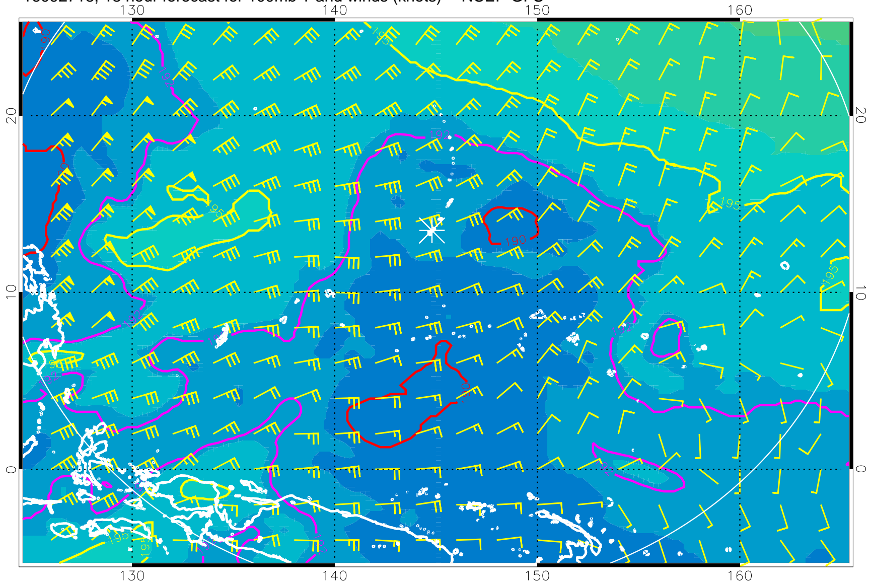
16092718, 18 hour forecast for 100mb T and winds (knots) -- NCEP GFS
