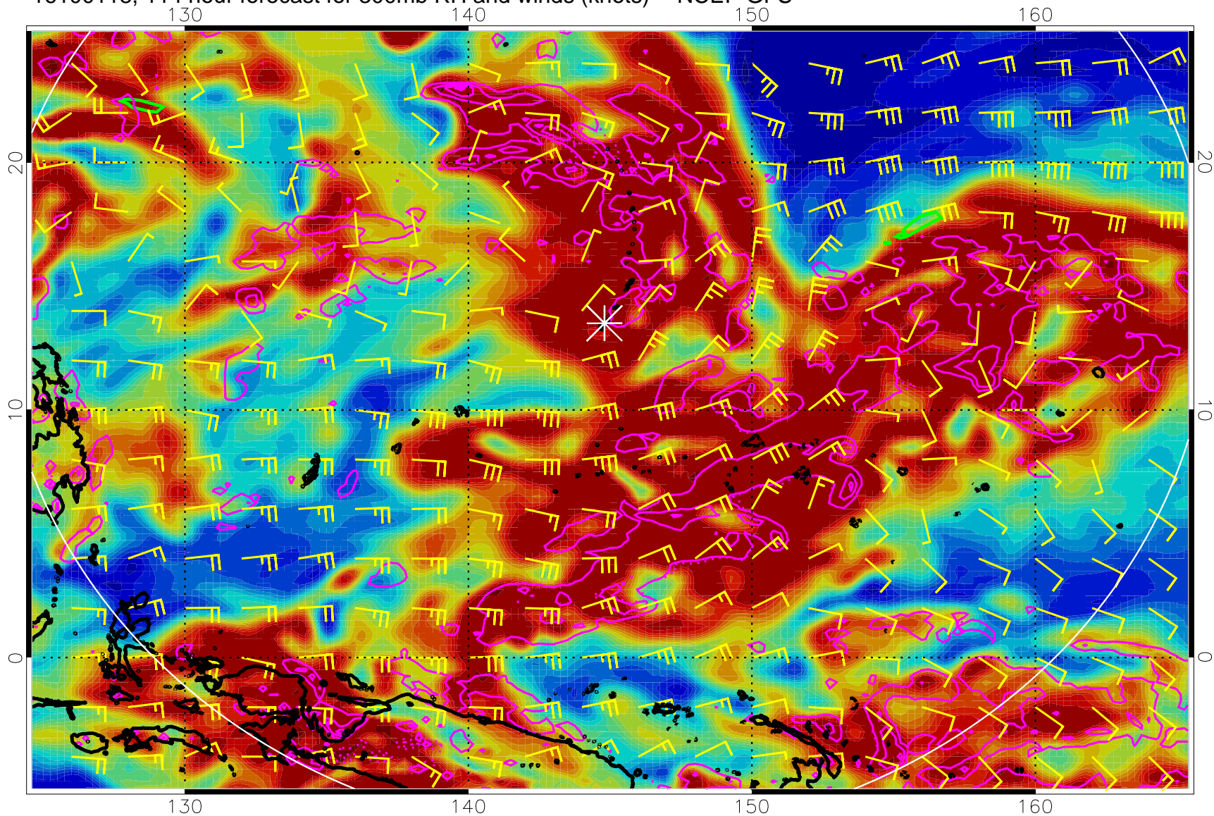
16100118, 114 hour forecast for 300mb RH and winds (knots) -- NCEP GFS
