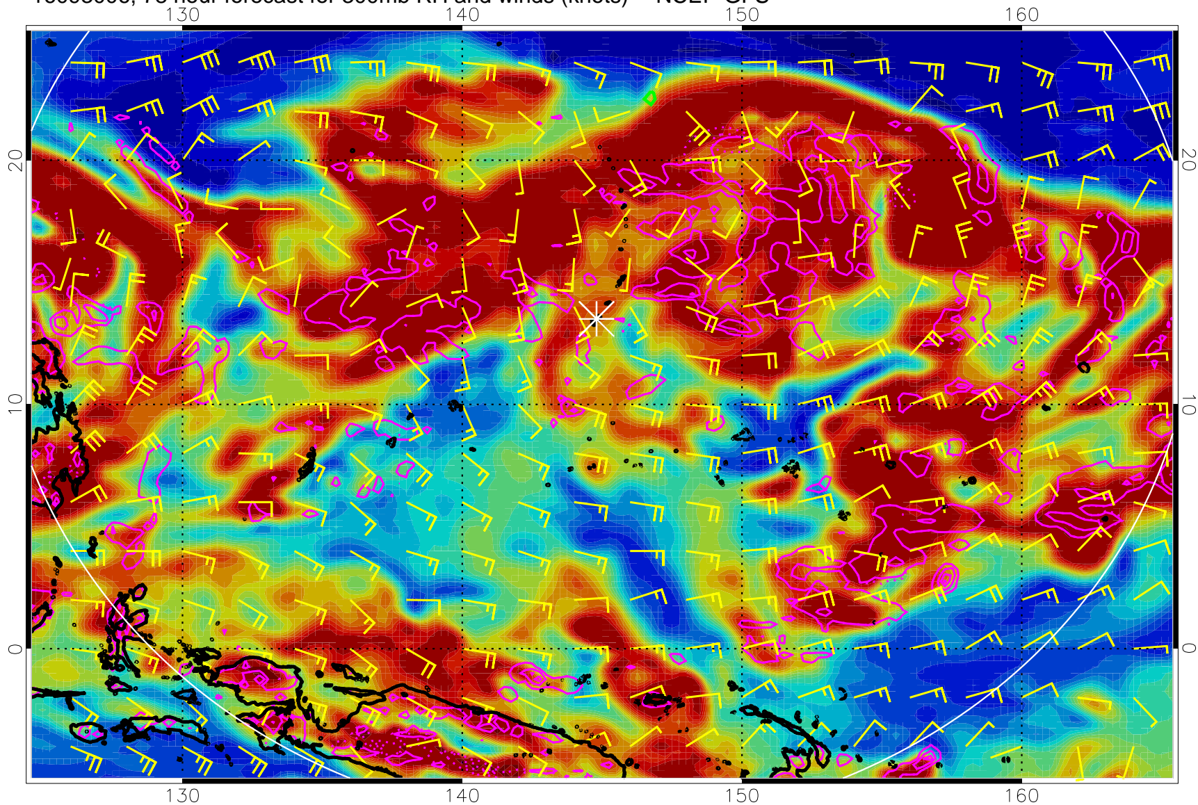
16093006, 78 hour forecast for 300mb RH and winds (knots) -- NCEP GFS
