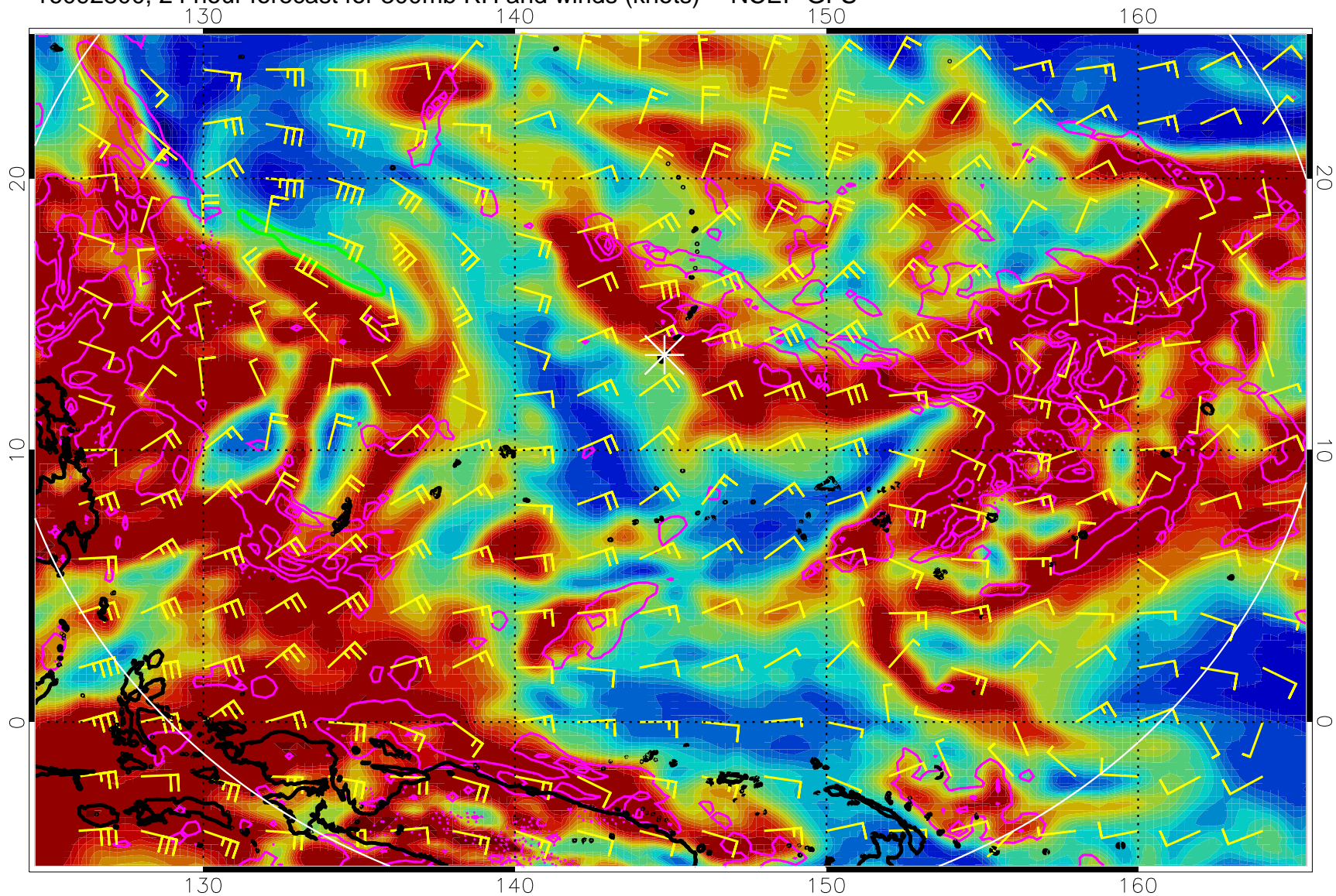
16092800, 24 hour forecast for 300mb RH and winds (knots) -- NCEP GFS
