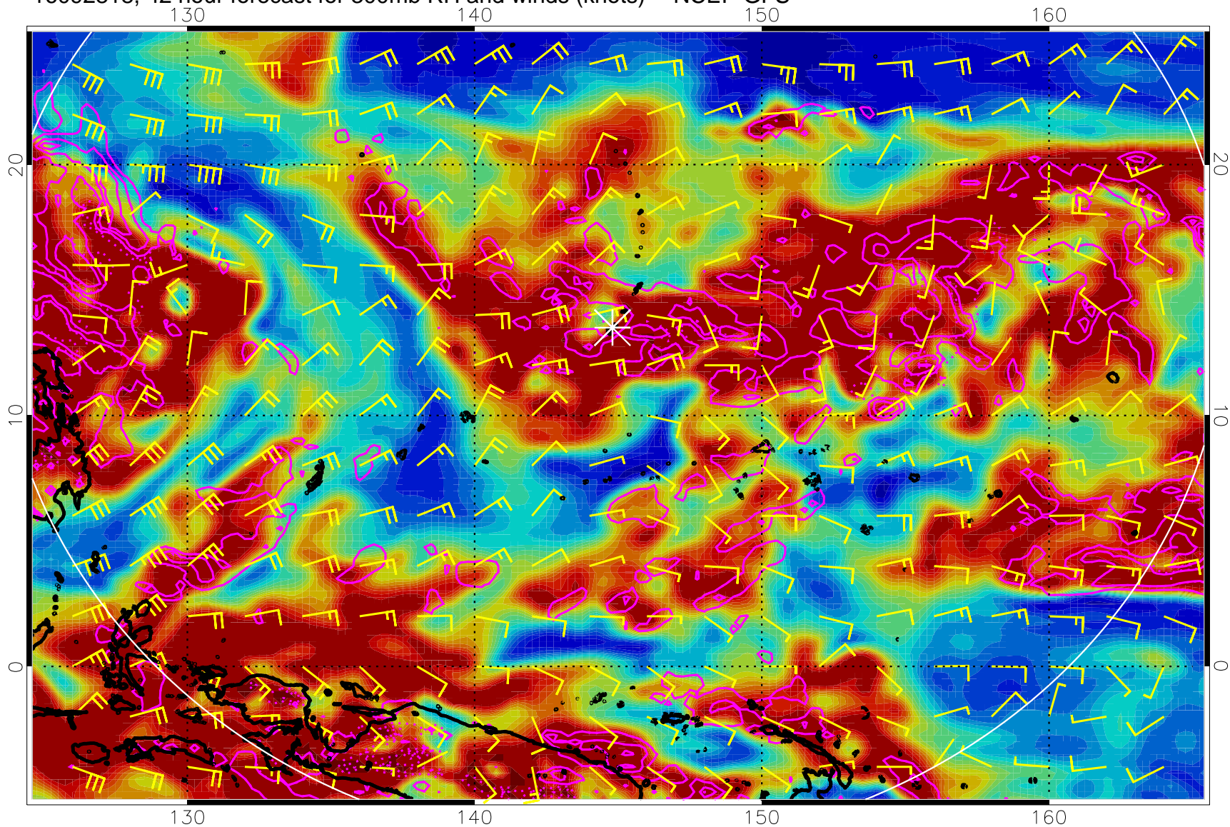
16092818, 42 hour forecast for 300mb RH and winds (knots) -- NCEP GFS
