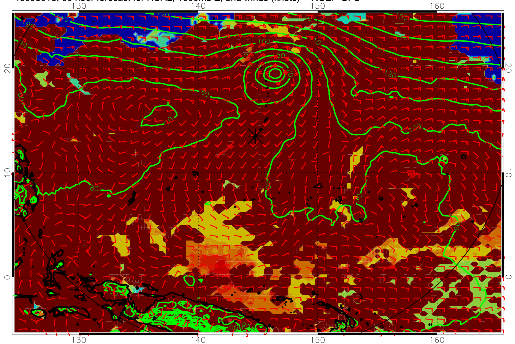
16093018, 90 hour forecast for HCAL, 1000mb Z, and winds (knots) -- NCEP GFS
