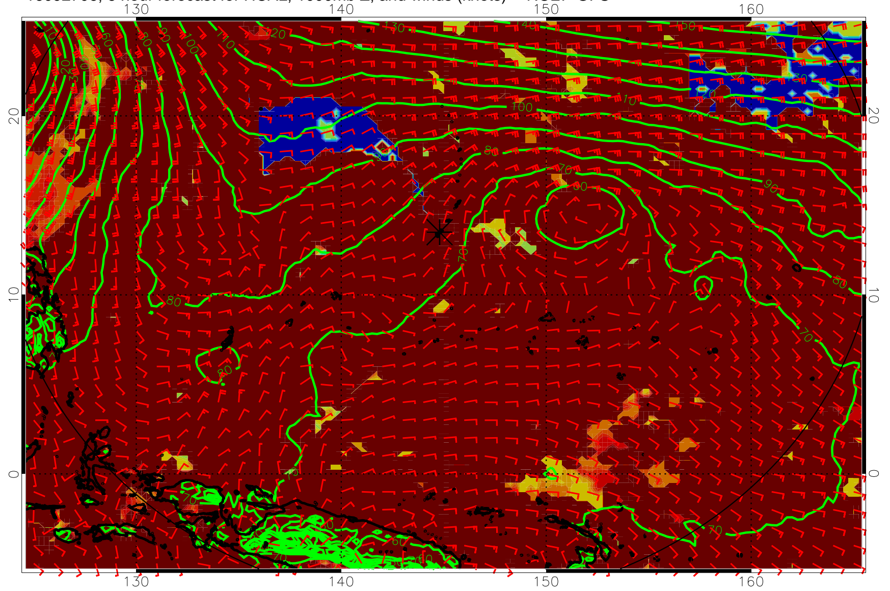
16092706, 6 hour forecast for HCAL, 1000mb Z, and winds (knots) -- NCEP GFS
