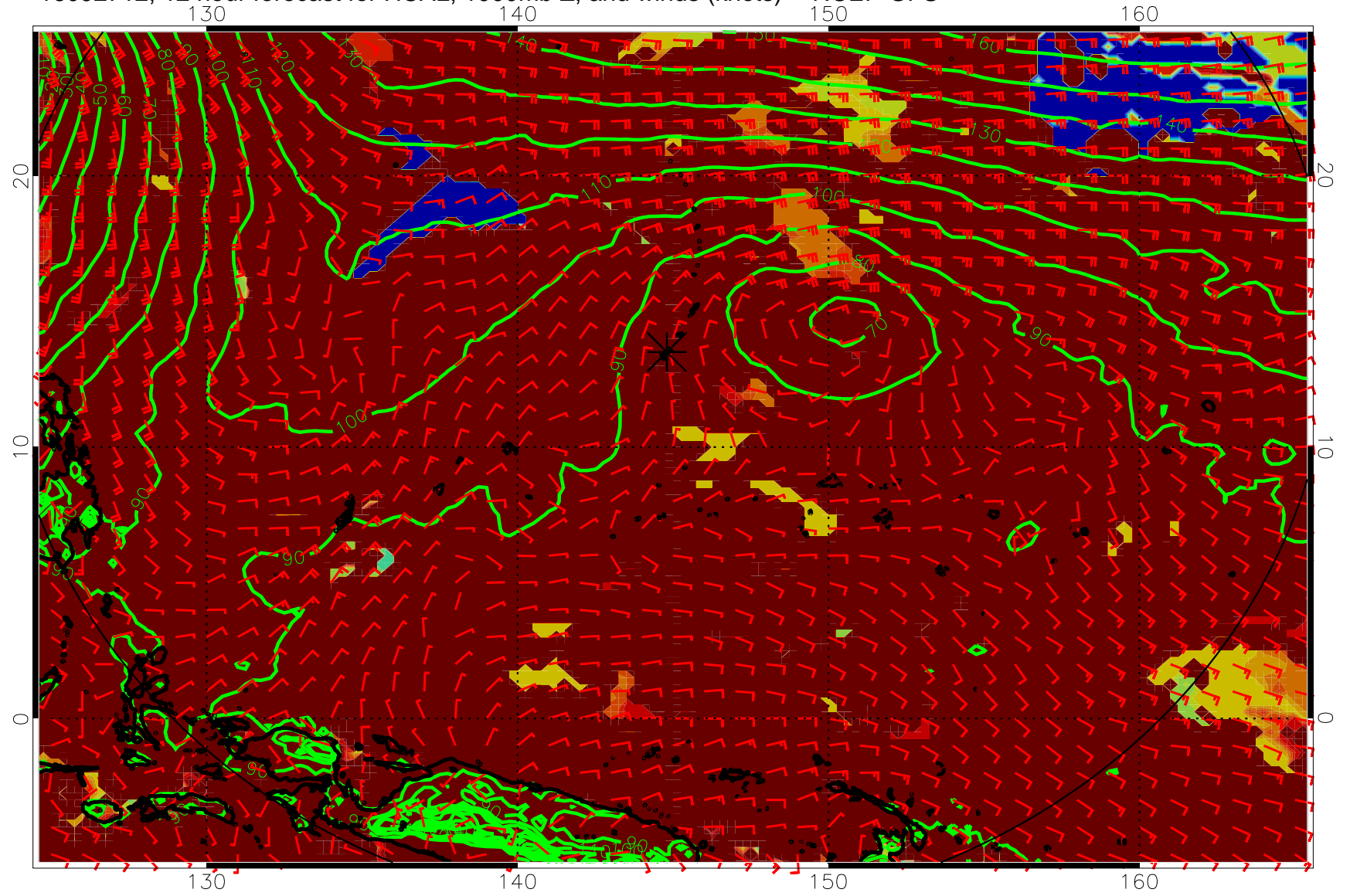
16092712, 12 hour forecast for HCAL, 1000mb Z, and winds (knots) -- NCEP GFS
