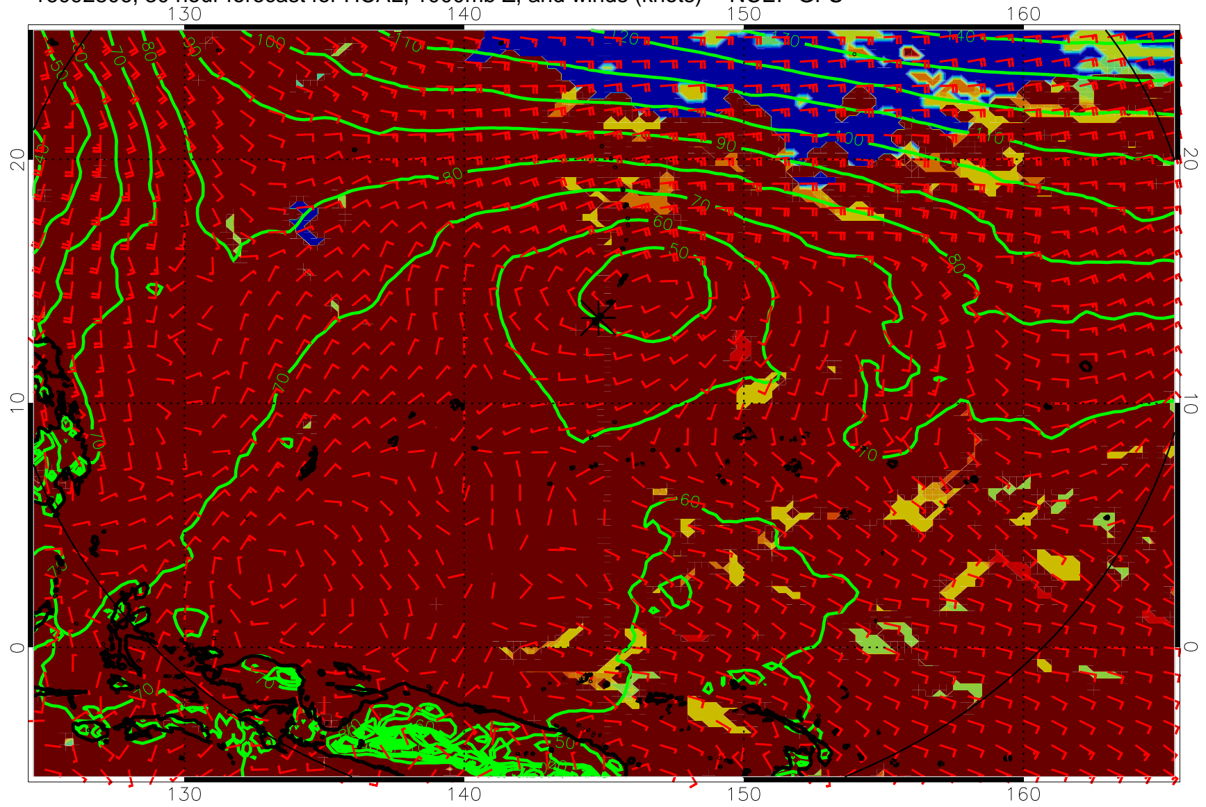
16092806, 30 hour forecast for HCAL, 1000mb Z, and winds (knots) -- NCEP GFS
