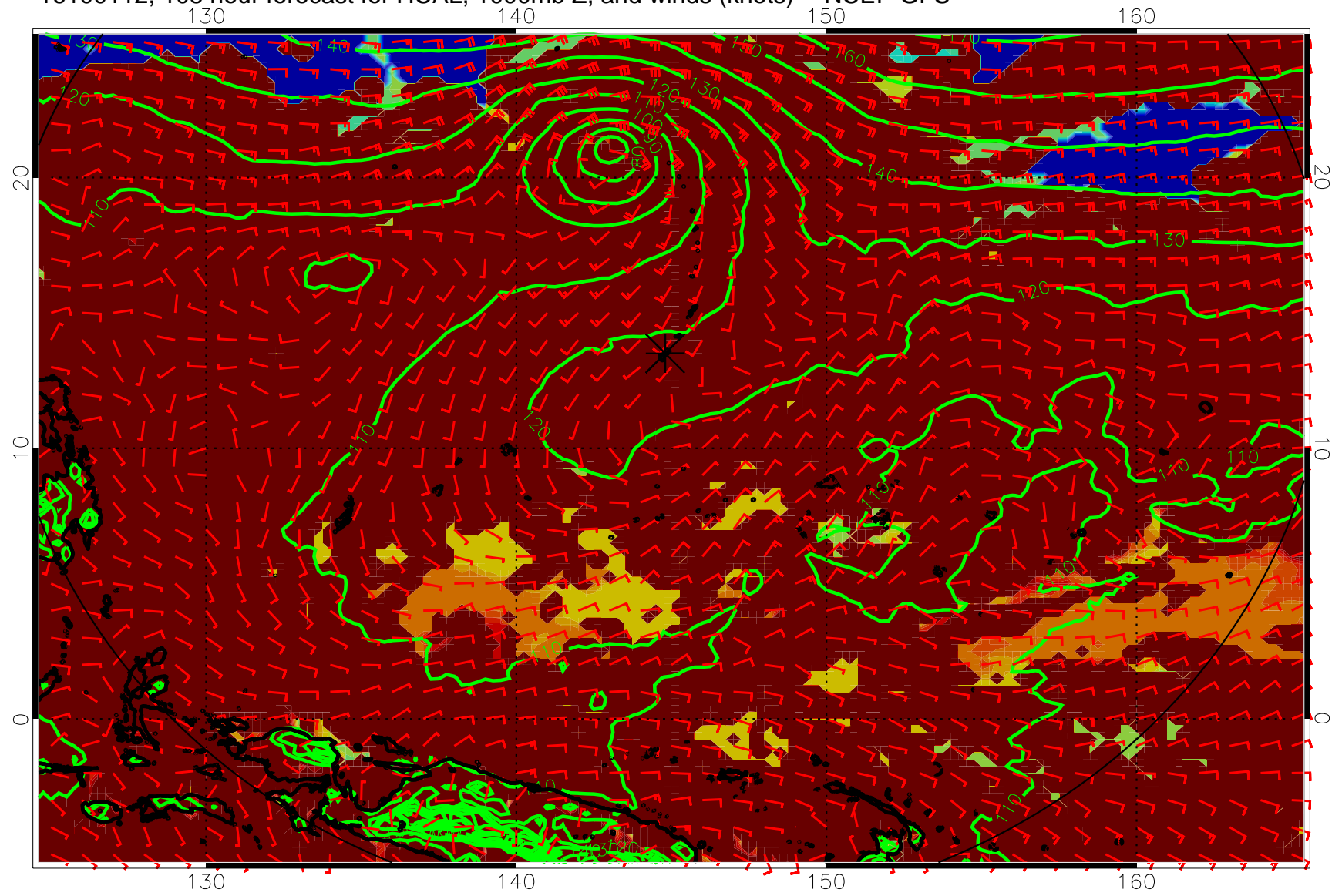
16100112, 108 hour forecast for HCAL, 1000mb Z, and winds (knots) -- NCEP GFS
