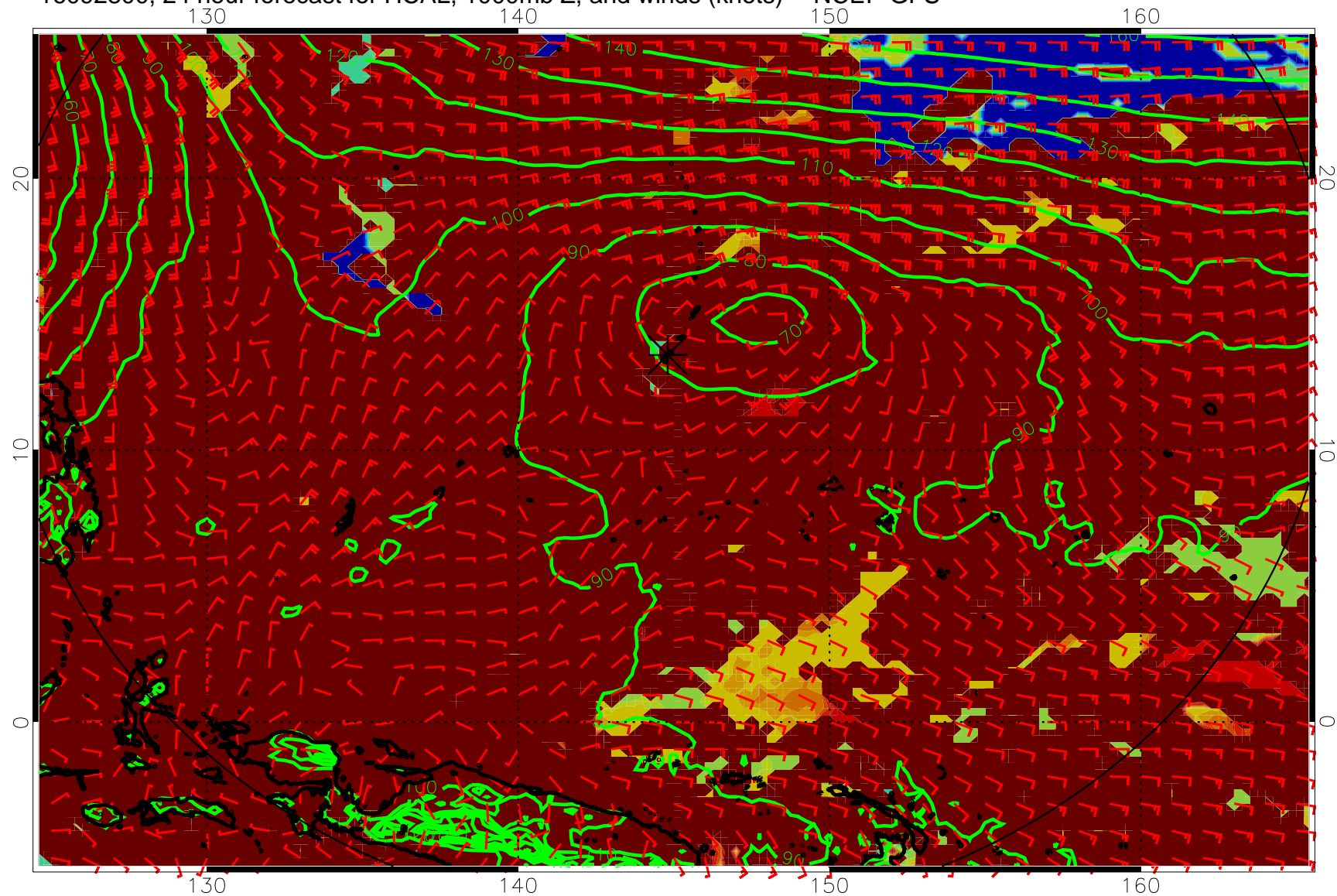
16092800, 24 hour forecast for HCAL, 1000mb Z, and winds (knots) -- NCEP GFS
