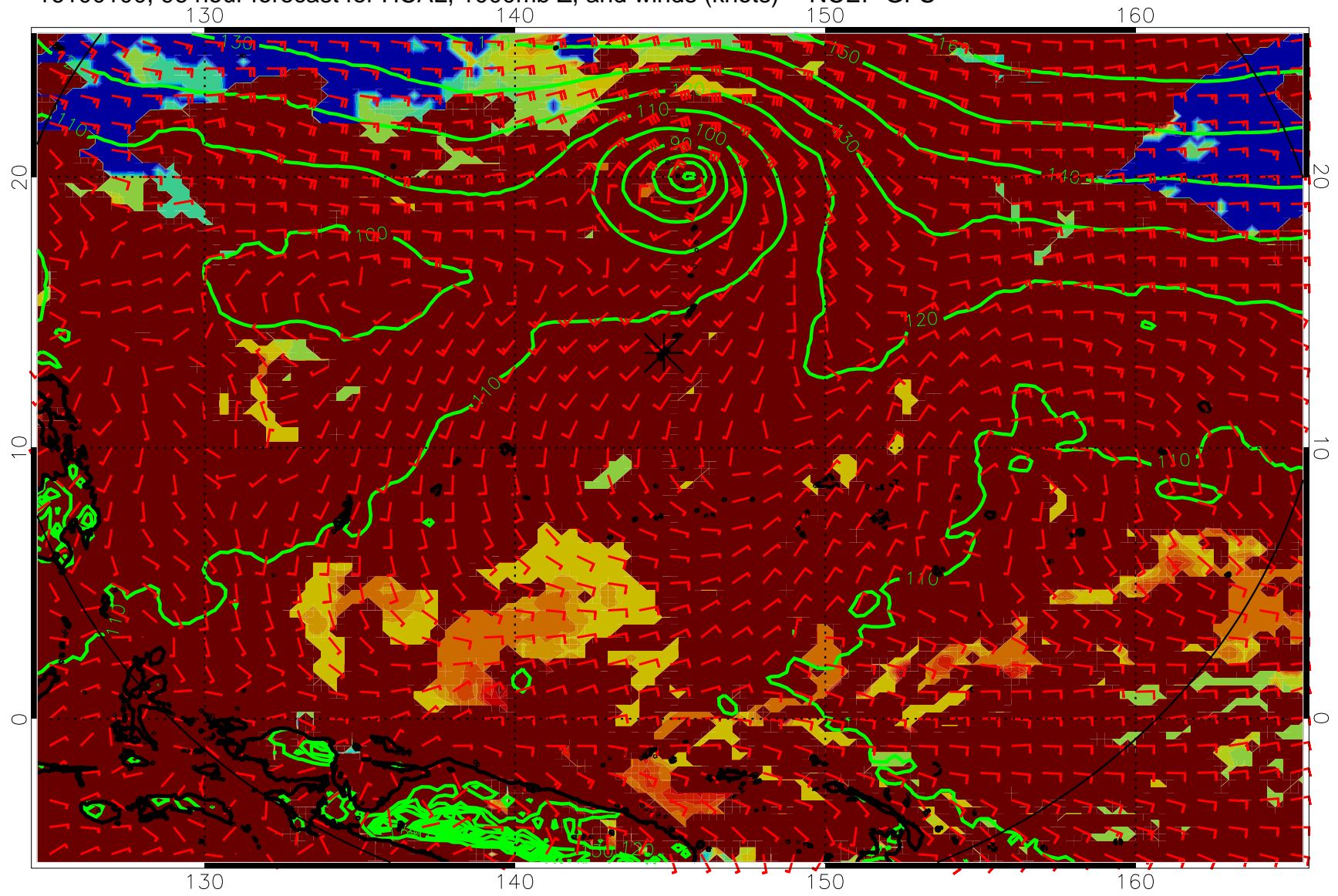
16100100, 96 hour forecast for HCAL, 1000mb Z, and winds (knots) -- NCEP GFS
