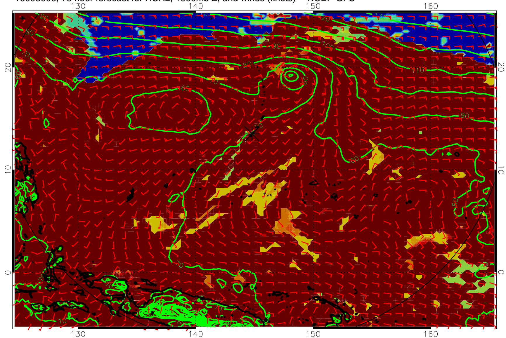
16093006, 78 hour forecast for HCAL, 1000mb Z, and winds (knots) -- NCEP GFS
