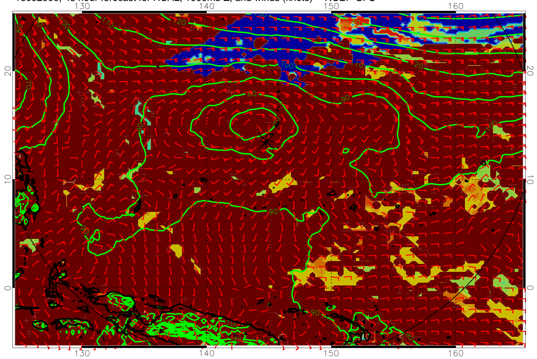
16092900, 48 hour forecast for HCAL, 1000mb Z, and winds (knots) -- NCEP GFS
