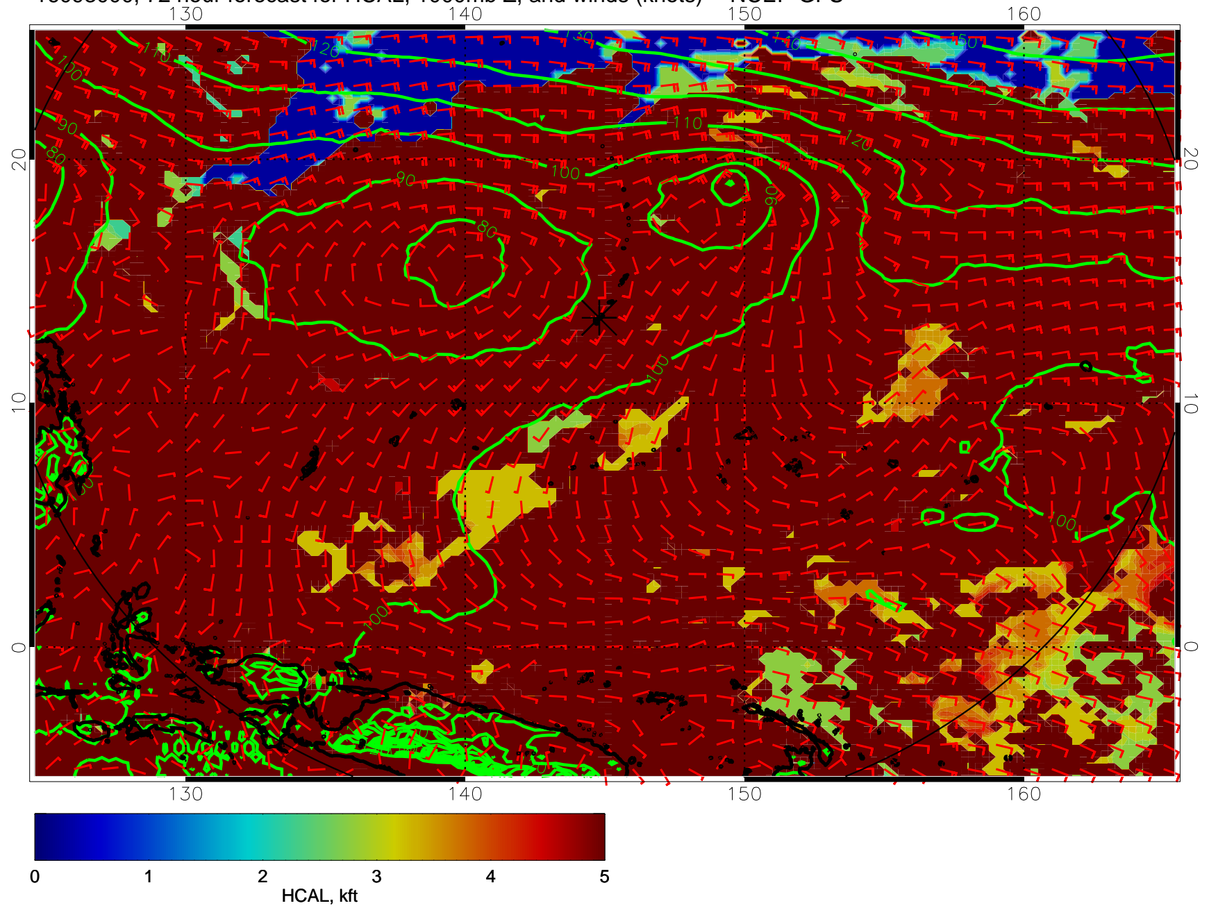
16093000, 72 hour forecast for HCAL, 1000mb Z, and winds (knots) -- NCEP GFS
