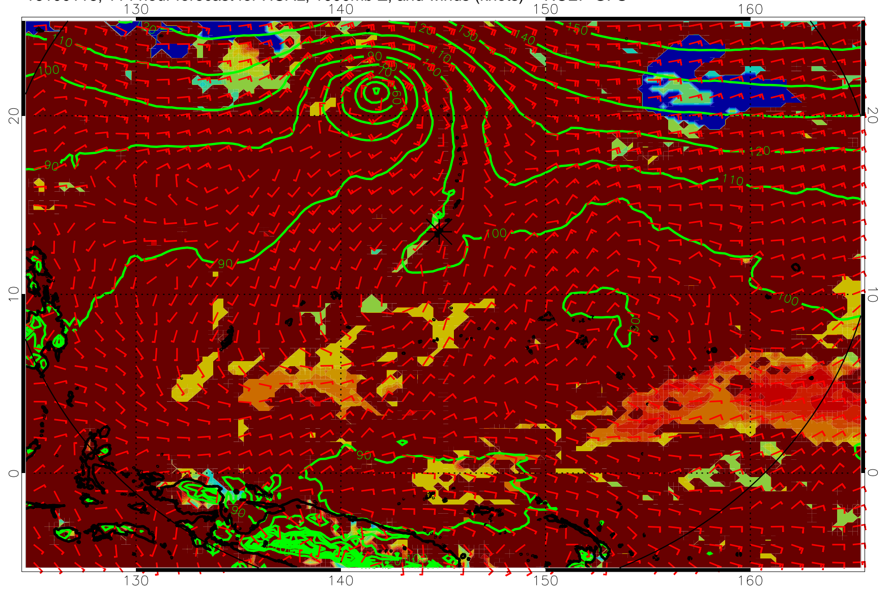
16100118, 114 hour forecast for HCAL, 1000mb Z, and winds (knots) -- NCEP GFS
