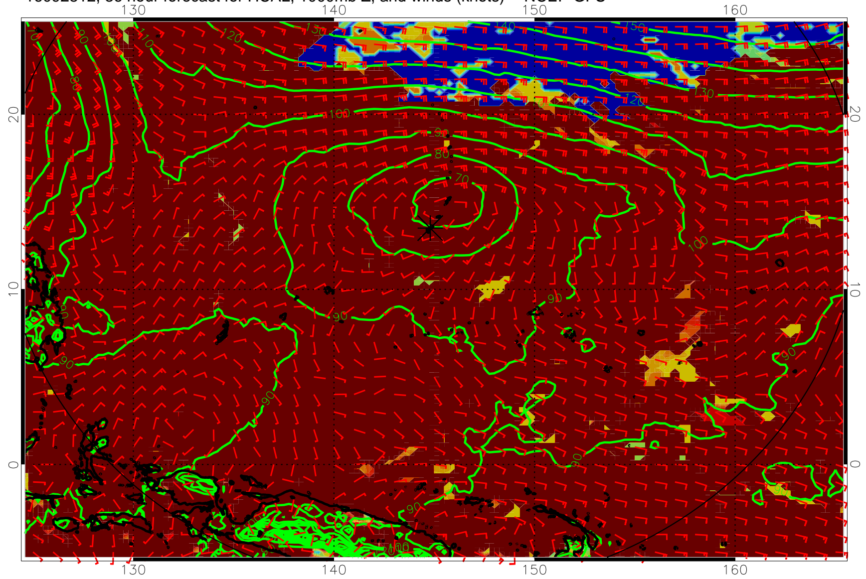
16092812, 36 hour forecast for HCAL, 1000mb Z, and winds (knots) -- NCEP GFS
