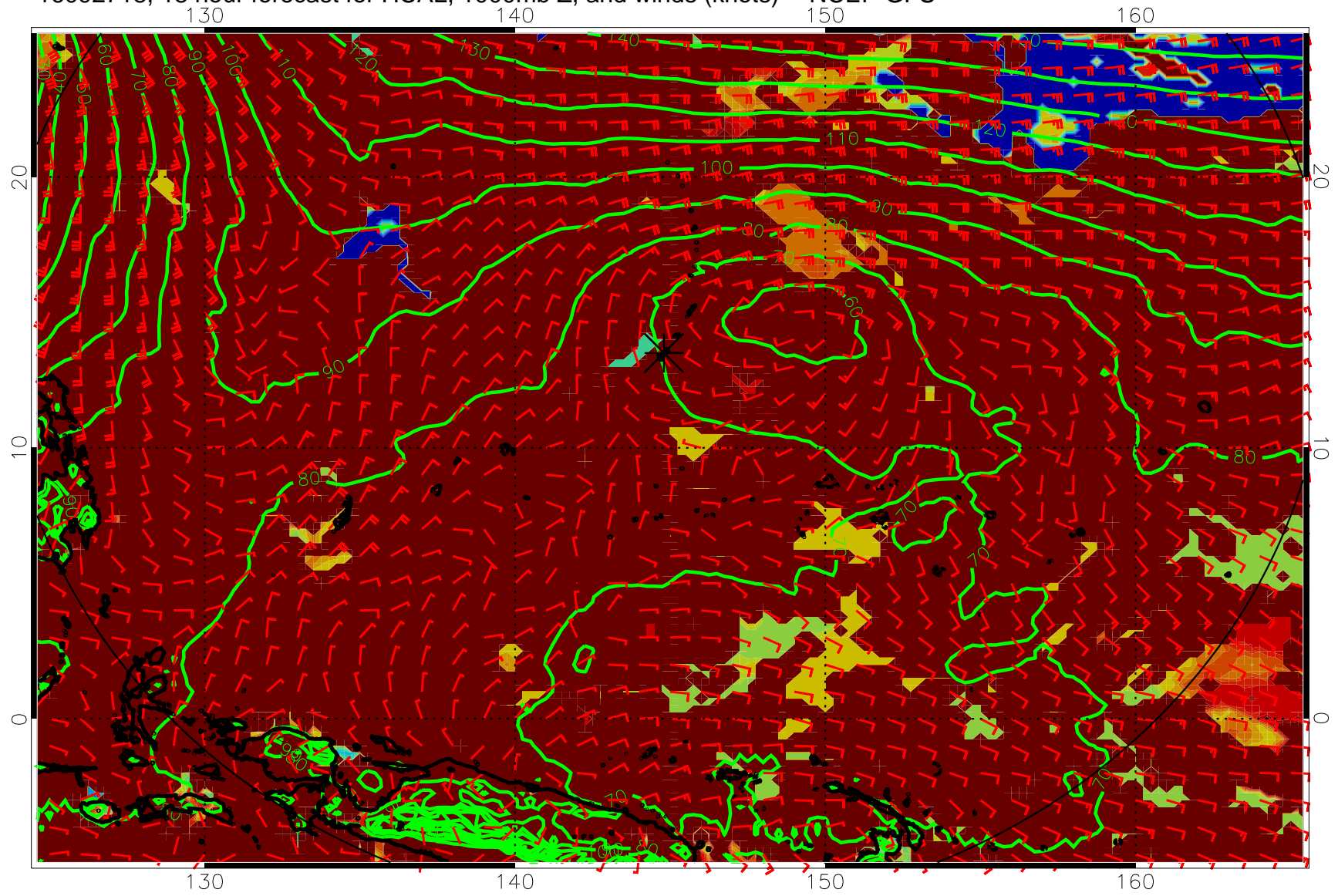
16092718, 18 hour forecast for HCAL, 1000mb Z, and winds (knots) -- NCEP GFS
