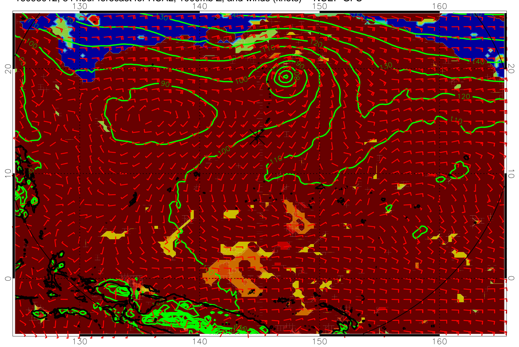
16093012, 84 hour forecast for HCAL, 1000mb Z, and winds (knots) -- NCEP GFS
