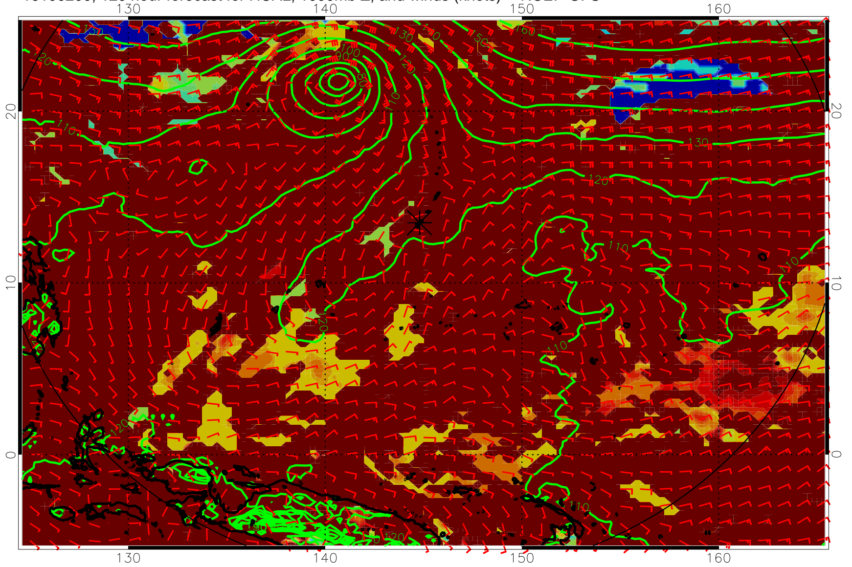
16100200, 120 hour forecast for HCAL, 1000mb Z, and winds (knots) -- NCEP GFS
