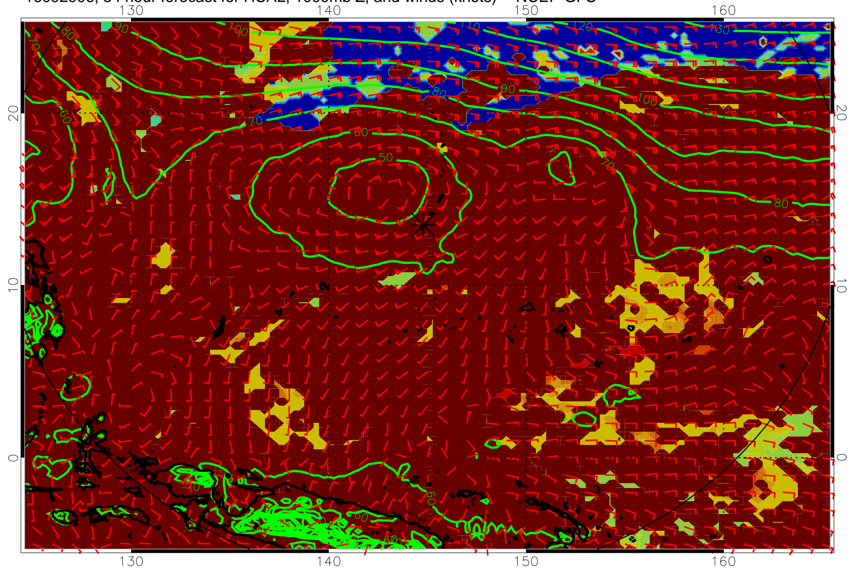
16092906, 54 hour forecast for HCAL, 1000mb Z, and winds (knots) -- NCEP GFS
