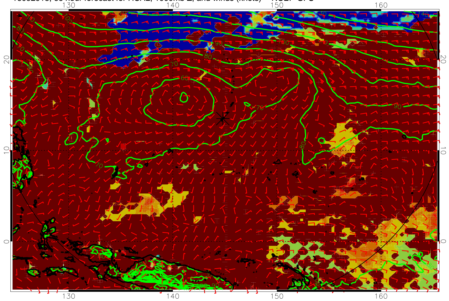
16092918, 66 hour forecast for HCAL, 1000mb Z, and winds (knots) -- NCEP GFS
