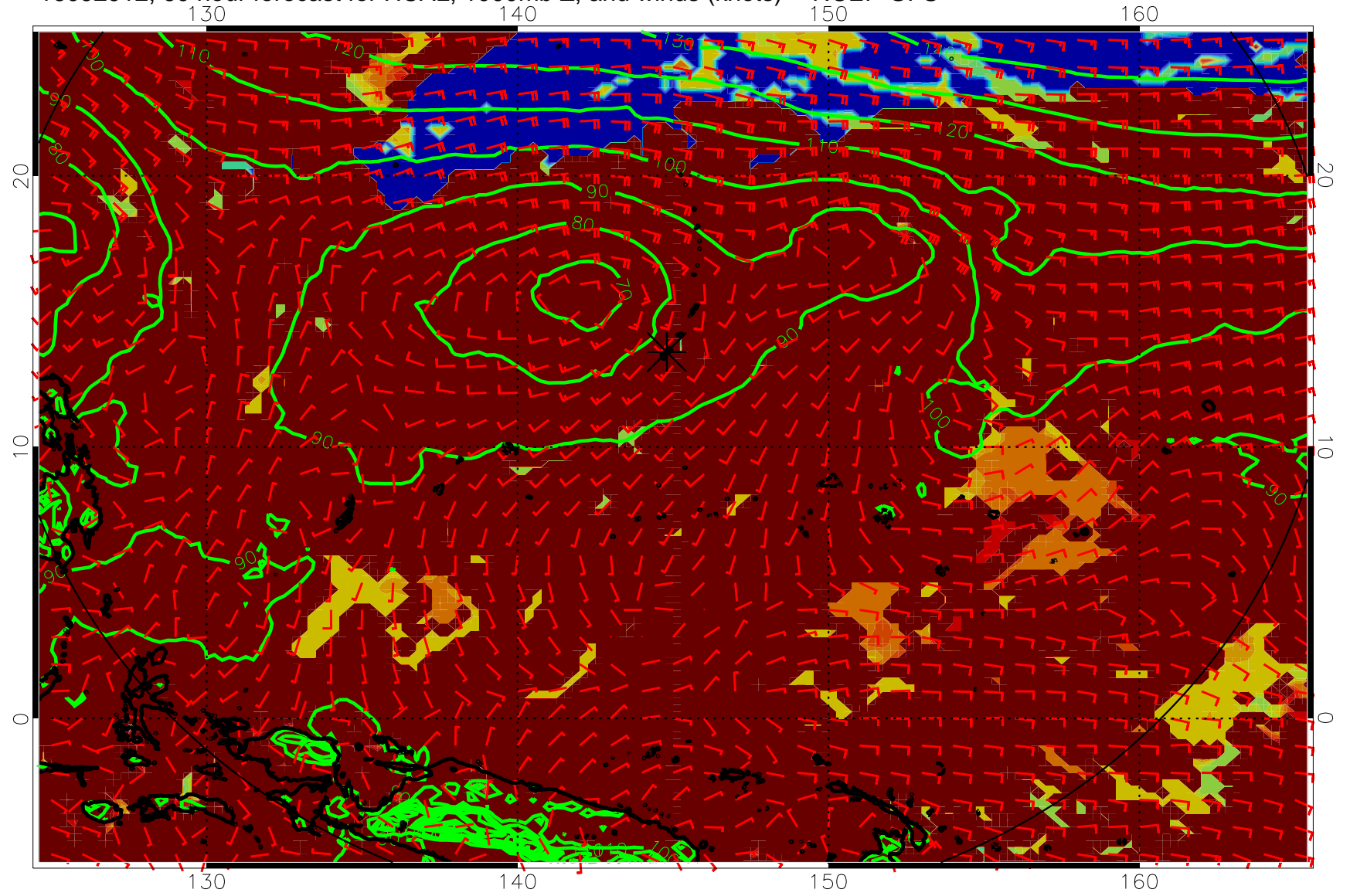
16092912, 60 hour forecast for HCAL, 1000mb Z, and winds (knots) -- NCEP GFS
