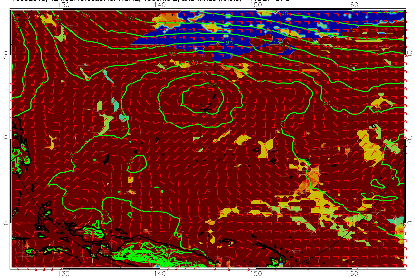
16092818, 42 hour forecast for HCAL, 1000mb Z, and winds (knots) -- NCEP GFS
