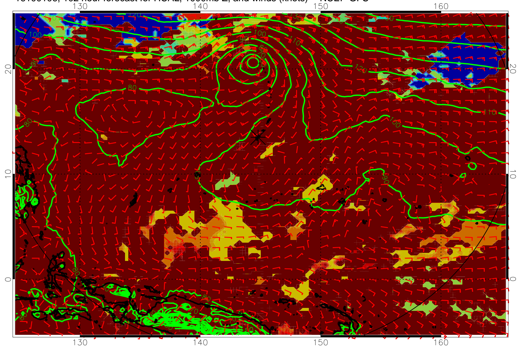
16100106, 102 hour forecast for HCAL, 1000mb Z, and winds (knots) -- NCEP GFS
