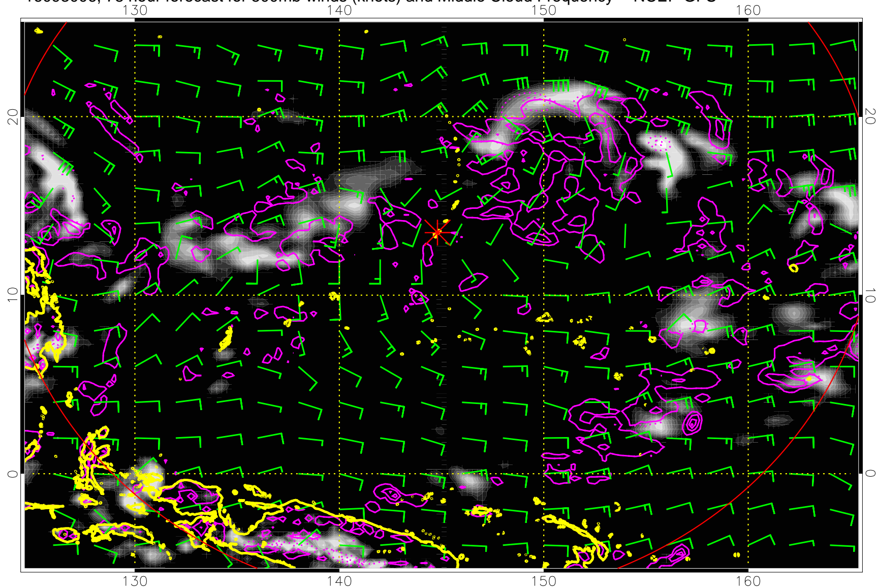
16093006, 78 hour forecast for 500mb winds (knots) and Middle Cloud Frequency -- NCEP GFS
