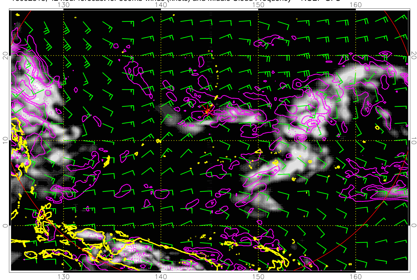
16092818, 42 hour forecast for 500mb winds (knots) and Middle Cloud Frequency -- NCEP GFS
