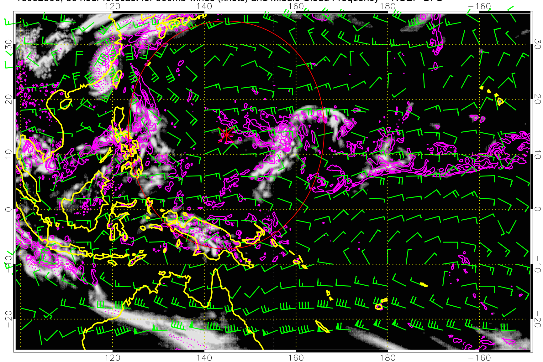
16092806, 30 hour forecast for 500mb winds (knots) and Middle Cloud Frequency -- NCEP GFS
