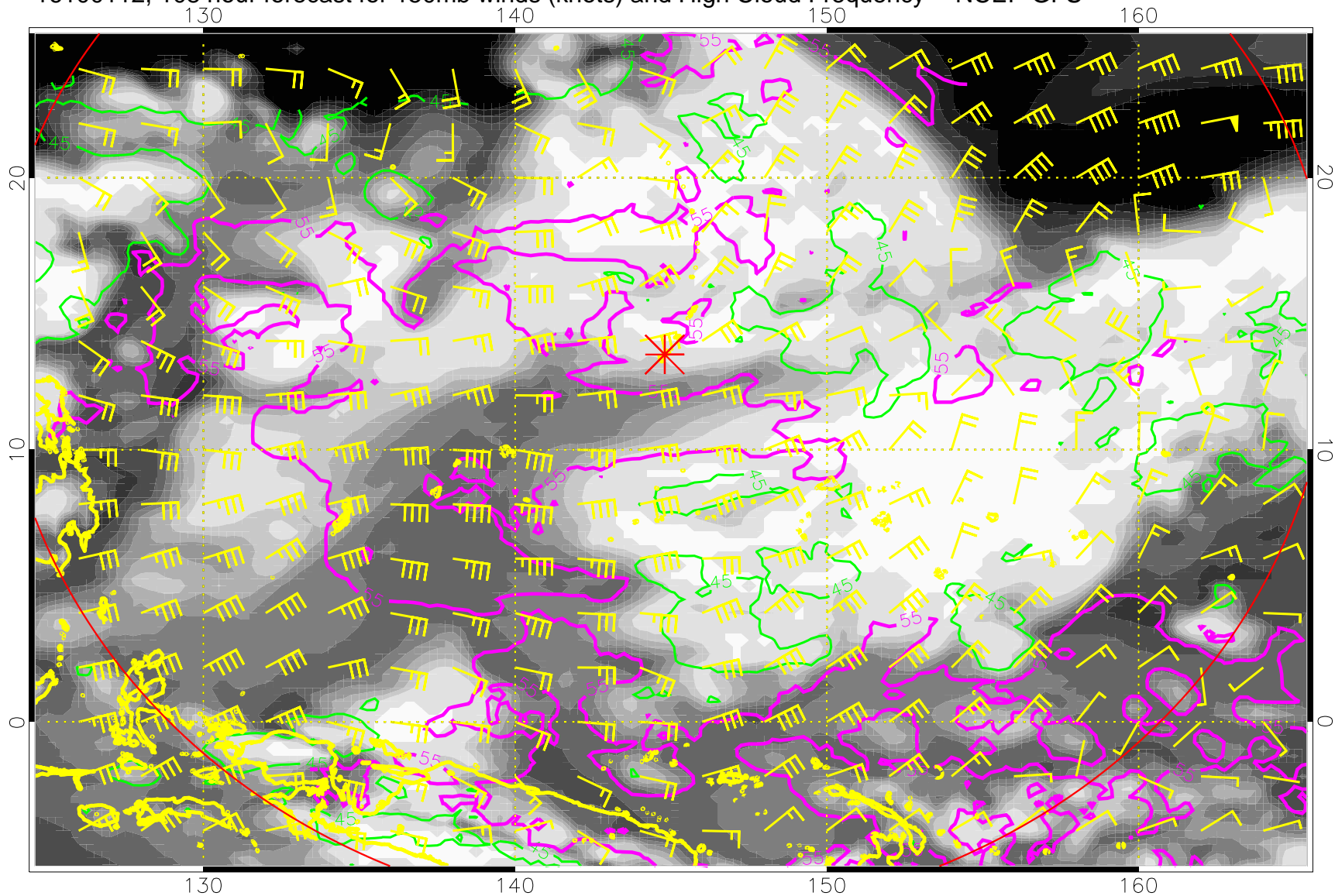
16100112, 108 hour forecast for 150mb winds (knots) and High Cloud Frequency -- NCEP GFS
