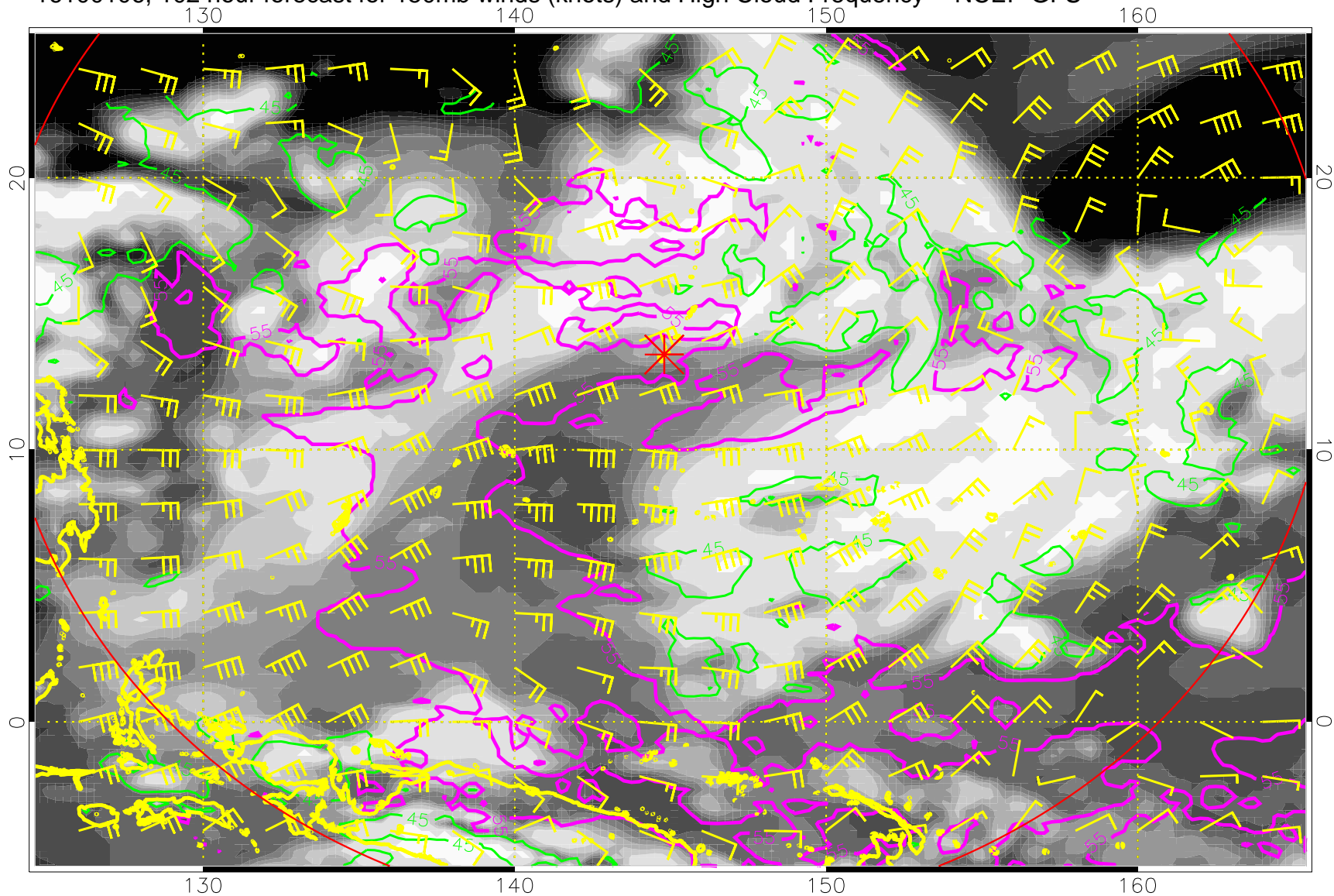
16100106, 102 hour forecast for 150mb winds (knots) and High Cloud Frequency -- NCEP GFS
