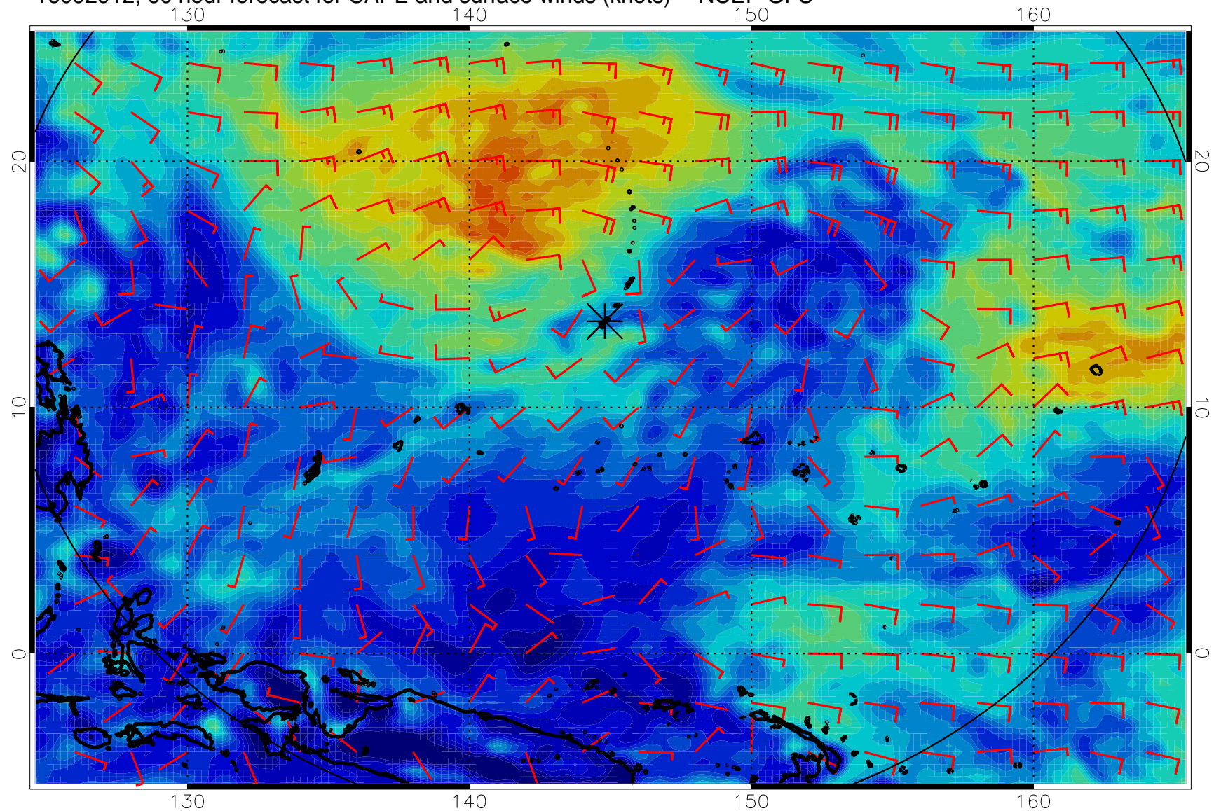
16092912, 60 hour forecast for CAPE and surface winds (knots) -- NCEP GFS
