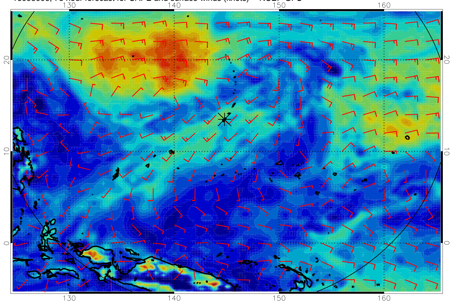
16093006, 78 hour forecast for CAPE and surface winds (knots) -- NCEP GFS
