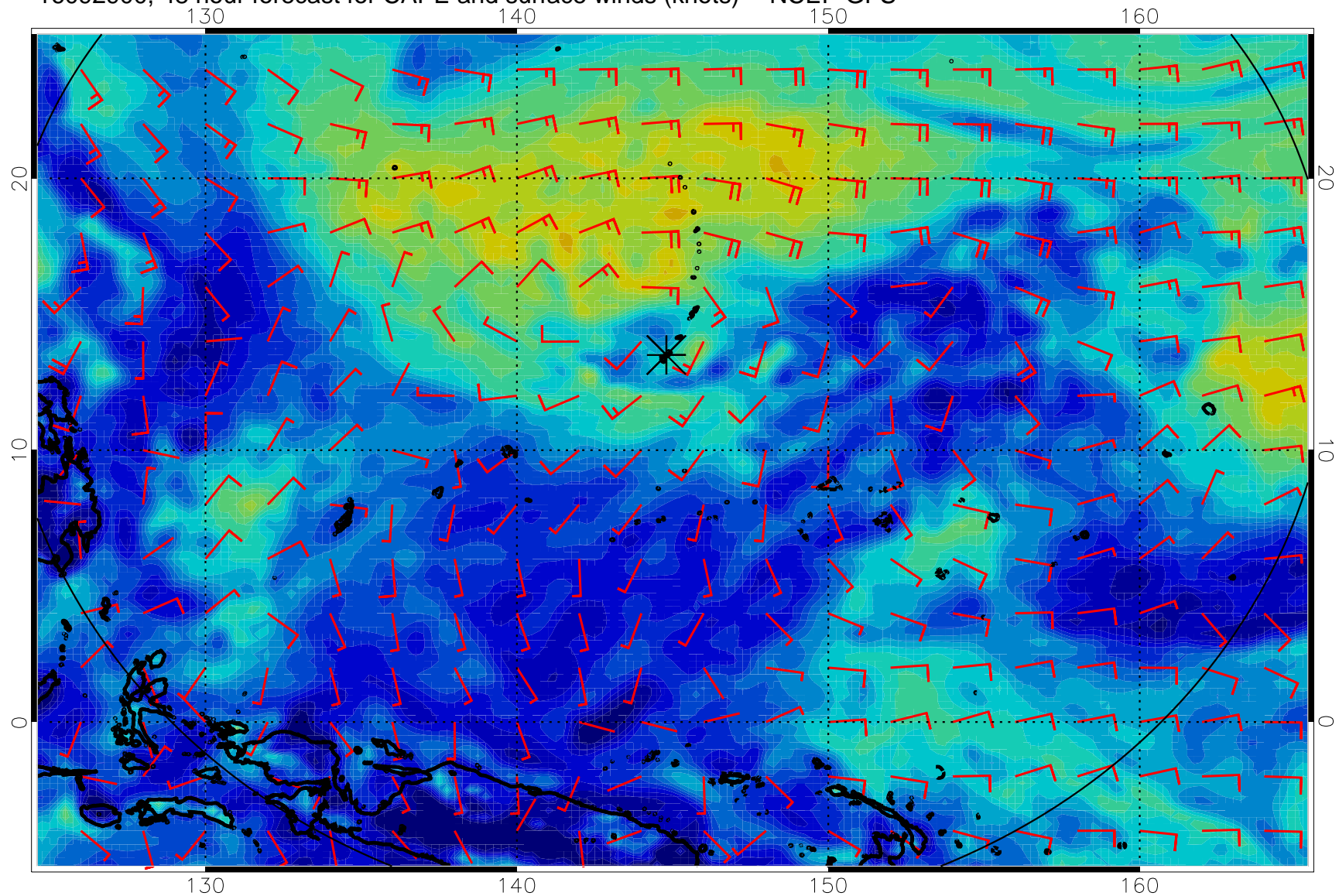
16092900, 48 hour forecast for CAPE and surface winds (knots) -- NCEP GFS
