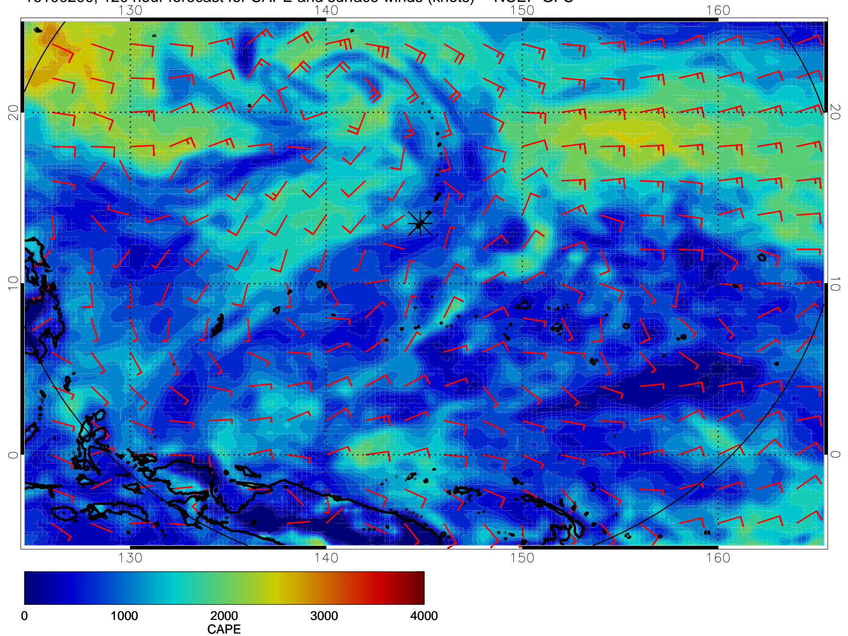
16100200, 120 hour forecast for CAPE and surface winds (knots) -- NCEP GFS
