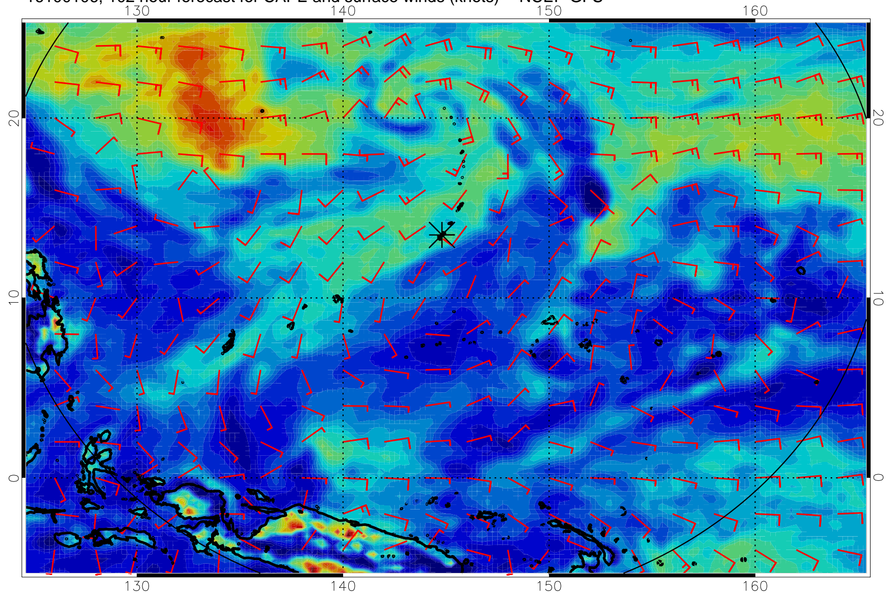
16100106, 102 hour forecast for CAPE and surface winds (knots) -- NCEP GFS
