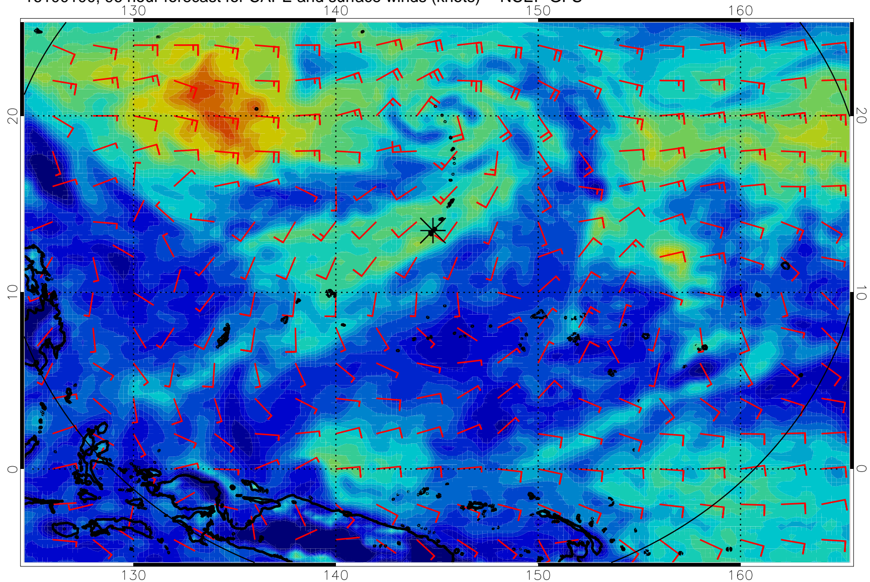
16100100, 96 hour forecast for CAPE and surface winds (knots) -- NCEP GFS
