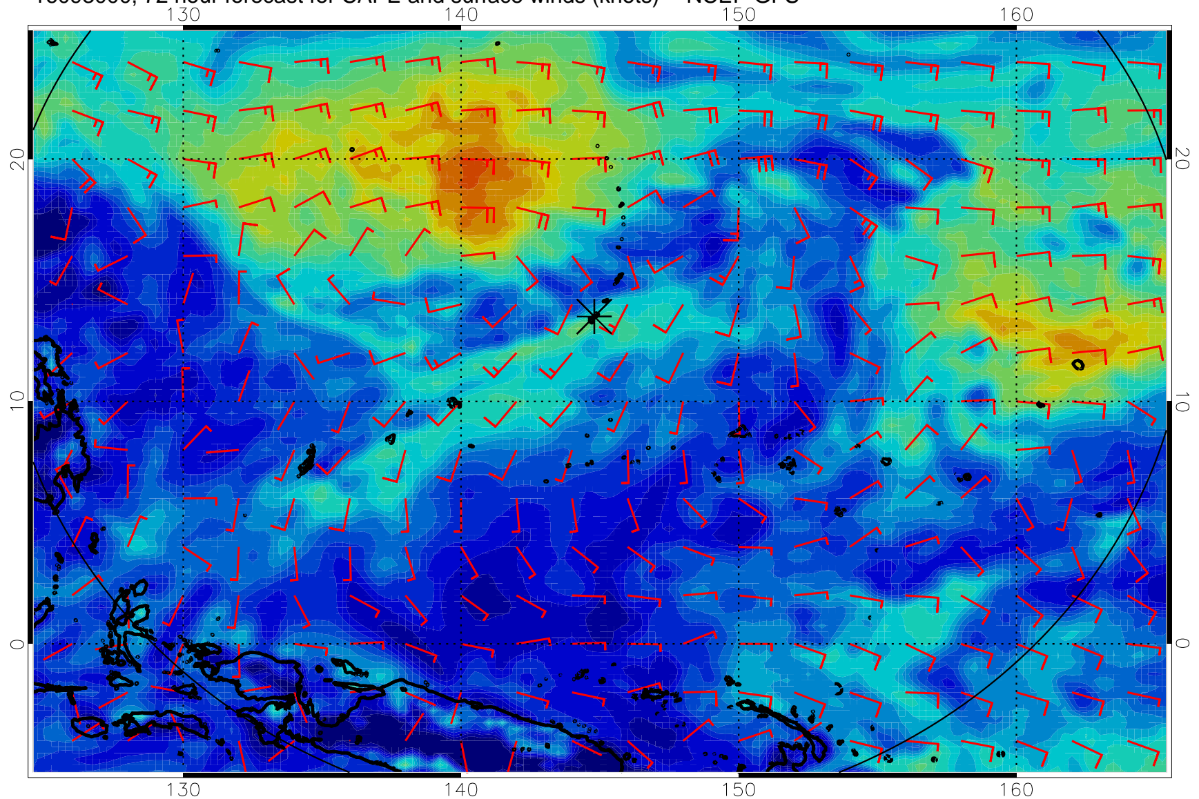
16093000, 72 hour forecast for CAPE and surface winds (knots) -- NCEP GFS
