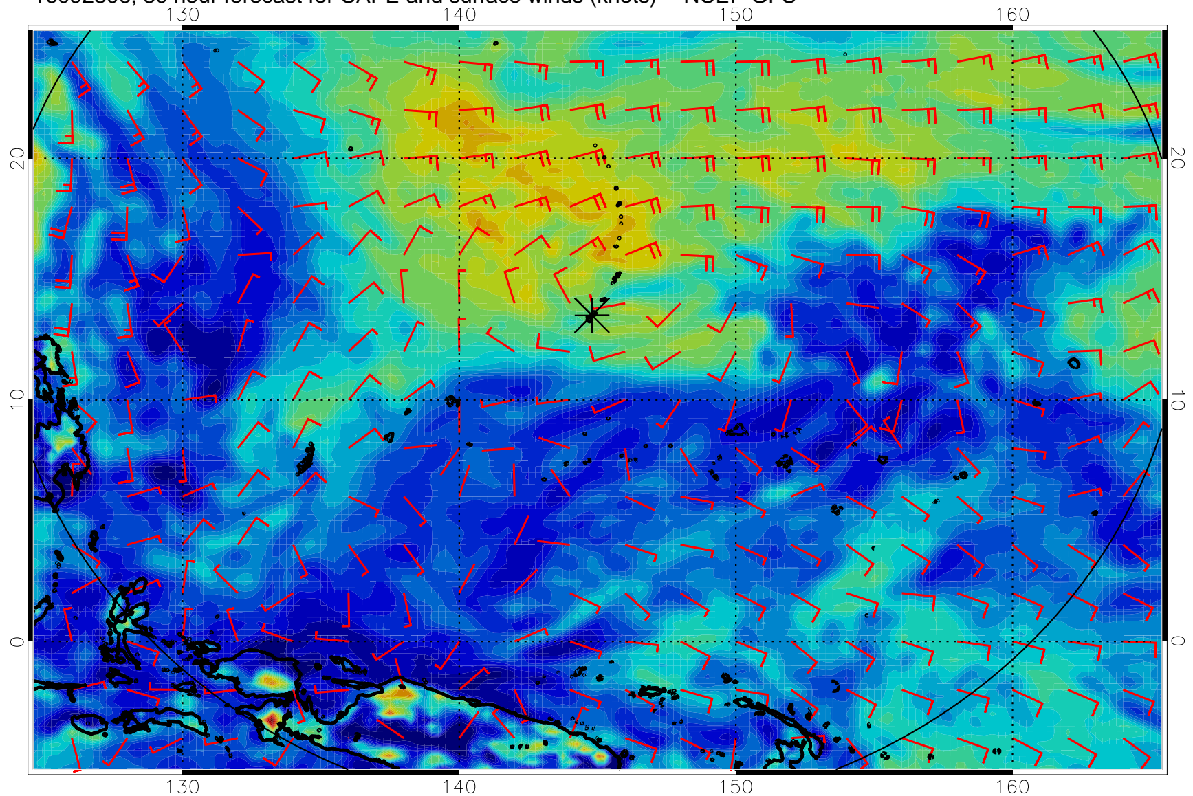
16092806, 30 hour forecast for CAPE and surface winds (knots) -- NCEP GFS
