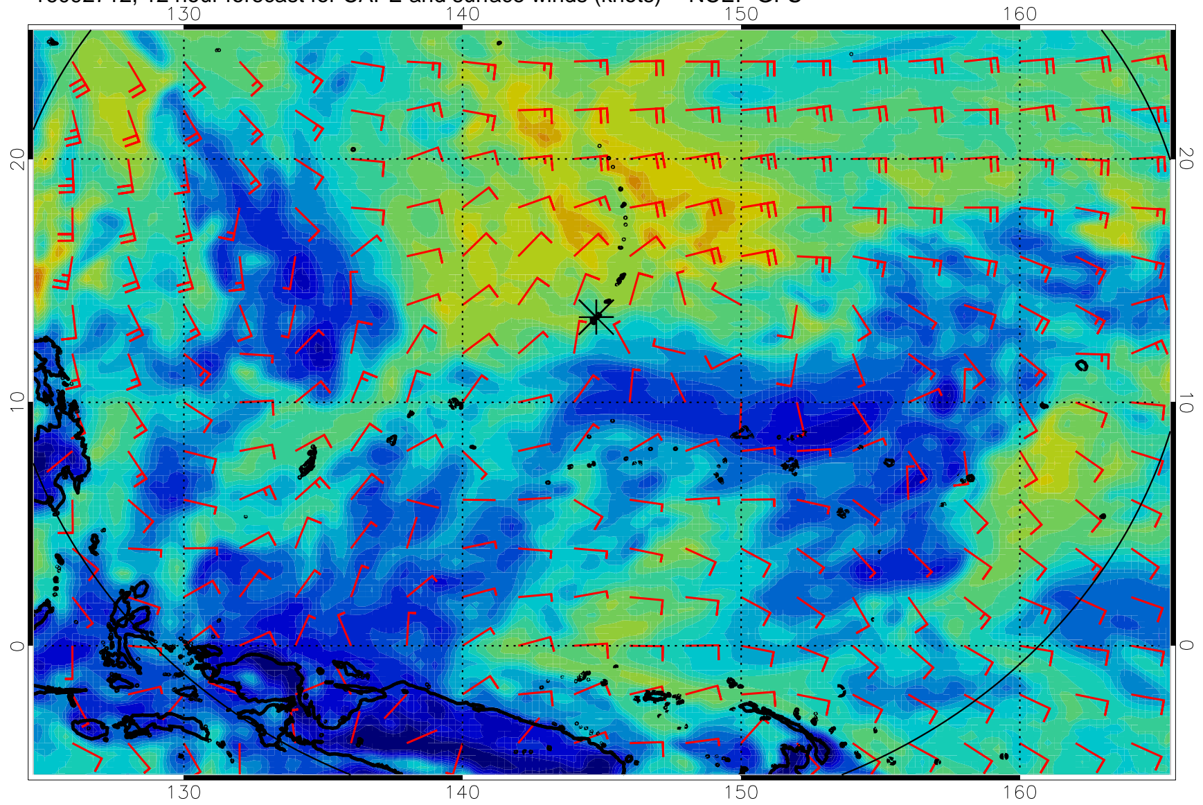
16092712, 12 hour forecast for CAPE and surface winds (knots) -- NCEP GFS
