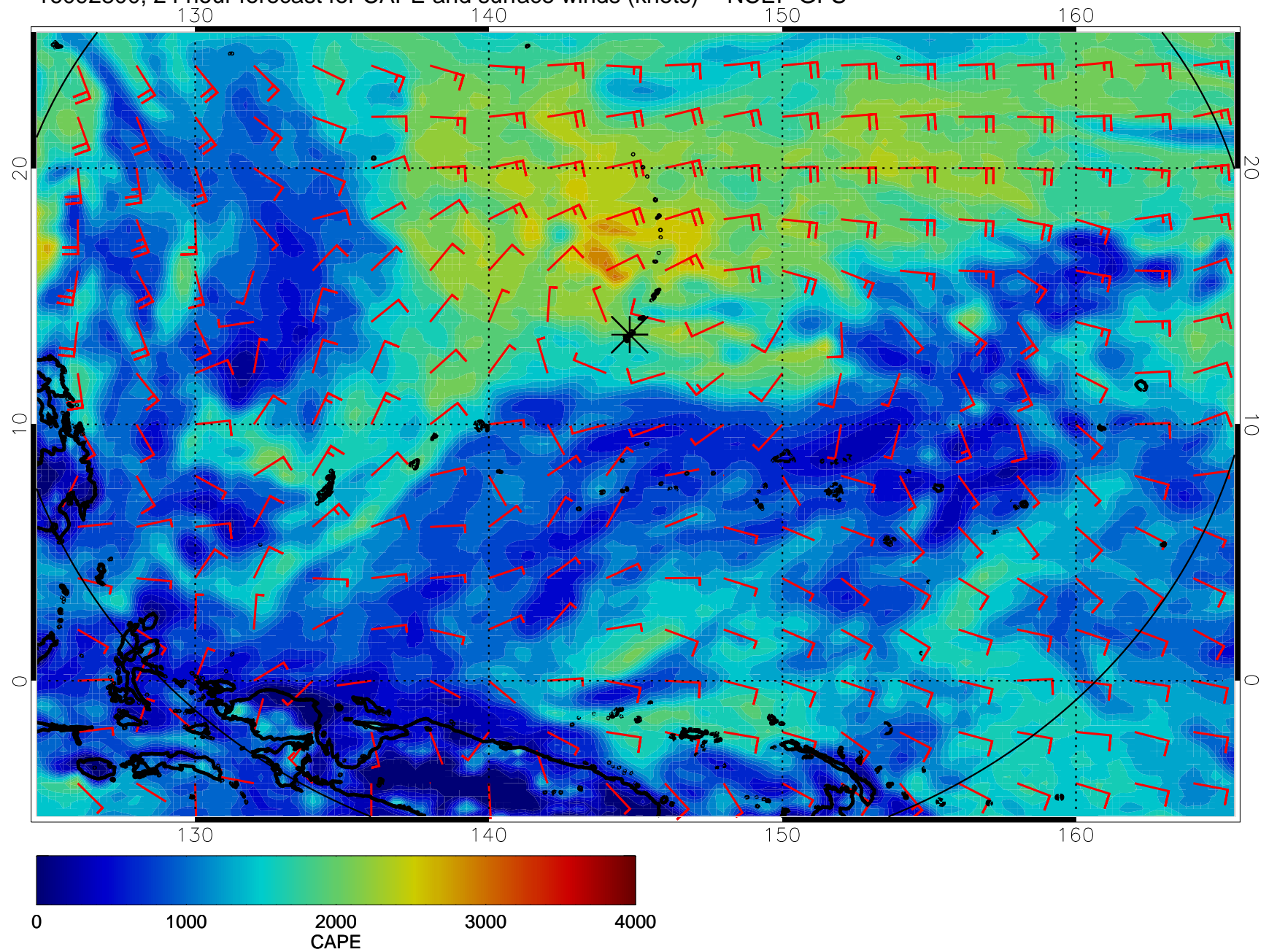
16092800, 24 hour forecast for CAPE and surface winds (knots) -- NCEP GFS
