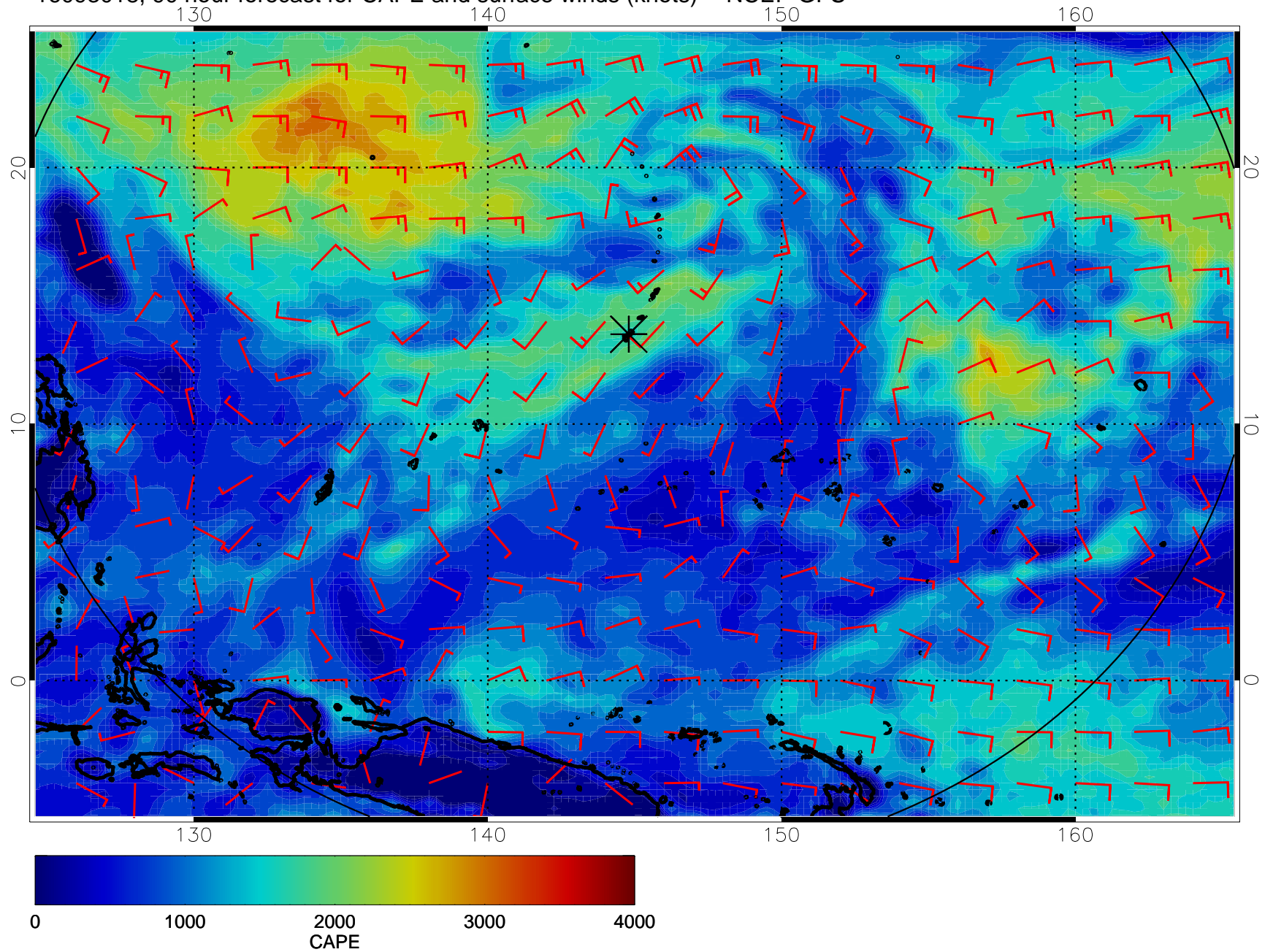
16093018, 90 hour forecast for CAPE and surface winds (knots) -- NCEP GFS
