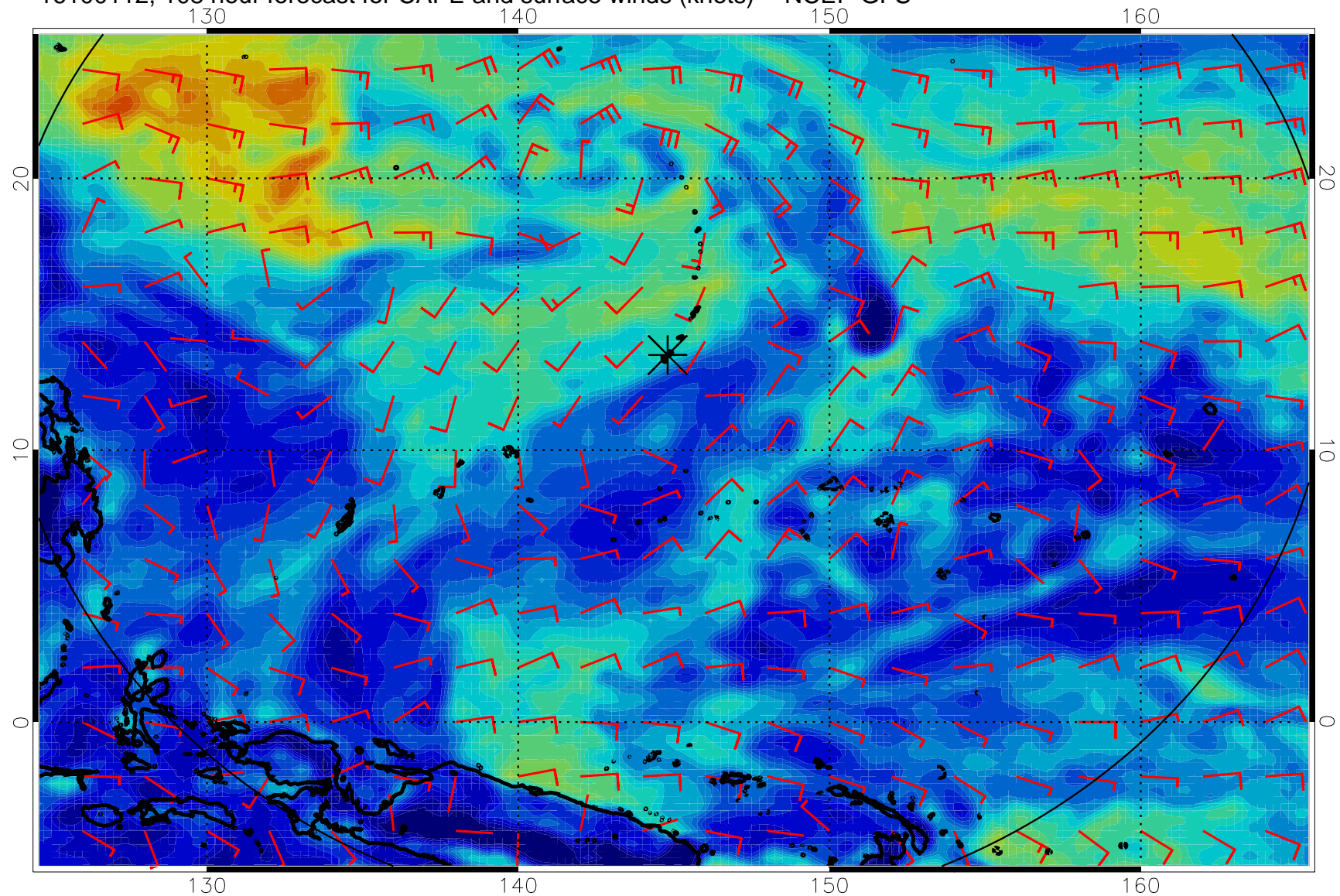
16100112, 108 hour forecast for CAPE and surface winds (knots) -- NCEP GFS
