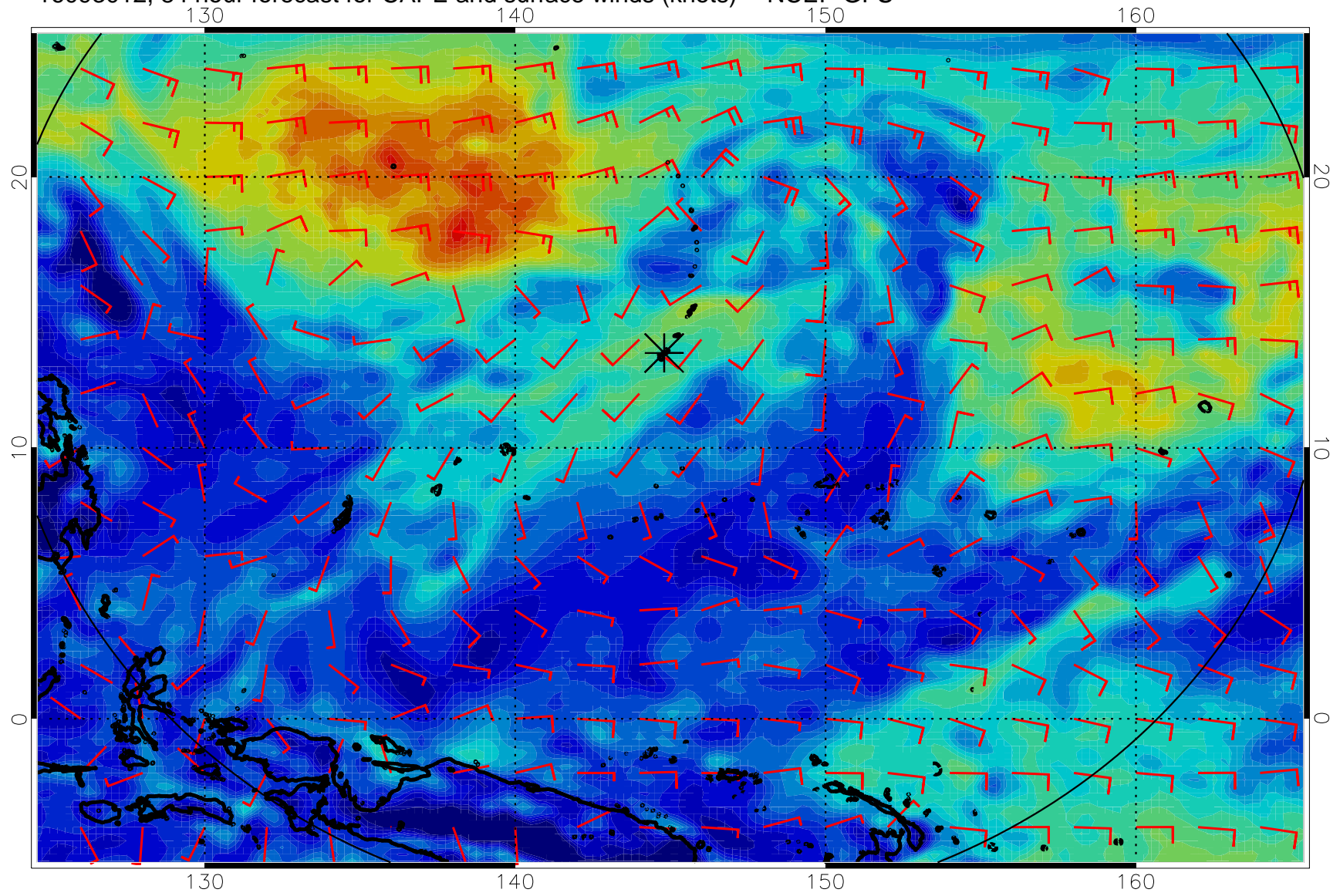
16093012, 84 hour forecast for CAPE and surface winds (knots) -- NCEP GFS
