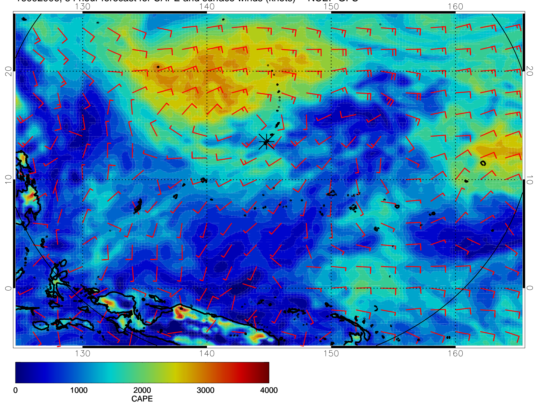
16092906, 54 hour forecast for CAPE and surface winds (knots) -- NCEP GFS
