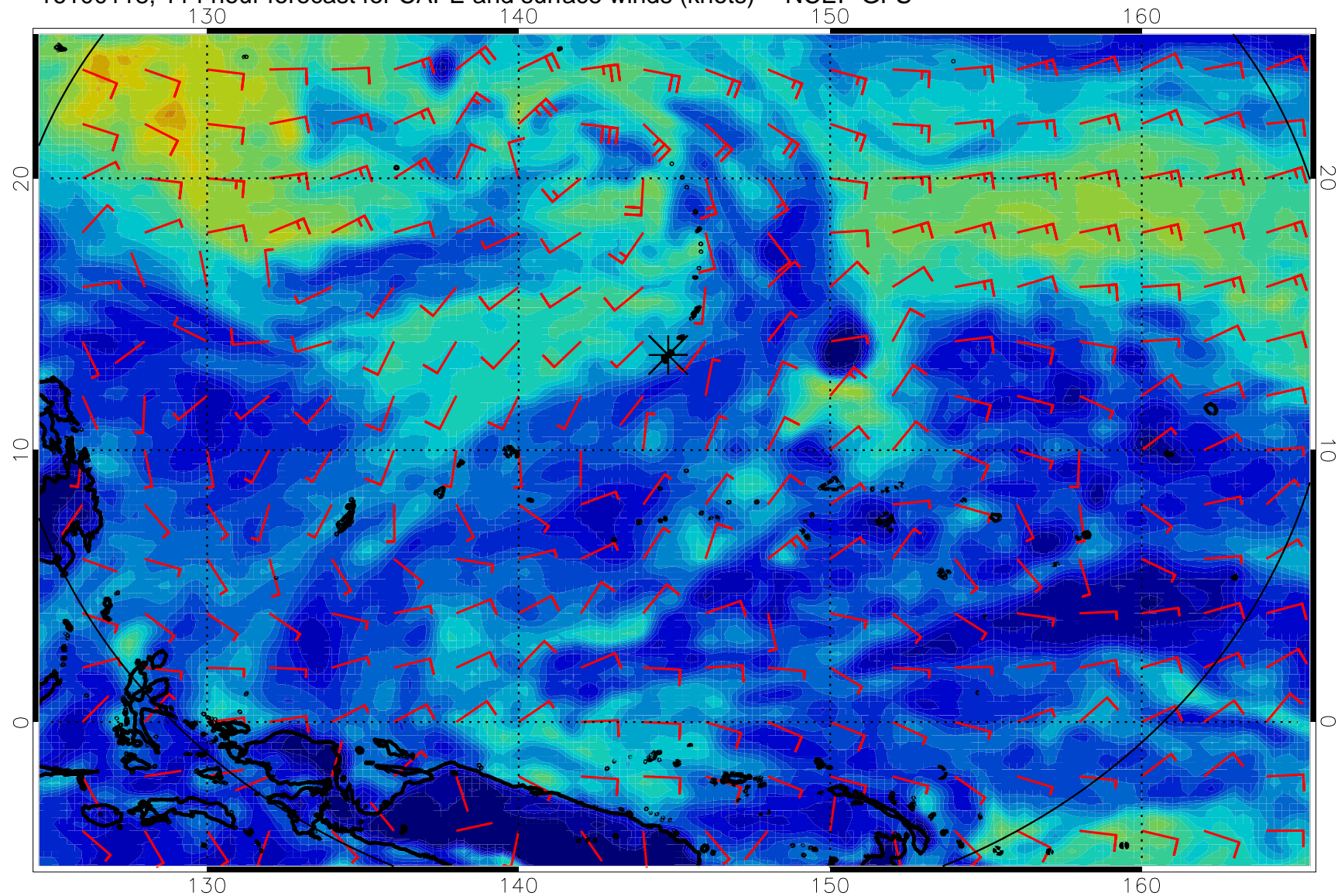
16100118, 114 hour forecast for CAPE and surface winds (knots) -- NCEP GFS
