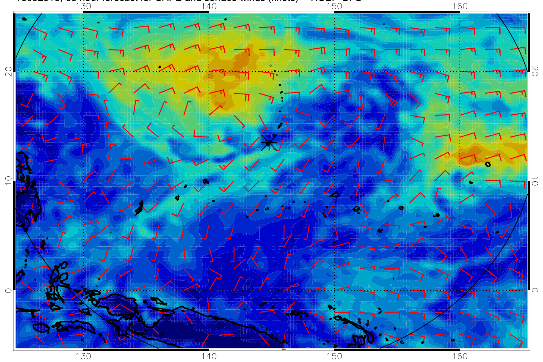
16092918, 66 hour forecast for CAPE and surface winds (knots) -- NCEP GFS
