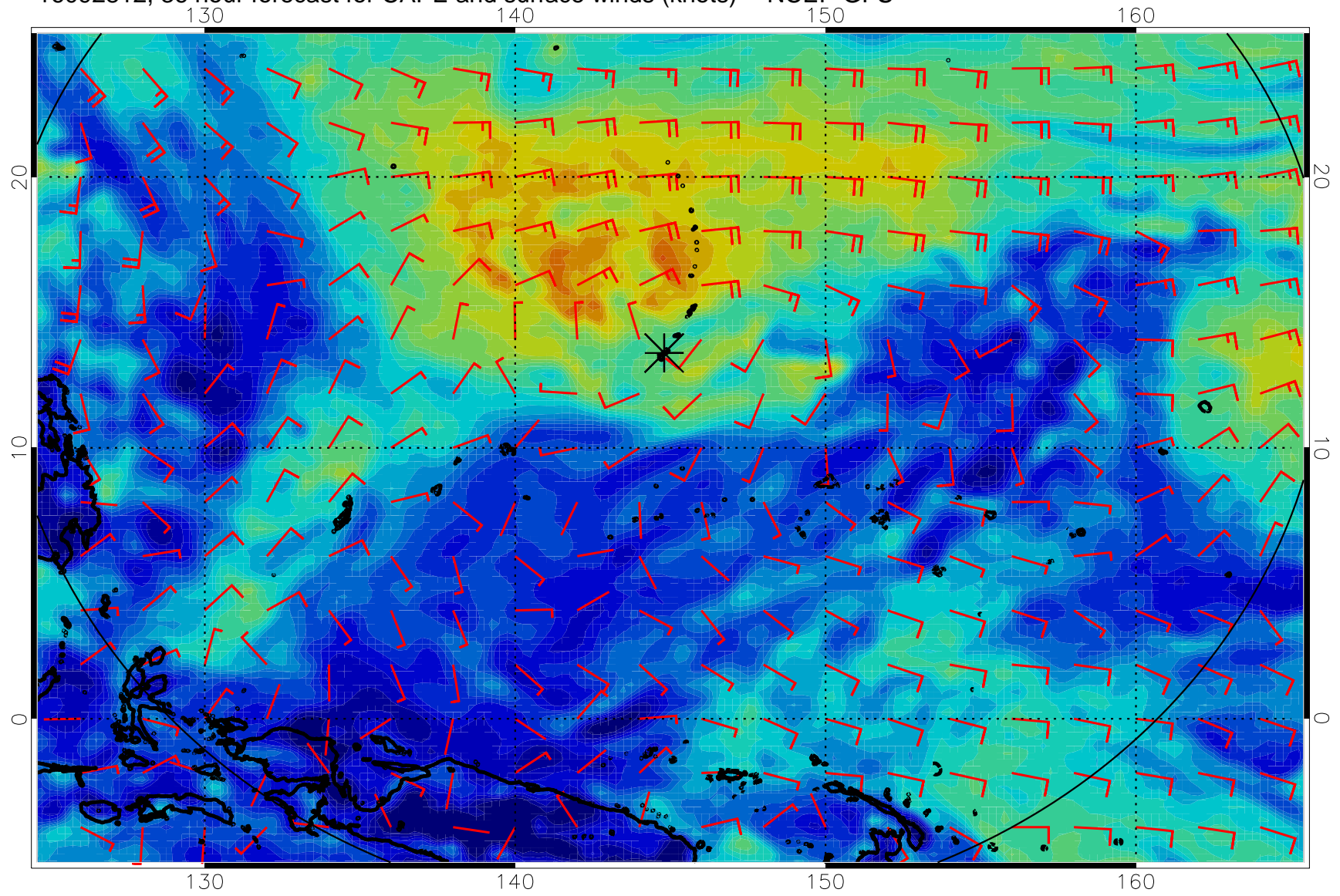
16092812, 36 hour forecast for CAPE and surface winds (knots) -- NCEP GFS
