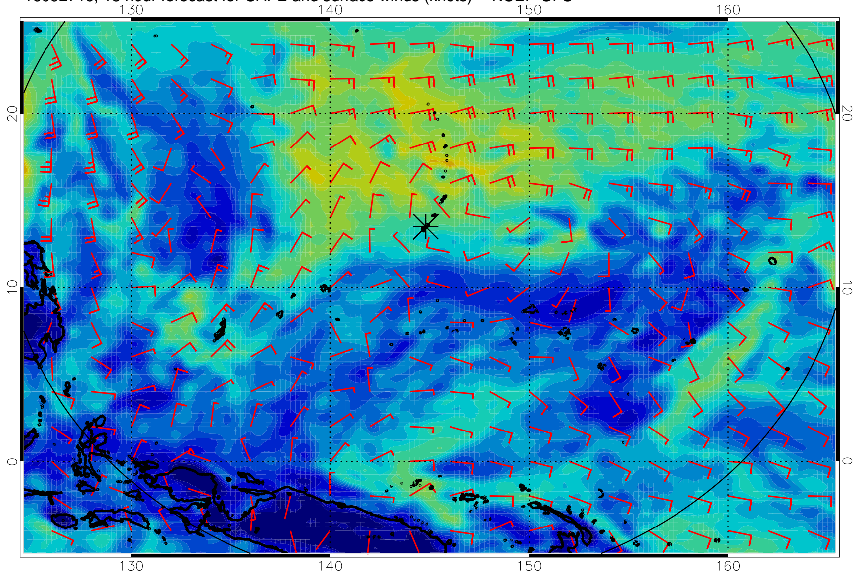
16092718, 18 hour forecast for CAPE and surface winds (knots) -- NCEP GFS
