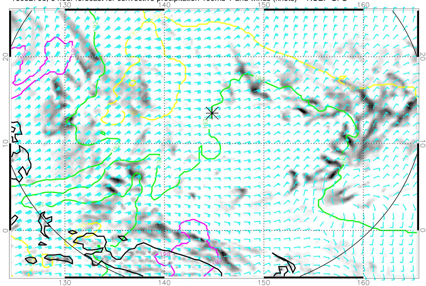
16092706, 6 hour forecast for convective precipitation 100mb T and winds (knots) -- NCEP GFS
