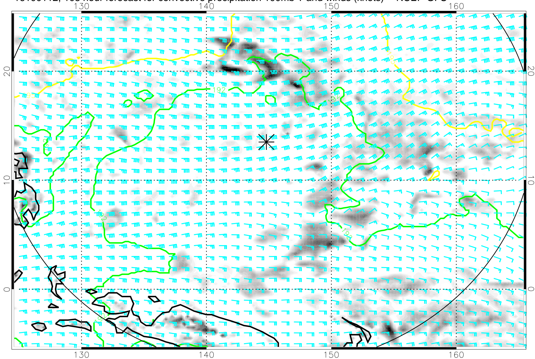
16100112, 108 hour forecast for convective precipitation 100mb T and winds (knots) -- NCEP GFS
