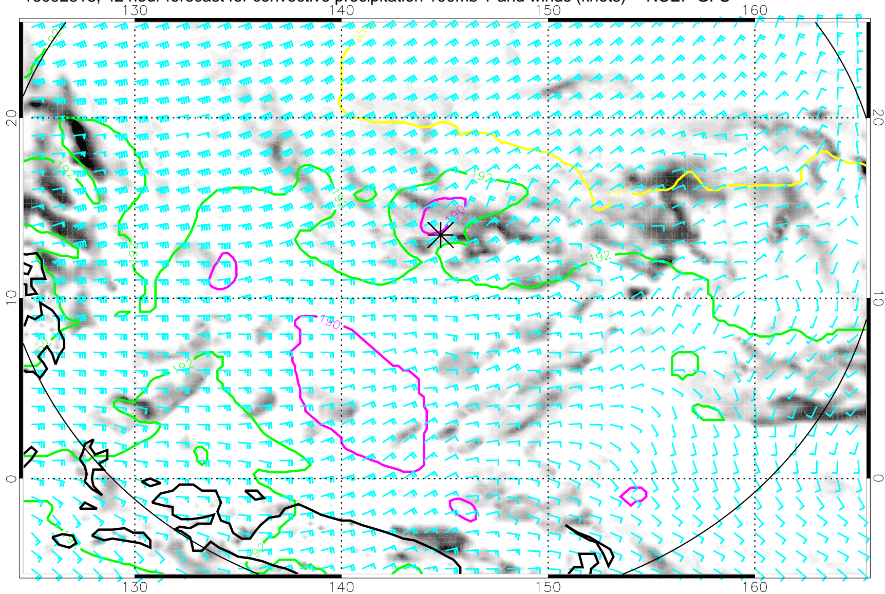
16092818, 42 hour forecast for convective precipitation 100mb T and winds (knots) -- NCEP GFS
