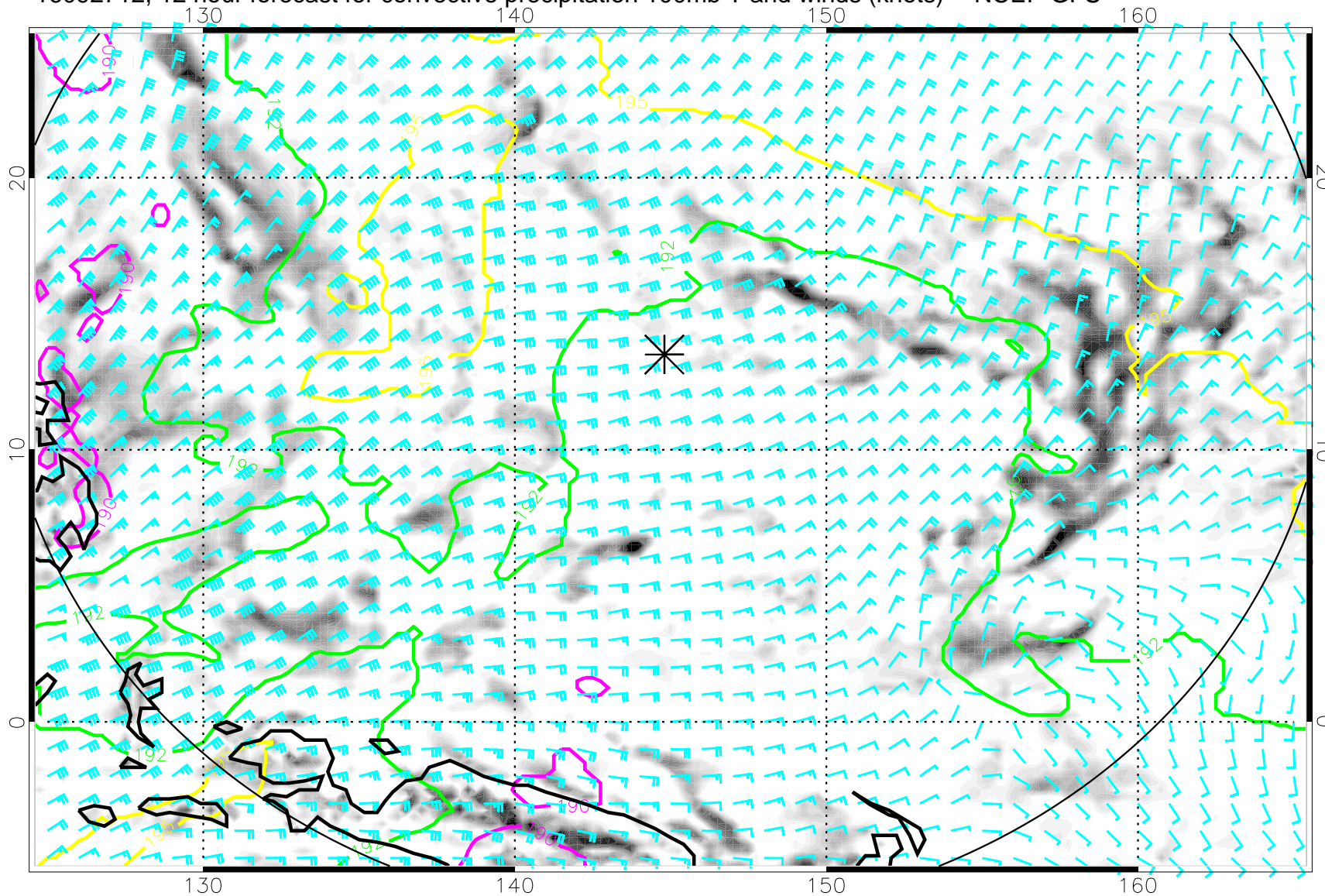
16092712, 12 hour forecast for convective precipitation 100mb T and winds (knots) -- NCEP GFS
