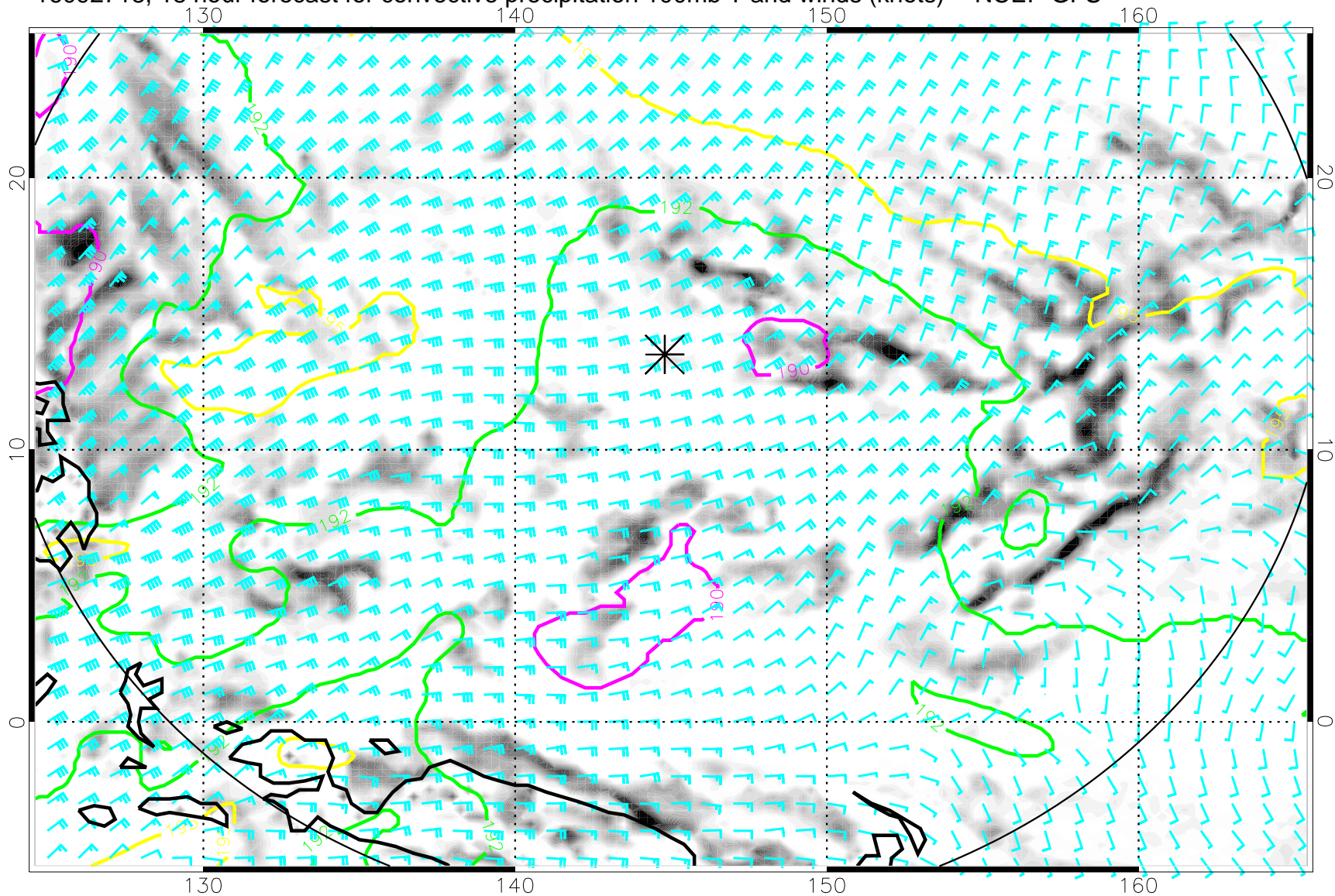
16092718, 18 hour forecast for convective precipitation 100mb T and winds (knots) -- NCEP GFS
