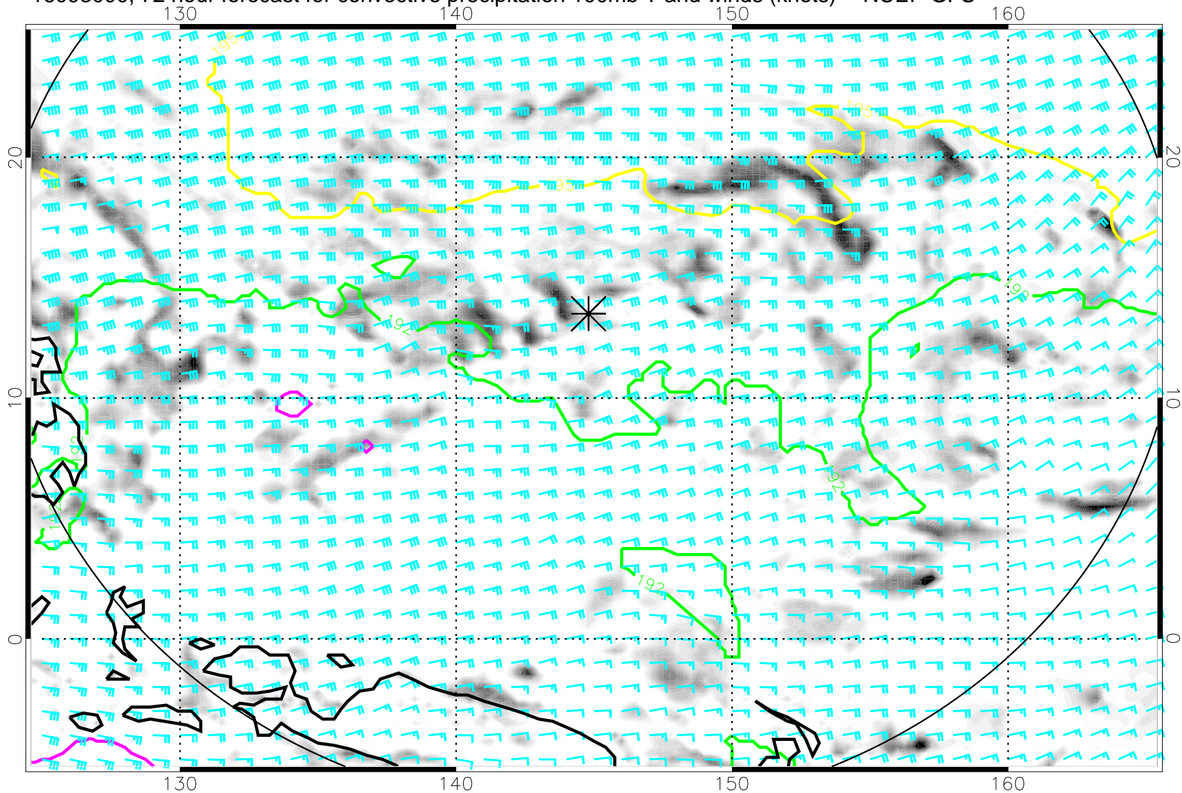
16093000, 72 hour forecast for convective precipitation 100mb T and winds (knots) -- NCEP GFS
