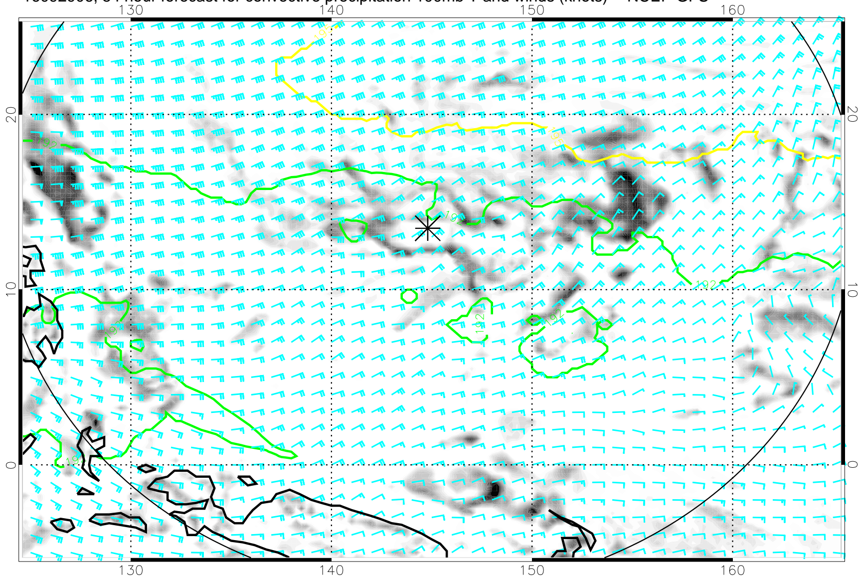
16092906, 54 hour forecast for convective precipitation 100mb T and winds (knots) -- NCEP GFS
