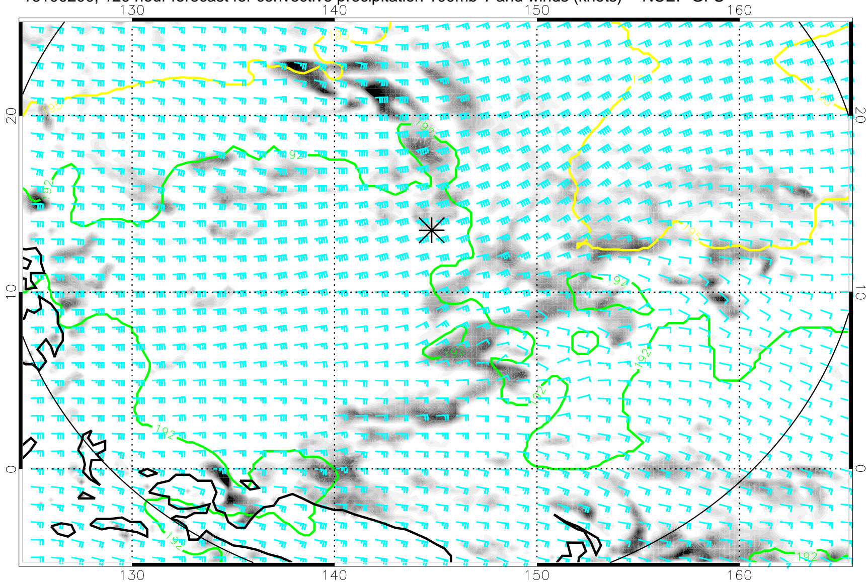
16100200, 120 hour forecast for convective precipitation 100mb T and winds (knots) -- NCEP GFS
