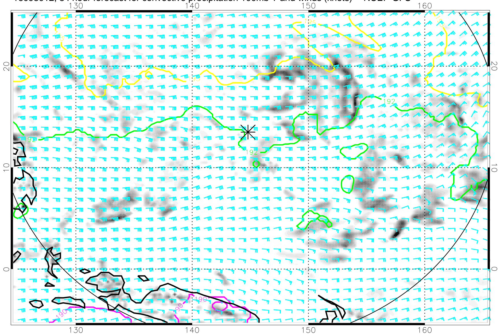
16093012, 84 hour forecast for convective precipitation 100mb T and winds (knots) -- NCEP GFS
