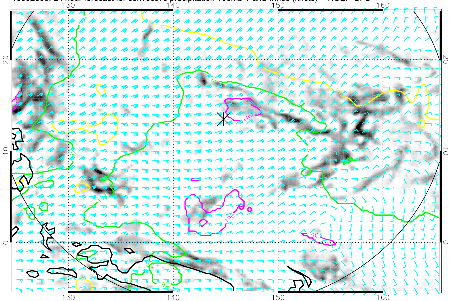
16092800, 24 hour forecast for convective precipitation 100mb T and winds (knots) -- NCEP GFS
