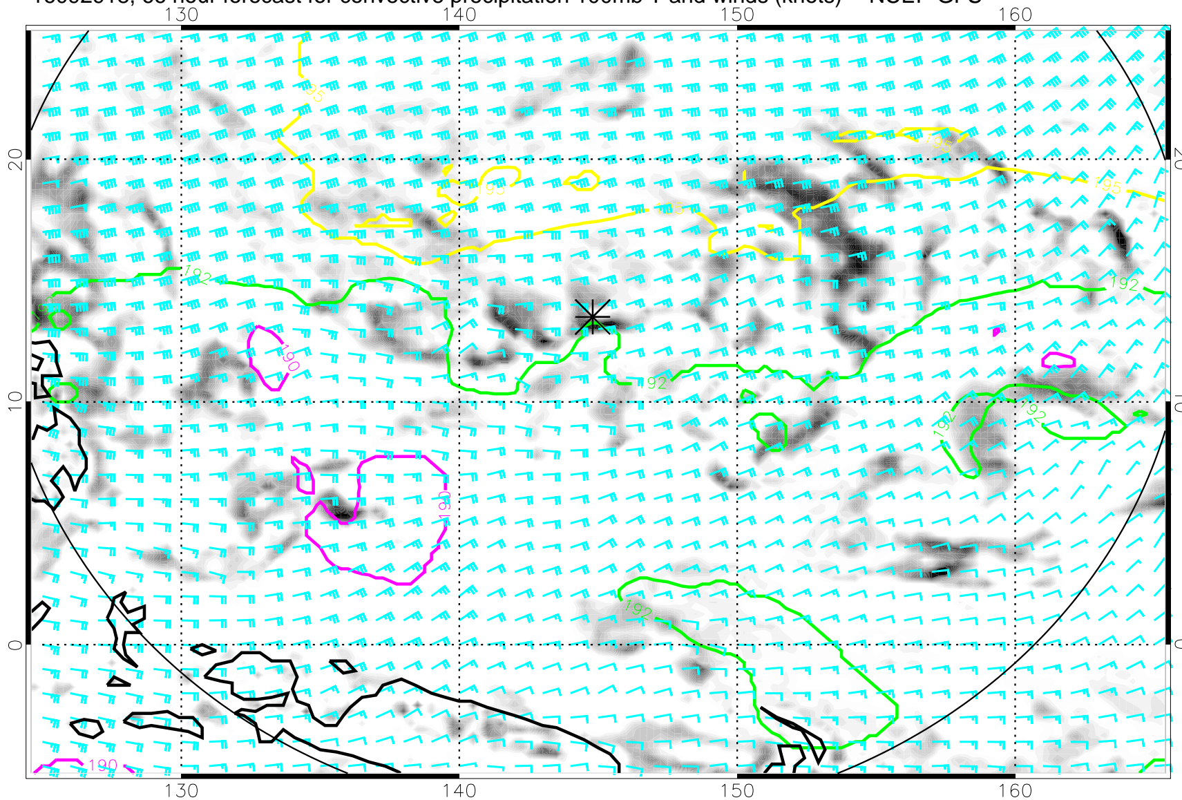
16092918, 66 hour forecast for convective precipitation 100mb T and winds (knots) -- NCEP GFS
