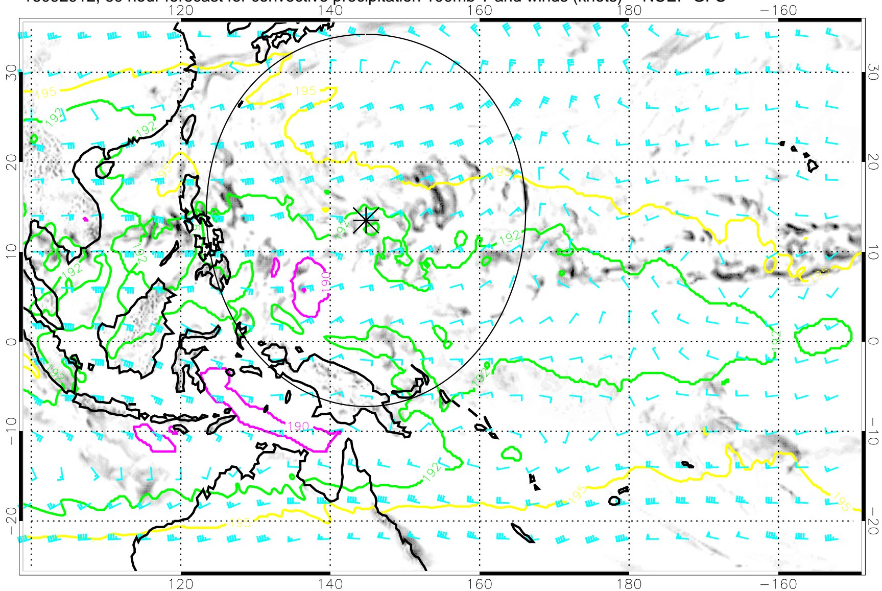
16092912, 60 hour forecast for convective precipitation 100mb T and winds (knots) -- NCEP GFS
