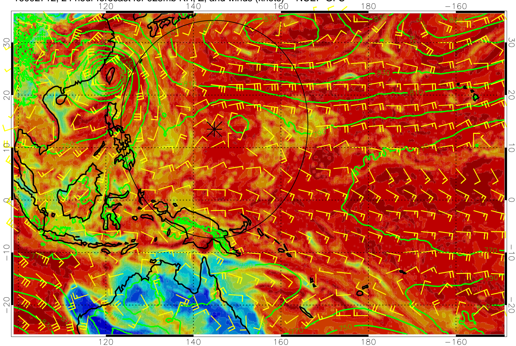
16092712, 24 hour forecast for 925mb RH, Z, and winds (knots) -- NCEP GFS
