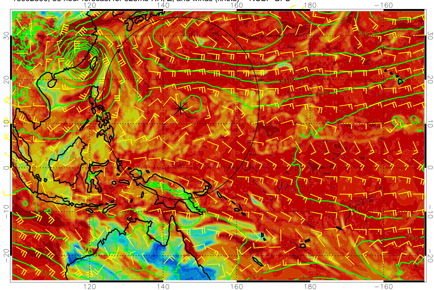
16092800, 36 hour forecast for 925mb RH, Z, and winds (knots) -- NCEP GFS
