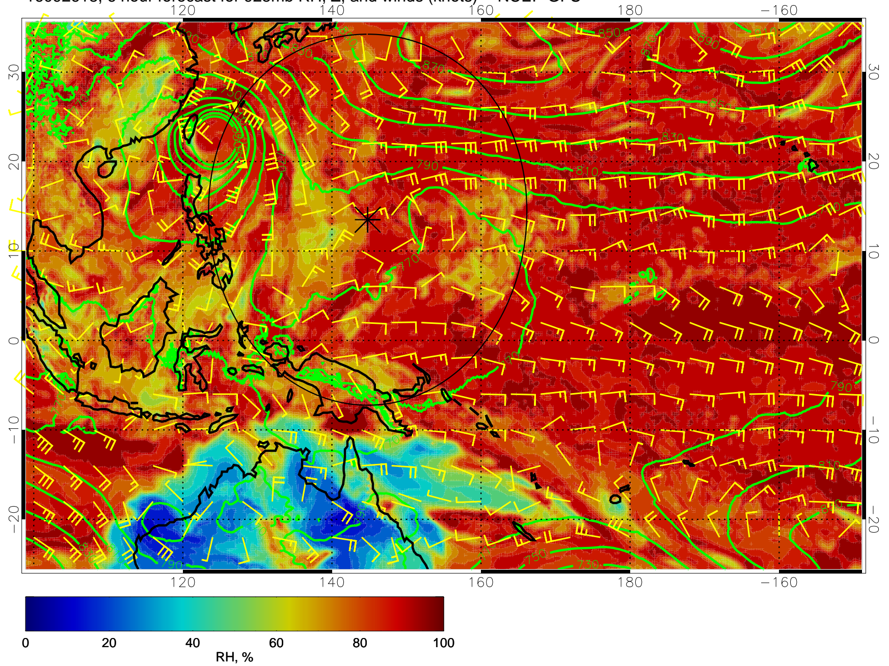
16092618, 6 hour forecast for 925mb RH, Z, and winds (knots) -- NCEP GFS
