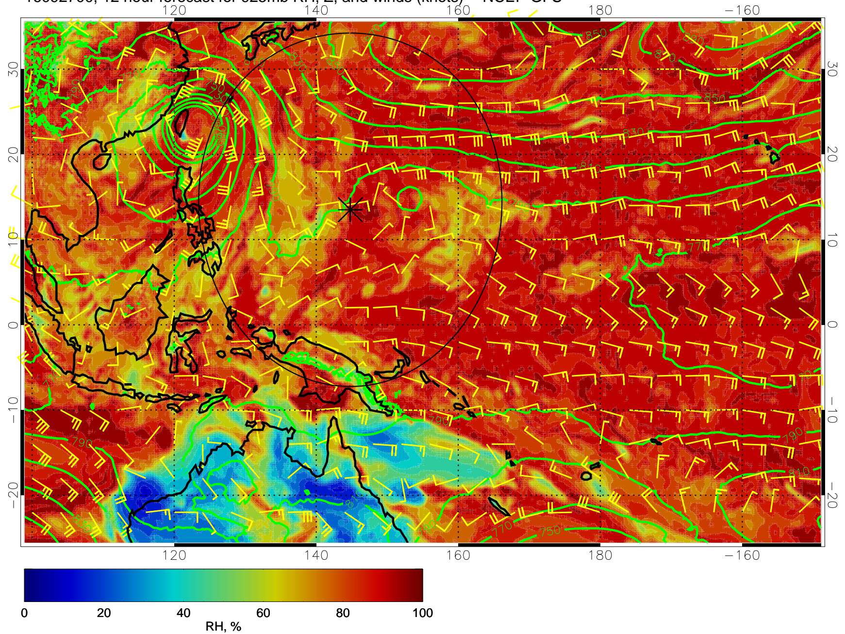
16092700, 12 hour forecast for 925mb RH, Z, and winds (knots) -- NCEP GFS
