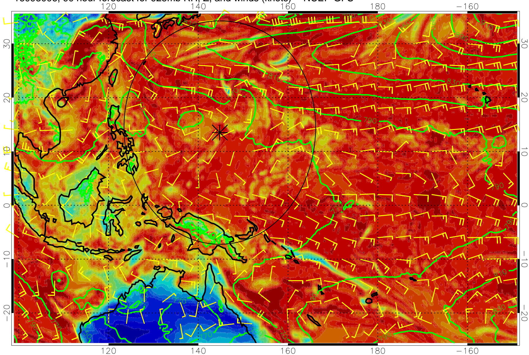
16093006, 90 hour forecast for 925mb RH, Z, and winds (knots) -- NCEP GFS
