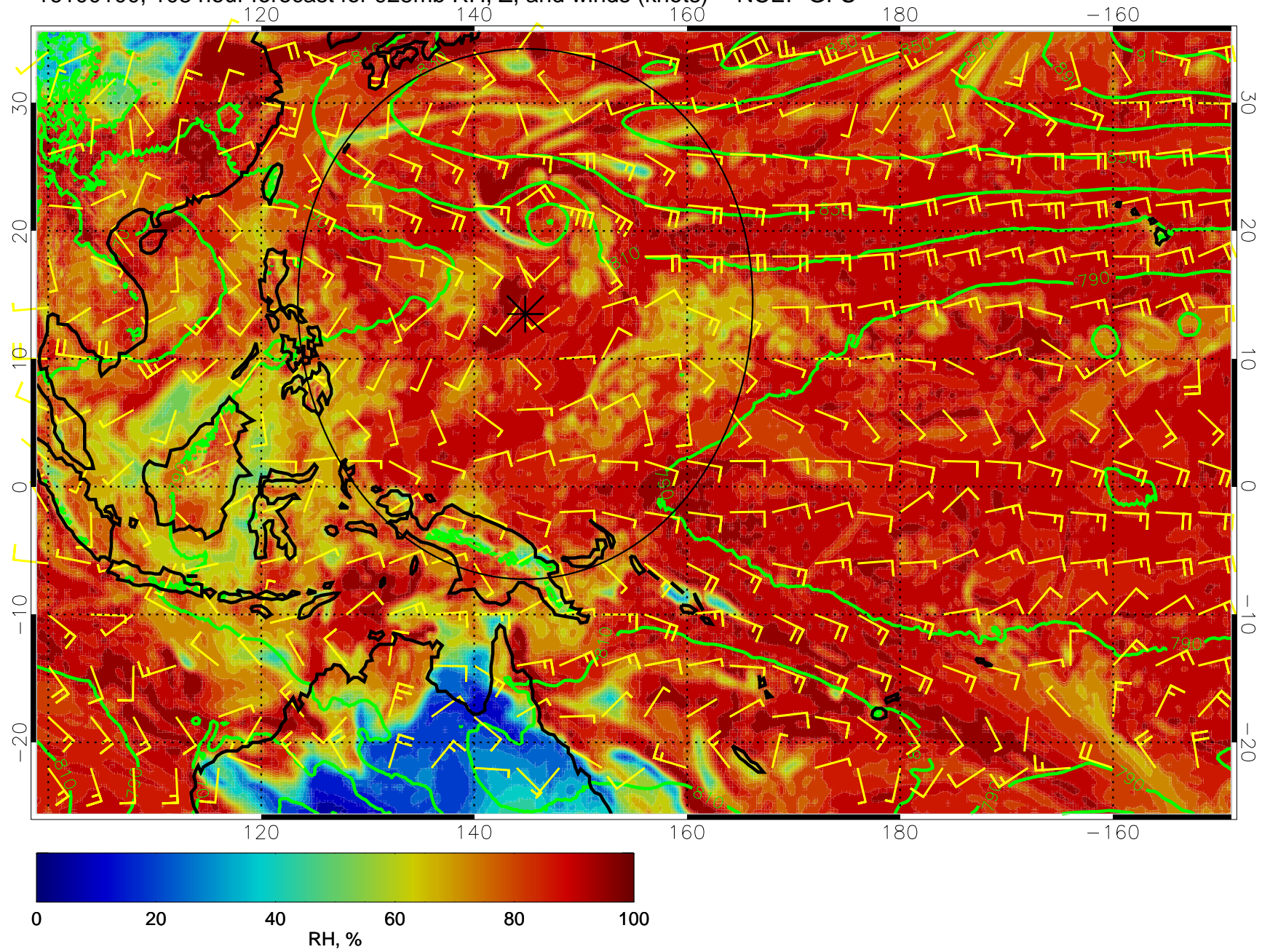
16100100, 108 hour forecast for 925mb RH, Z, and winds (knots) -- NCEP GFS
