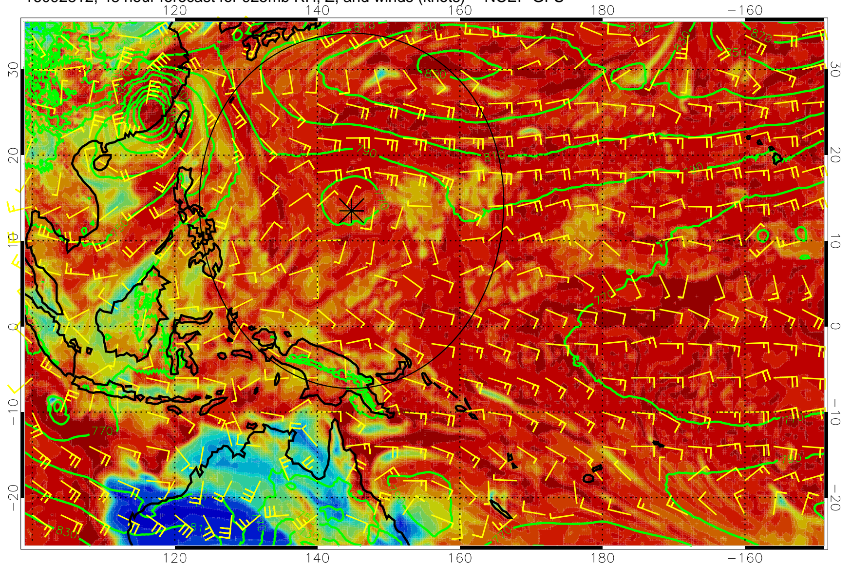
16092812, 48 hour forecast for 925mb RH, Z, and winds (knots) -- NCEP GFS
