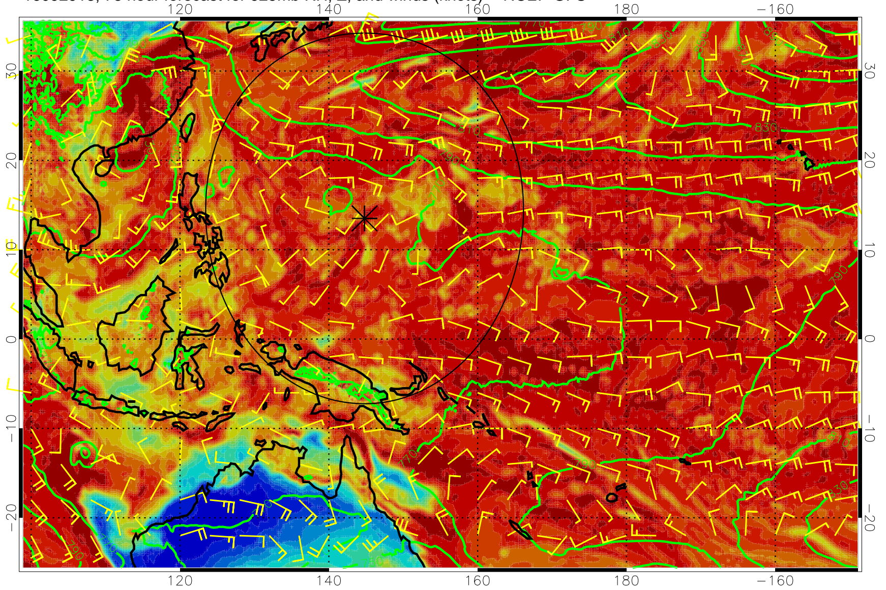
16092918, 78 hour forecast for 925mb RH, Z, and winds (knots) -- NCEP GFS
