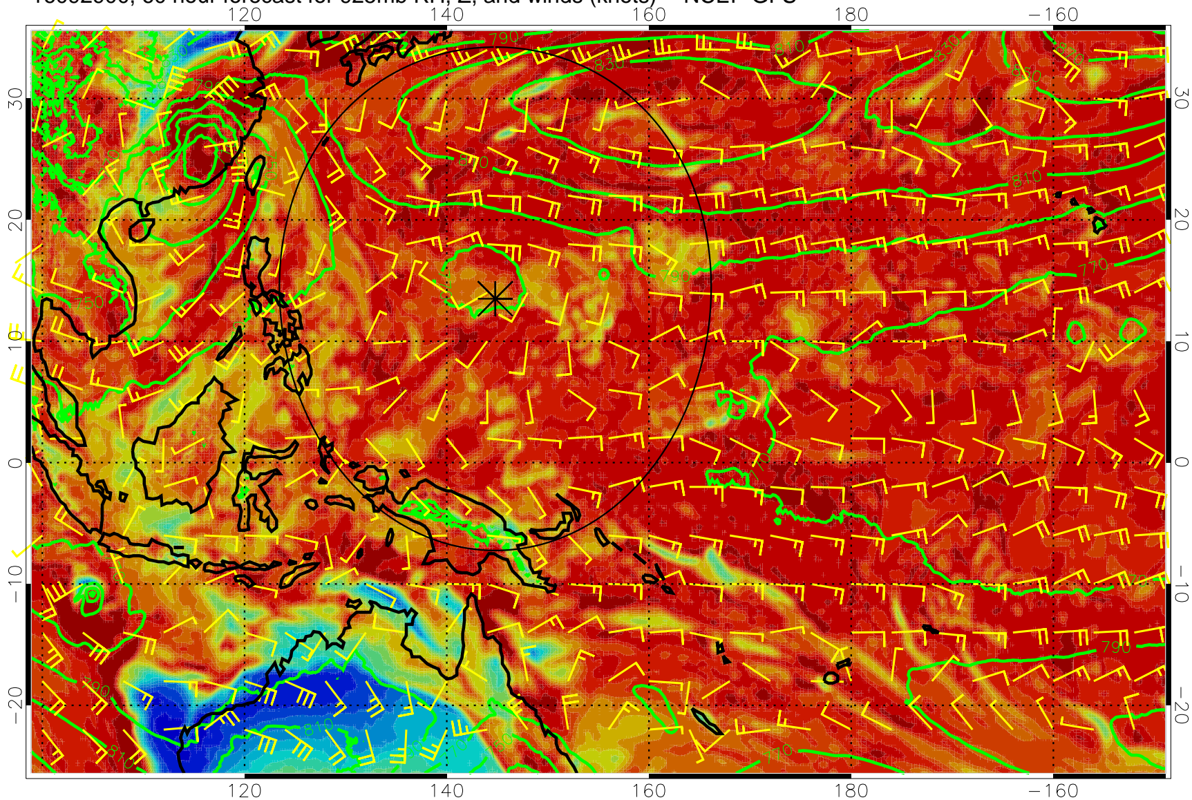
16092900, 60 hour forecast for 925mb RH, Z, and winds (knots) -- NCEP GFS
