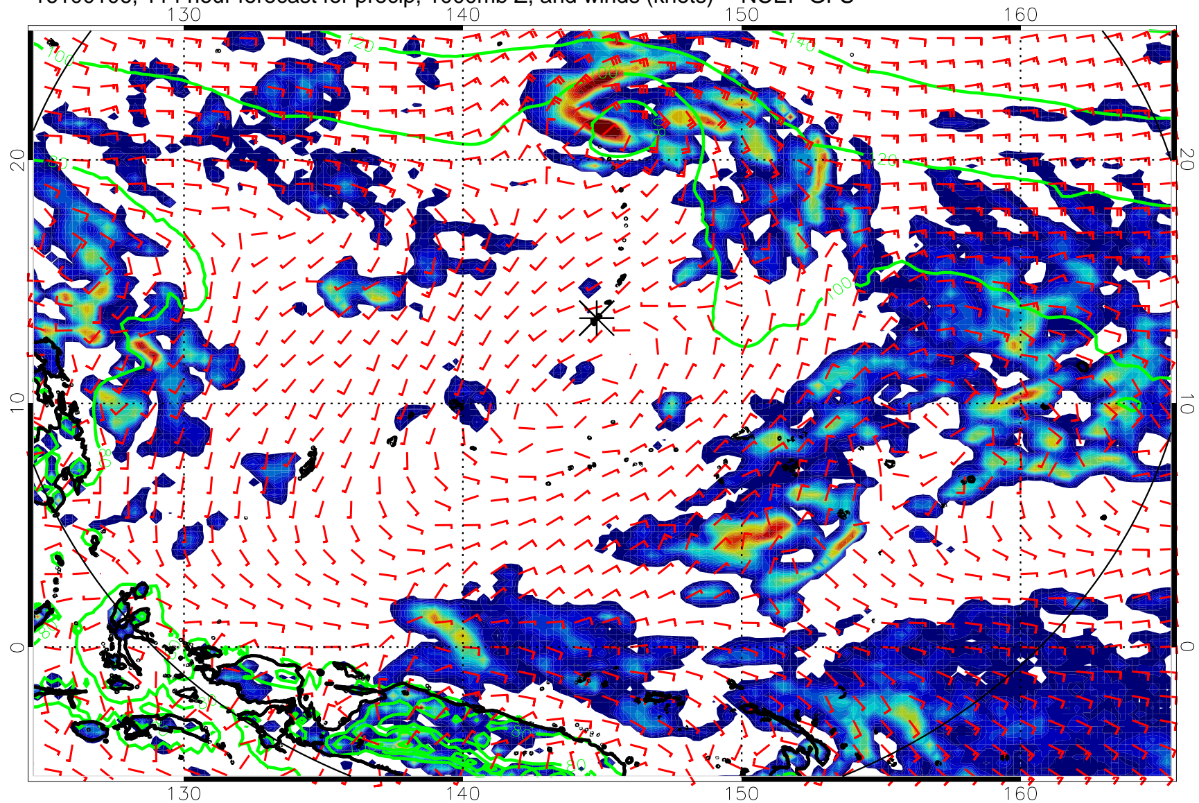
16100106, 114 hour forecast for precip, 1000mb Z, and winds (knots) -- NCEP GFS
