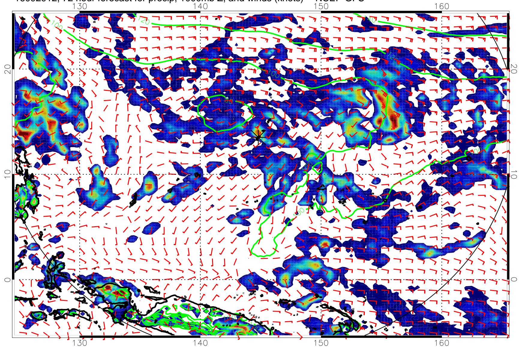
16092912, 72 hour forecast for precip, 1000mb Z, and winds (knots) -- NCEP GFS
