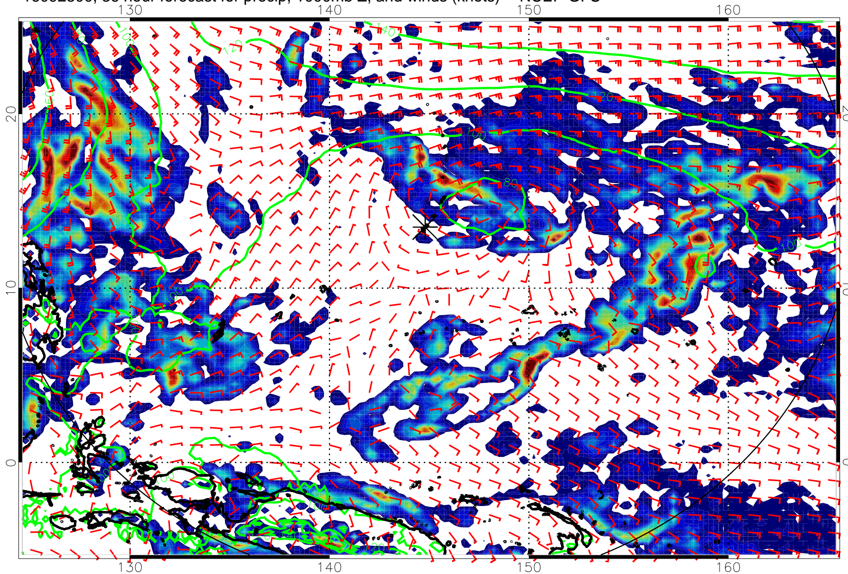
16092800, 36 hour forecast for precip, 1000mb Z, and winds (knots) -- NCEP GFS
