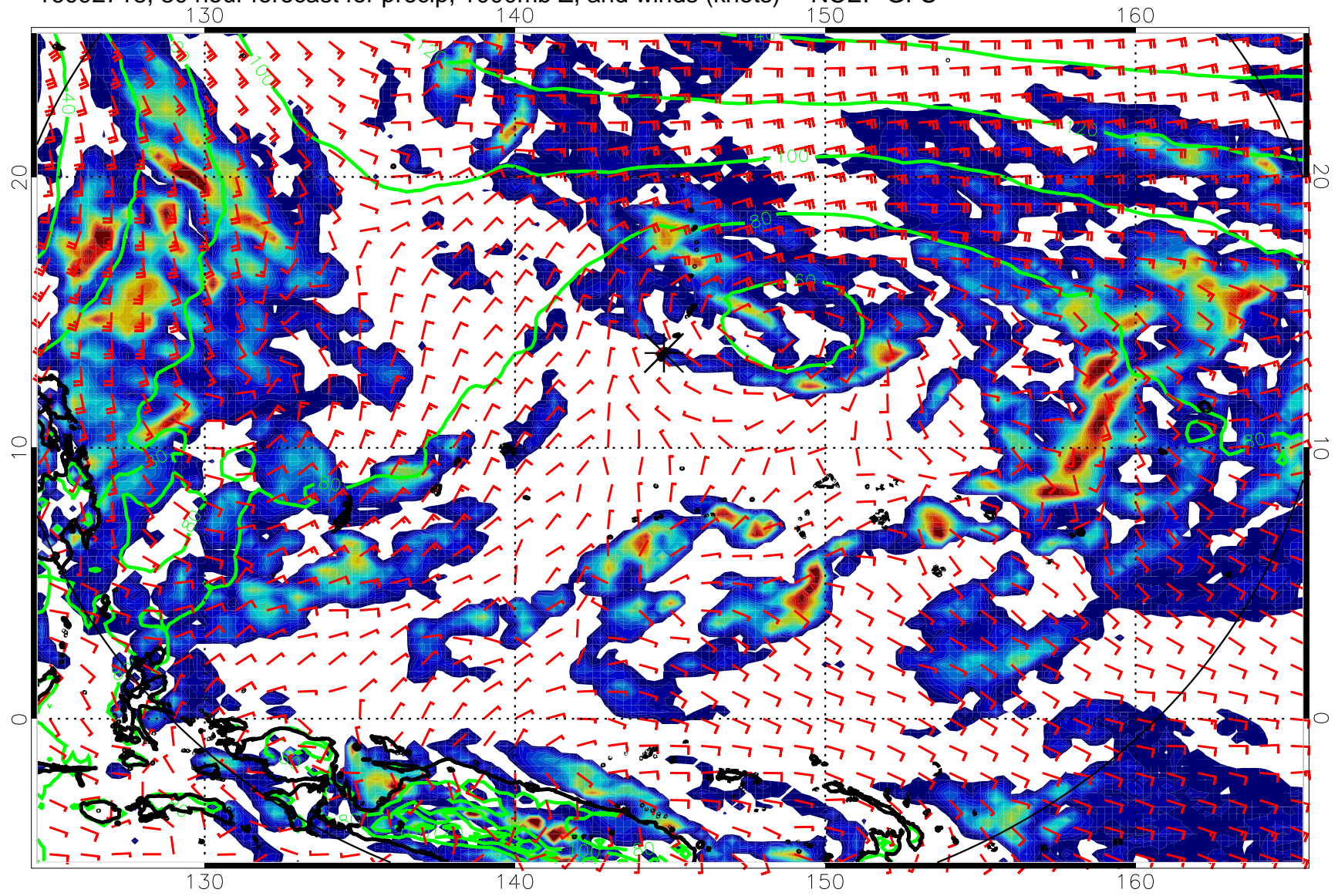
16092718, 30 hour forecast for precip, 1000mb Z, and winds (knots) -- NCEP GFS
