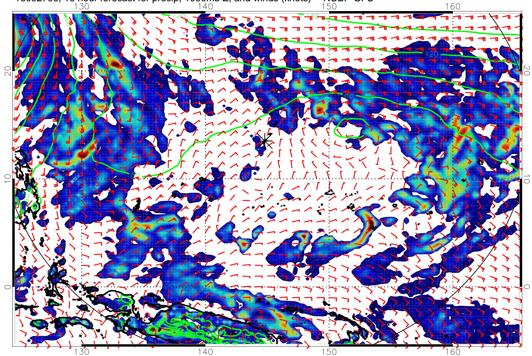
16092706, 18 hour forecast for precip, 1000mb Z, and winds (knots) -- NCEP GFS
