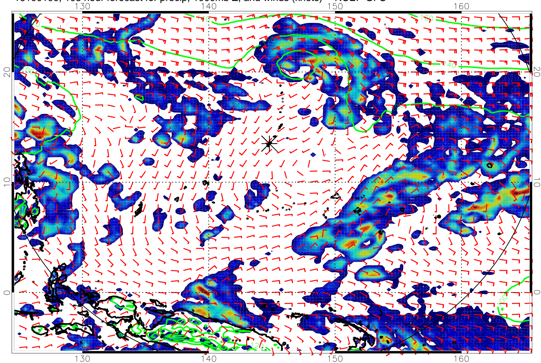
16100100, 108 hour forecast for precip, 1000mb Z, and winds (knots) -- NCEP GFS
