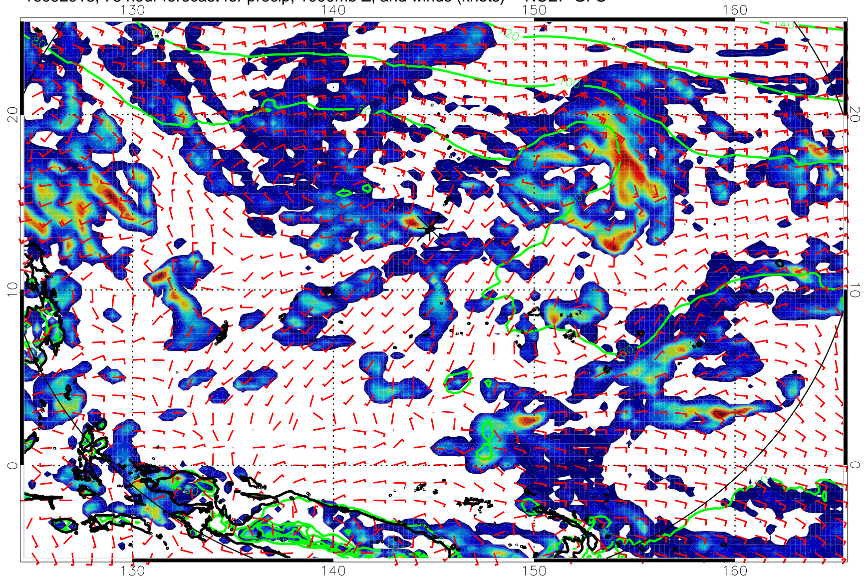
16092918, 78 hour forecast for precip, 1000mb Z, and winds (knots) -- NCEP GFS
