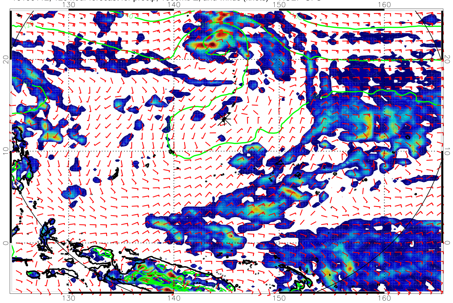
16100112, 120 hour forecast for precip, 1000mb Z, and winds (knots) -- NCEP GFS
