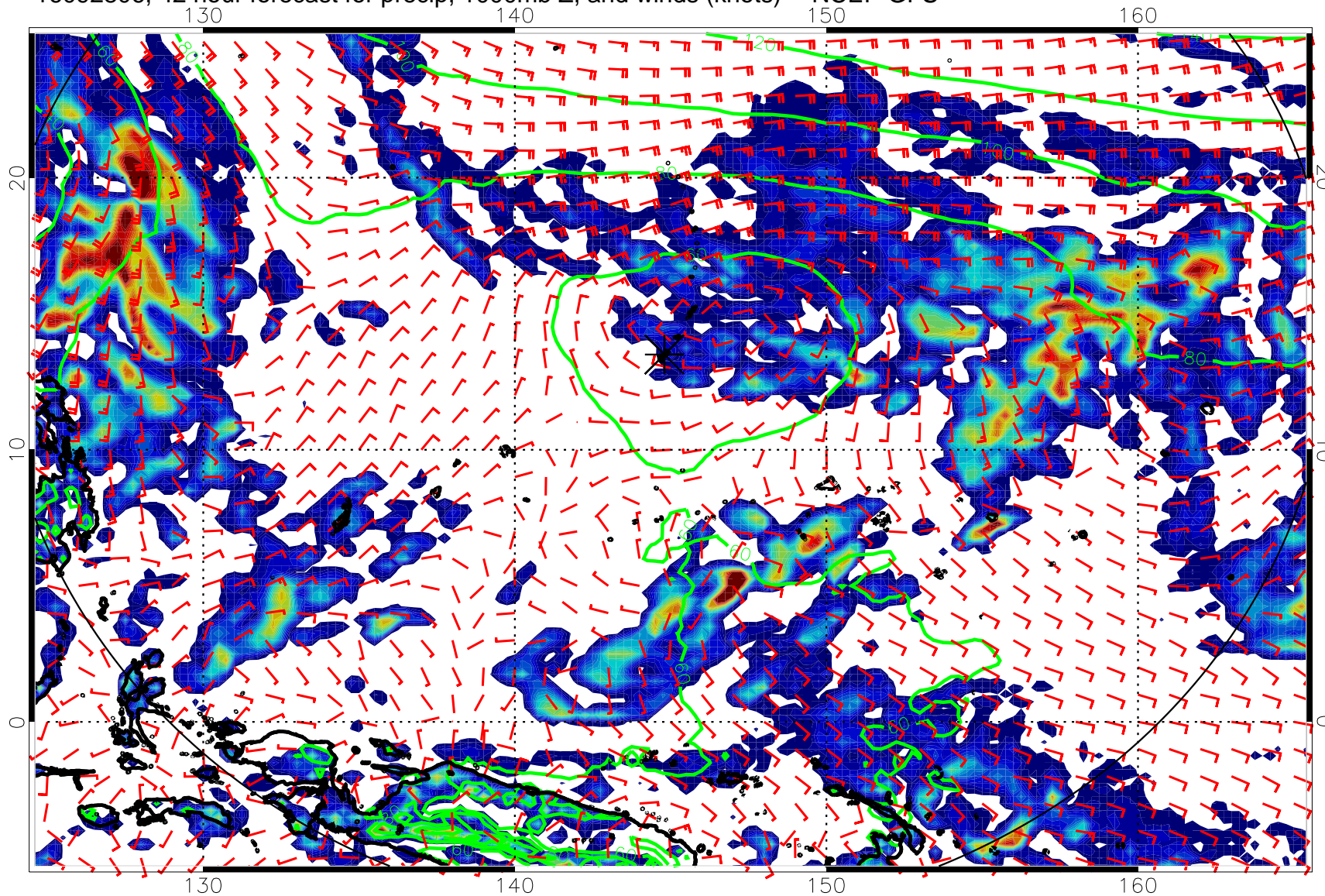
16092806, 42 hour forecast for precip, 1000mb Z, and winds (knots) -- NCEP GFS
