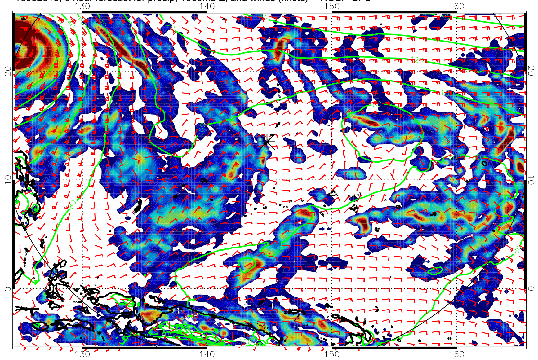
16092618, 6 hour forecast for precip, 1000mb Z, and winds (knots) -- NCEP GFS
