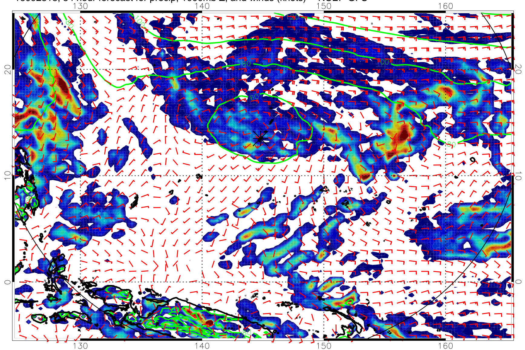
16092818, 54 hour forecast for precip, 1000mb Z, and winds (knots) -- NCEP GFS
