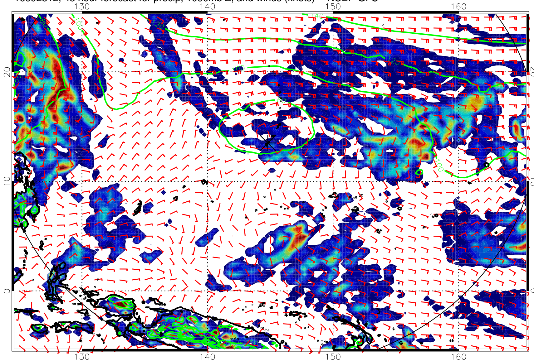
16092812, 48 hour forecast for precip, 1000mb Z, and winds (knots) -- NCEP GFS
