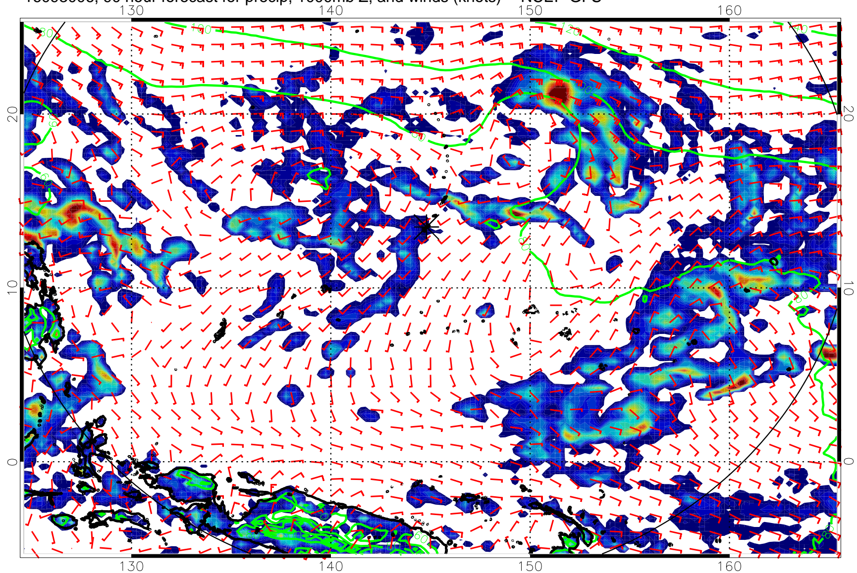
16093006, 90 hour forecast for precip, 1000mb Z, and winds (knots) -- NCEP GFS
