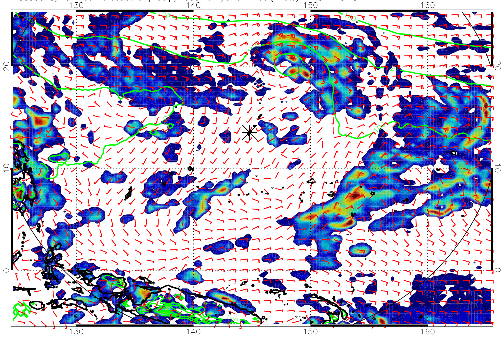
16093018, 102 hour forecast for precip, 1000mb Z, and winds (knots) -- NCEP GFS
