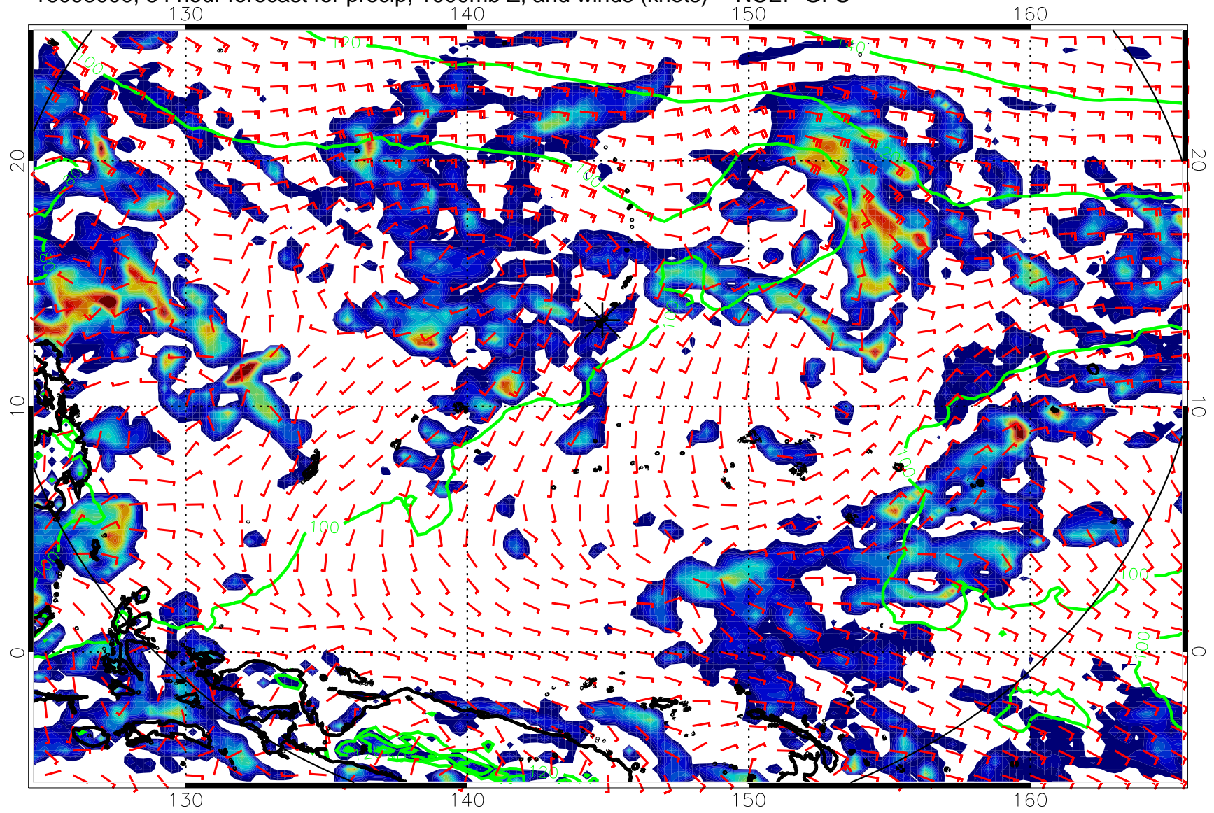
16093000, 84 hour forecast for precip, 1000mb Z, and winds (knots) -- NCEP GFS
