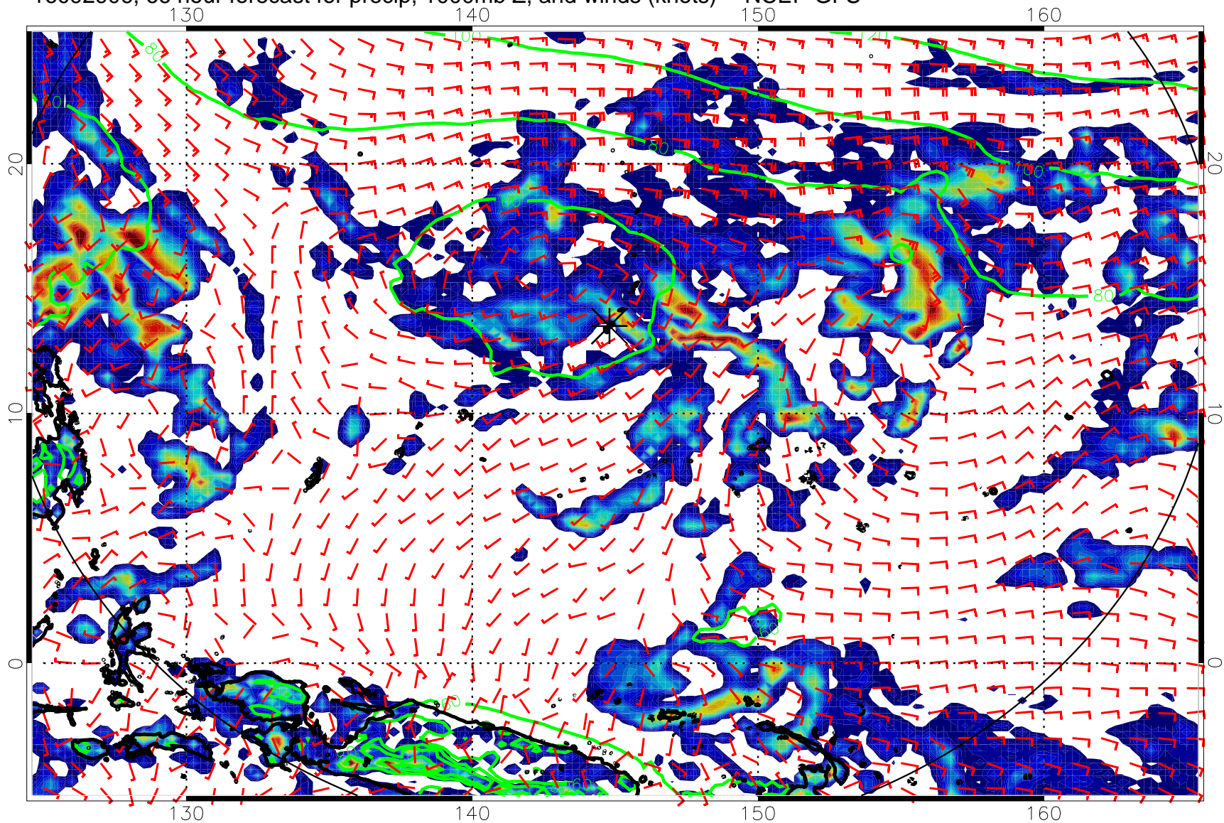
16092906, 66 hour forecast for precip, 1000mb Z, and winds (knots) -- NCEP GFS
