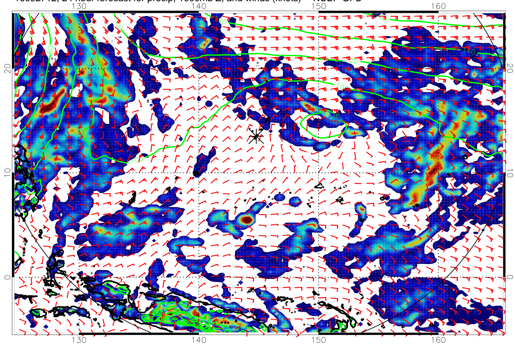
16092712, 24 hour forecast for precip, 1000mb Z, and winds (knots) -- NCEP GFS
