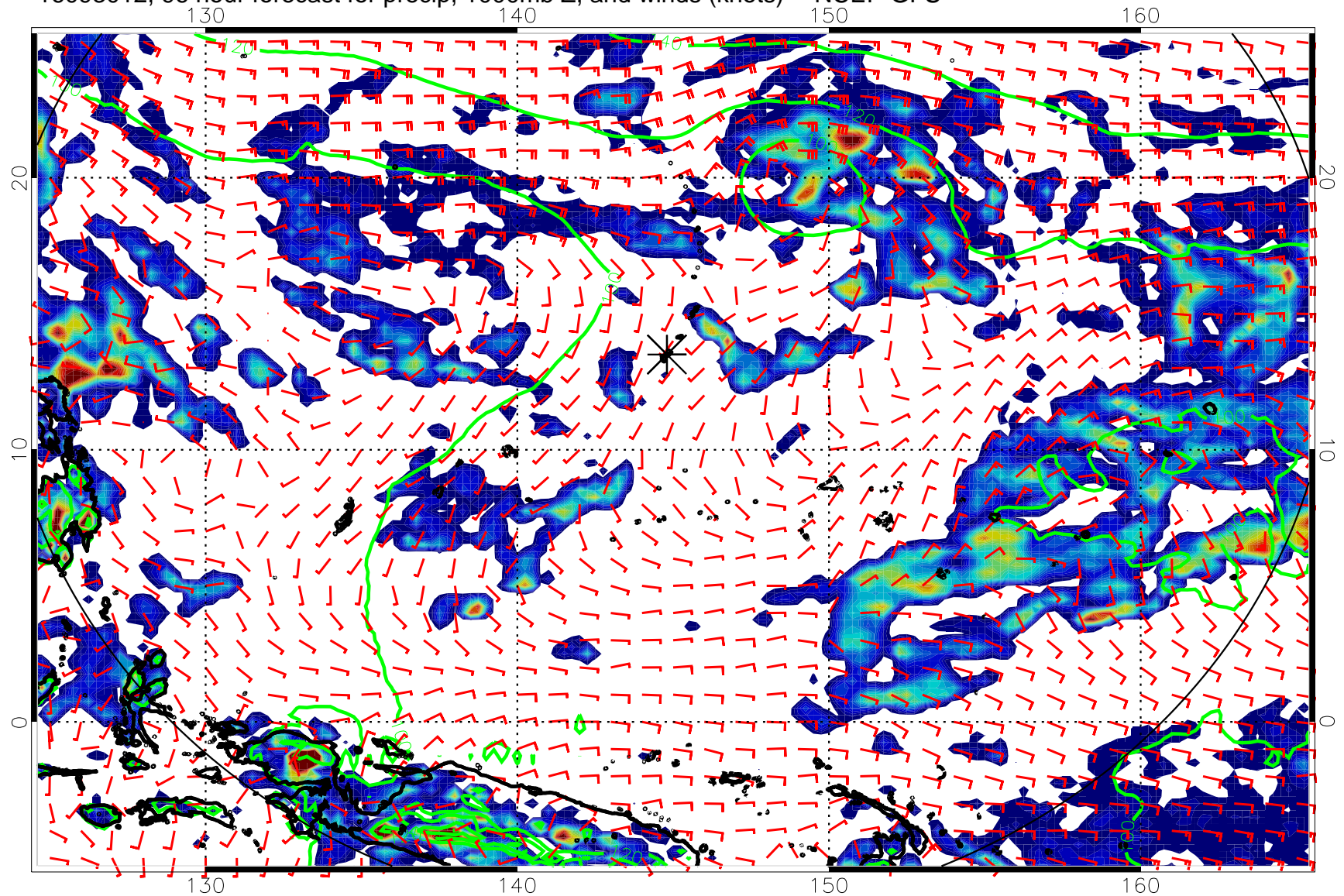
16093012, 96 hour forecast for precip, 1000mb Z, and winds (knots) -- NCEP GFS
