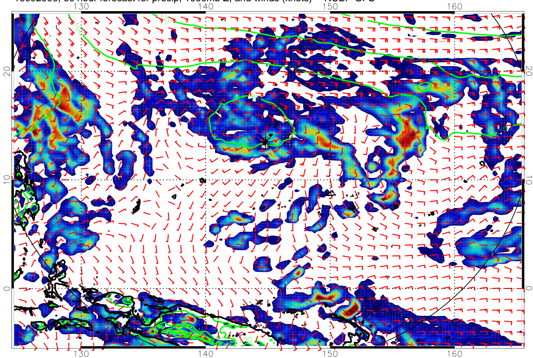
16092900, 60 hour forecast for precip, 1000mb Z, and winds (knots) -- NCEP GFS
