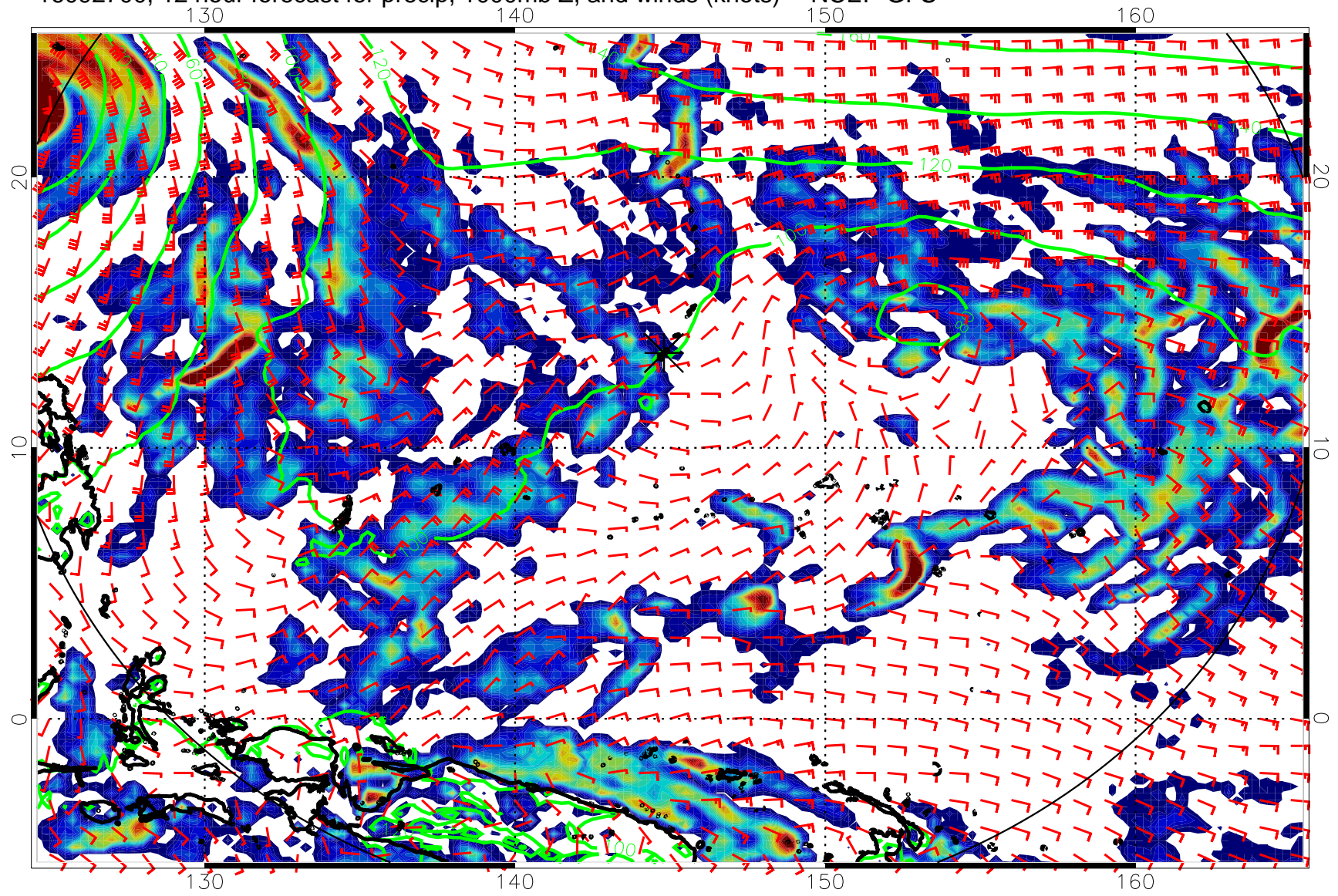
16092700, 12 hour forecast for precip, 1000mb Z, and winds (knots) -- NCEP GFS
