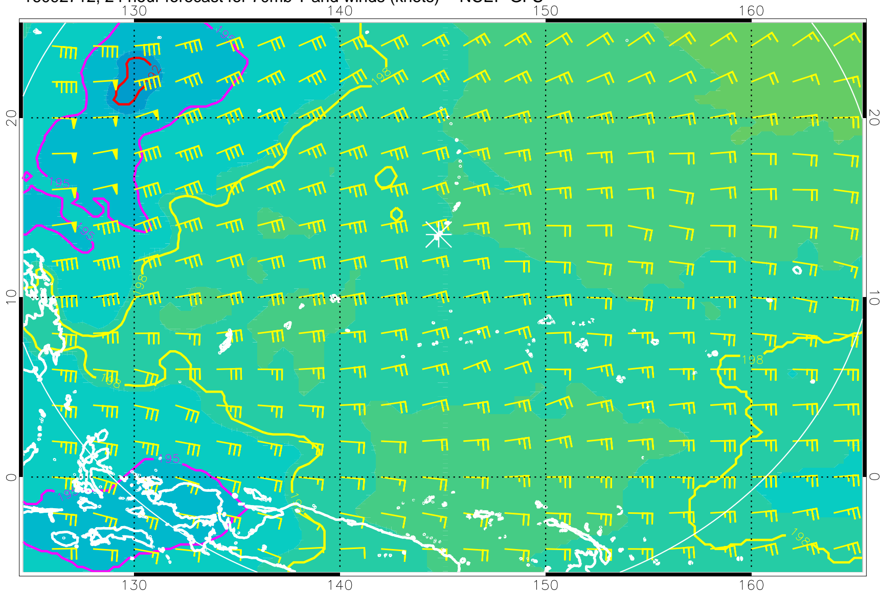
16092712, 24 hour forecast for 70mb T and winds (knots) -- NCEP GFS
