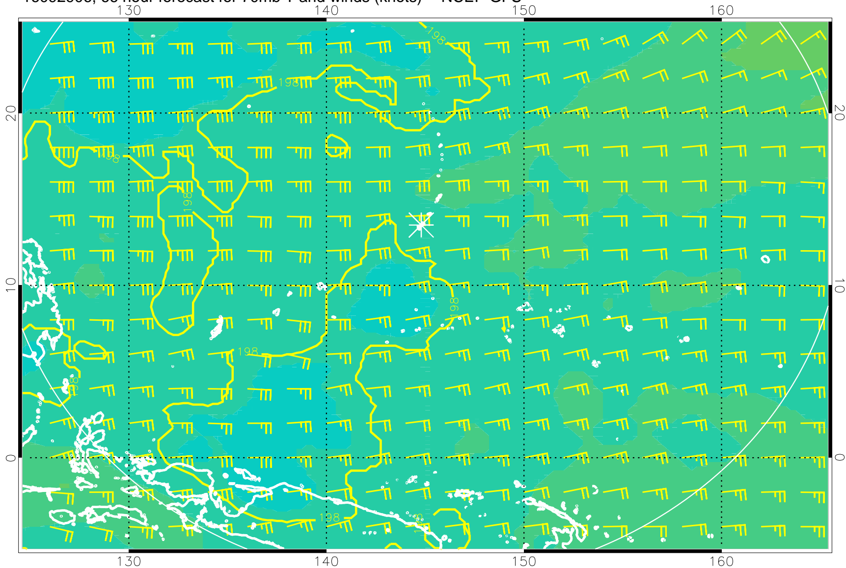
16092906, 66 hour forecast for 70mb T and winds (knots) -- NCEP GFS
