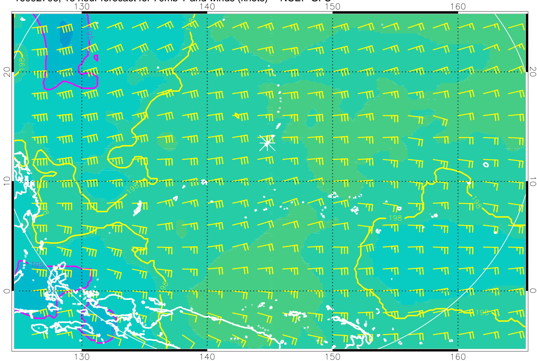
16092706, 18 hour forecast for 70mb T and winds (knots) -- NCEP GFS
