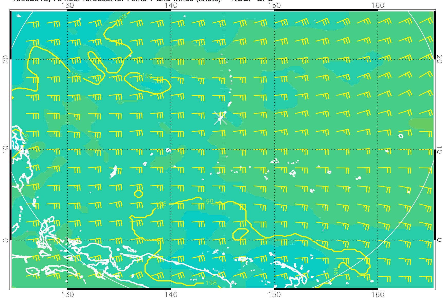
16092918, 78 hour forecast for 70mb T and winds (knots) -- NCEP GFS
