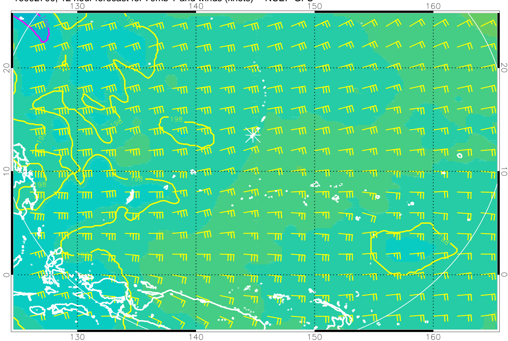
16092700, 12 hour forecast for 70mb T and winds (knots) -- NCEP GFS
