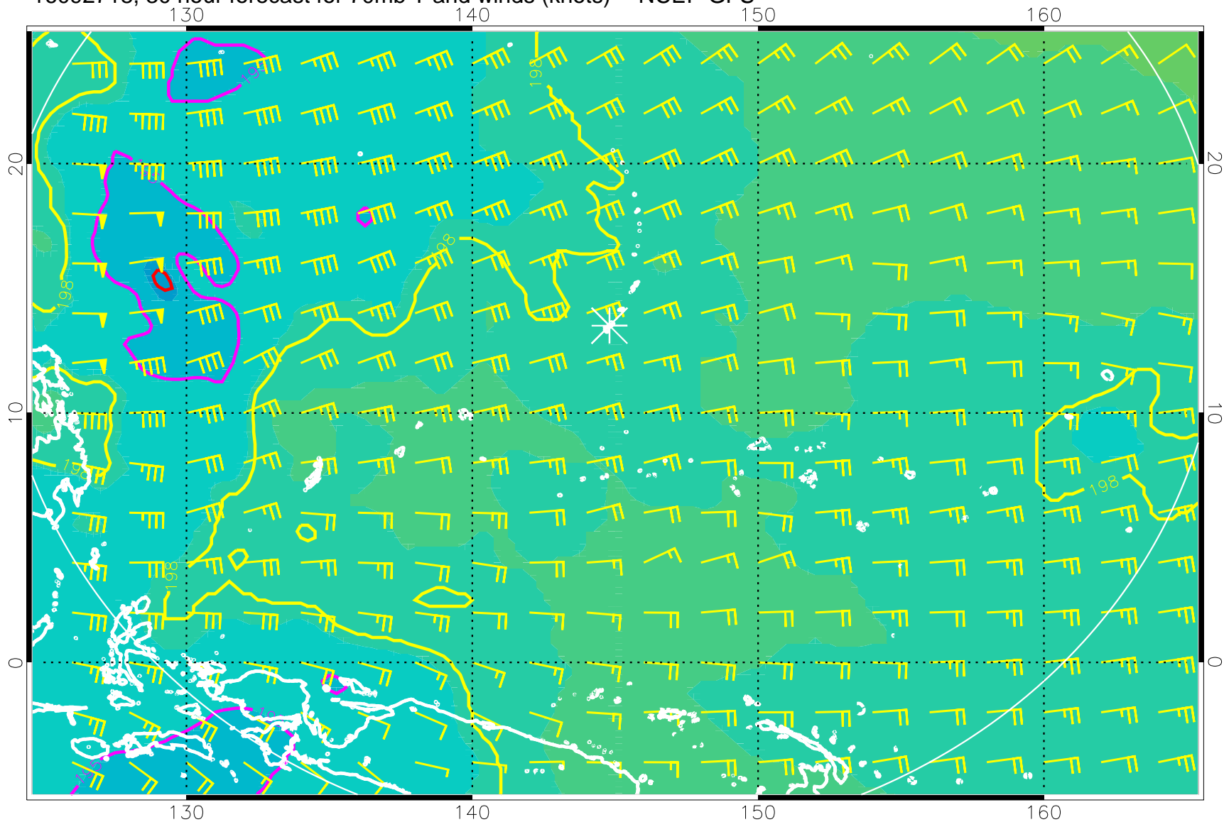
16092718, 30 hour forecast for 70mb T and winds (knots) -- NCEP GFS
