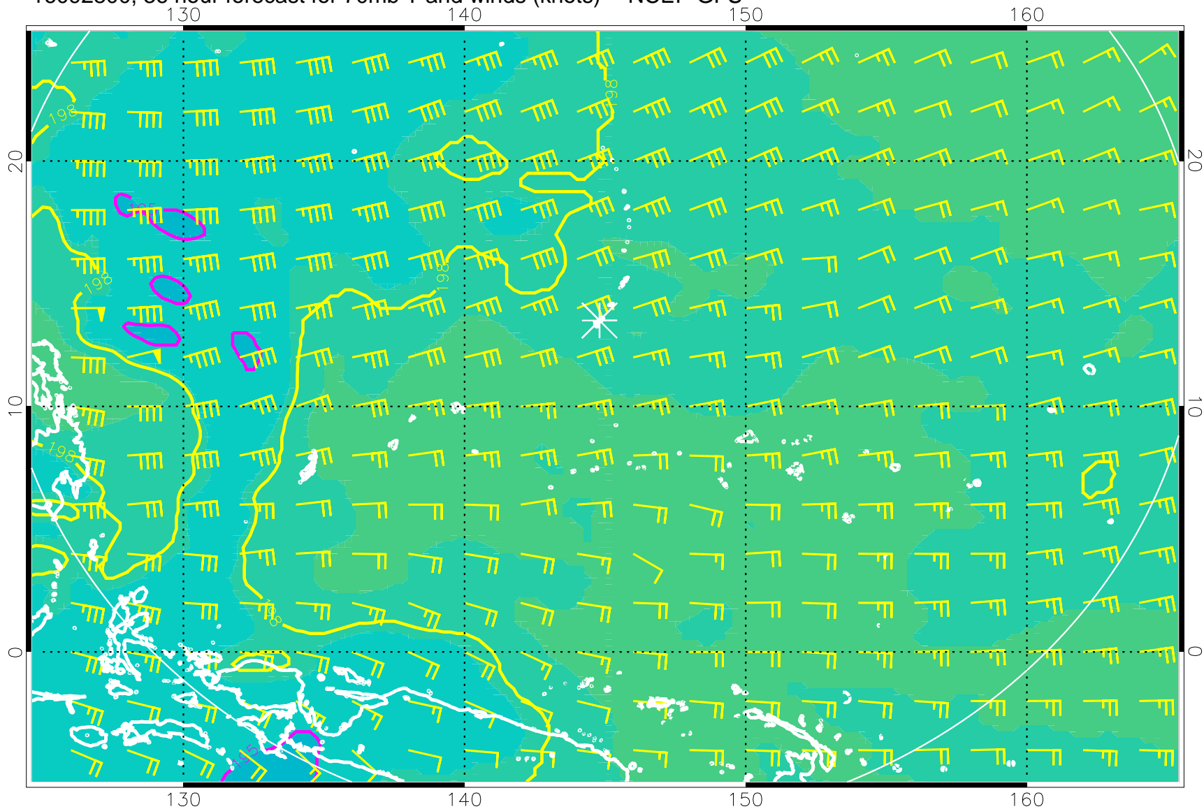
16092800, 36 hour forecast for 70mb T and winds (knots) -- NCEP GFS
