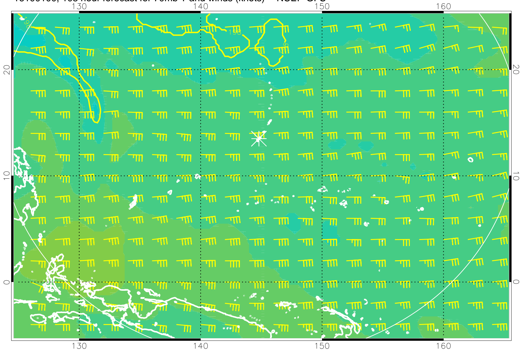
16100100, 108 hour forecast for 70mb T and winds (knots) -- NCEP GFS
