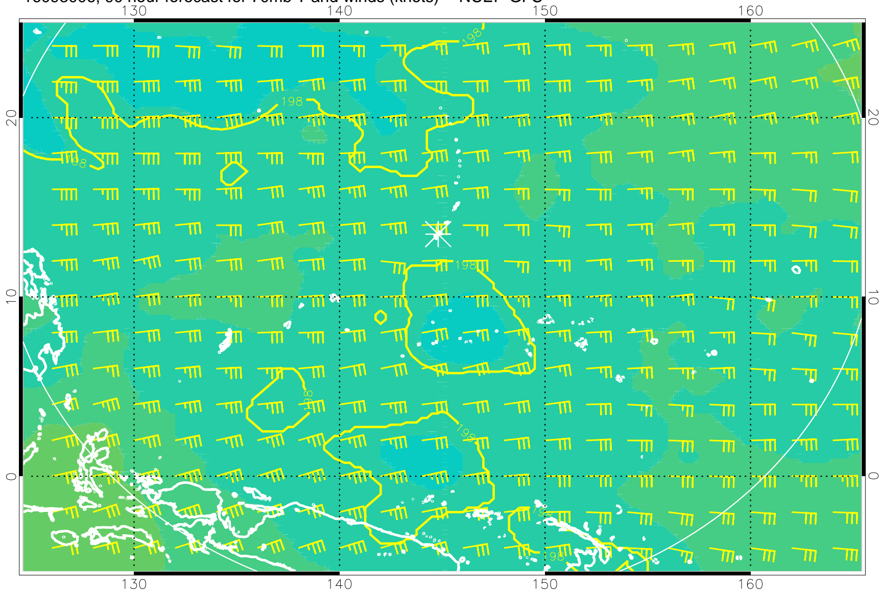
16093006, 90 hour forecast for 70mb T and winds (knots) -- NCEP GFS
