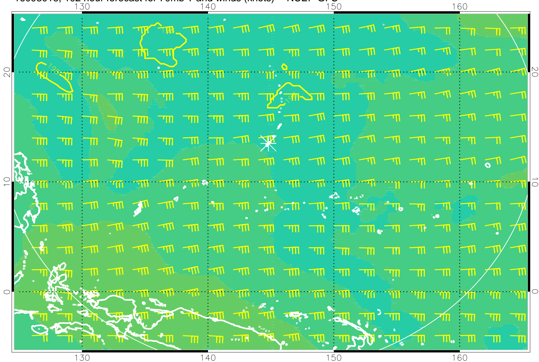
16093018, 102 hour forecast for 70mb T and winds (knots) -- NCEP GFS
