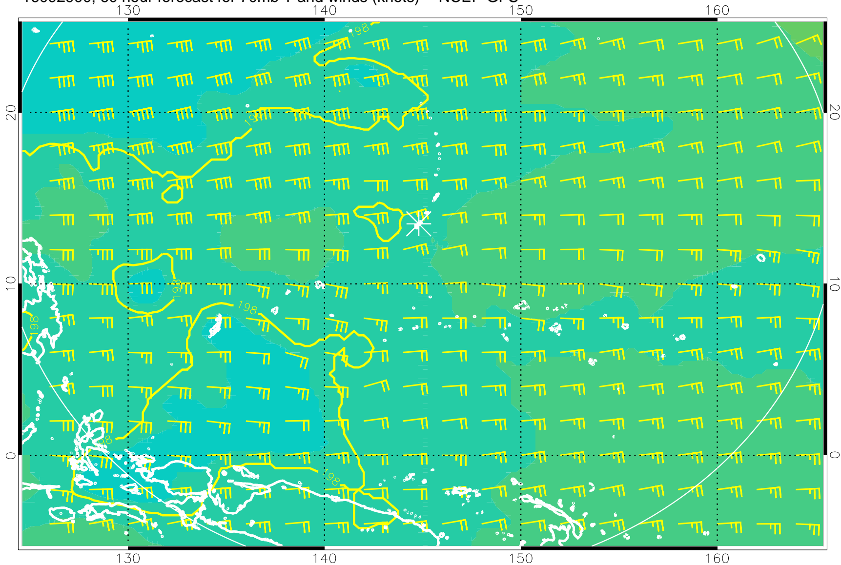
16092900, 60 hour forecast for 70mb T and winds (knots) -- NCEP GFS
