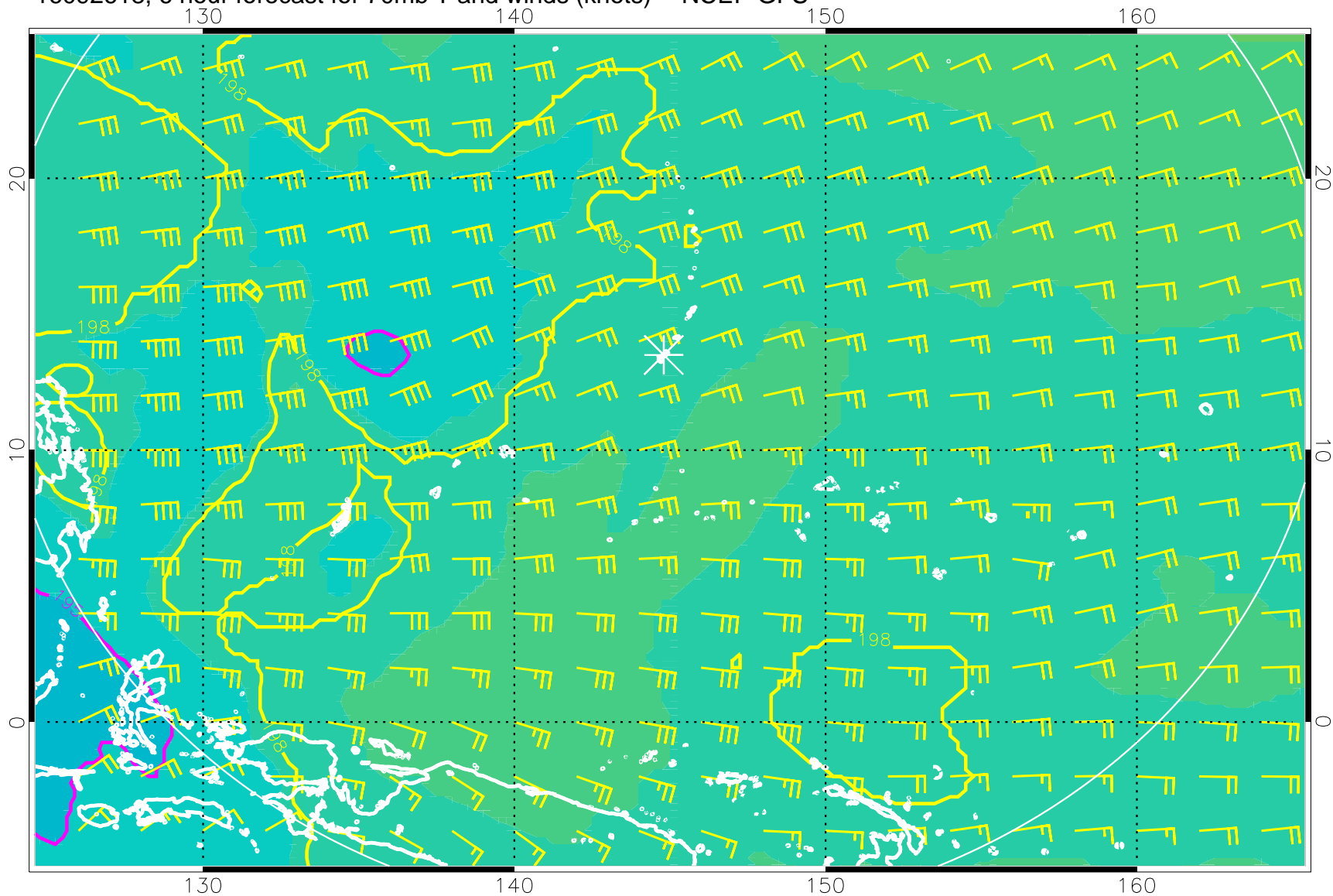
16092618, 6 hour forecast for 70mb T and winds (knots) -- NCEP GFS
