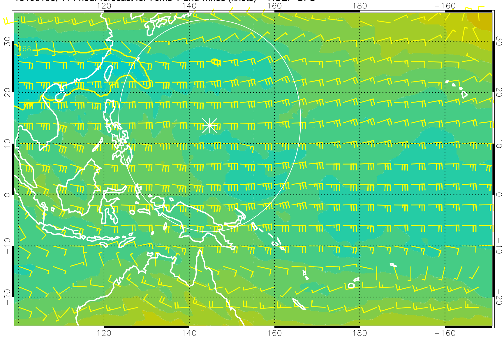
16100106, 114 hour forecast for 70mb T and winds (knots) -- NCEP GFS
