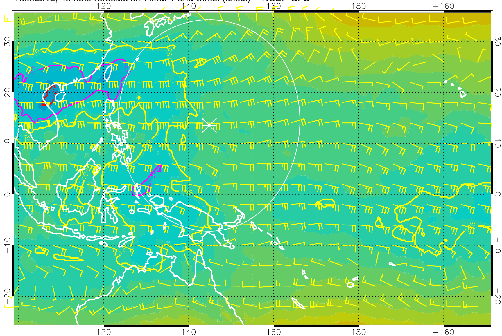
16092812, 48 hour forecast for 70mb T and winds (knots) -- NCEP GFS
