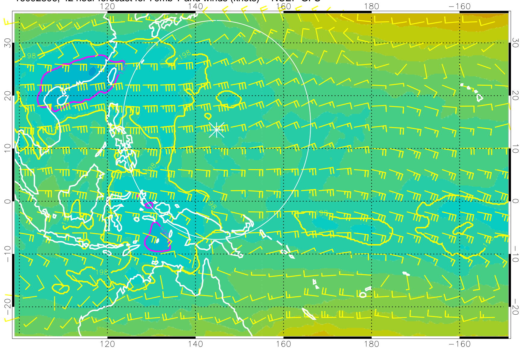
16092806, 42 hour forecast for 70mb T and winds (knots) -- NCEP GFS
