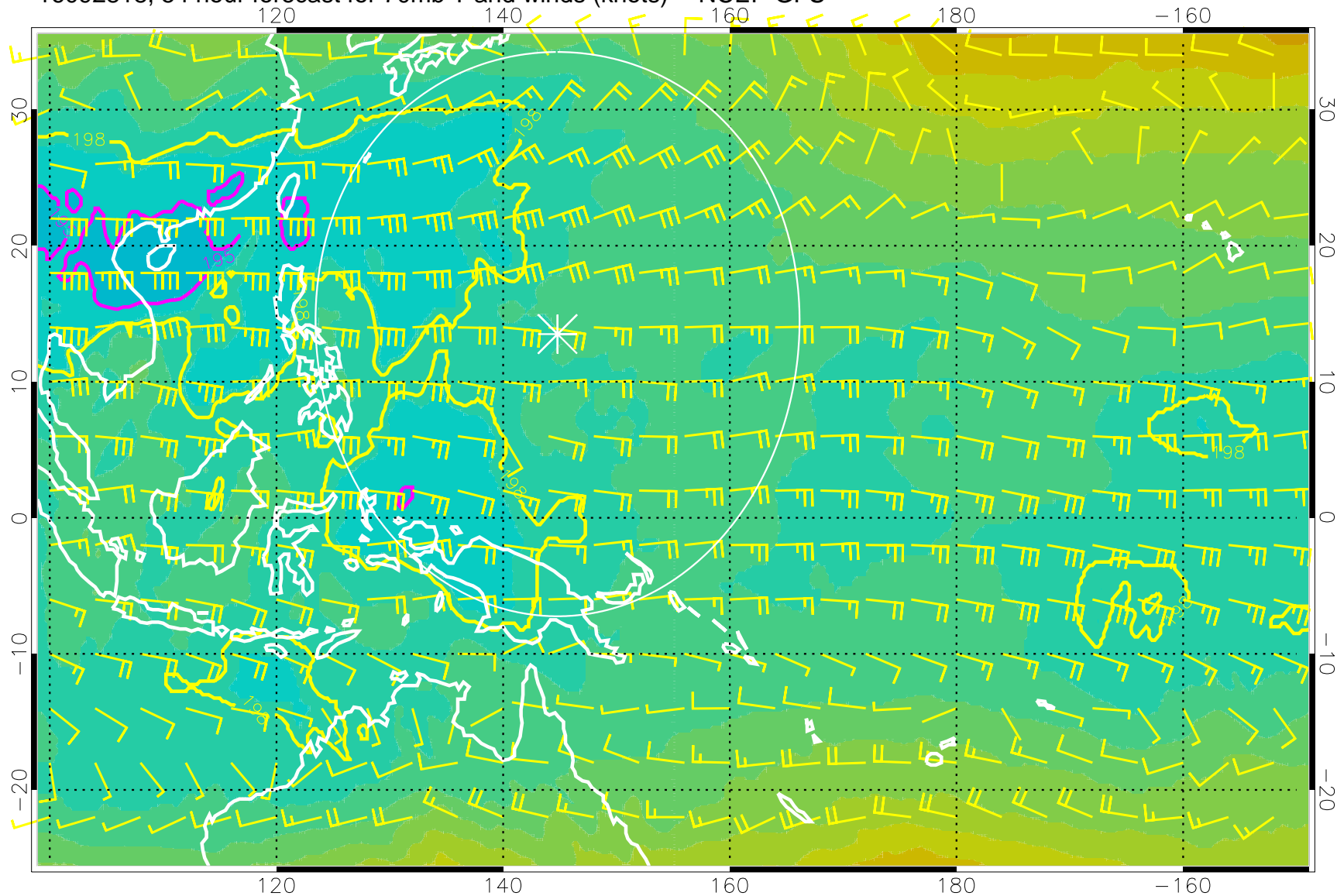
16092818, 54 hour forecast for 70mb T and winds (knots) -- NCEP GFS
