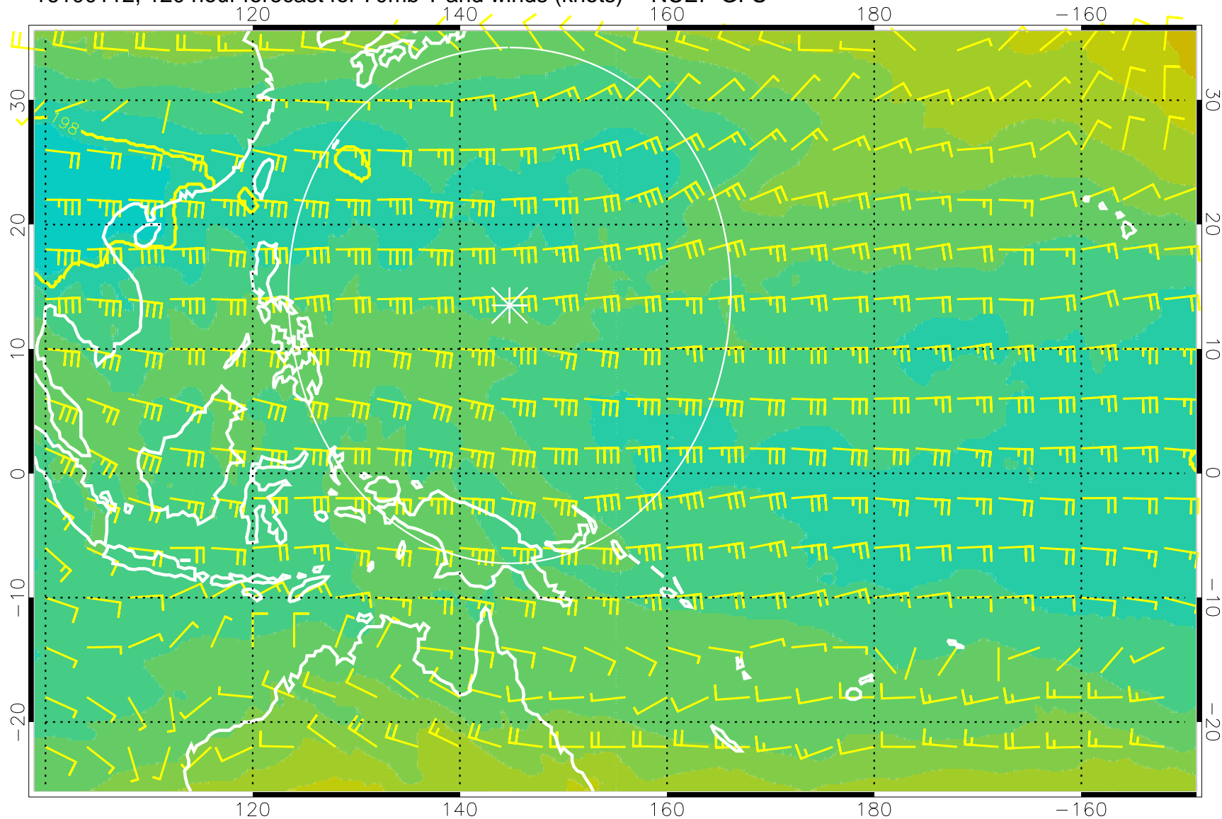
16100112, 120 hour forecast for 70mb T and winds (knots) -- NCEP GFS
