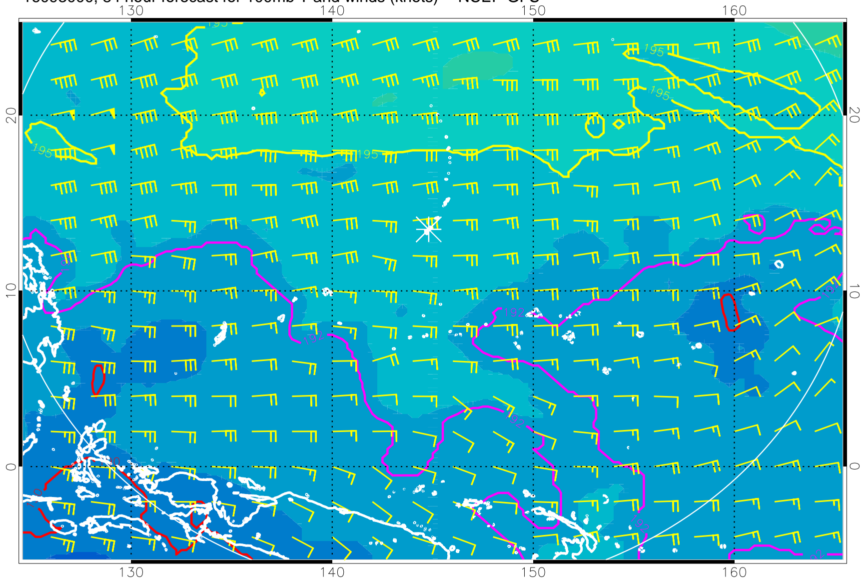
16093000, 84 hour forecast for 100mb T and winds (knots) -- NCEP GFS
