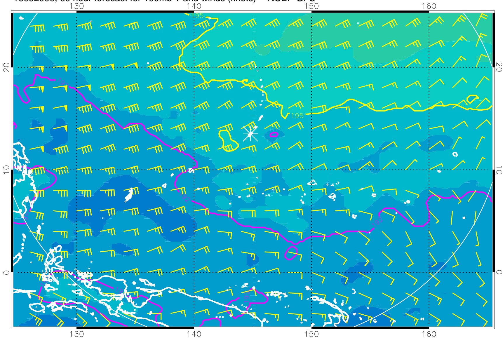
16092900, 60 hour forecast for 100mb T and winds (knots) -- NCEP GFS
