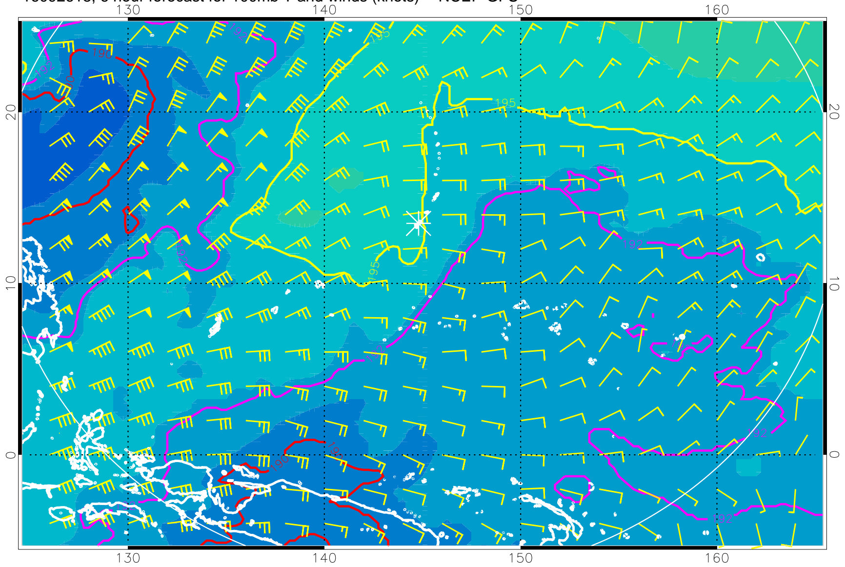
16092618, 6 hour forecast for 100mb T and winds (knots) -- NCEP GFS
