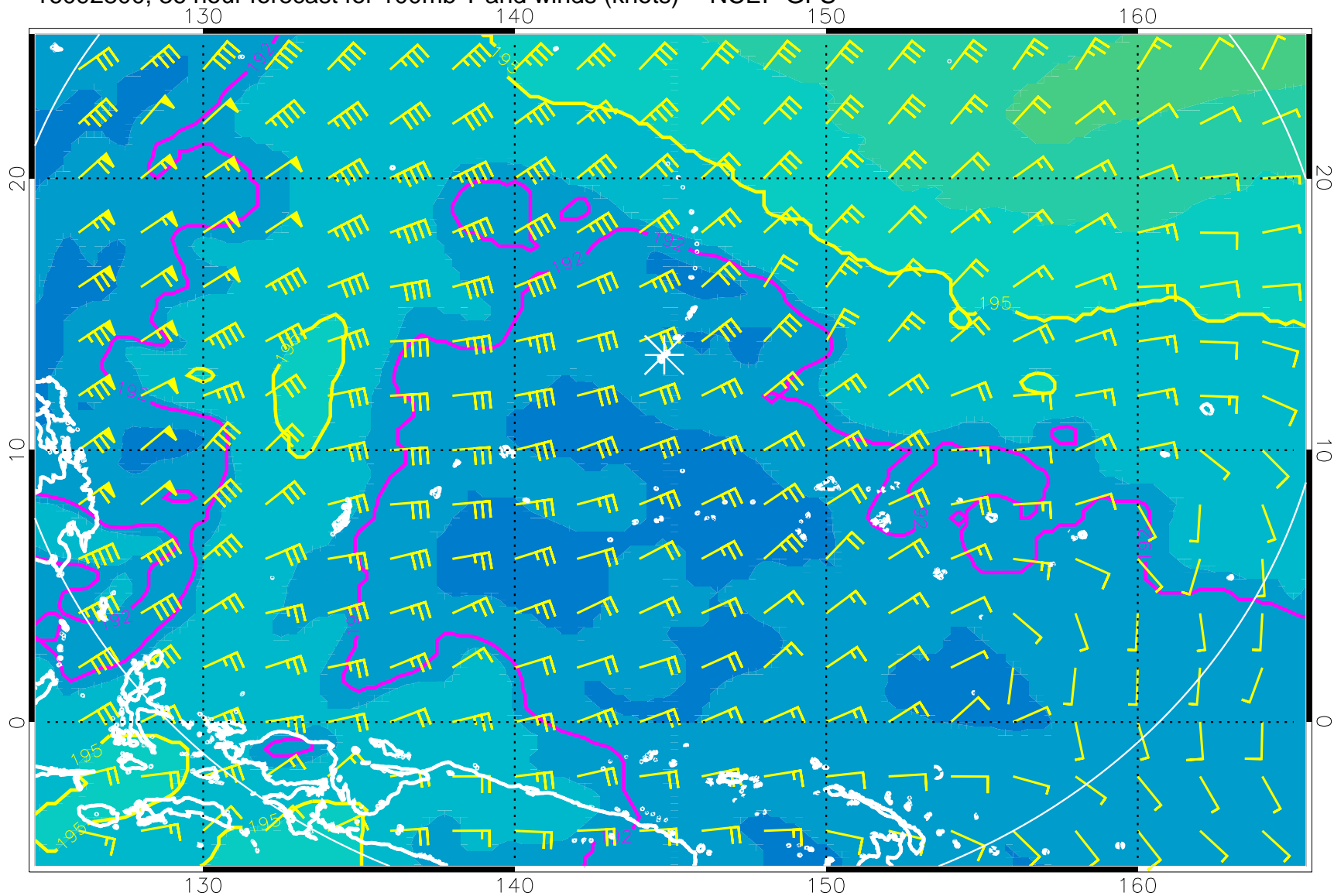
16092800, 36 hour forecast for 100mb T and winds (knots) -- NCEP GFS
