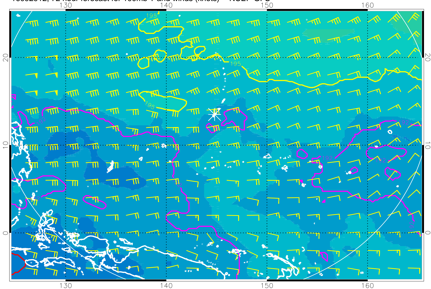
16092912, 72 hour forecast for 100mb T and winds (knots) -- NCEP GFS
