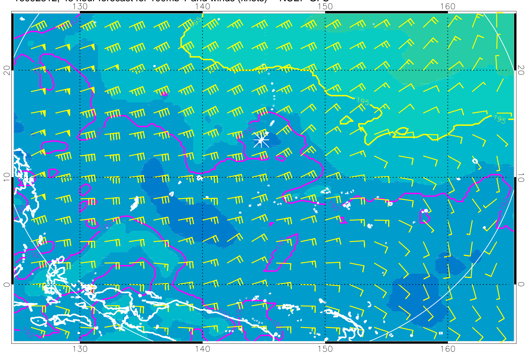
16092812, 48 hour forecast for 100mb T and winds (knots) -- NCEP GFS
