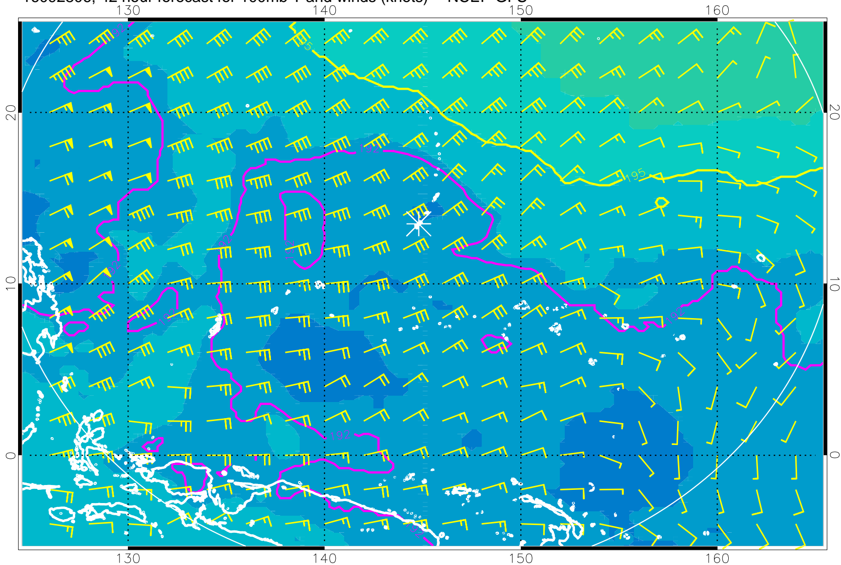
16092806, 42 hour forecast for 100mb T and winds (knots) -- NCEP GFS
