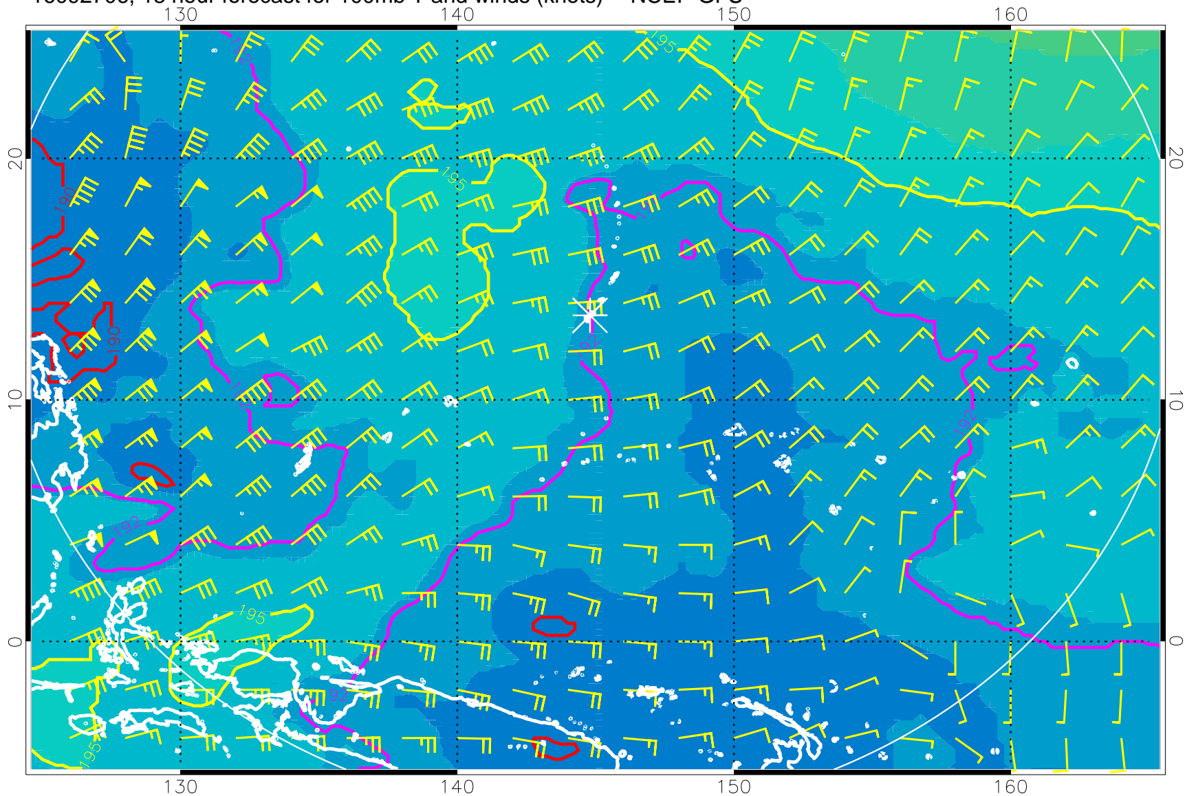
16092706, 18 hour forecast for 100mb T and winds (knots) -- NCEP GFS
