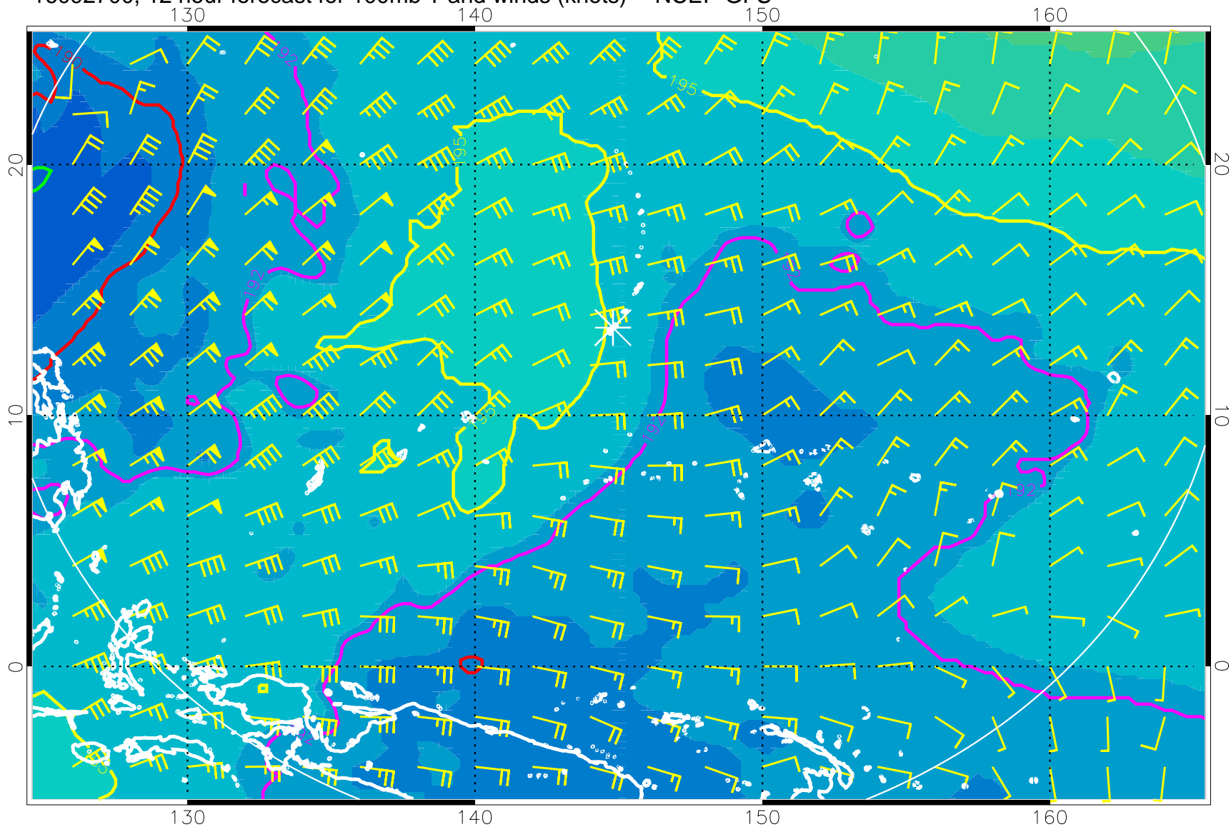
16092700, 12 hour forecast for 100mb T and winds (knots) -- NCEP GFS
