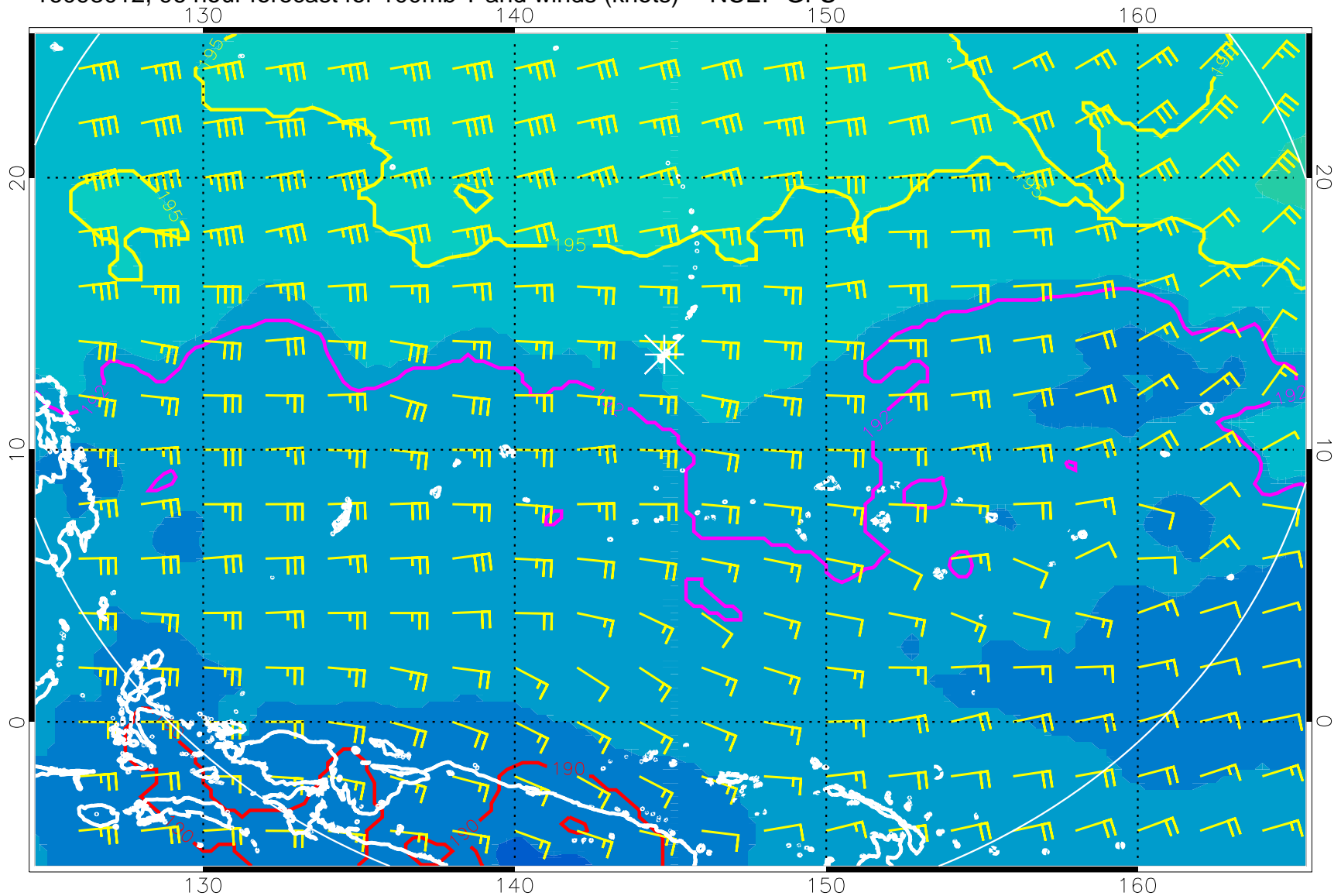
16093012, 96 hour forecast for 100mb T and winds (knots) -- NCEP GFS
