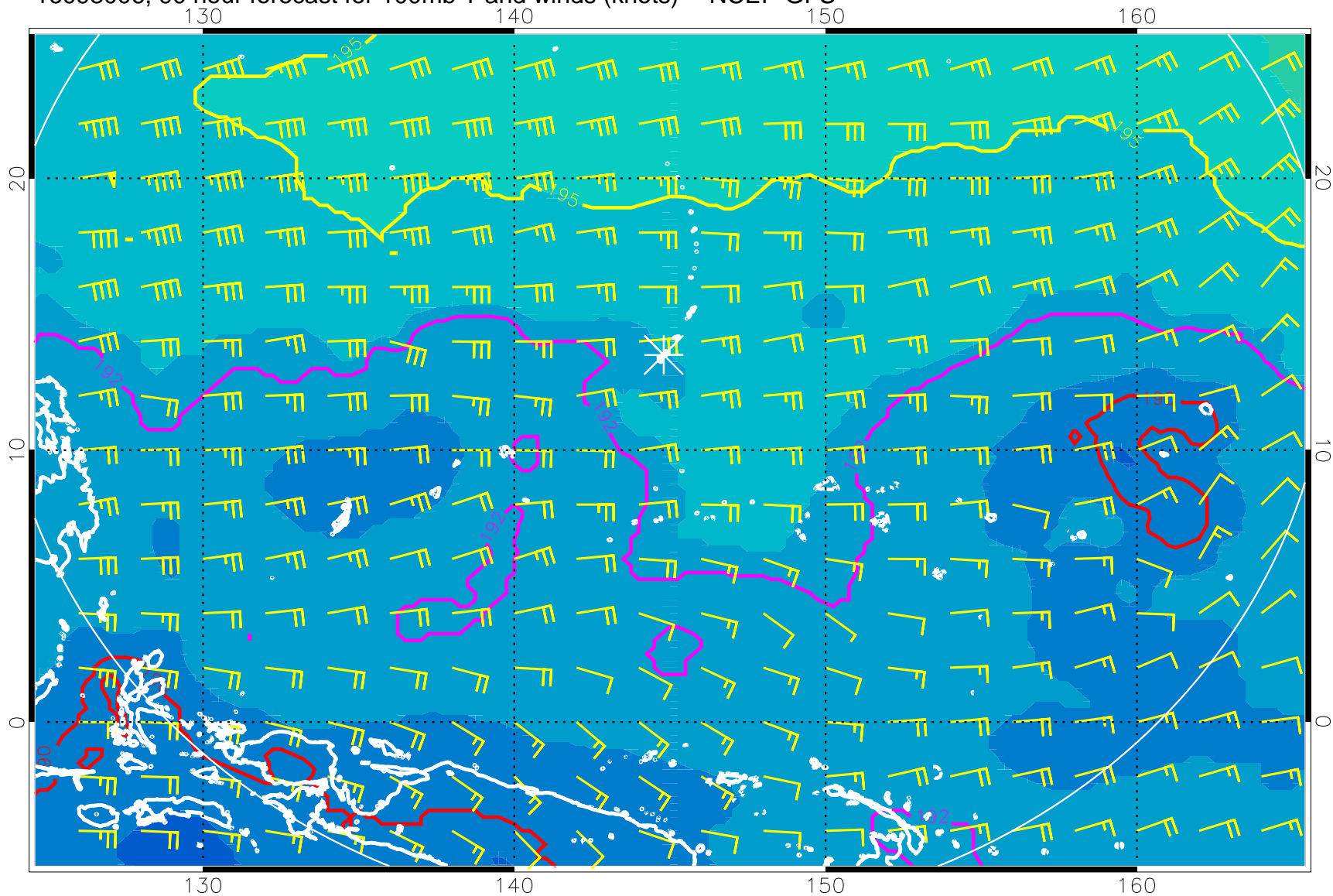
16093006, 90 hour forecast for 100mb T and winds (knots) -- NCEP GFS
