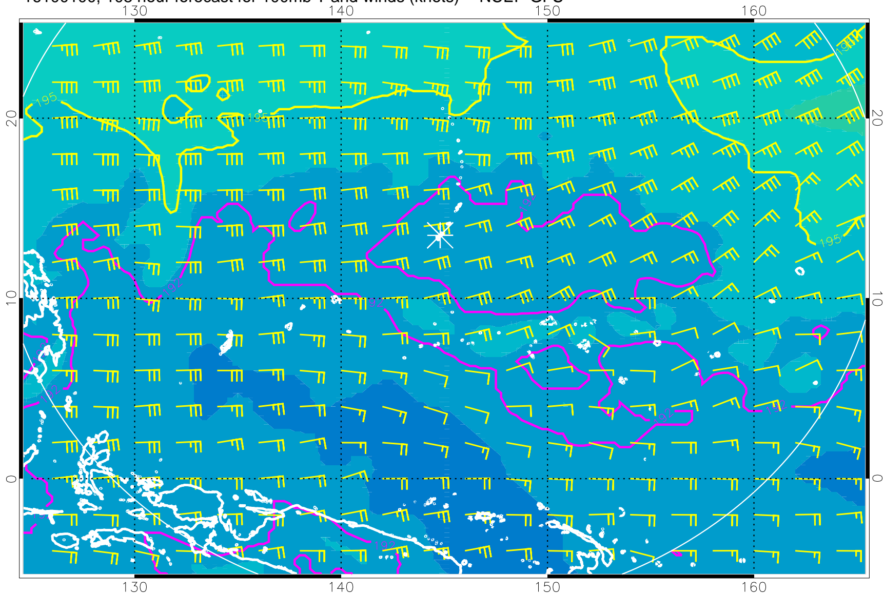
16100100, 108 hour forecast for 100mb T and winds (knots) -- NCEP GFS
