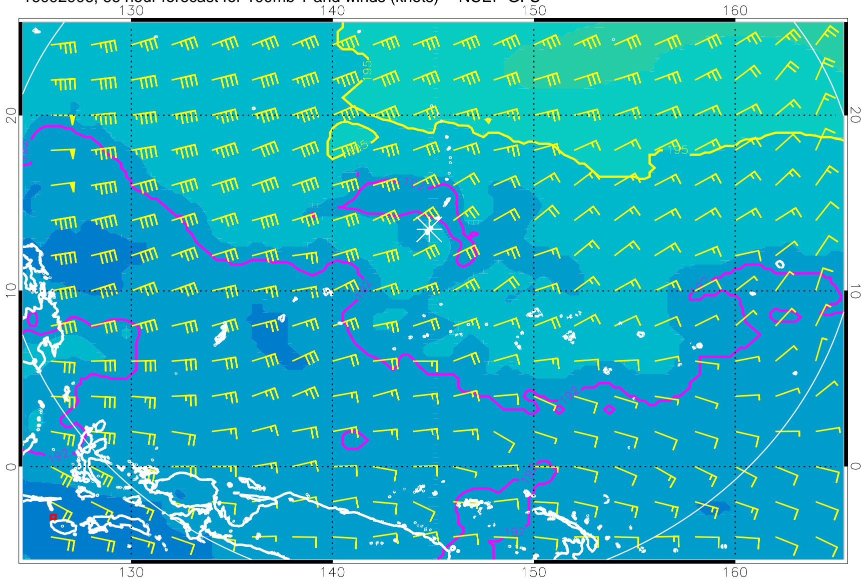
16092906, 66 hour forecast for 100mb T and winds (knots) -- NCEP GFS
