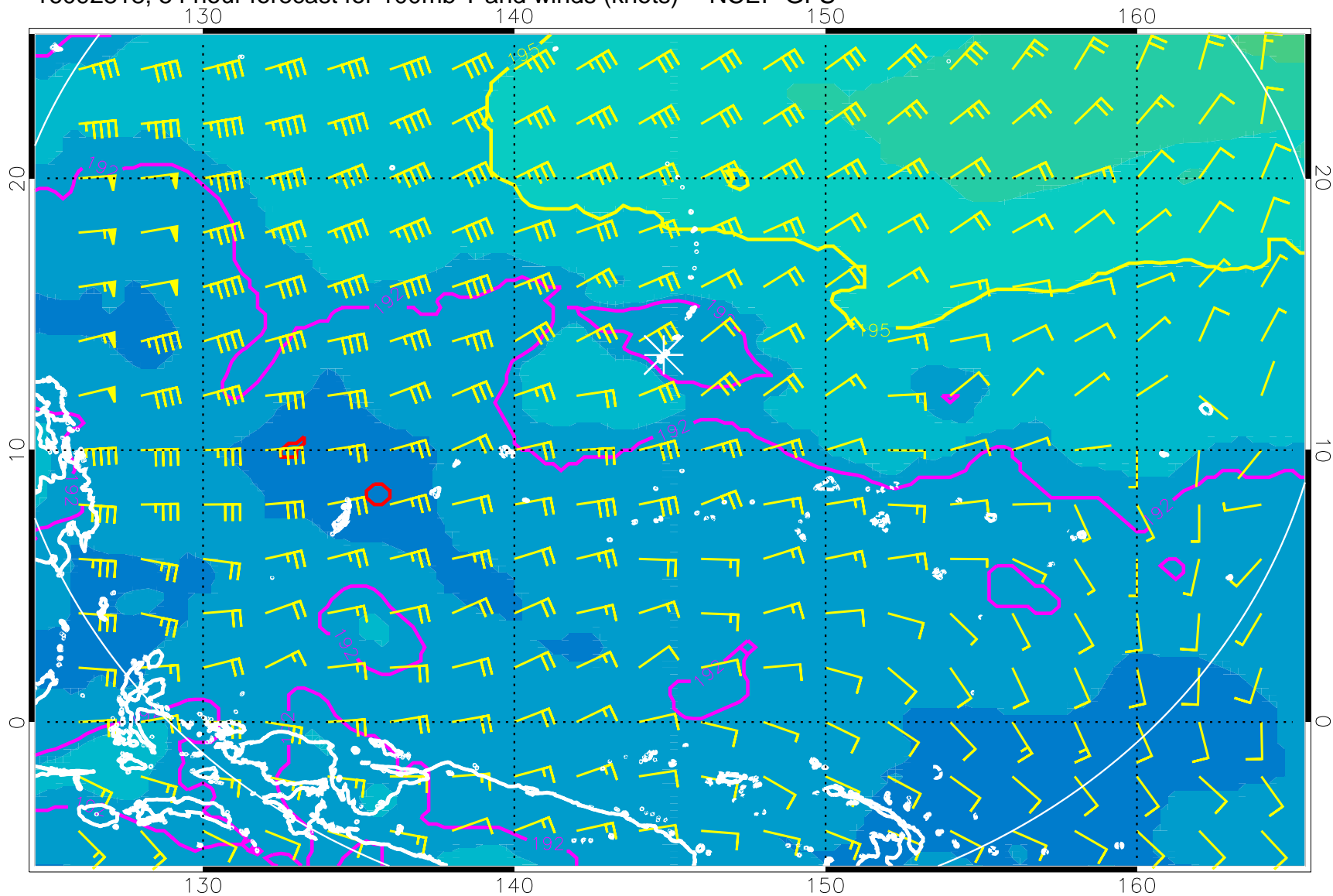
16092818, 54 hour forecast for 100mb T and winds (knots) -- NCEP GFS
