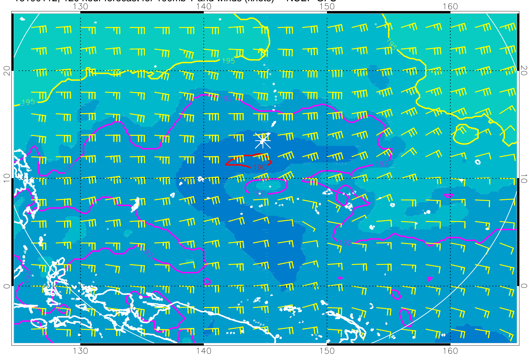
16100112, 120 hour forecast for 100mb T and winds (knots) -- NCEP GFS
