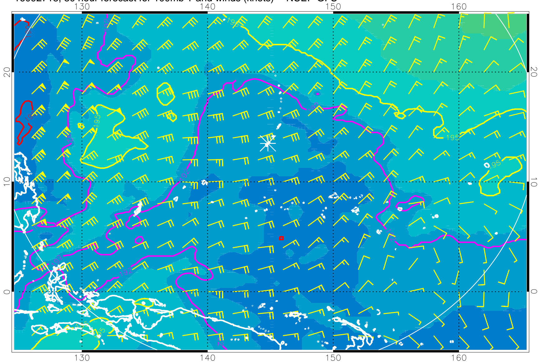
16092718, 30 hour forecast for 100mb T and winds (knots) -- NCEP GFS
