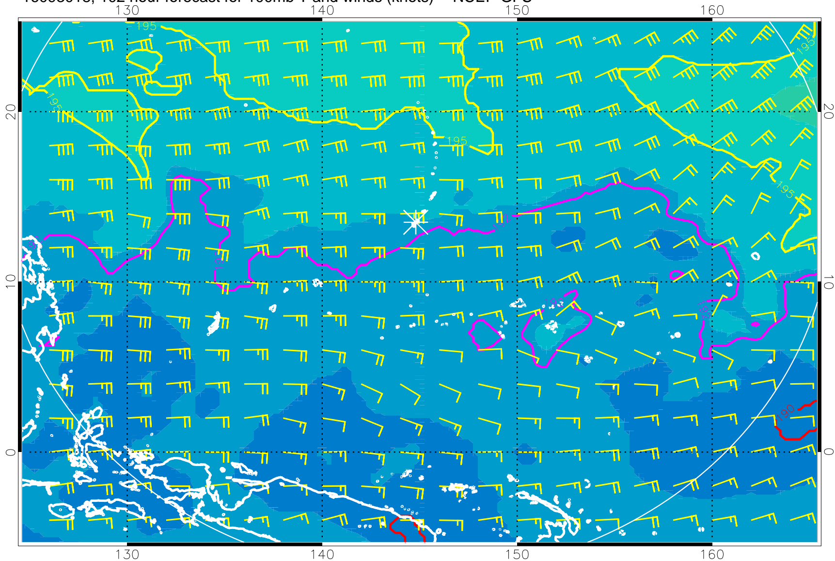
16093018, 102 hour forecast for 100mb T and winds (knots) -- NCEP GFS
