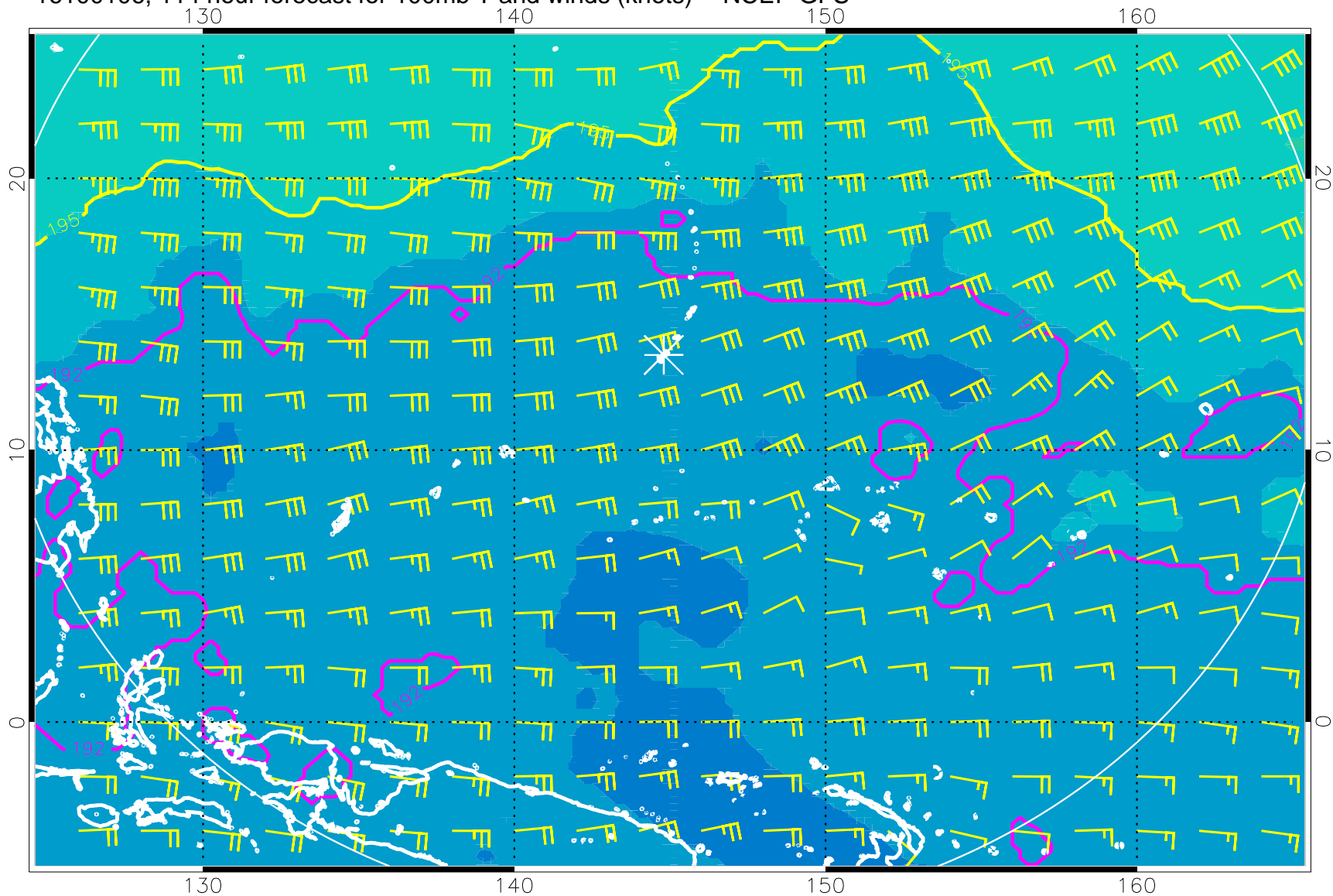
16100106, 114 hour forecast for 100mb T and winds (knots) -- NCEP GFS
