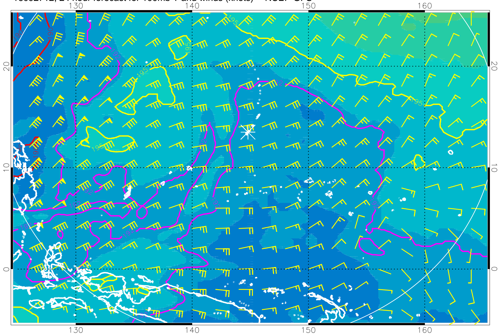
16092712, 24 hour forecast for 100mb T and winds (knots) -- NCEP GFS
