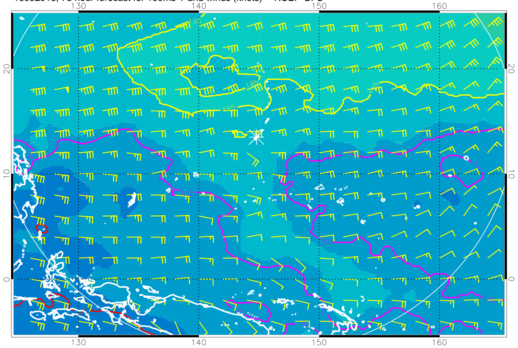
16092918, 78 hour forecast for 100mb T and winds (knots) -- NCEP GFS
