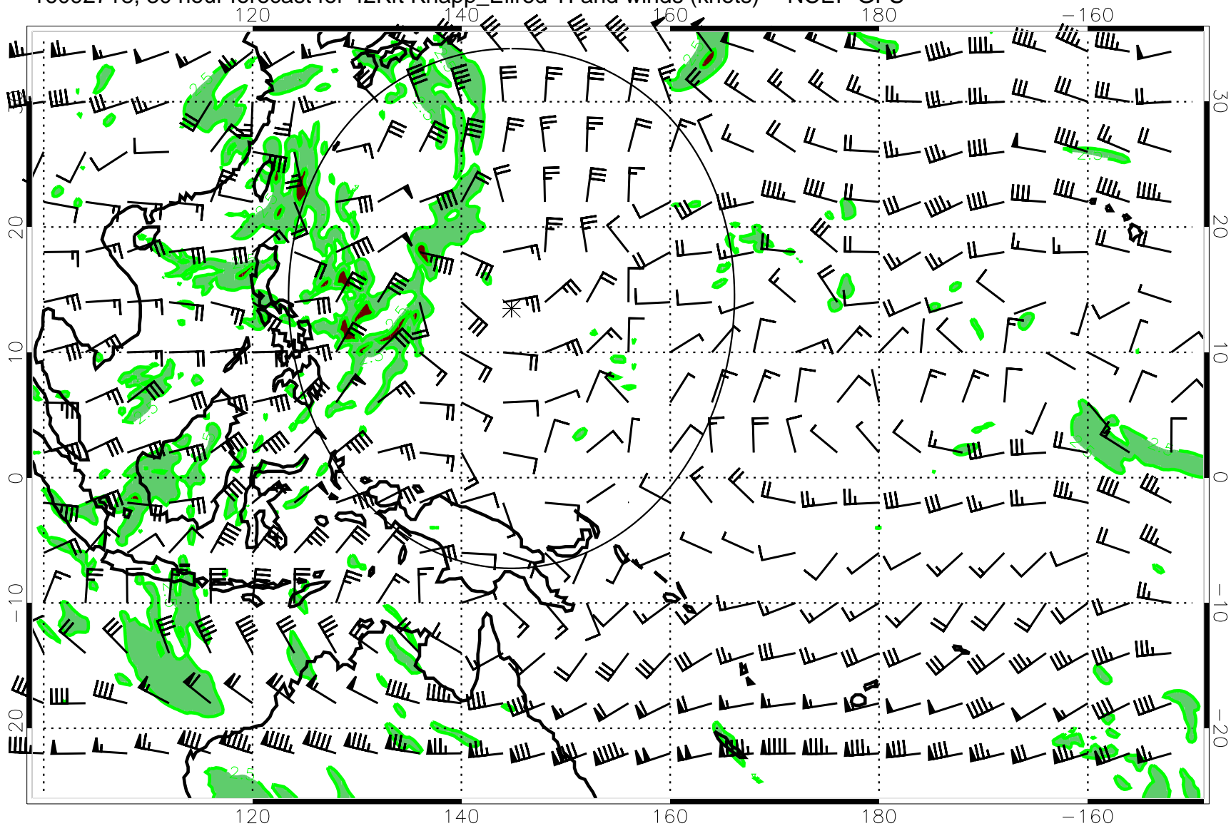
16092718, 30 hour forecast for 42Kft Knapp_Ellrod TI and winds (knots) -- NCEP GFS
