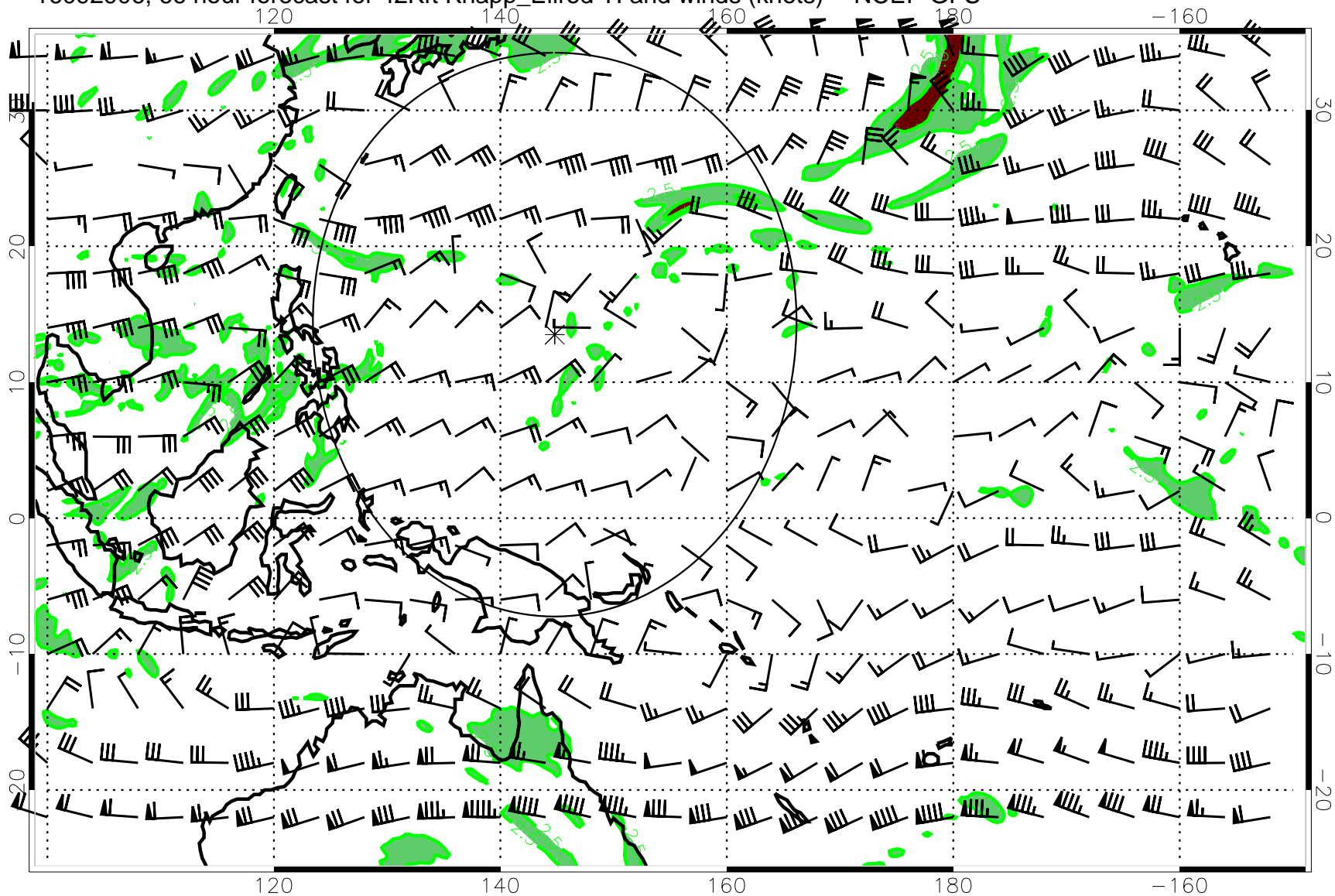
16092906, 66 hour forecast for 42Kft Knapp_Ellrod TI and winds (knots) -- NCEP GFS
