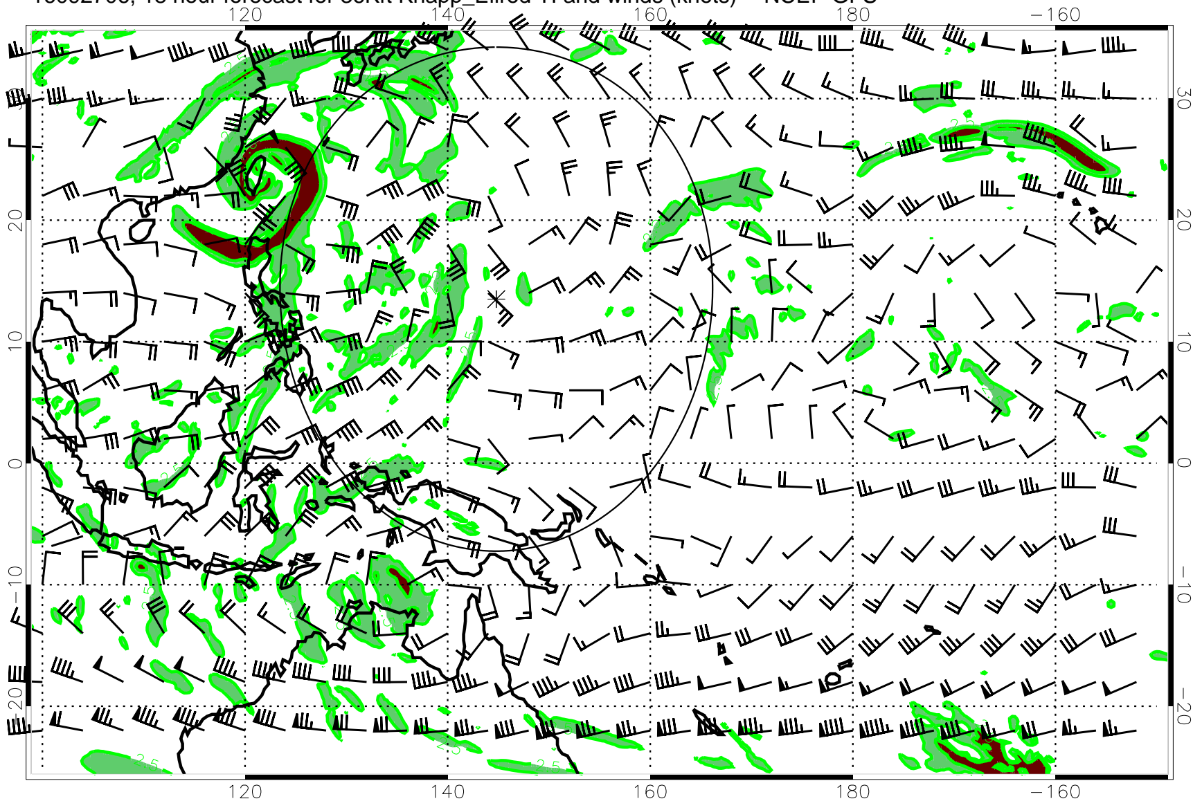
16092706, 18 hour forecast for 36Kft Knapp_Ellrod TI and winds (knots) -- NCEP GFS
