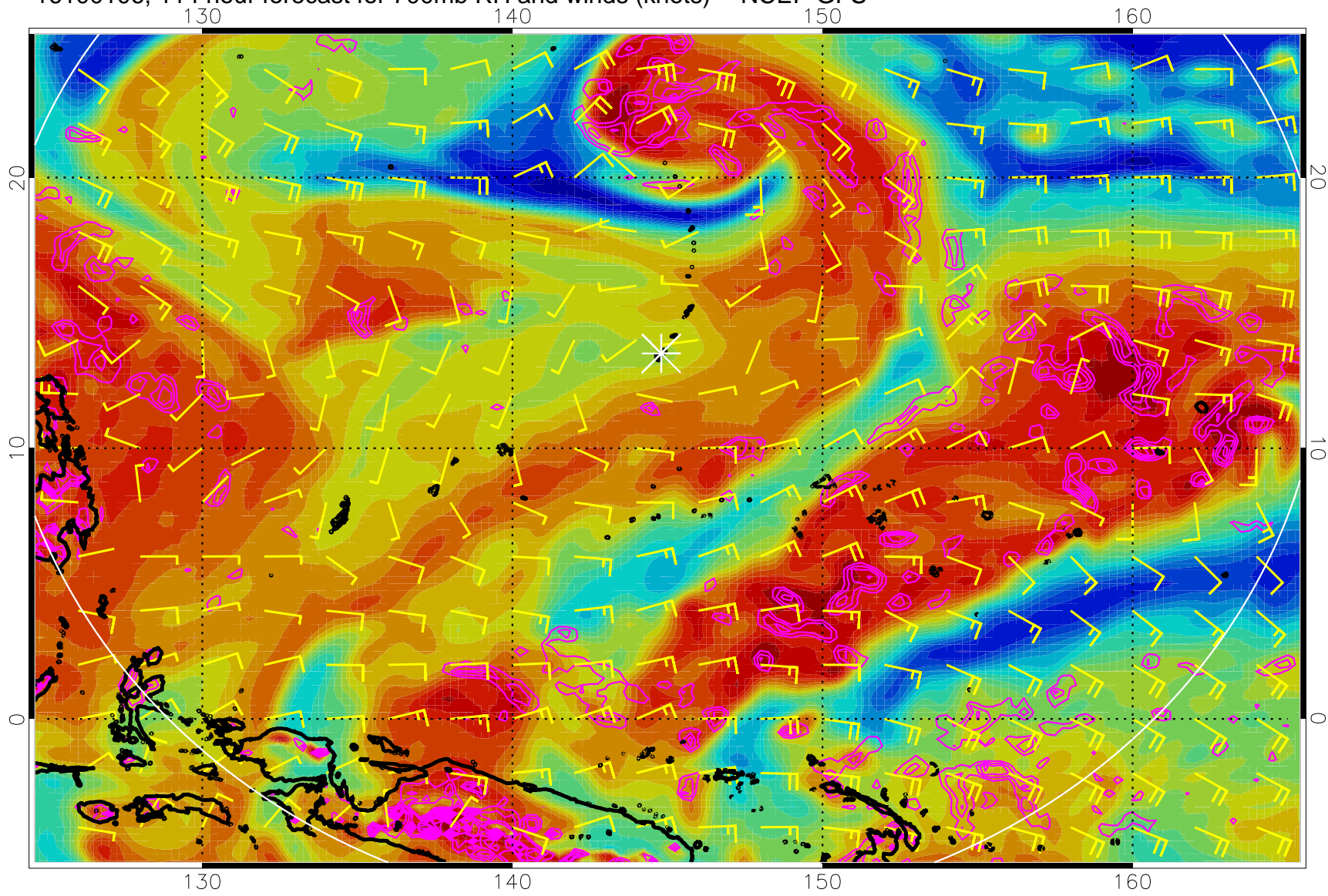
16100106, 114 hour forecast for 700mb RH and winds (knots) -- NCEP GFS
