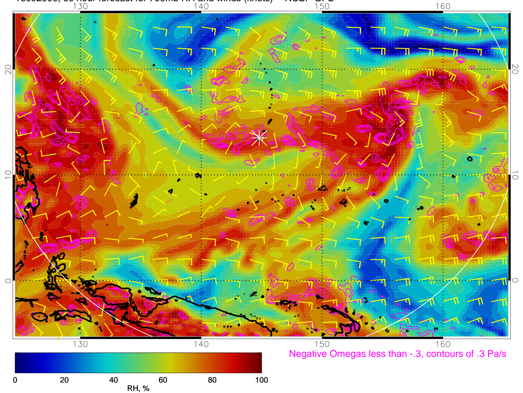
16092900, 60 hour forecast for 700mb RH and winds (knots) -- NCEP GFS
