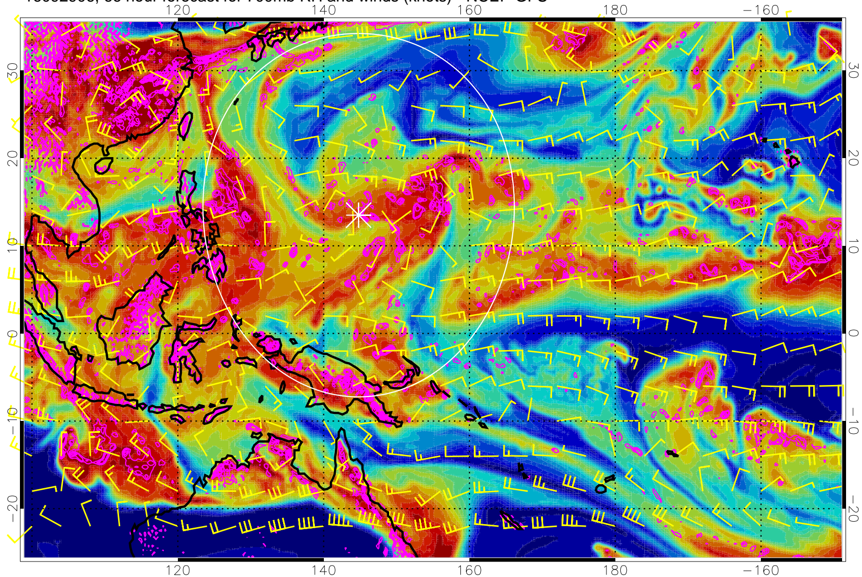
16092906, 66 hour forecast for 700mb RH and winds (knots) - NCEP GFS
