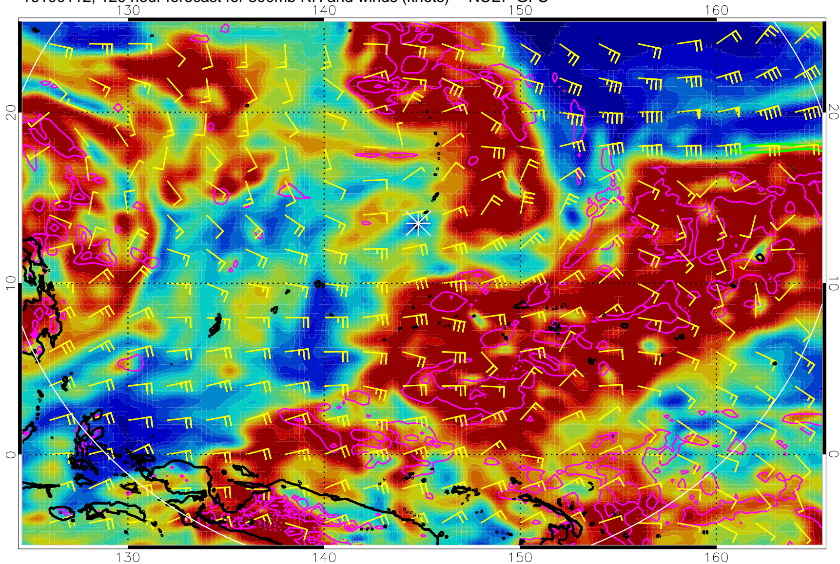
16100112, 120 hour forecast for 300mb RH and winds (knots) -- NCEP GFS
