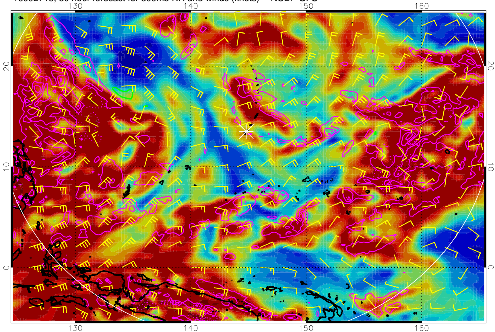
16092718, 30 hour forecast for 300mb RH and winds (knots) -- NCEP GFS
