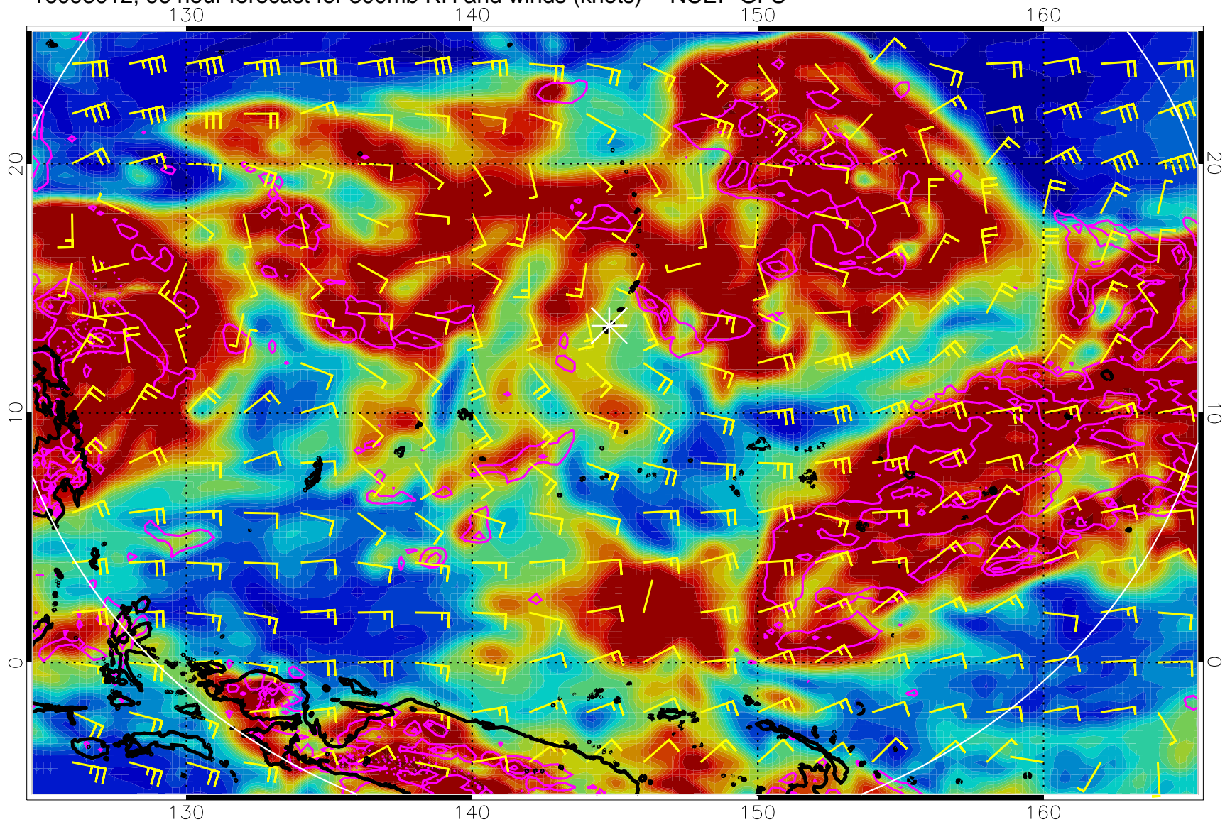
16093012, 96 hour forecast for 300mb RH and winds (knots) -- NCEP GFS
