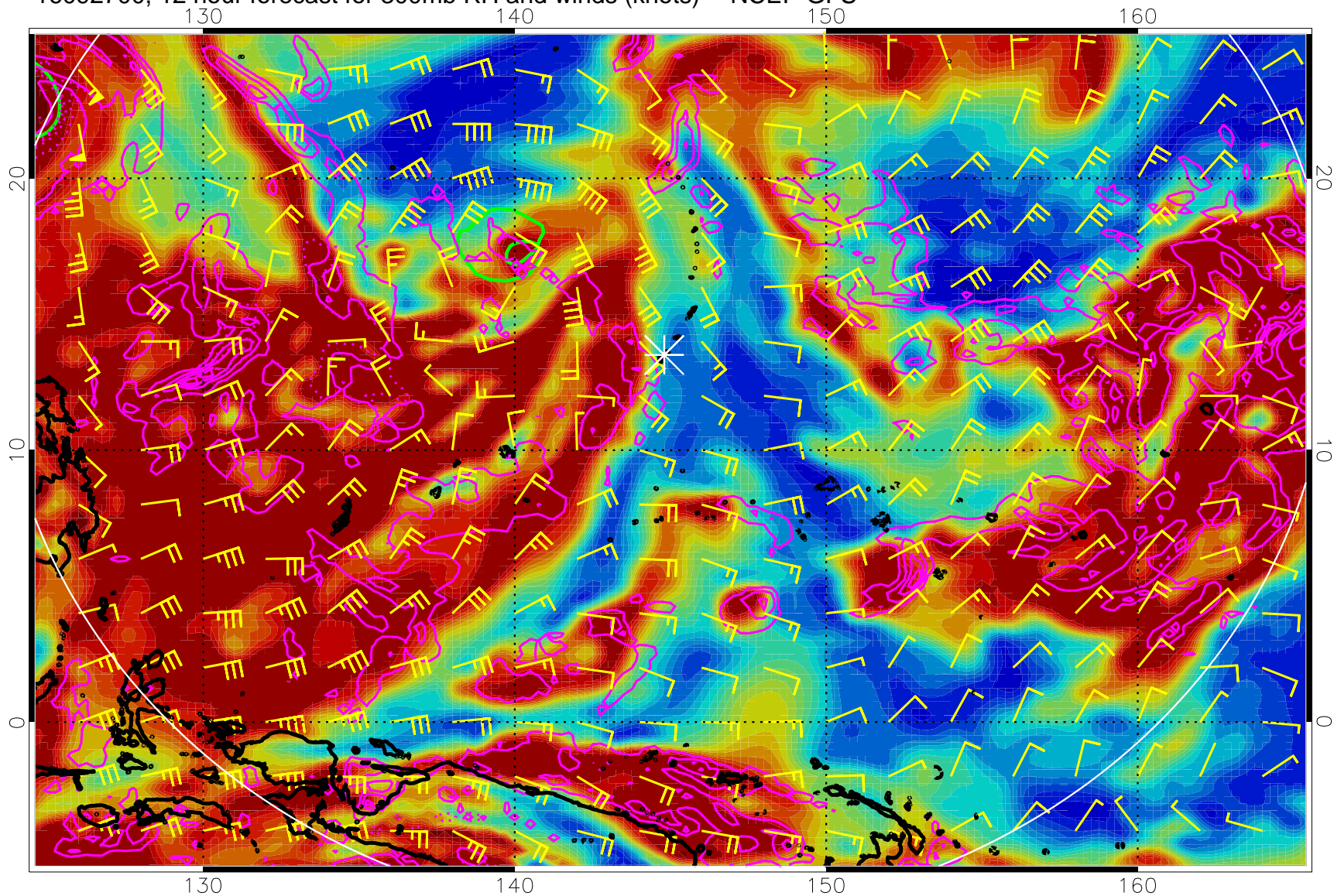
16092700, 12 hour forecast for 300mb RH and winds (knots) -- NCEP GFS
