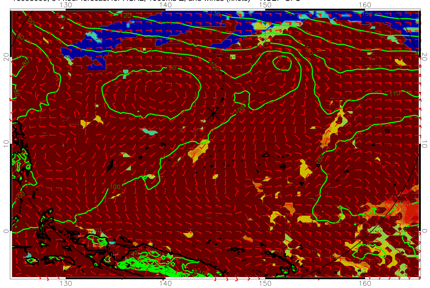
16093000, 84 hour forecast for HCAL, 1000mb Z, and winds (knots) -- NCEP GFS
