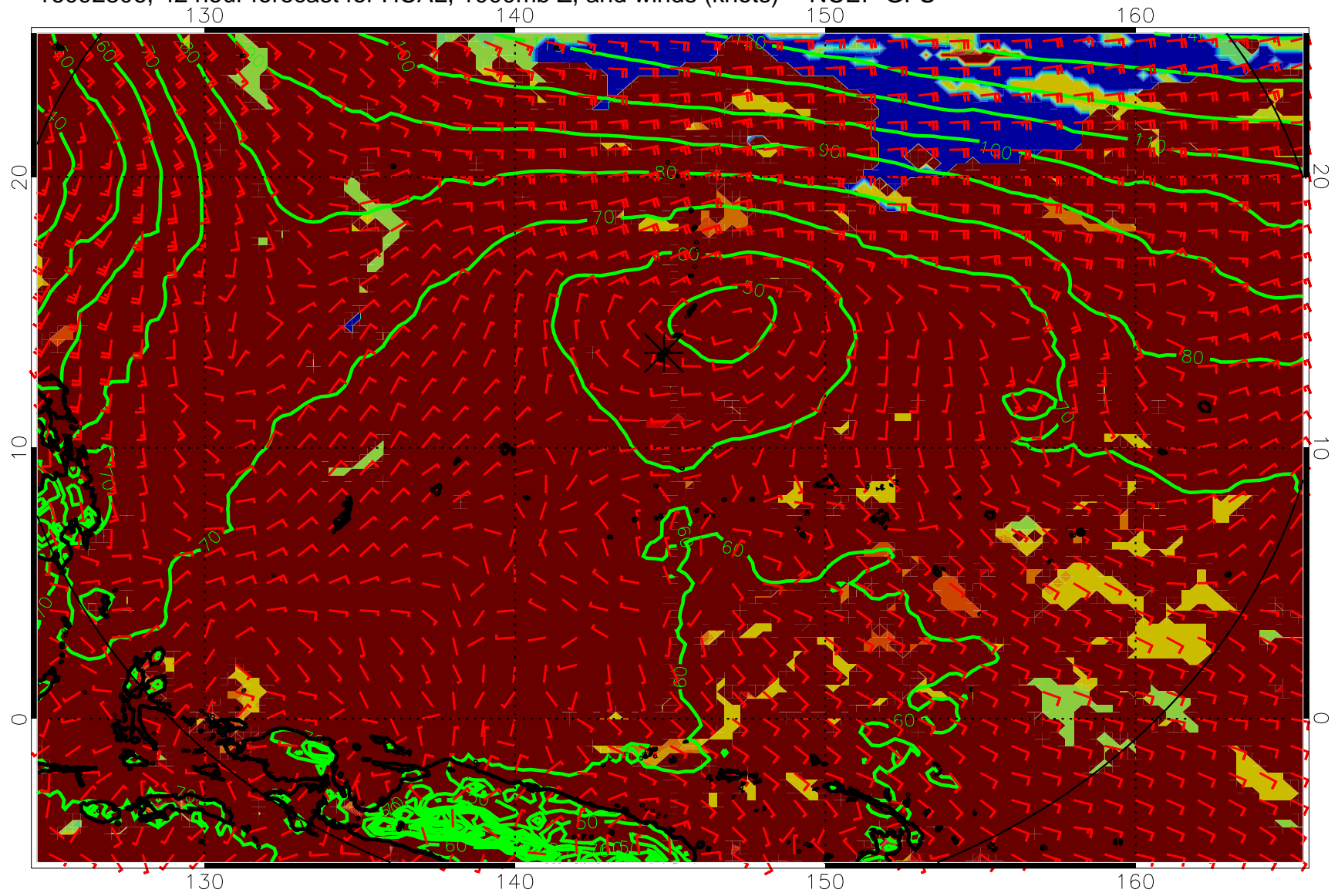
16092806, 42 hour forecast for HCAL, 1000mb Z, and winds (knots) -- NCEP GFS
