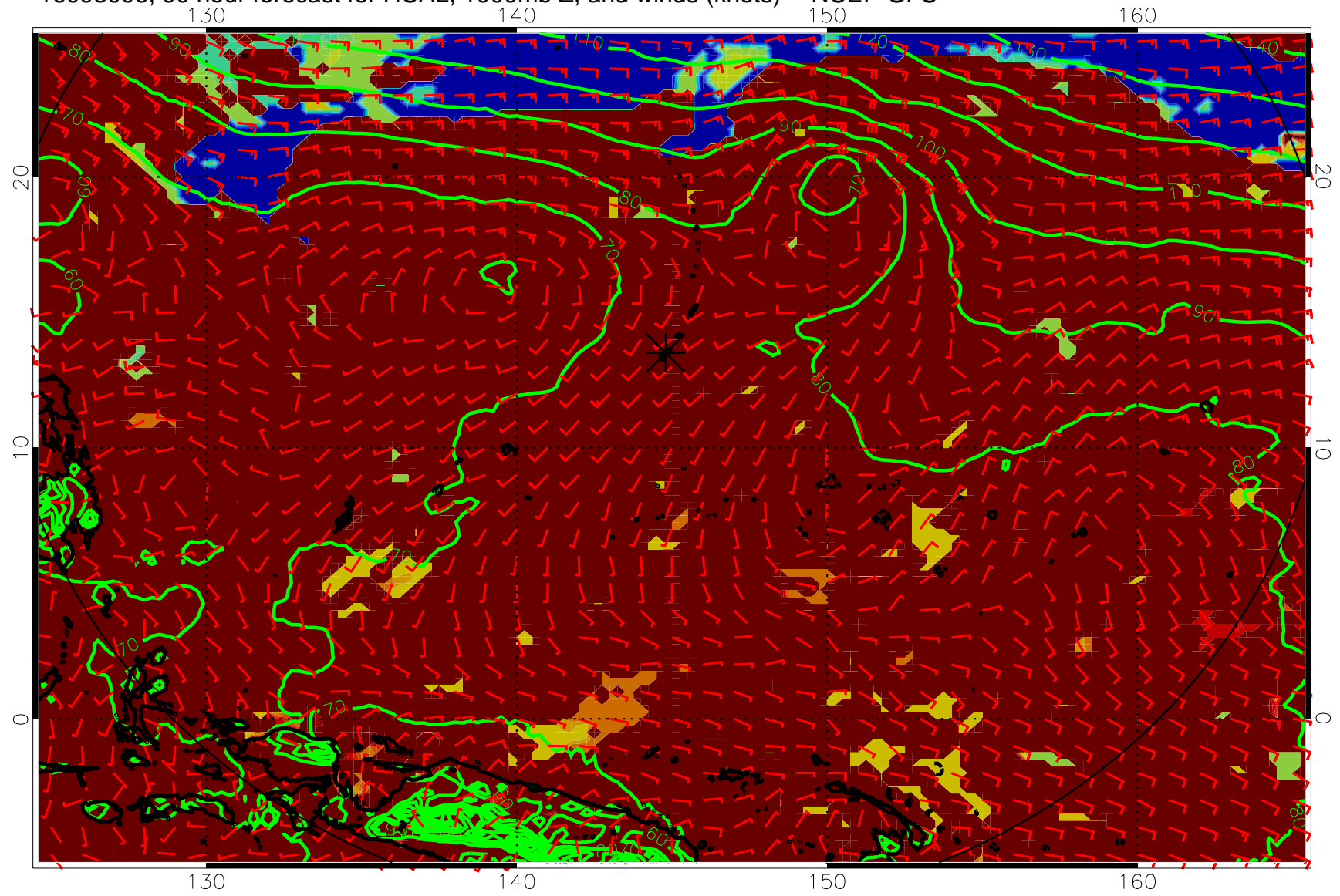
16093006, 90 hour forecast for HCAL, 1000mb Z, and winds (knots) -- NCEP GFS
