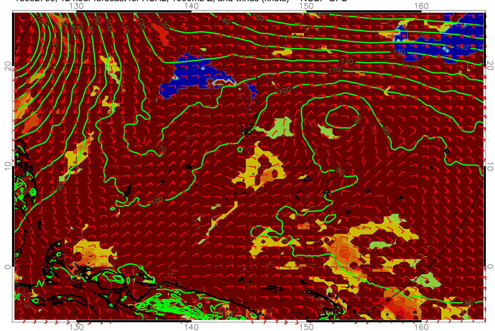
16092700, 12 hour forecast for HCAL, 1000mb Z, and winds (knots) -- NCEP GFS
