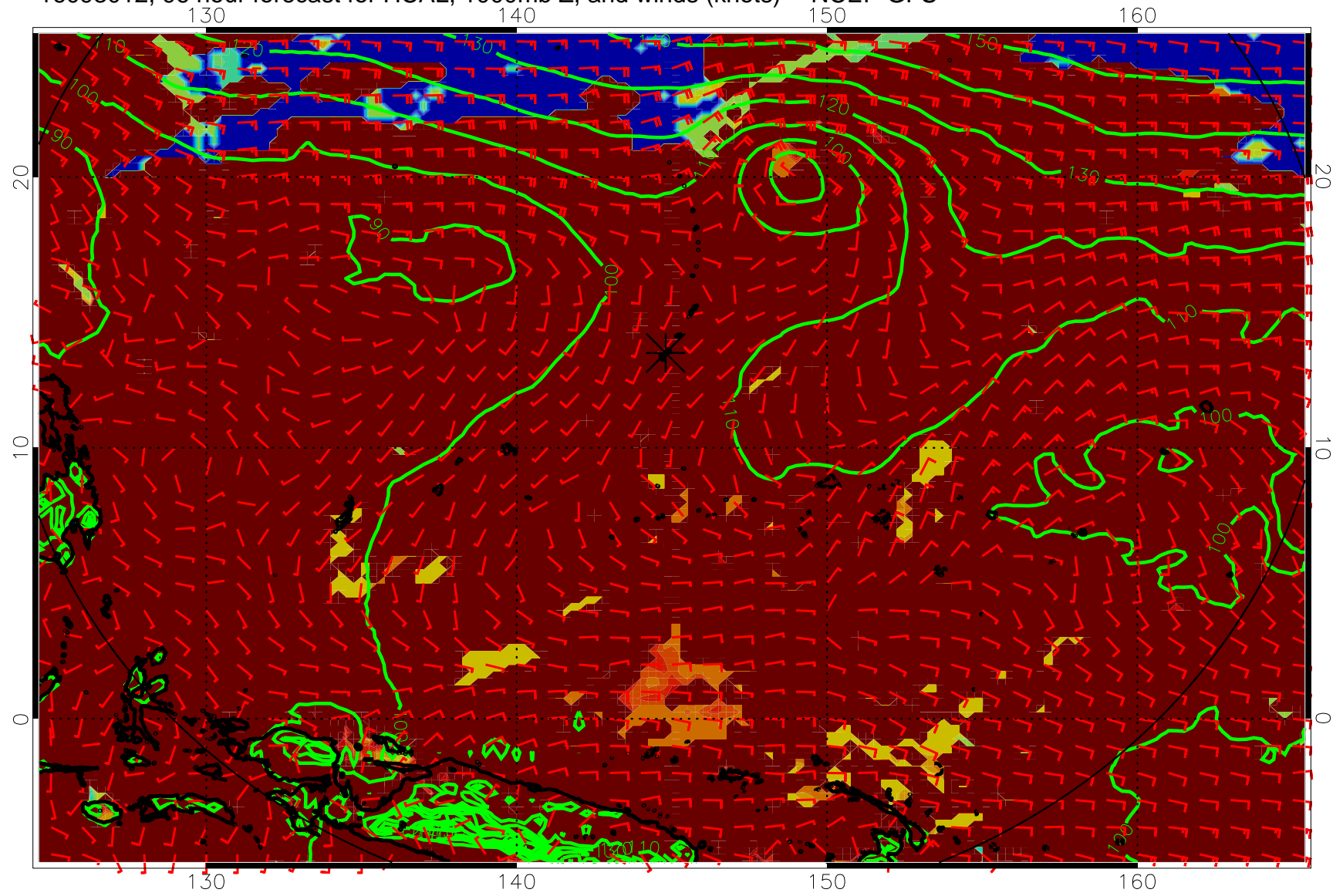
16093012, 96 hour forecast for HCAL, 1000mb Z, and winds (knots) -- NCEP GFS
