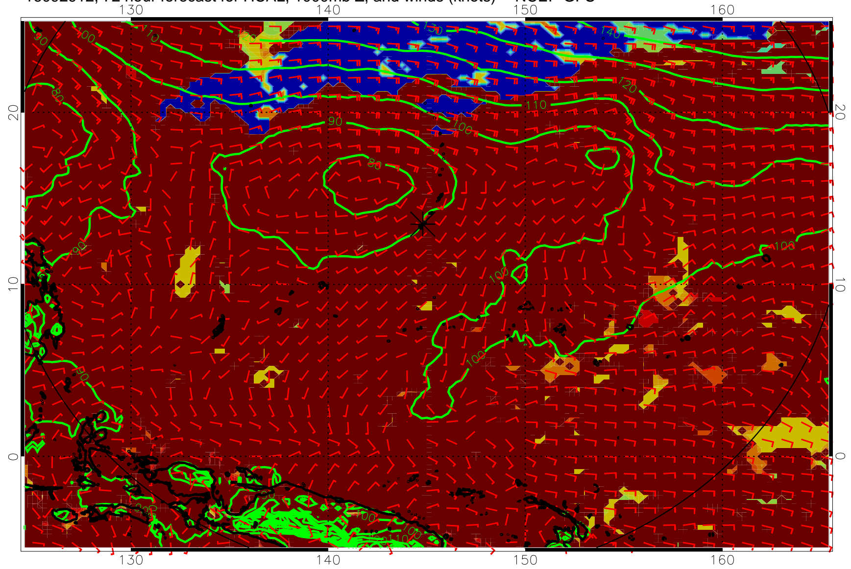
16092912, 72 hour forecast for HCAL, 1000mb Z, and winds (knots) -- NCEP GFS
