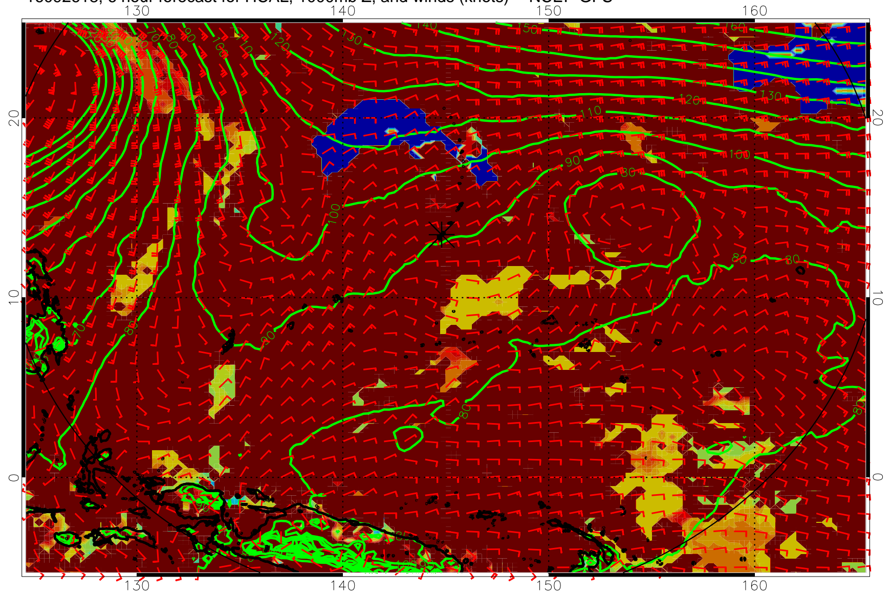
16092618, 6 hour forecast for HCAL, 1000mb Z, and winds (knots) -- NCEP GFS
