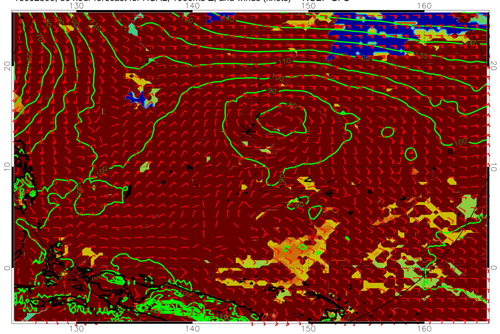
16092800, 36 hour forecast for HCAL, 1000mb Z, and winds (knots) -- NCEP GFS
