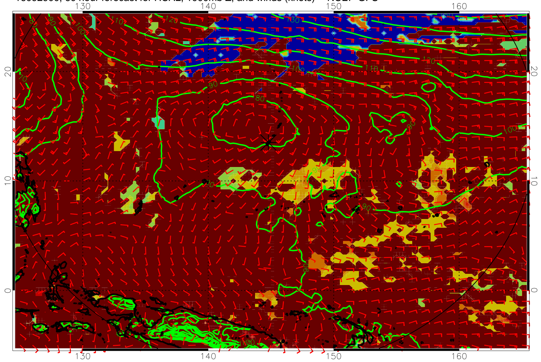
16092900, 60 hour forecast for HCAL, 1000mb Z, and winds (knots) -- NCEP GFS
