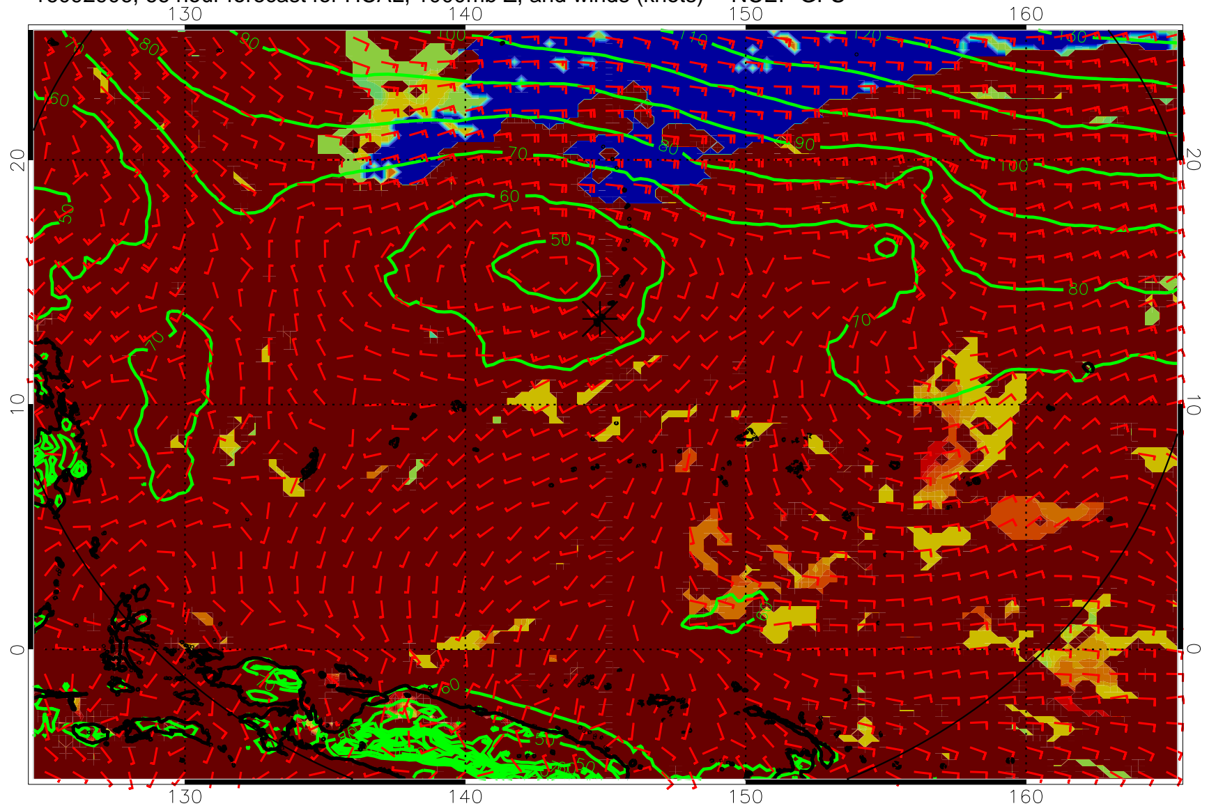
16092906, 66 hour forecast for HCAL, 1000mb Z, and winds (knots) -- NCEP GFS
