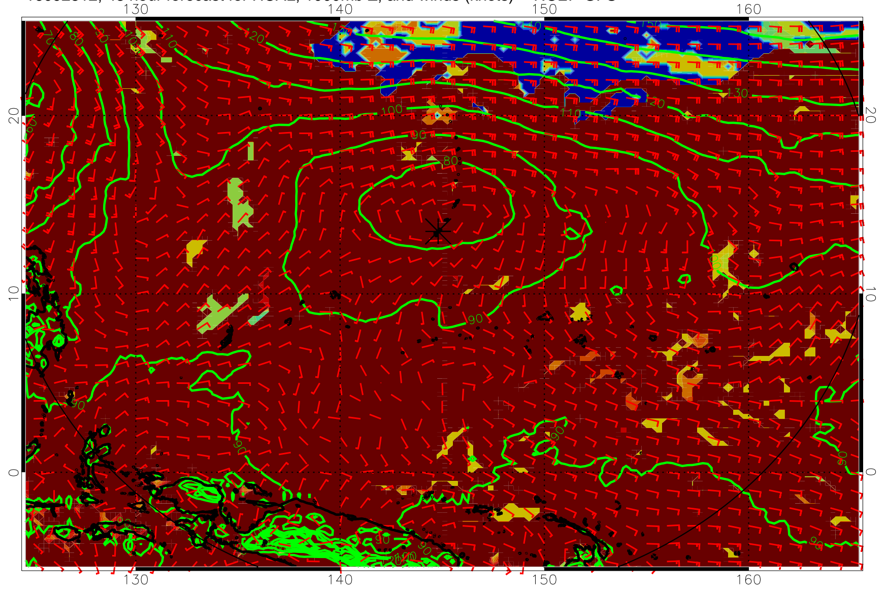
16092812, 48 hour forecast for HCAL, 1000mb Z, and winds (knots) -- NCEP GFS
