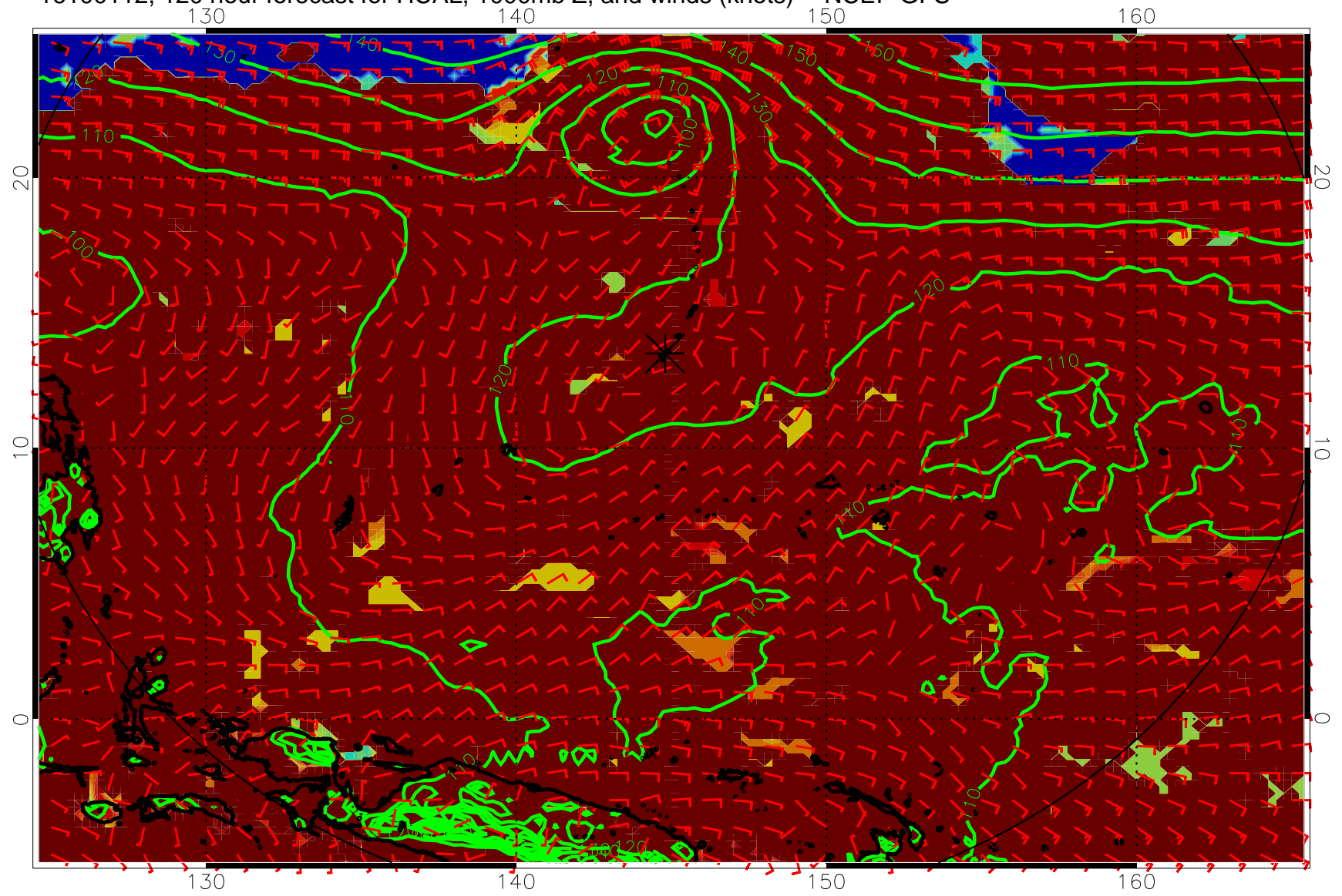
16100112, 120 hour forecast for HCAL, 1000mb Z, and winds (knots) -- NCEP GFS
