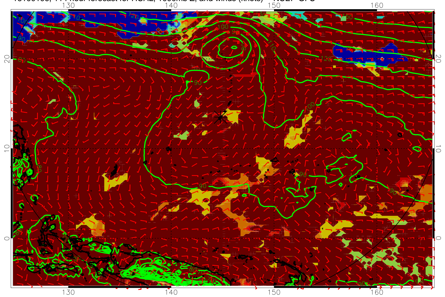
16100106, 114 hour forecast for HCAL, 1000mb Z, and winds (knots) -- NCEP GFS
