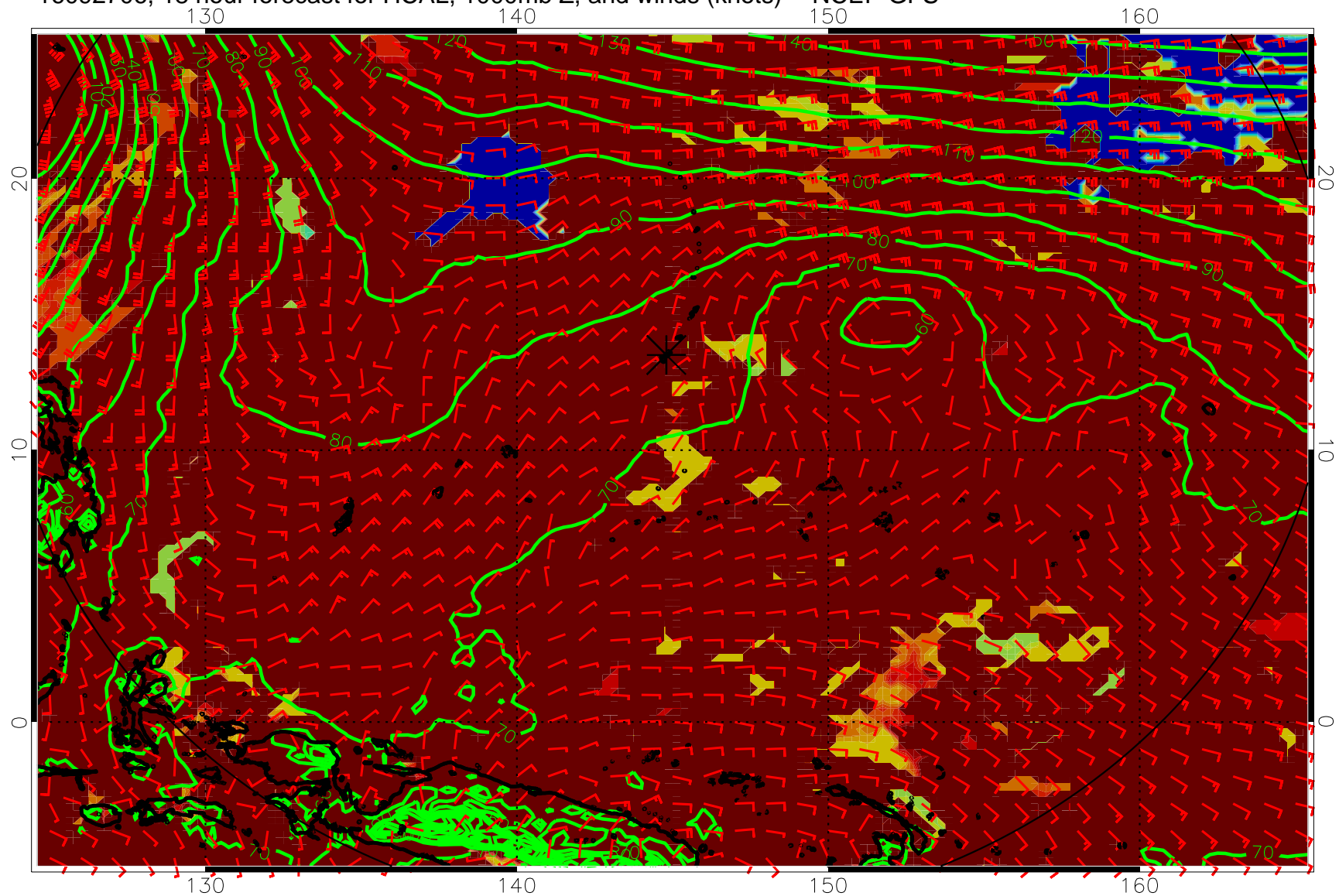
16092706, 18 hour forecast for HCAL, 1000mb Z, and winds (knots) -- NCEP GFS
