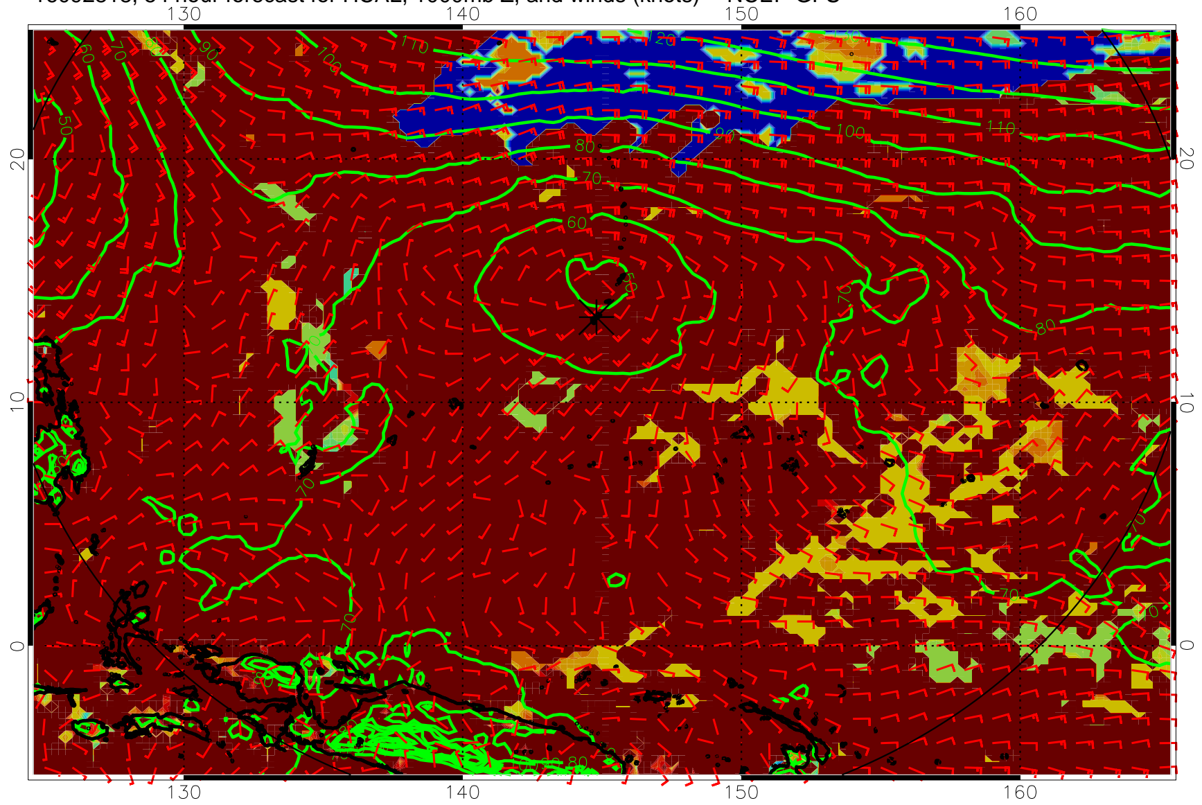
16092818, 54 hour forecast for HCAL, 1000mb Z, and winds (knots) -- NCEP GFS
