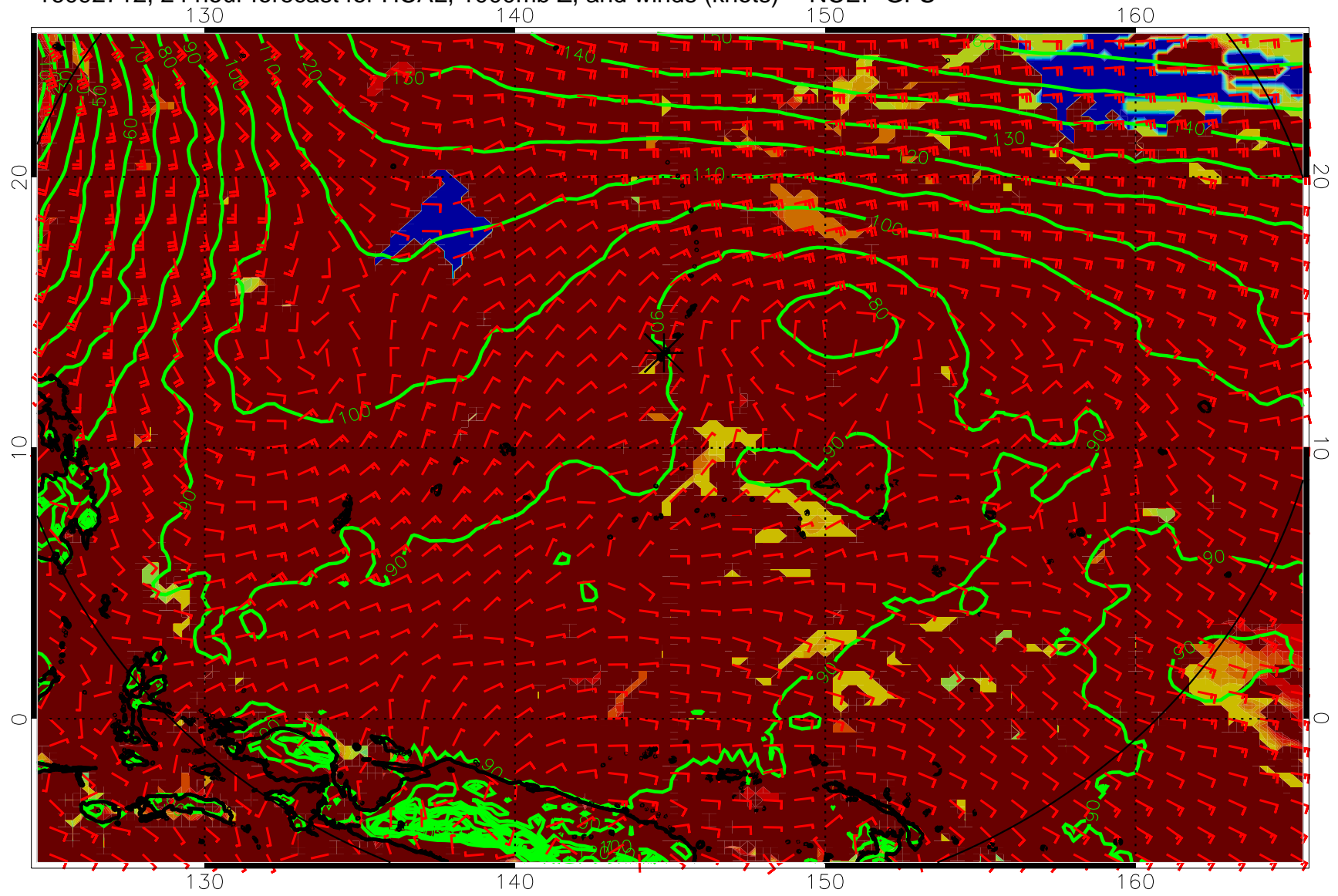
16092712, 24 hour forecast for HCAL, 1000mb Z, and winds (knots) -- NCEP GFS
