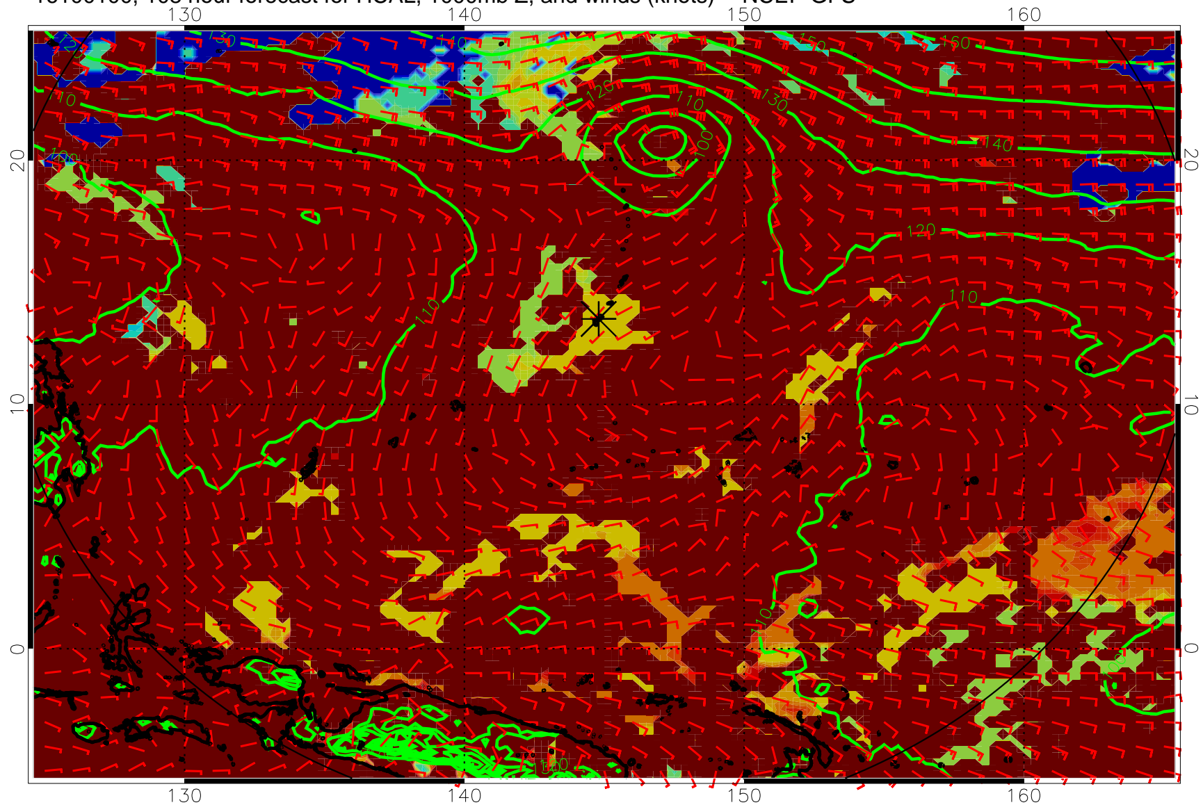
16100100, 108 hour forecast for HCAL, 1000mb Z, and winds (knots) -- NCEP GFS
