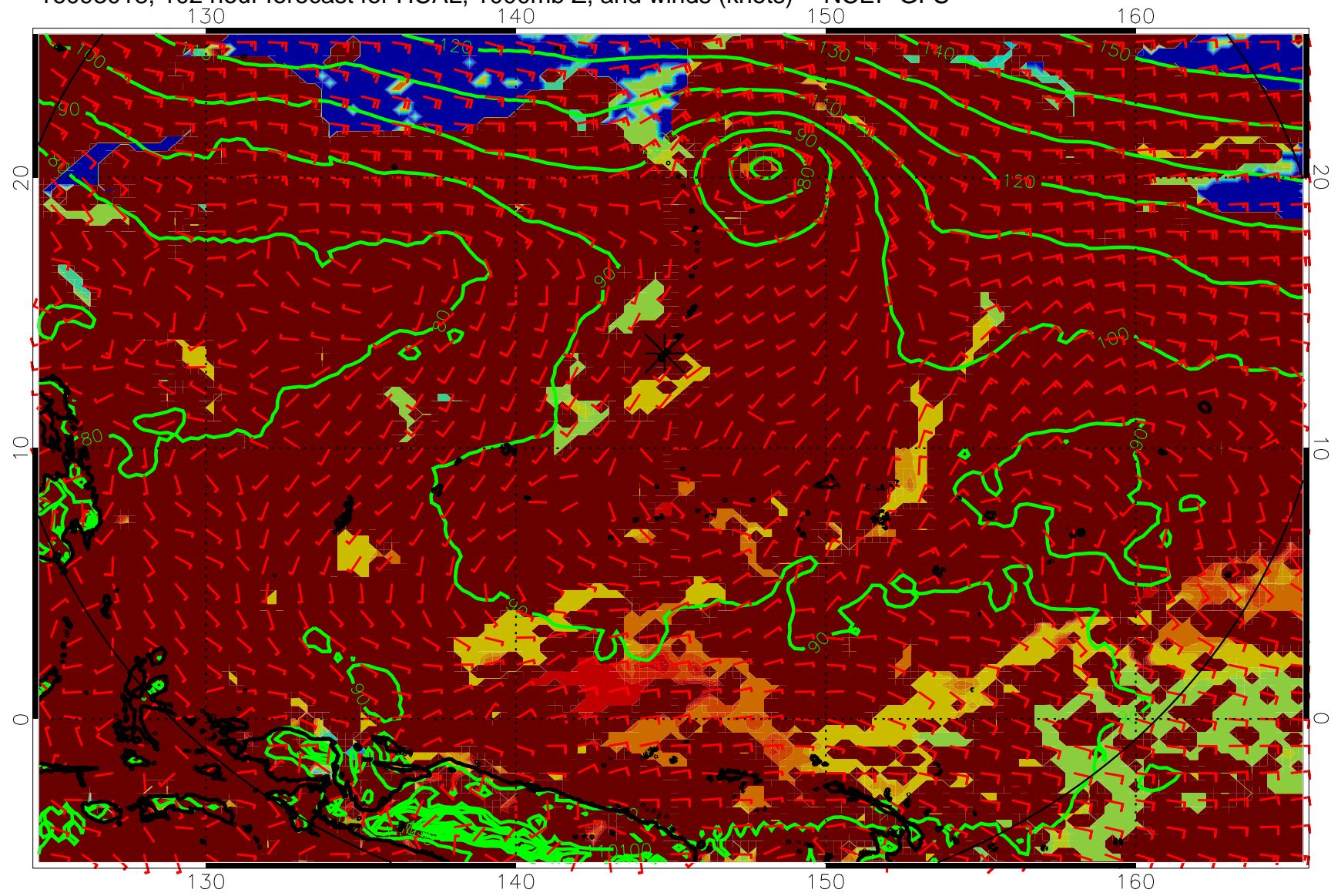
16093018, 102 hour forecast for HCAL, 1000mb Z, and winds (knots) -- NCEP GFS
