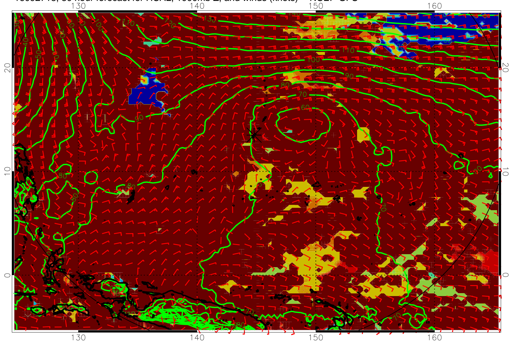
16092718, 30 hour forecast for HCAL, 1000mb Z, and winds (knots) -- NCEP GFS
