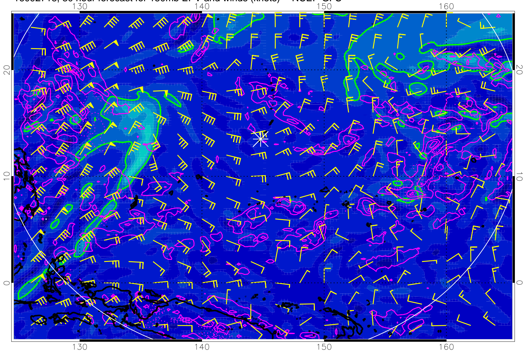
16092718, 30 hour forecast for 150mb EPV and winds (knots) -- NCEP GFS
