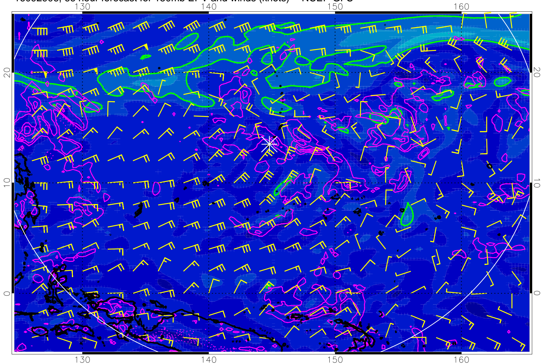
16092906, 66 hour forecast for 150mb EPV and winds (knots) -- NCEP GFS
