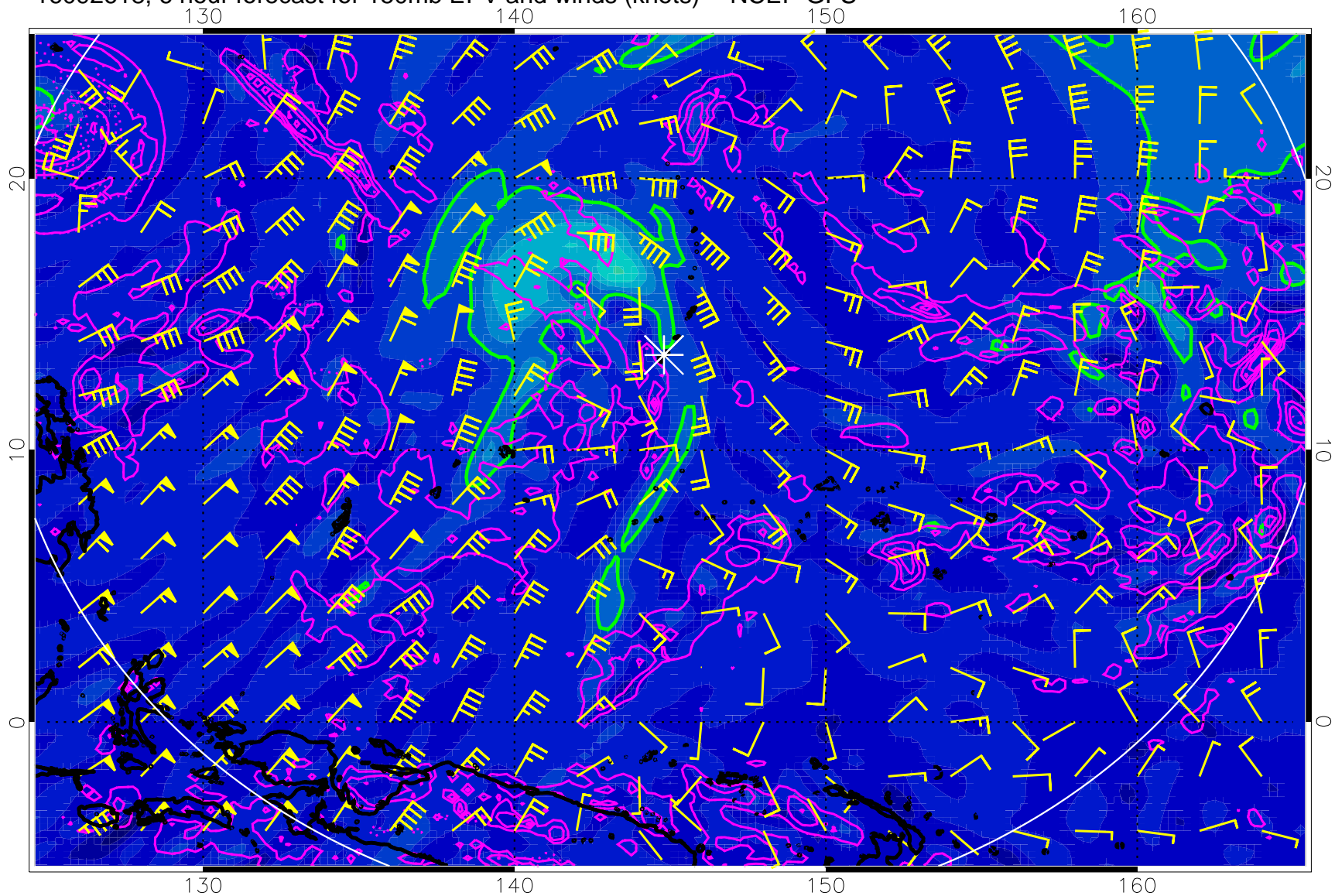
16092618, 6 hour forecast for 150mb EPV and winds (knots) -- NCEP GFS
