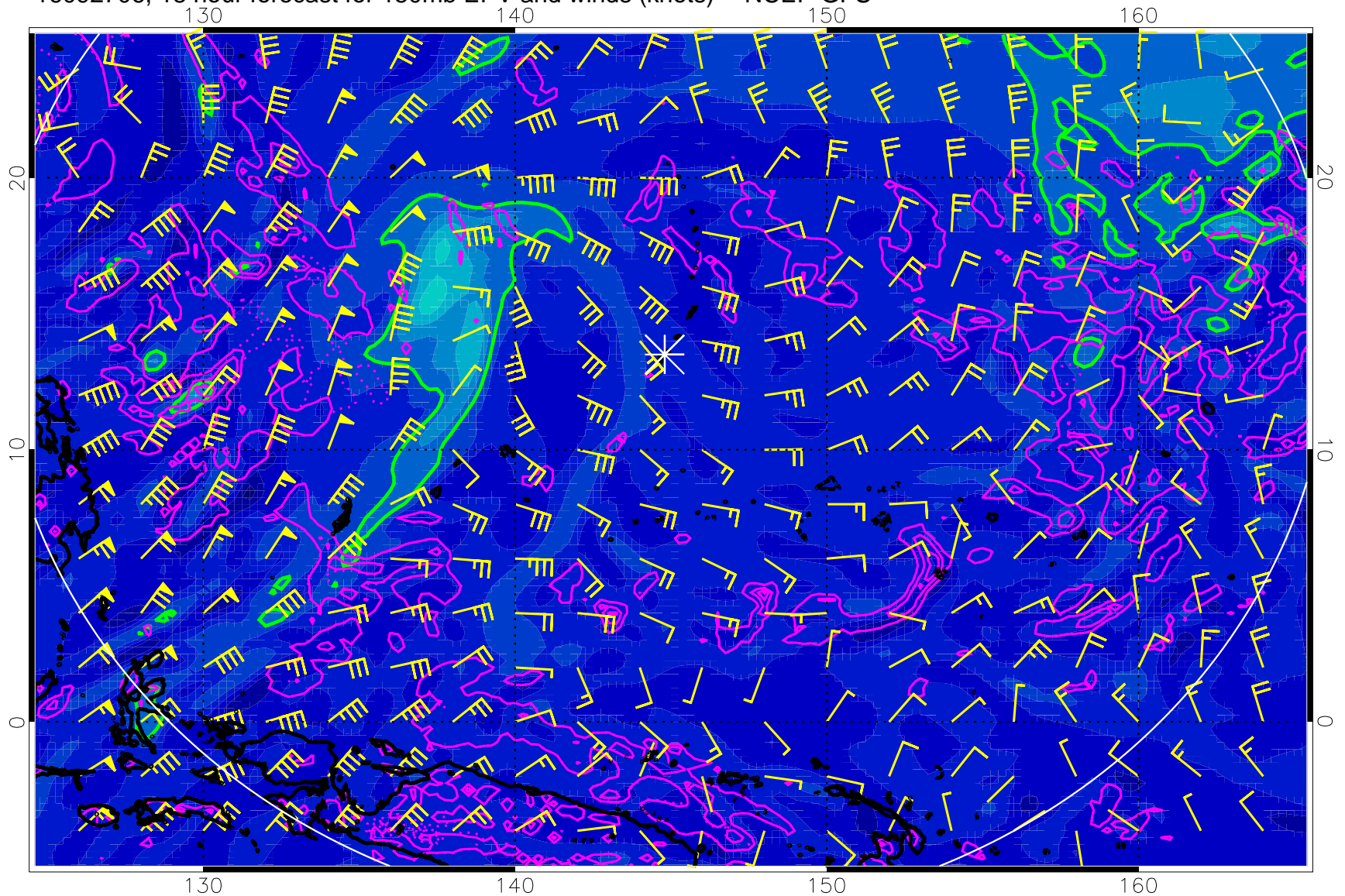
16092706, 18 hour forecast for 150mb EPV and winds (knots) -- NCEP GFS
