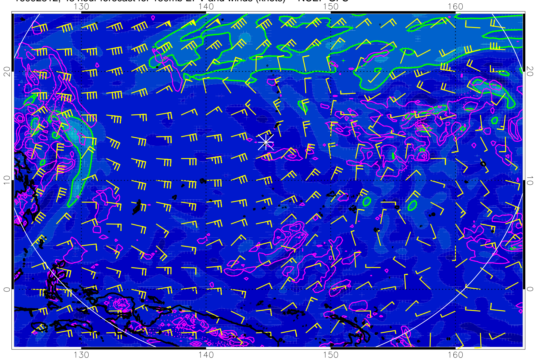
16092812, 48 hour forecast for 150mb EPV and winds (knots) -- NCEP GFS
