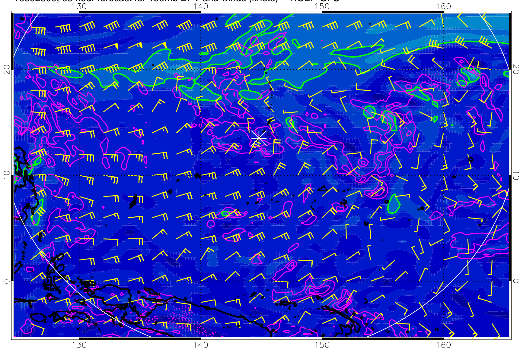
16092900, 60 hour forecast for 150mb EPV and winds (knots) -- NCEP GFS
