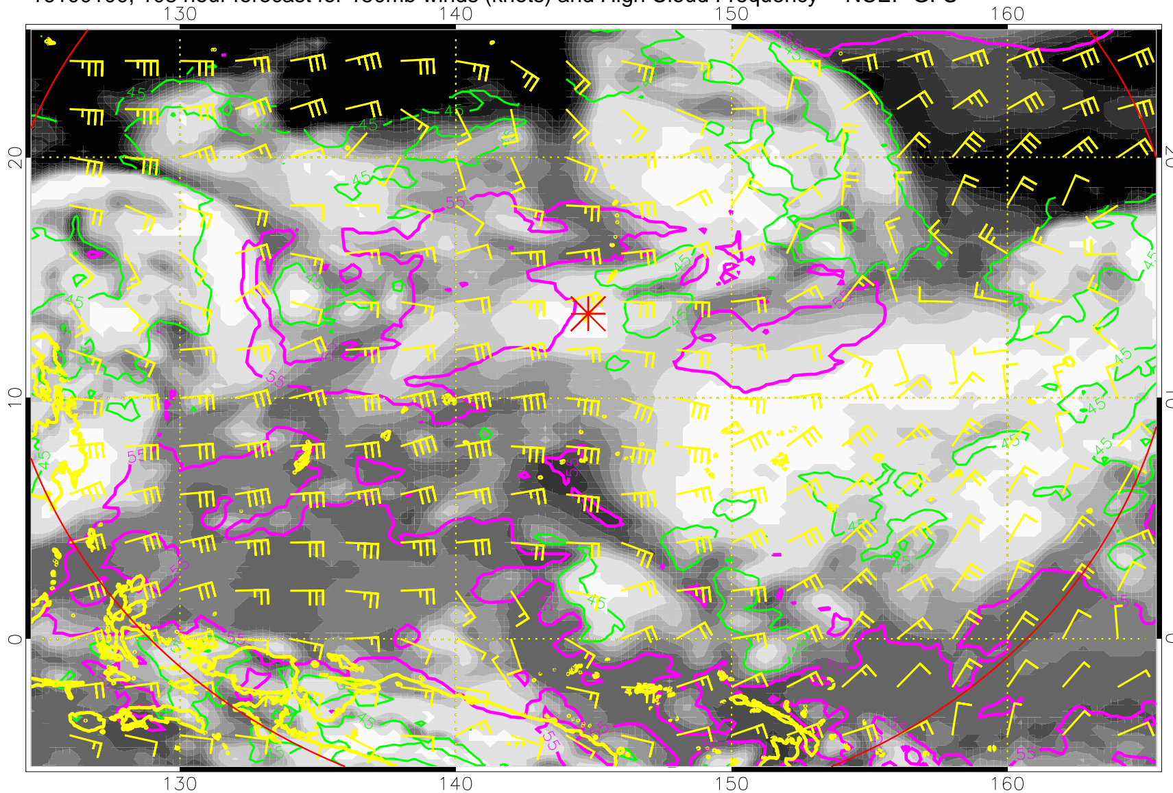
16100100, 108 hour forecast for 150mb winds (knots) and High Cloud Frequency -- NCEP GFS
