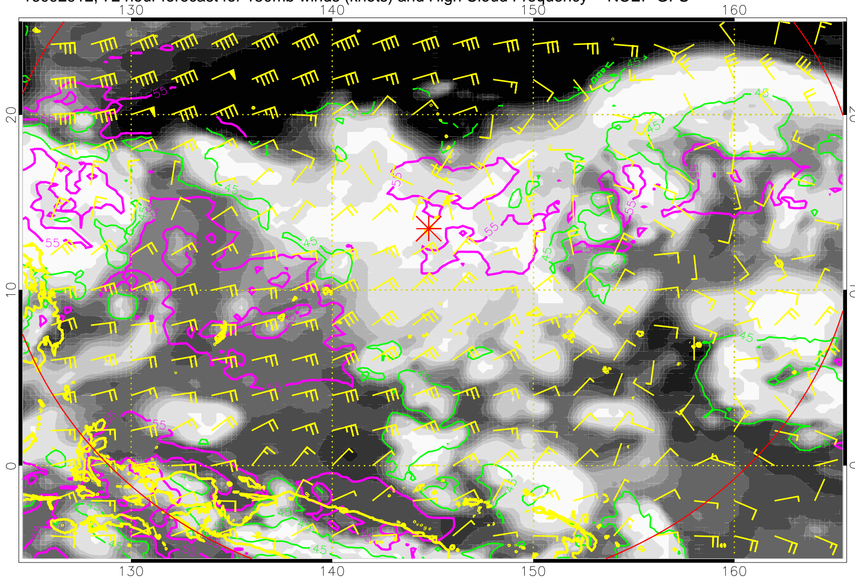
16092912, 72 hour forecast for 150mb winds (knots) and High Cloud Frequency -- NCEP GFS
