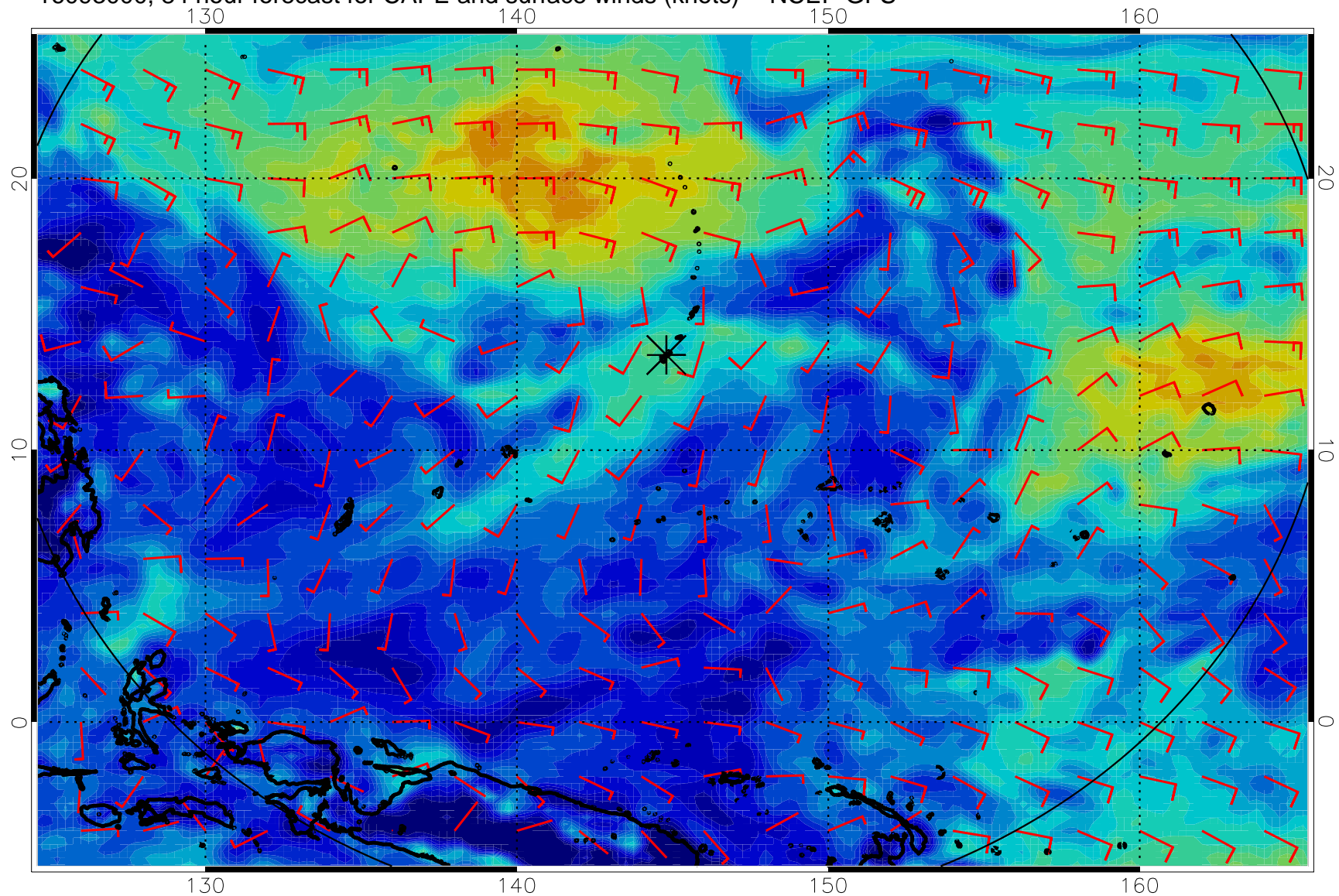
16093000, 84 hour forecast for CAPE and surface winds (knots) -- NCEP GFS
