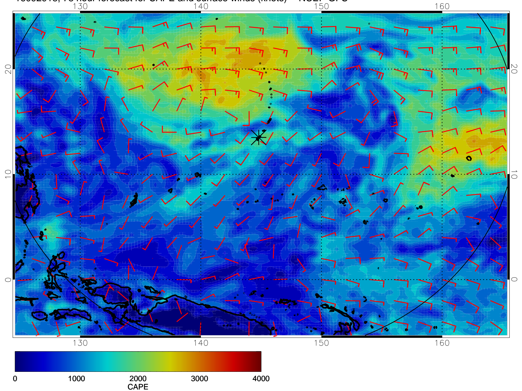
16092918, 78 hour forecast for CAPE and surface winds (knots) -- NCEP GFS
