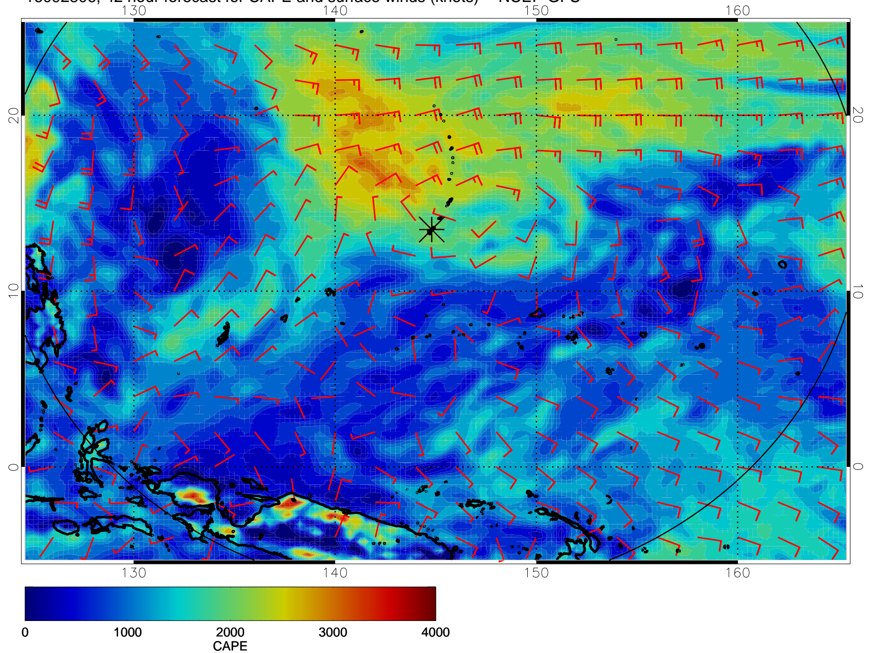
16092806, 42 hour forecast for CAPE and surface winds (knots) -- NCEP GFS
