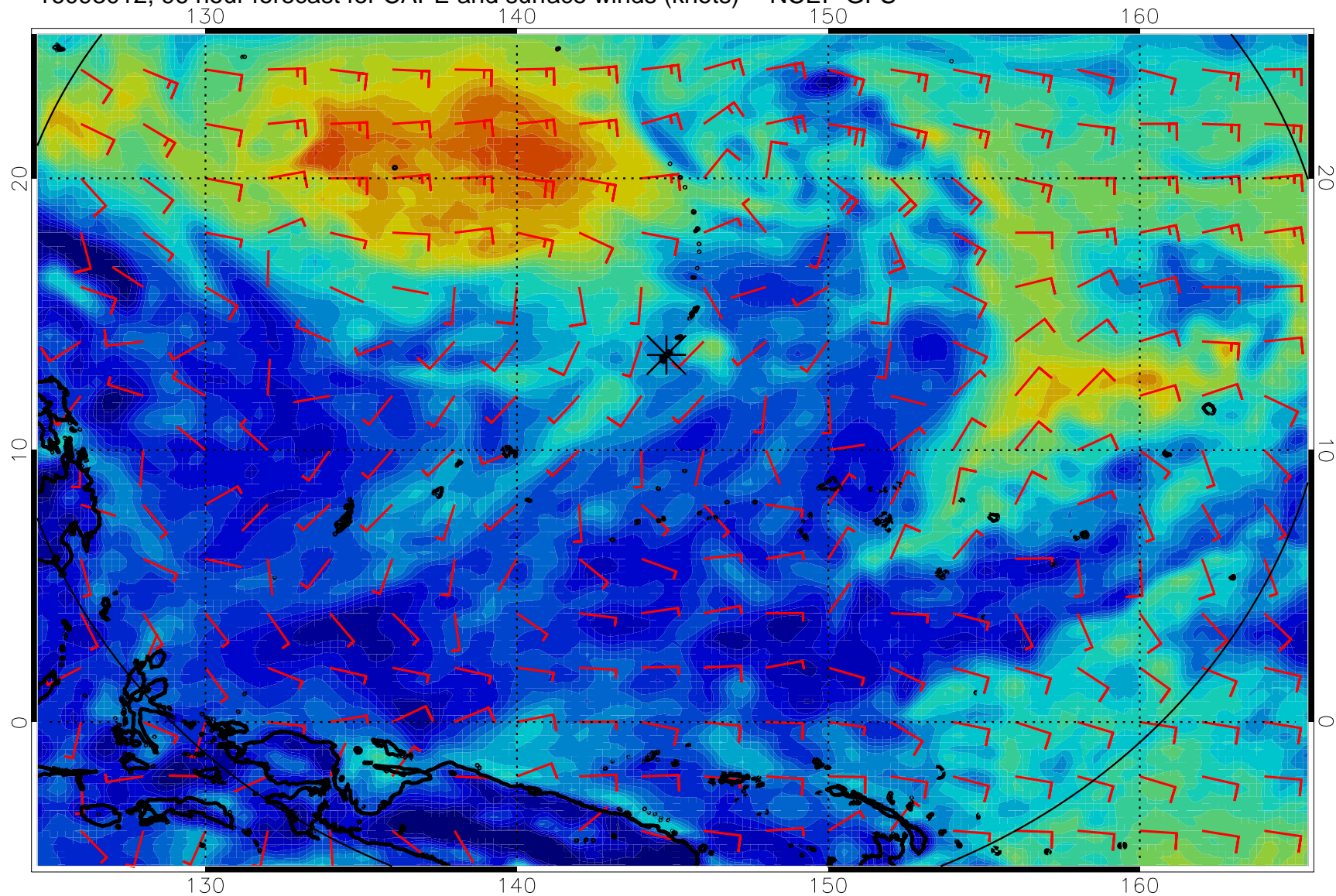
16093012, 96 hour forecast for CAPE and surface winds (knots) -- NCEP GFS
