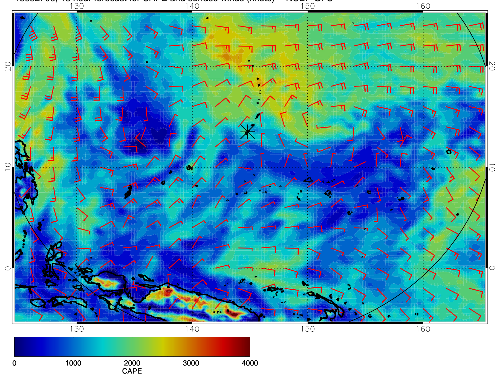
16092706, 18 hour forecast for CAPE and surface winds (knots) -- NCEP GFS
