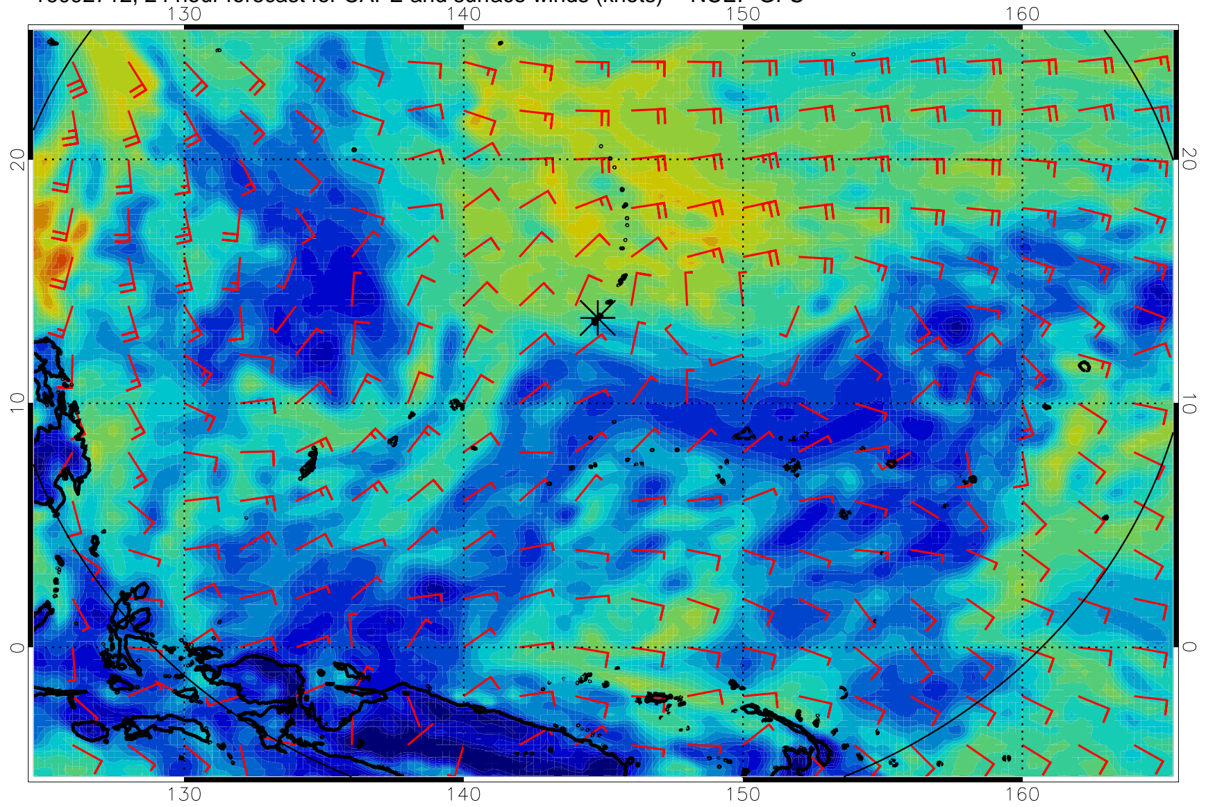
16092712, 24 hour forecast for CAPE and surface winds (knots) -- NCEP GFS
