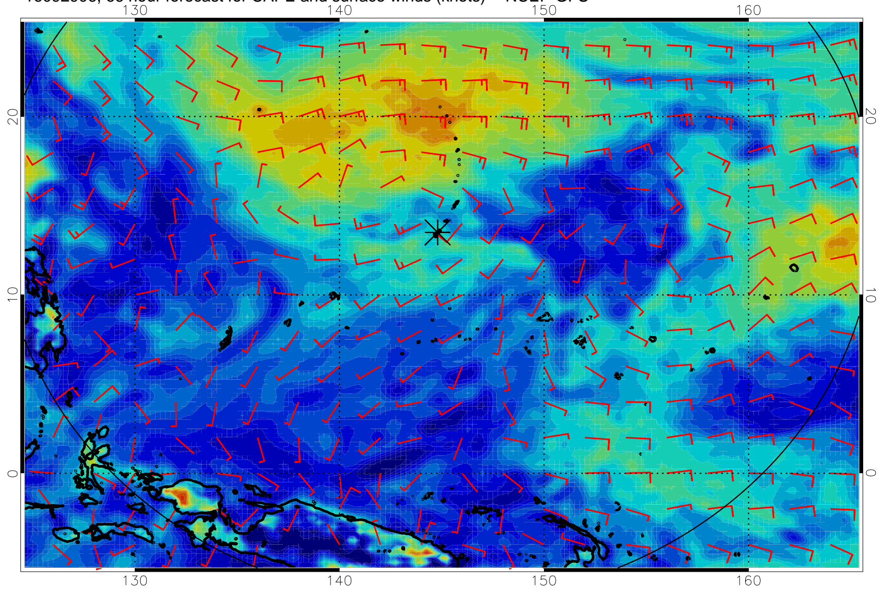
16092906, 66 hour forecast for CAPE and surface winds (knots) -- NCEP GFS
