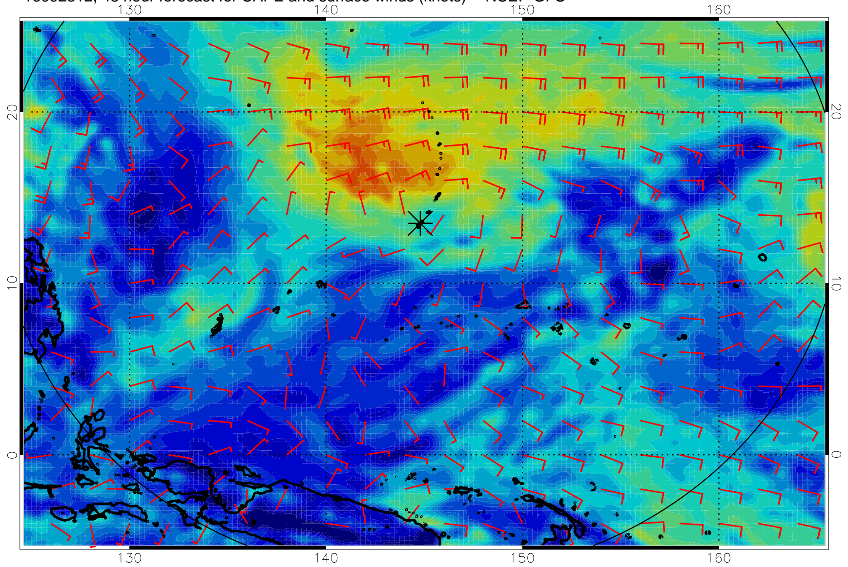
16092812, 48 hour forecast for CAPE and surface winds (knots) -- NCEP GFS
