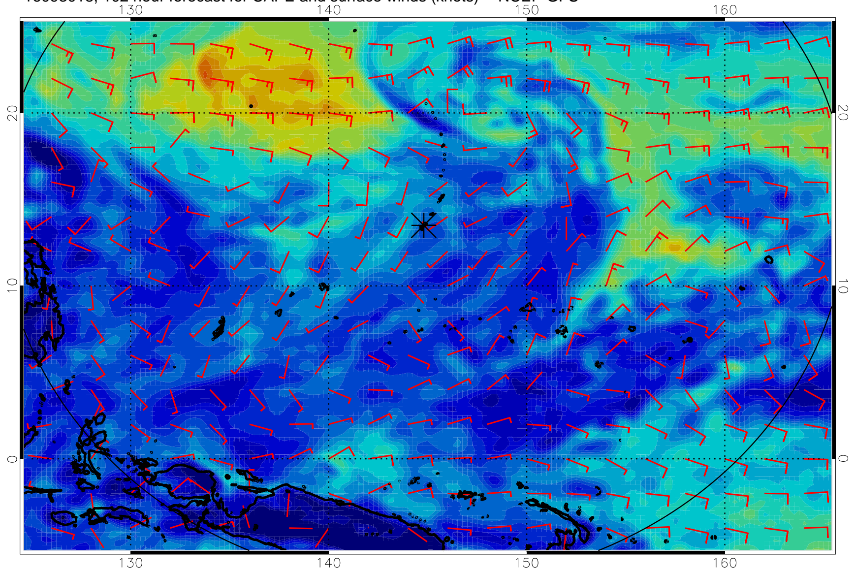
16093018, 102 hour forecast for CAPE and surface winds (knots) -- NCEP GFS
