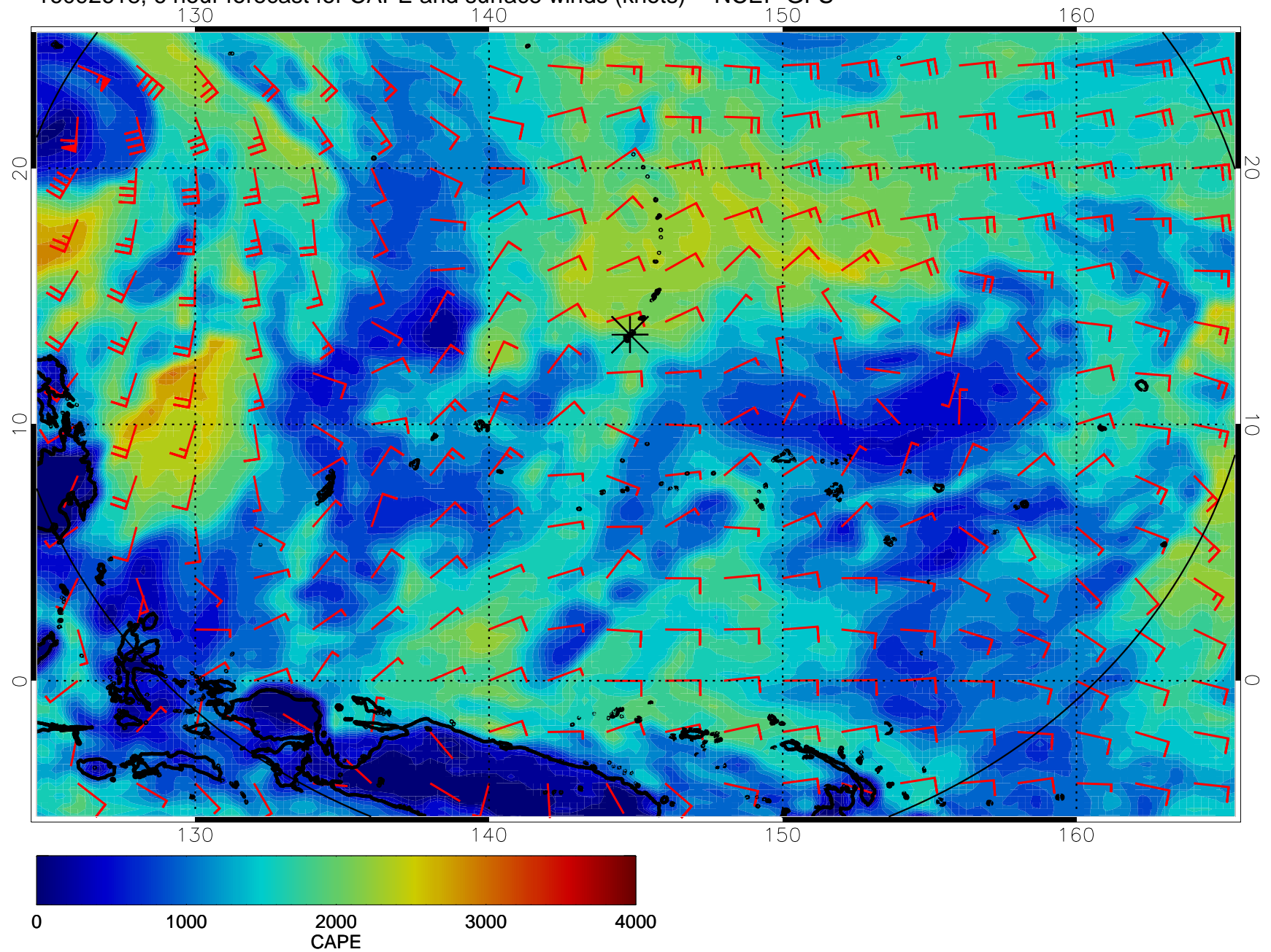
16092618, 6 hour forecast for CAPE and surface winds (knots) -- NCEP GFS
