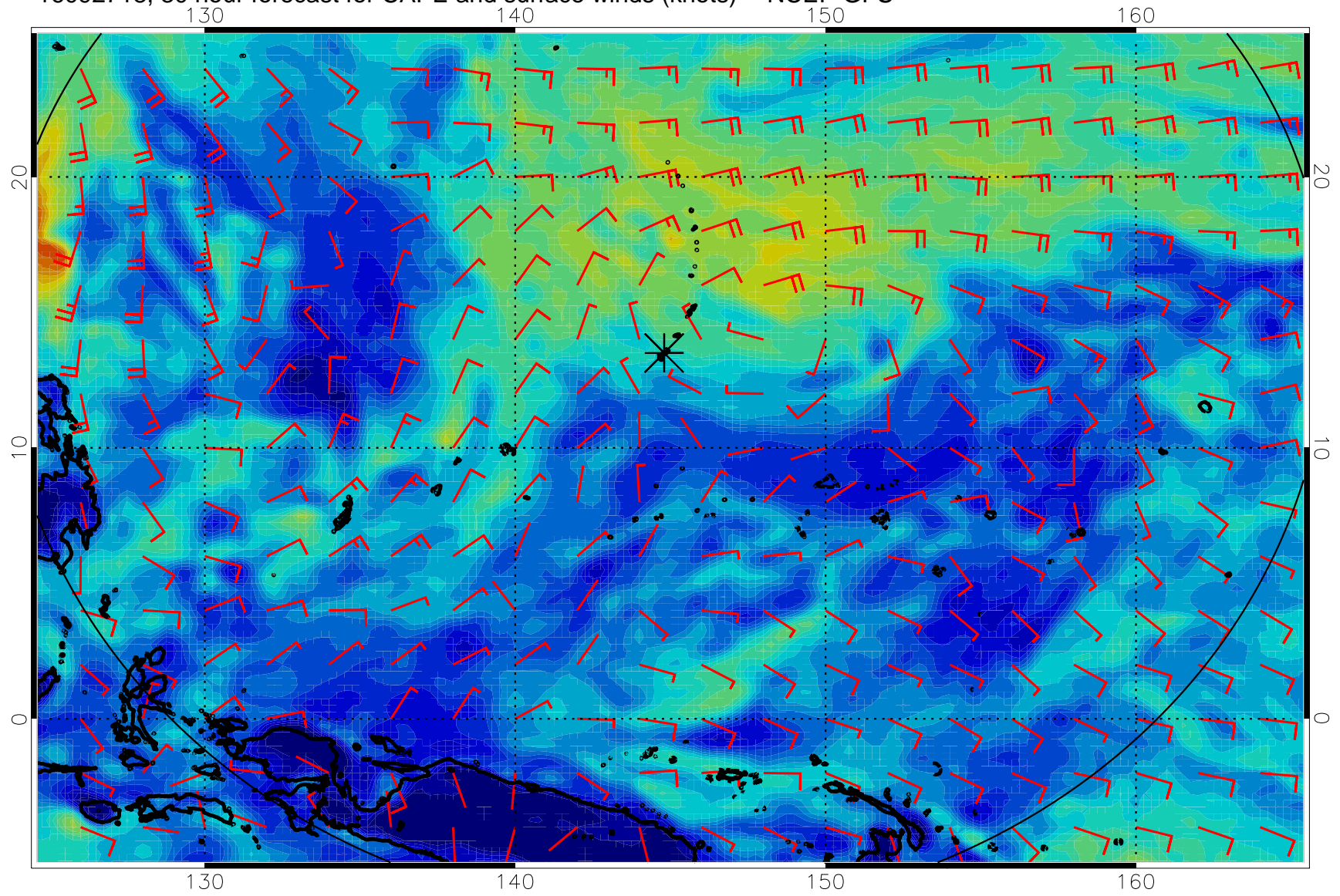
16092718, 30 hour forecast for CAPE and surface winds (knots) -- NCEP GFS
