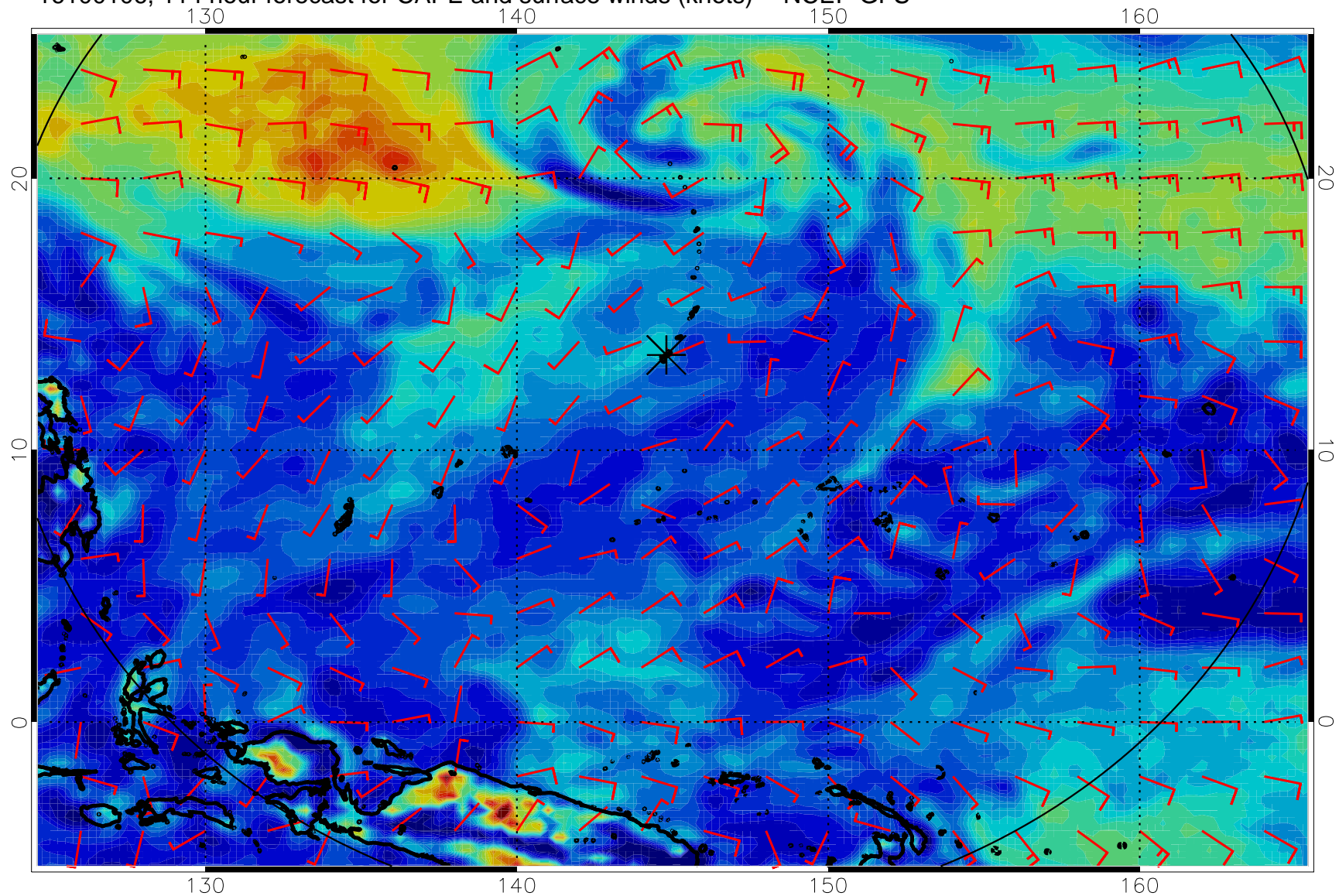
16100106, 114 hour forecast for CAPE and surface winds (knots) -- NCEP GFS
