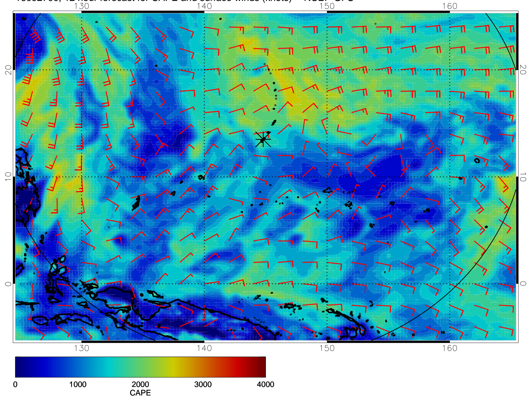
16092700, 12 hour forecast for CAPE and surface winds (knots) -- NCEP GFS
