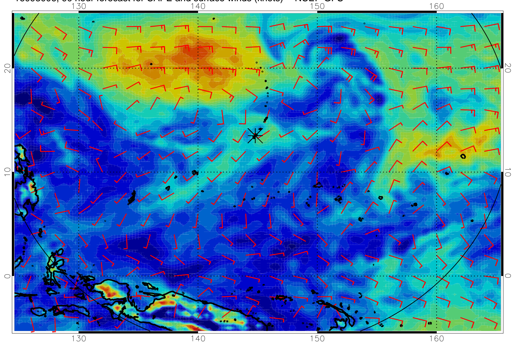
16093006, 90 hour forecast for CAPE and surface winds (knots) -- NCEP GFS
