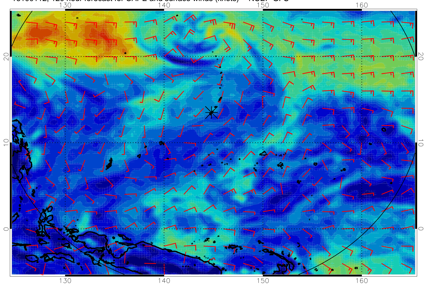
16100112, 120 hour forecast for CAPE and surface winds (knots) -- NCEP GFS
