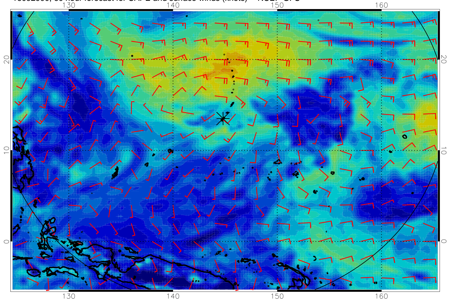
16092900, 60 hour forecast for CAPE and surface winds (knots) -- NCEP GFS
