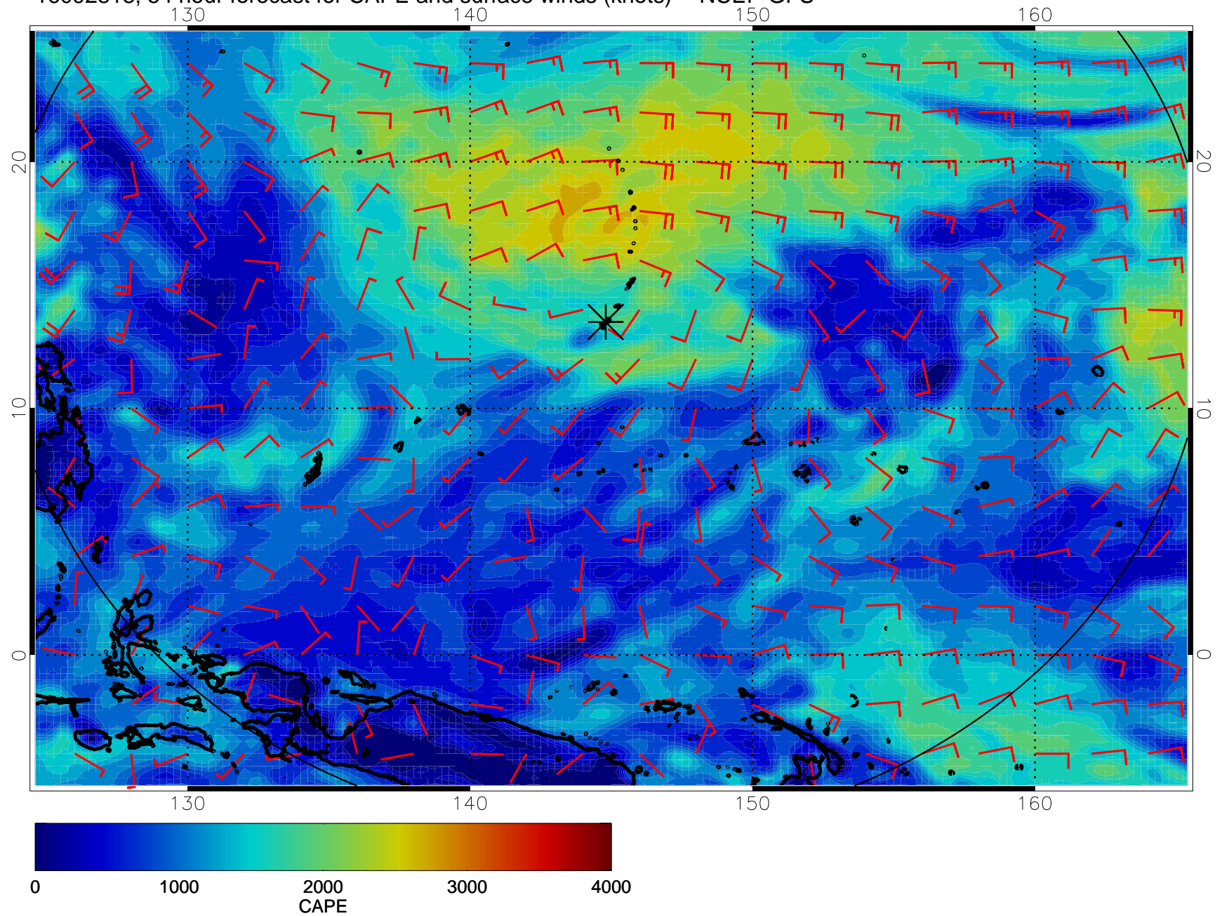
16092818, 54 hour forecast for CAPE and surface winds (knots) -- NCEP GFS
