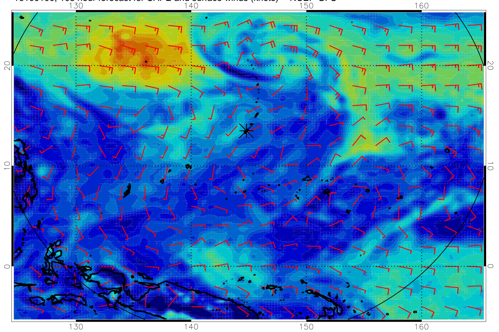
16100100, 108 hour forecast for CAPE and surface winds (knots) -- NCEP GFS
