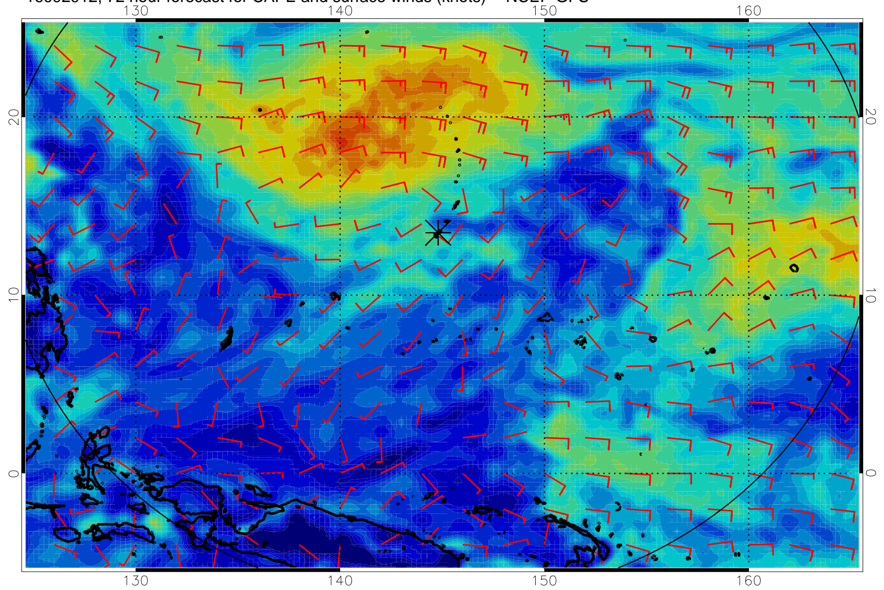
16092912, 72 hour forecast for CAPE and surface winds (knots) -- NCEP GFS
