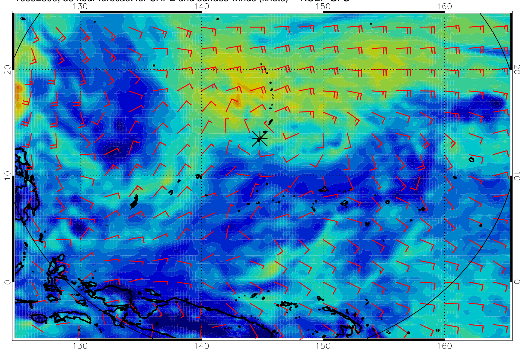
16092800, 36 hour forecast for CAPE and surface winds (knots) -- NCEP GFS
