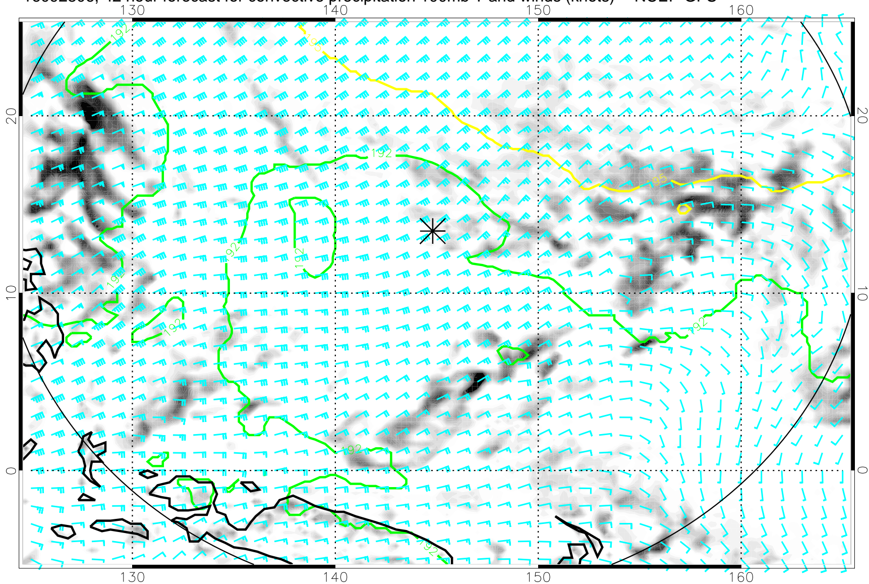
16092806, 42 hour forecast for convective precipitation 100mb T and winds (knots) -- NCEP GFS
