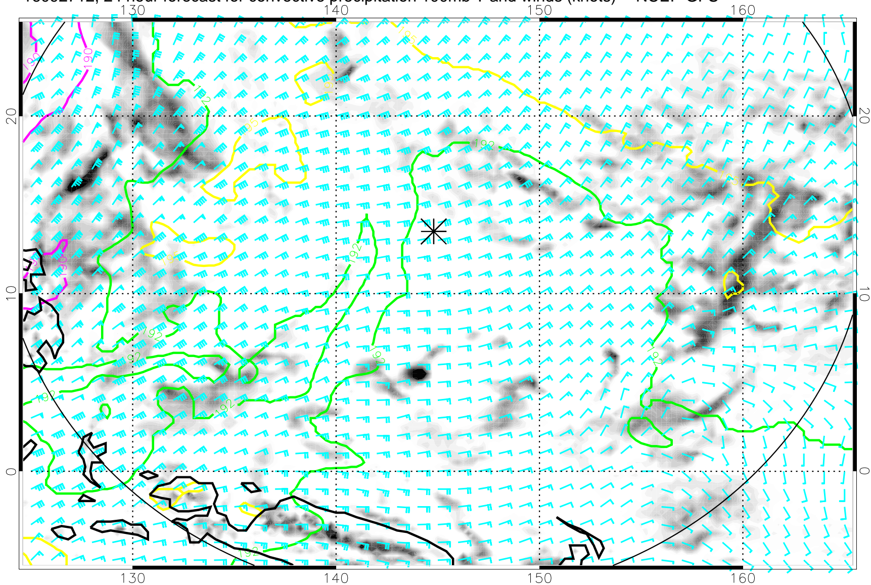
16092712, 24 hour forecast for convective precipitation 100mb T and winds (knots) -- NCEP GFS
