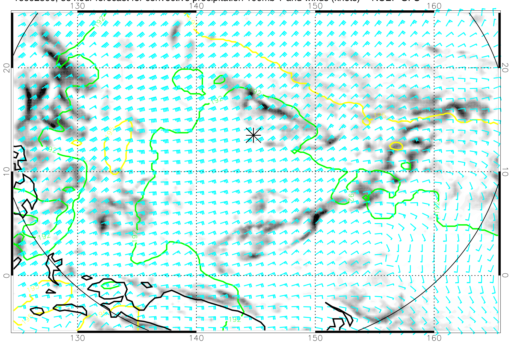
16092800, 36 hour forecast for convective precipitation 100mb T and winds (knots) -- NCEP GFS
