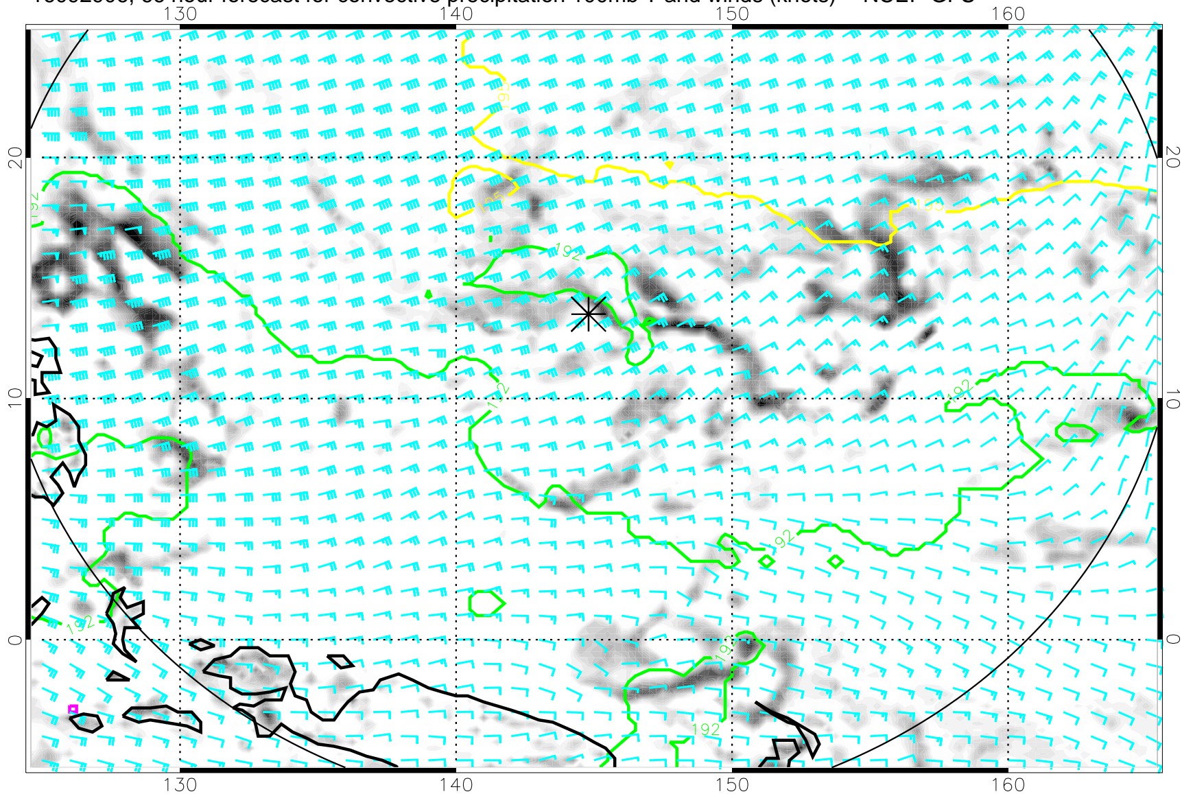
16092906, 66 hour forecast for convective precipitation 100mb T and winds (knots) -- NCEP GFS
