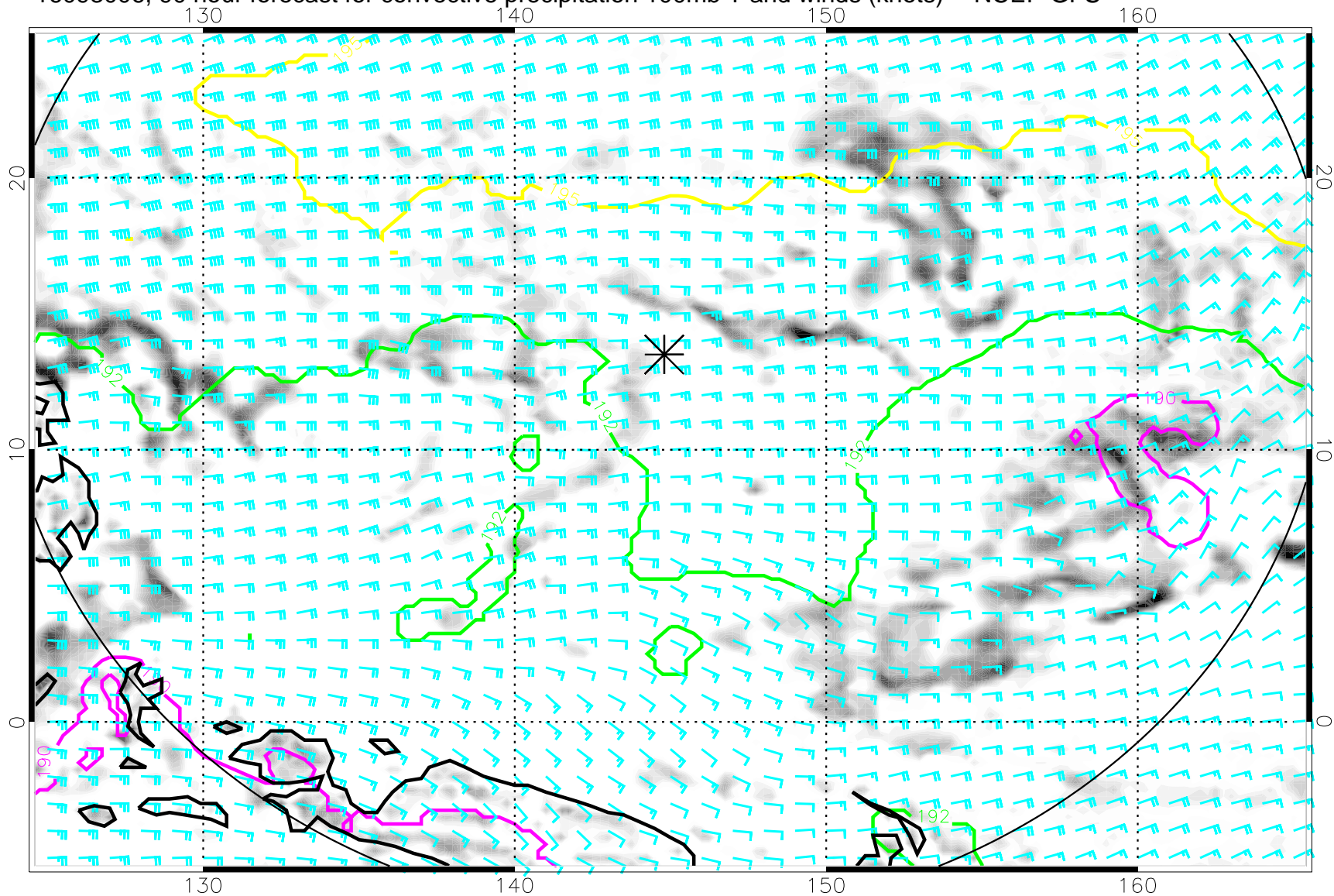
16093006, 90 hour forecast for convective precipitation 100mb T and winds (knots) -- NCEP GFS
