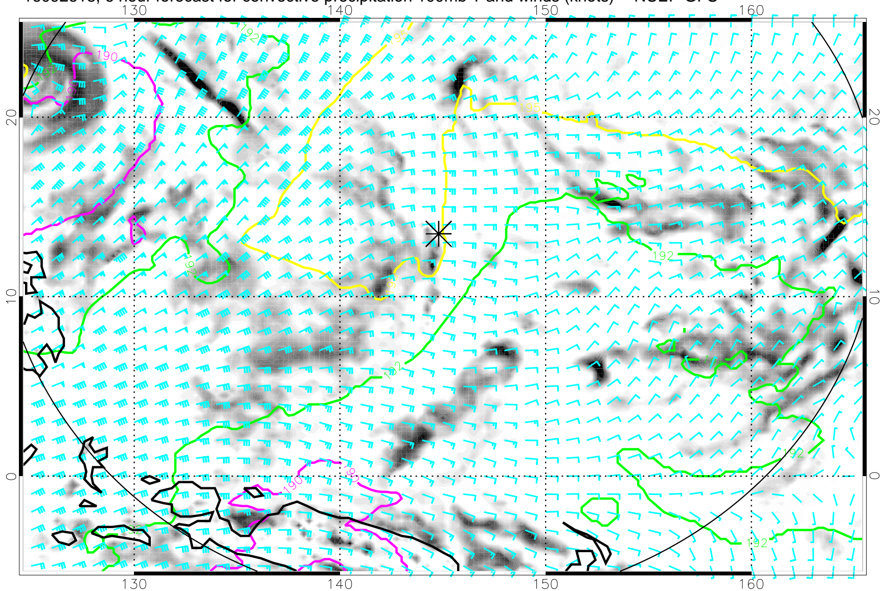
16092618, 6 hour forecast for convective precipitation 100mb T and winds (knots) -- NCEP GFS
