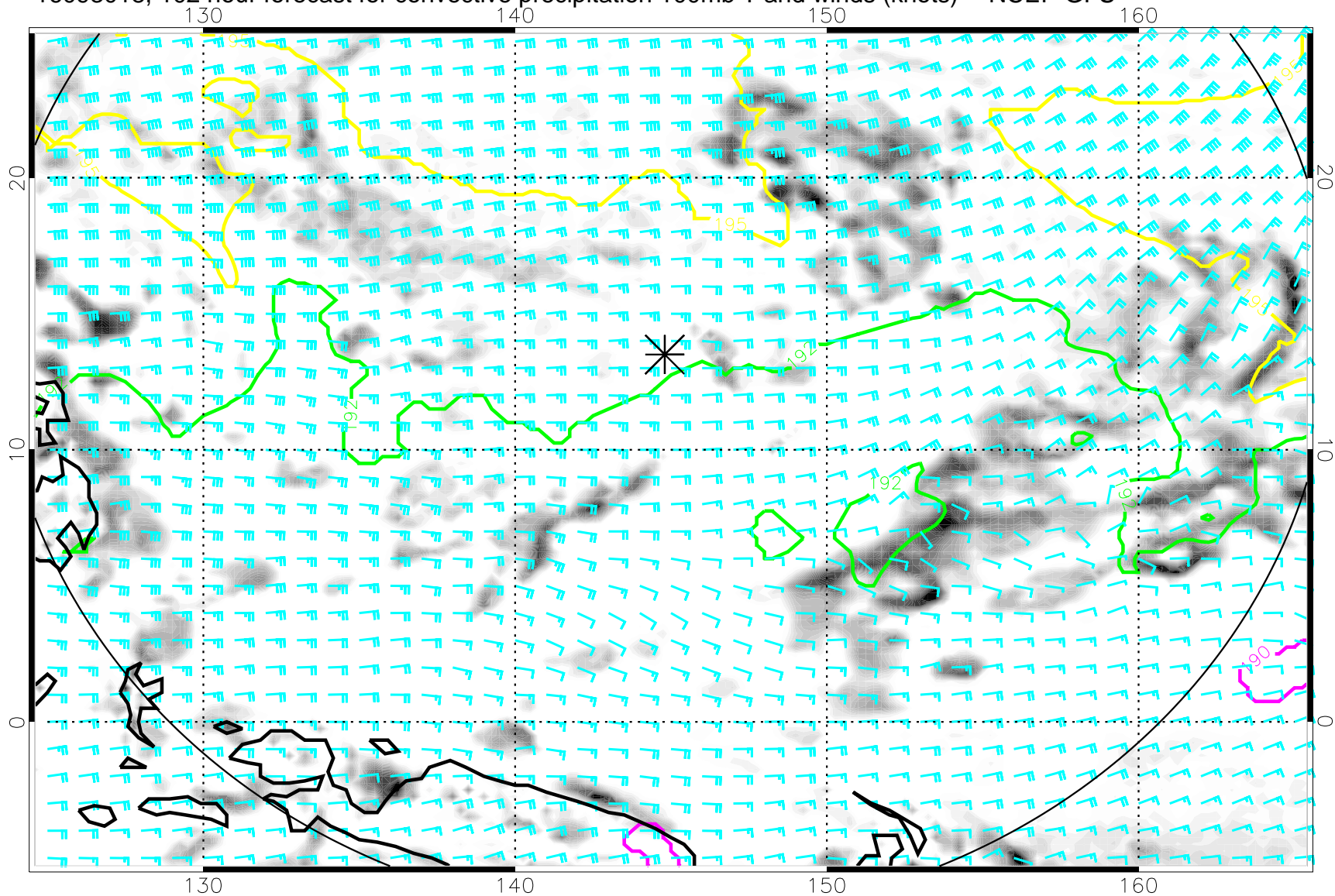
16093018, 102 hour forecast for convective precipitation 100mb T and winds (knots) -- NCEP GFS
