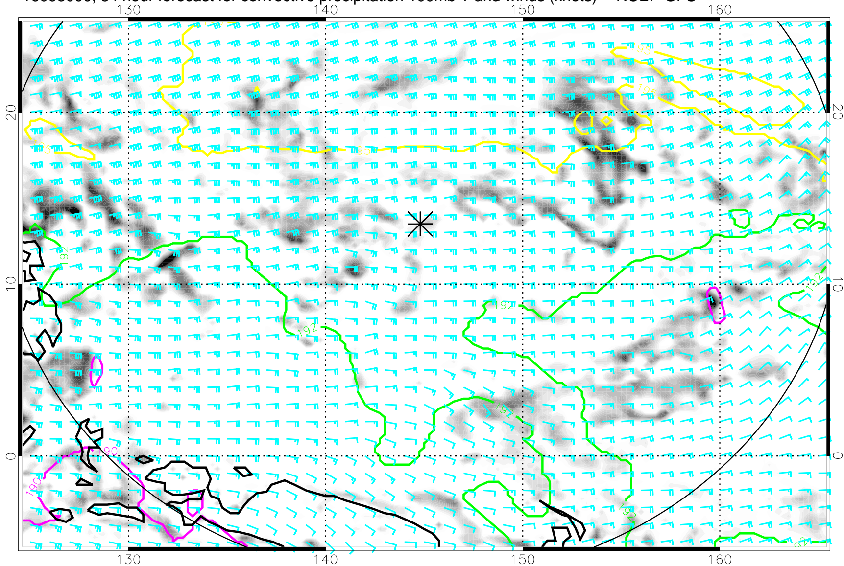
16093000, 84 hour forecast for convective precipitation 100mb T and winds (knots) -- NCEP GFS
