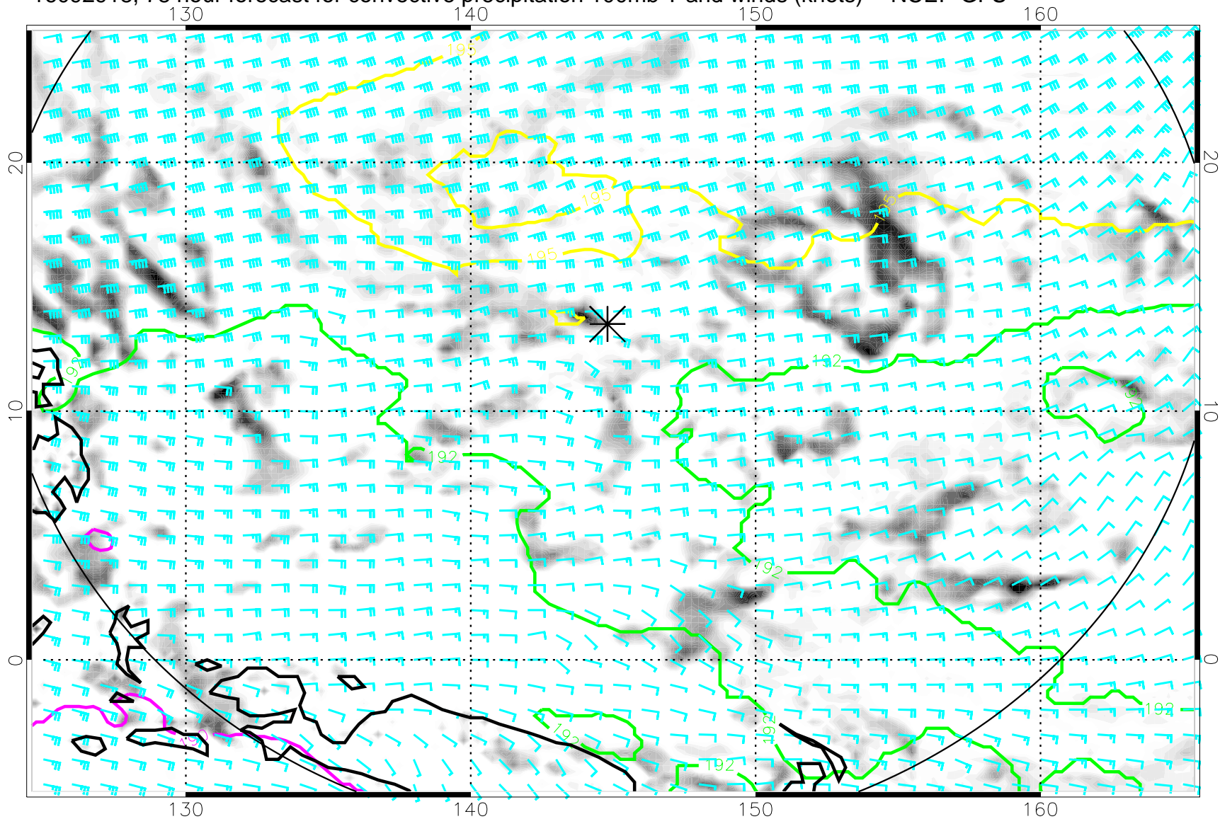
16092918, 78 hour forecast for convective precipitation 100mb T and winds (knots) -- NCEP GFS
