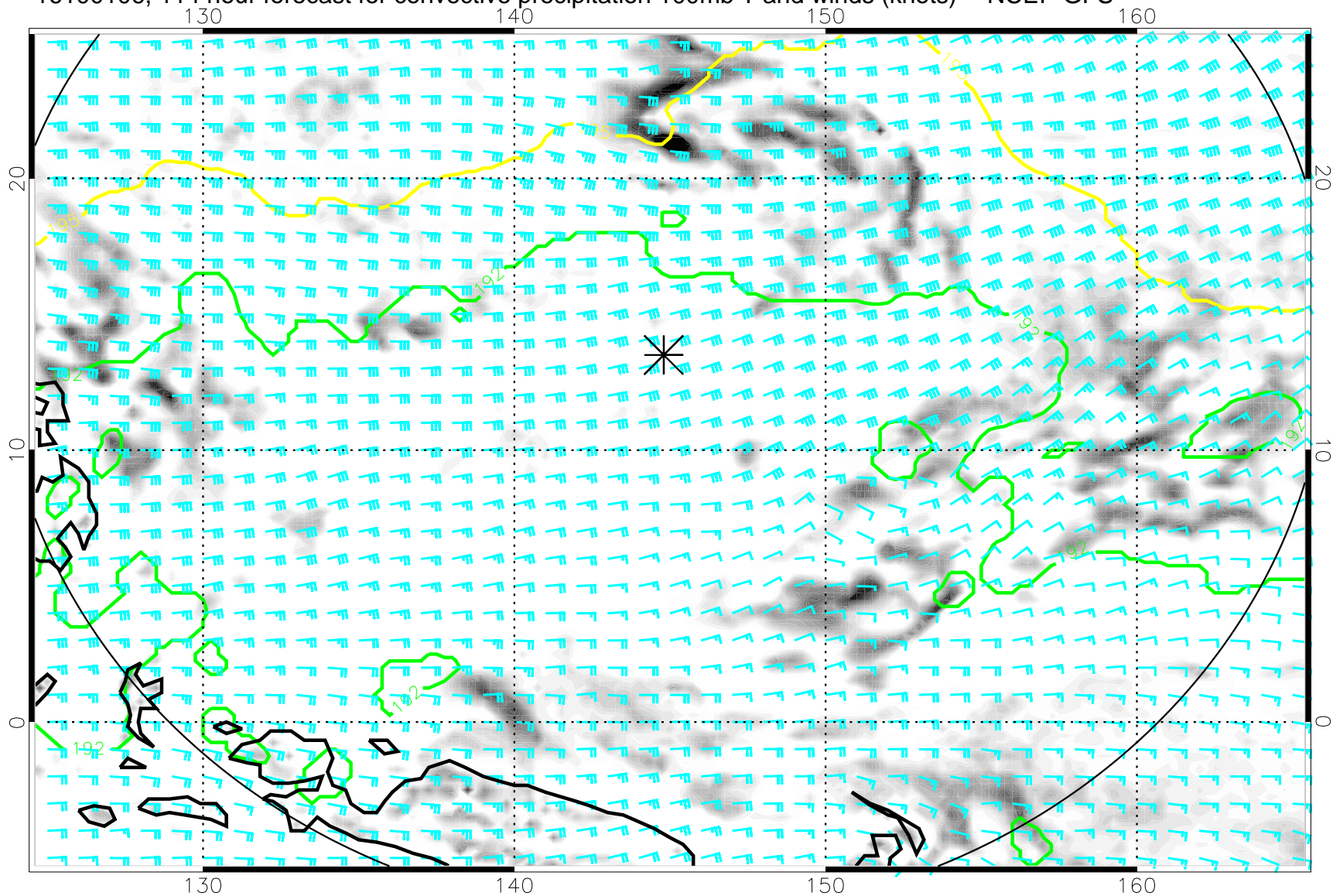
16100106, 114 hour forecast for convective precipitation 100mb T and winds (knots) -- NCEP GFS
