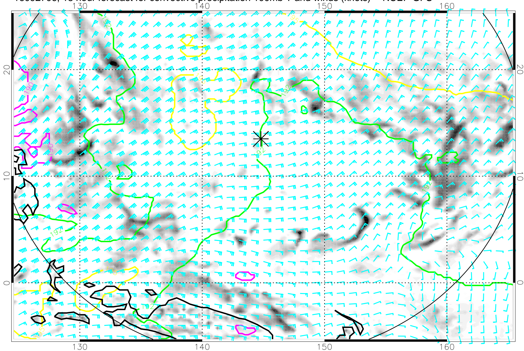
16092706, 18 hour forecast for convective precipitation 100mb T and winds (knots) -- NCEP GFS
