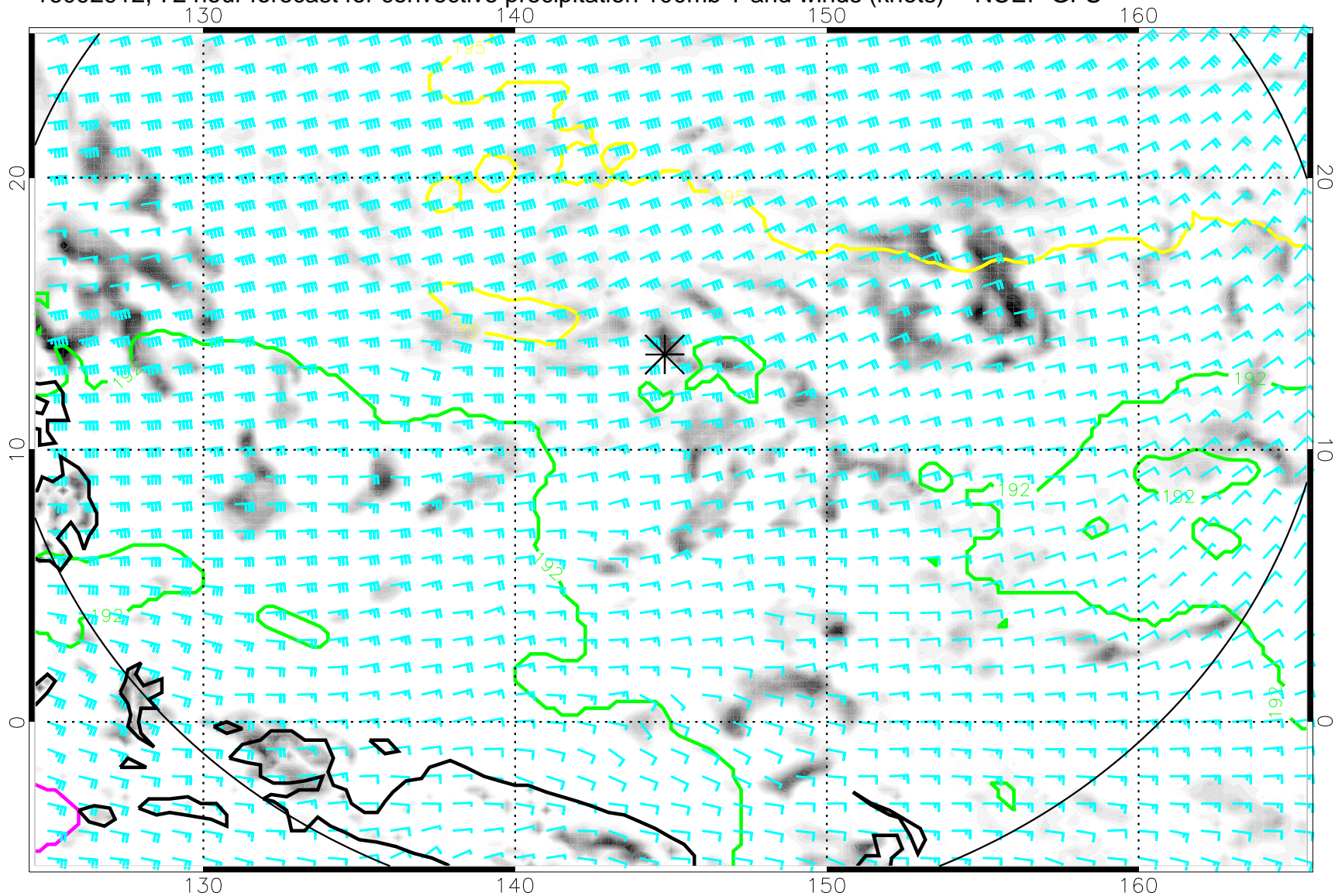
16092912, 72 hour forecast for convective precipitation 100mb T and winds (knots) -- NCEP GFS
