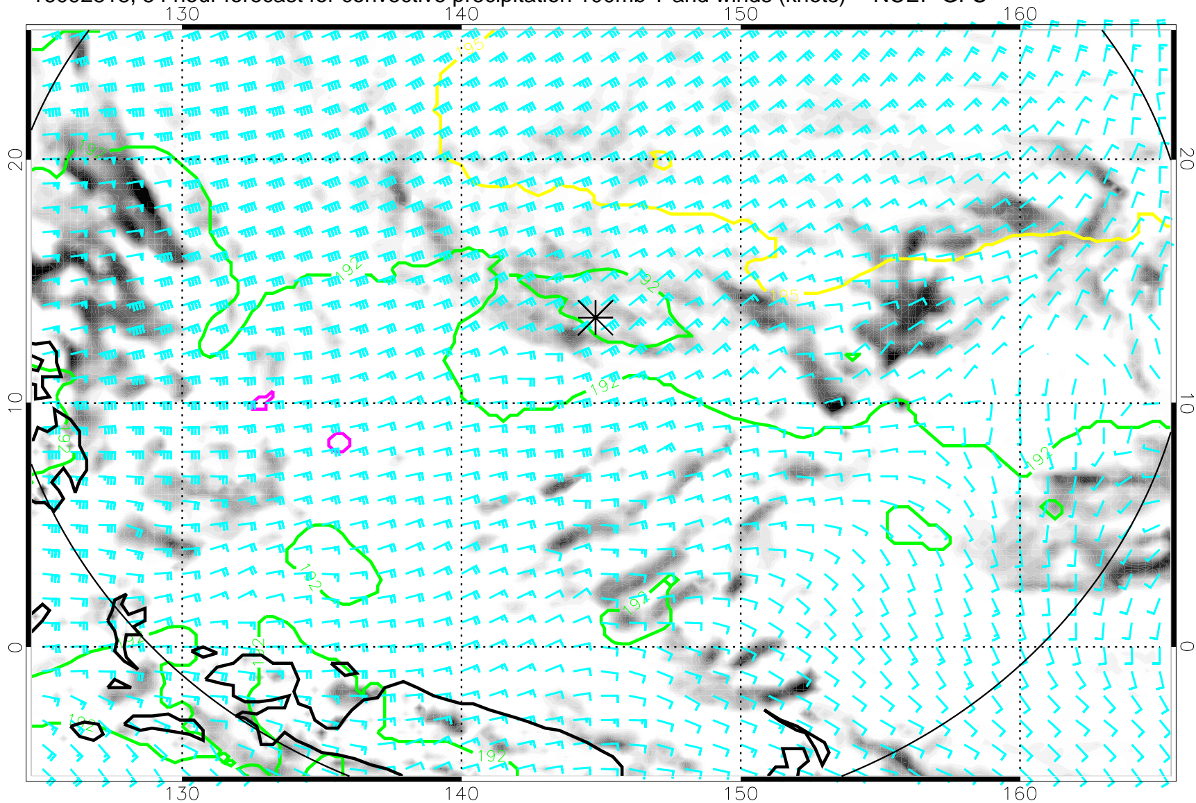
16092818, 54 hour forecast for convective precipitation 100mb T and winds (knots) -- NCEP GFS
