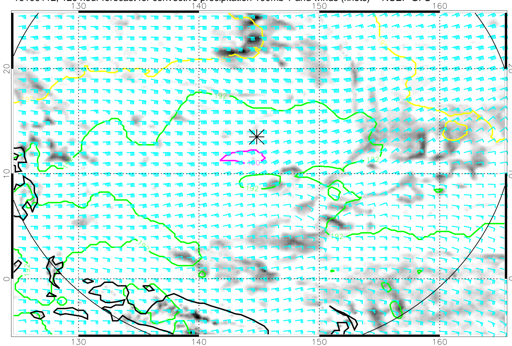
16100112, 120 hour forecast for convective precipitation 100mb T and winds (knots) -- NCEP GFS
