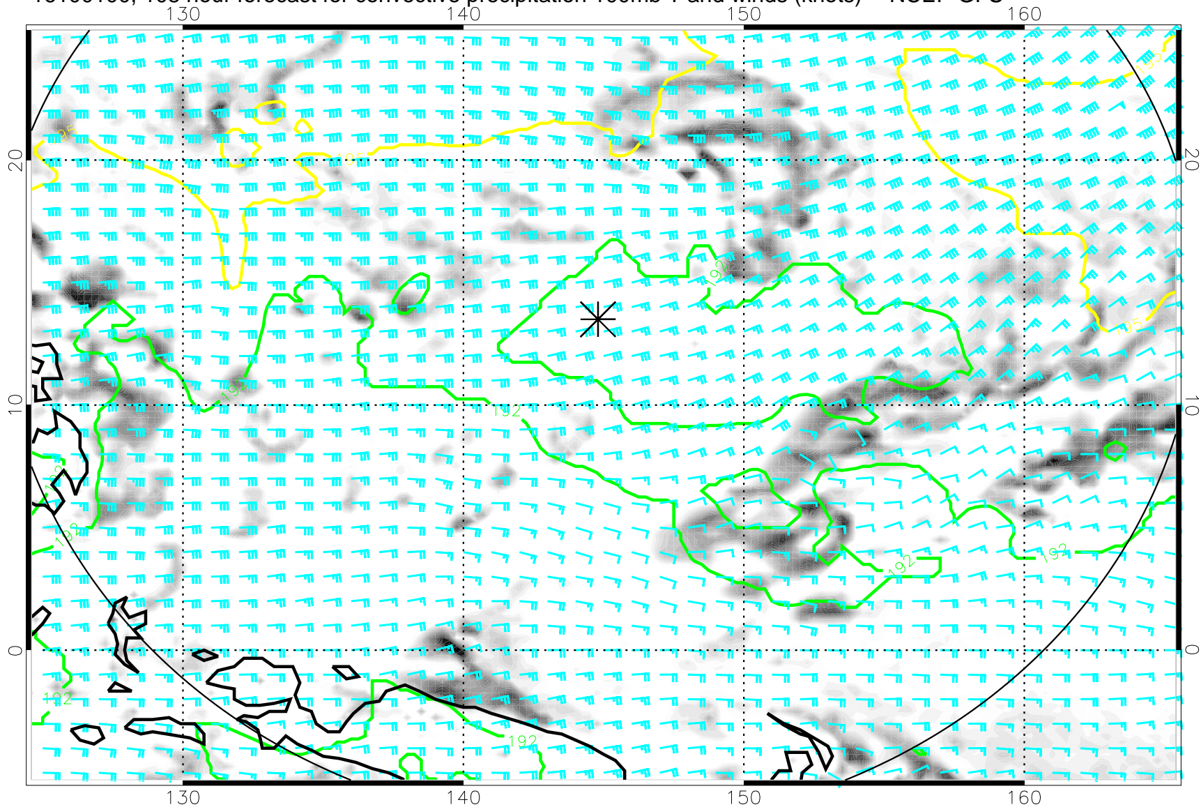
16100100, 108 hour forecast for convective precipitation 100mb T and winds (knots) -- NCEP GFS
