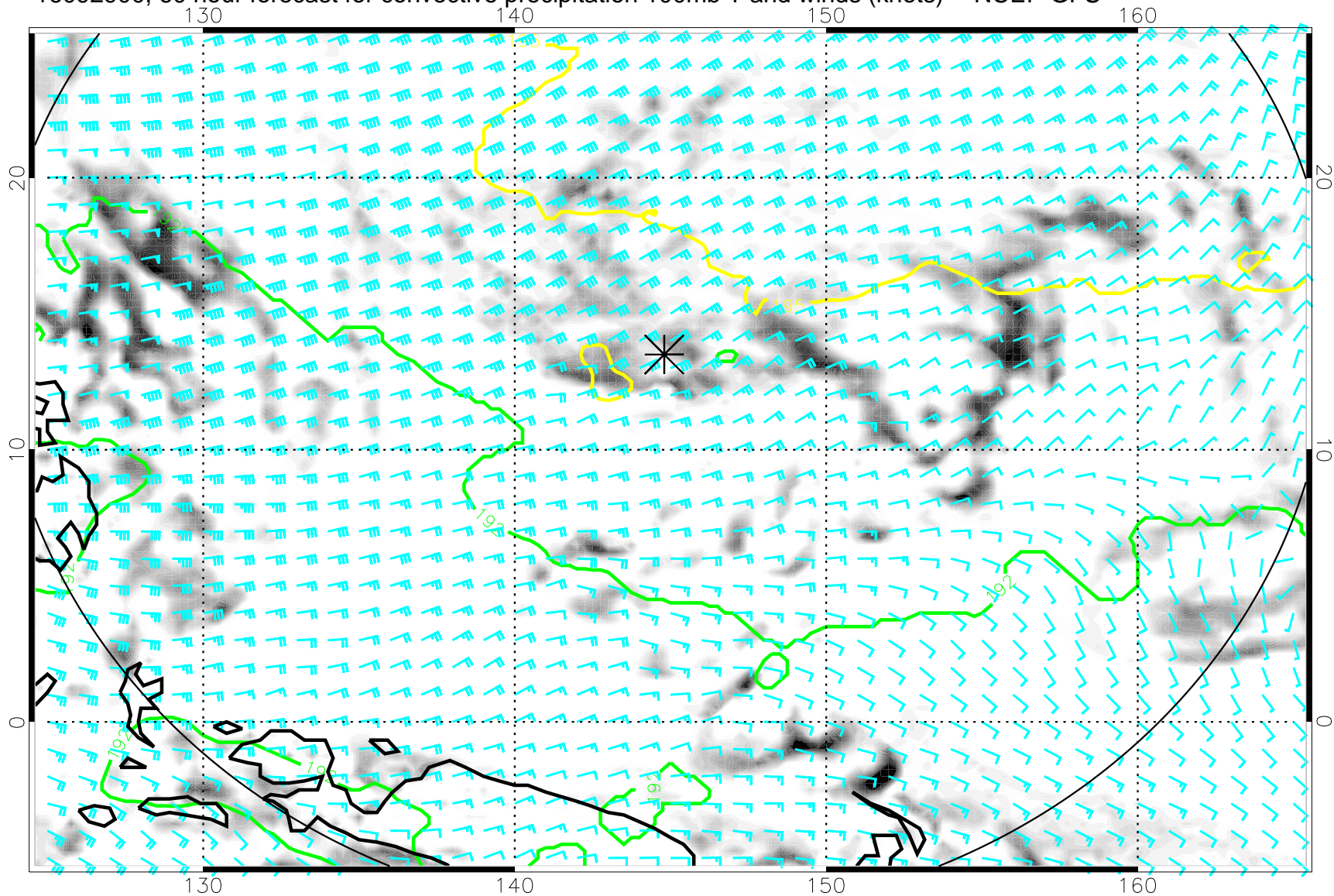
16092900, 60 hour forecast for convective precipitation 100mb T and winds (knots) -- NCEP GFS
