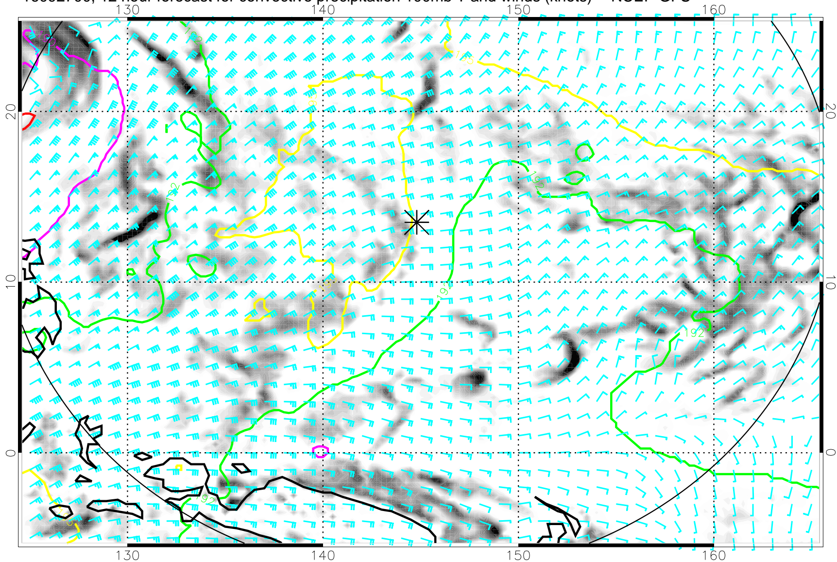
16092700, 12 hour forecast for convective precipitation 100mb T and winds (knots) -- NCEP GFS
