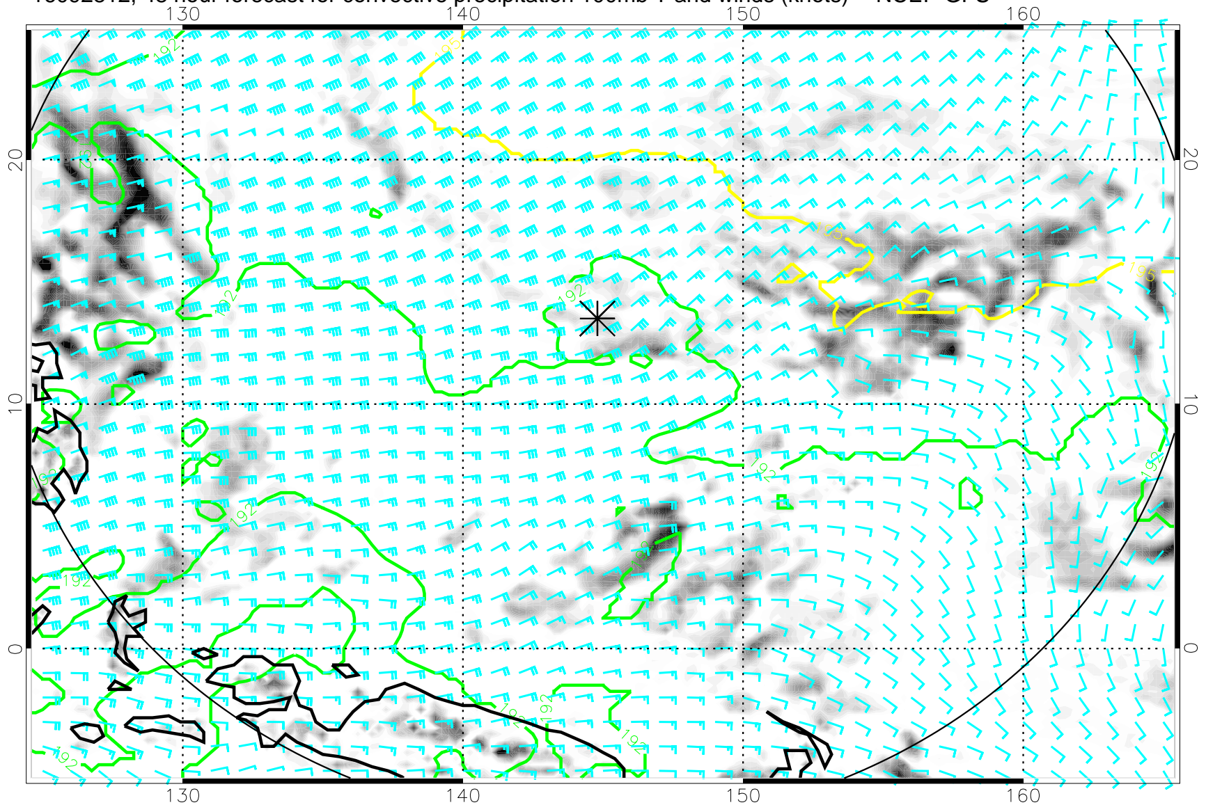
16092812, 48 hour forecast for convective precipitation 100mb T and winds (knots) -- NCEP GFS
