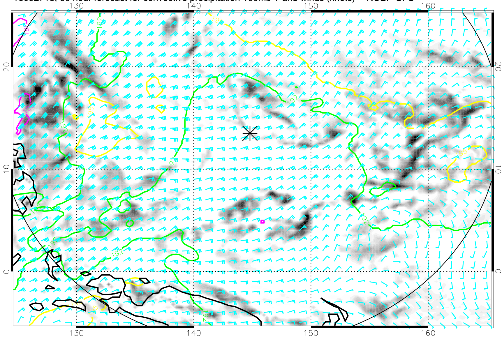
16092718, 30 hour forecast for convective precipitation 100mb T and winds (knots) -- NCEP GFS
