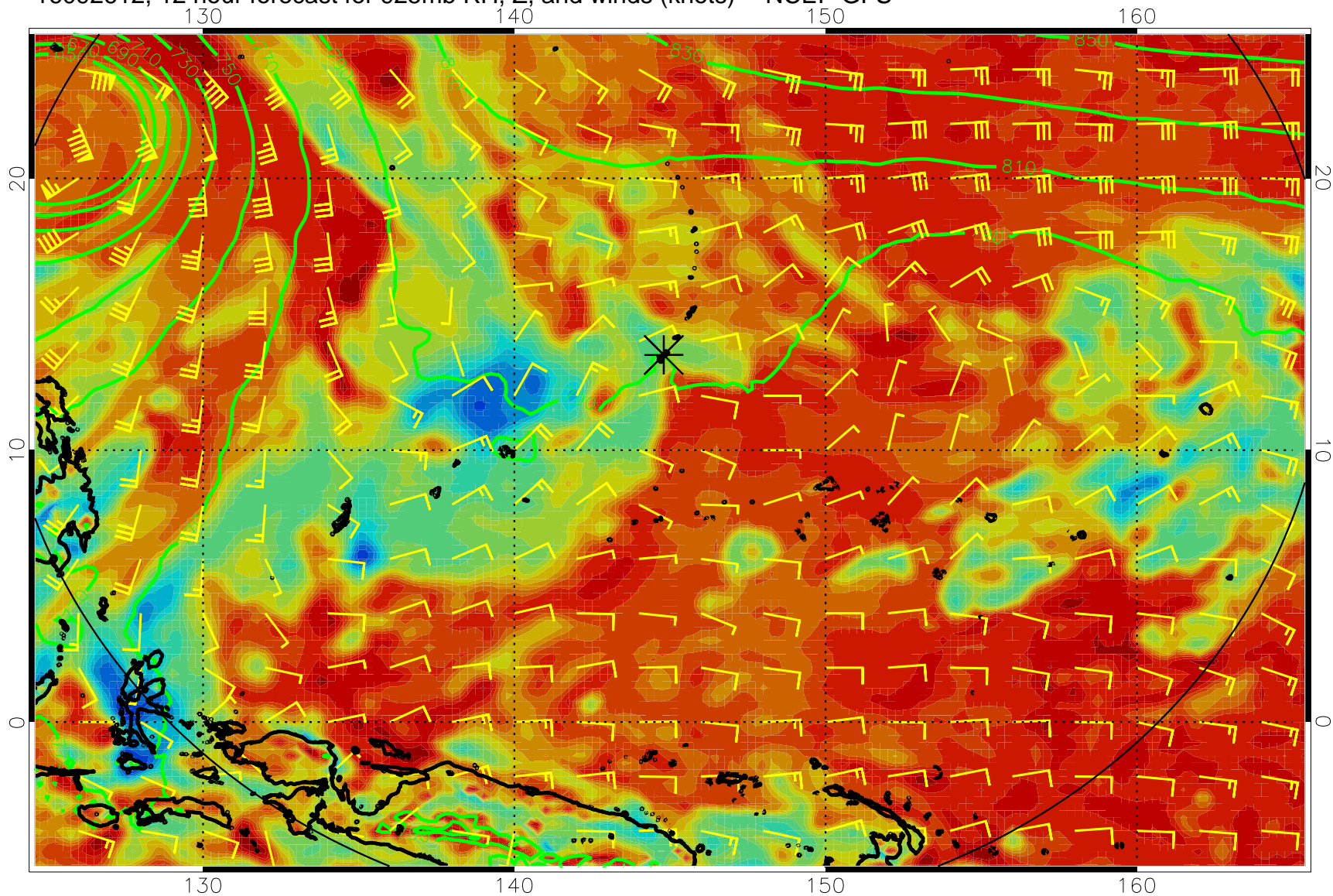
16092612, 12 hour forecast for 925mb RH, Z, and winds (knots) -- NCEP GFS
