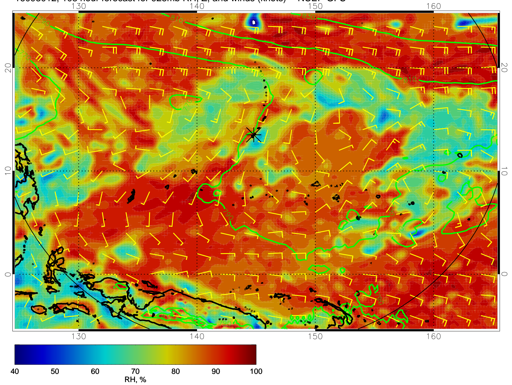
16093012, 108 hour forecast for 925mb RH, Z, and winds (knots) -- NCEP GFS
