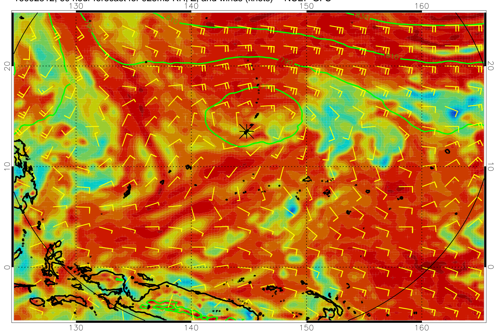
16092812, 60 hour forecast for 925mb RH, Z, and winds (knots) -- NCEP GFS
