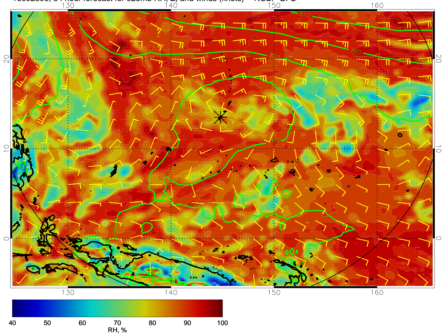
16092806, 54 hour forecast for 925mb RH, Z, and winds (knots) -- NCEP GFS
