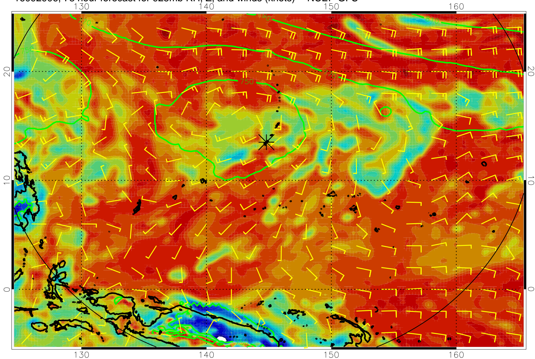
16092906, 78 hour forecast for 925mb RH, Z, and winds (knots) -- NCEP GFS
