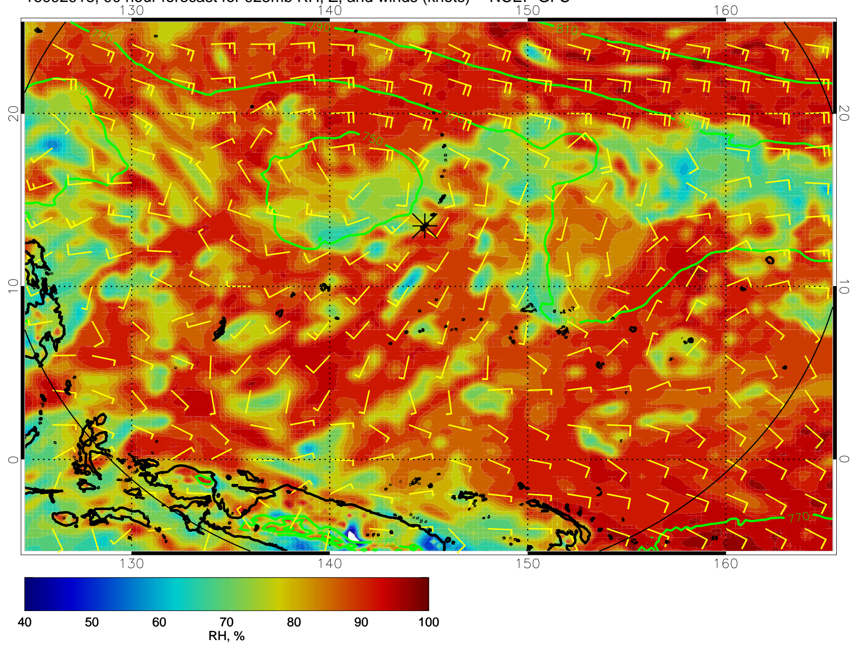
16092918, 90 hour forecast for 925mb RH, Z, and winds (knots) -- NCEP GFS
