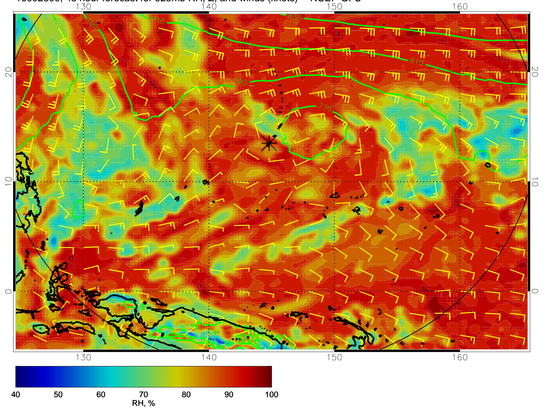
16092800, 48 hour forecast for 925mb RH, Z, and winds (knots) -- NCEP GFS
