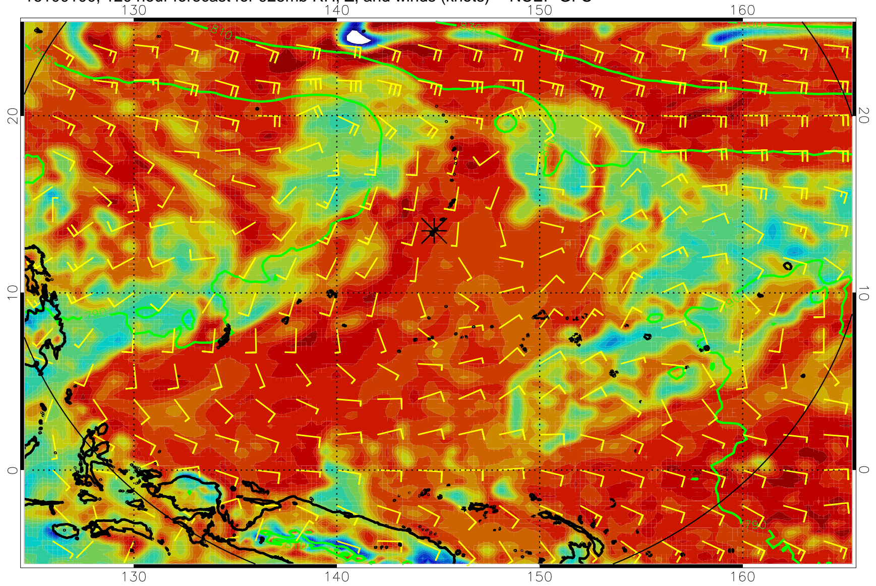
16100100, 120 hour forecast for 925mb RH, Z, and winds (knots) -- NCEP GFS
