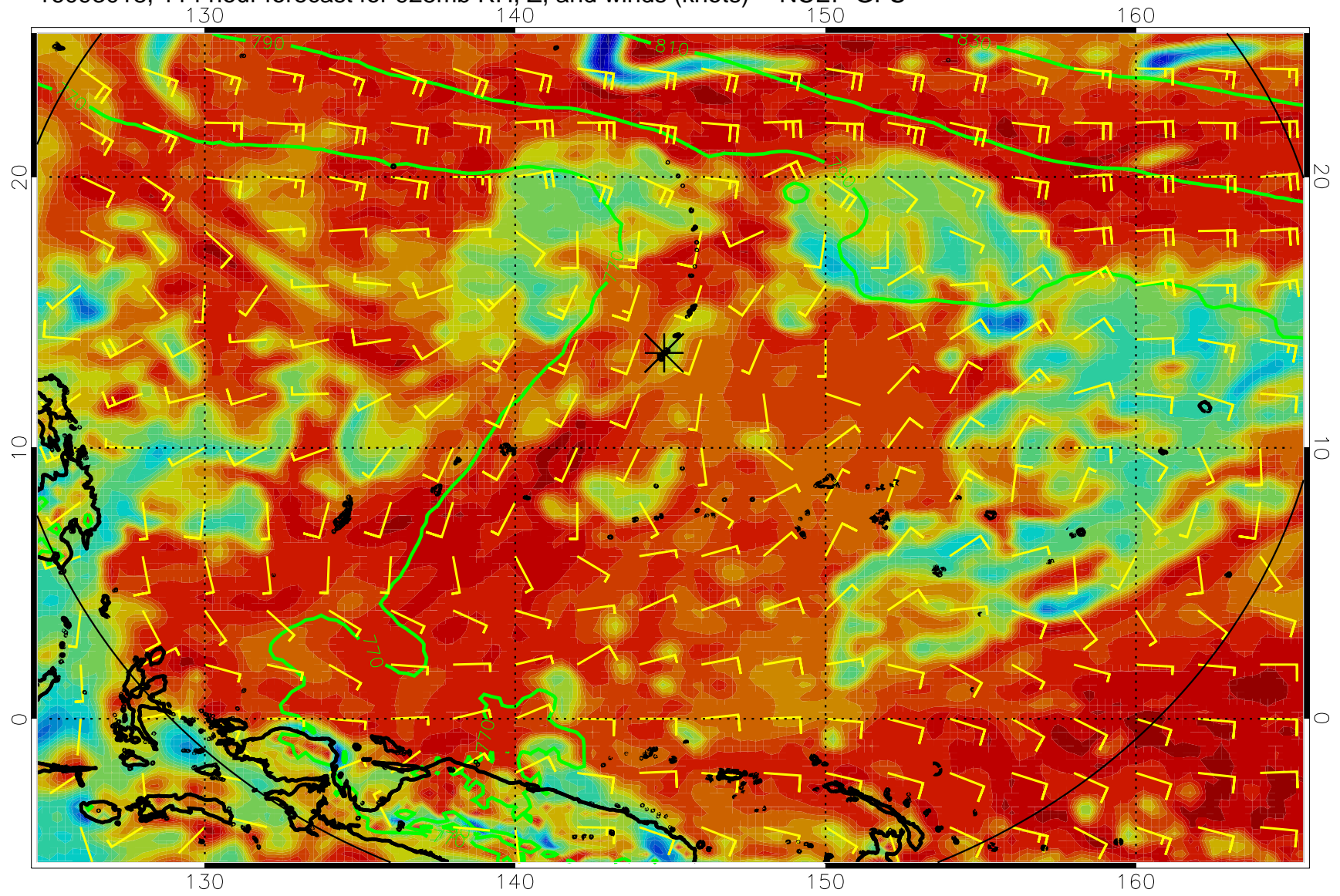
16093018, 114 hour forecast for 925mb RH, Z, and winds (knots) -- NCEP GFS
