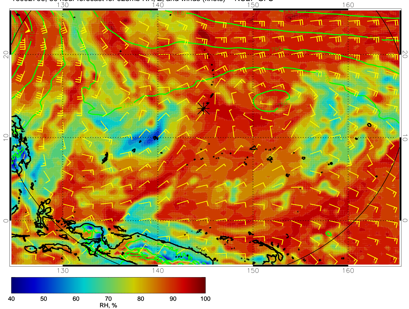
16092706, 30 hour forecast for 925mb RH, Z, and winds (knots) -- NCEP GFS
