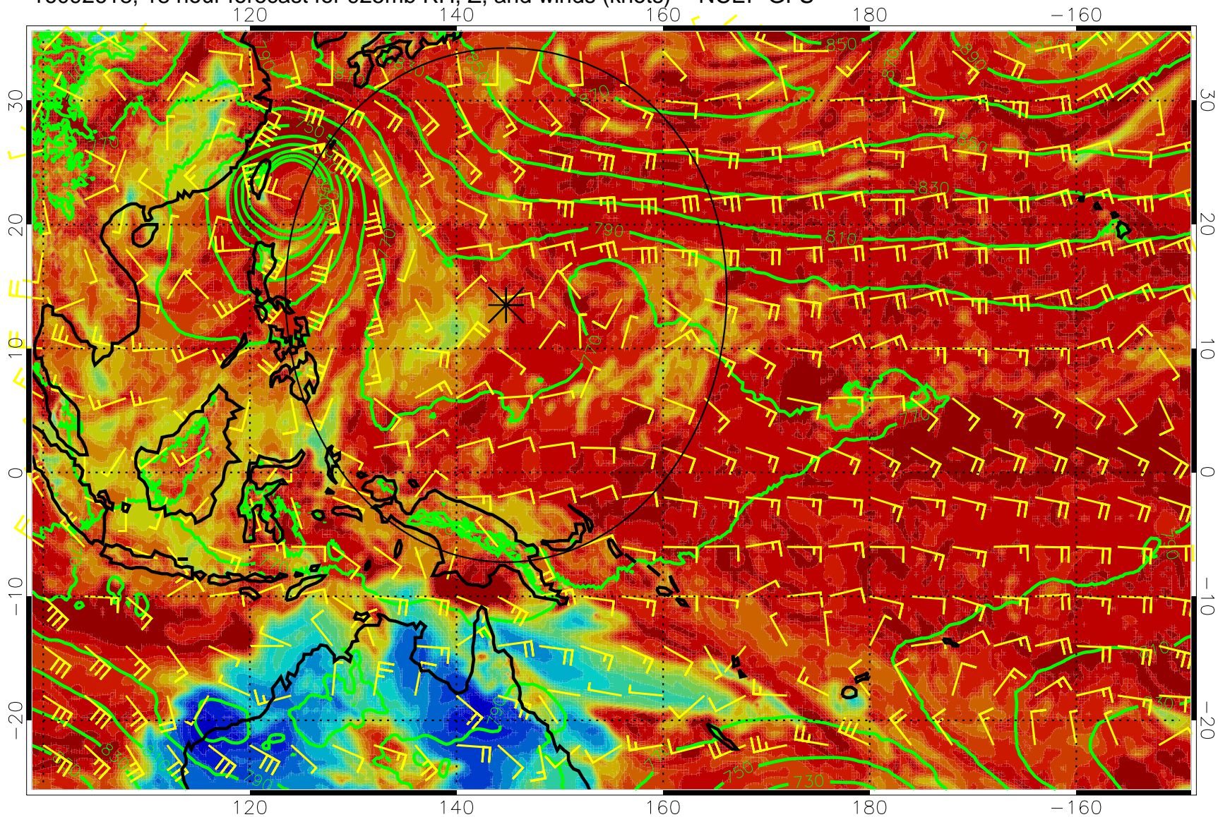
16092618, 18 hour forecast for 925mb RH, Z, and winds (knots) -- NCEP GFS
