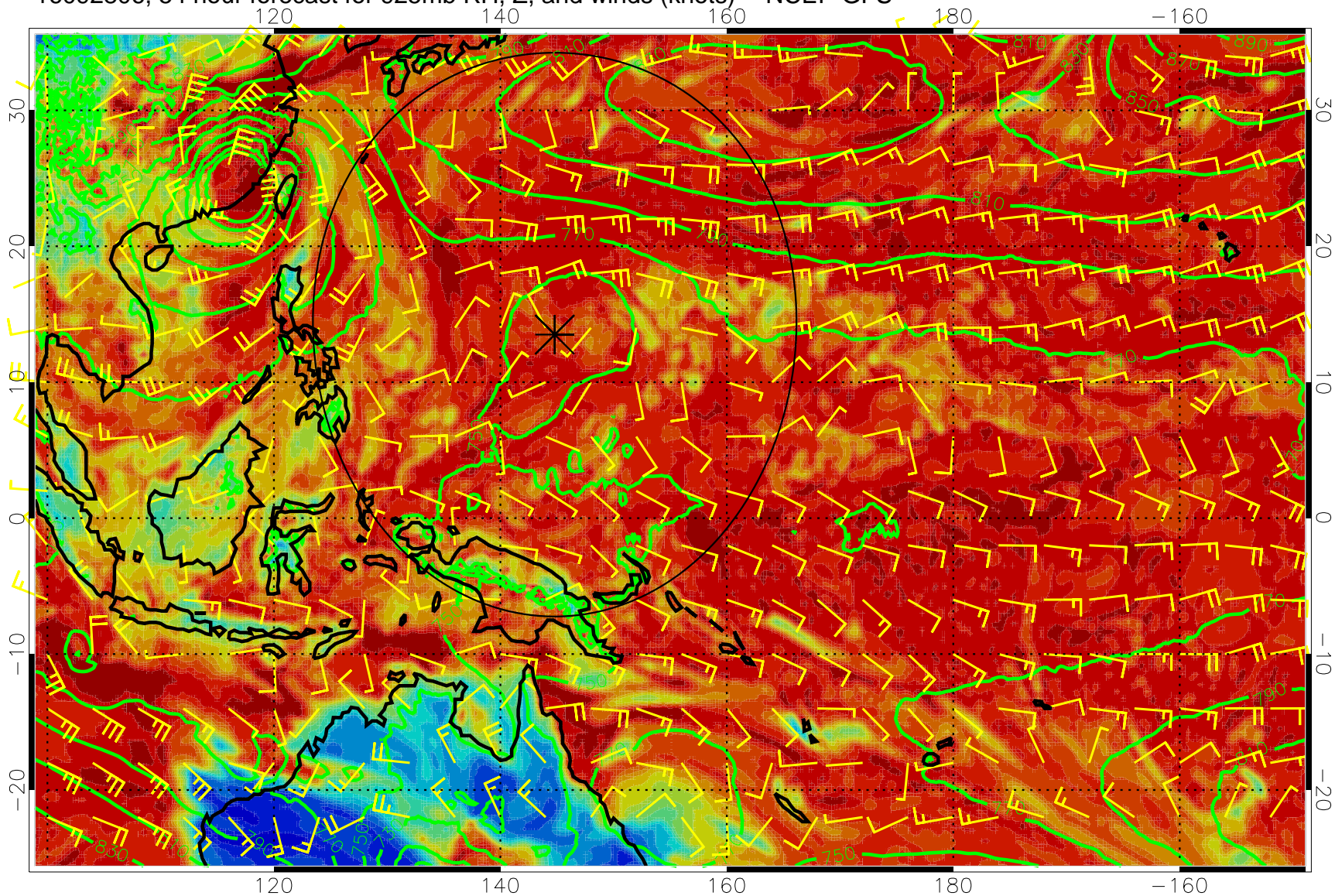
16092806, 54 hour forecast for 925mb RH, Z, and winds (knots) -- NCEP GFS
