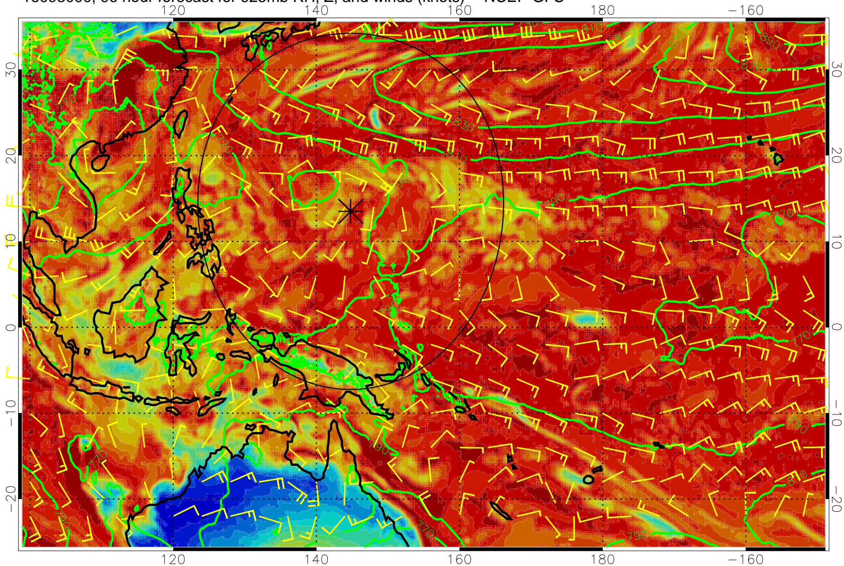
16093000, 96 hour forecast for 925mb RH, Z, and winds (knots) -- NCEP GFS
