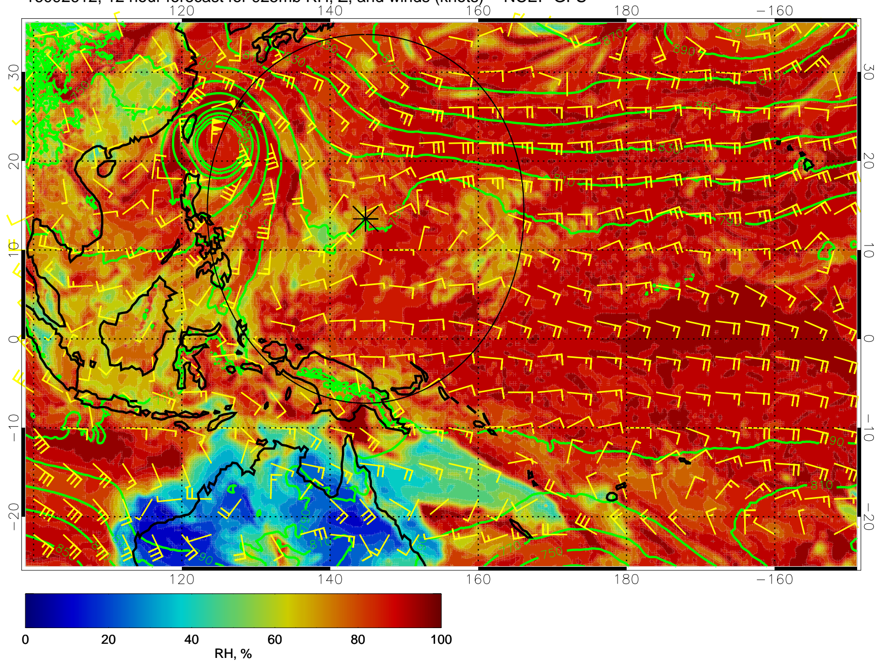
16092612, 12 hour forecast for 925mb RH, Z, and winds (knots) -- NCEP GFS
