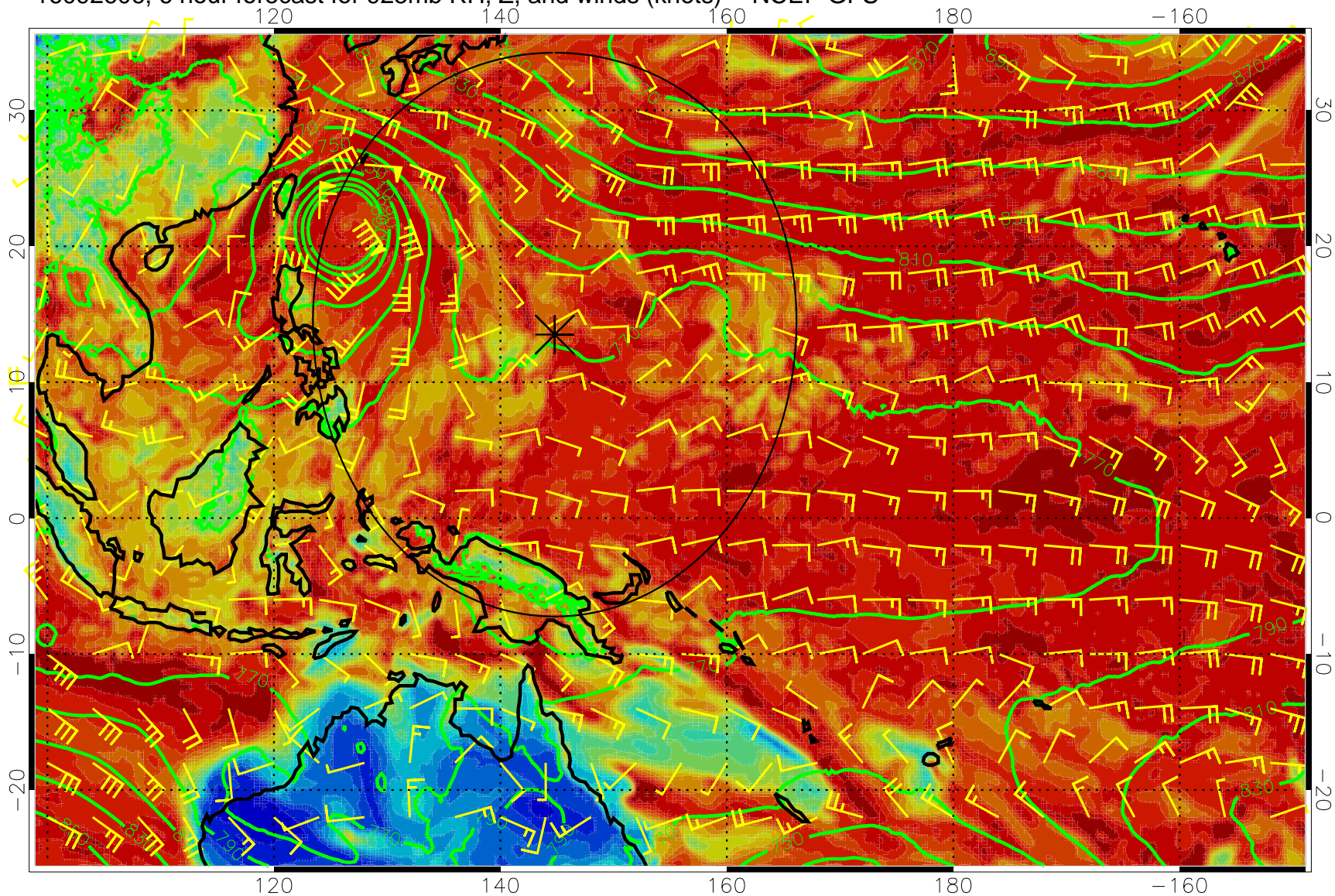
16092606, 6 hour forecast for 925mb RH, Z, and winds (knots) -- NCEP GFS
