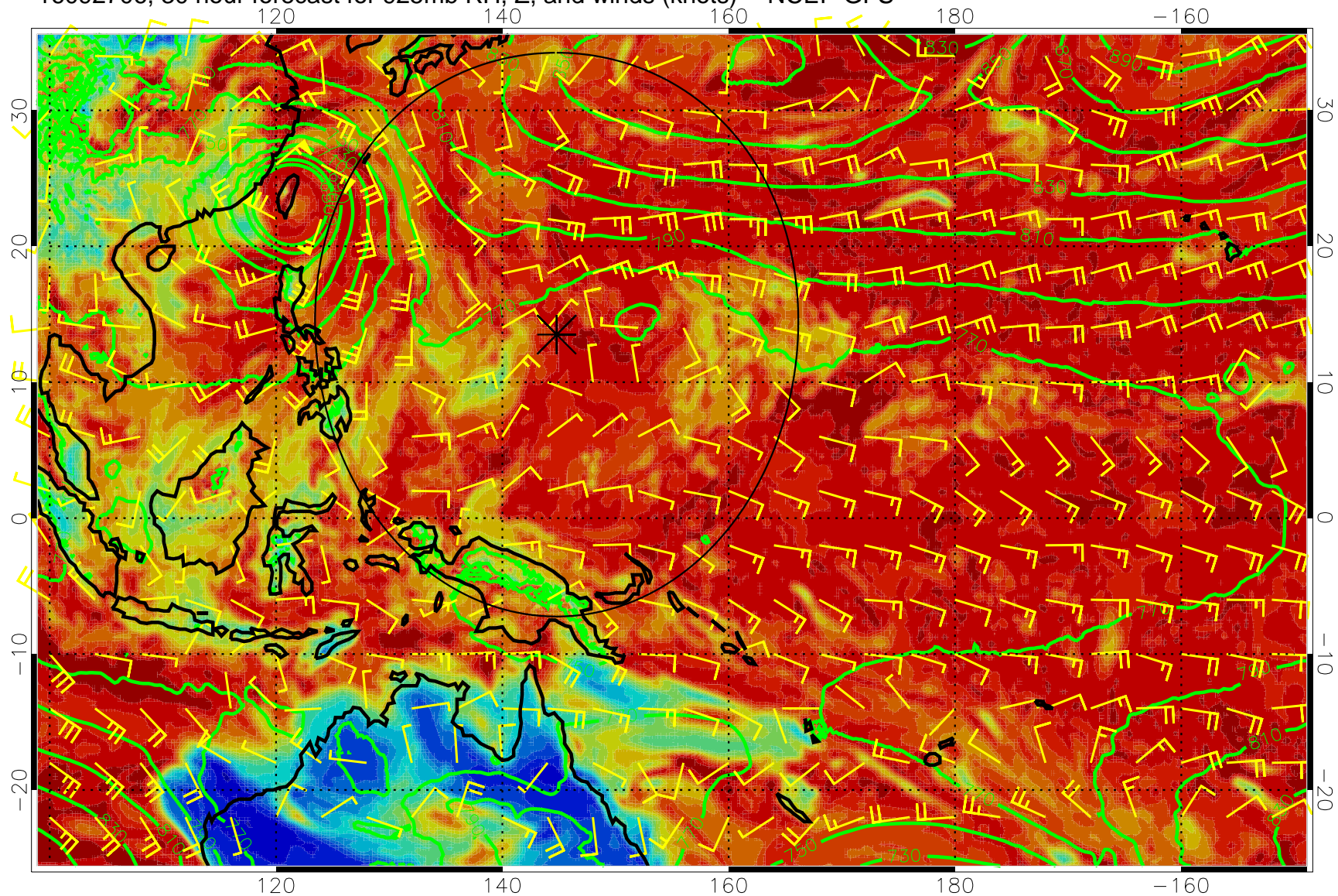
16092706, 30 hour forecast for 925mb RH, Z, and winds (knots) -- NCEP GFS
