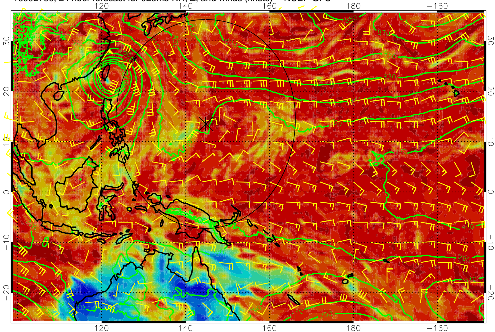
16092700, 24 hour forecast for 925mb RH, Z, and winds (knots) -- NCEP GFS
