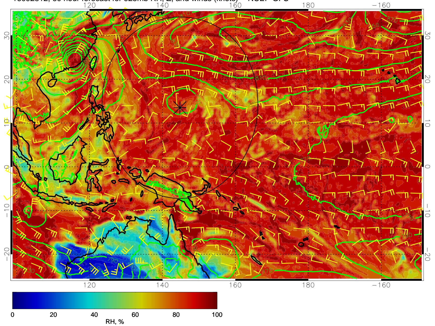
16092812, 60 hour forecast for 925mb RH, Z, and winds (knots) -- NCEP GFS
