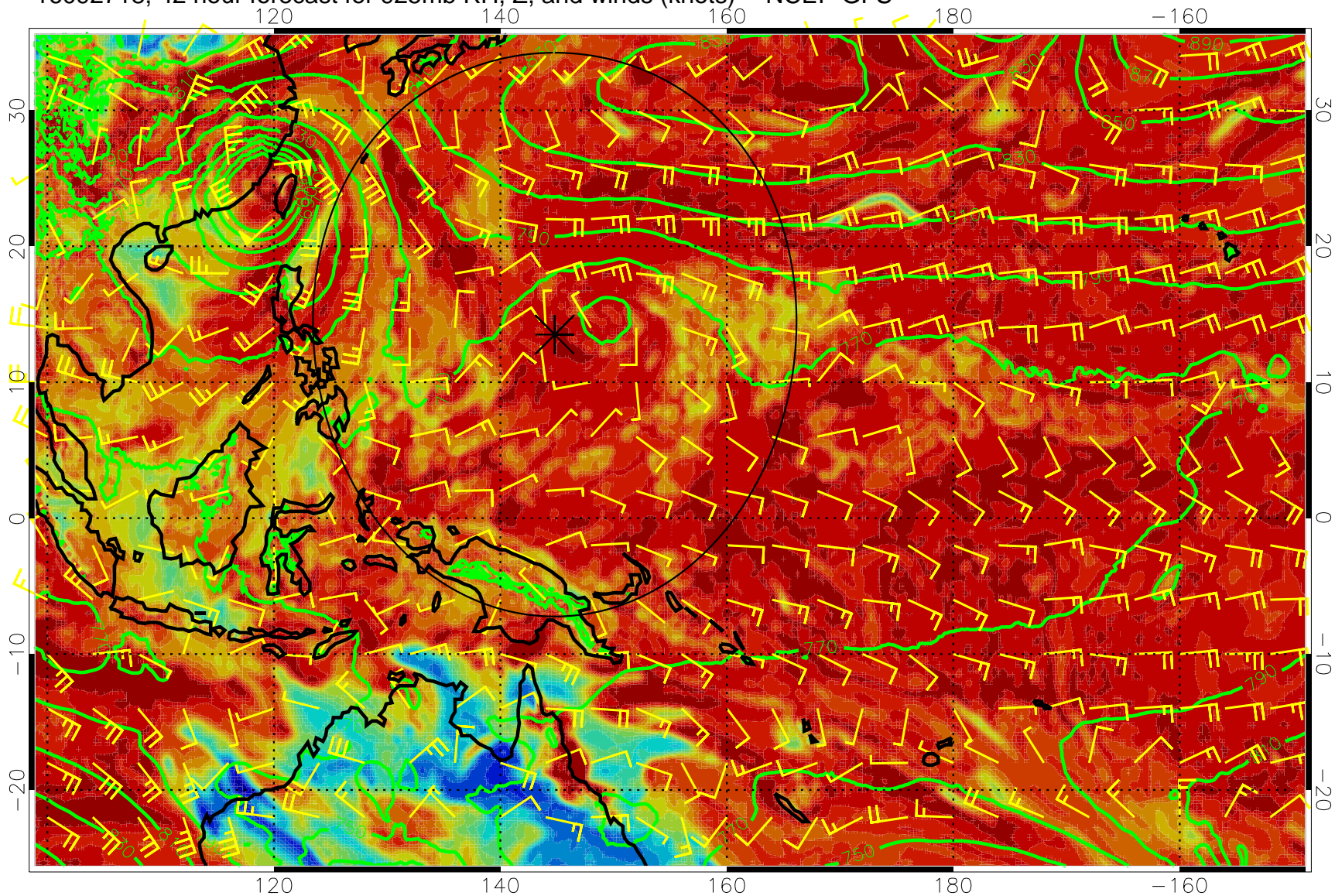
16092718, 42 hour forecast for 925mb RH, Z, and winds (knots) -- NCEP GFS
