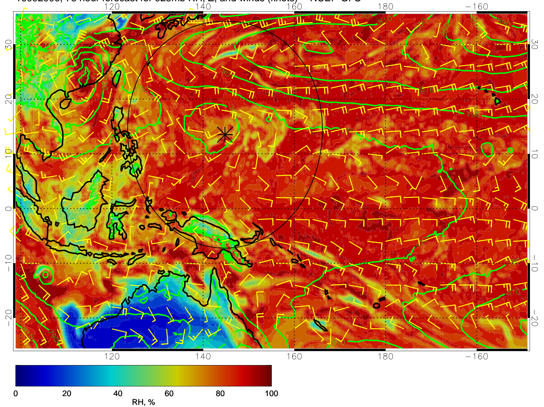
16092906, 78 hour forecast for 925mb RH, Z, and winds (knots) -- NCEP GFS
