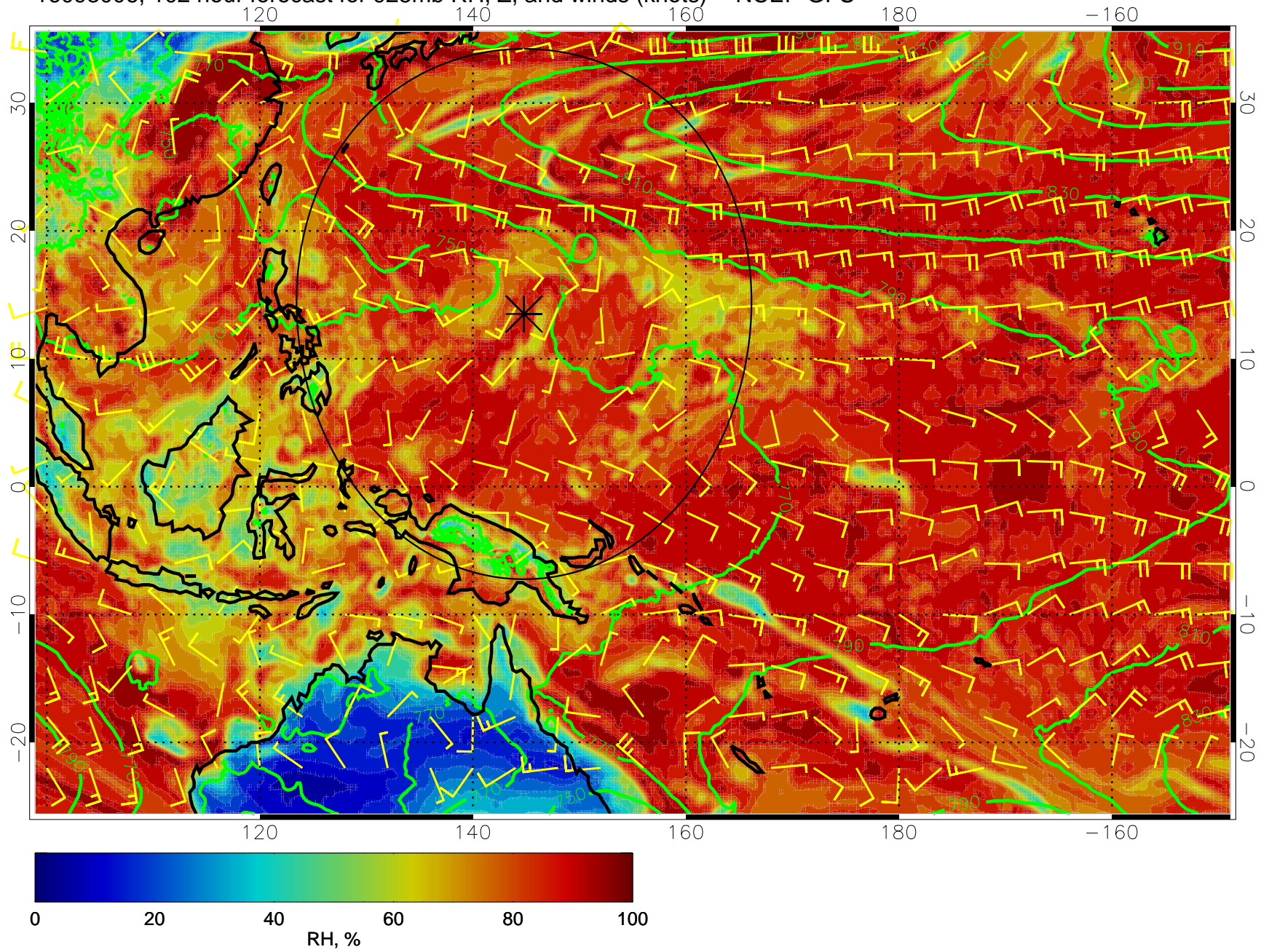
16093006, 102 hour forecast for 925mb RH, Z, and winds (knots) -- NCEP GFS
