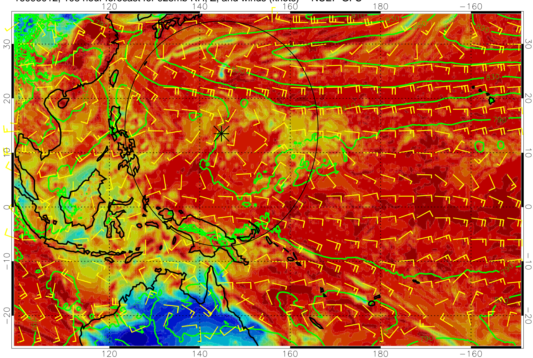
16093012, 108 hour forecast for 925mb RH, Z, and winds (knots) -- NCEP GFS
