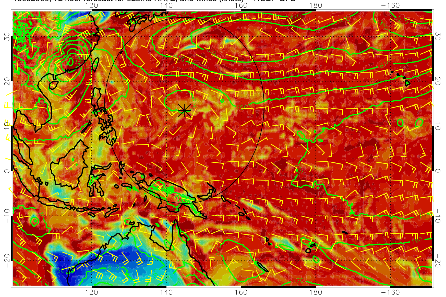
16092900, 72 hour forecast for 925mb RH, Z, and winds (knots) -- NCEP GFS
