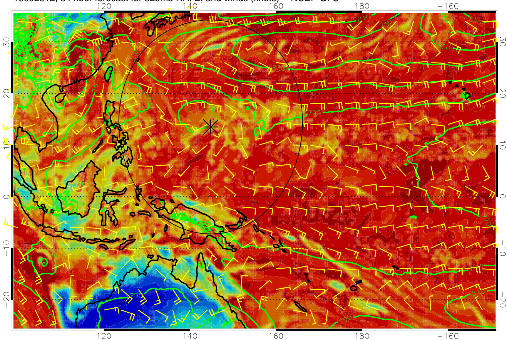
16092912, 84 hour forecast for 925mb RH, Z, and winds (knots) -- NCEP GFS
