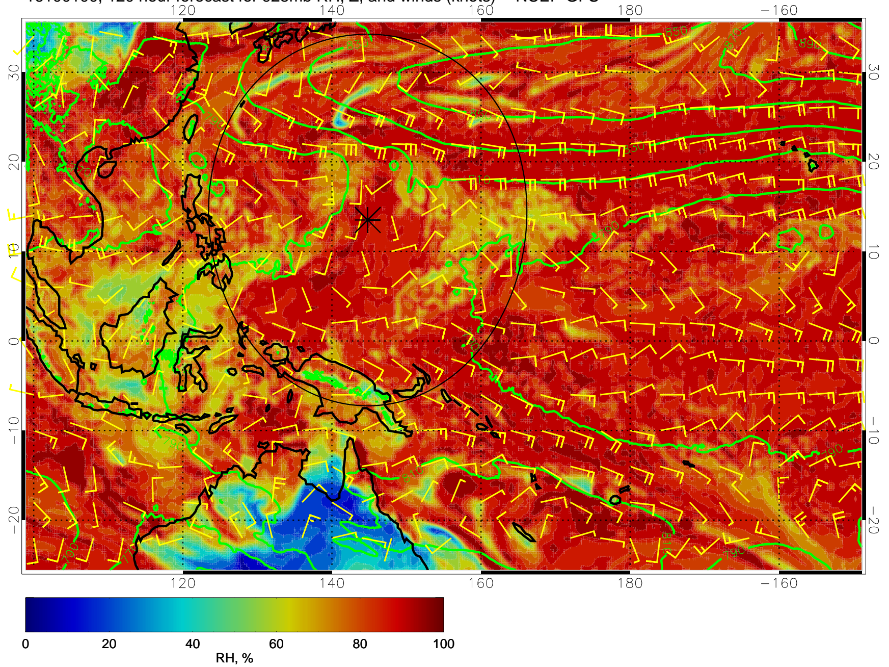
16100100, 120 hour forecast for 925mb RH, Z, and winds (knots) -- NCEP GFS
