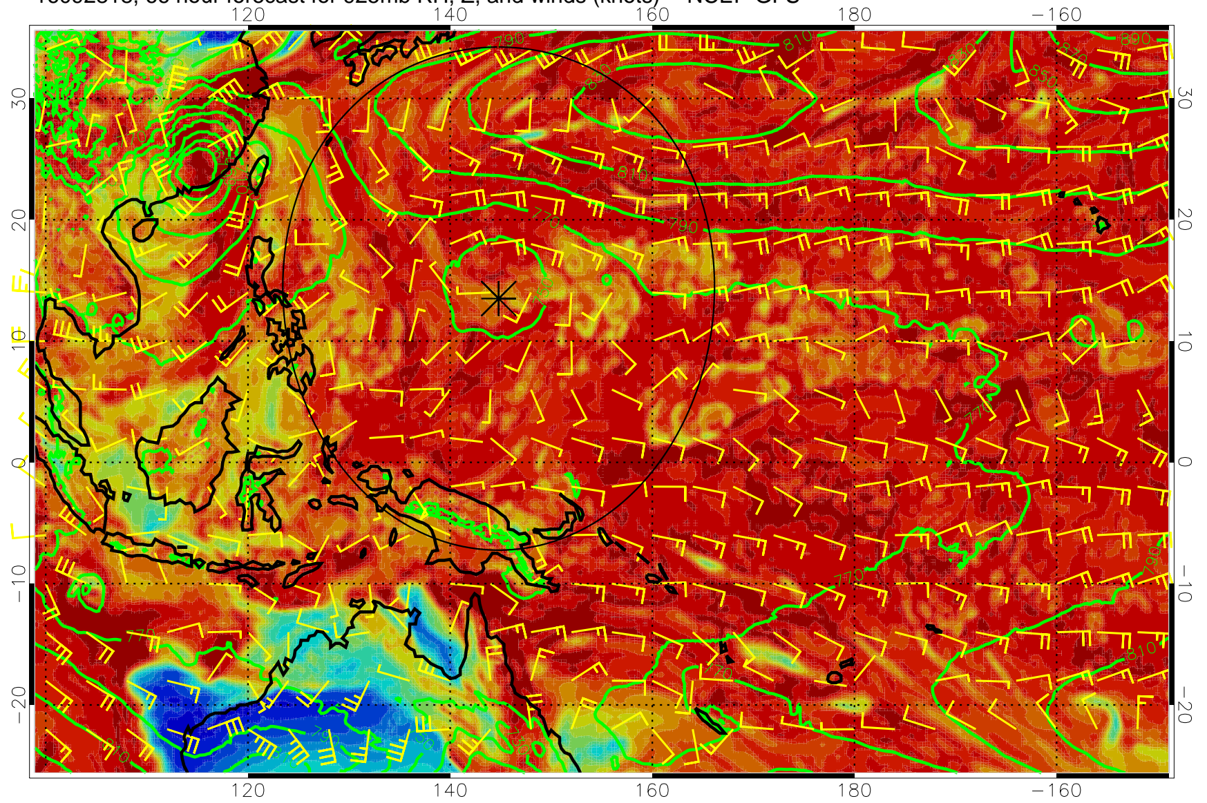
16092818, 66 hour forecast for 925mb RH, Z, and winds (knots) -- NCEP GFS
