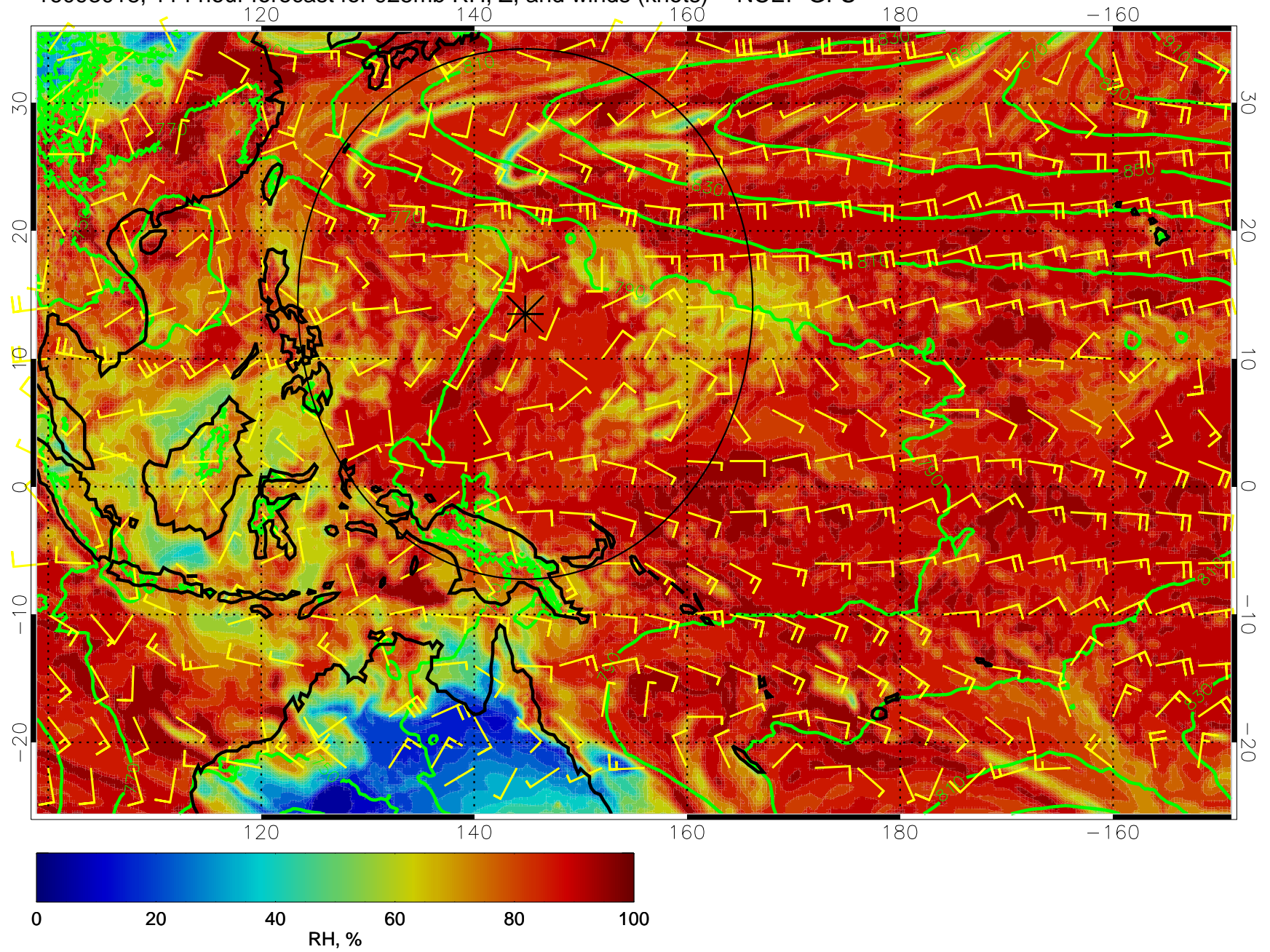
16093018, 114 hour forecast for 925mb RH, Z, and winds (knots) -- NCEP GFS
