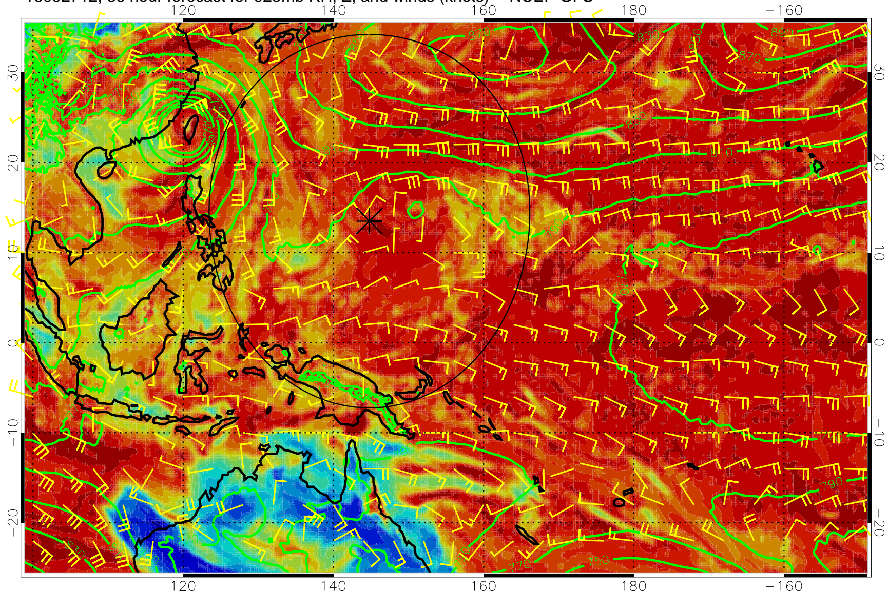
16092712, 36 hour forecast for 925mb RH, Z, and winds (knots) -- NCEP GFS
