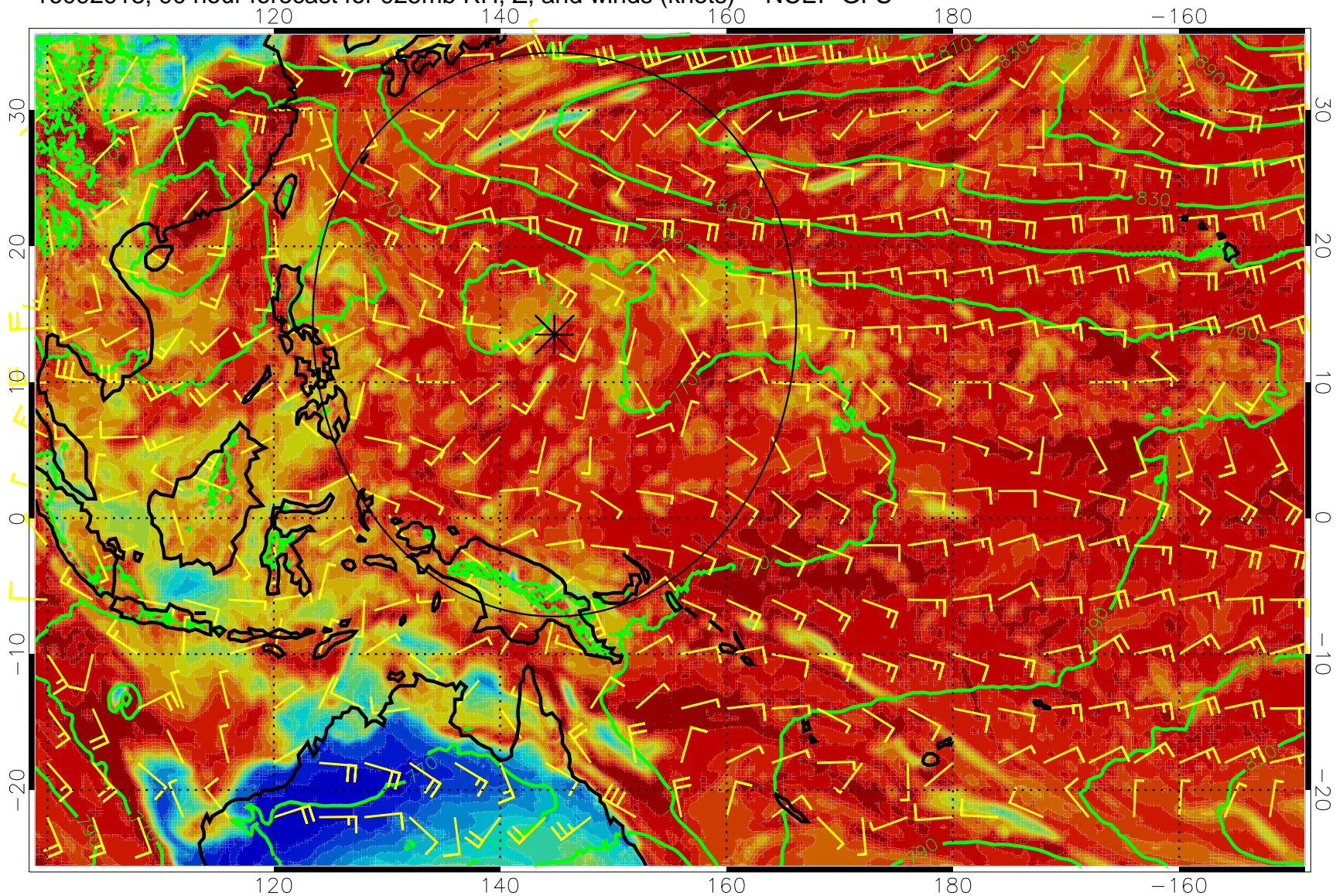
16092918, 90 hour forecast for 925mb RH, Z, and winds (knots) -- NCEP GFS
