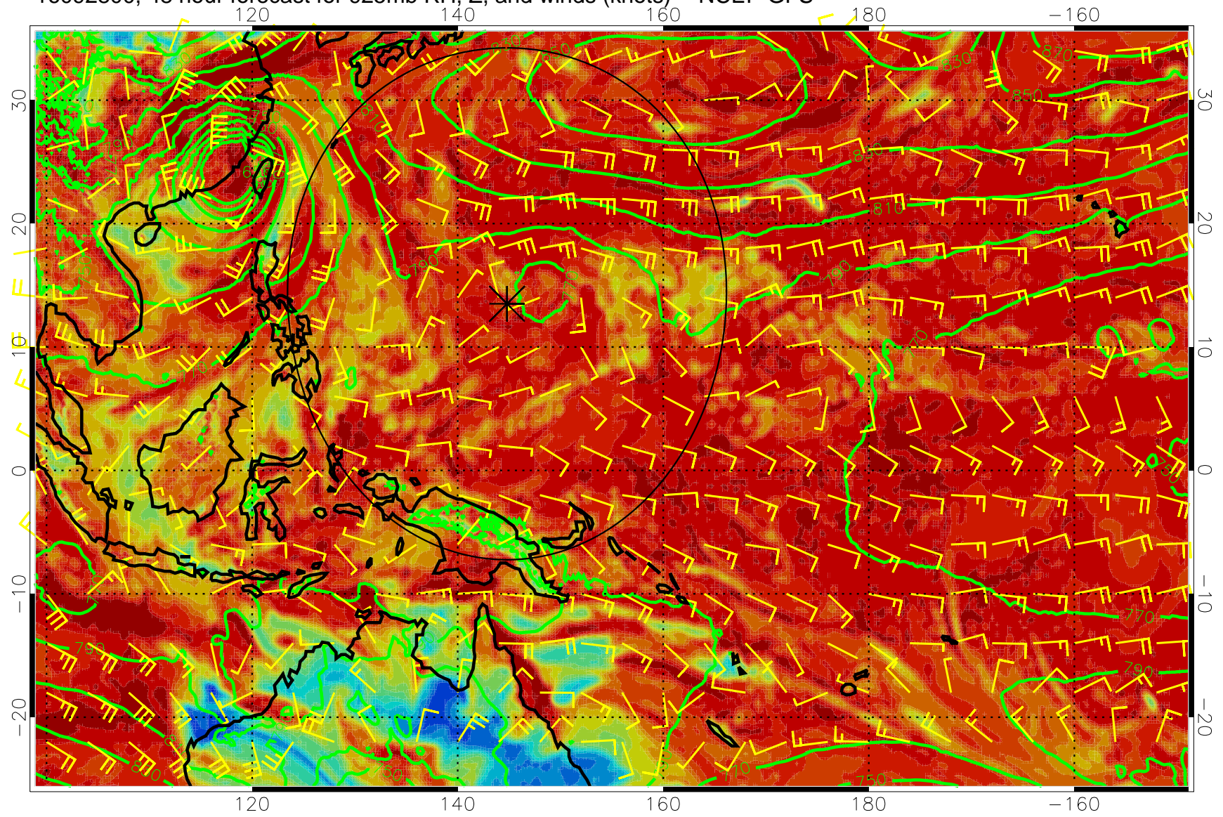
16092800, 48 hour forecast for 925mb RH, Z, and winds (knots) -- NCEP GFS
