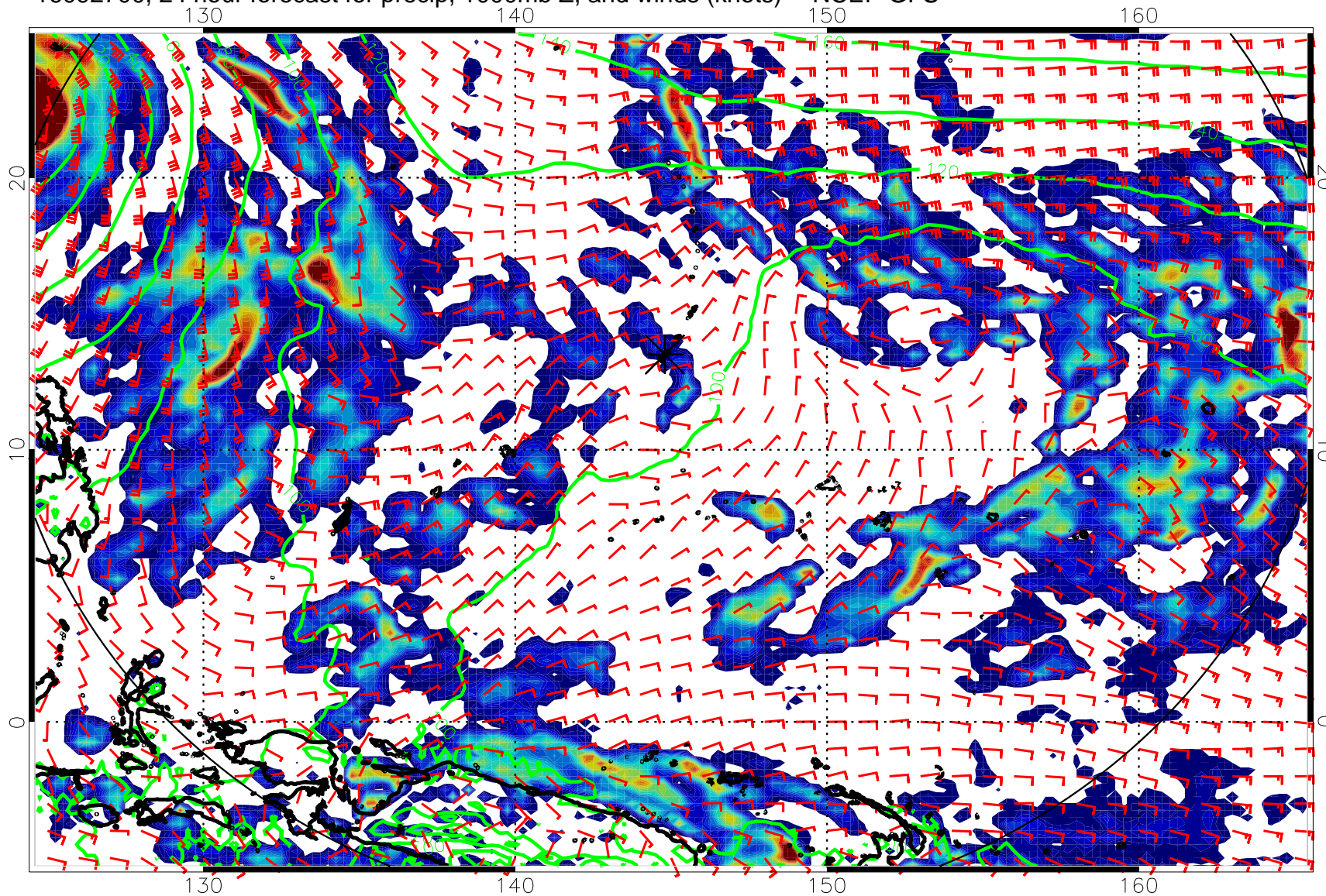
16092700, 24 hour forecast for precip, 1000mb Z, and winds (knots) -- NCEP GFS
