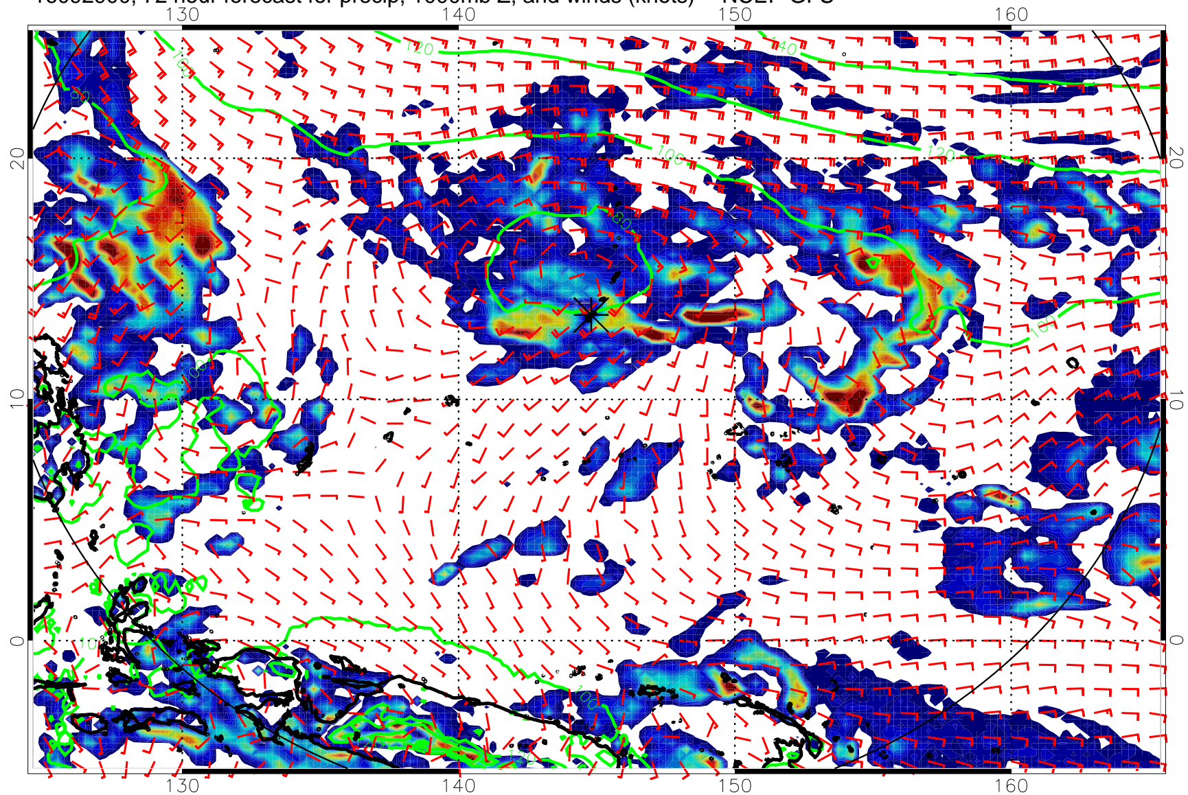
16092900, 72 hour forecast for precip, 1000mb Z, and winds (knots) -- NCEP GFS
