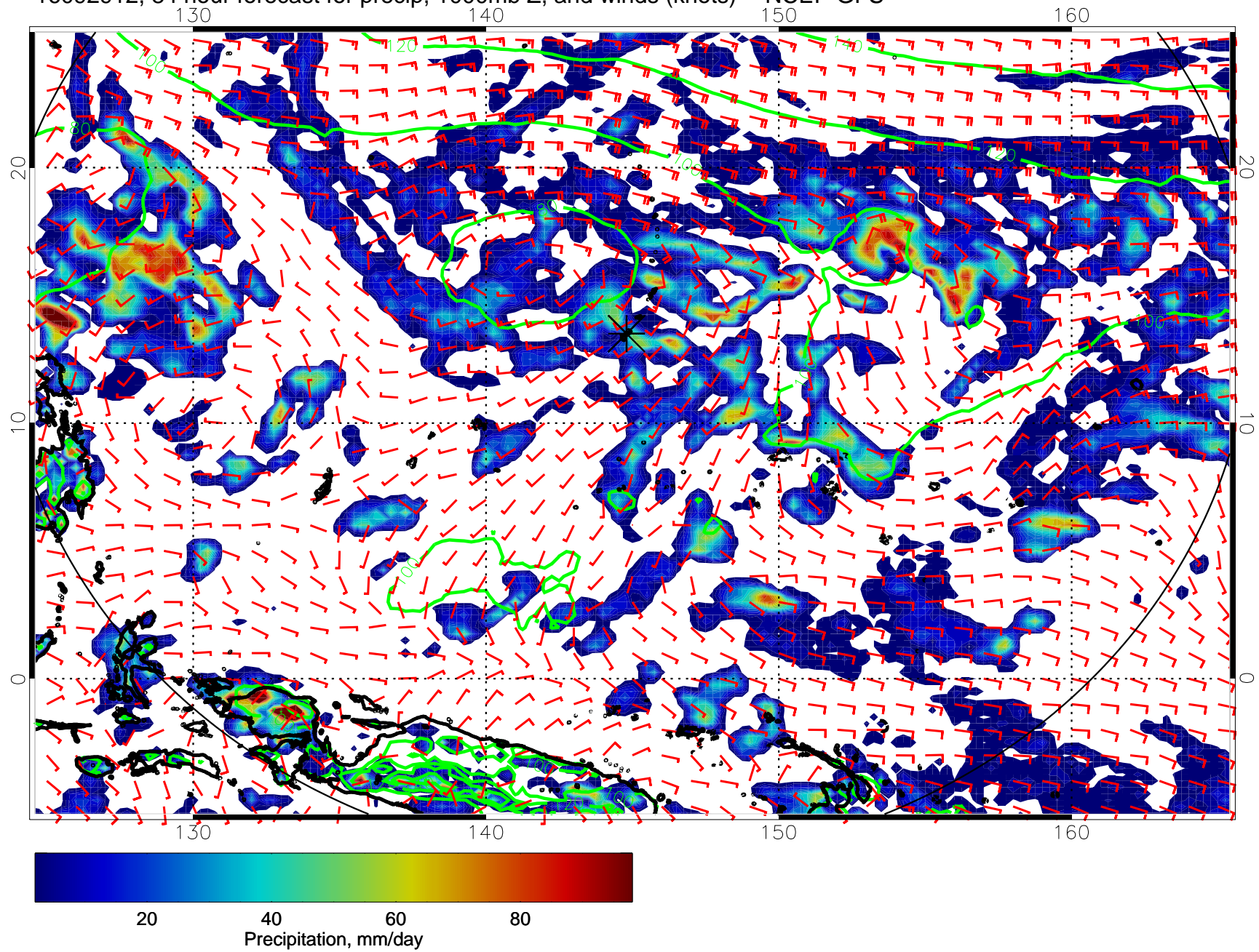
16092912, 84 hour forecast for precip, 1000mb Z, and winds (knots) -- NCEP GFS
