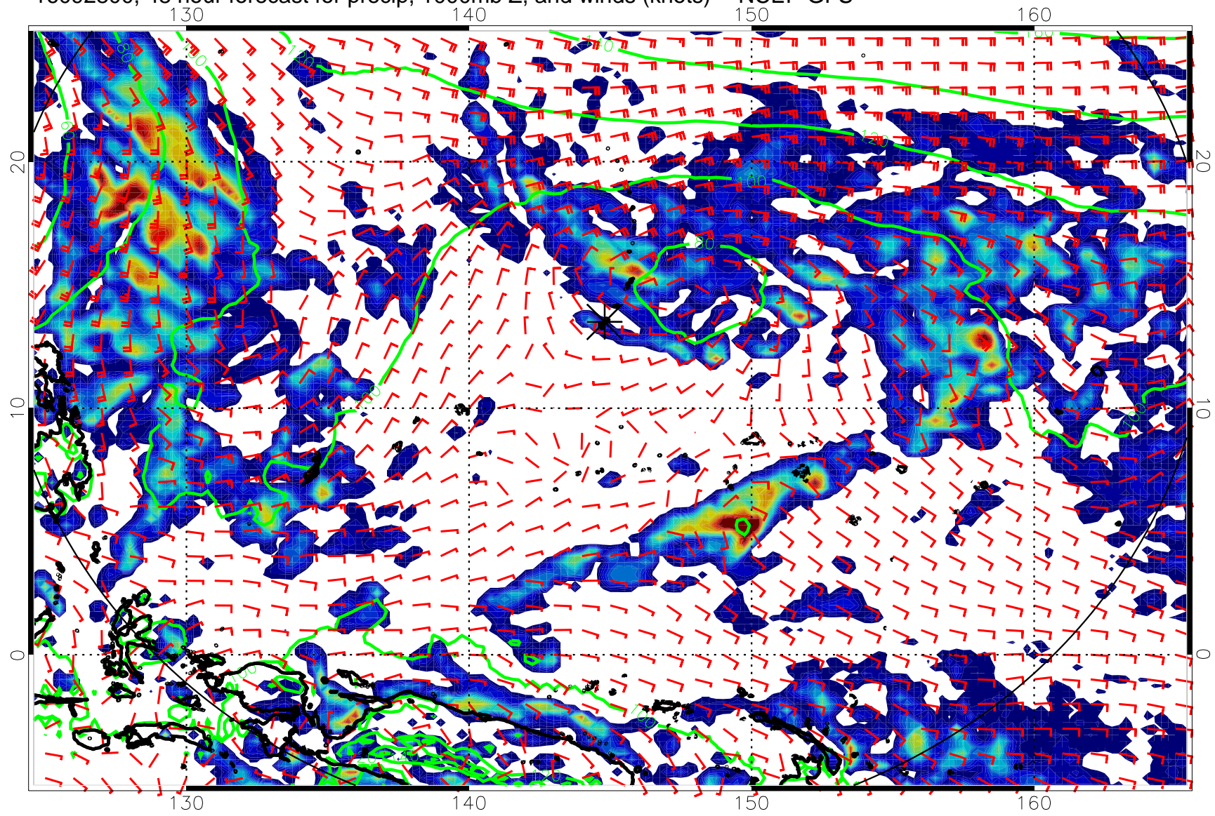
16092800, 48 hour forecast for precip, 1000mb Z, and winds (knots) -- NCEP GFS
