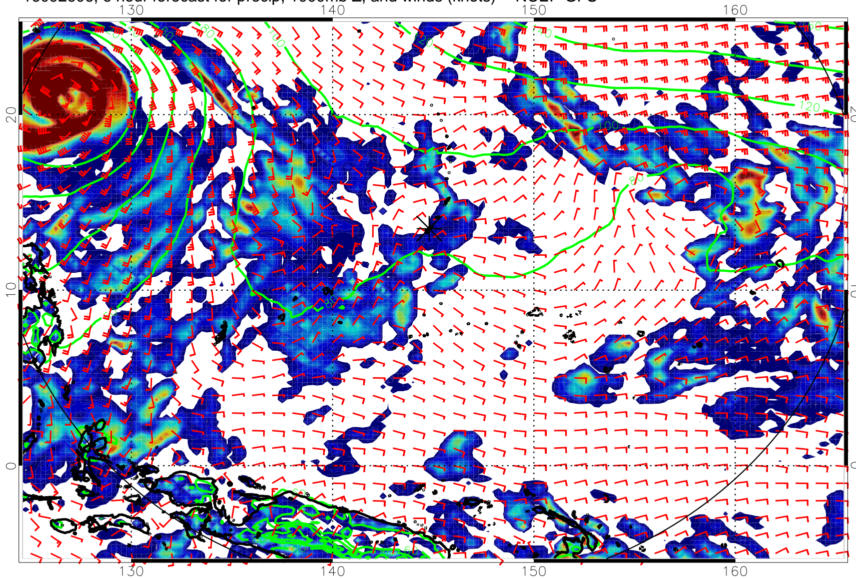
16092606, 6 hour forecast for precip, 1000mb Z, and winds (knots) -- NCEP GFS
