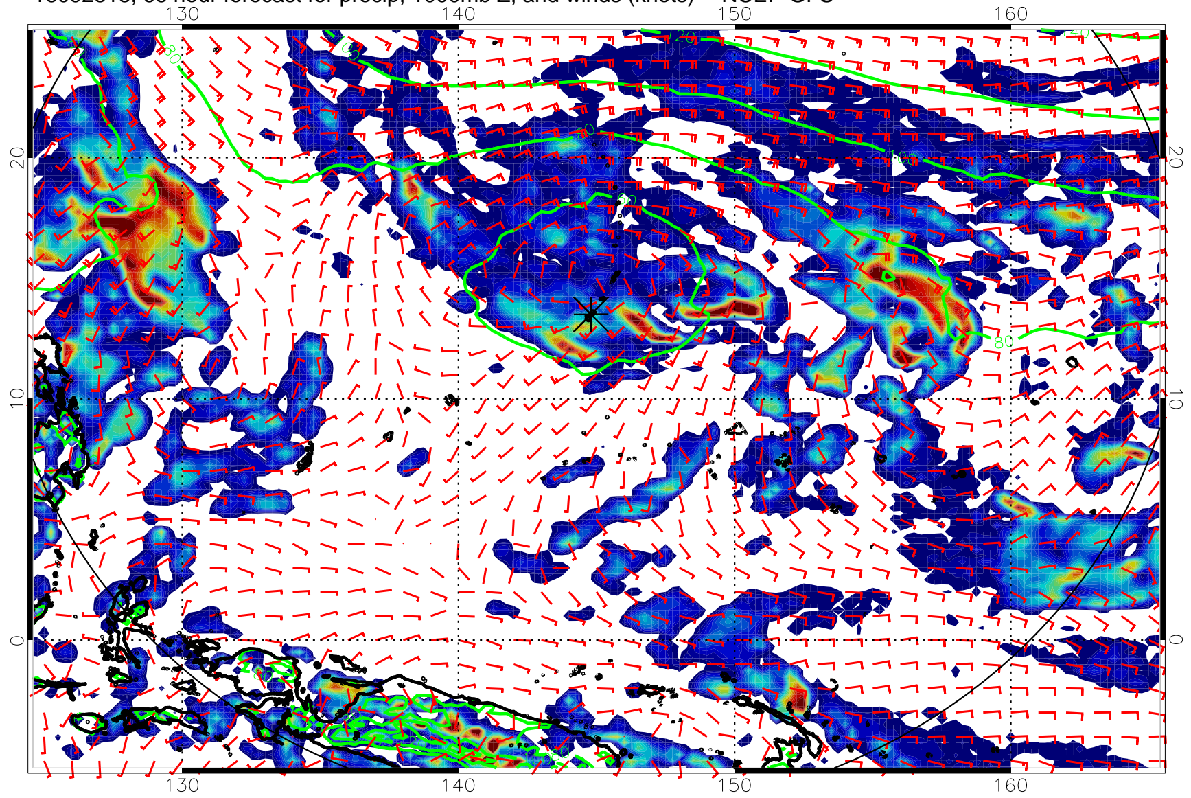
16092818, 66 hour forecast for precip, 1000mb Z, and winds (knots) -- NCEP GFS
