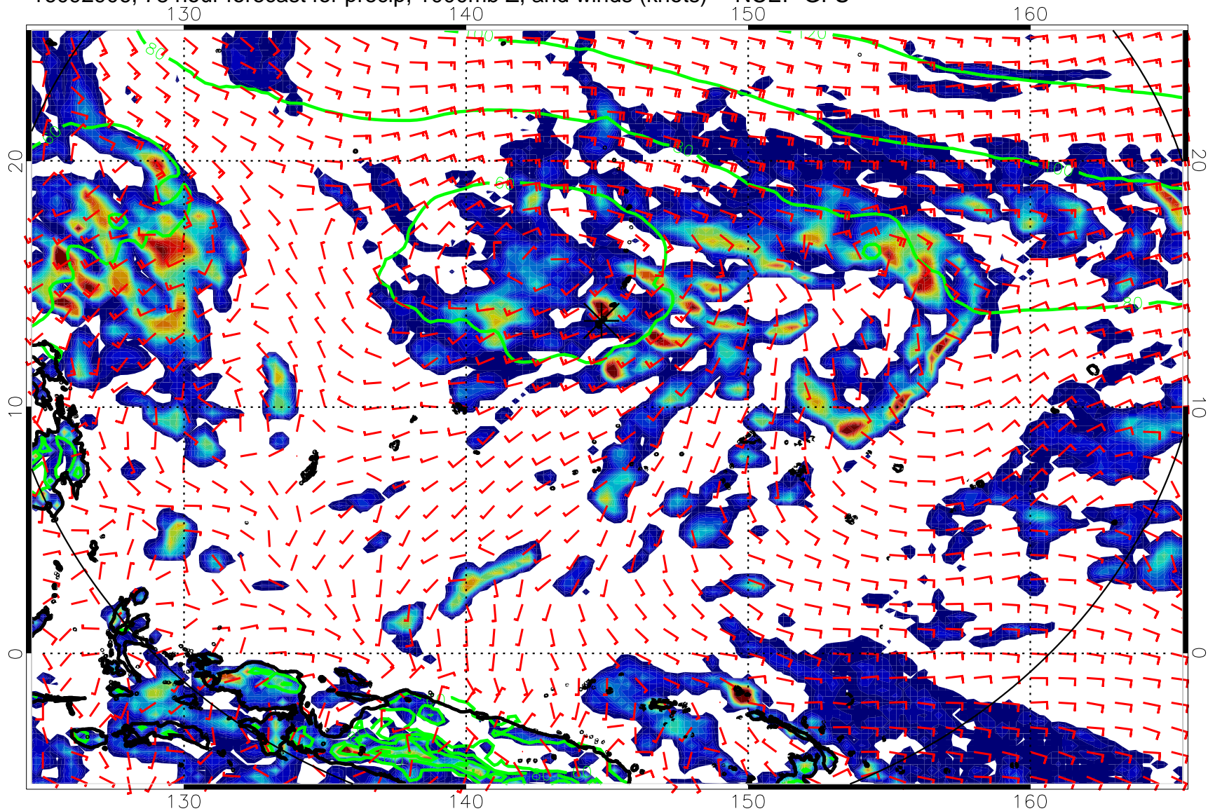
16092906, 78 hour forecast for precip, 1000mb Z, and winds (knots) -- NCEP GFS
