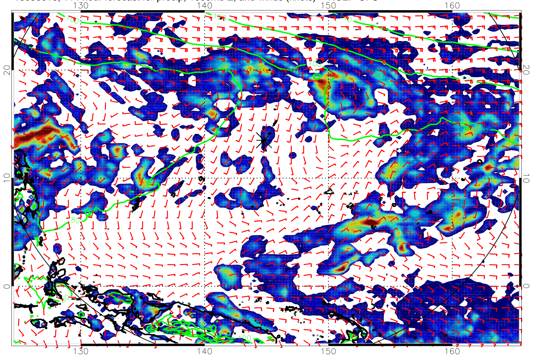
16093018, 114 hour forecast for precip, 1000mb Z, and winds (knots) -- NCEP GFS
