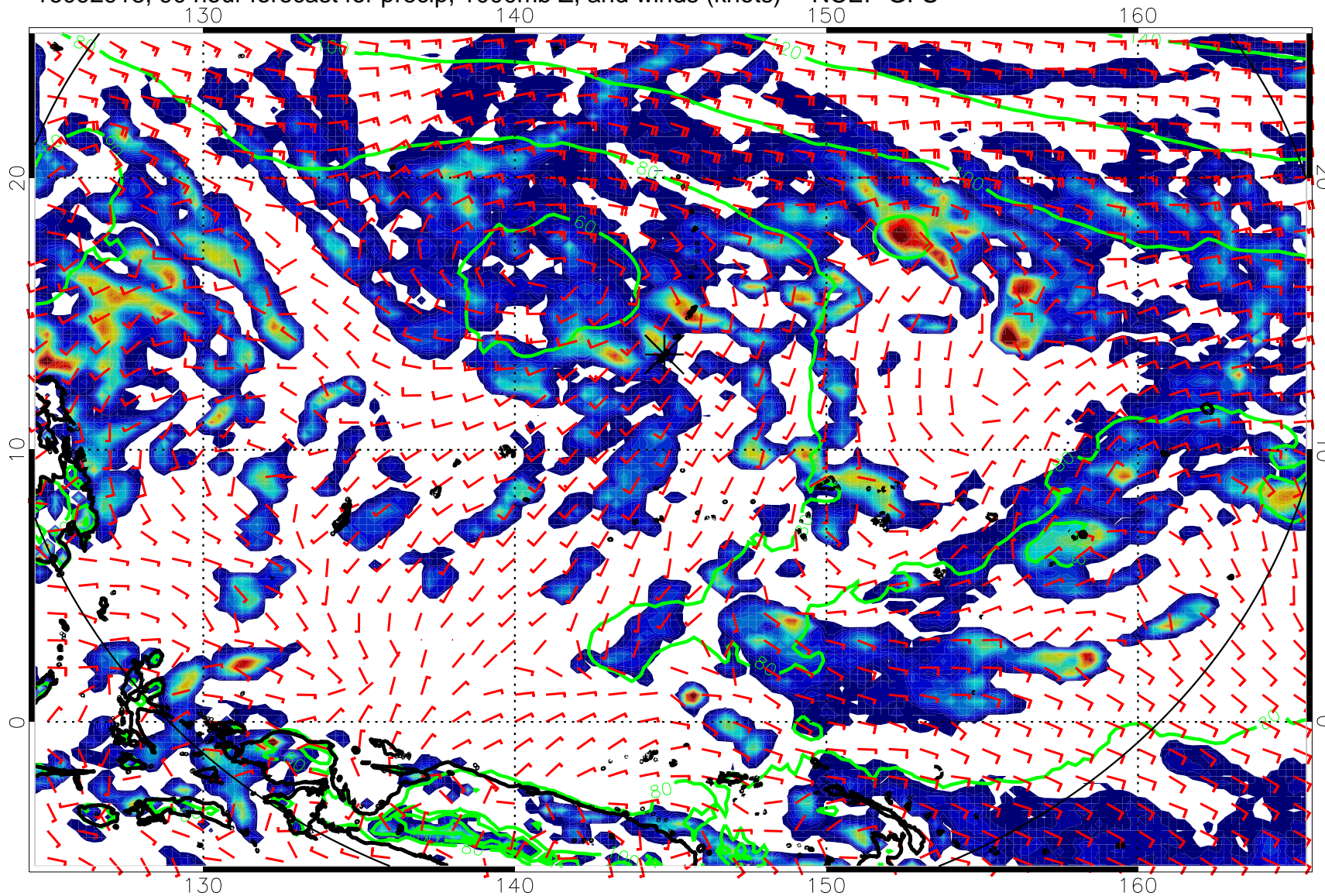
16092918, 90 hour forecast for precip, 1000mb Z, and winds (knots) -- NCEP GFS
