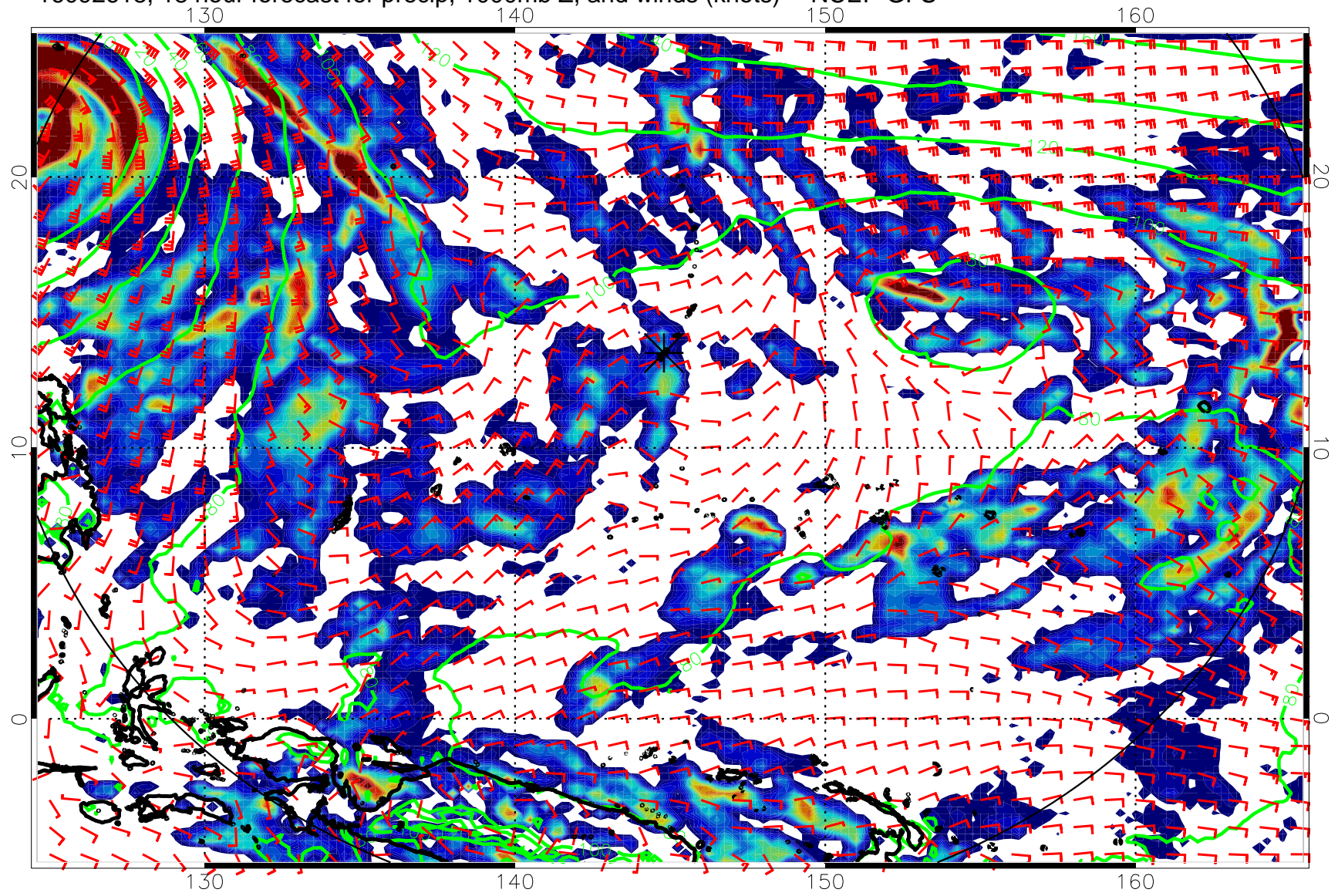
16092618, 18 hour forecast for precip, 1000mb Z, and winds (knots) -- NCEP GFS
