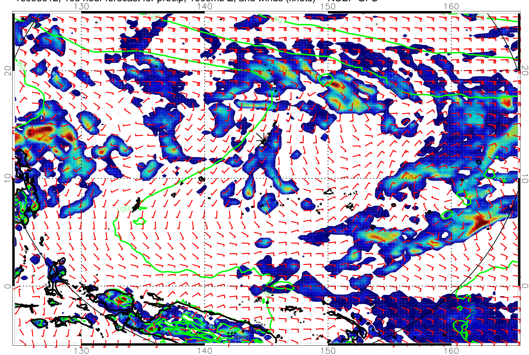
16093012, 108 hour forecast for precip, 1000mb Z, and winds (knots) -- NCEP GFS
