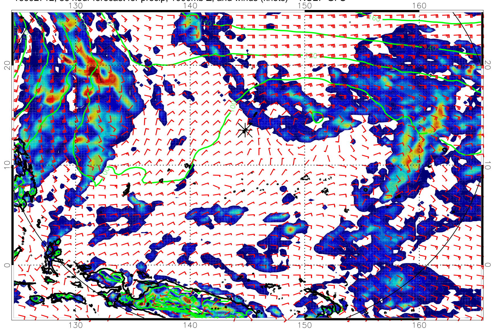
16092712, 36 hour forecast for precip, 1000mb Z, and winds (knots) -- NCEP GFS
