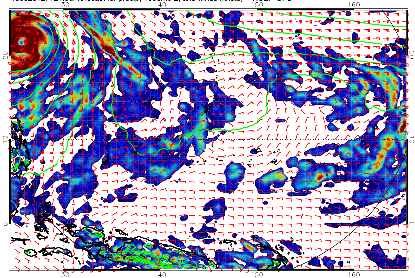
16092612, 12 hour forecast for precip, 1000mb Z, and winds (knots) -- NCEP GFS
