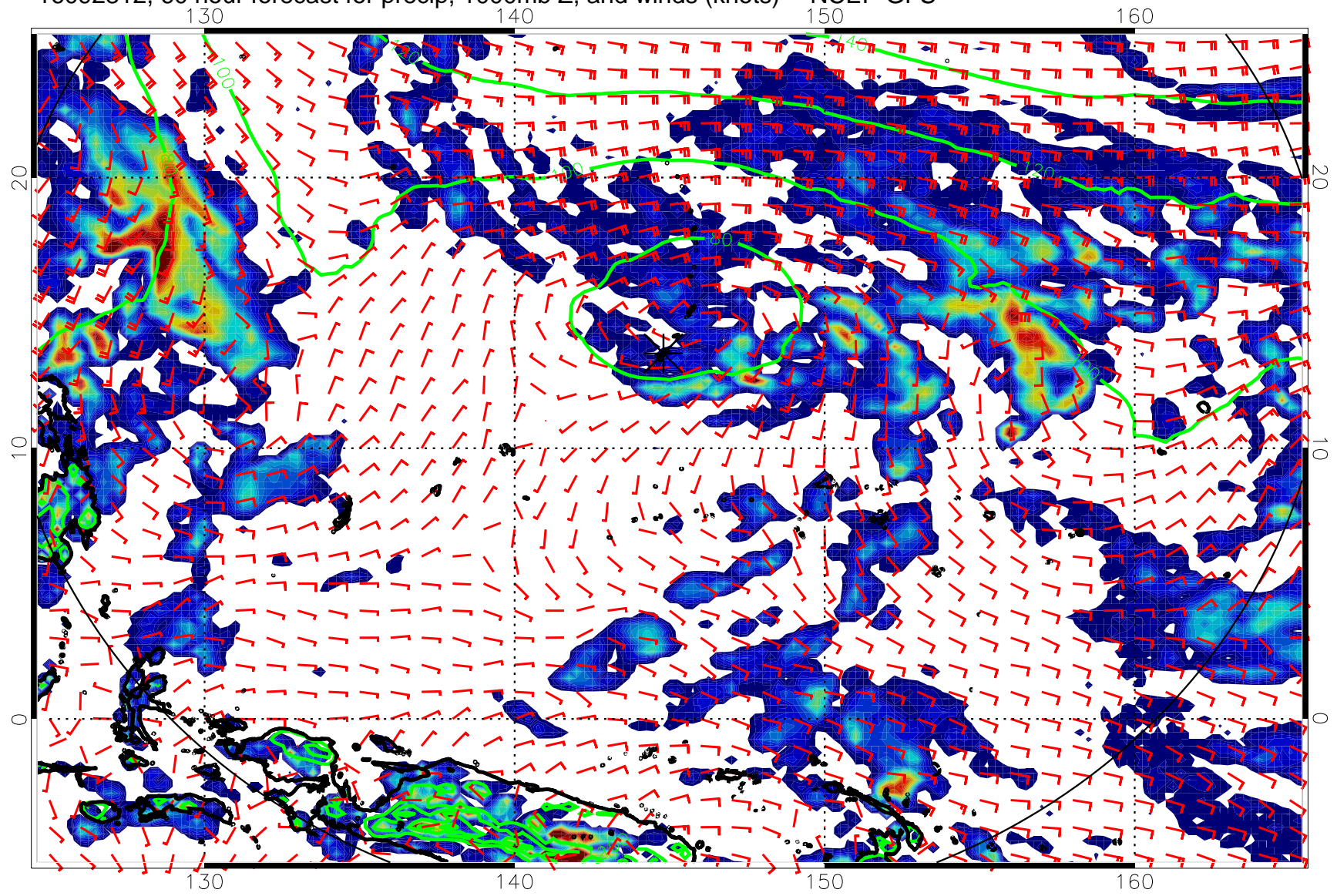
16092812, 60 hour forecast for precip, 1000mb Z, and winds (knots) -- NCEP GFS
