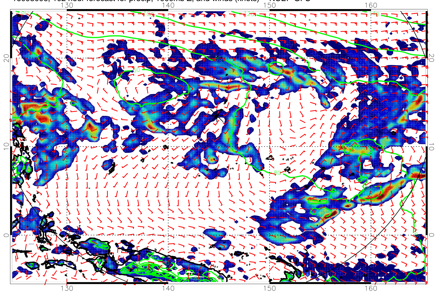
16093006, 102 hour forecast for precip, 1000mb Z, and winds (knots) -- NCEP GFS
