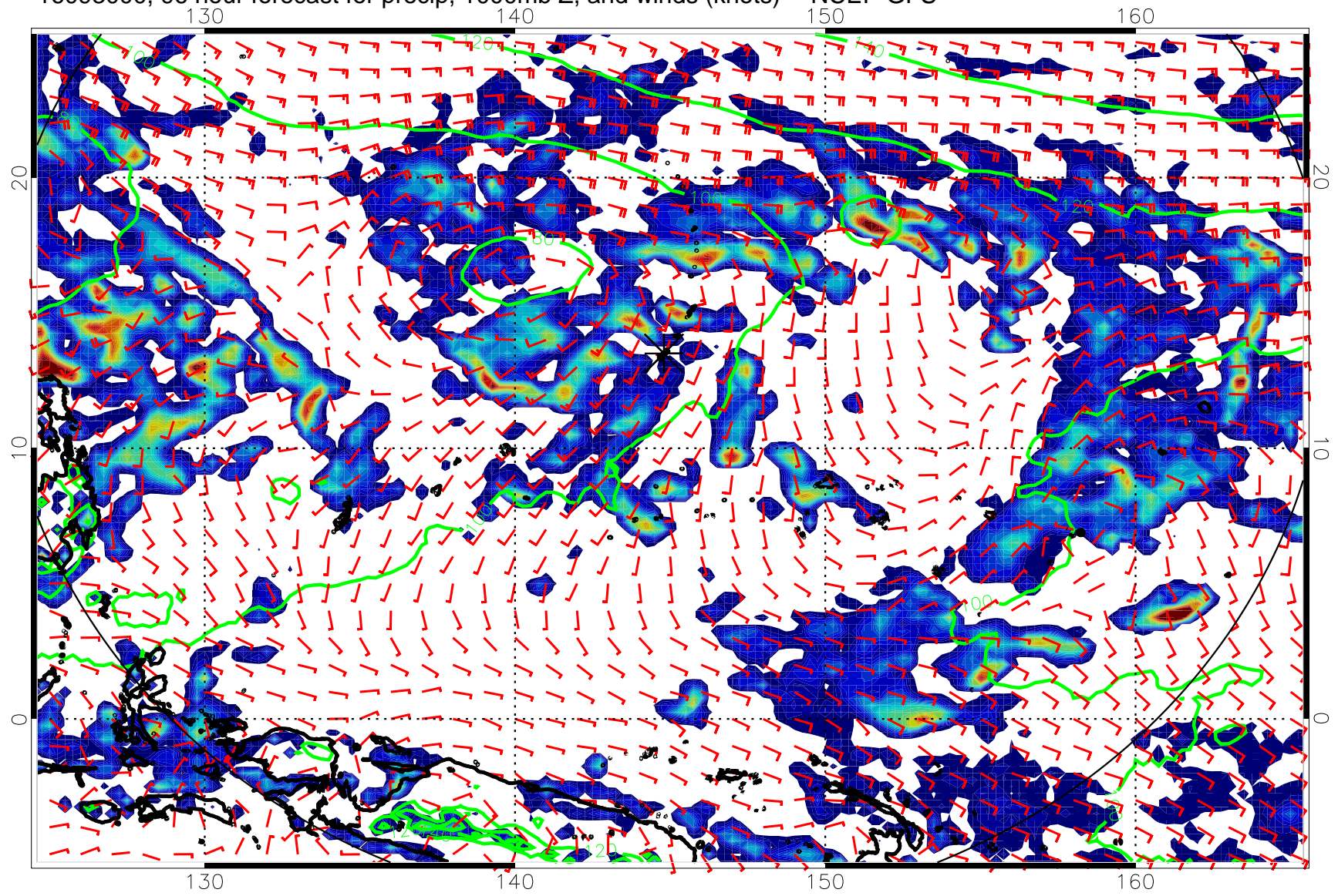
16093000, 96 hour forecast for precip, 1000mb Z, and winds (knots) -- NCEP GFS
