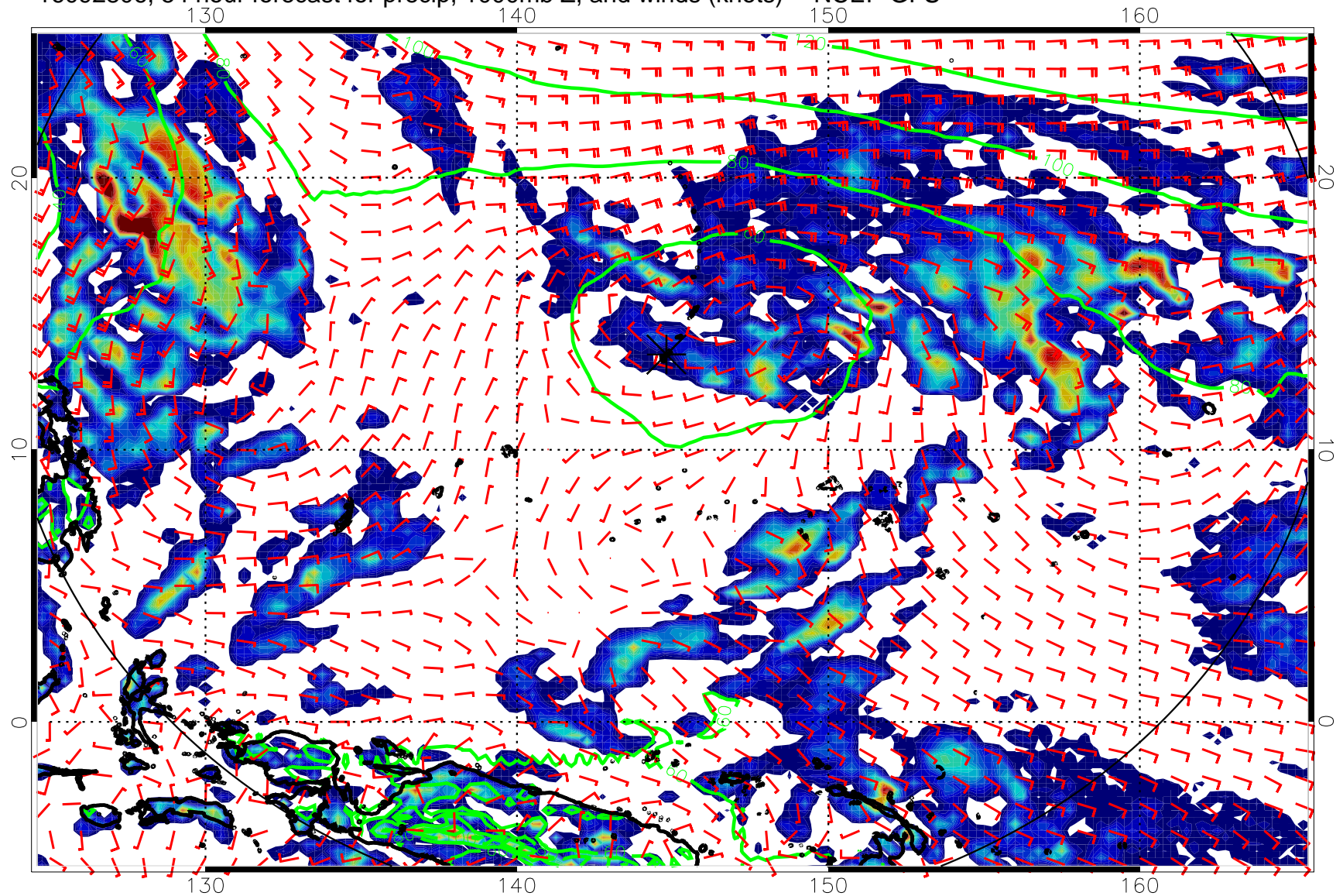
16092806, 54 hour forecast for precip, 1000mb Z, and winds (knots) -- NCEP GFS
