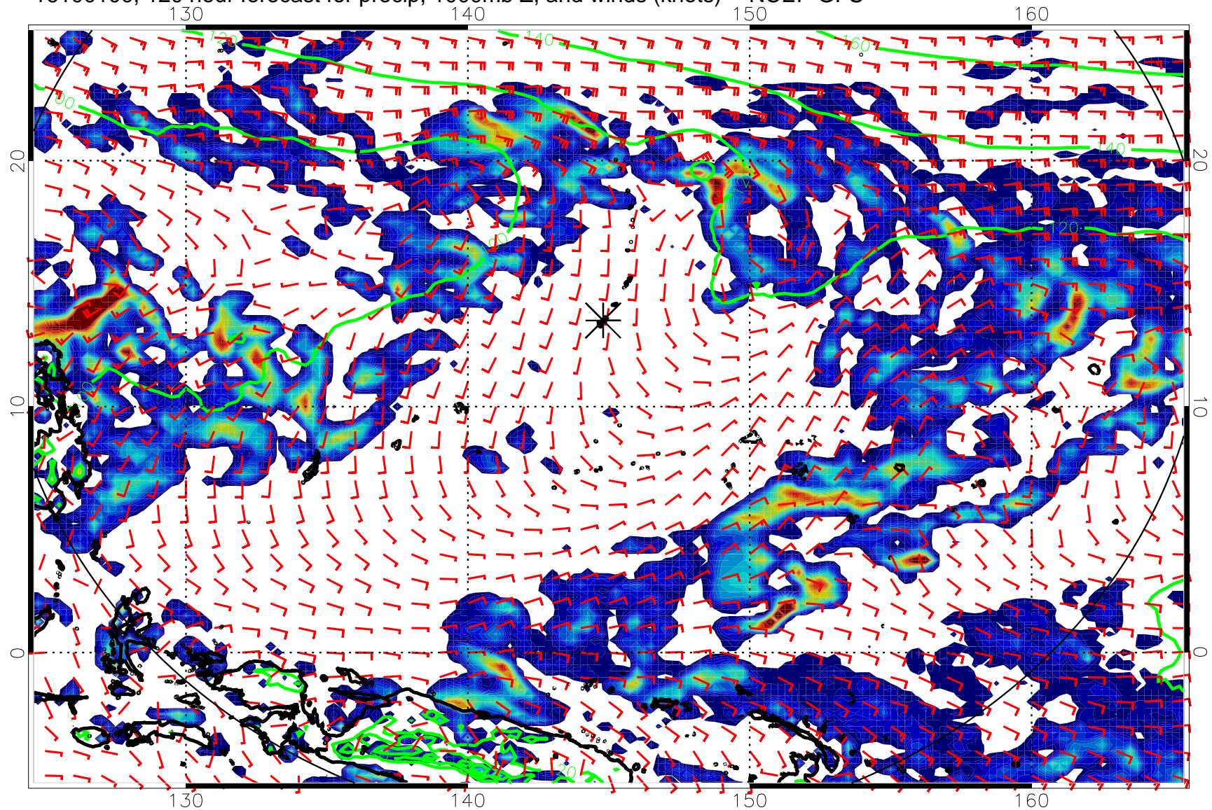
16100100, 120 hour forecast for precip, 1000mb Z, and winds (knots) -- NCEP GFS
