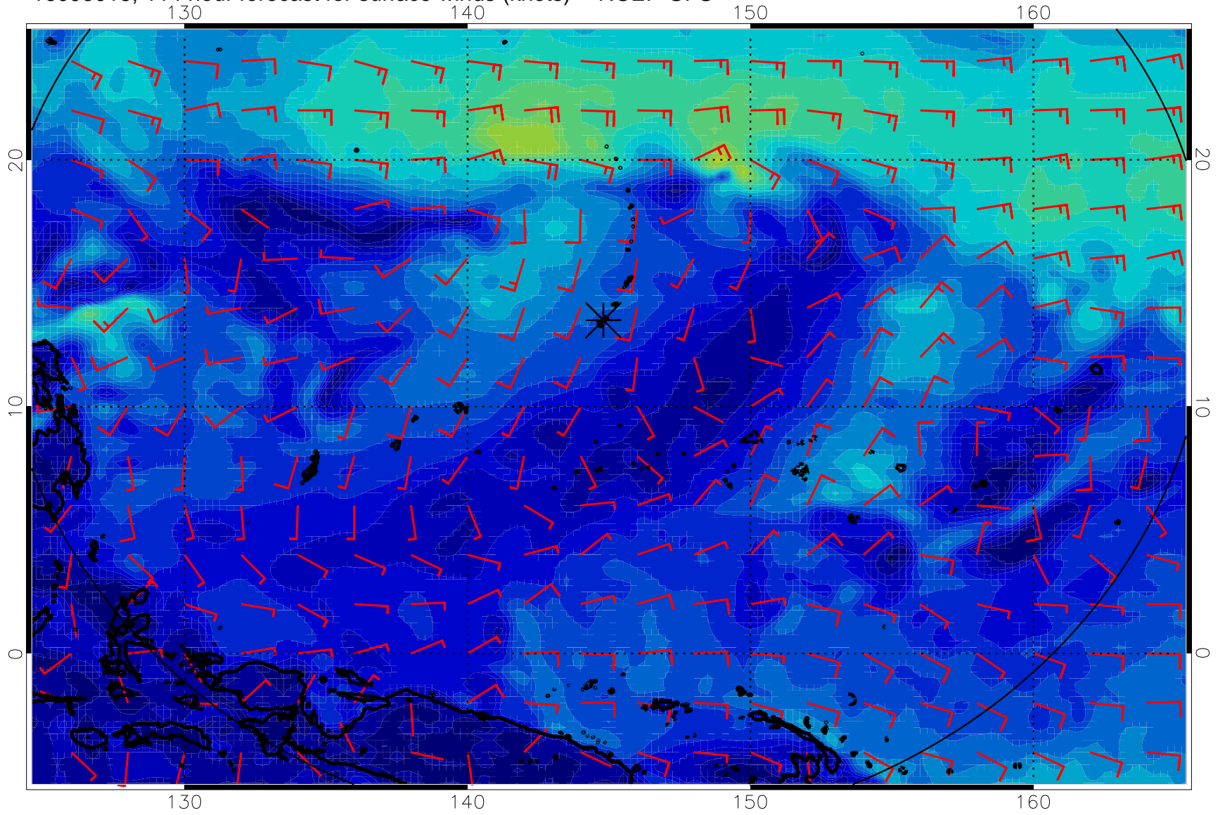
16093018, 114 hour forecast for surface winds (knots) -- NCEP GFS
