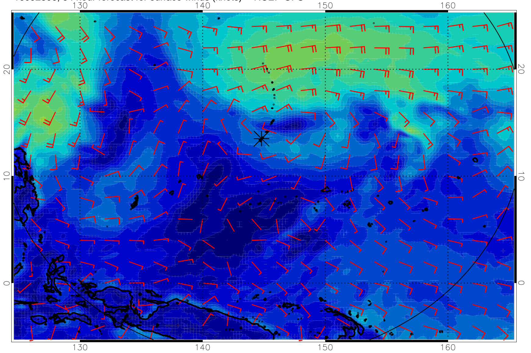
16092806, 54 hour forecast for surface winds (knots) -- NCEP GFS
