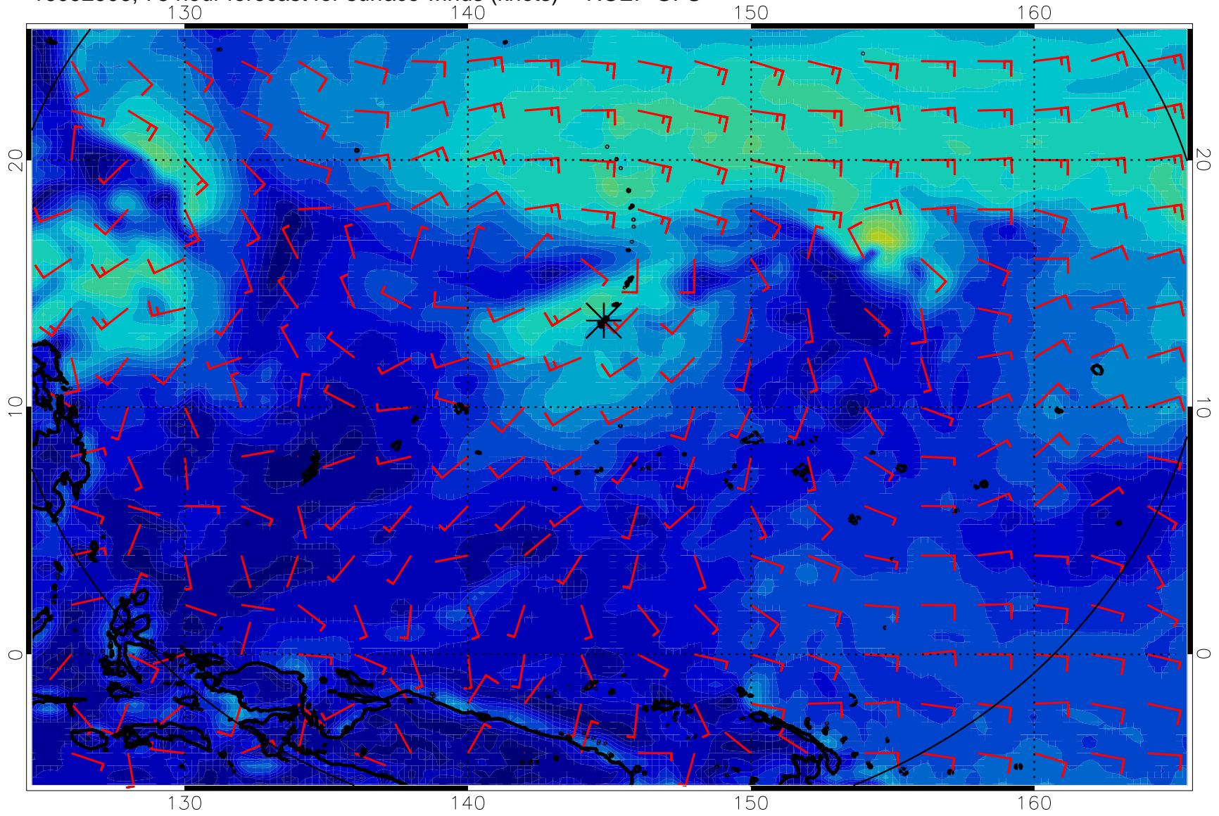
16092906, 78 hour forecast for surface winds (knots) -- NCEP GFS
