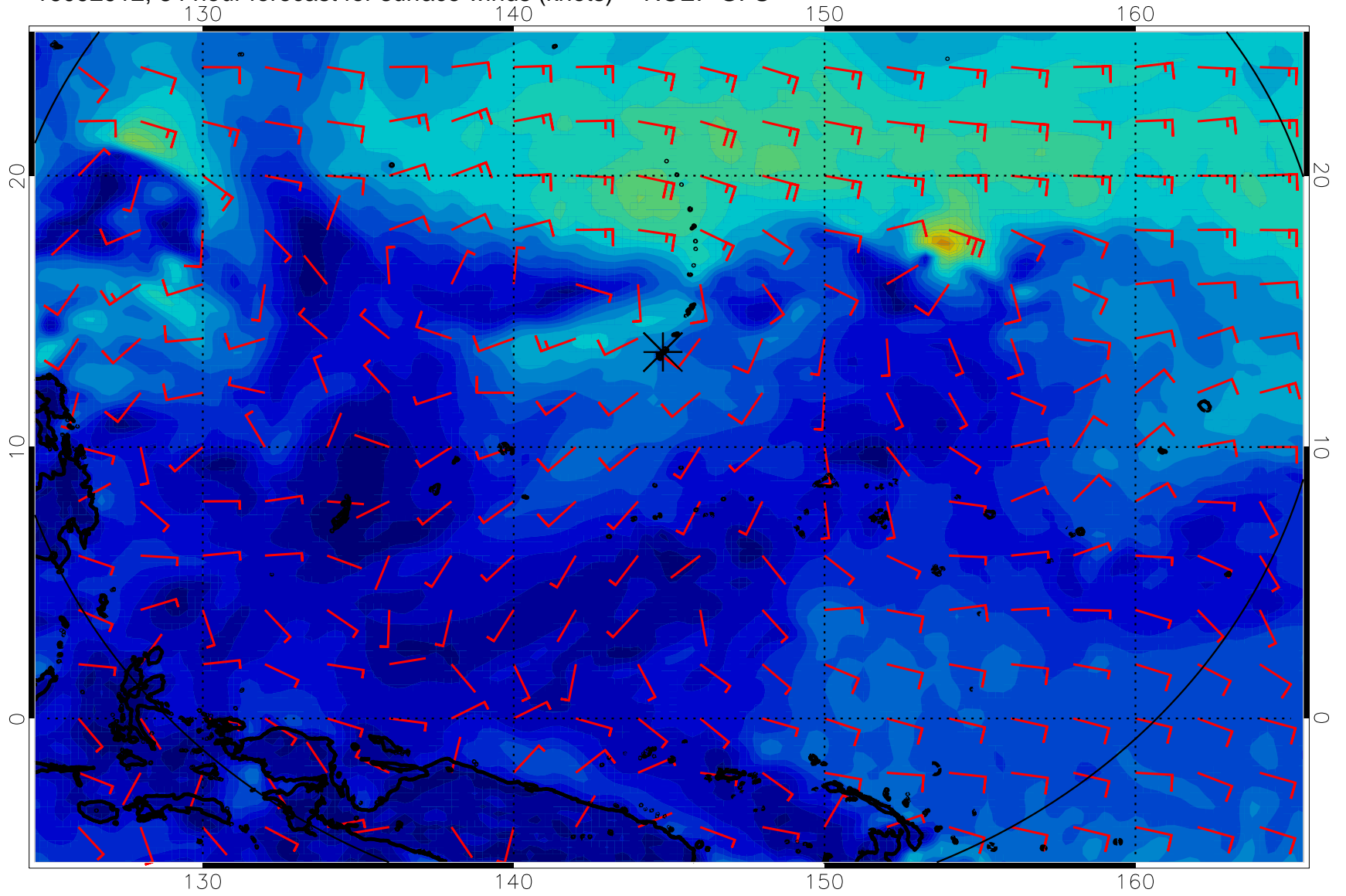
16092912, 84 hour forecast for surface winds (knots) -- NCEP GFS
