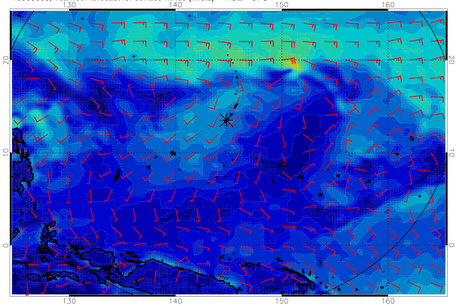
16093006, 102 hour forecast for surface winds (knots) -- NCEP GFS
