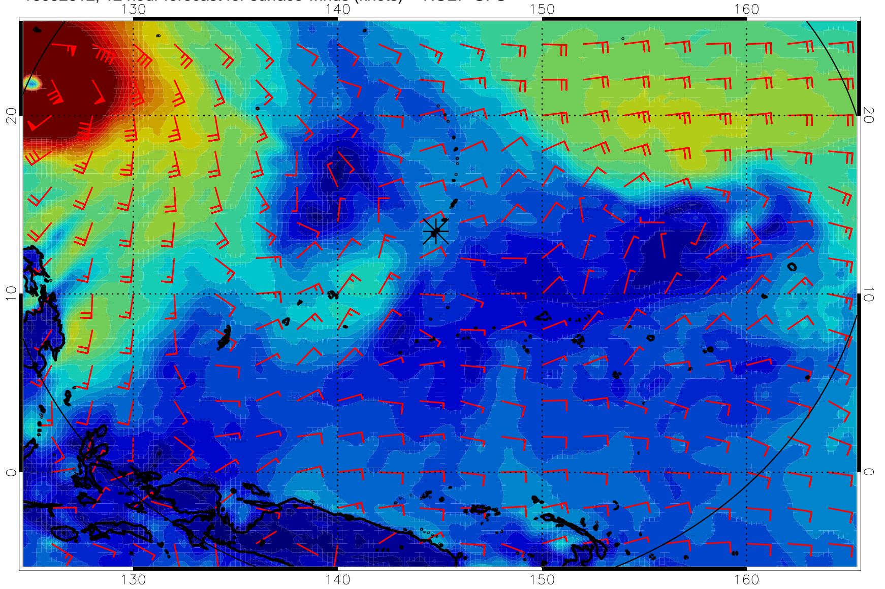
16092612, 12 hour forecast for surface winds (knots) -- NCEP GFS
