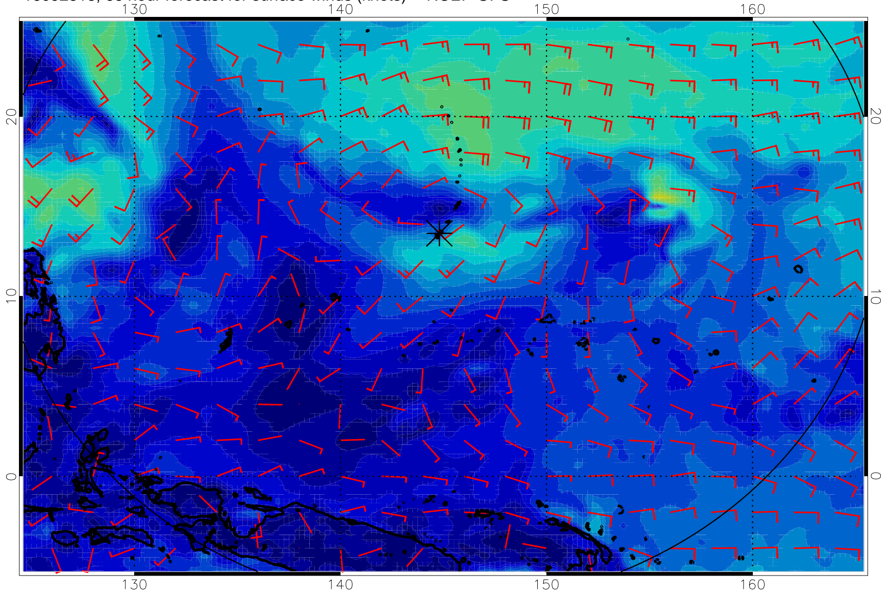
16092818, 66 hour forecast for surface winds (knots) -- NCEP GFS
