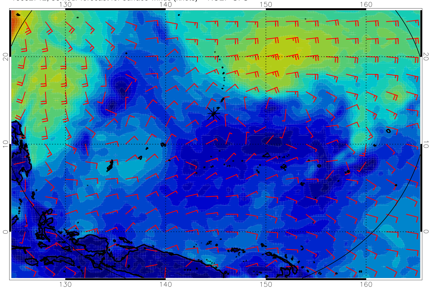
16092712, 36 hour forecast for surface winds (knots) -- NCEP GFS
