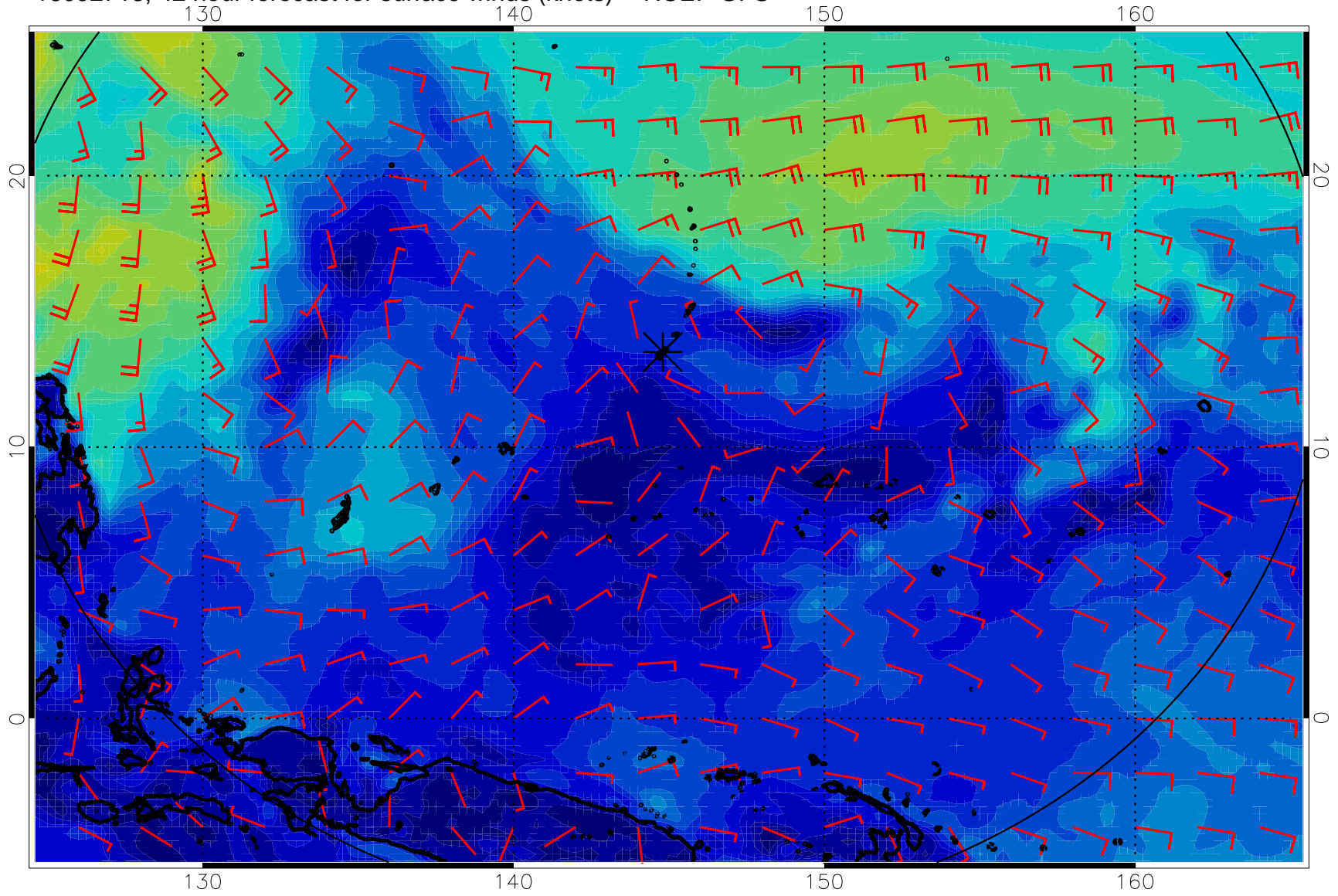
16092718, 42 hour forecast for surface winds (knots) -- NCEP GFS
