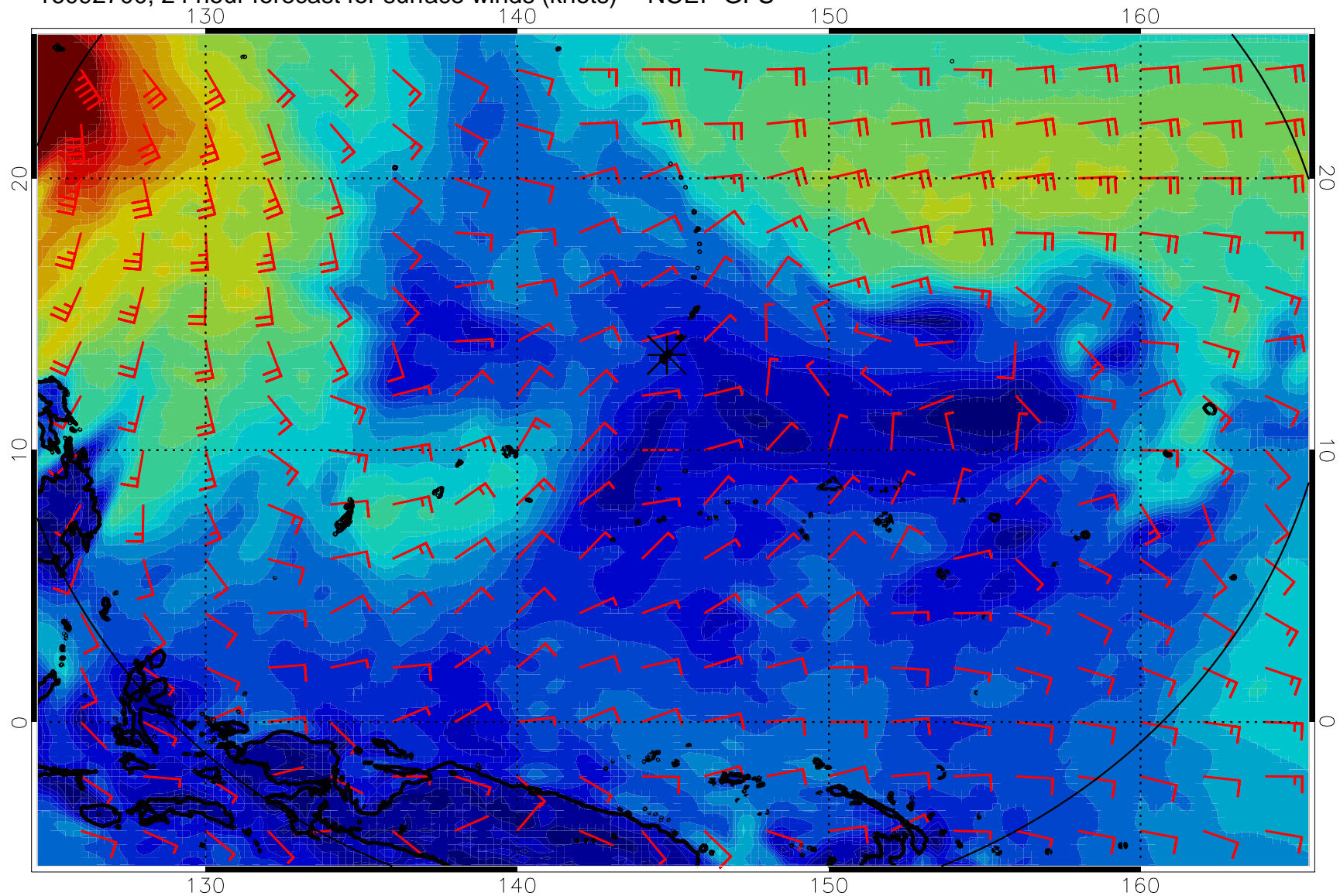
16092700, 24 hour forecast for surface winds (knots) -- NCEP GFS
