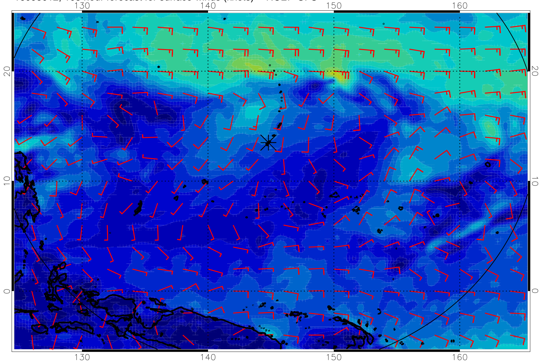
16093012, 108 hour forecast for surface winds (knots) -- NCEP GFS
