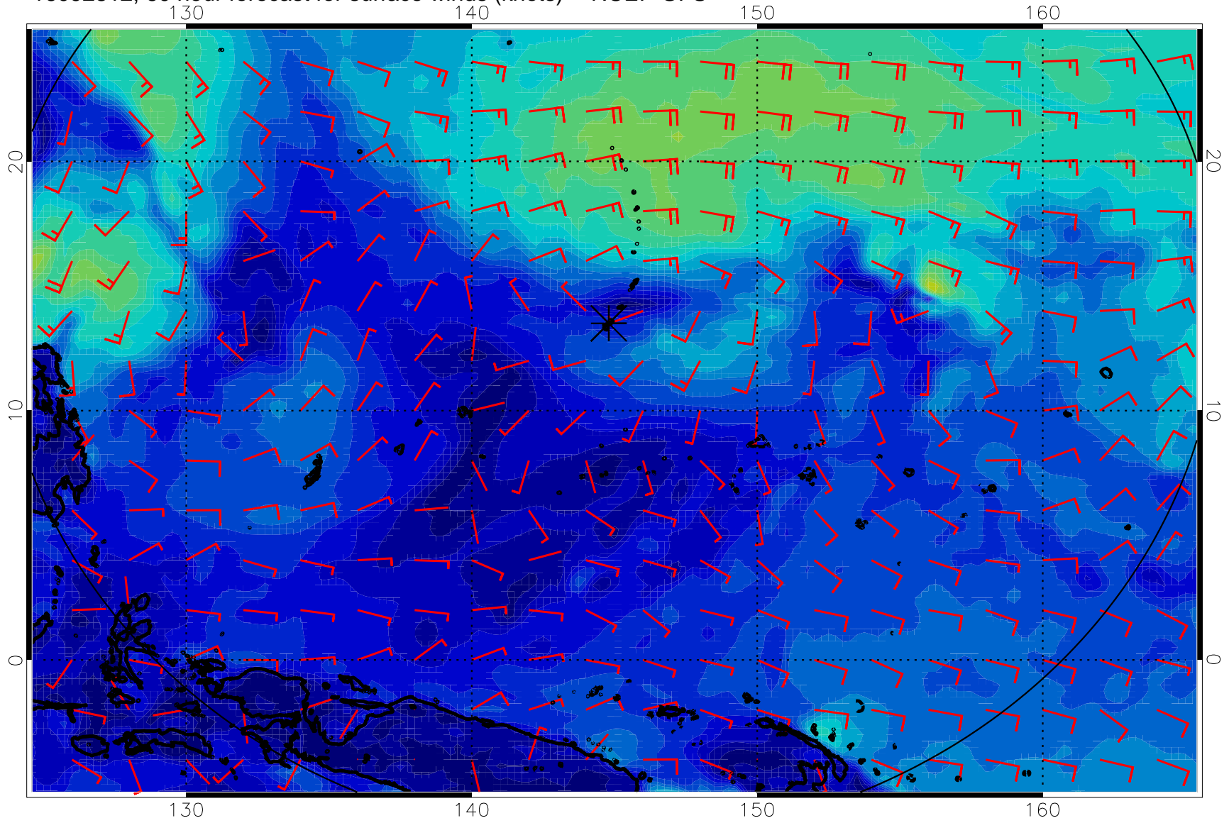
16092812, 60 hour forecast for surface winds (knots) -- NCEP GFS
