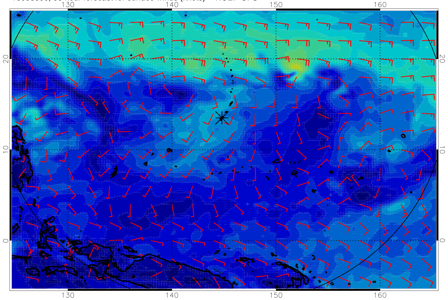
16093000, 96 hour forecast for surface winds (knots) -- NCEP GFS
