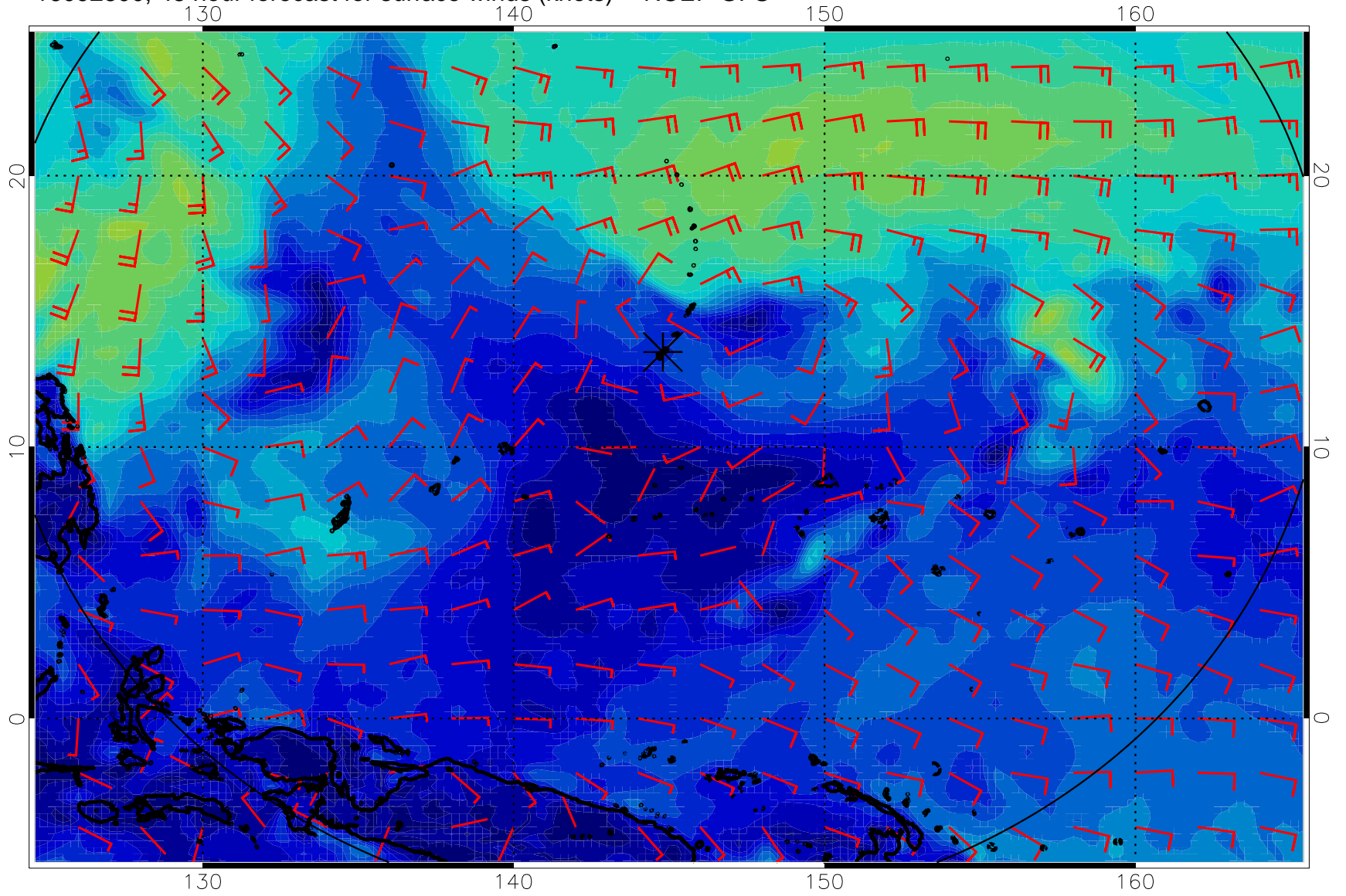
16092800, 48 hour forecast for surface winds (knots) -- NCEP GFS
