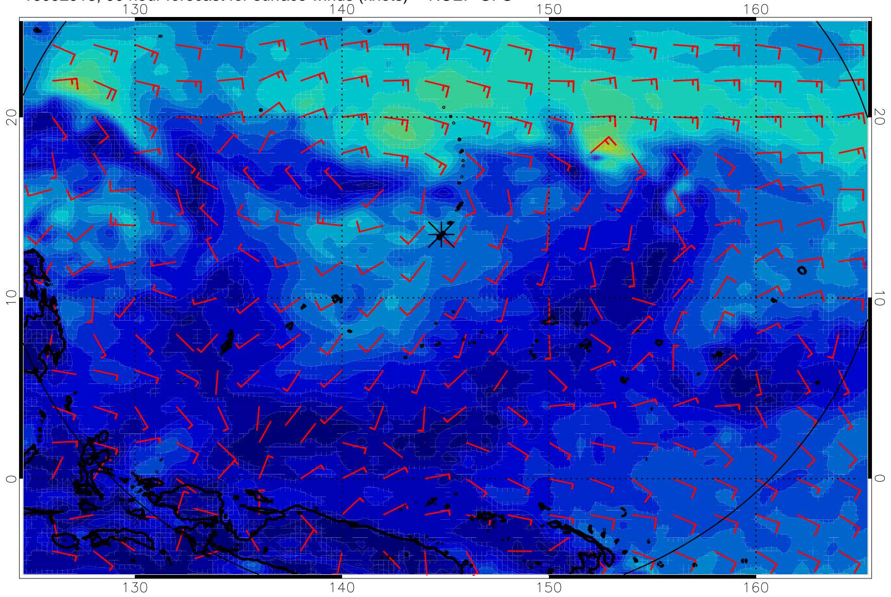
16092918, 90 hour forecast for surface winds (knots) -- NCEP GFS
