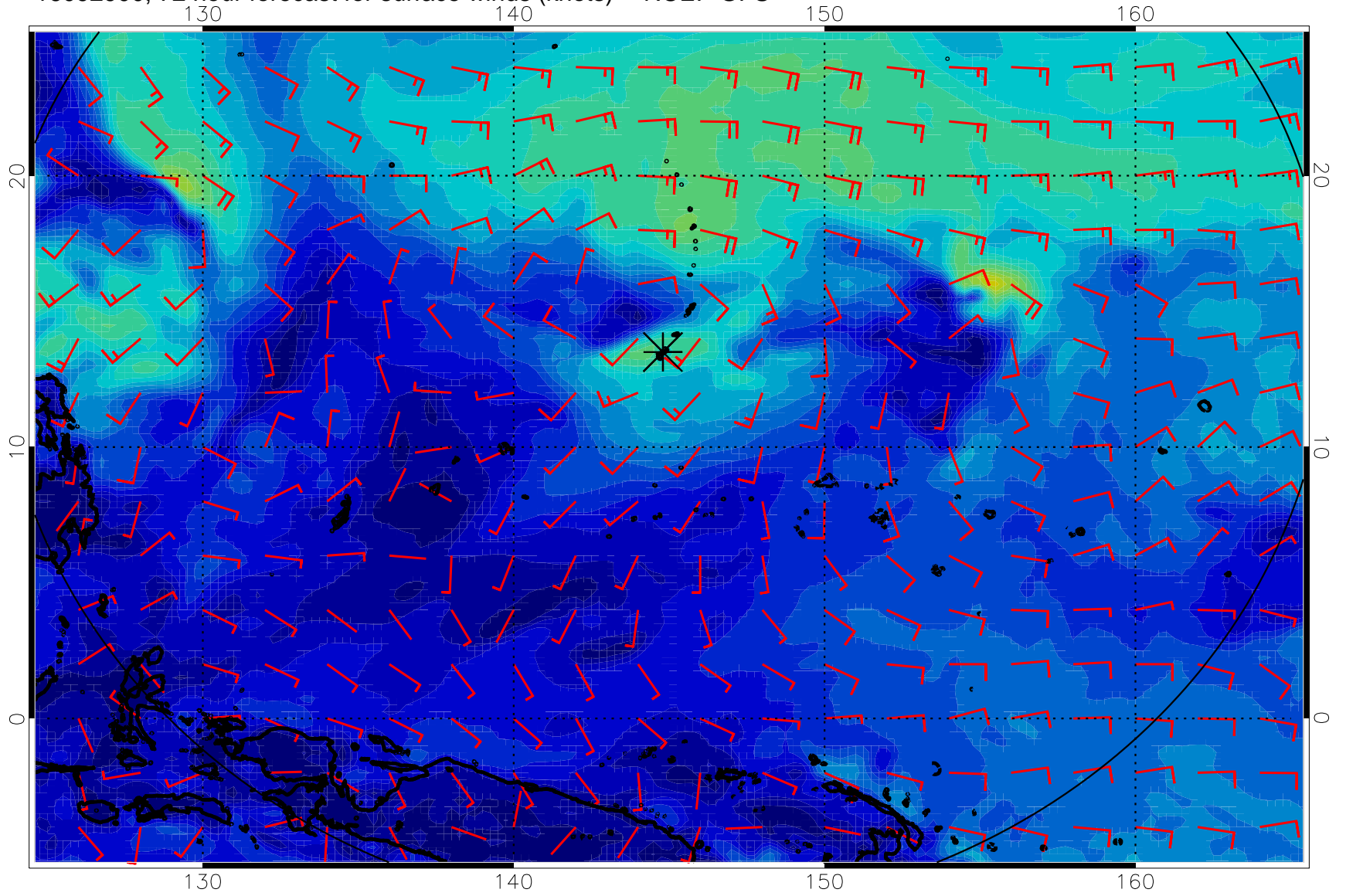
16092900, 72 hour forecast for surface winds (knots) -- NCEP GFS
