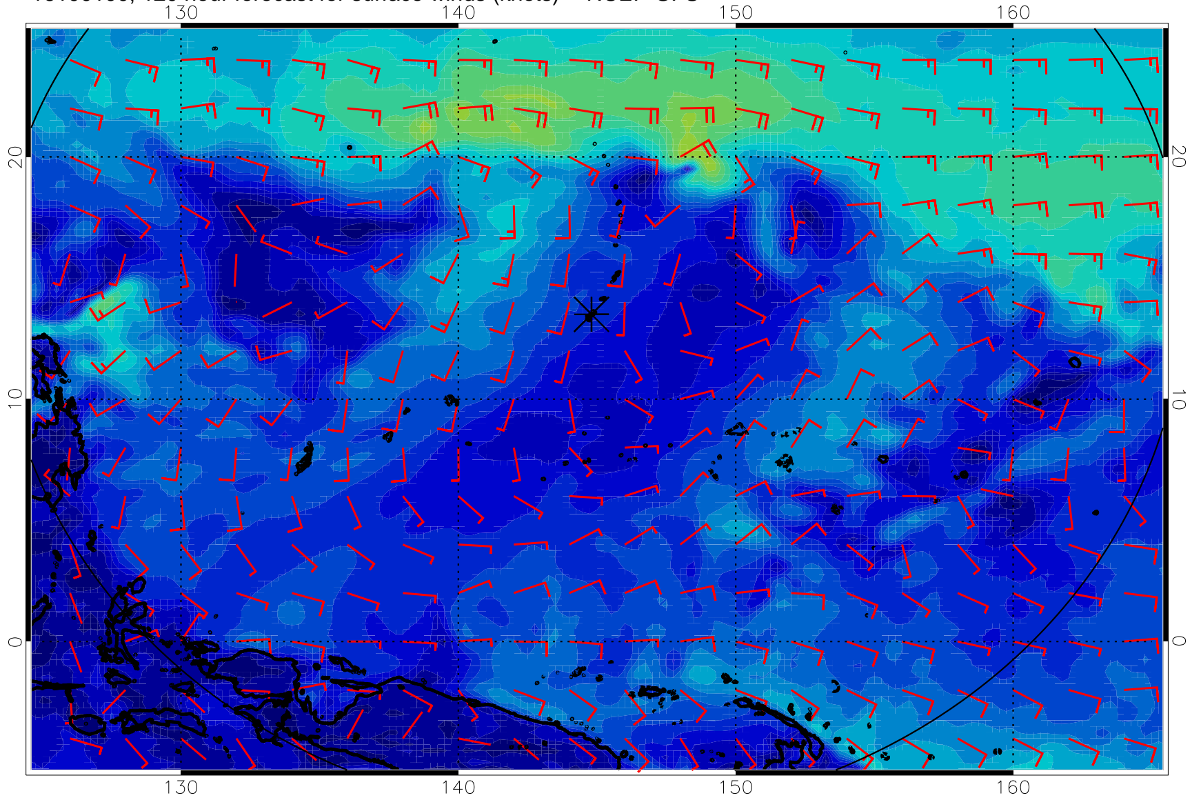
16100100, 120 hour forecast for surface winds (knots) -- NCEP GFS
