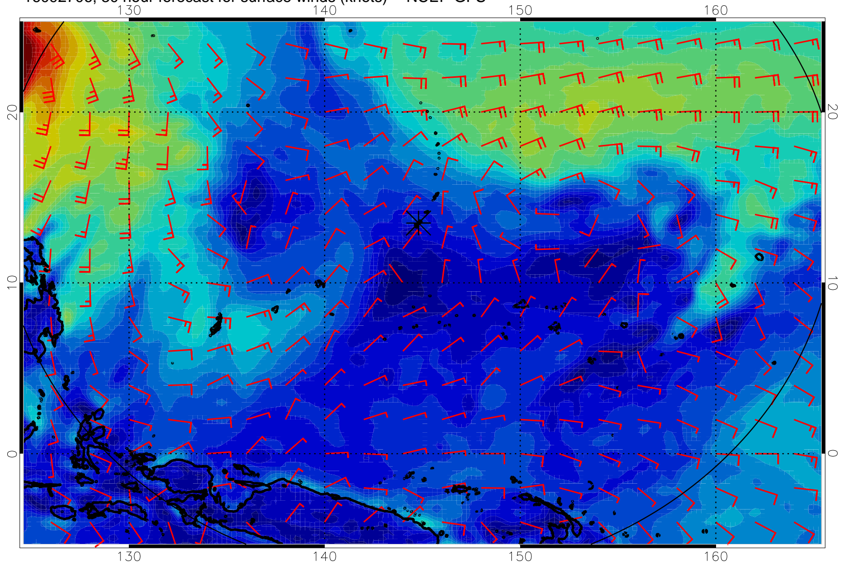
16092706, 30 hour forecast for surface winds (knots) -- NCEP GFS
