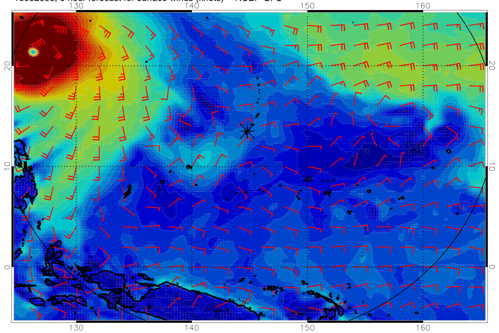
16092606, 6 hour forecast for surface winds (knots) -- NCEP GFS
