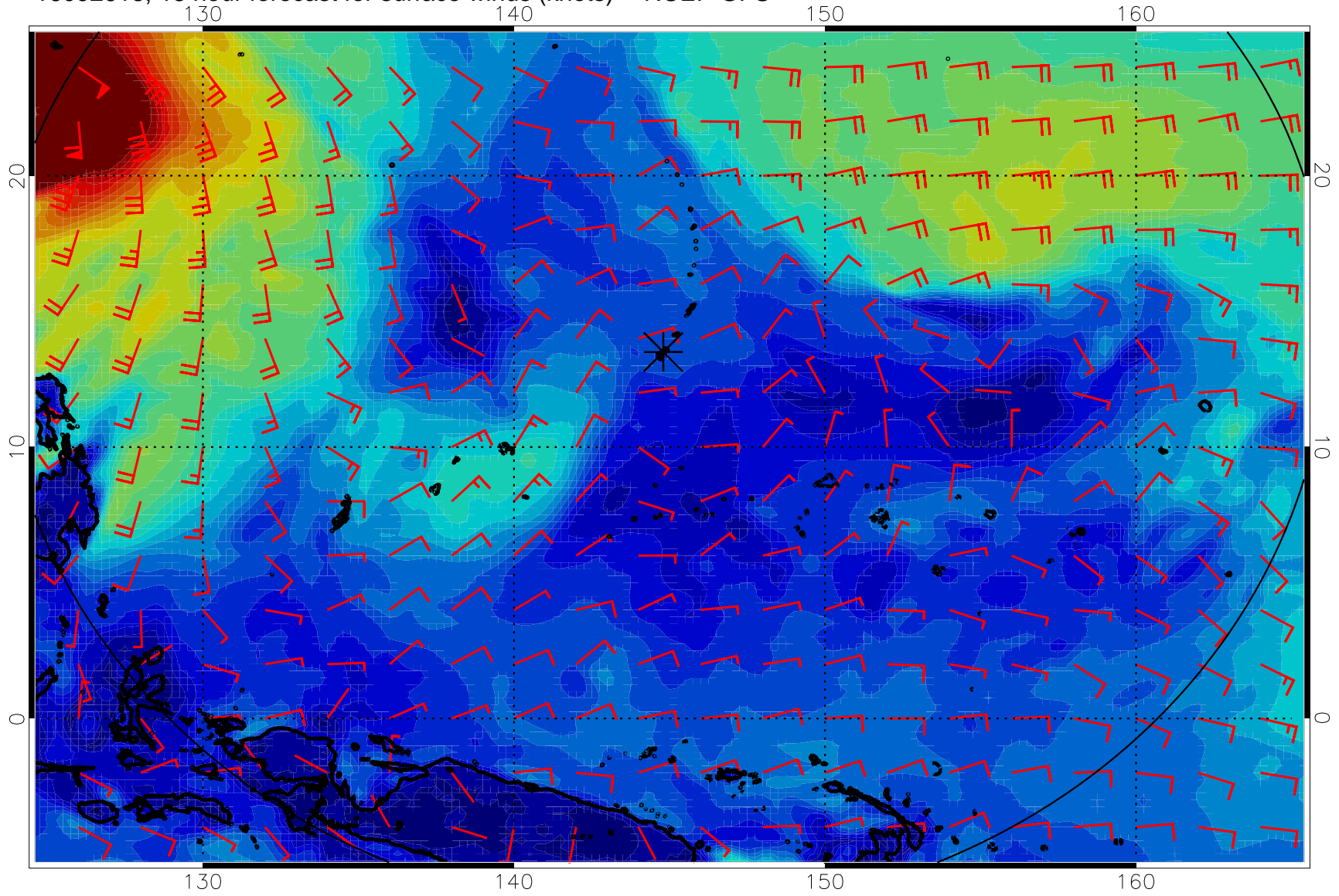
16092618, 18 hour forecast for surface winds (knots) -- NCEP GFS
