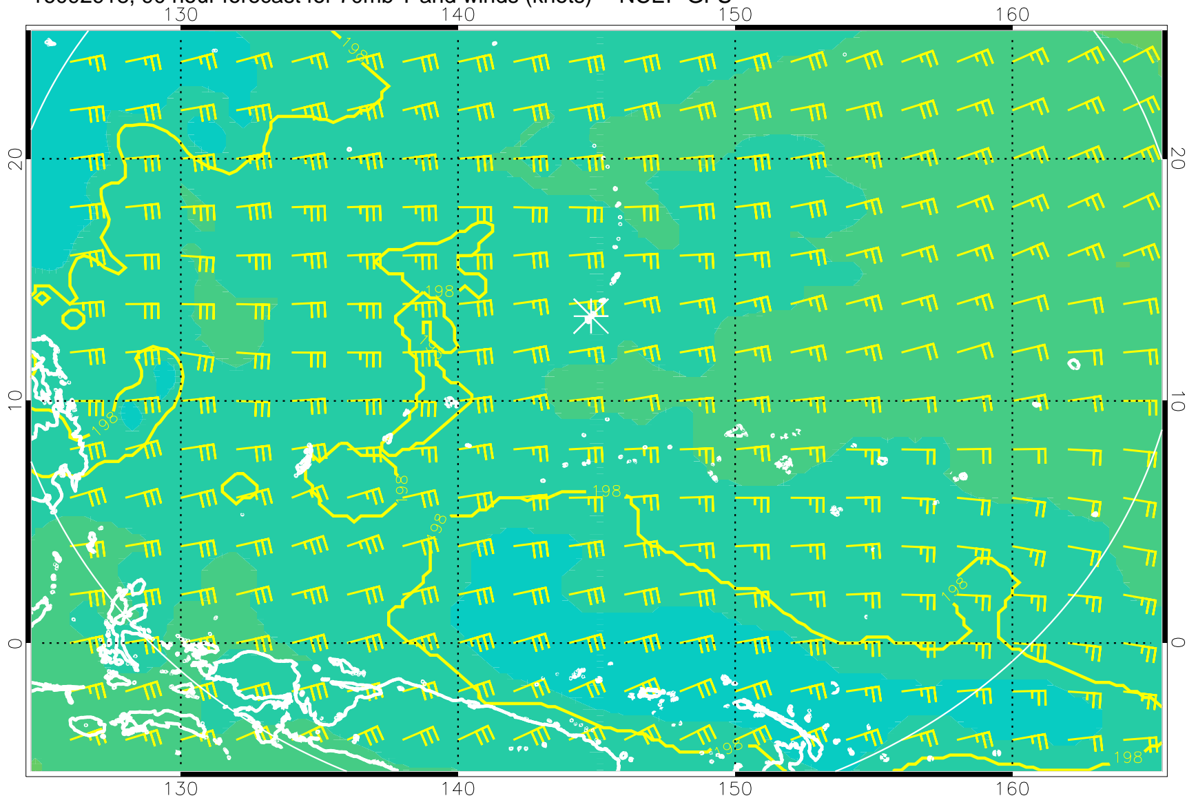
16092918, 90 hour forecast for 70mb T and winds (knots) -- NCEP GFS
