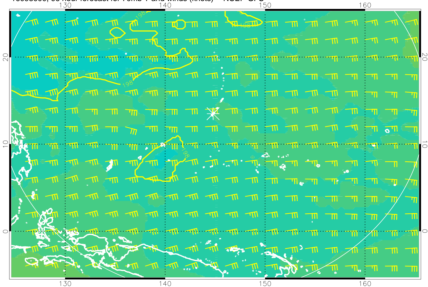
16093000, 96 hour forecast for 70mb T and winds (knots) -- NCEP GFS
