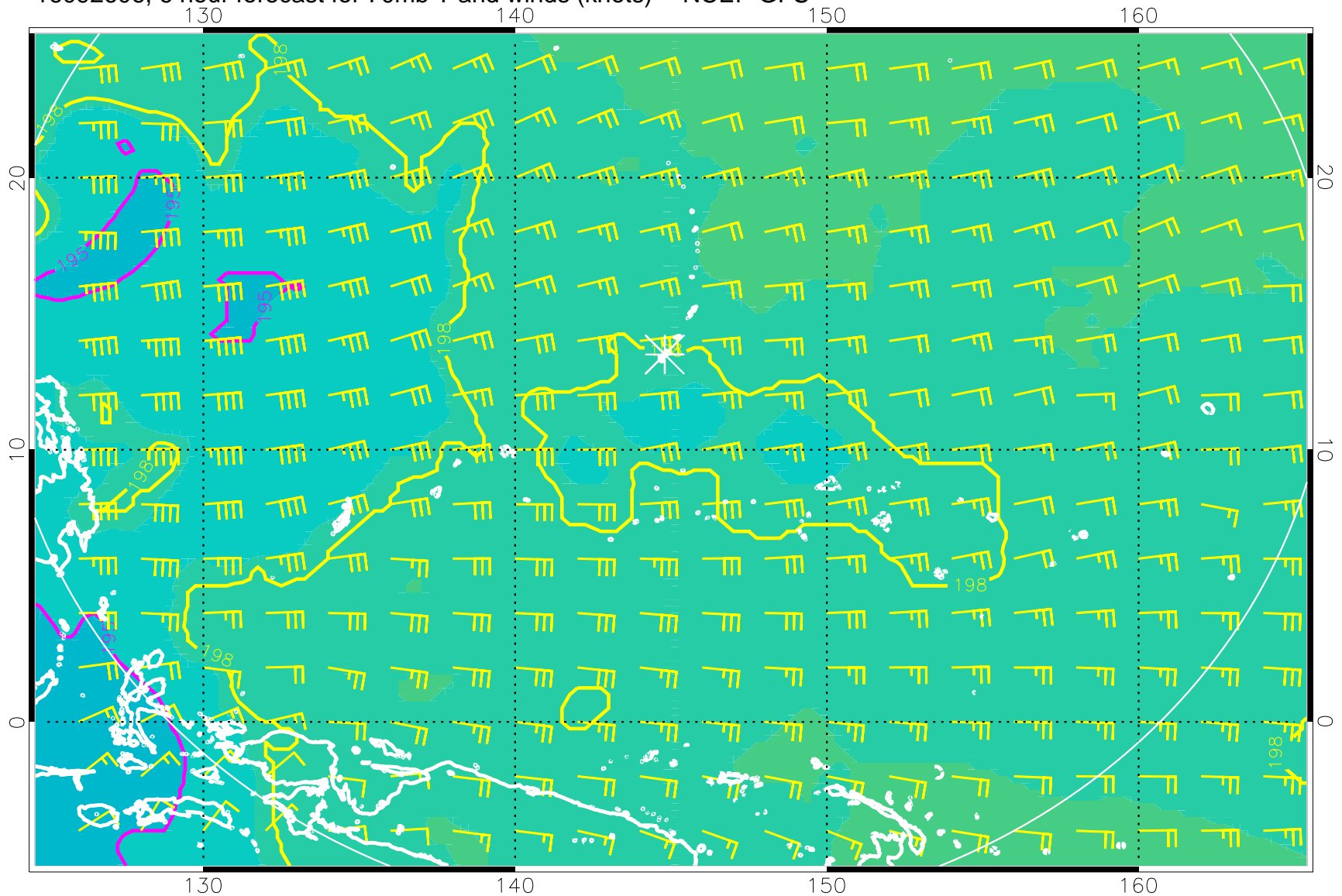
16092606, 6 hour forecast for 70mb T and winds (knots) -- NCEP GFS
