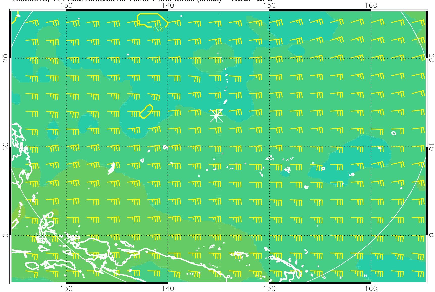
16093018, 114 hour forecast for 70mb T and winds (knots) -- NCEP GFS
