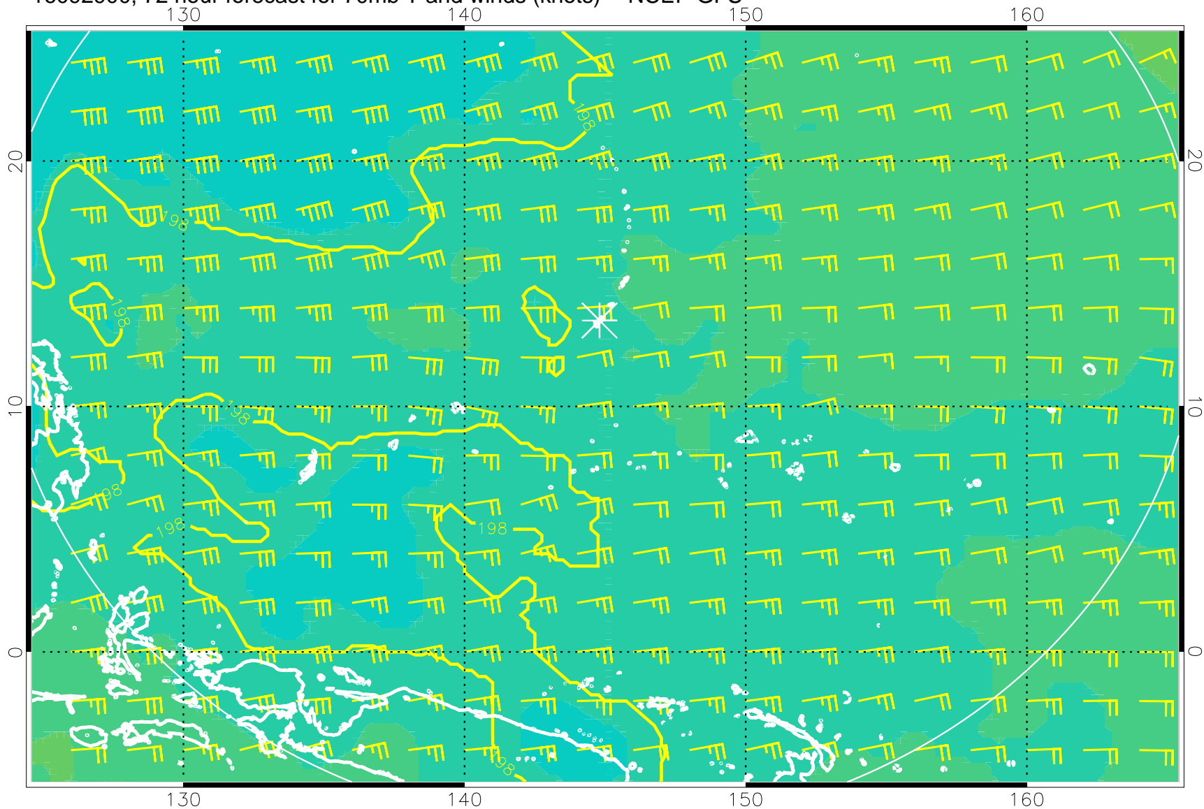
16092900, 72 hour forecast for 70mb T and winds (knots) -- NCEP GFS
