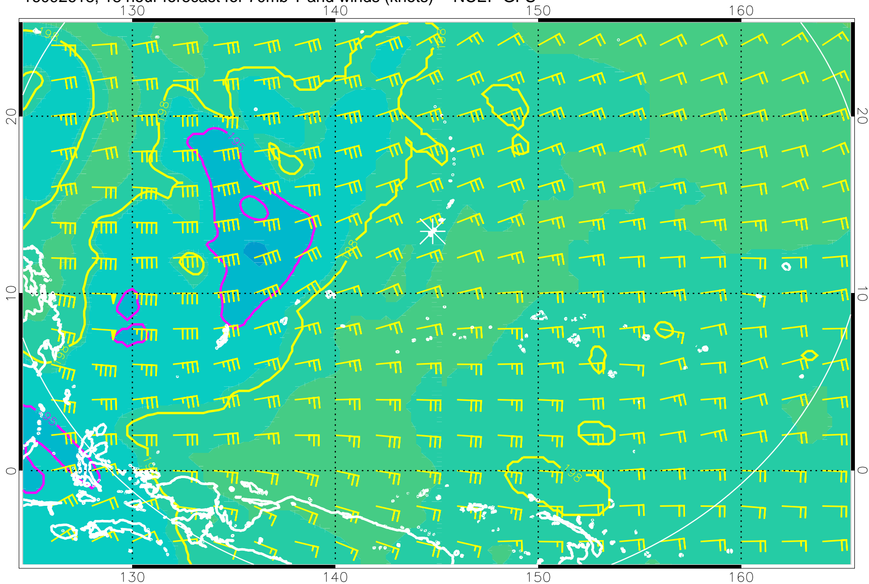
16092618, 18 hour forecast for 70mb T and winds (knots) -- NCEP GFS
