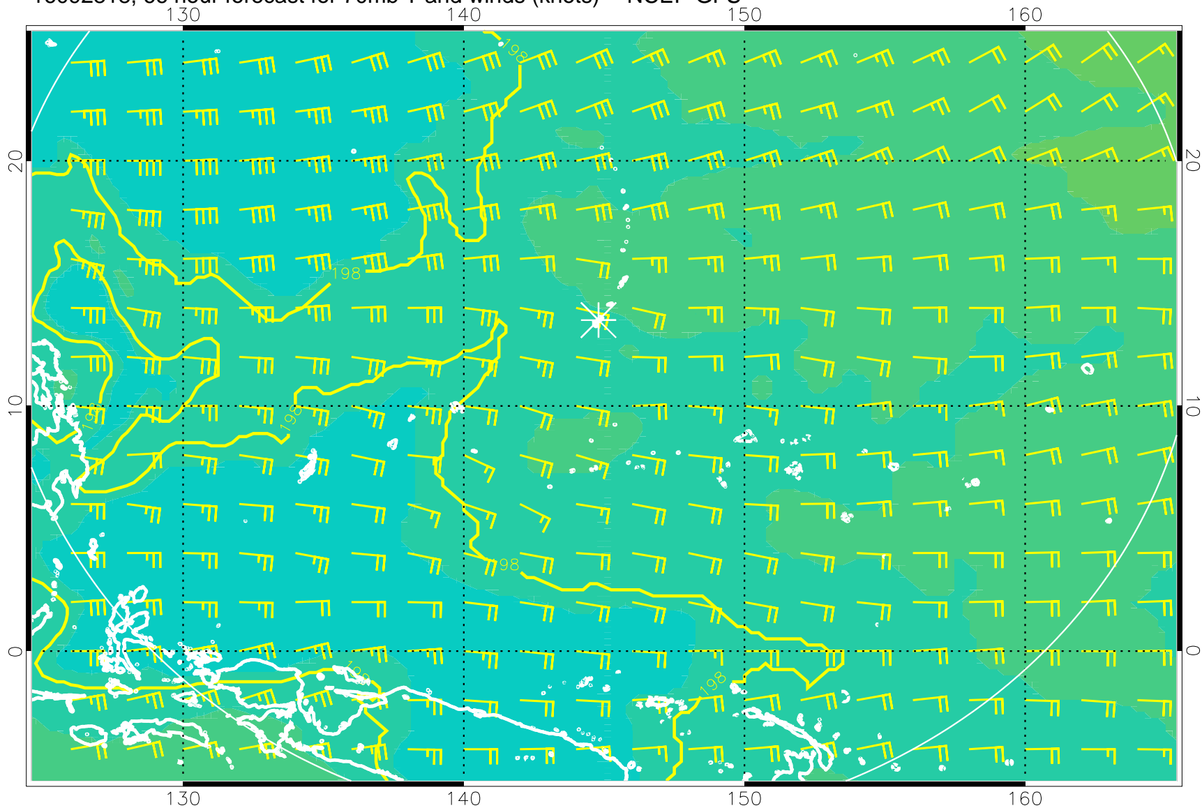
16092818, 66 hour forecast for 70mb T and winds (knots) -- NCEP GFS
