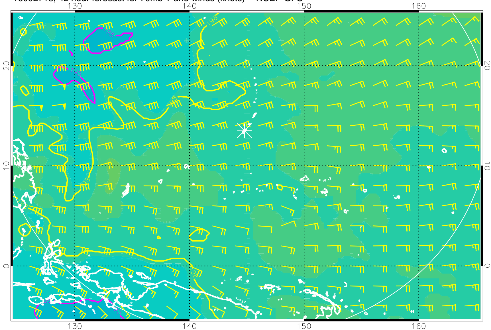
16092718, 42 hour forecast for 70mb T and winds (knots) -- NCEP GFS
