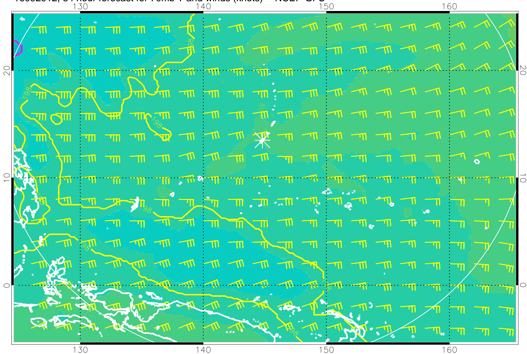
16092912, 84 hour forecast for 70mb T and winds (knots) -- NCEP GFS
