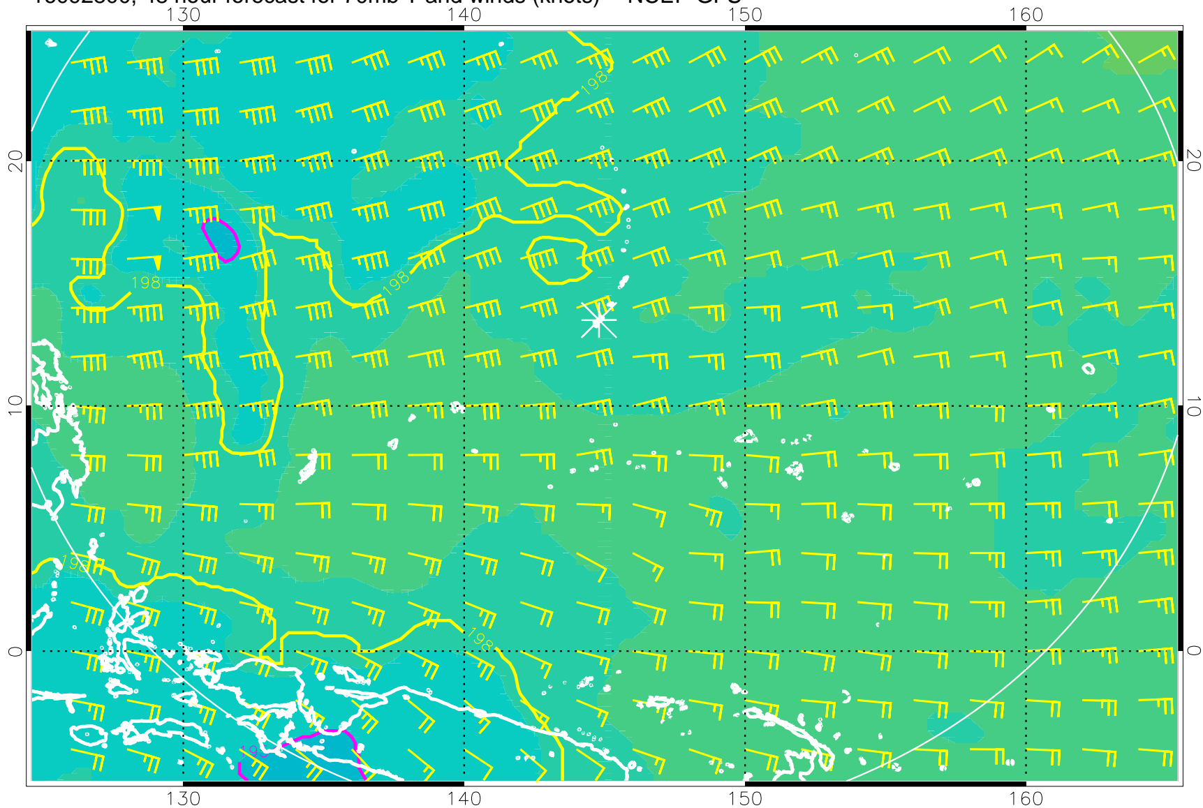
16092800, 48 hour forecast for 70mb T and winds (knots) -- NCEP GFS
