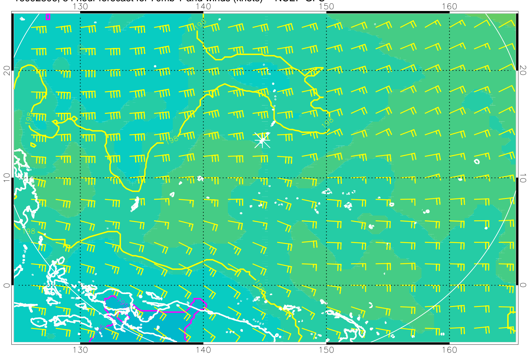
16092806, 54 hour forecast for 70mb T and winds (knots) -- NCEP GFS
