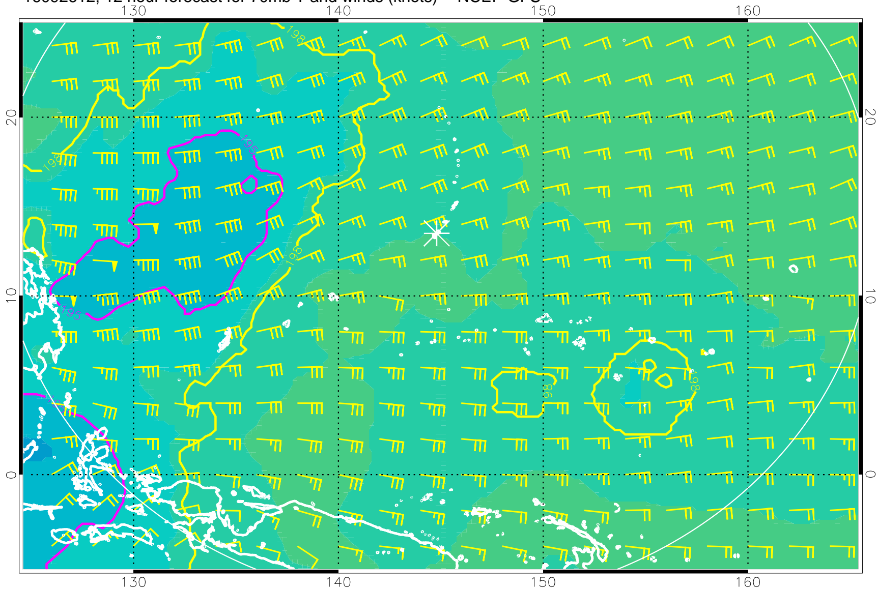
16092612, 12 hour forecast for 70mb T and winds (knots) -- NCEP GFS
