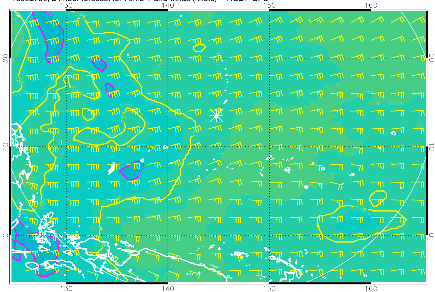
16092700, 24 hour forecast for 70mb T and winds (knots) -- NCEP GFS
