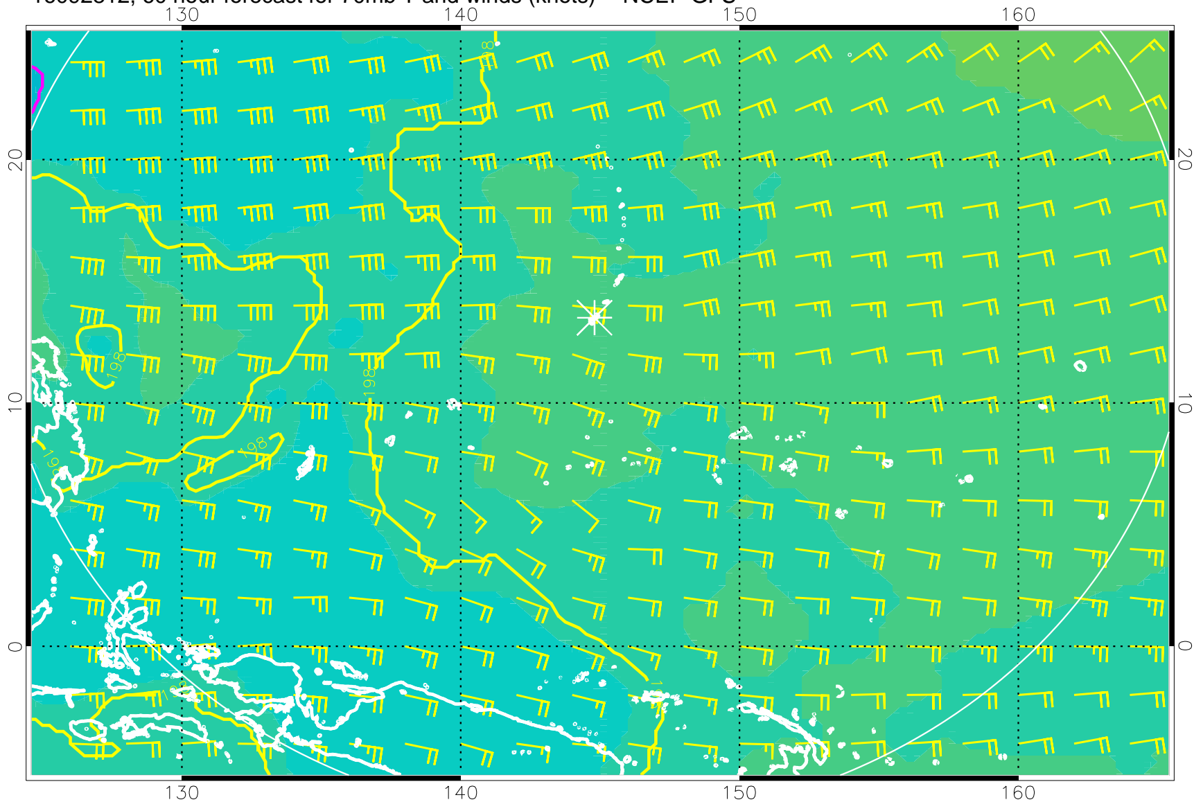
16092812, 60 hour forecast for 70mb T and winds (knots) -- NCEP GFS
