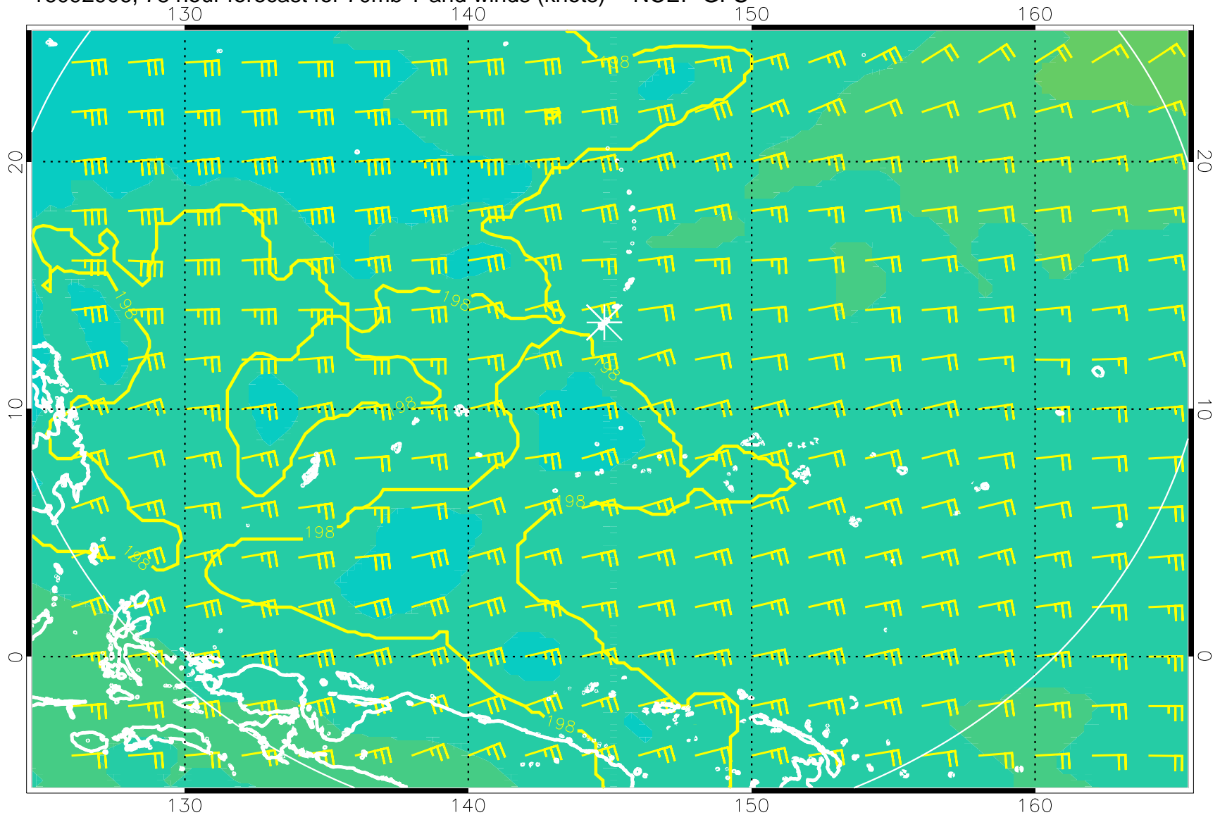
16092906, 78 hour forecast for 70mb T and winds (knots) -- NCEP GFS
