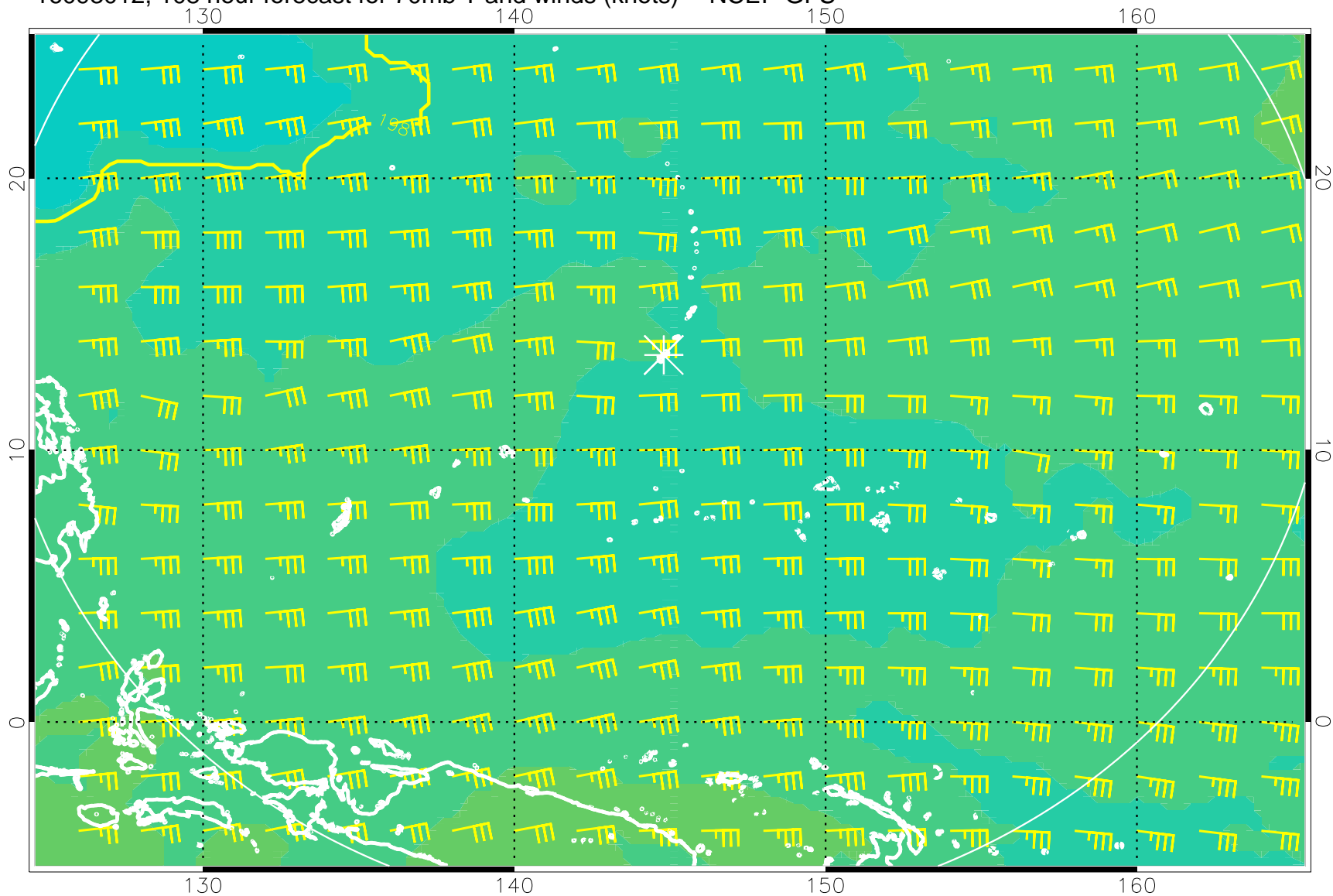
16093012, 108 hour forecast for 70mb T and winds (knots) -- NCEP GFS
