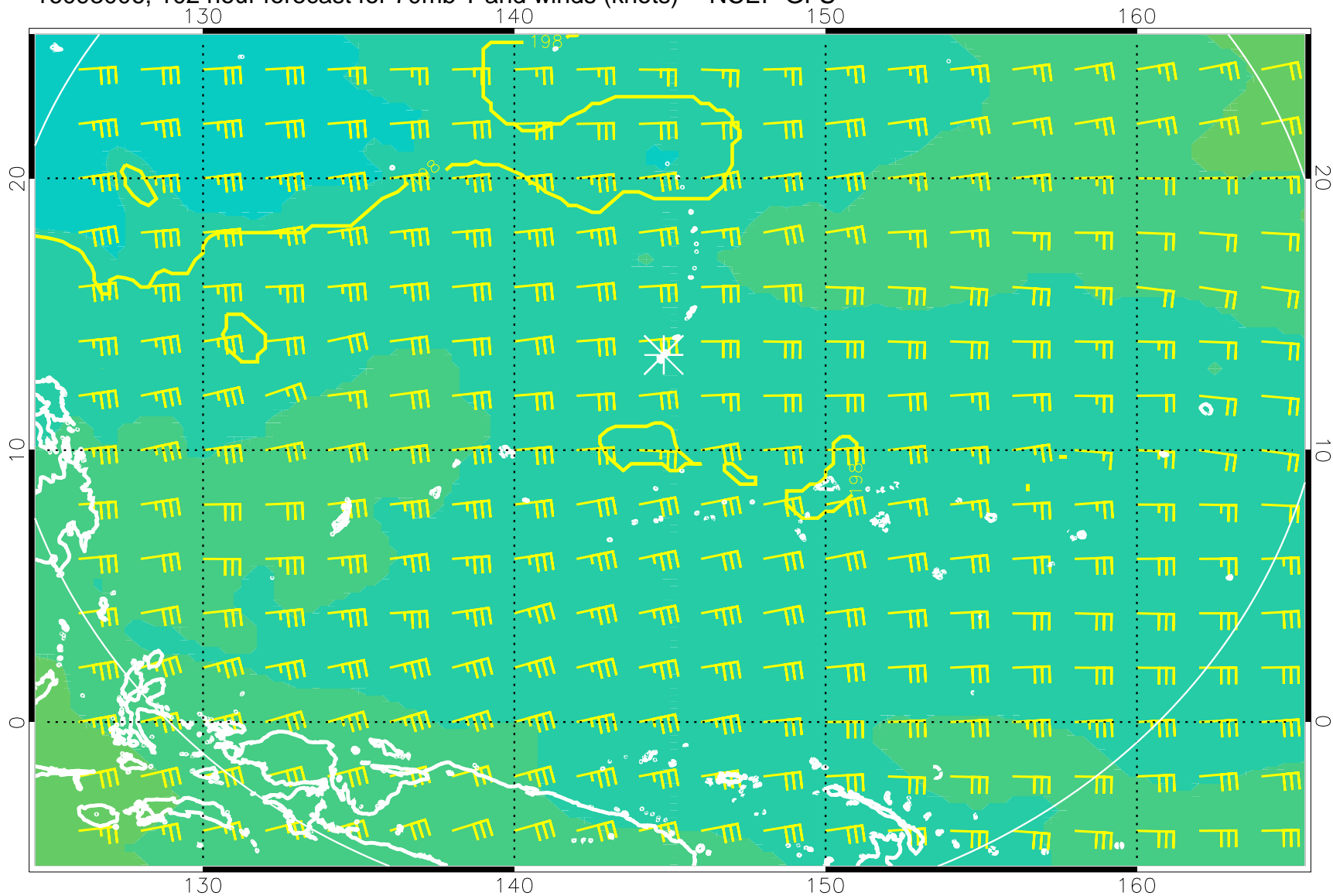
16093006, 102 hour forecast for 70mb T and winds (knots) -- NCEP GFS
