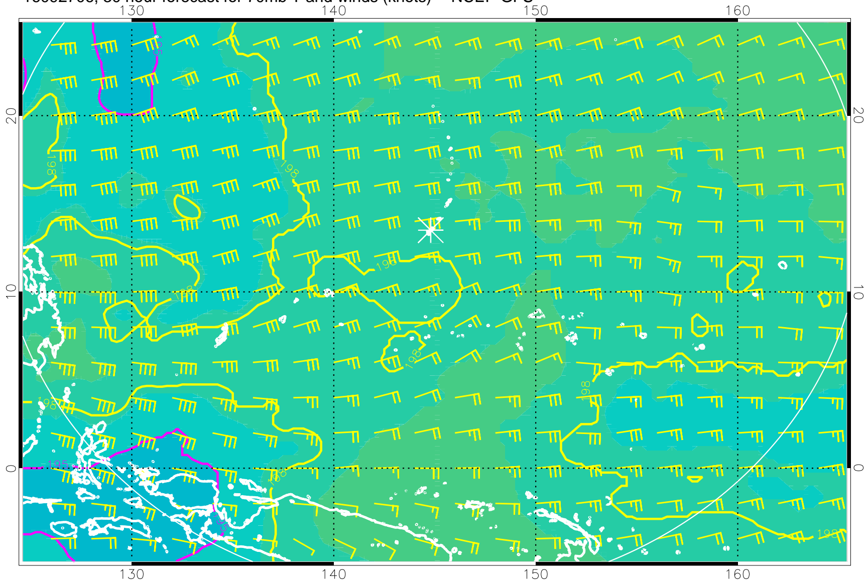
16092706, 30 hour forecast for 70mb T and winds (knots) -- NCEP GFS
