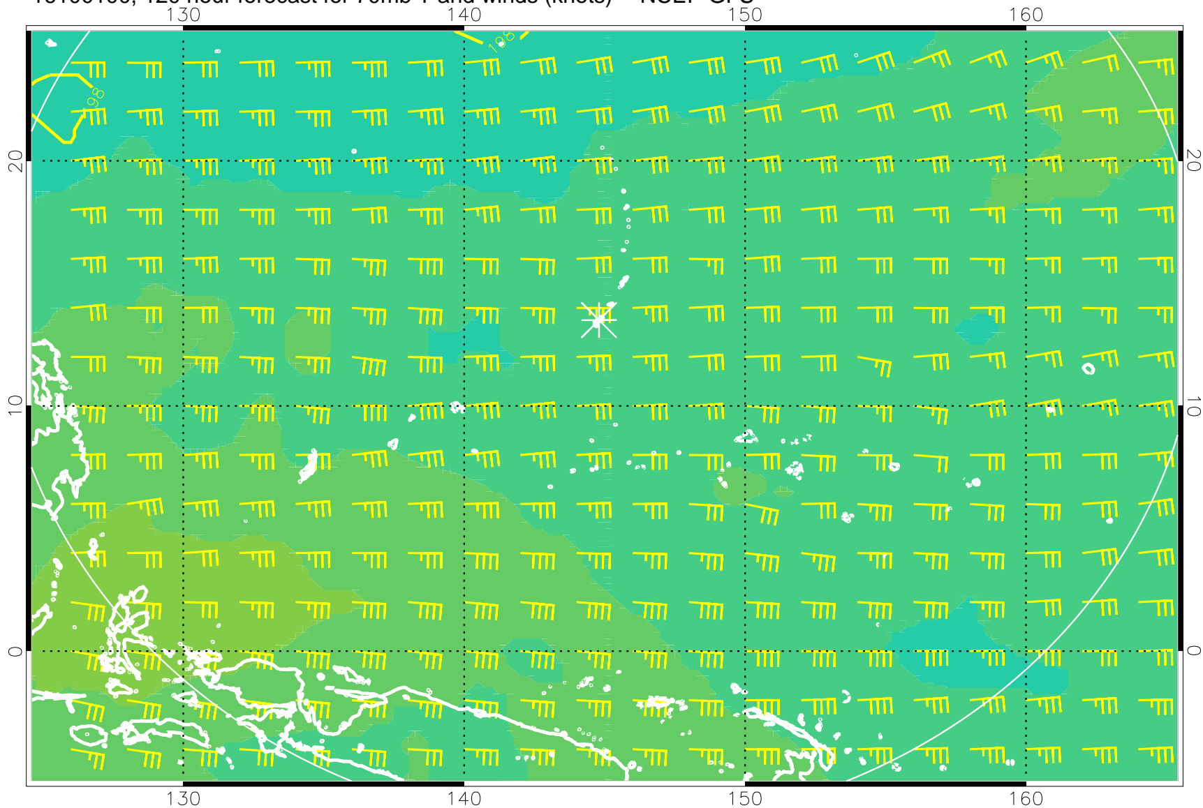
16100100, 120 hour forecast for 70mb T and winds (knots) -- NCEP GFS
