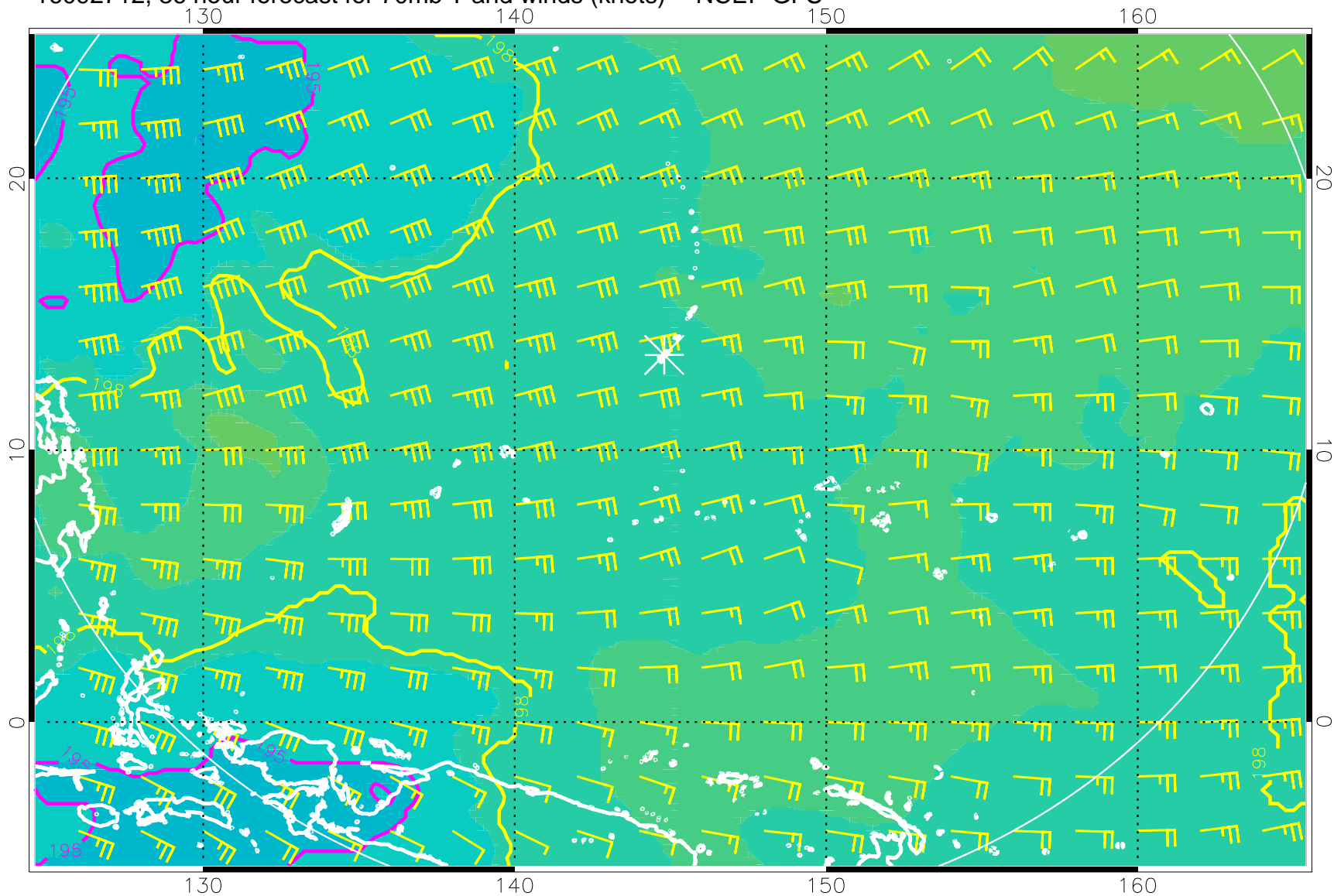
16092712, 36 hour forecast for 70mb T and winds (knots) -- NCEP GFS
