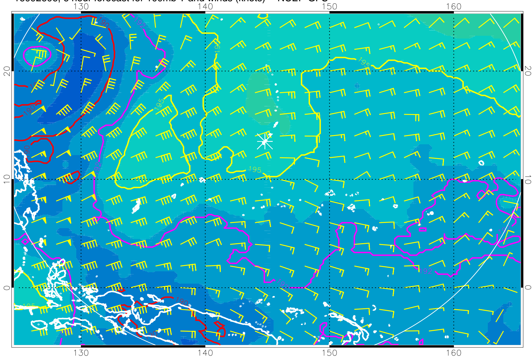
16092606, 6 hour forecast for 100mb T and winds (knots) -- NCEP GFS
