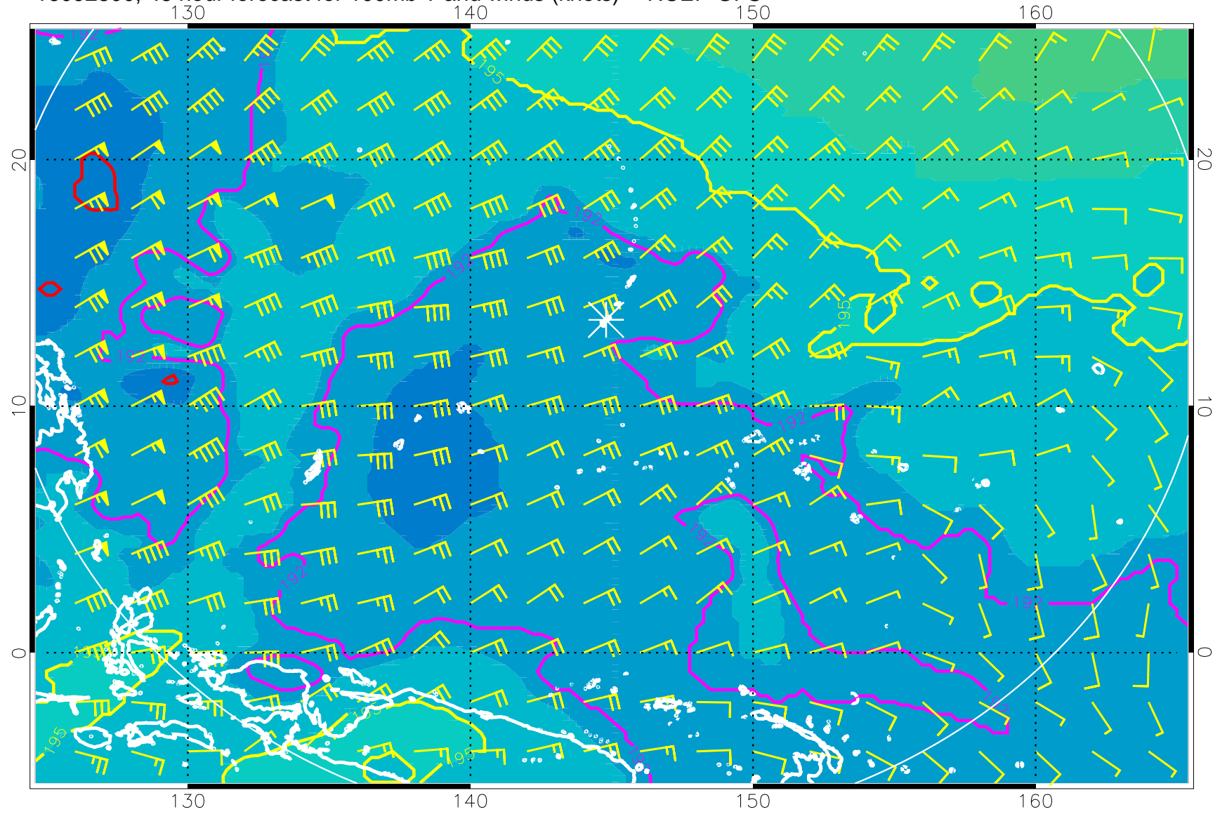
16092800, 48 hour forecast for 100mb T and winds (knots) -- NCEP GFS
