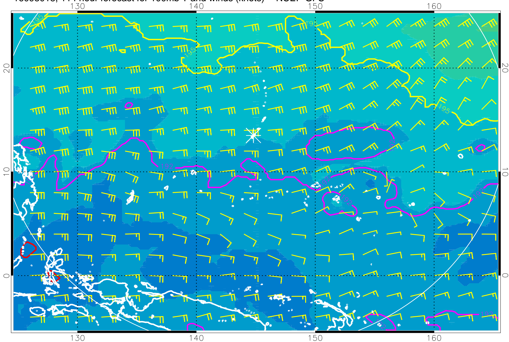
16093018, 114 hour forecast for 100mb T and winds (knots) -- NCEP GFS
