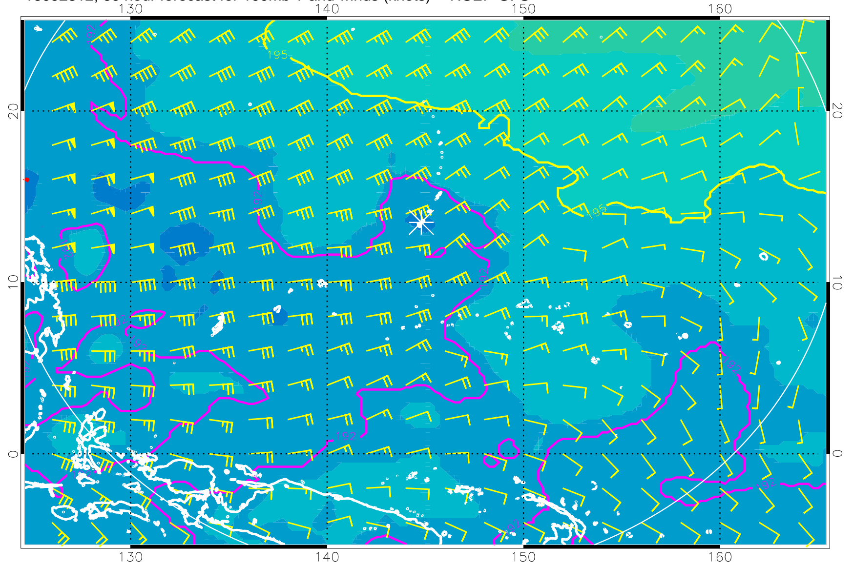
16092812, 60 hour forecast for 100mb T and winds (knots) -- NCEP GFS
