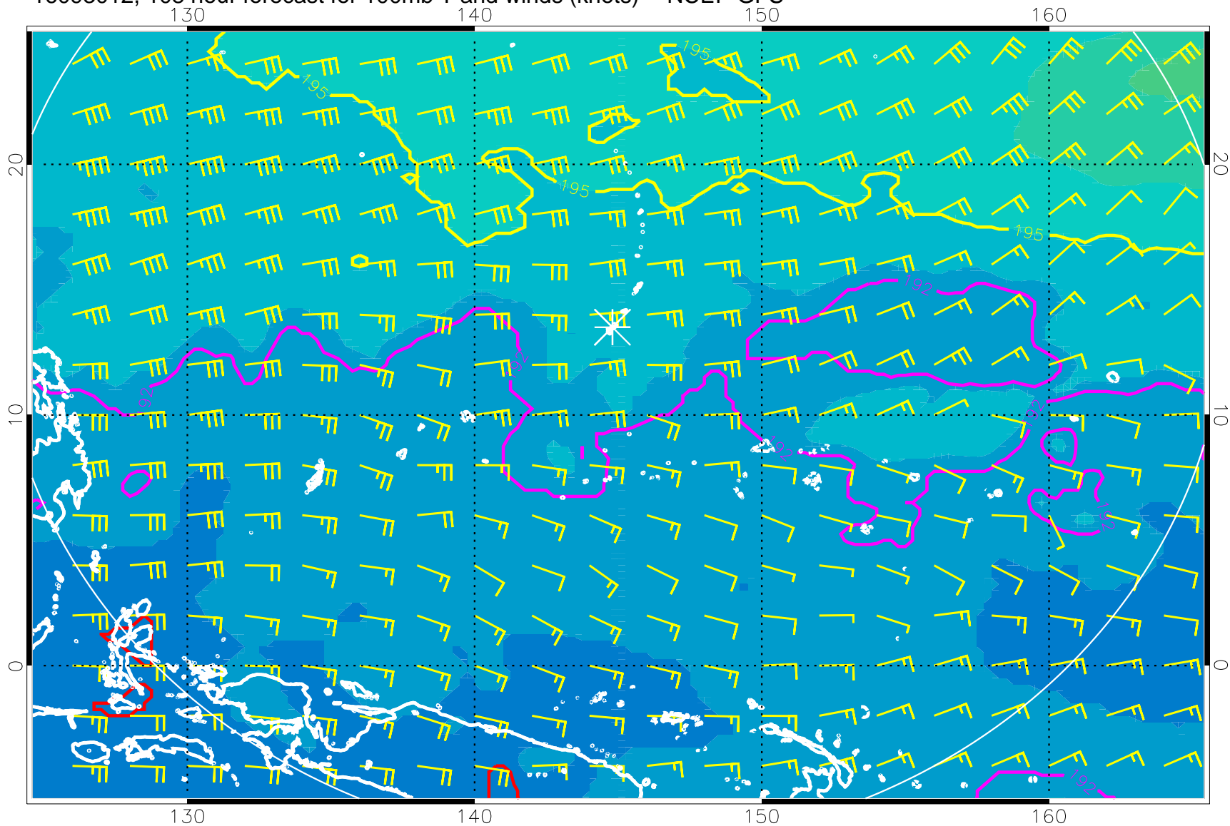
16093012, 108 hour forecast for 100mb T and winds (knots) -- NCEP GFS
