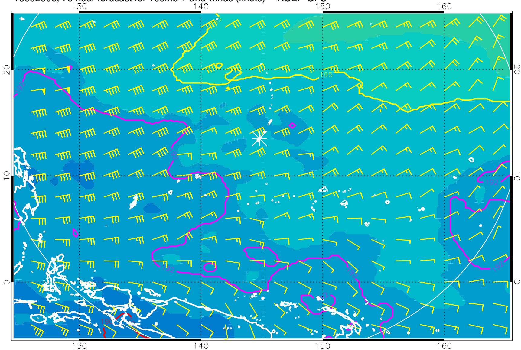
16092906, 78 hour forecast for 100mb T and winds (knots) -- NCEP GFS
