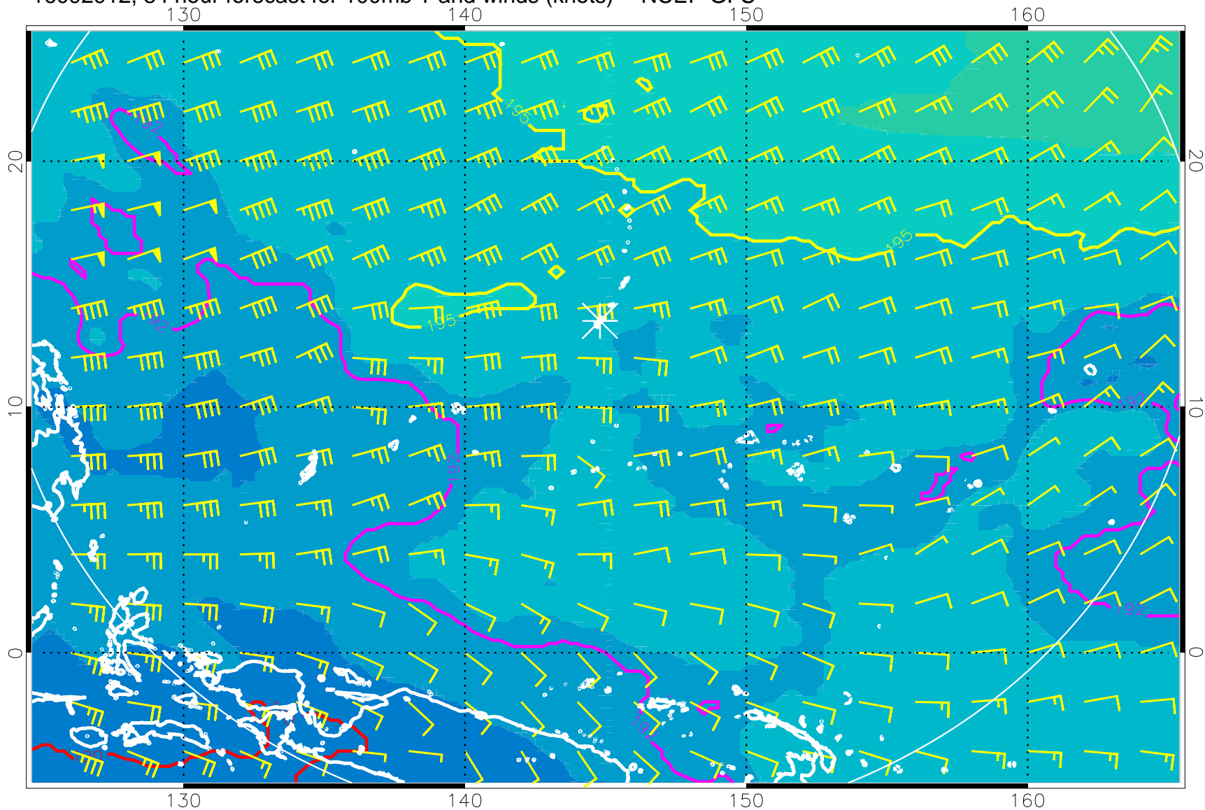
16092912, 84 hour forecast for 100mb T and winds (knots) -- NCEP GFS
