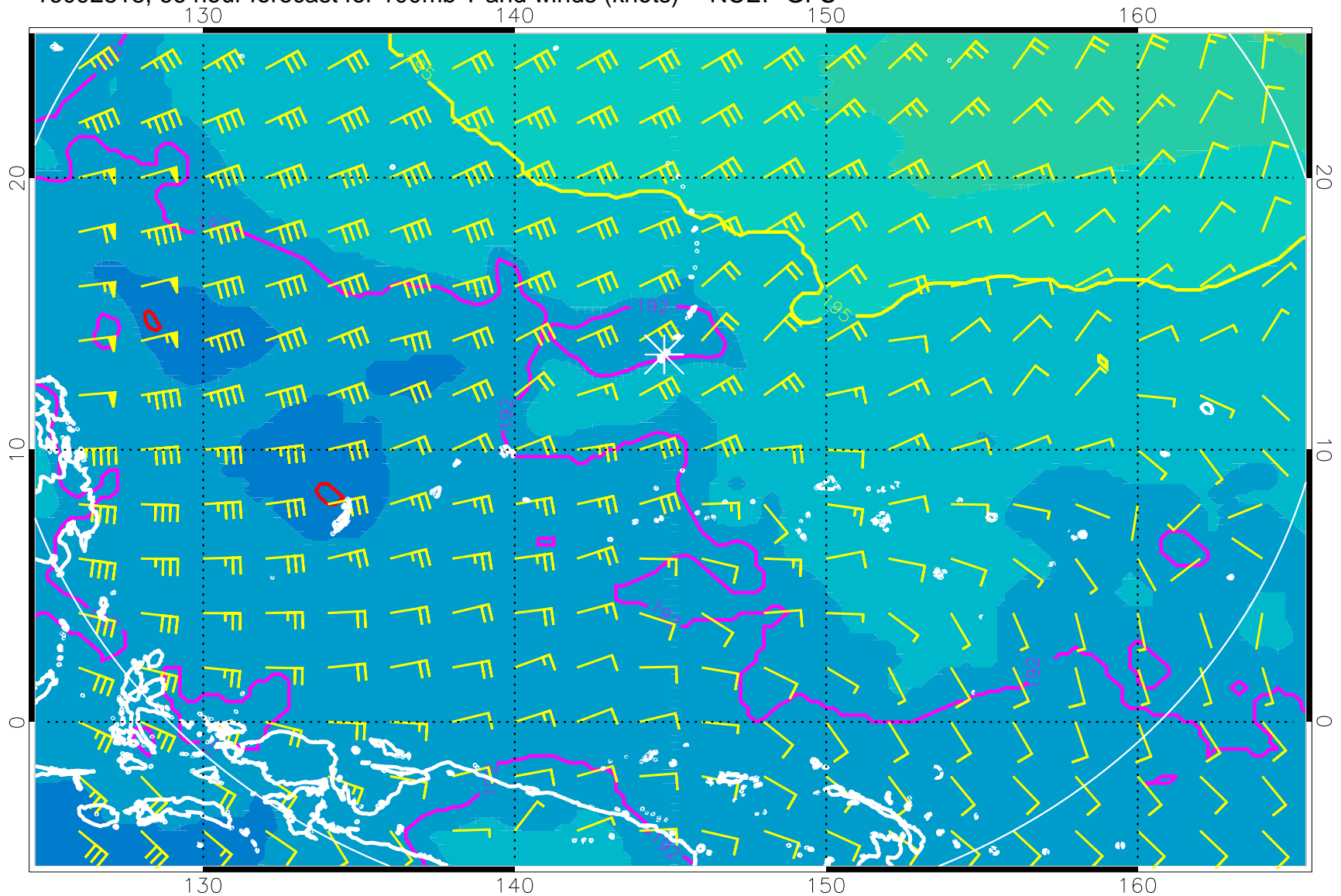
16092818, 66 hour forecast for 100mb T and winds (knots) -- NCEP GFS
