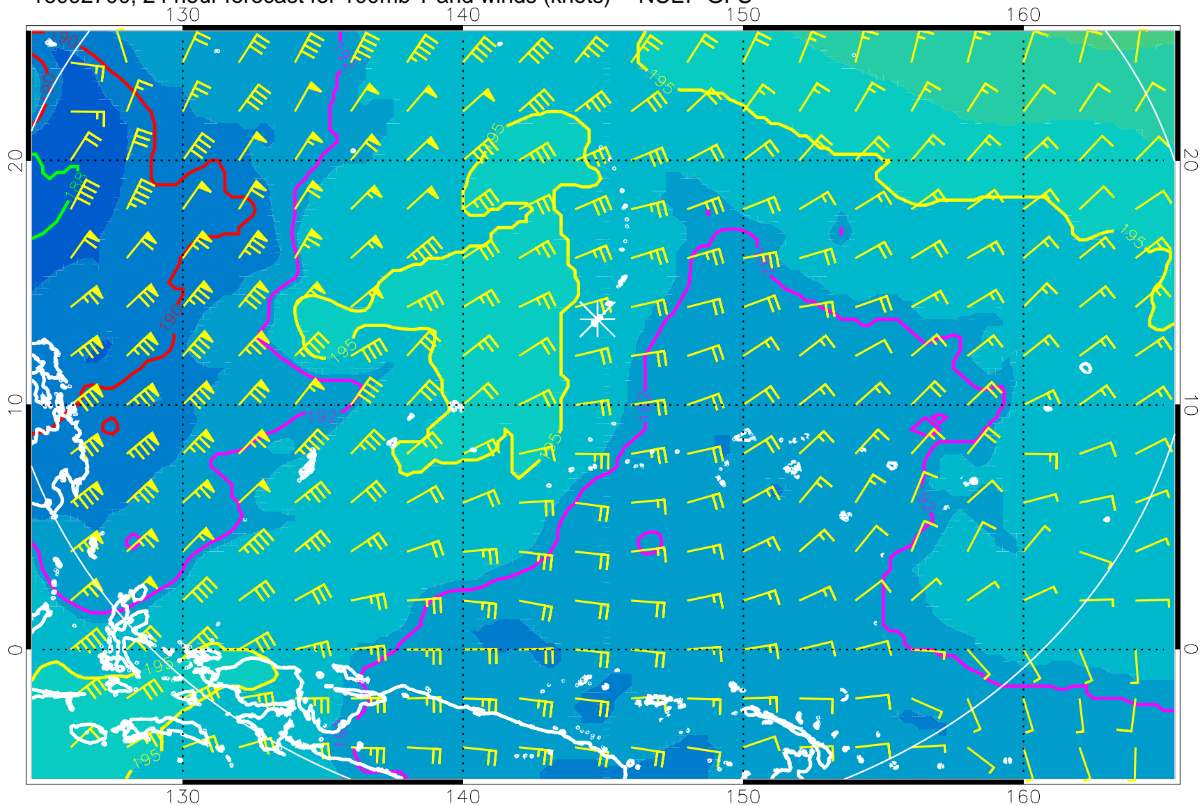
16092700, 24 hour forecast for 100mb T and winds (knots) -- NCEP GFS
