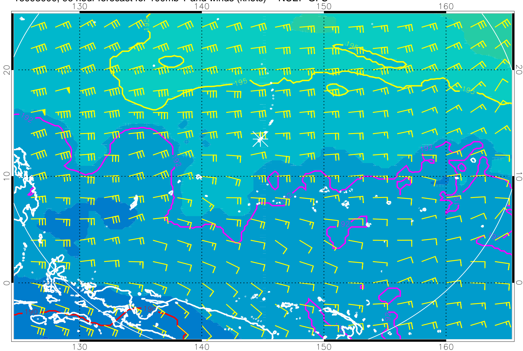
16093000, 96 hour forecast for 100mb T and winds (knots) -- NCEP GFS
