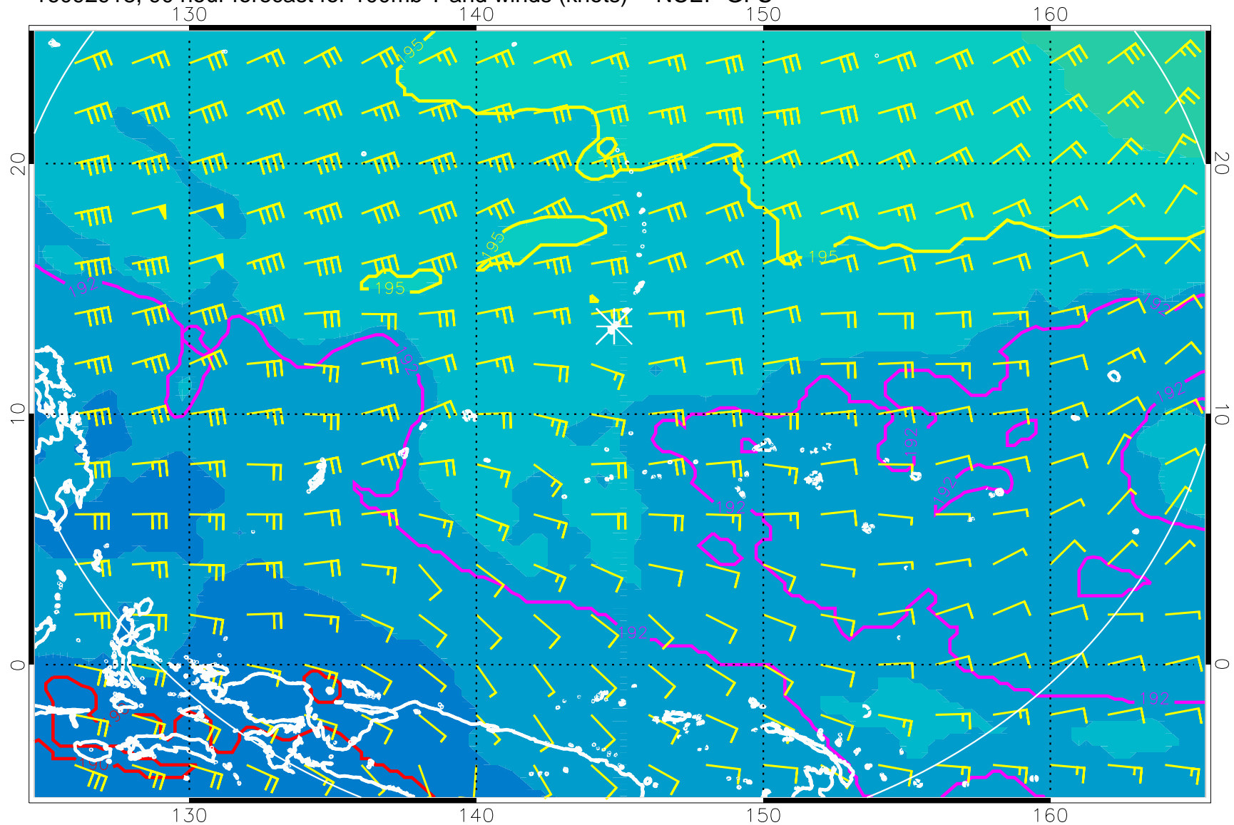
16092918, 90 hour forecast for 100mb T and winds (knots) -- NCEP GFS
