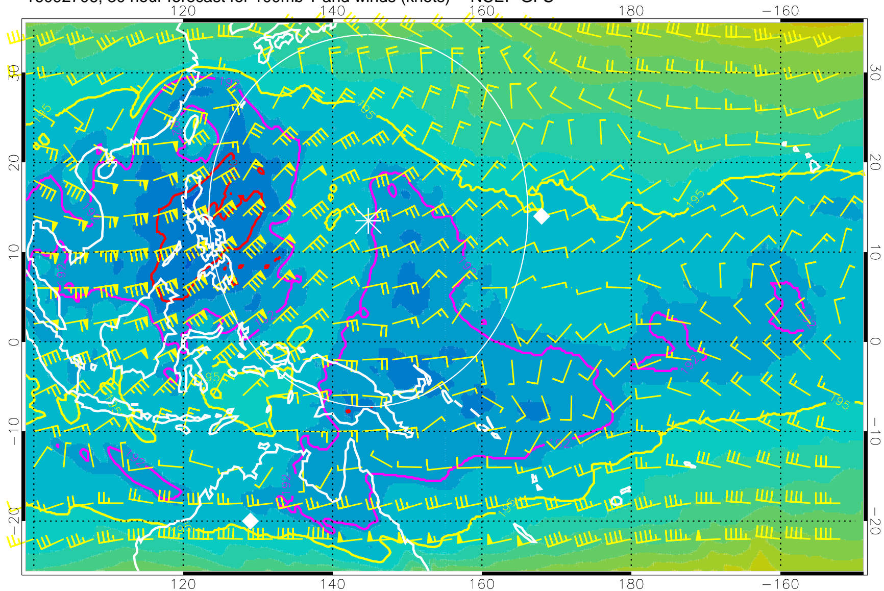
16092706, 30 hour forecast for 100mb T and winds (knots) -- NCEP GFS
