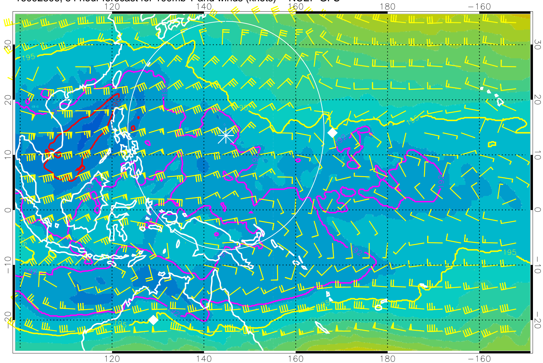
16092806, 54 hour forecast for 100mb T and winds (knots) -- NCEP GFS
