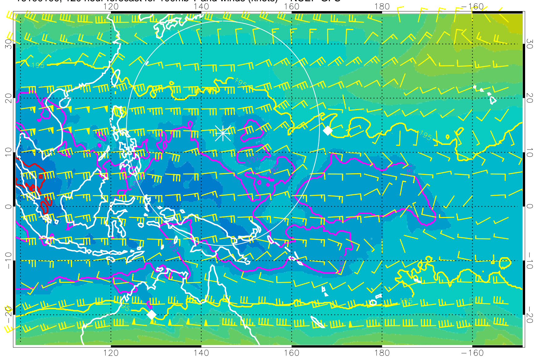
16100100, 120 hour forecast for 100mb T and winds (knots) -- NCEP GFS
