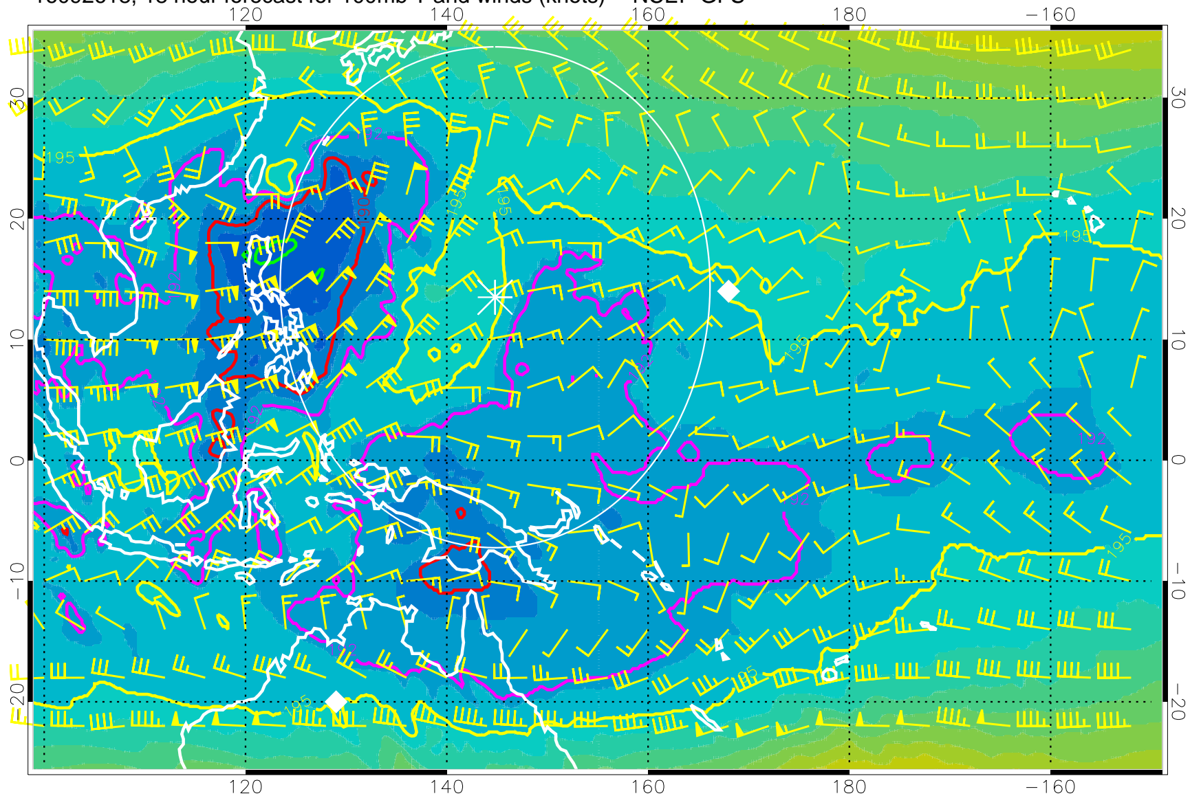
16092618, 18 hour forecast for 100mb T and winds (knots) -- NCEP GFS
