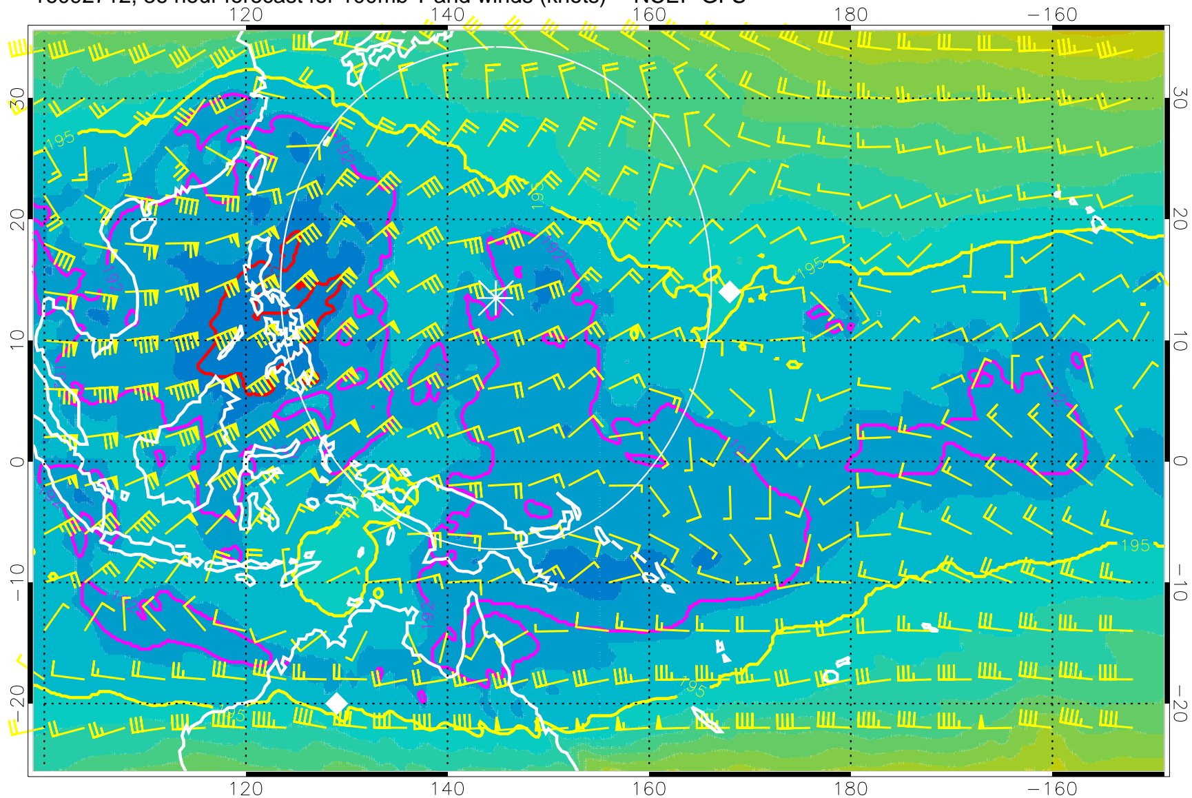
16092712, 36 hour forecast for 100mb T and winds (knots) -- NCEP GFS
