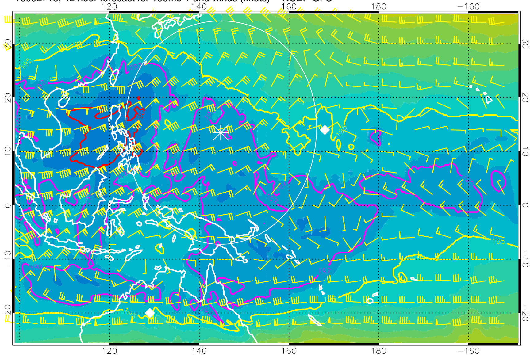
16092718, 42 hour forecast for 100mb T and winds (knots) -- NCEP GFS
