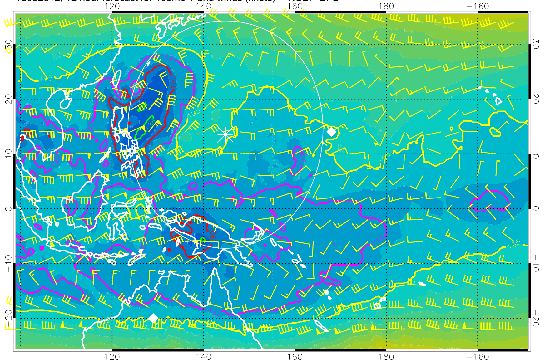
16092612, 12 hour forecast for 100mb T and winds (knots) -- NCEP GFS
