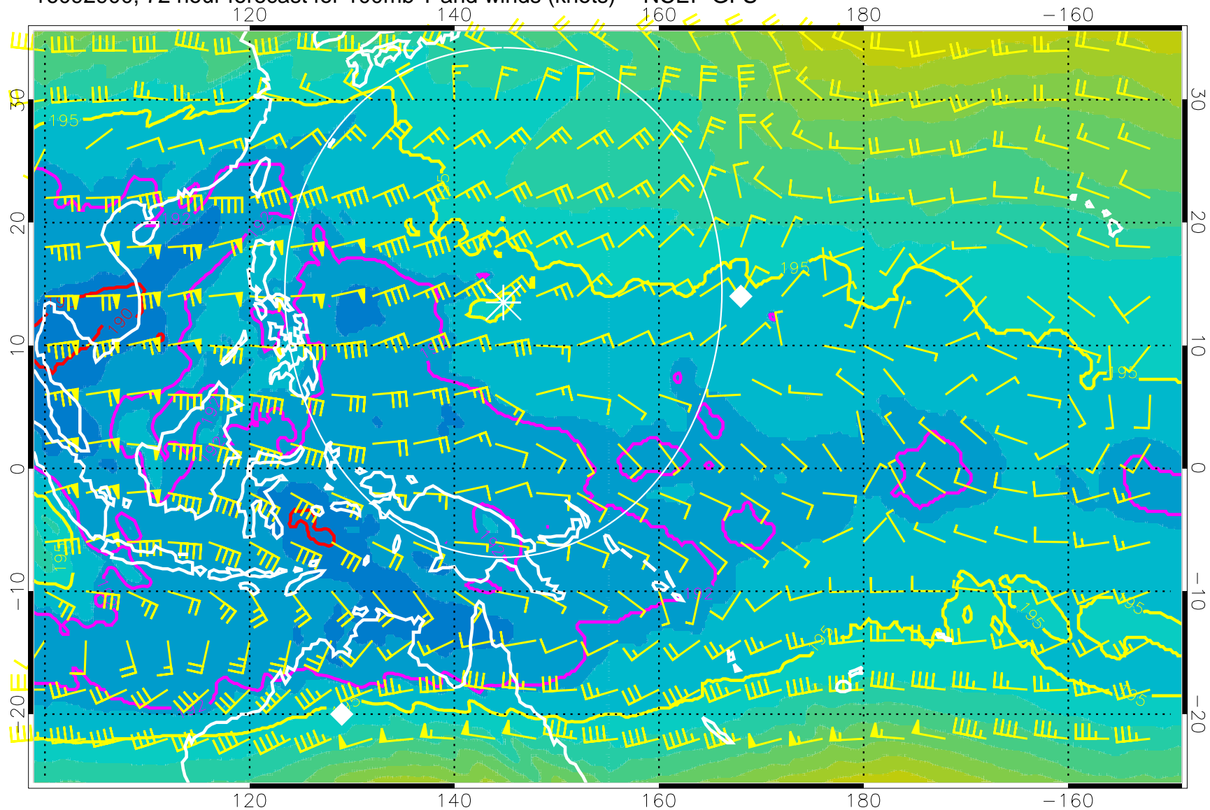
16092900, 72 hour forecast for 100mb T and winds (knots) -- NCEP GFS
