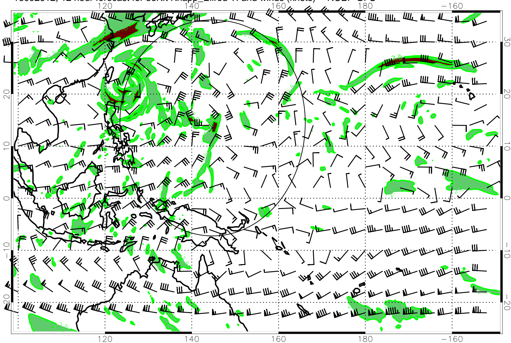
16092612, 12 hour forecast for 36Kft Knapp_Ellrod TI and winds (knots) -- NCEP GFS
