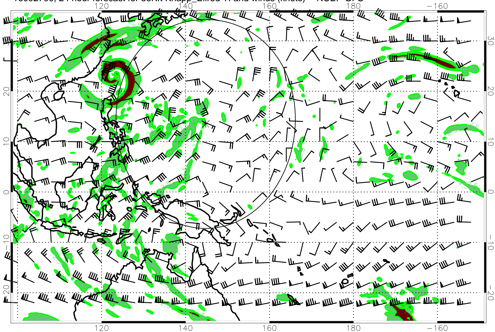
16092700, 24 hour forecast for 36Kft Knapp_Ellrod TI and winds (knots) -- NCEP GFS
