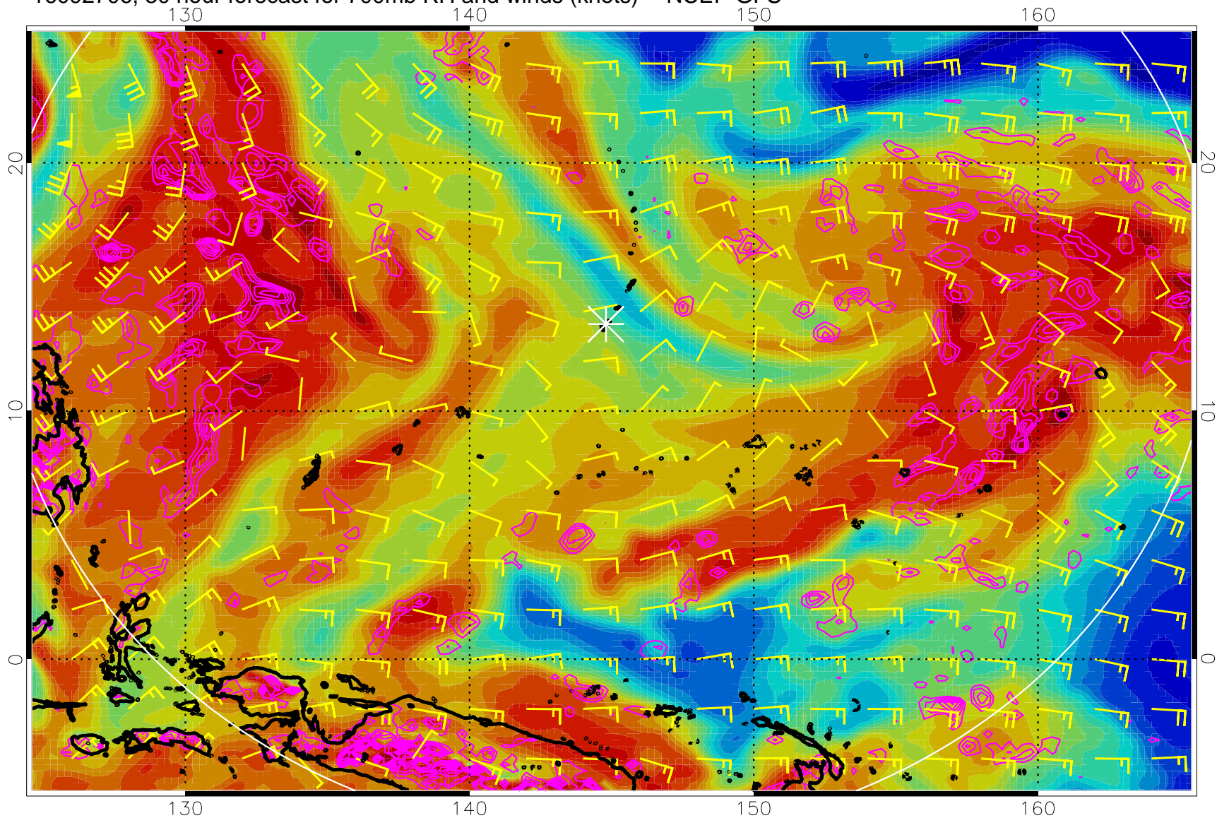
16092706, 30 hour forecast for 700mb RH and winds (knots) -- NCEP GFS
