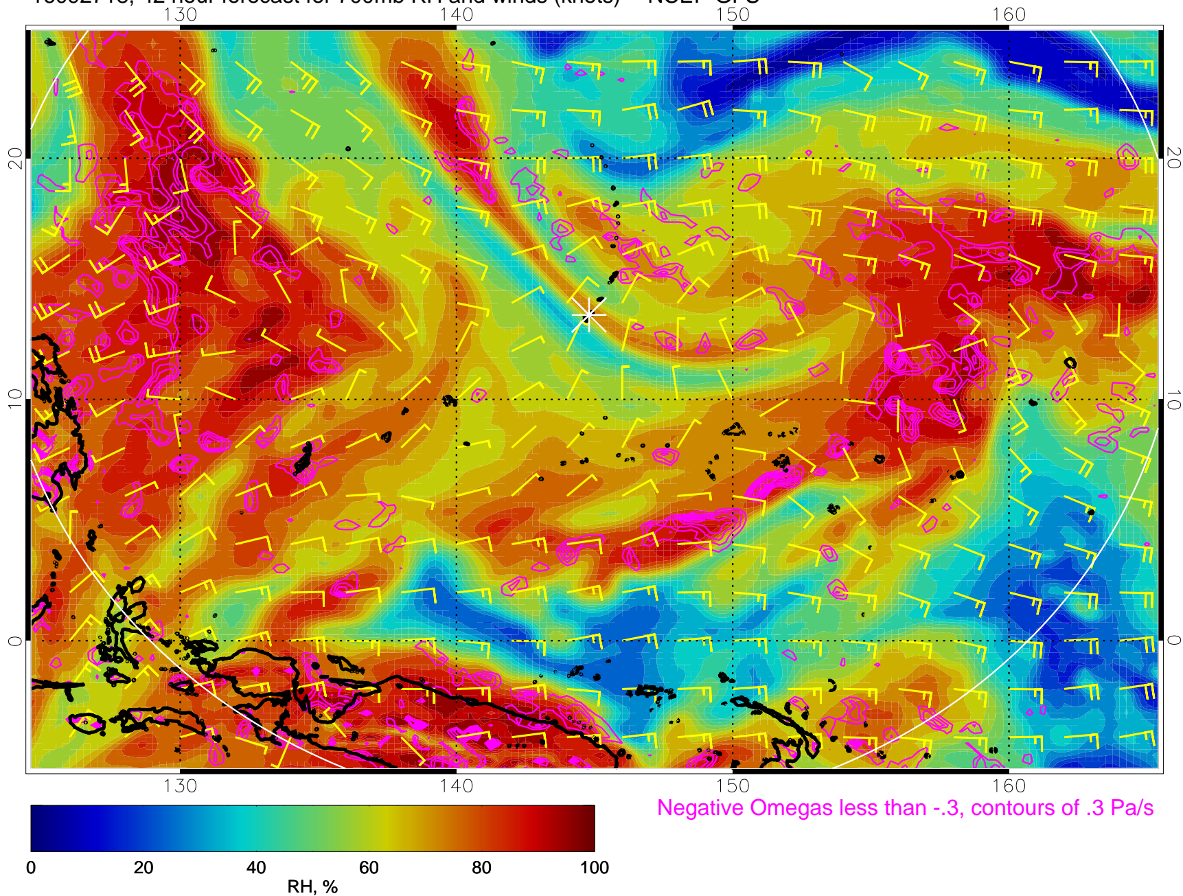
16092718, 42 hour forecast for 700mb RH and winds (knots) -- NCEP GFS
