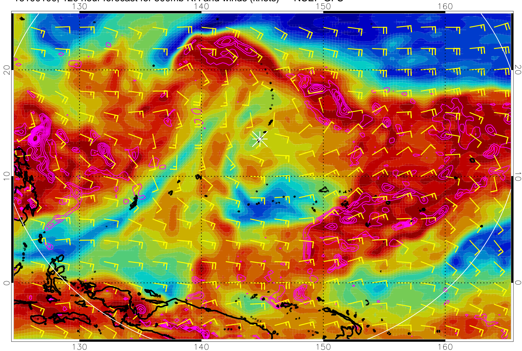
16100100, 120 hour forecast for 500mb RH and winds (knots) -- NCEP GFS
