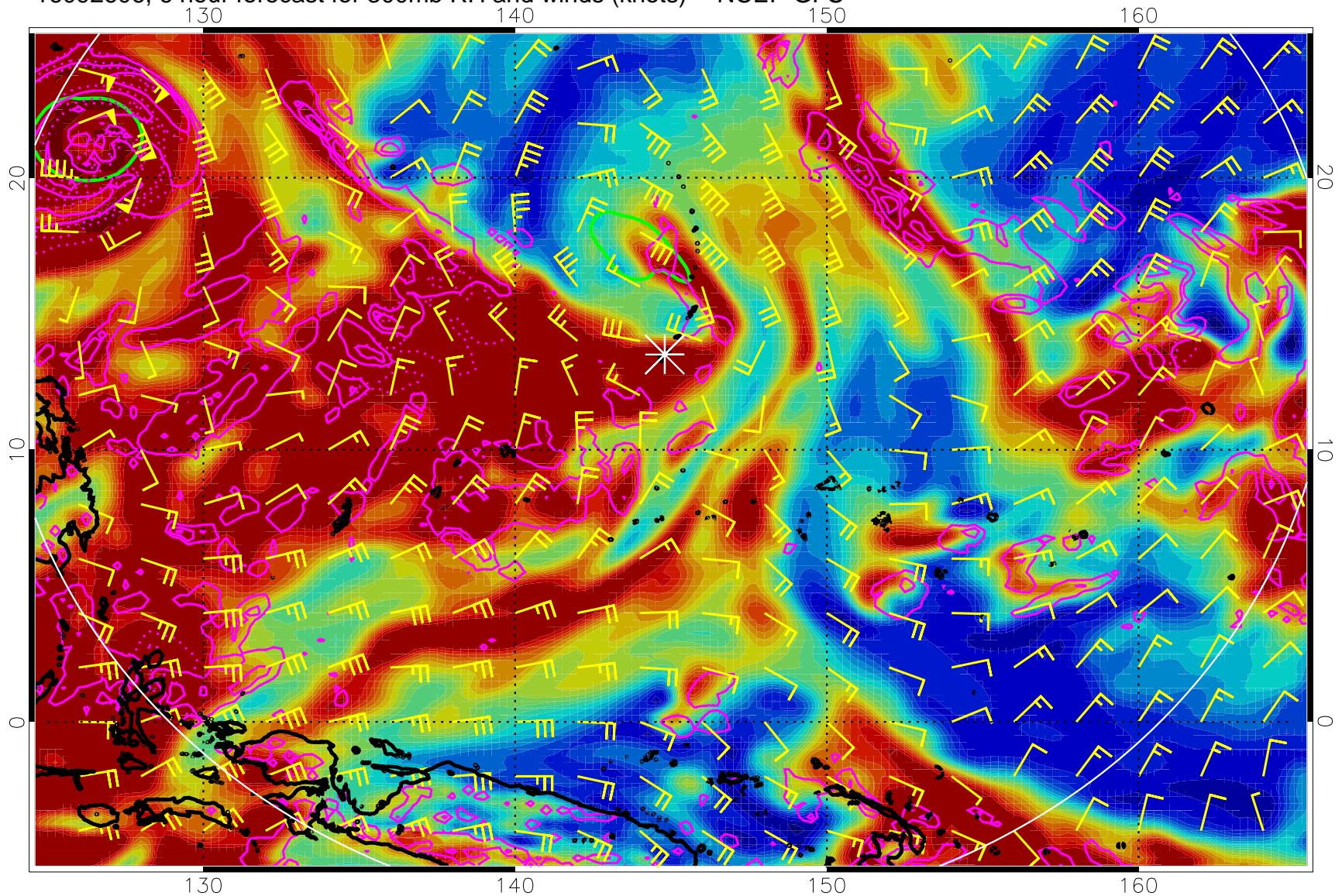
16092606, 6 hour forecast for 300mb RH and winds (knots) -- NCEP GFS
