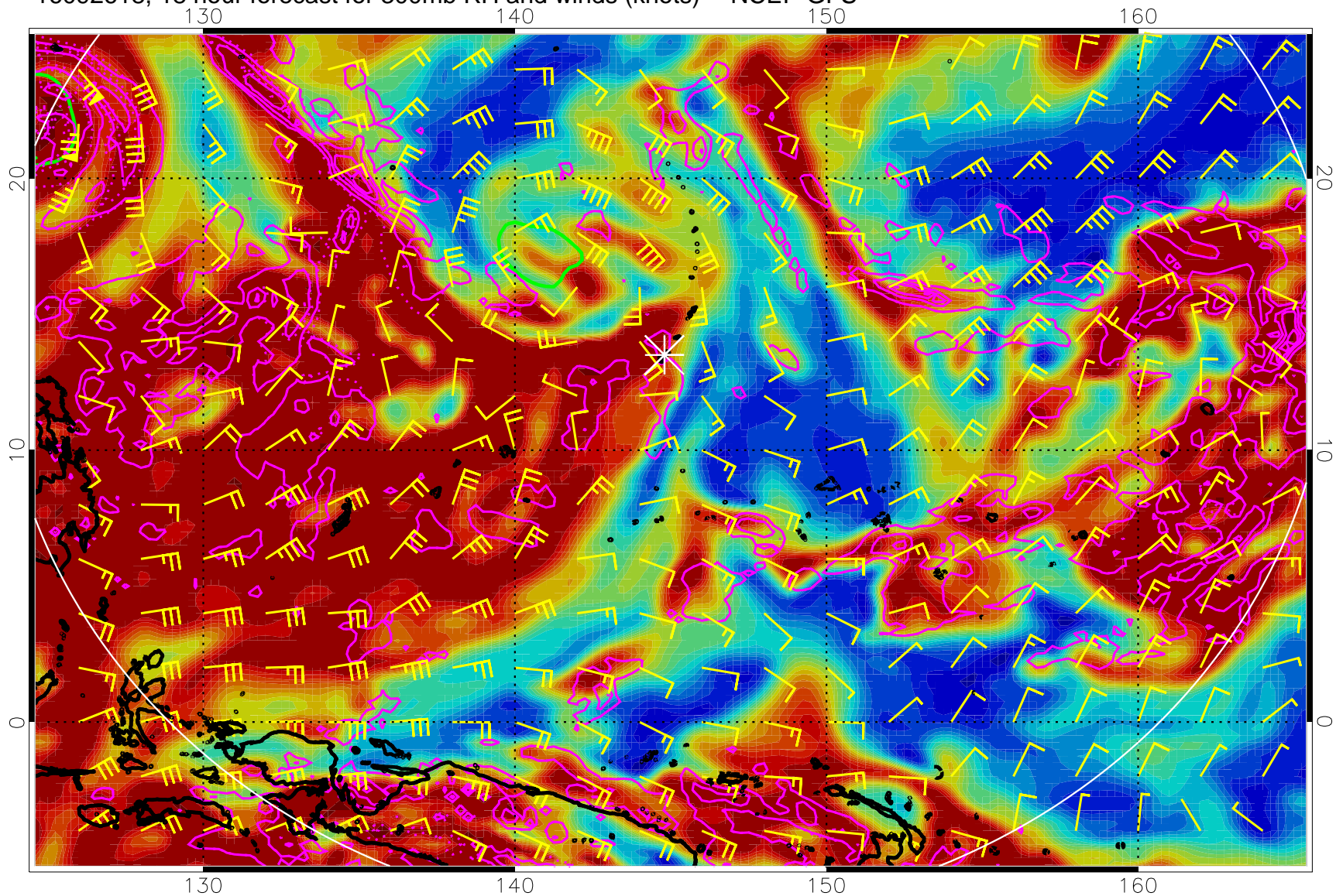
16092618, 18 hour forecast for 300mb RH and winds (knots) -- NCEP GFS
