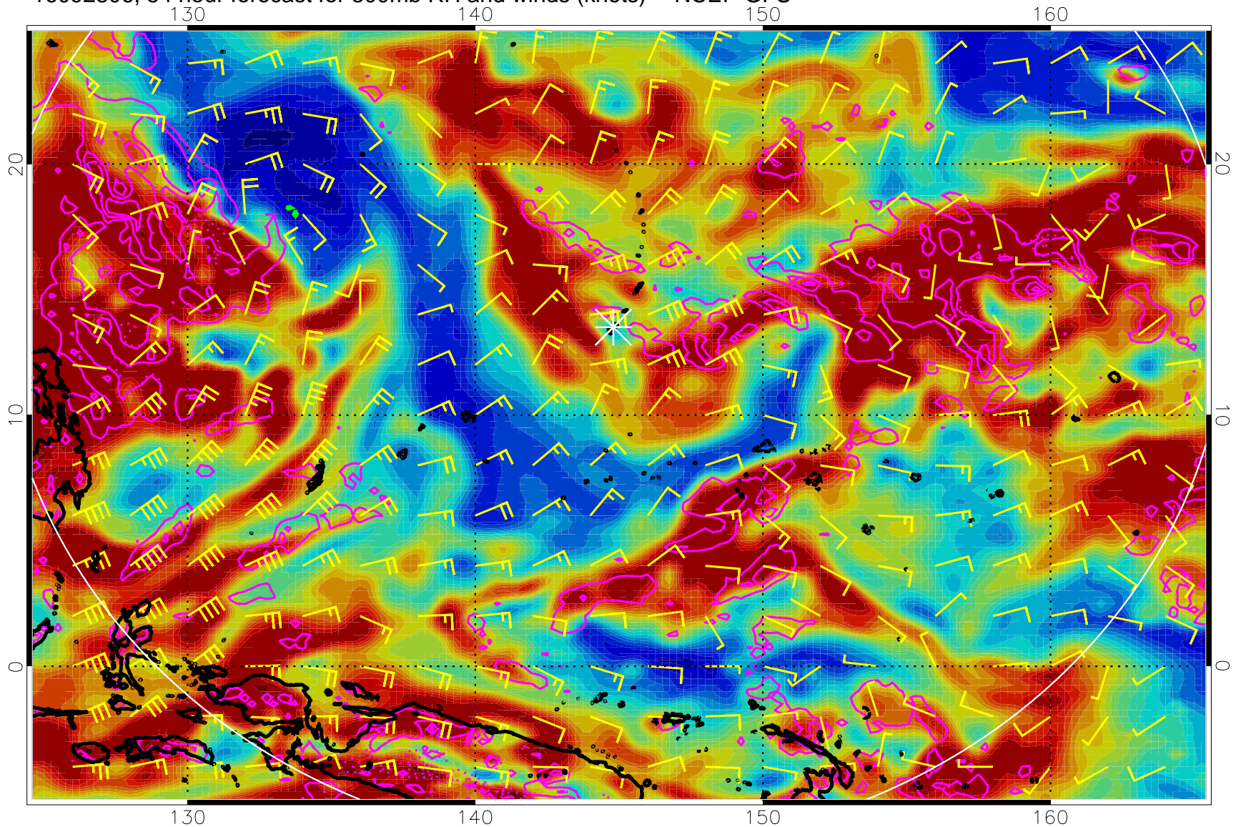
16092806, 54 hour forecast for 300mb RH and winds (knots) -- NCEP GFS
