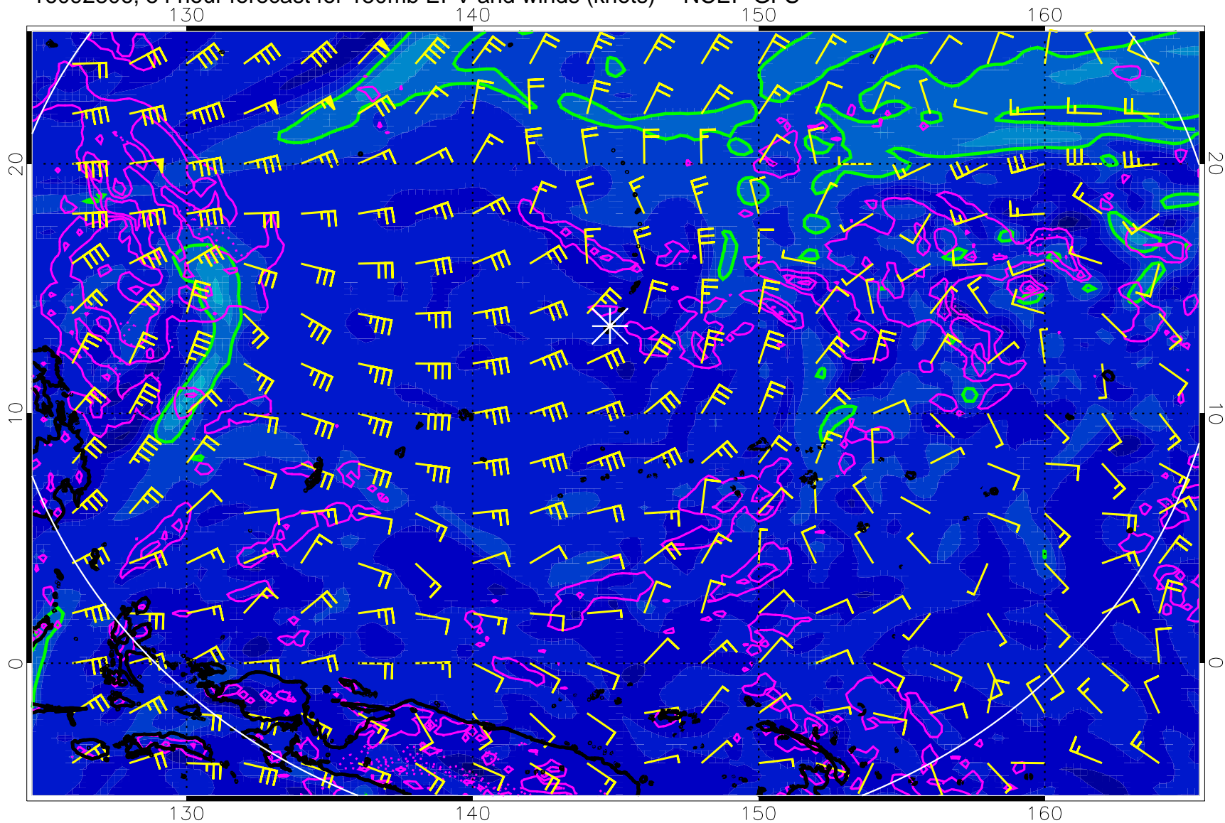
16092806, 54 hour forecast for 150mb EPV and winds (knots) -- NCEP GFS
