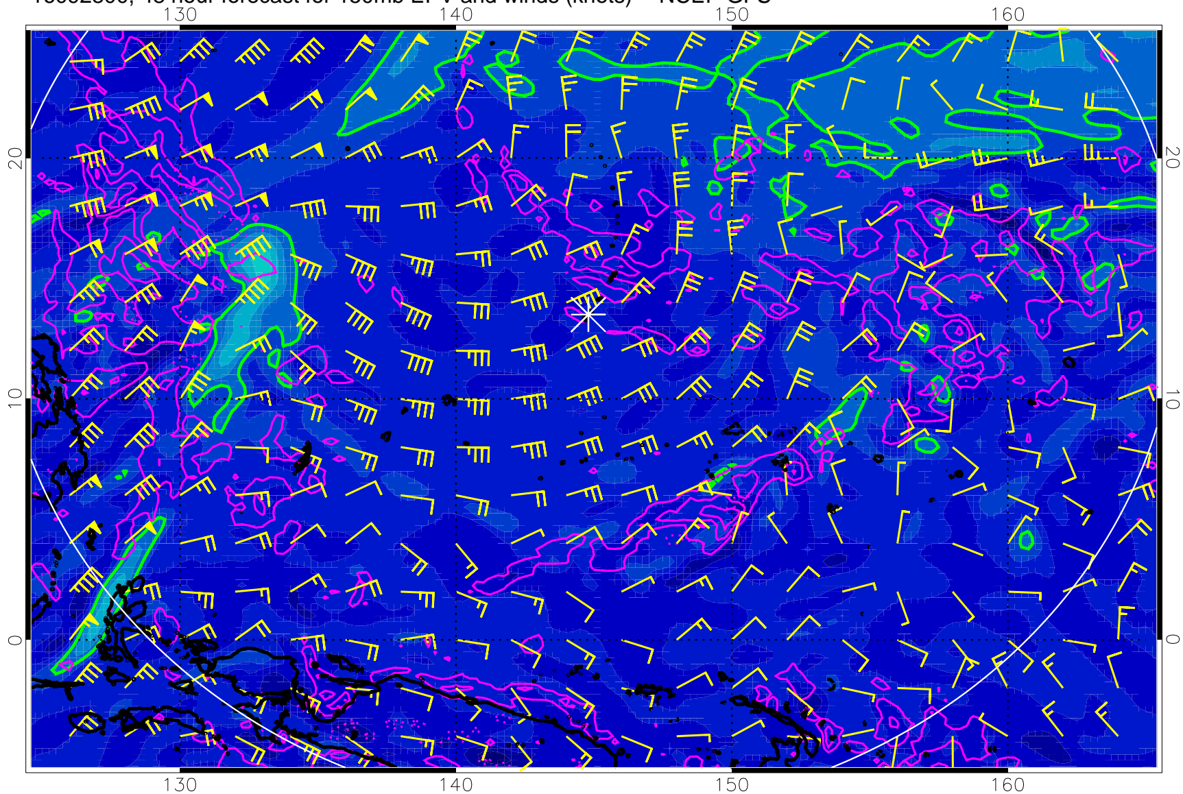
16092800, 48 hour forecast for 150mb EPV and winds (knots) -- NCEP GFS
