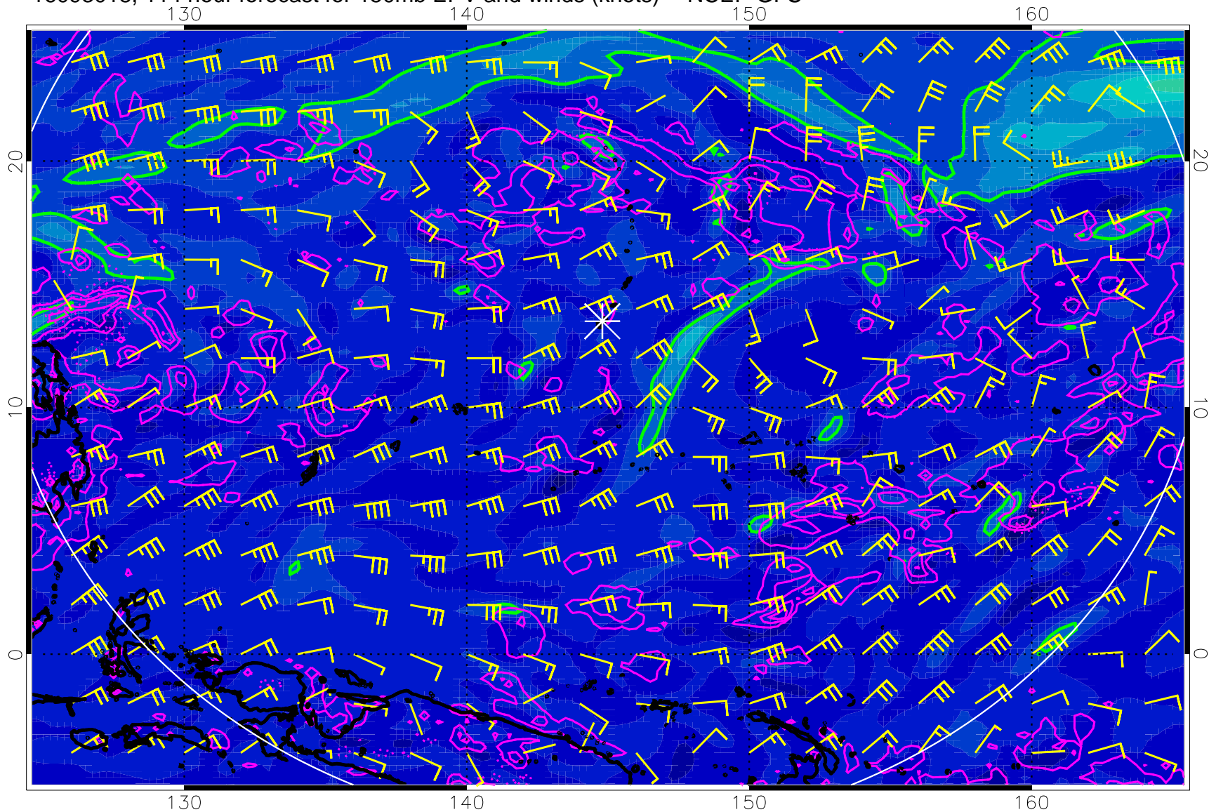
16093018, 114 hour forecast for 150mb EPV and winds (knots) -- NCEP GFS
