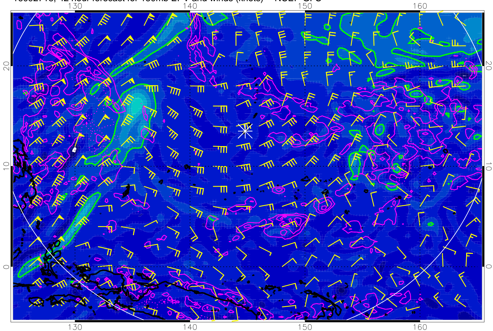
16092718, 42 hour forecast for 150mb EPV and winds (knots) -- NCEP GFS
