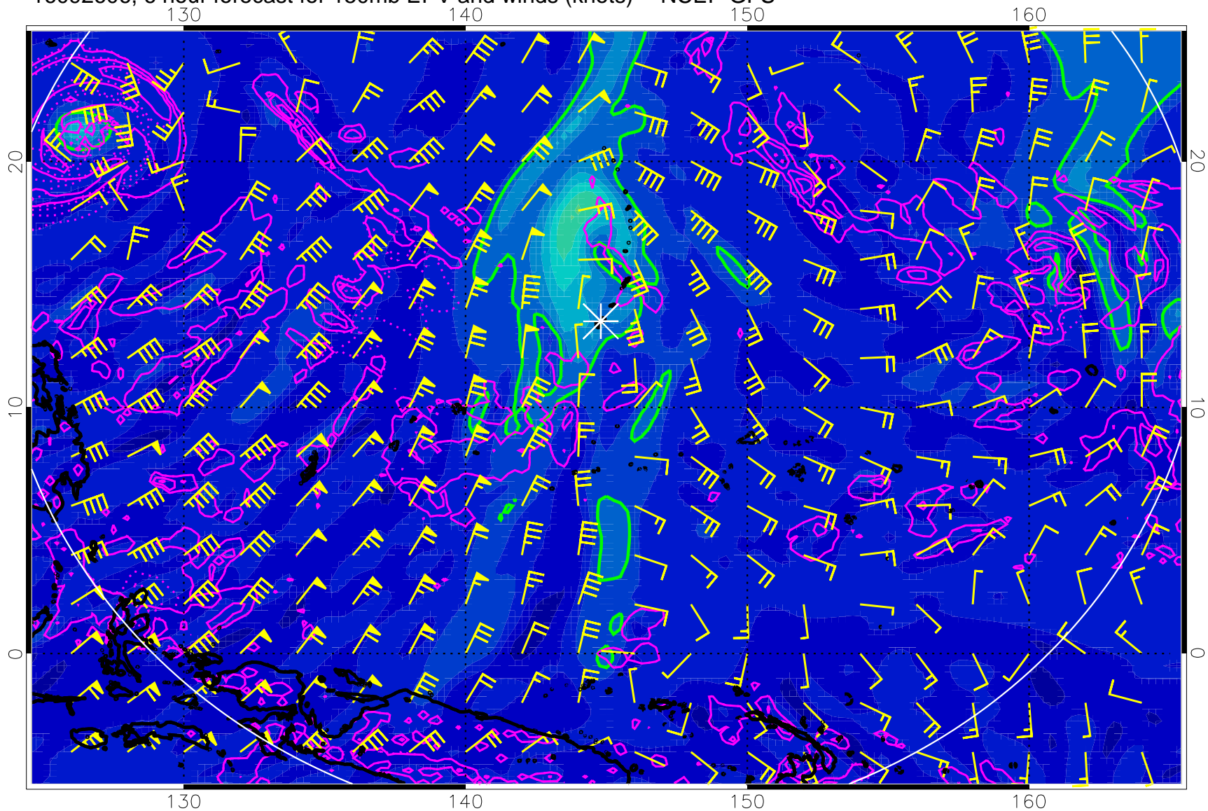
16092606, 6 hour forecast for 150mb EPV and winds (knots) -- NCEP GFS
