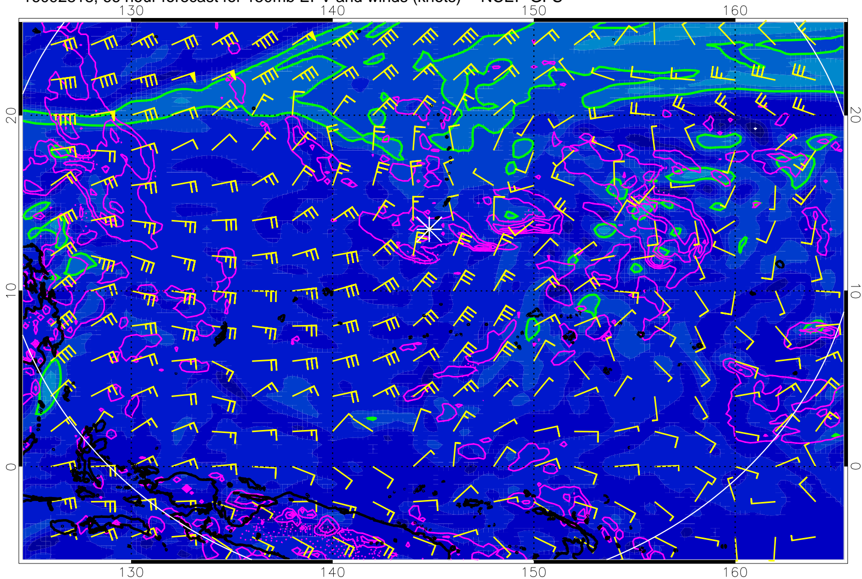
16092818, 66 hour forecast for 150mb EPV and winds (knots) -- NCEP GFS
