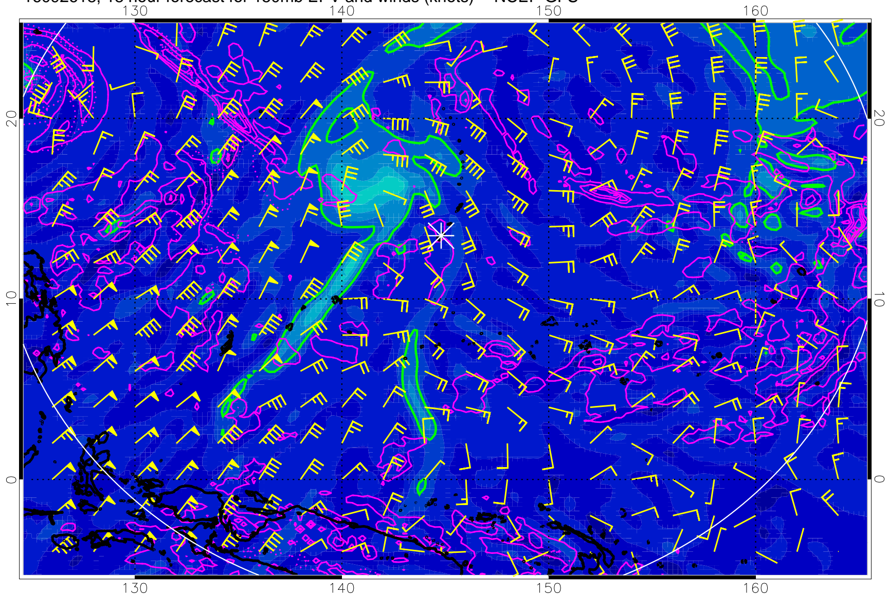
16092618, 18 hour forecast for 150mb EPV and winds (knots) -- NCEP GFS
