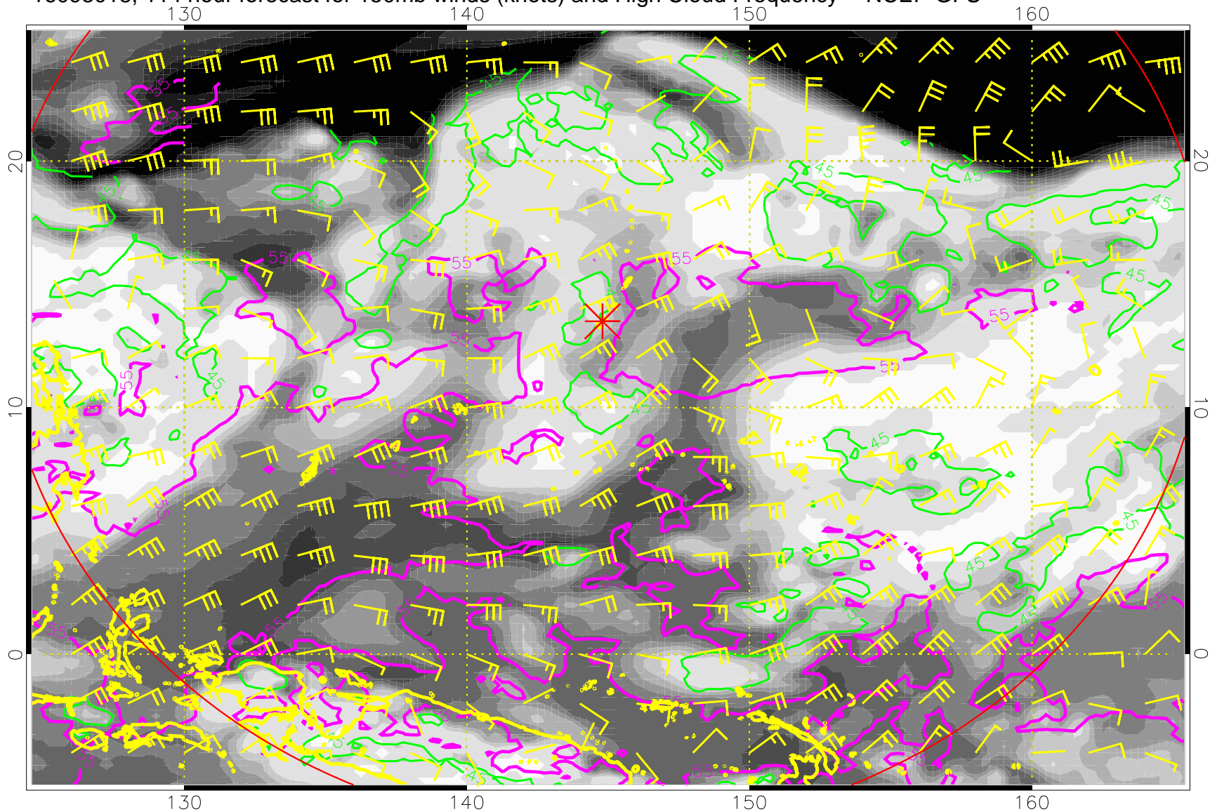
16093018, 114 hour forecast for 150mb winds (knots) and High Cloud Frequency -- NCEP GFS
