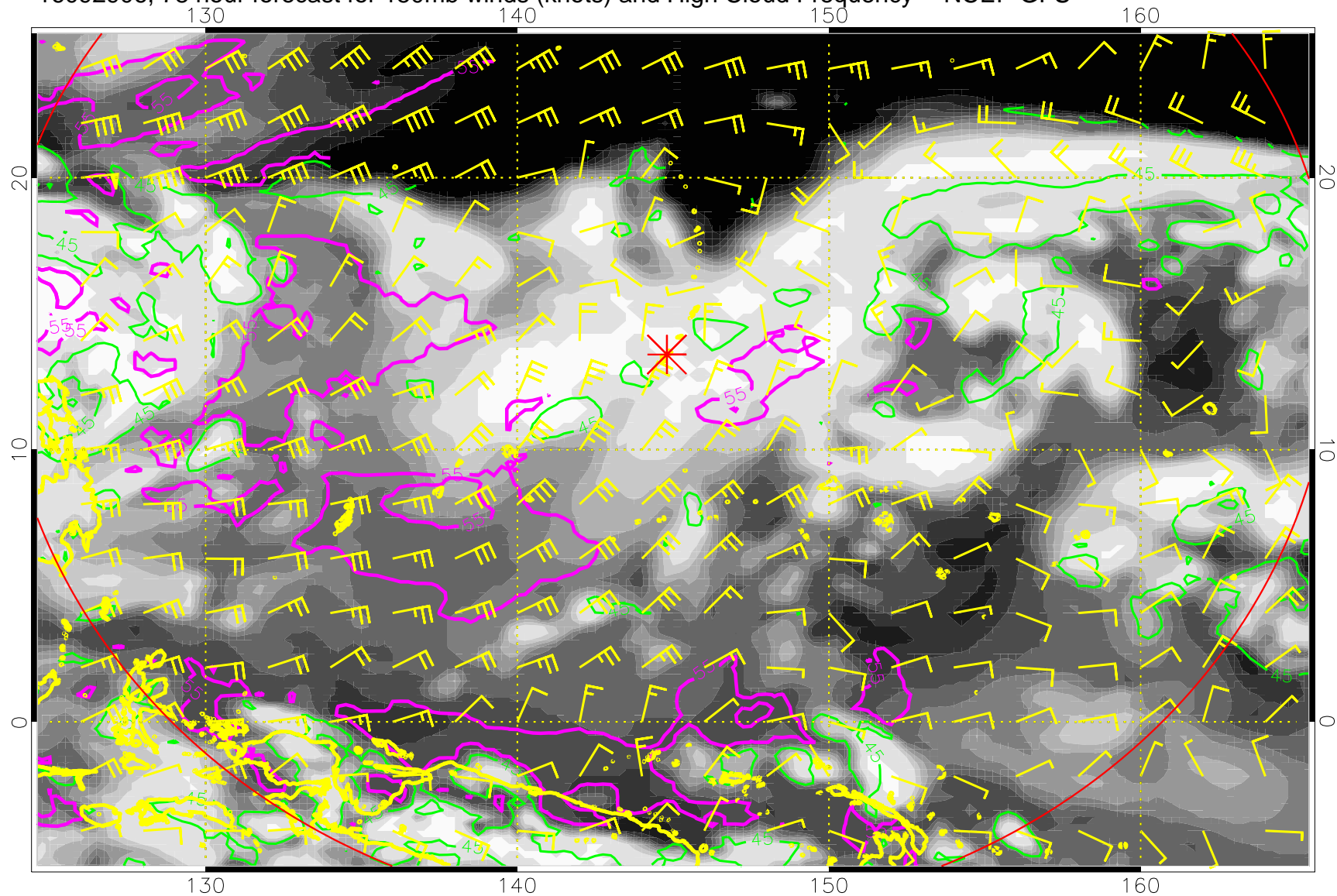
16092906, 78 hour forecast for 150mb winds (knots) and High Cloud Frequency -- NCEP GFS
