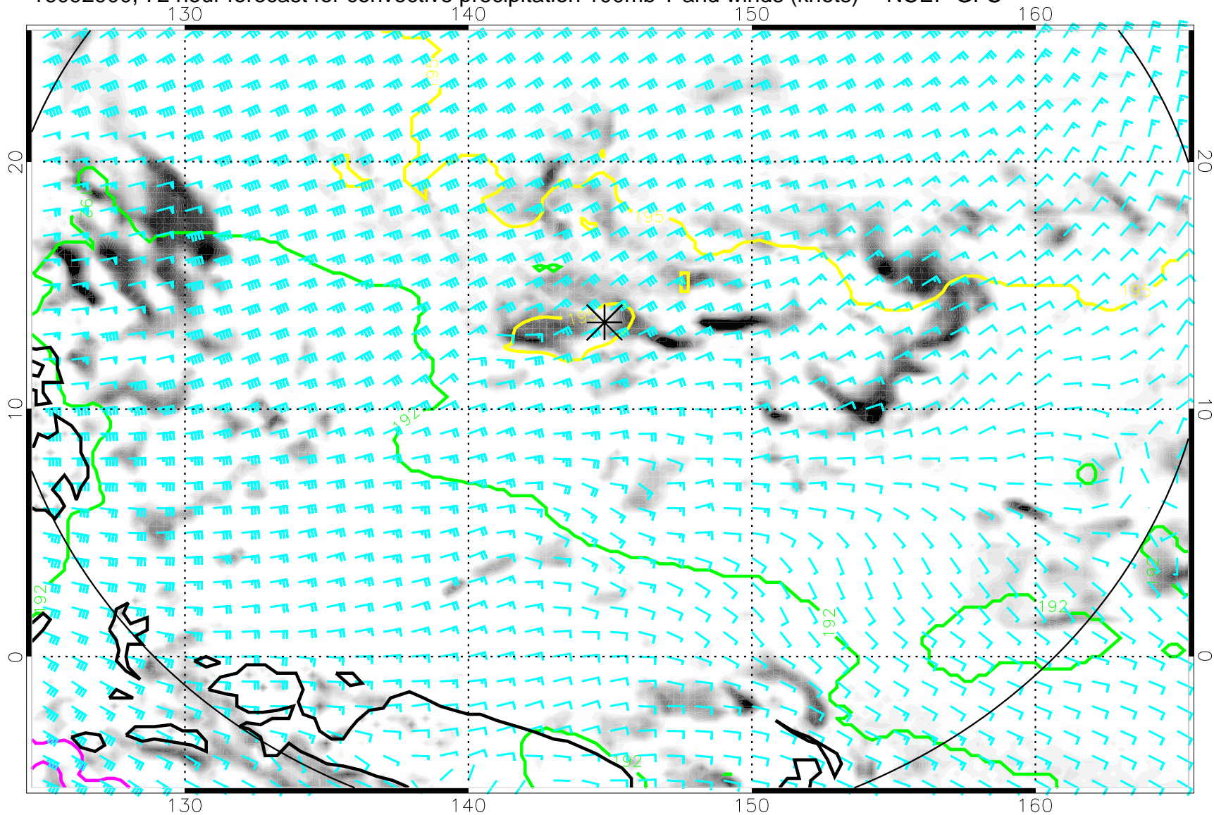
16092900, 72 hour forecast for convective precipitation 100mb T and winds (knots) -- NCEP GFS
