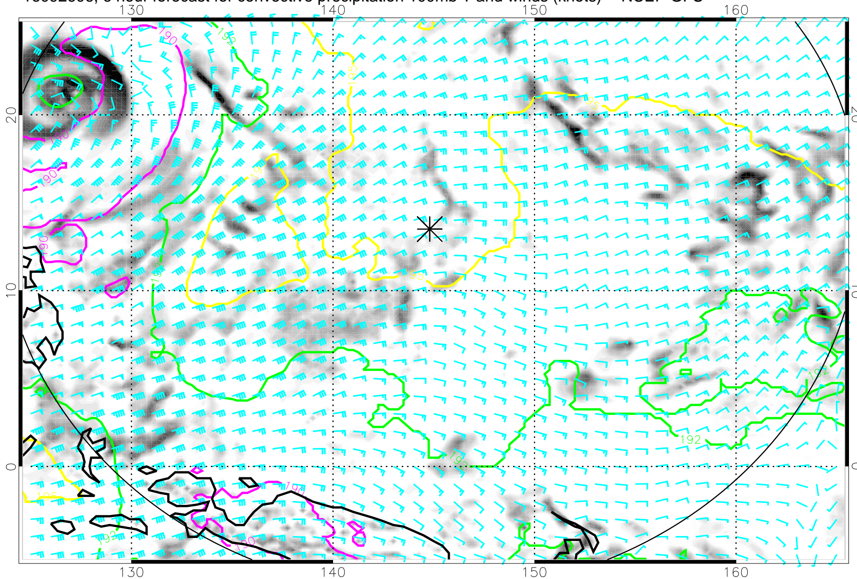
16092606, 6 hour forecast for convective precipitation 100mb T and winds (knots) -- NCEP GFS
