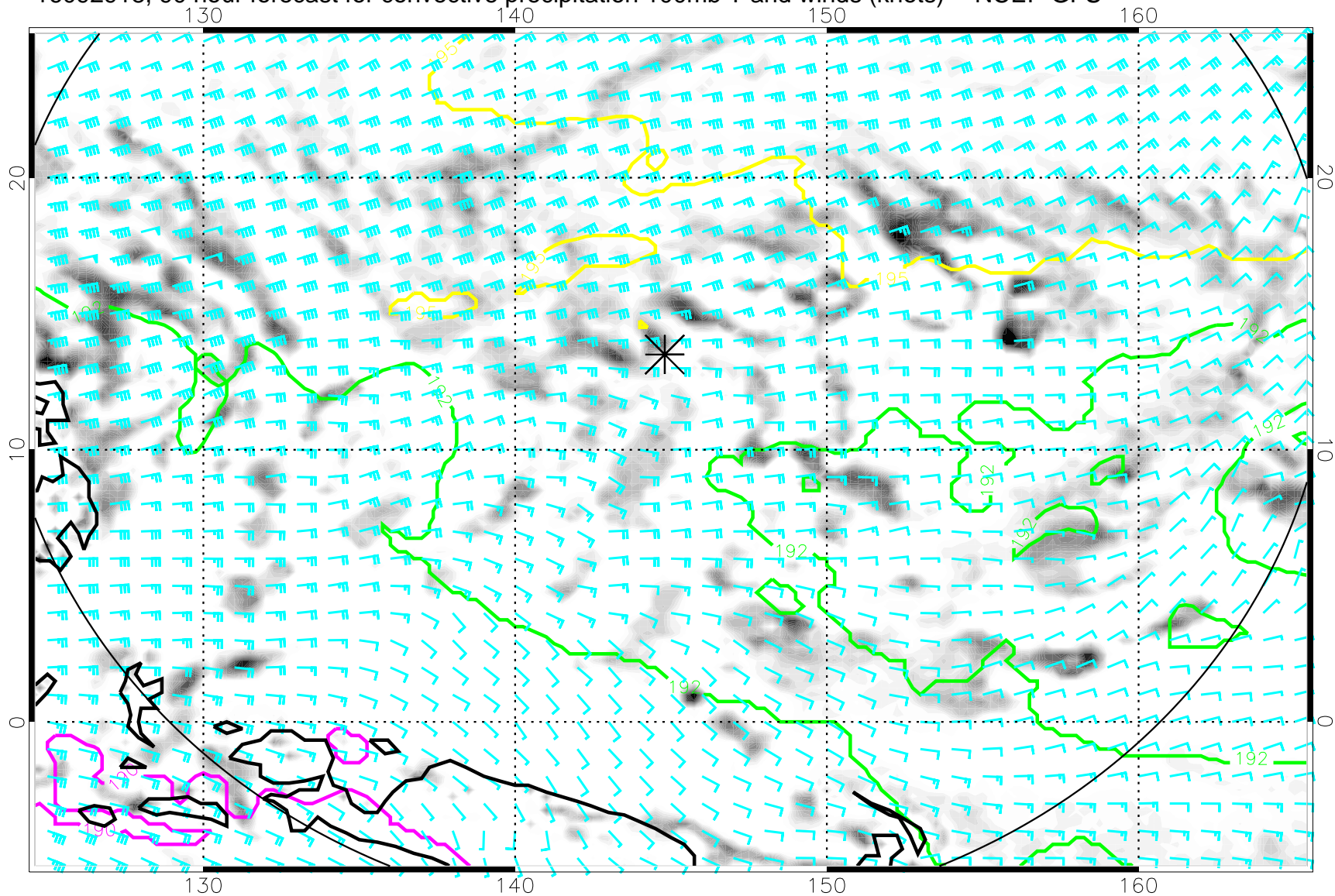
16092918, 90 hour forecast for convective precipitation 100mb T and winds (knots) -- NCEP GFS
