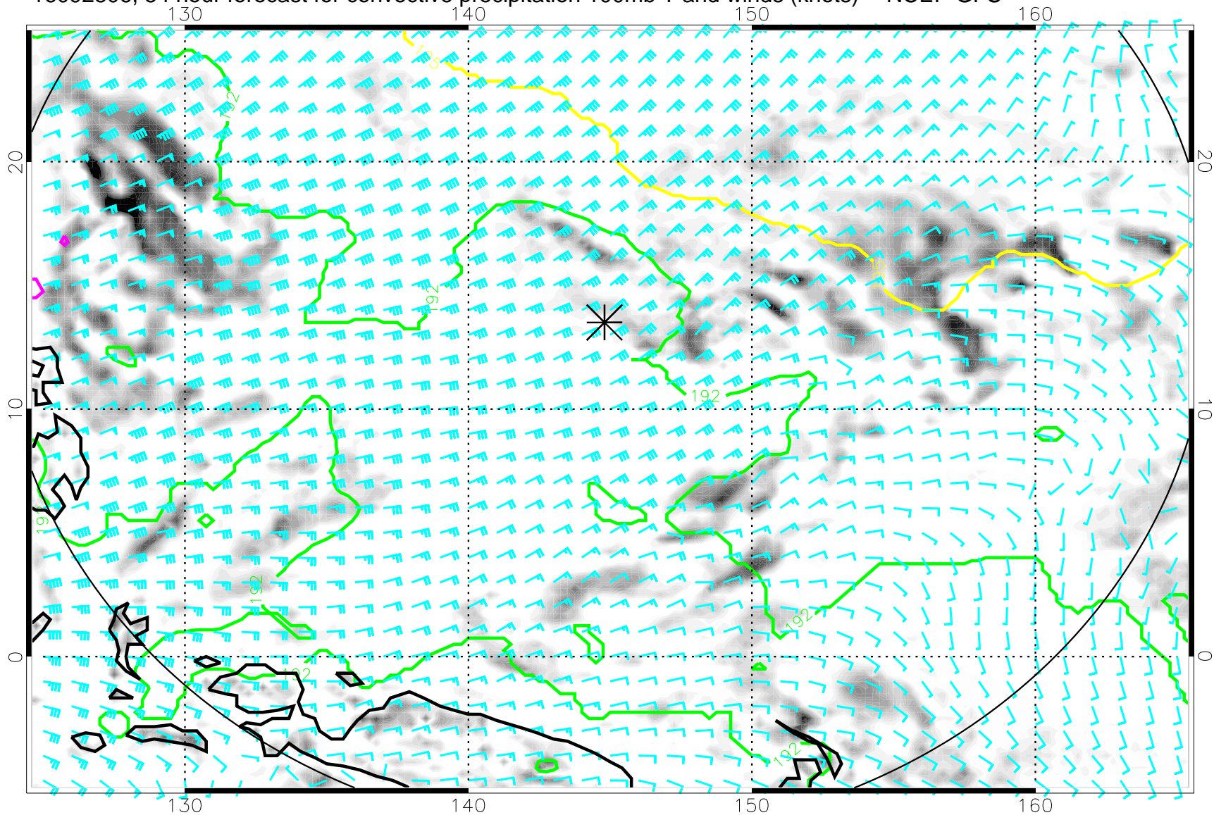
16092806, 54 hour forecast for convective precipitation 100mb T and winds (knots) -- NCEP GFS
