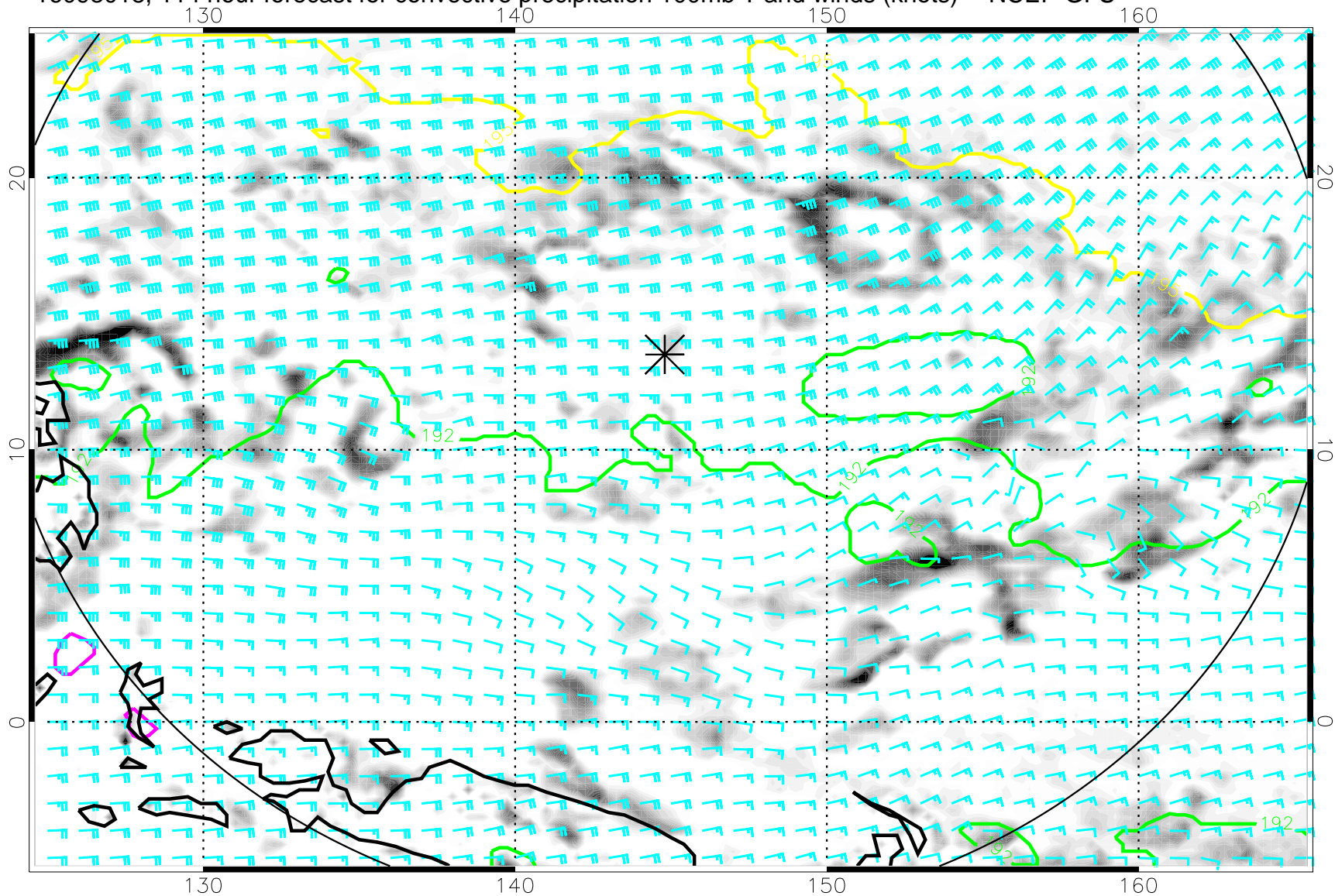
16093018, 114 hour forecast for convective precipitation 100mb T and winds (knots) -- NCEP GFS
