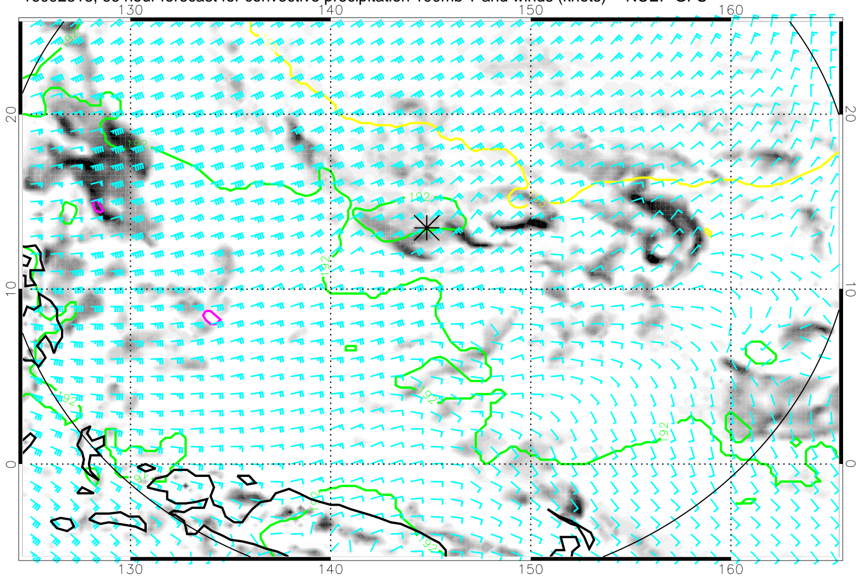
16092818, 66 hour forecast for convective precipitation 100mb T and winds (knots) -- NCEP GFS
