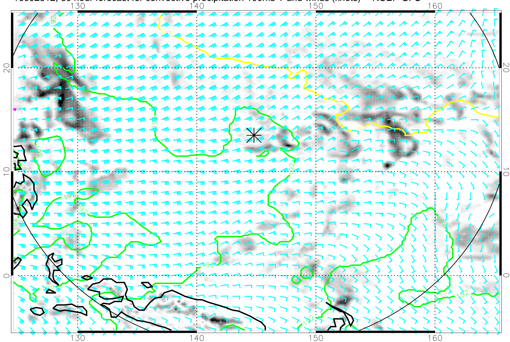
16092812, 60 hour forecast for convective precipitation 100mb T and winds (knots) -- NCEP GFS
