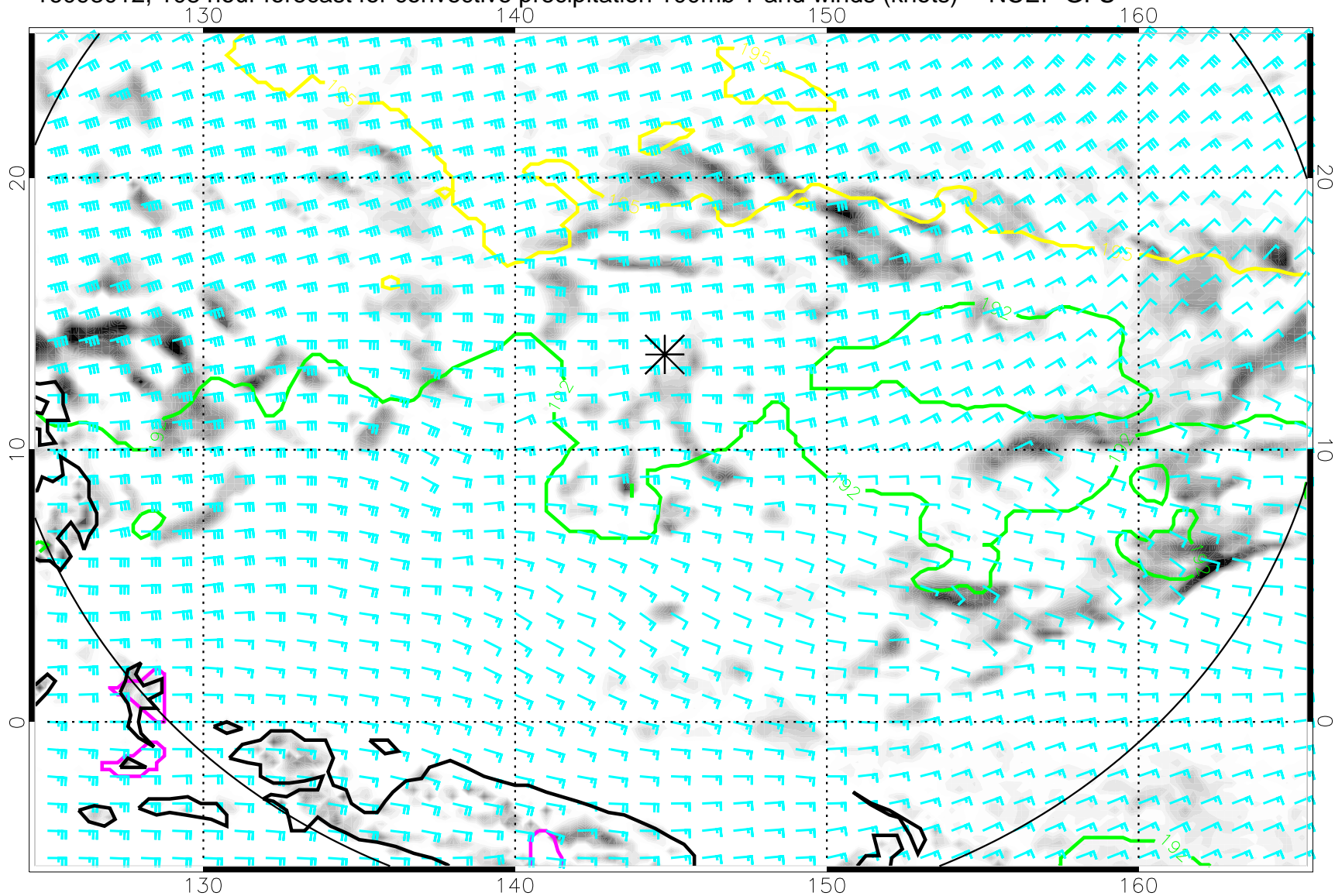
16093012, 108 hour forecast for convective precipitation 100mb T and winds (knots) -- NCEP GFS
