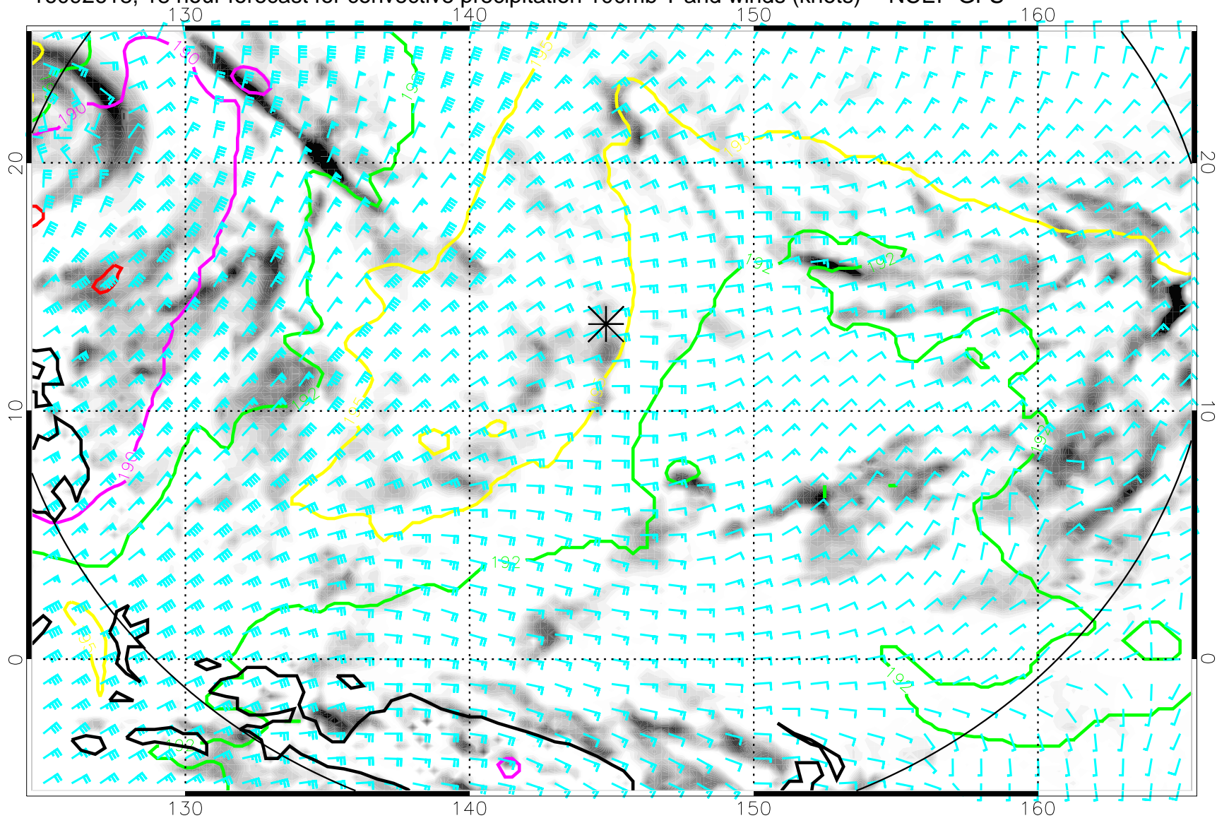
16092618, 18 hour forecast for convective precipitation 100mb T and winds (knots) -- NCEP GFS
