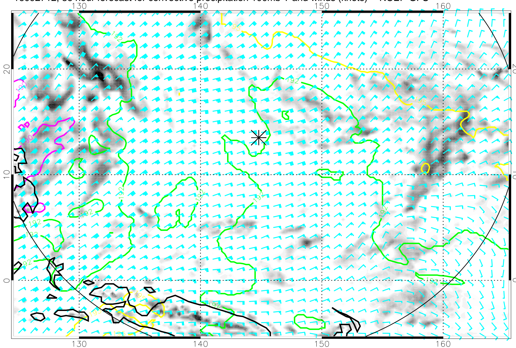
16092712, 36 hour forecast for convective precipitation 100mb T and winds (knots) -- NCEP GFS
