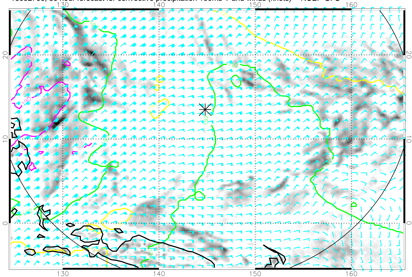
16092706, 30 hour forecast for convective precipitation 100mb T and winds (knots) -- NCEP GFS
