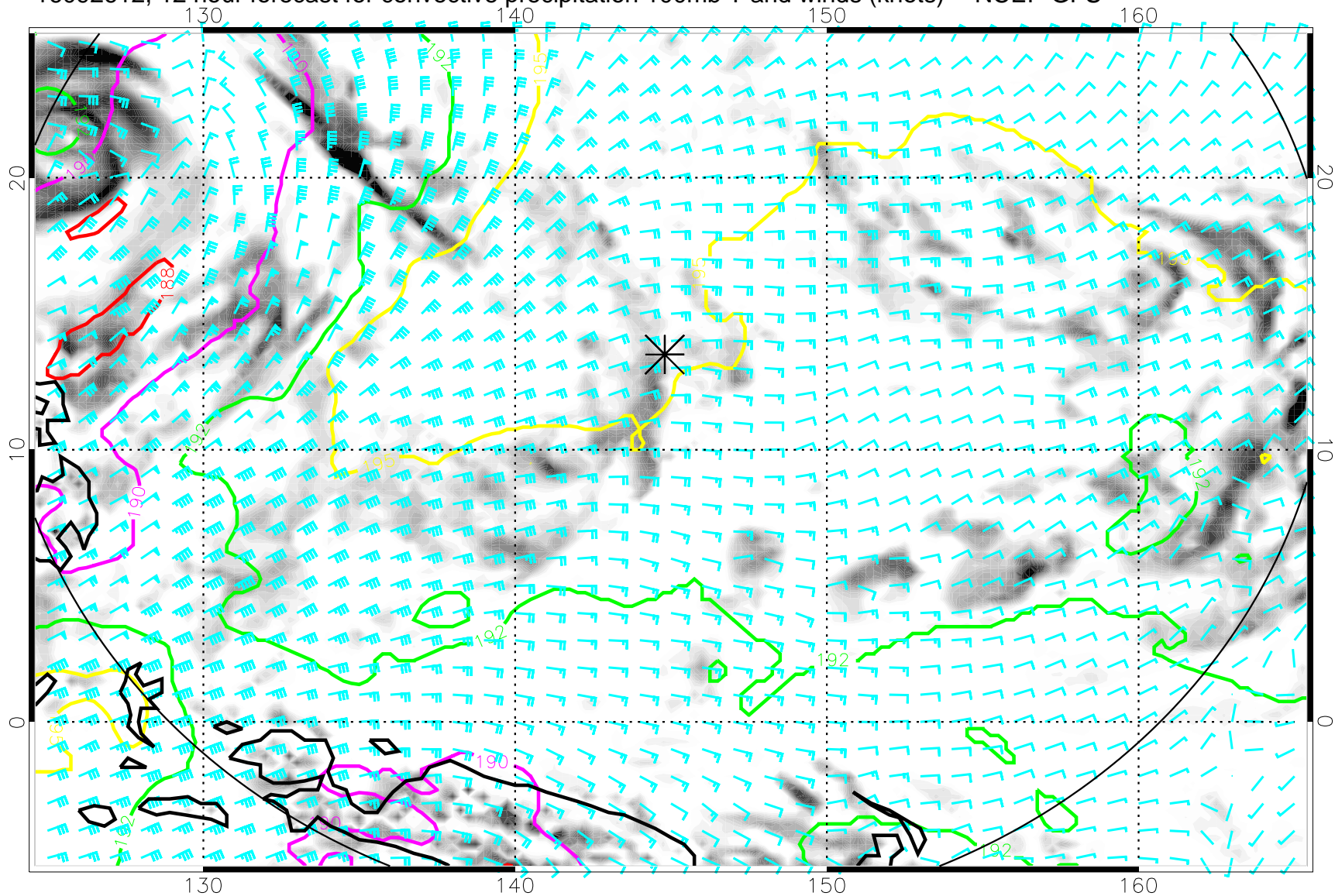
16092612, 12 hour forecast for convective precipitation 100mb T and winds (knots) -- NCEP GFS
