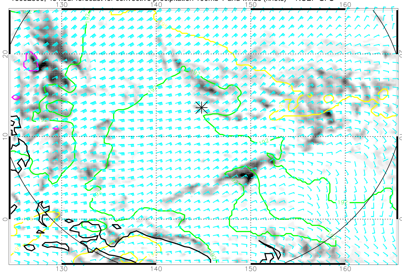
16092800, 48 hour forecast for convective precipitation 100mb T and winds (knots) -- NCEP GFS
