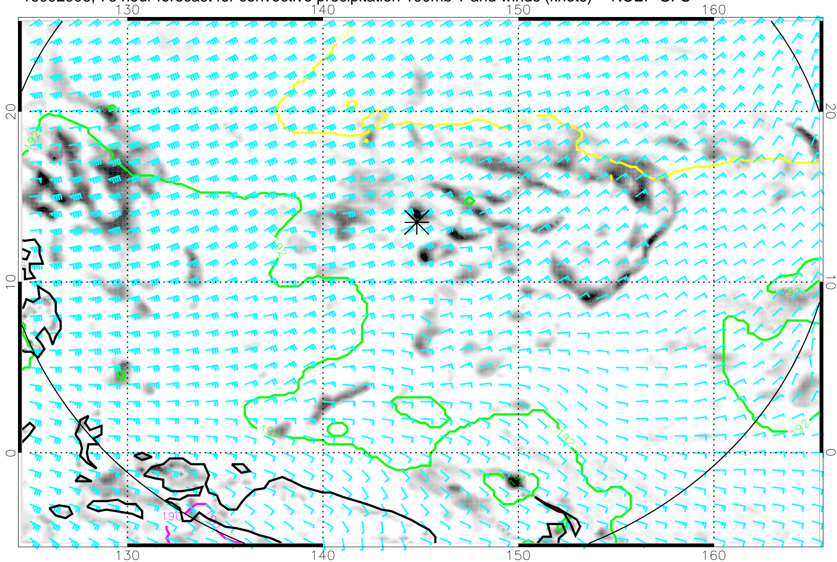
16092906, 78 hour forecast for convective precipitation 100mb T and winds (knots) -- NCEP GFS
