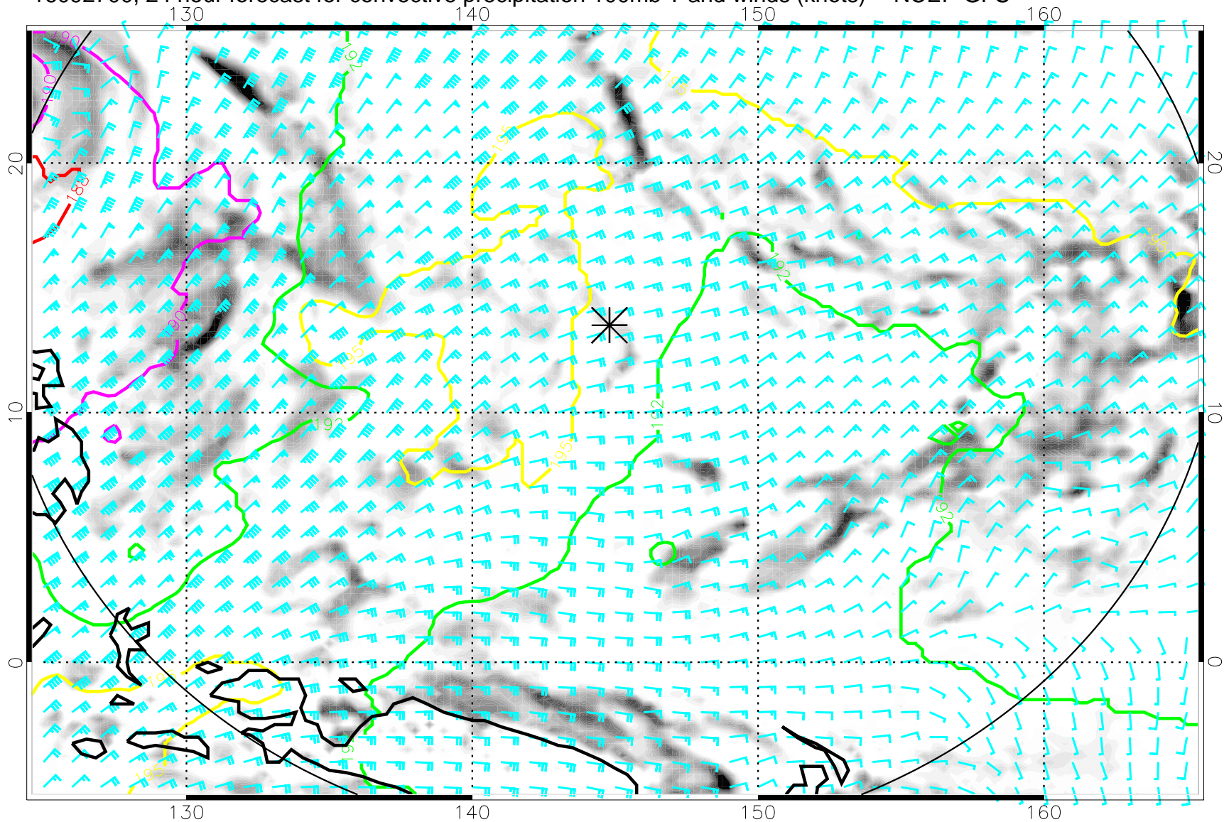
16092700, 24 hour forecast for convective precipitation 100mb T and winds (knots) -- NCEP GFS
