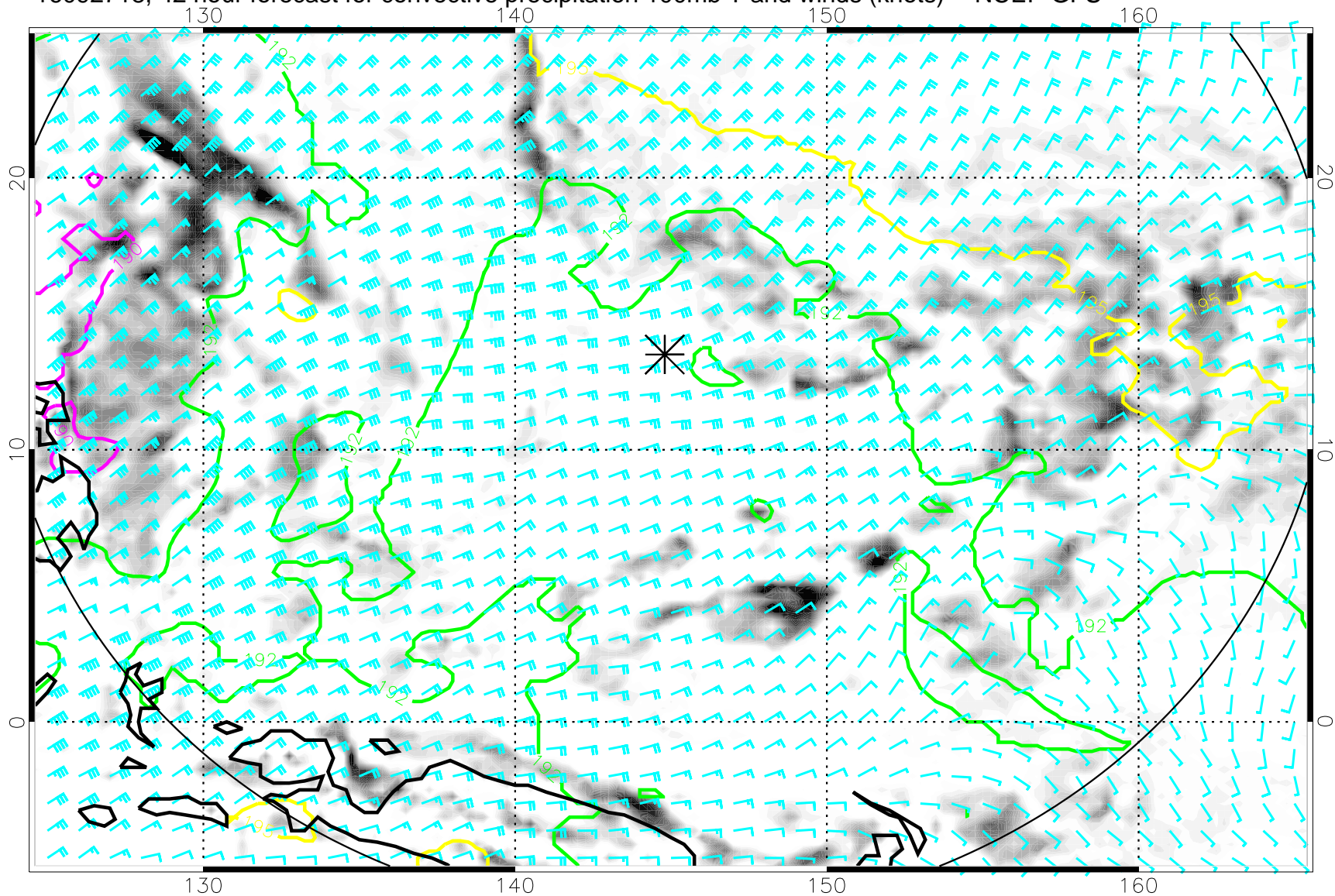
16092718, 42 hour forecast for convective precipitation 100mb T and winds (knots) -- NCEP GFS
