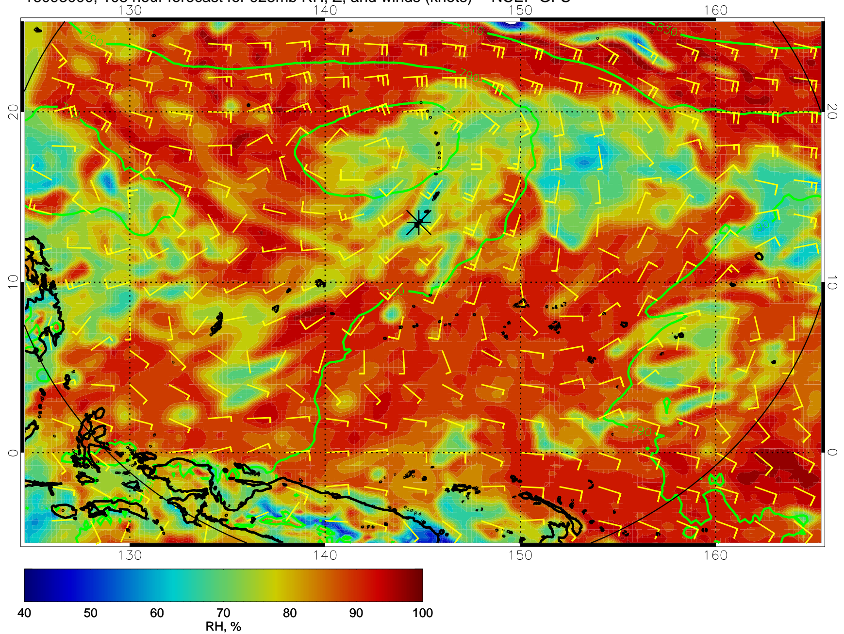
16093000, 108 hour forecast for 925mb RH, Z, and winds (knots) -- NCEP GFS
