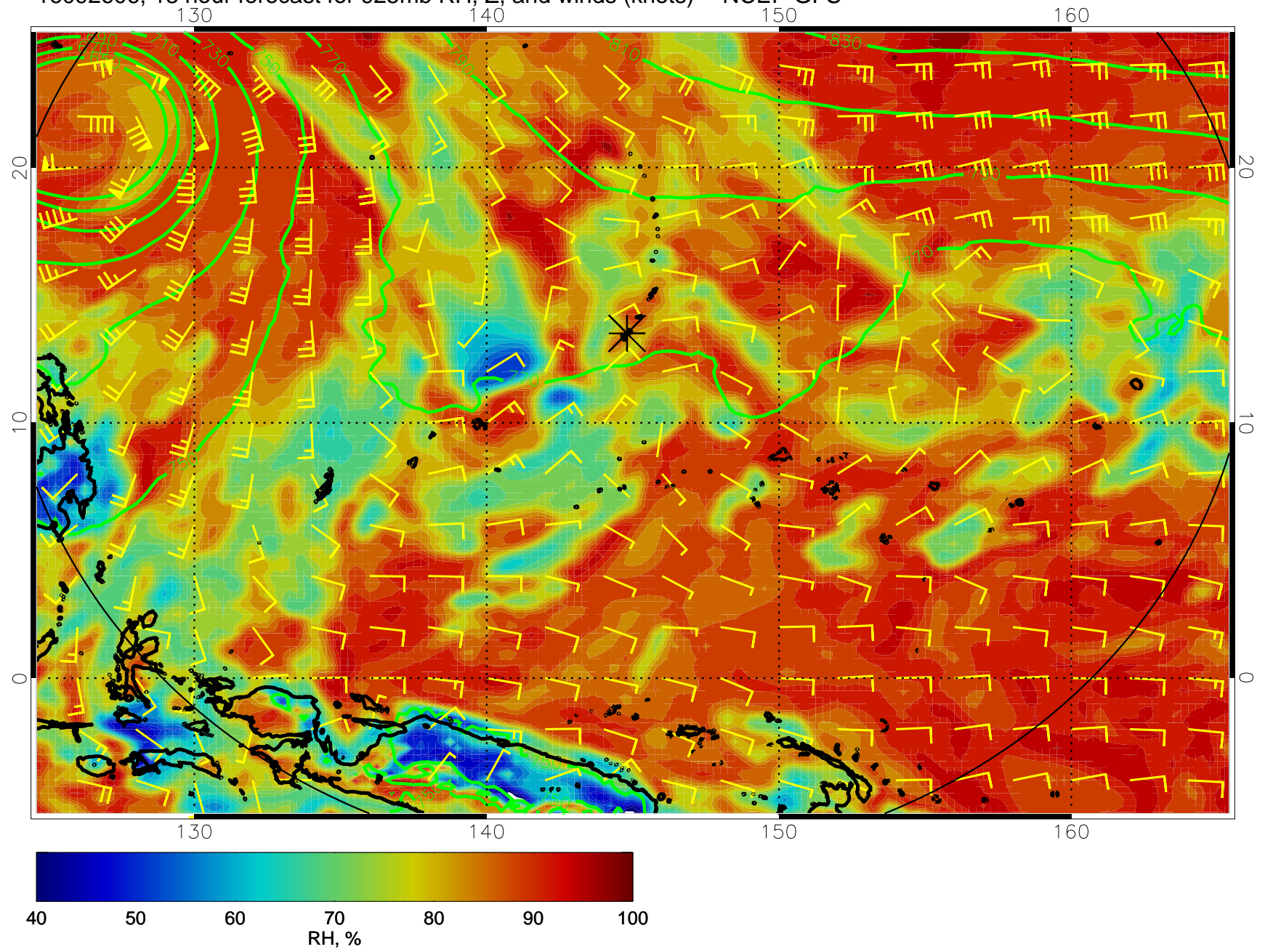
16092606, 18 hour forecast for 925mb RH, Z, and winds (knots) -- NCEP GFS
