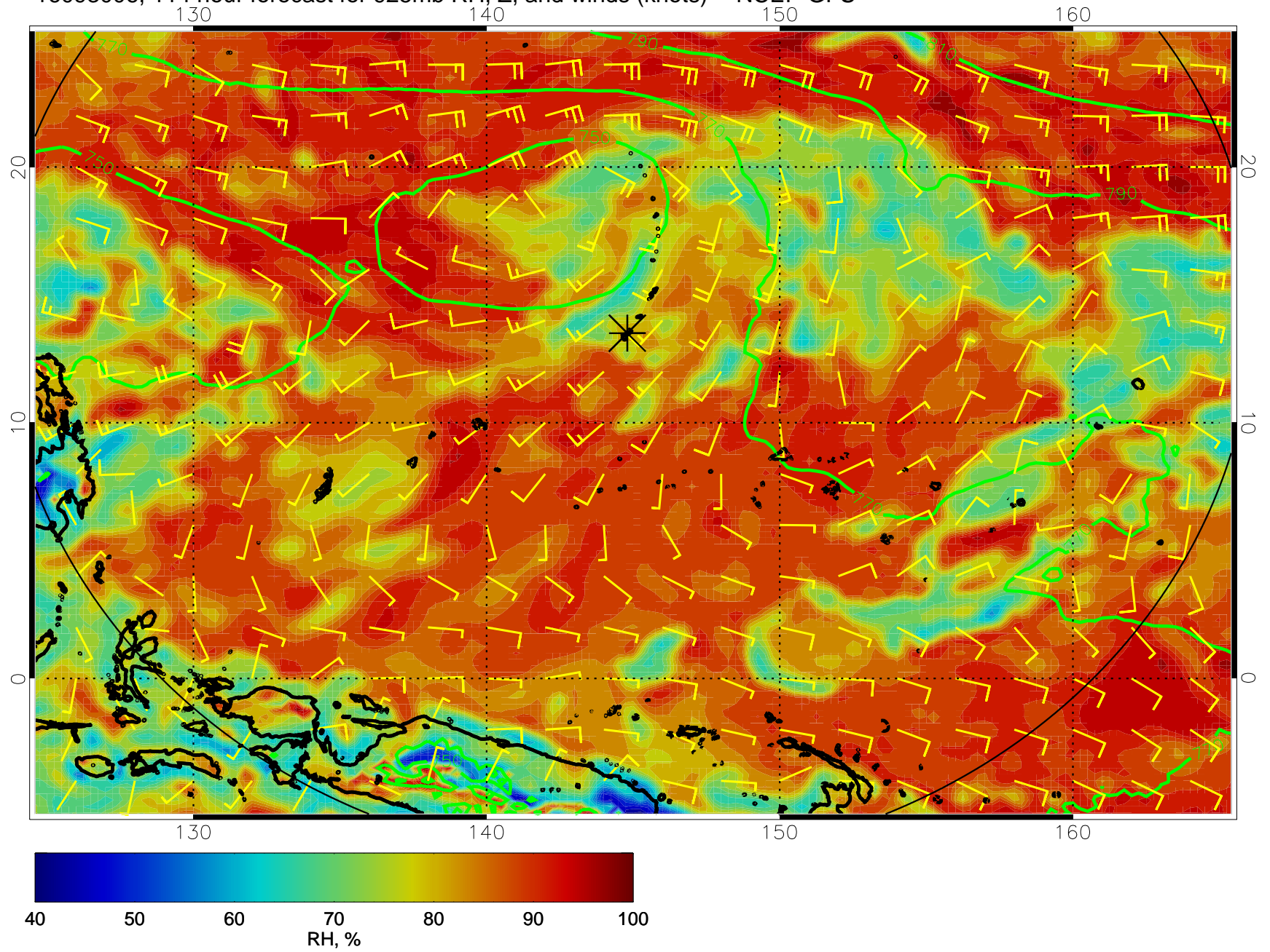
16093006, 114 hour forecast for 925mb RH, Z, and winds (knots) -- NCEP GFS
