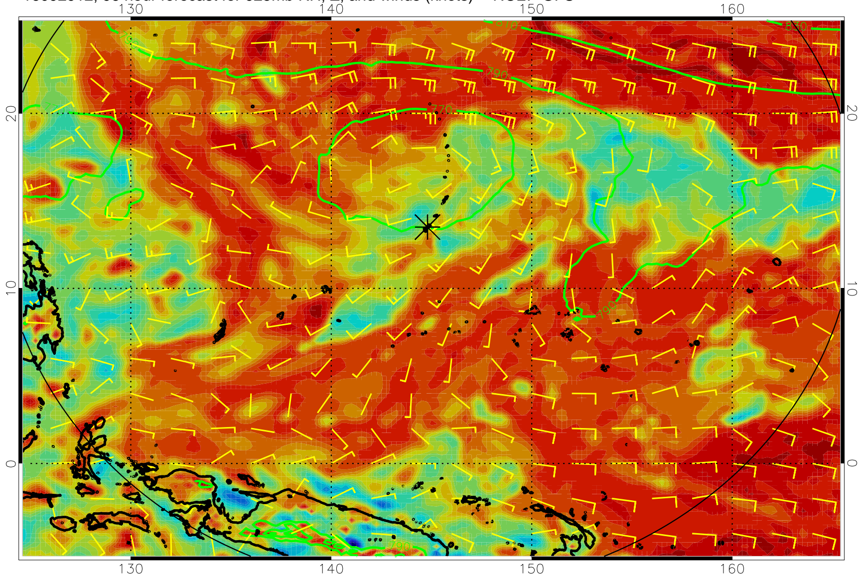
16092912, 96 hour forecast for 925mb RH, Z, and winds (knots) -- NCEP GFS
