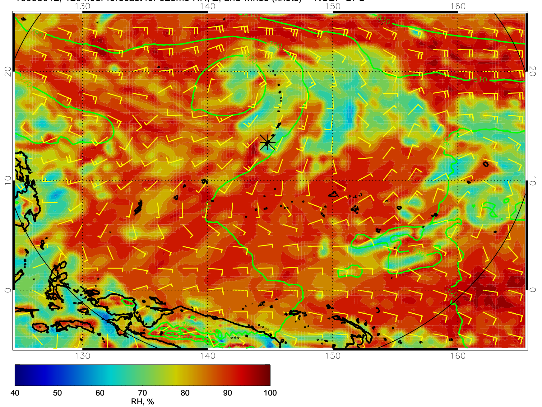
16093012, 120 hour forecast for 925mb RH, Z, and winds (knots) -- NCEP GFS
