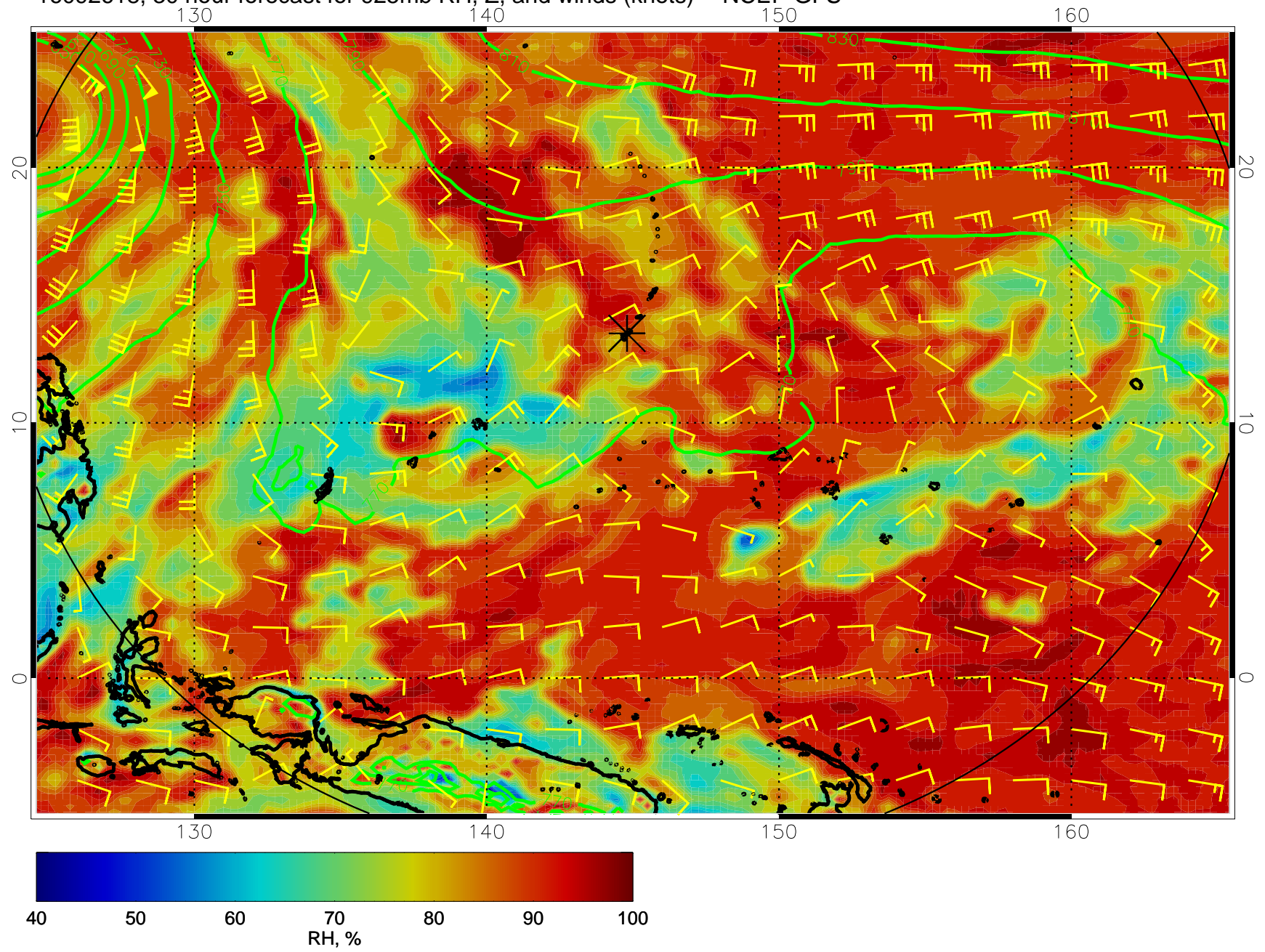
16092618, 30 hour forecast for 925mb RH, Z, and winds (knots) -- NCEP GFS
