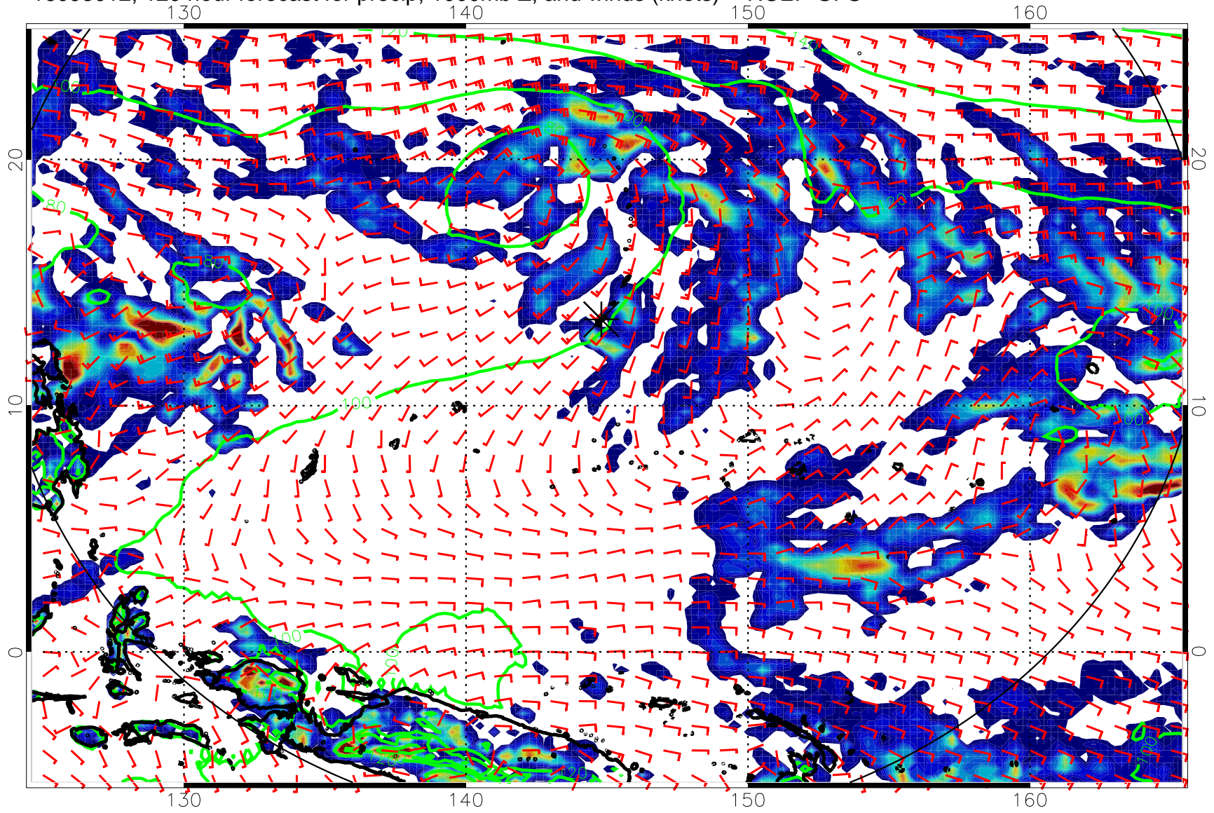
16093012, 120 hour forecast for precip, 1000mb Z, and winds (knots) -- NCEP GFS
