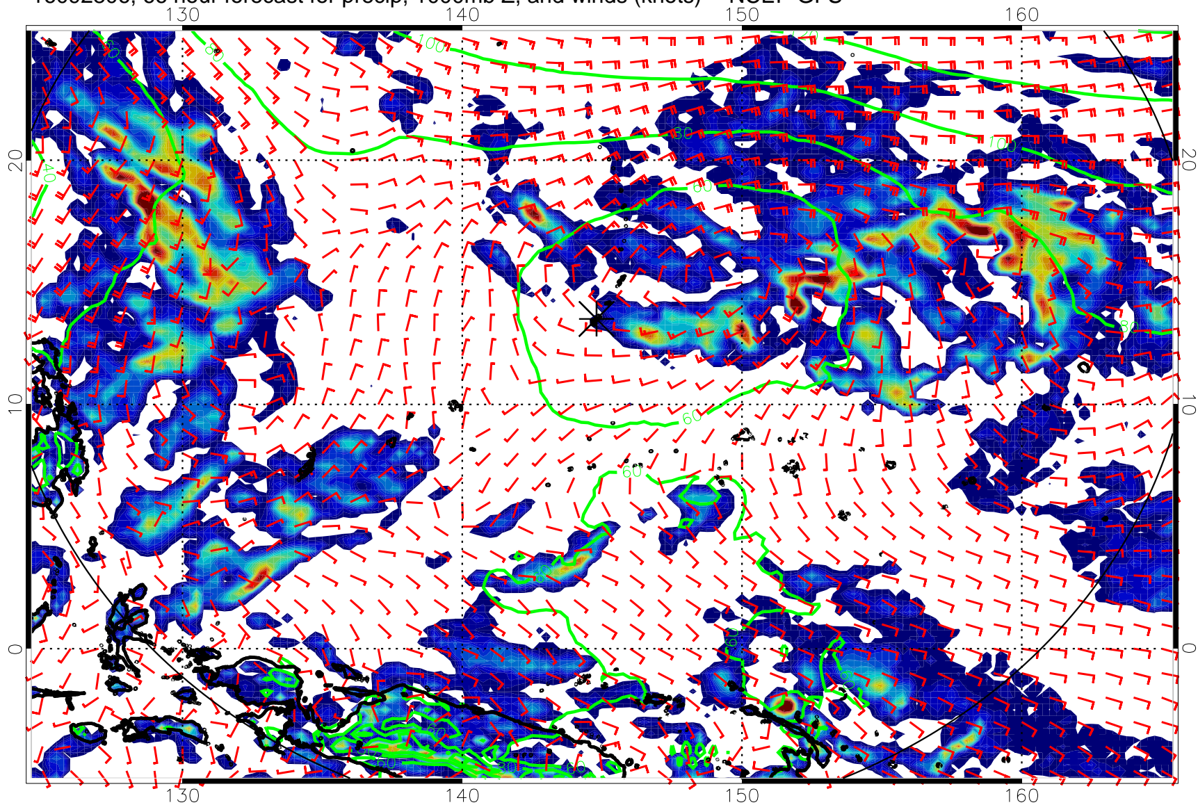
16092806, 66 hour forecast for precip, 1000mb Z, and winds (knots) -- NCEP GFS
