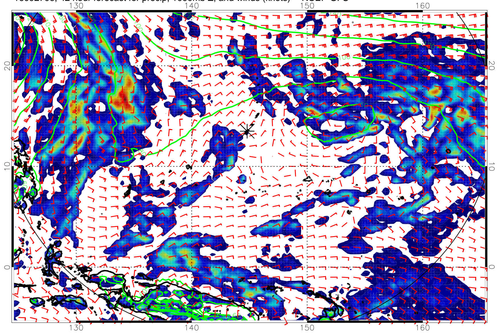
16092706, 42 hour forecast for precip, 1000mb Z, and winds (knots) -- NCEP GFS
