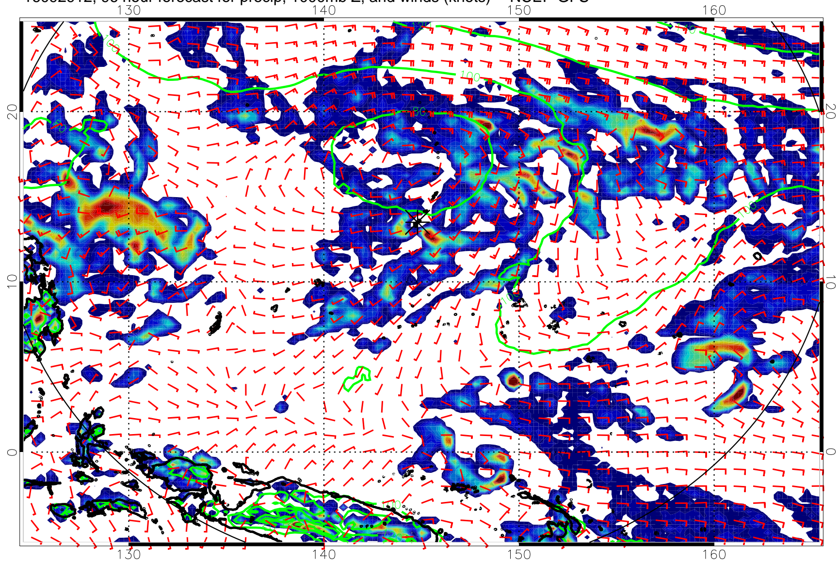
16092912, 96 hour forecast for precip, 1000mb Z, and winds (knots) -- NCEP GFS
