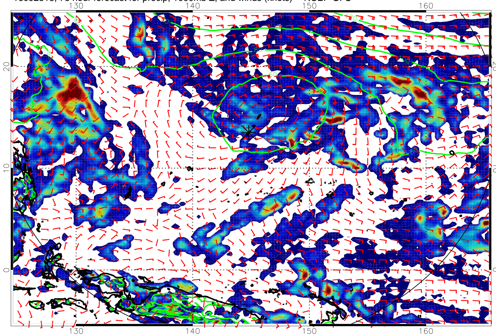
16092818, 78 hour forecast for precip, 1000mb Z, and winds (knots) -- NCEP GFS
