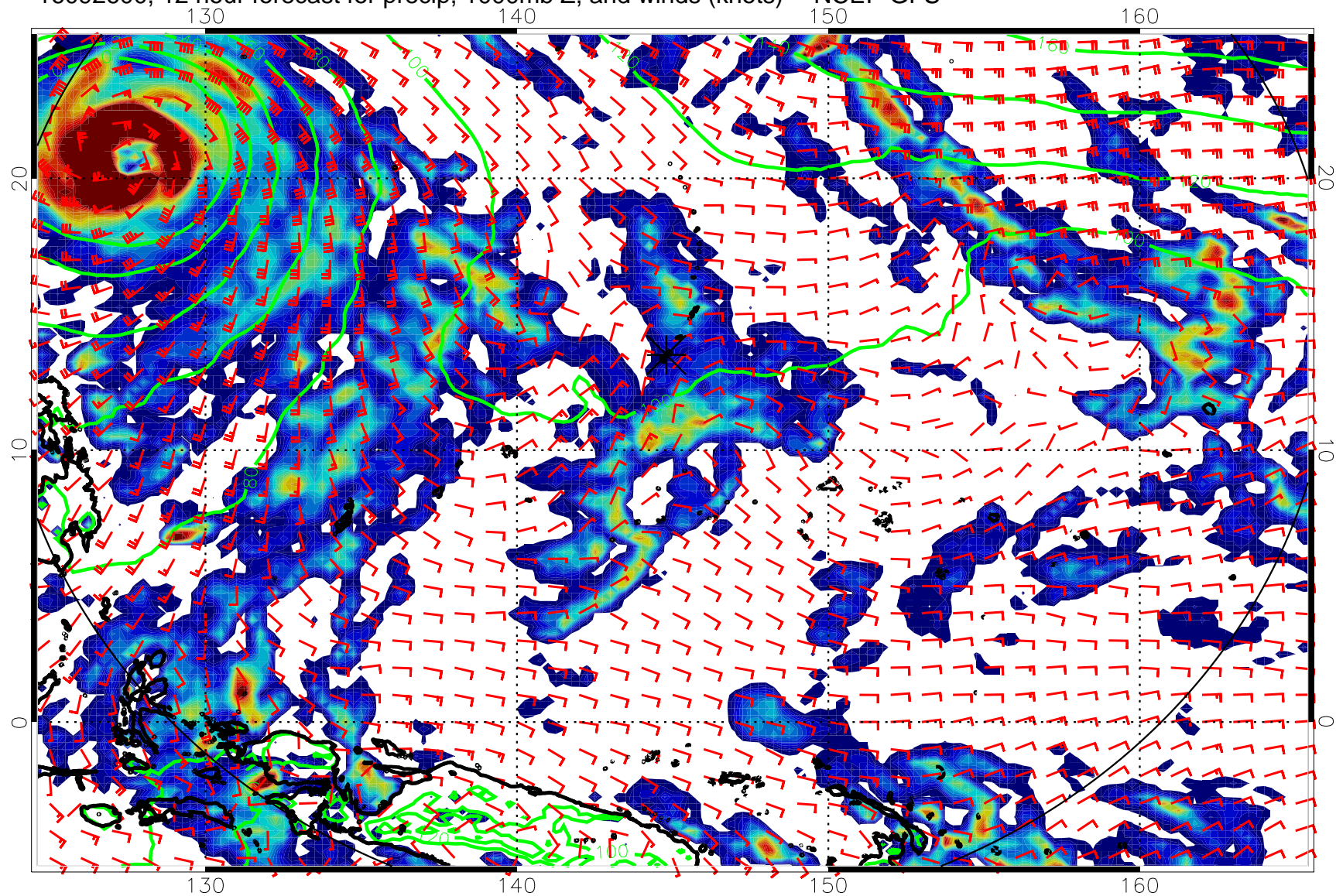
16092600, 12 hour forecast for precip, 1000mb Z, and winds (knots) -- NCEP GFS
