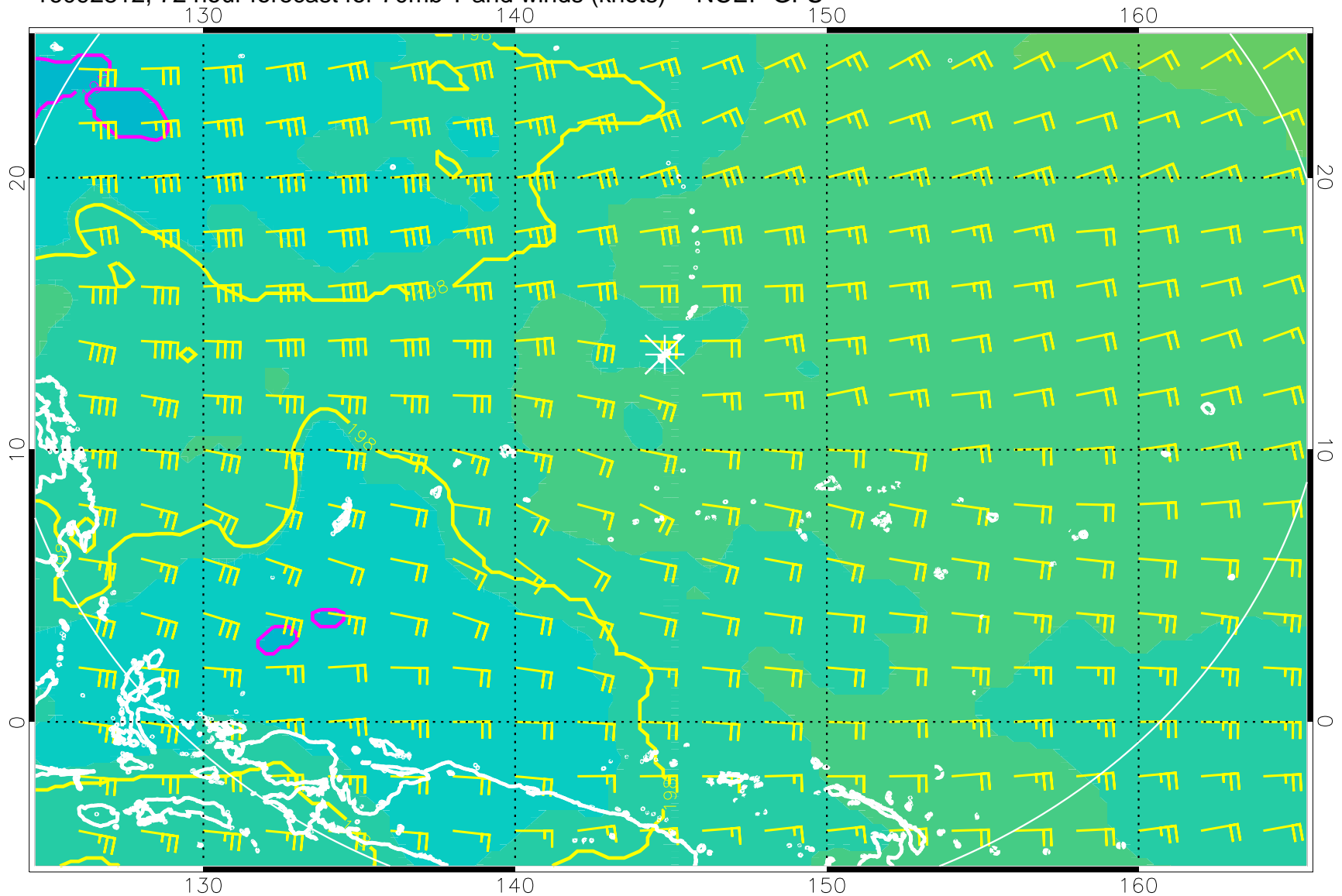
16092812, 72 hour forecast for 70mb T and winds (knots) -- NCEP GFS
