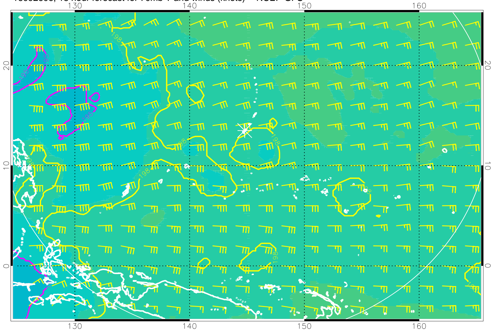
16092606, 18 hour forecast for 70mb T and winds (knots) -- NCEP GFS
