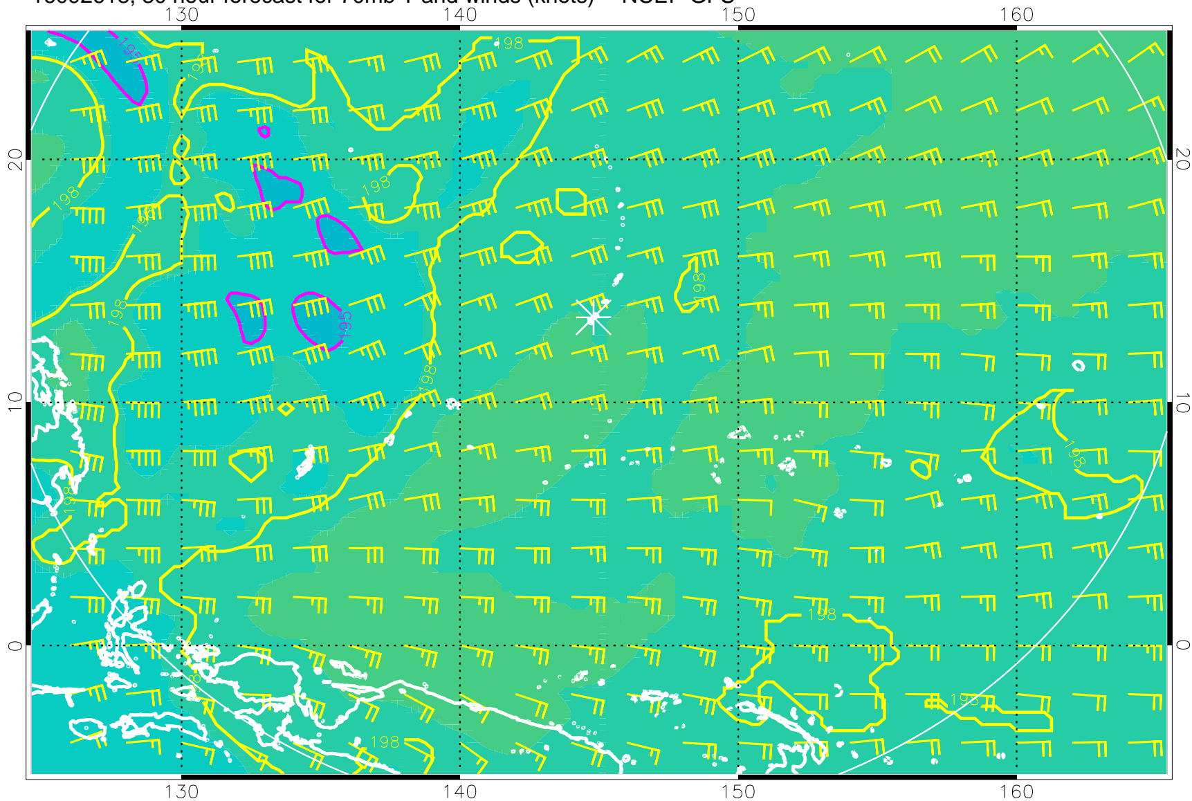
16092618, 30 hour forecast for 70mb T and winds (knots) -- NCEP GFS
