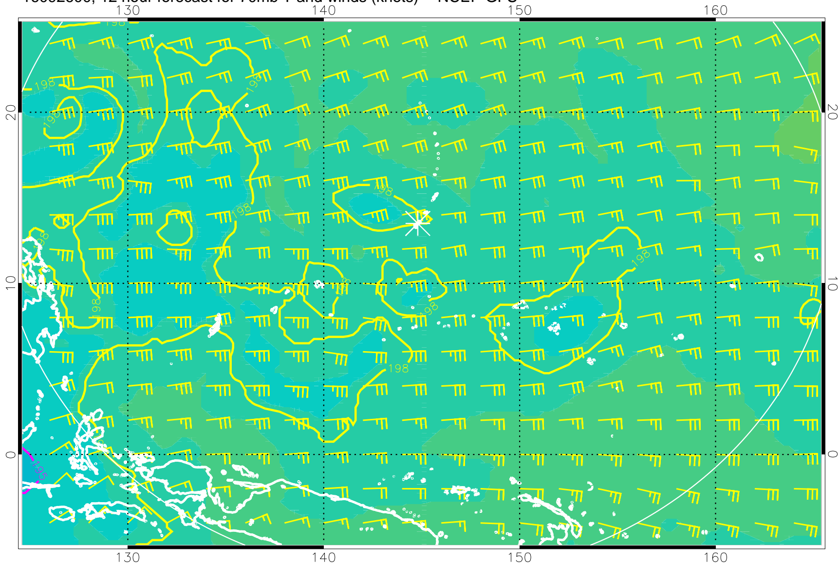
16092600, 12 hour forecast for 70mb T and winds (knots) -- NCEP GFS
