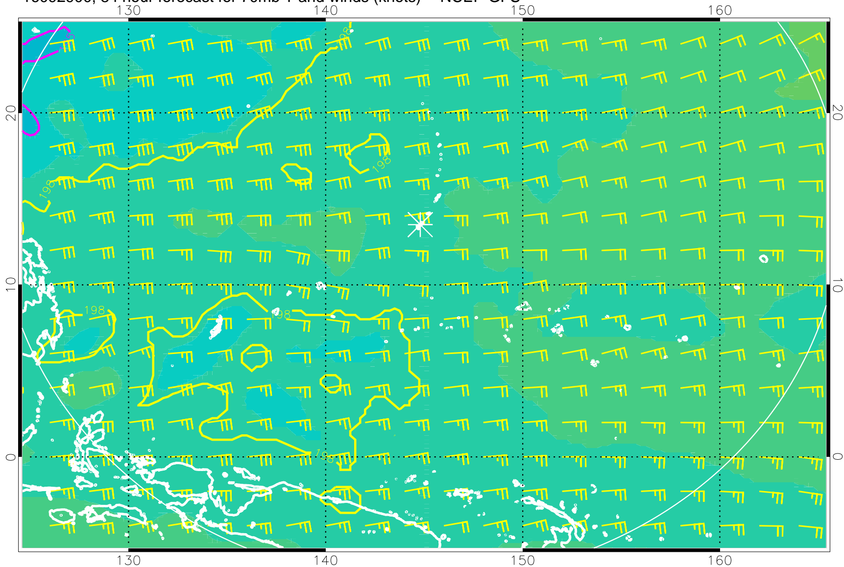
16092900, 84 hour forecast for 70mb T and winds (knots) -- NCEP GFS
