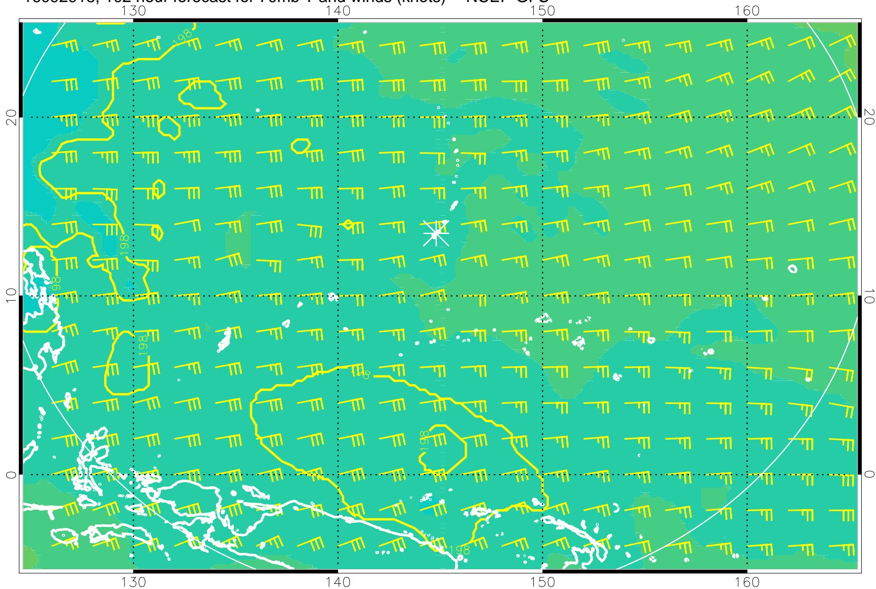
16092918, 102 hour forecast for 70mb T and winds (knots) -- NCEP GFS
