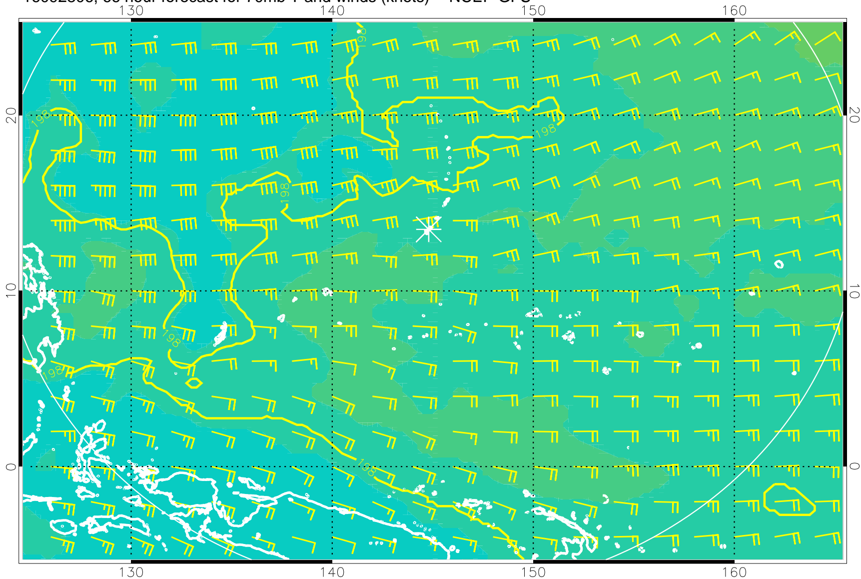
16092806, 66 hour forecast for 70mb T and winds (knots) -- NCEP GFS
