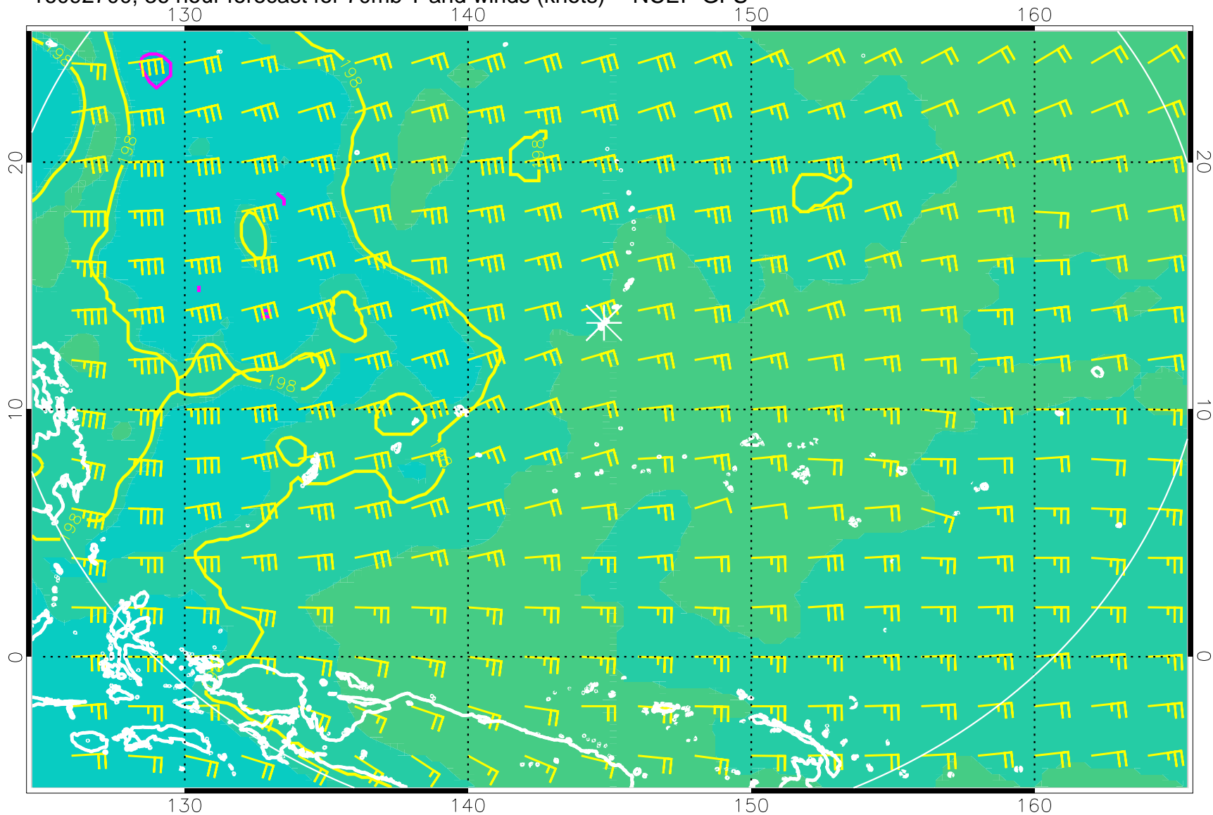
16092700, 36 hour forecast for 70mb T and winds (knots) -- NCEP GFS
