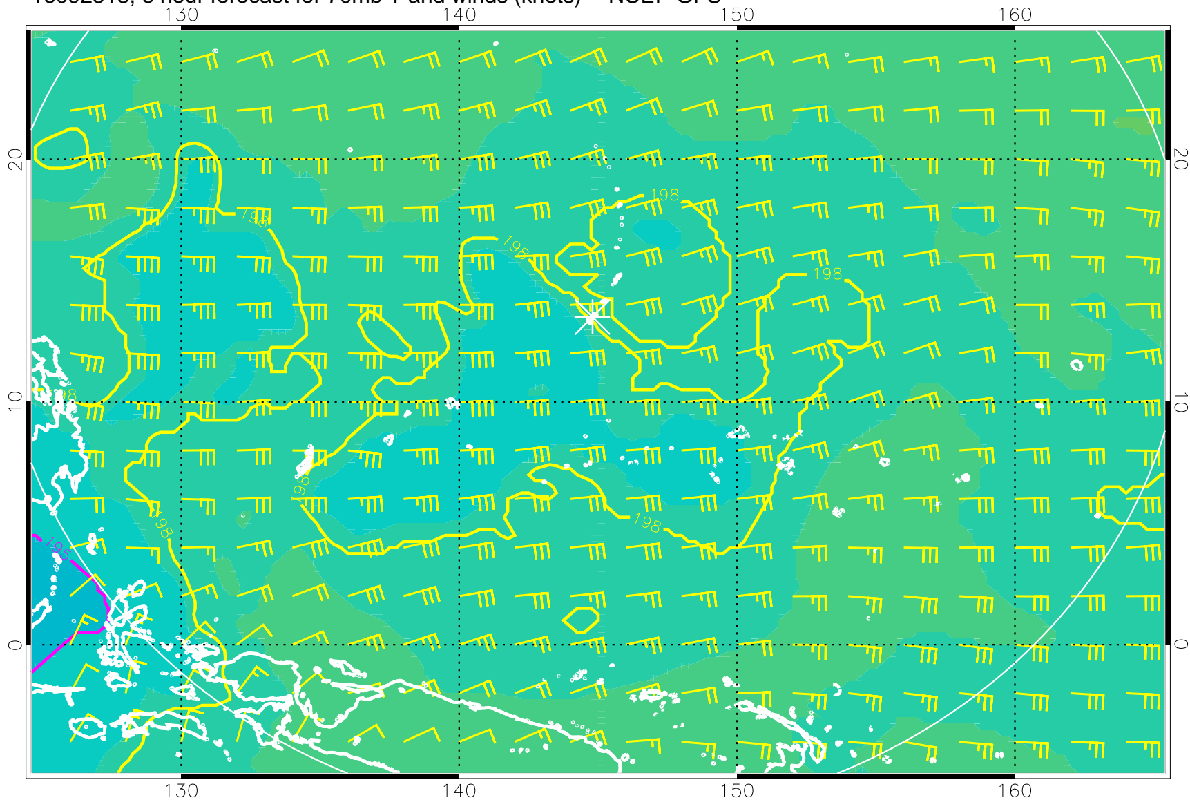
16092518, 6 hour forecast for 70mb T and winds (knots) -- NCEP GFS
