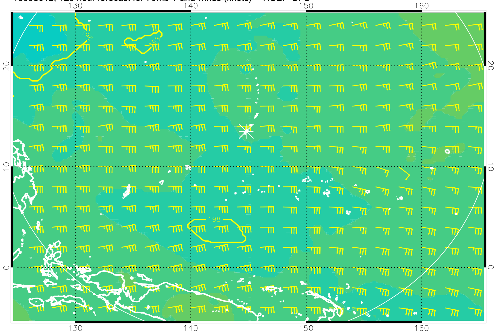
16093012, 120 hour forecast for 70mb T and winds (knots) -- NCEP GFS
