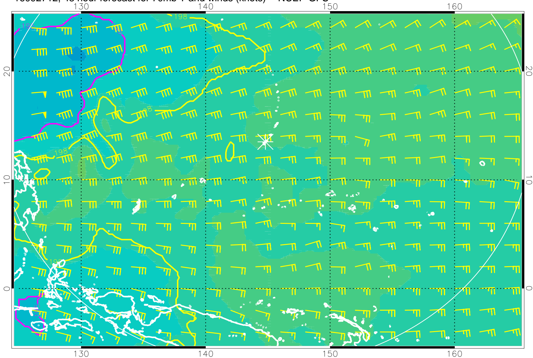
16092712, 48 hour forecast for 70mb T and winds (knots) -- NCEP GFS
