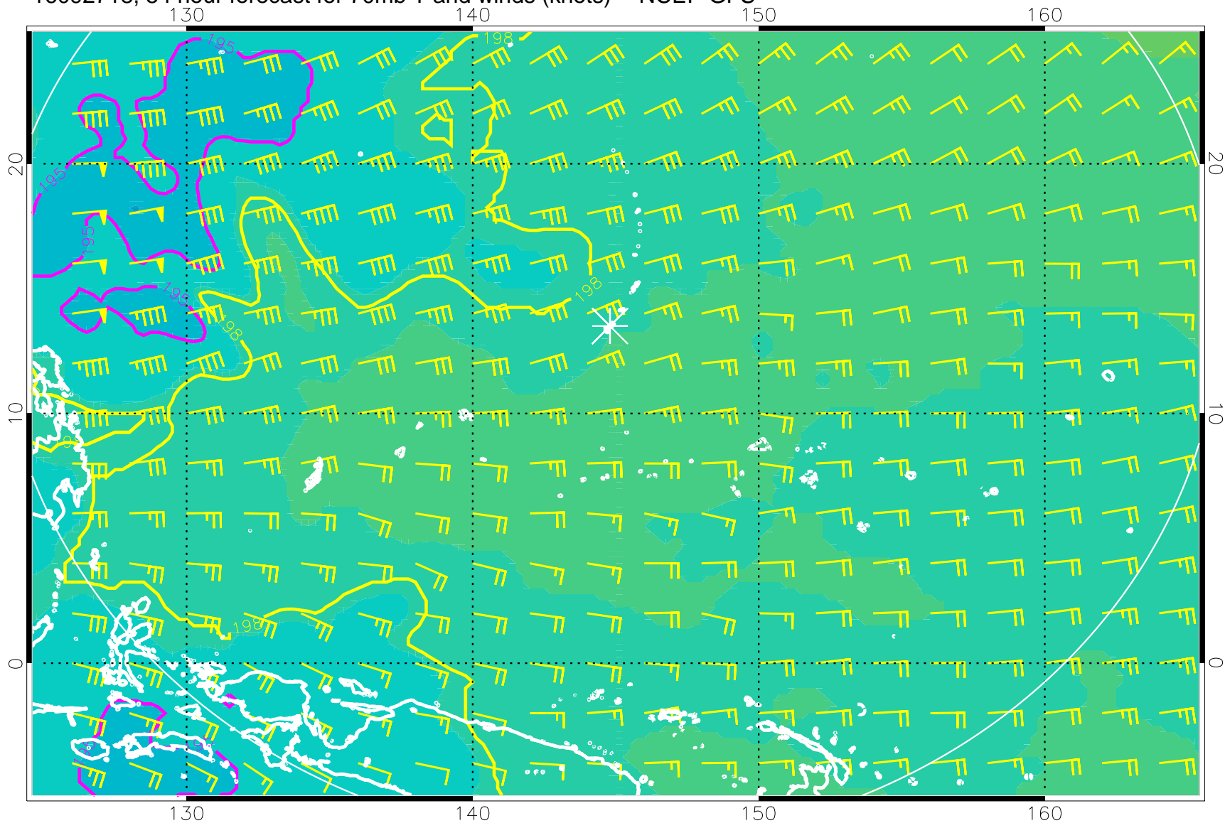
16092718, 54 hour forecast for 70mb T and winds (knots) -- NCEP GFS
