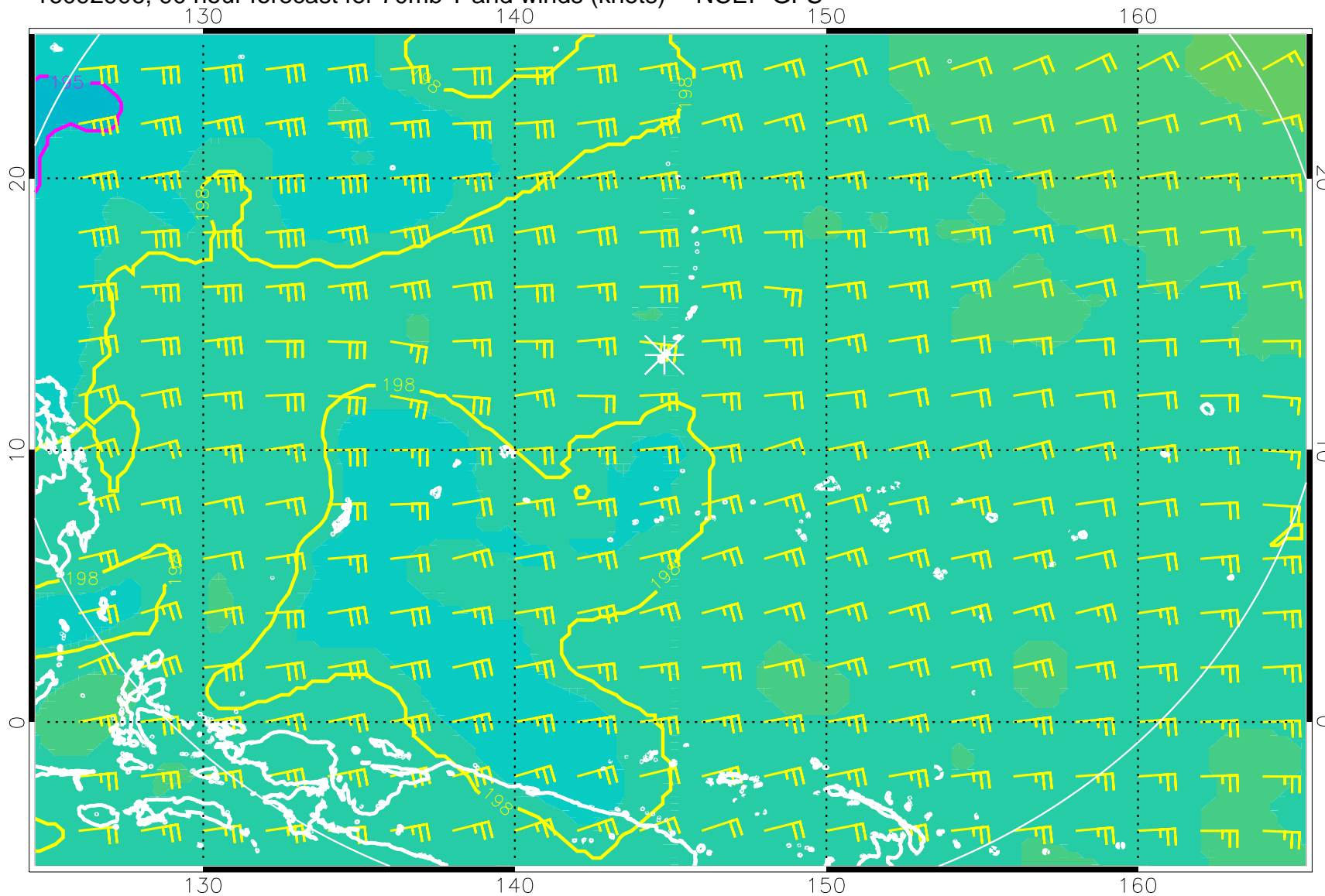
16092906, 90 hour forecast for 70mb T and winds (knots) -- NCEP GFS
