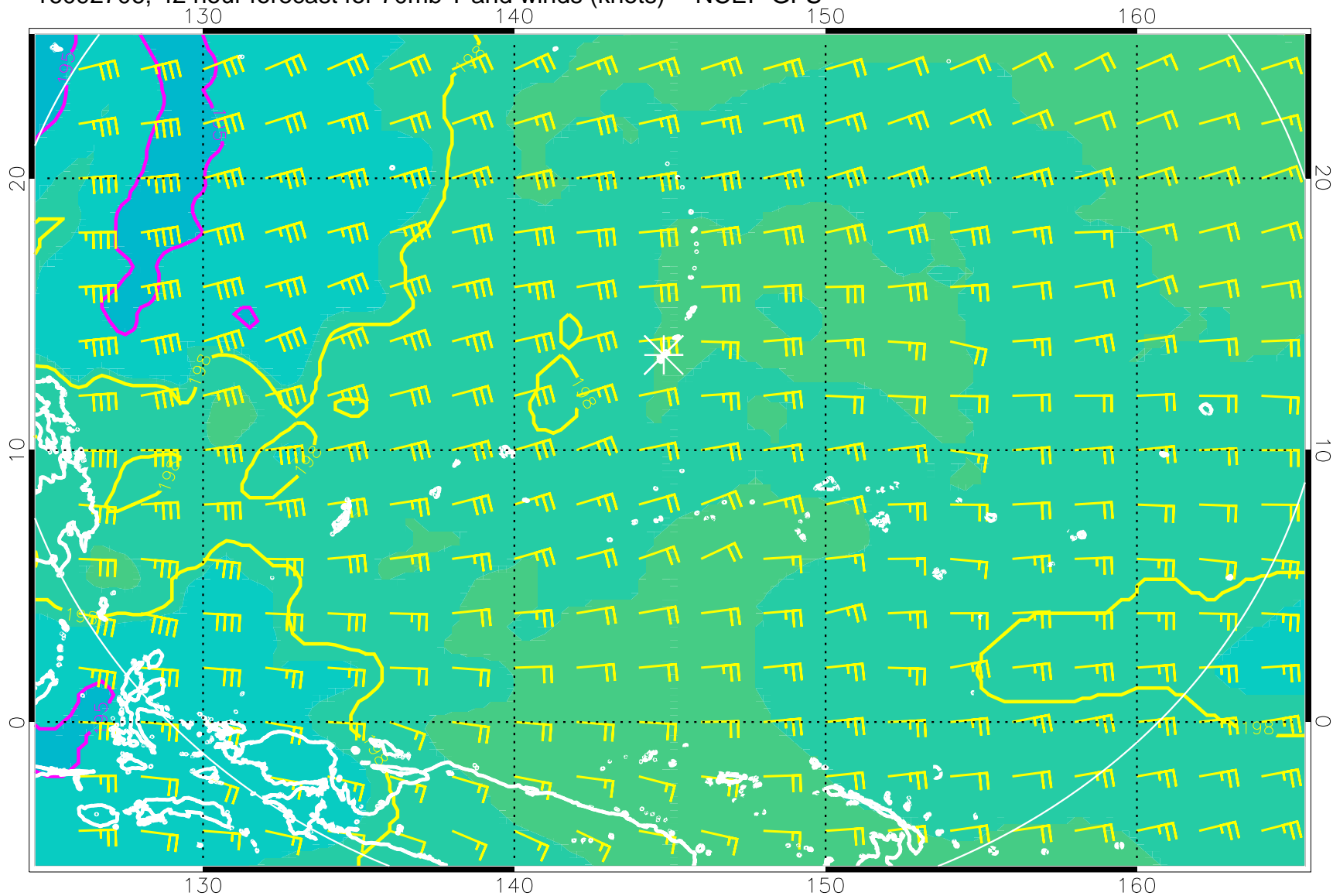
16092706, 42 hour forecast for 70mb T and winds (knots) -- NCEP GFS
