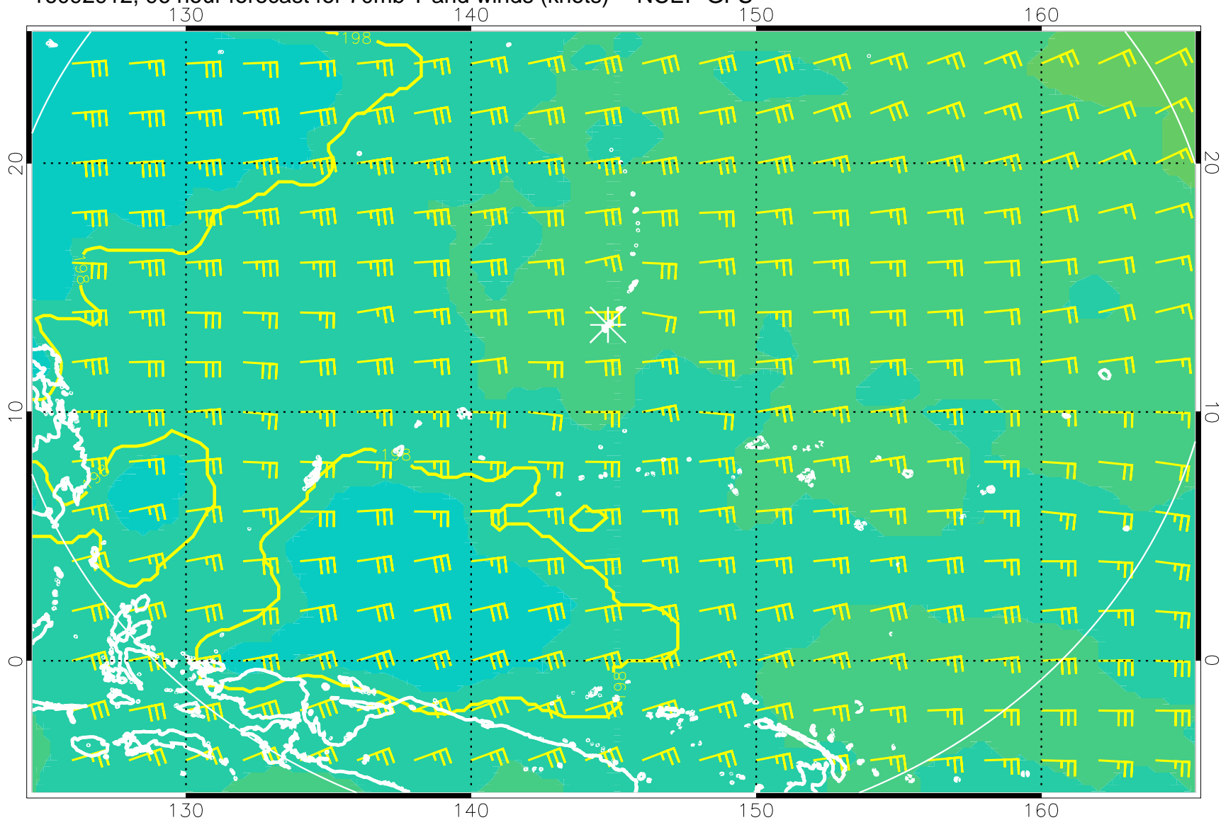
16092912, 96 hour forecast for 70mb T and winds (knots) -- NCEP GFS
