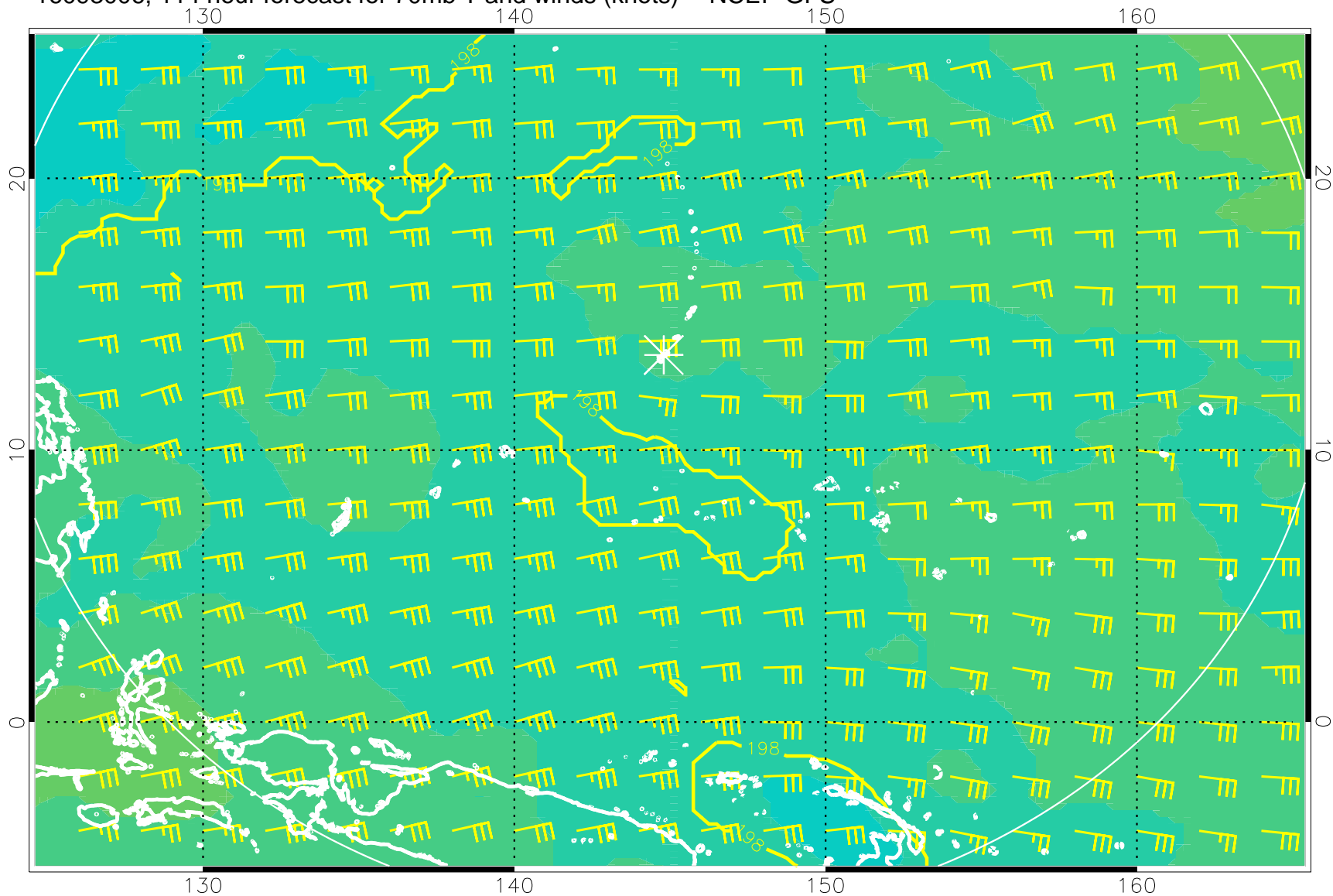
16093006, 114 hour forecast for 70mb T and winds (knots) -- NCEP GFS
