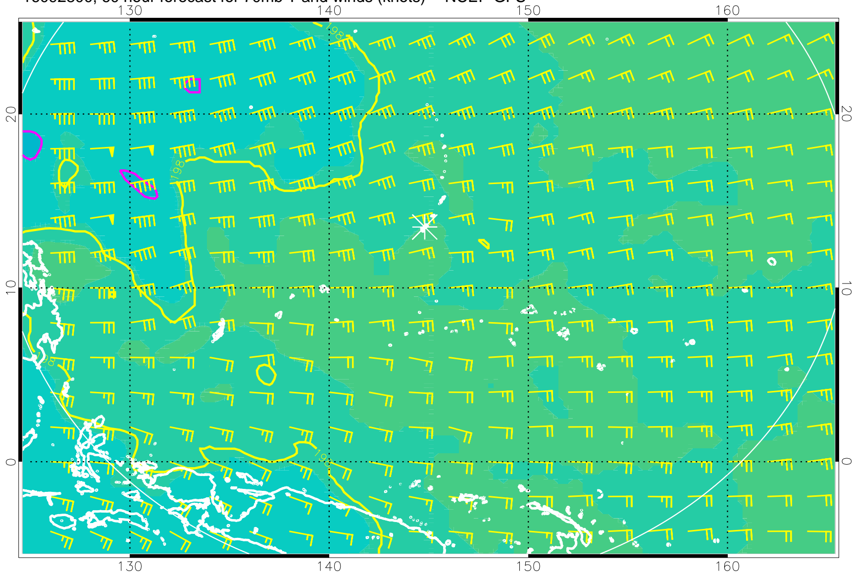
16092800, 60 hour forecast for 70mb T and winds (knots) -- NCEP GFS
