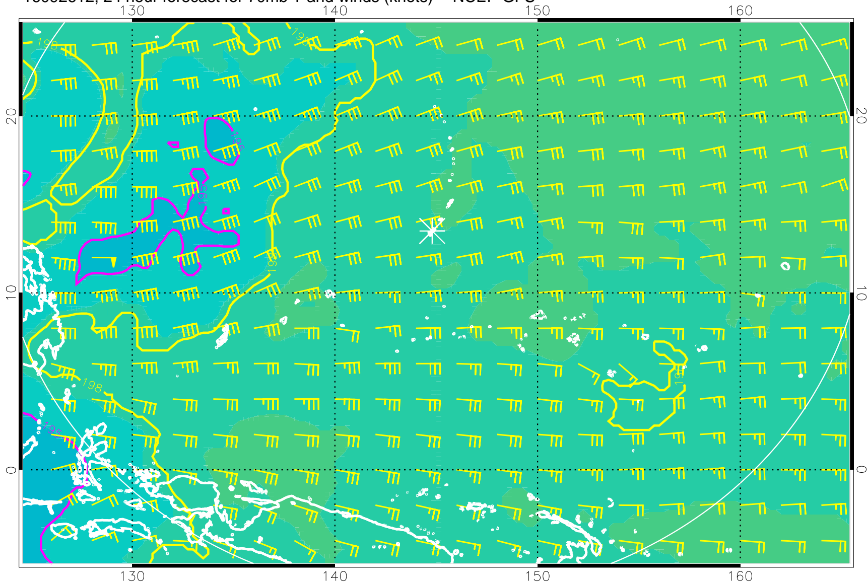
16092612, 24 hour forecast for 70mb T and winds (knots) -- NCEP GFS
