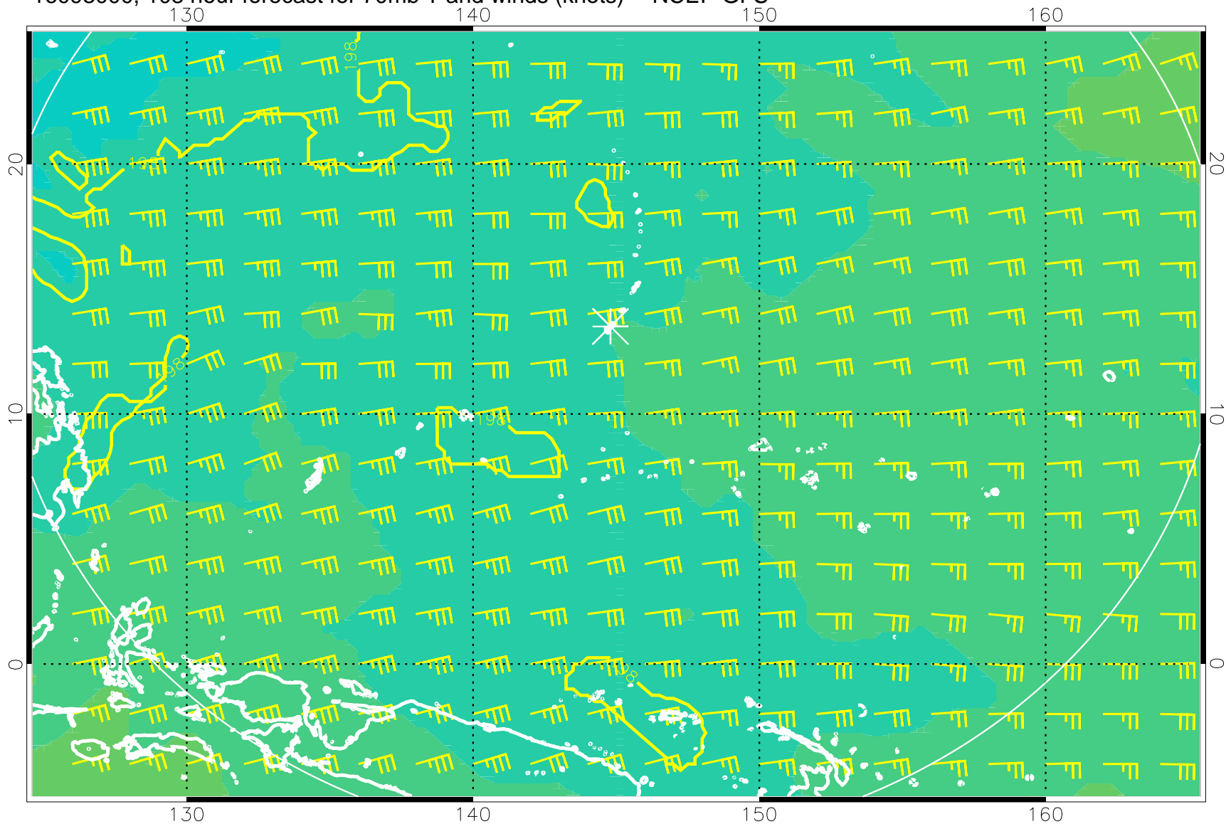
16093000, 108 hour forecast for 70mb T and winds (knots) -- NCEP GFS
