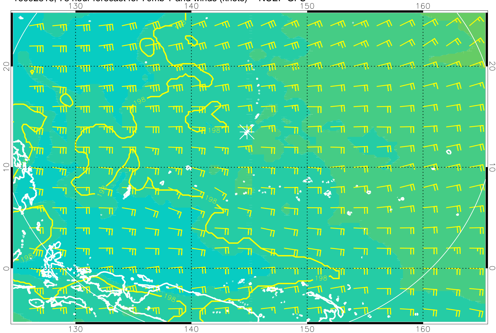
16092818, 78 hour forecast for 70mb T and winds (knots) -- NCEP GFS
