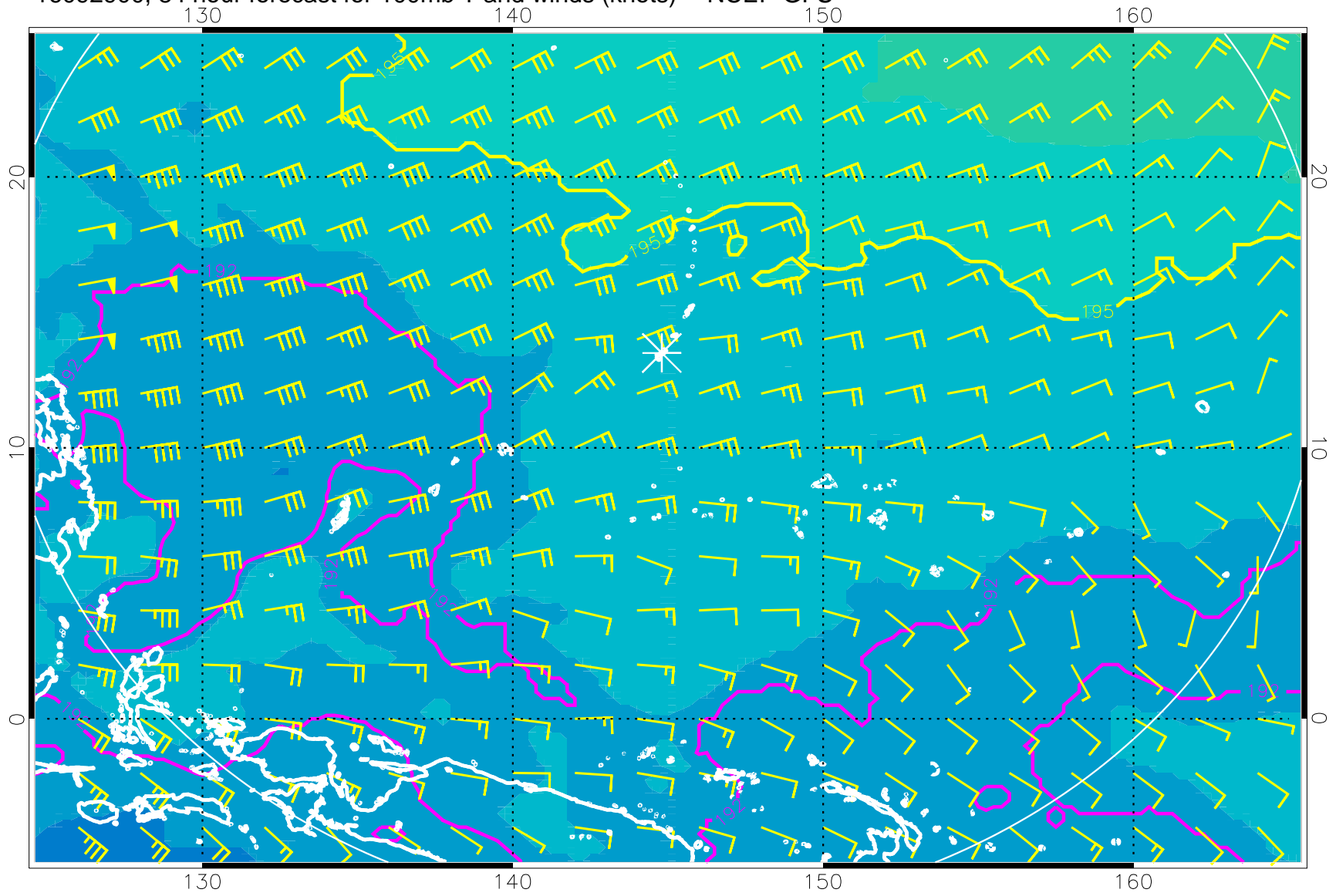
16092900, 84 hour forecast for 100mb T and winds (knots) -- NCEP GFS
