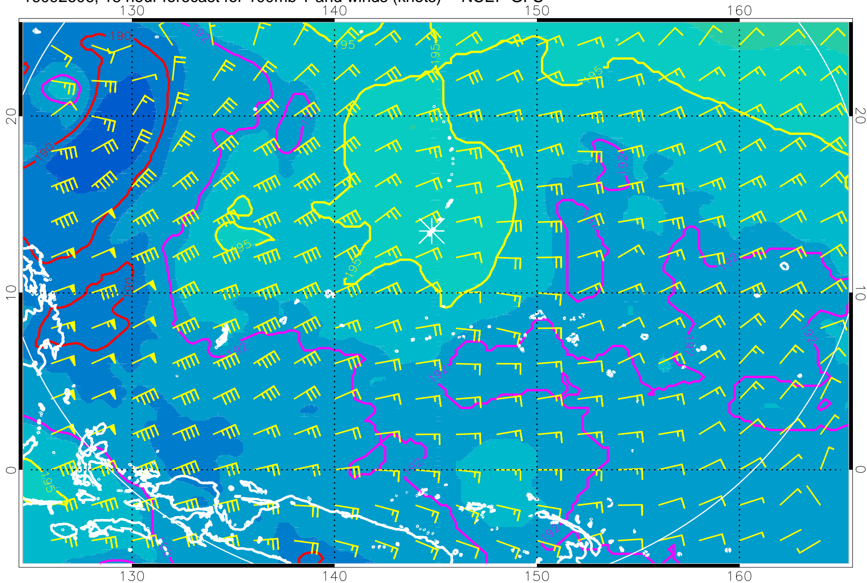
16092606, 18 hour forecast for 100mb T and winds (knots) -- NCEP GFS
