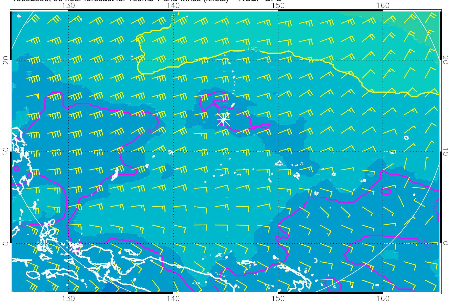
16092906, 90 hour forecast for 100mb T and winds (knots) -- NCEP GFS
