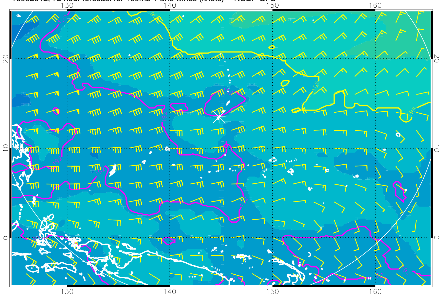
16092812, 72 hour forecast for 100mb T and winds (knots) -- NCEP GFS
