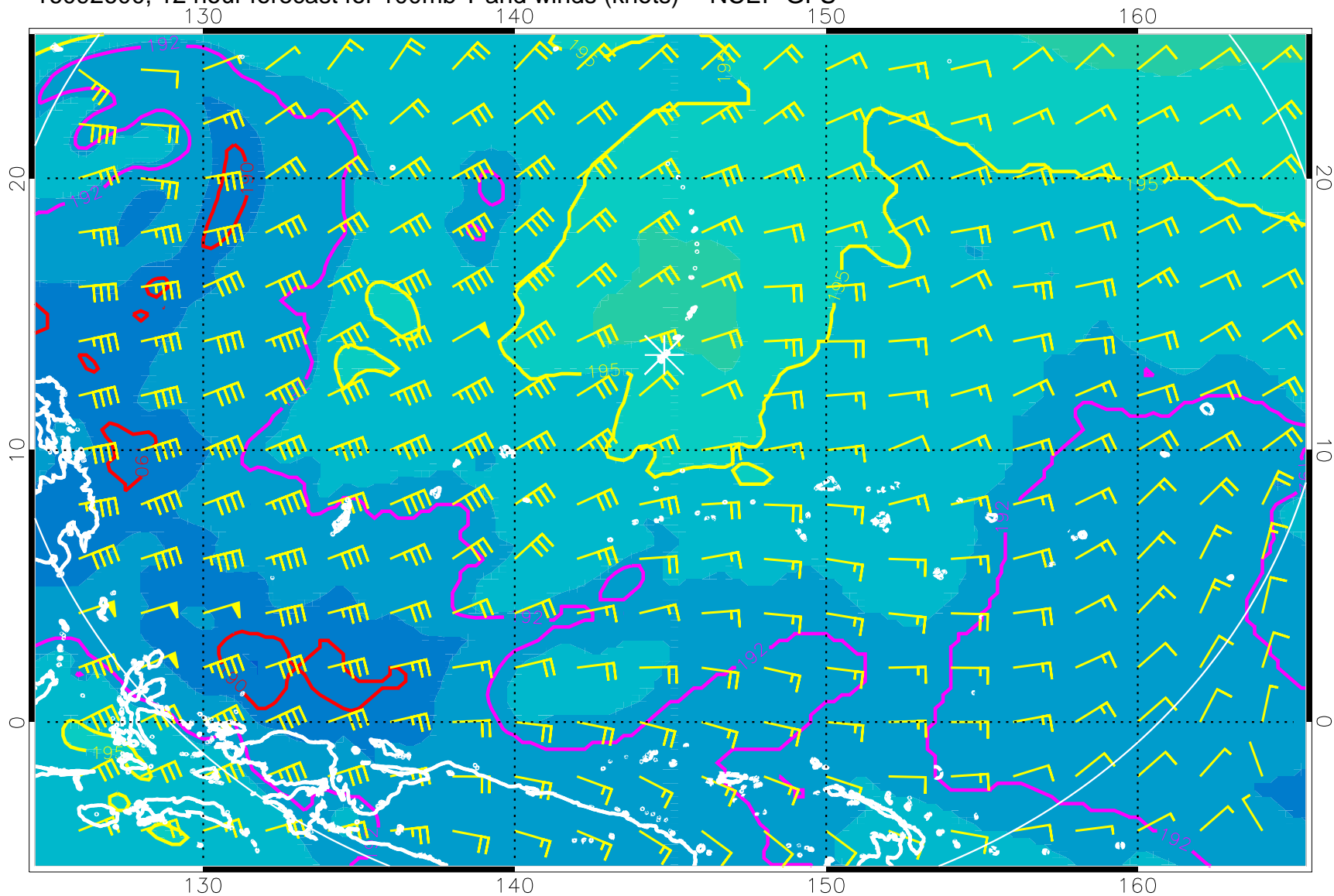
16092600, 12 hour forecast for 100mb T and winds (knots) -- NCEP GFS
