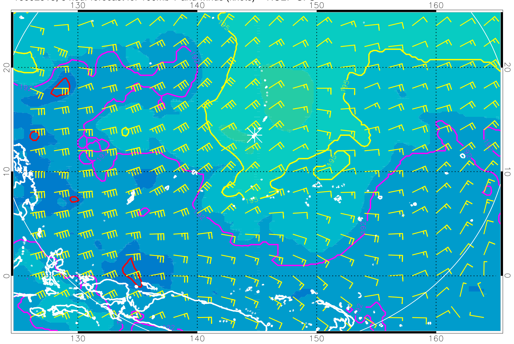
16092518, 6 hour forecast for 100mb T and winds (knots) -- NCEP GFS
