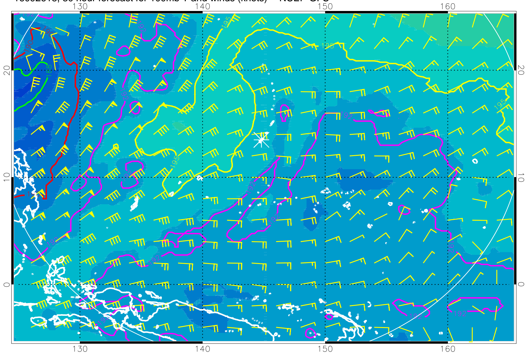
16092618, 30 hour forecast for 100mb T and winds (knots) -- NCEP GFS
