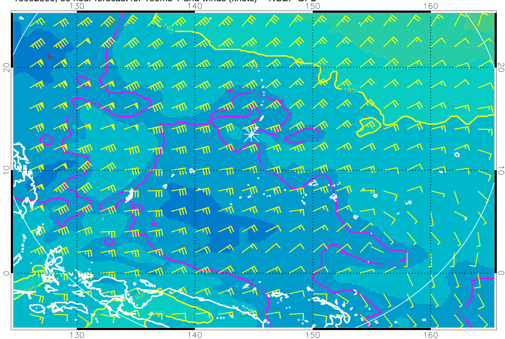
16092800, 60 hour forecast for 100mb T and winds (knots) -- NCEP GFS
