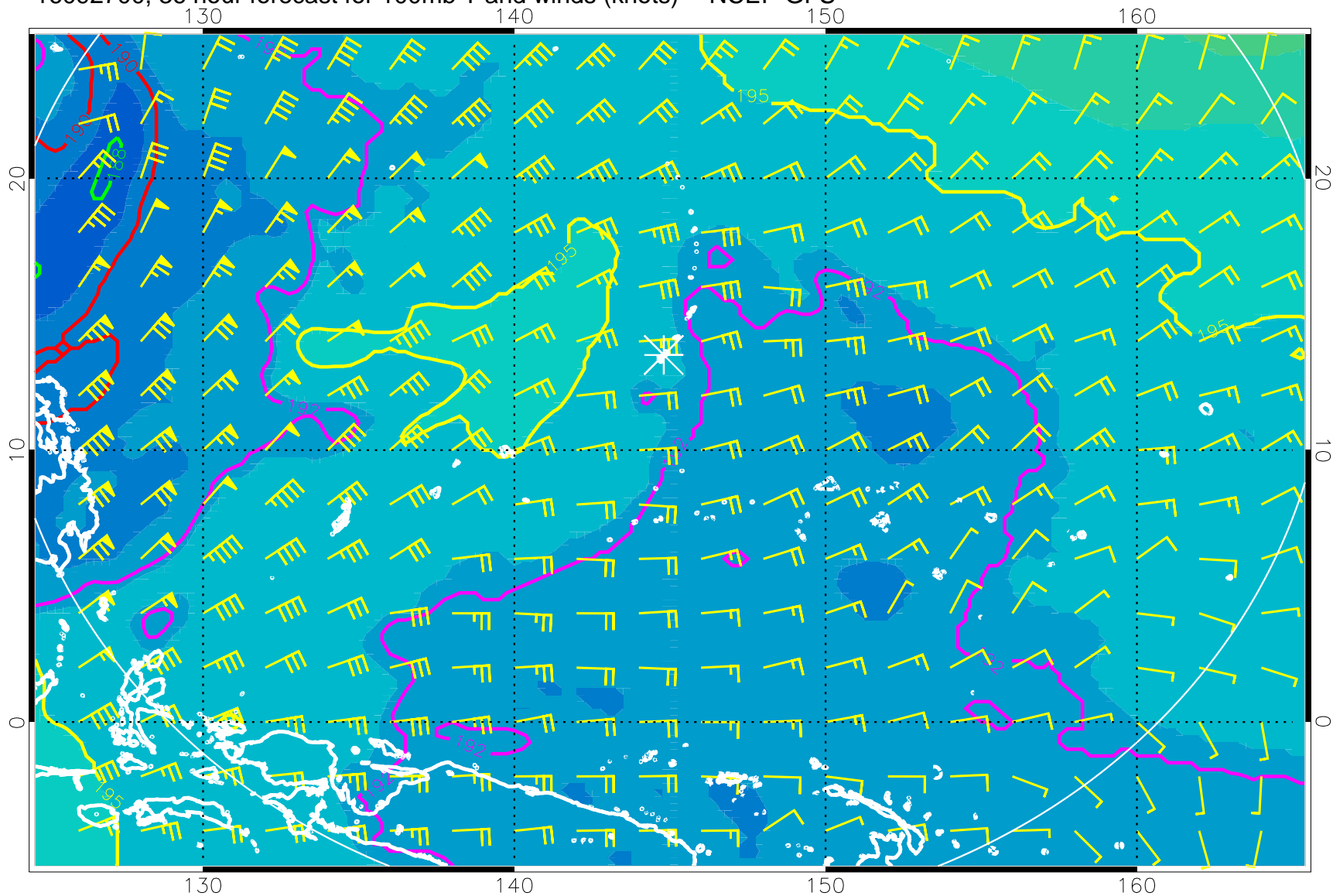
16092700, 36 hour forecast for 100mb T and winds (knots) -- NCEP GFS
