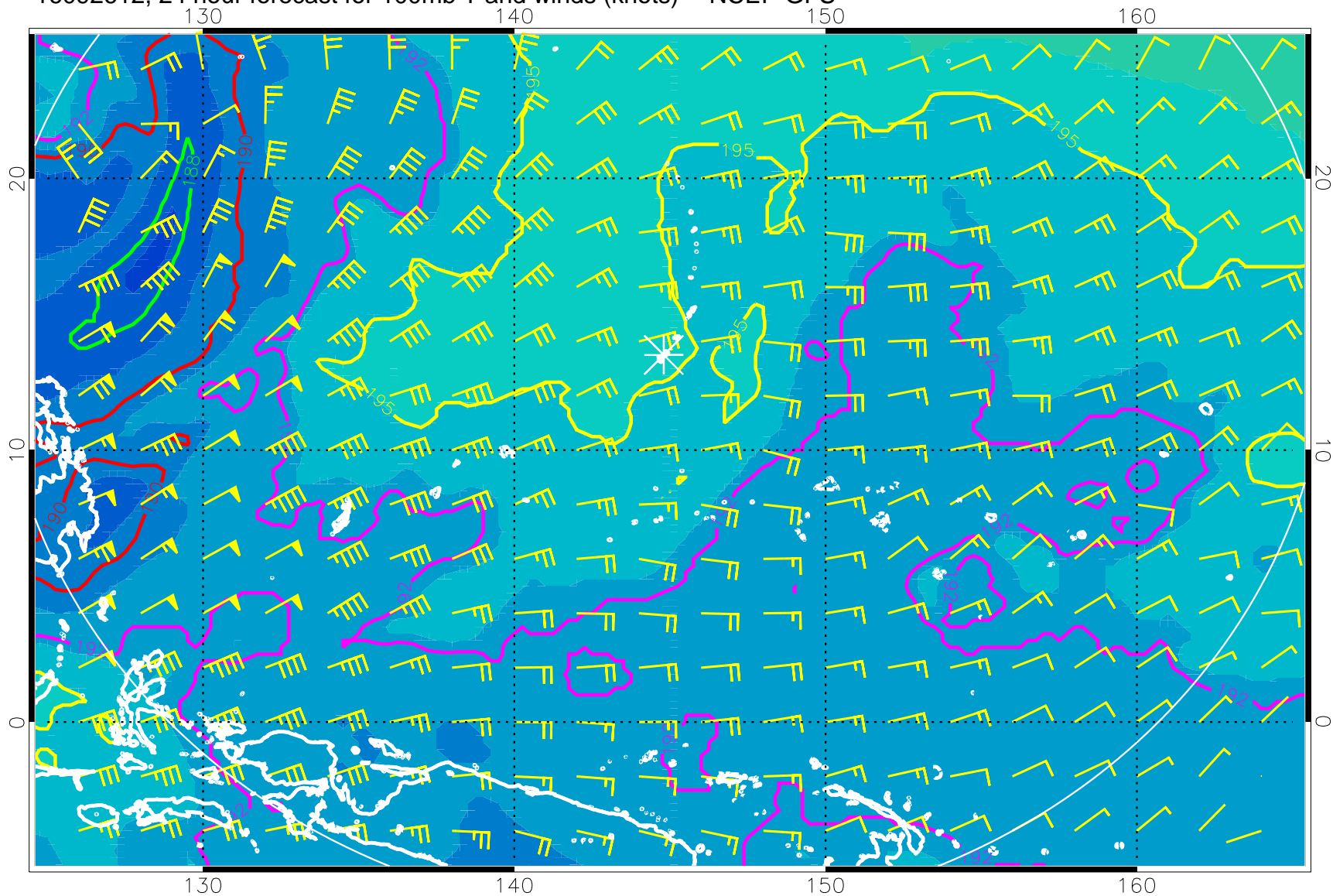
16092612, 24 hour forecast for 100mb T and winds (knots) -- NCEP GFS
