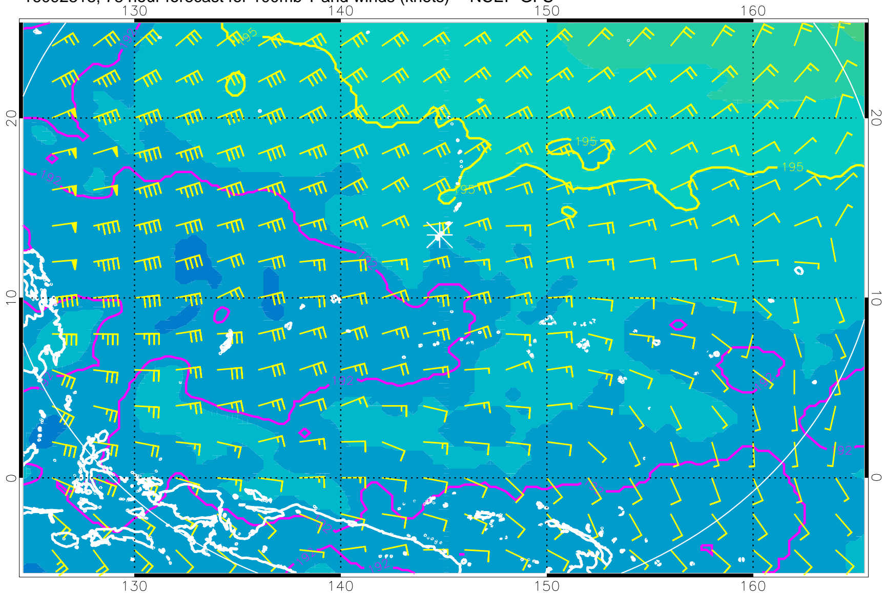
16092818, 78 hour forecast for 100mb T and winds (knots) -- NCEP GFS
