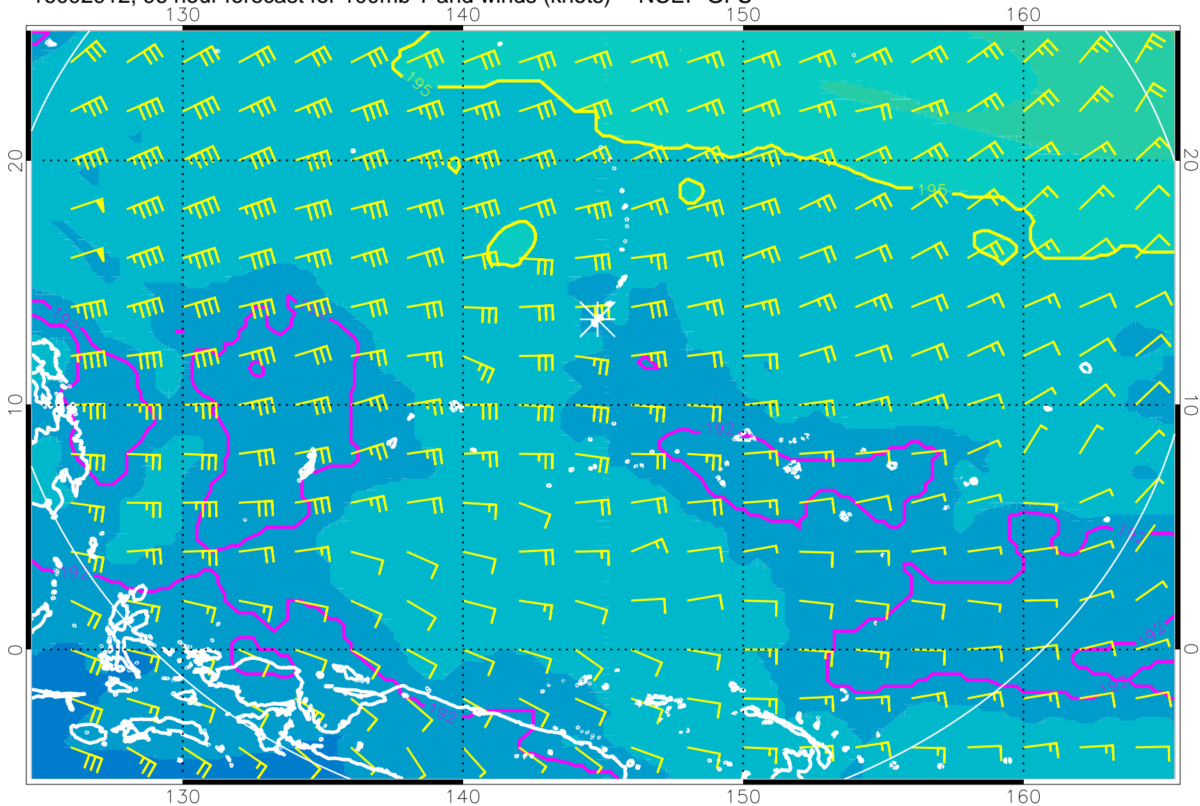
16092912, 96 hour forecast for 100mb T and winds (knots) -- NCEP GFS
