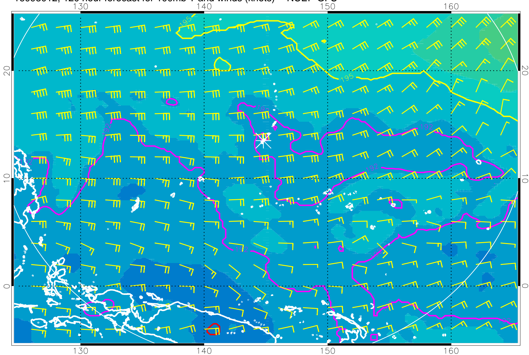
16093012, 120 hour forecast for 100mb T and winds (knots) -- NCEP GFS
