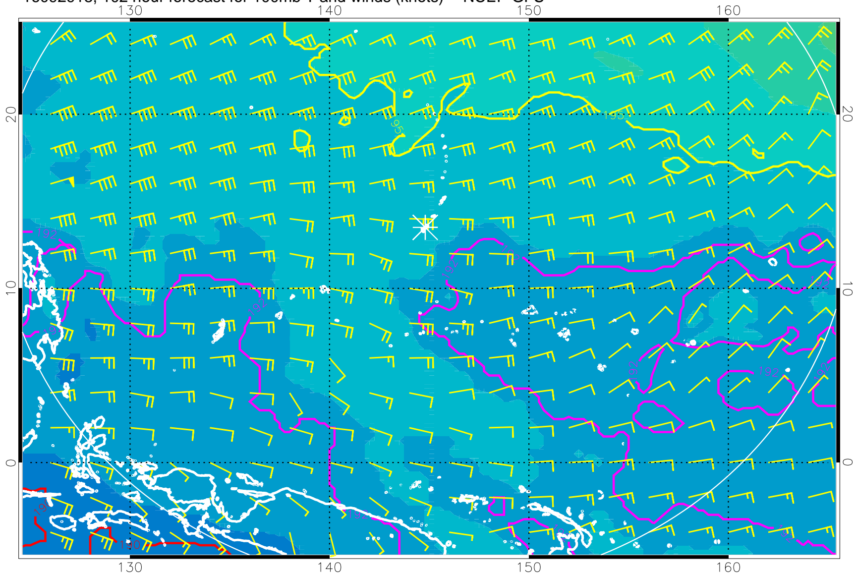
16092918, 102 hour forecast for 100mb T and winds (knots) -- NCEP GFS
