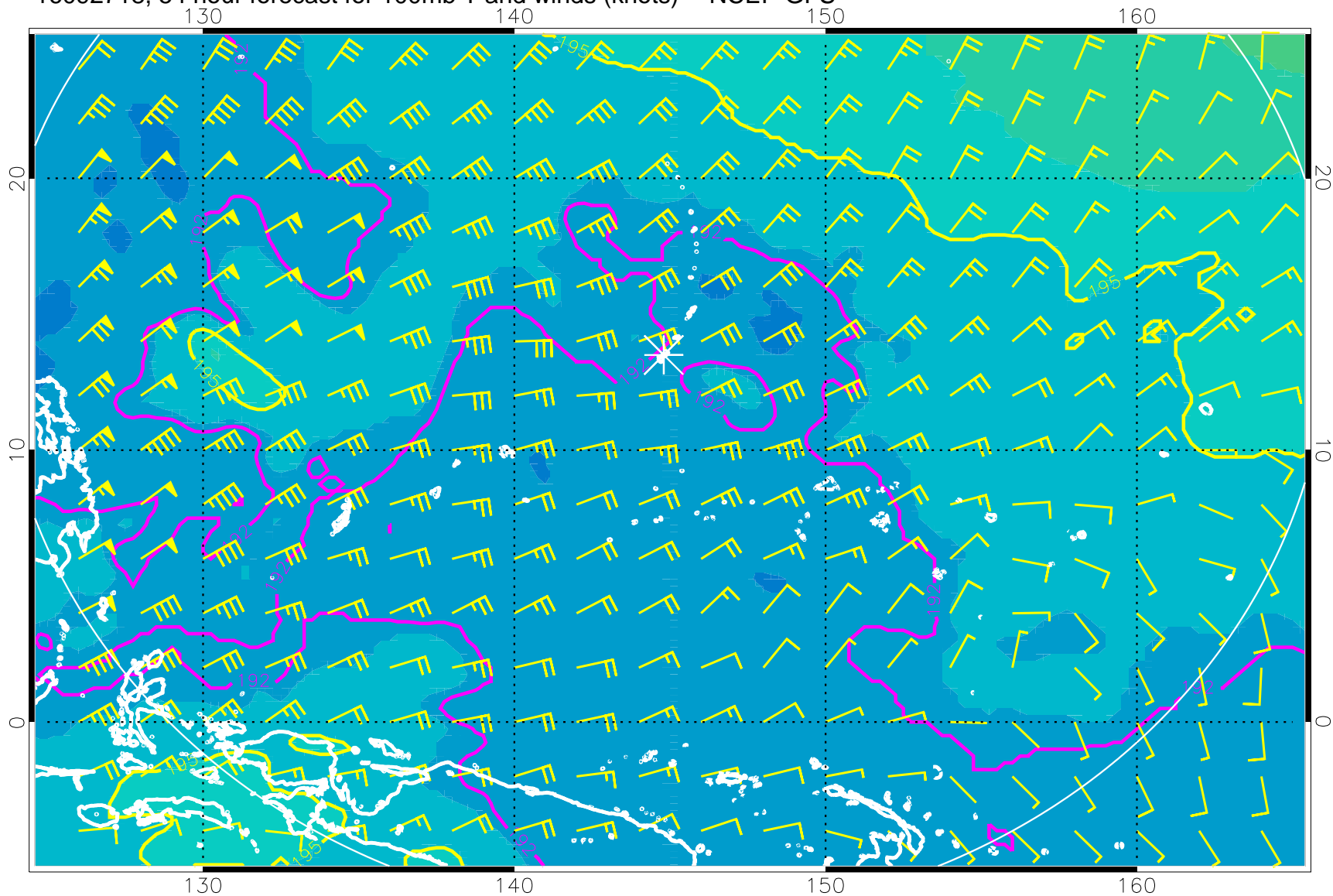
16092718, 54 hour forecast for 100mb T and winds (knots) -- NCEP GFS
