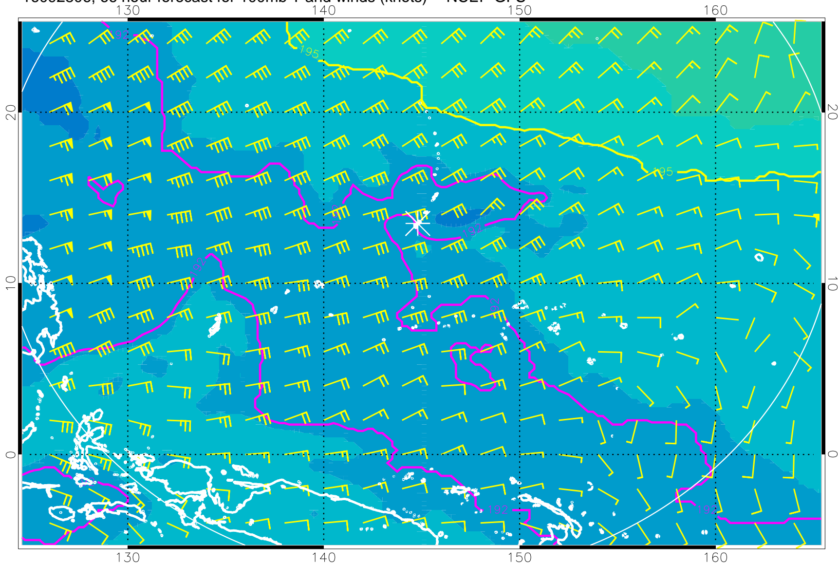
16092806, 66 hour forecast for 100mb T and winds (knots) -- NCEP GFS
