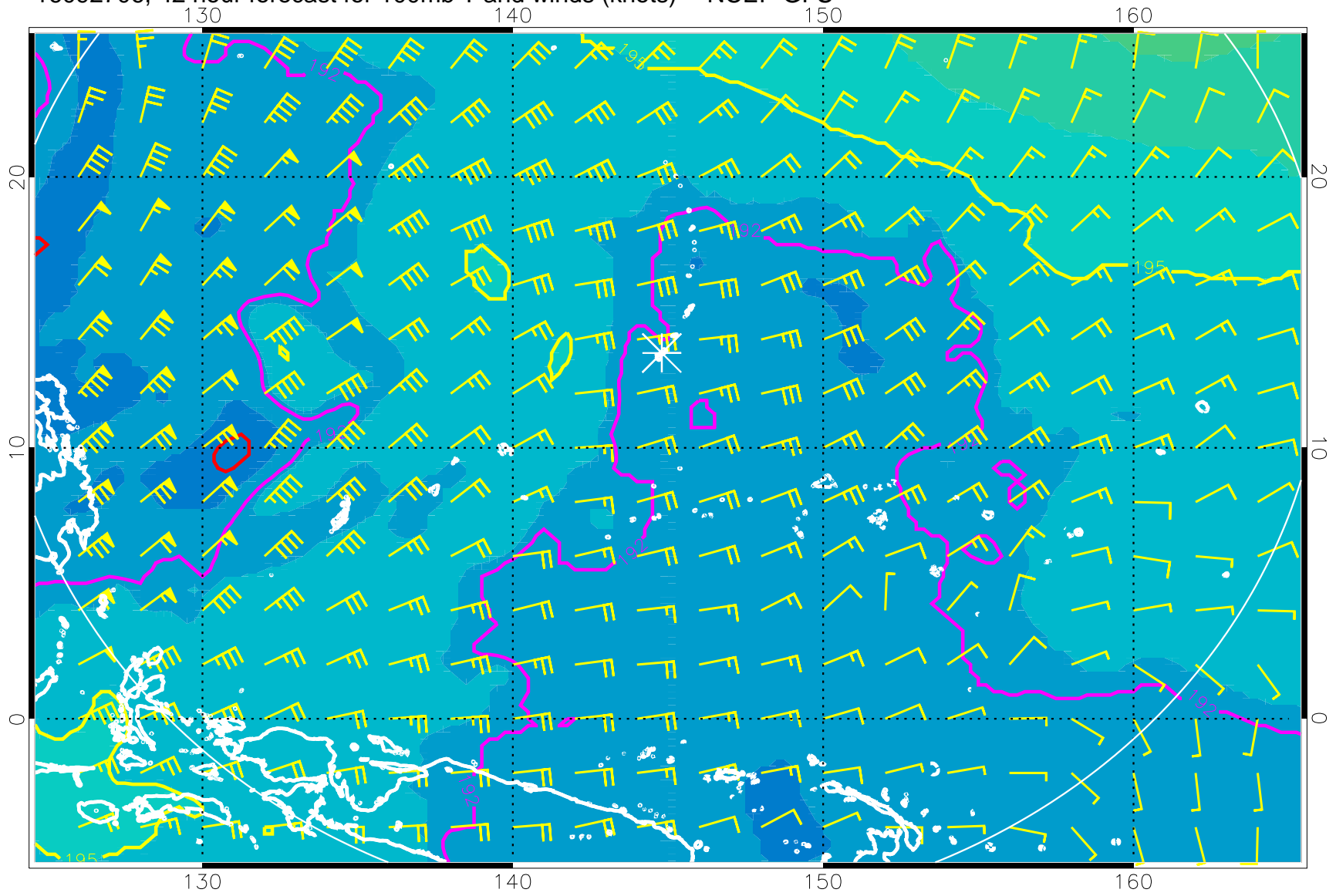
16092706, 42 hour forecast for 100mb T and winds (knots) -- NCEP GFS
