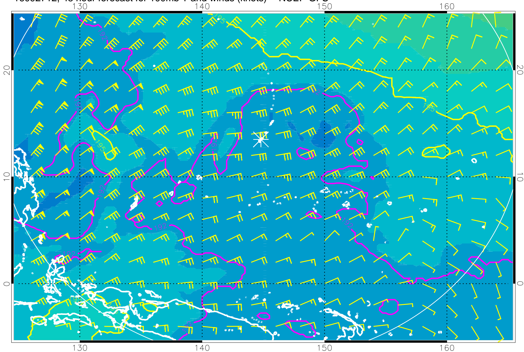
16092712, 48 hour forecast for 100mb T and winds (knots) -- NCEP GFS
