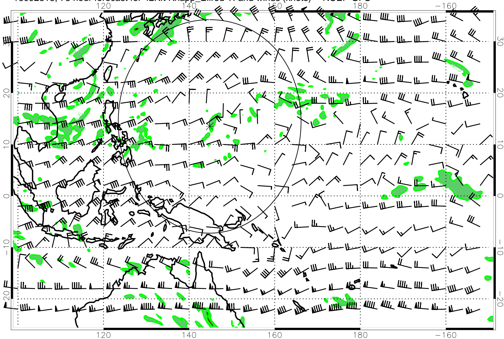
16092818, 78 hour forecast for 42Kft Knapp_Ellrod TI and winds (knots) -- NCEP GFS
