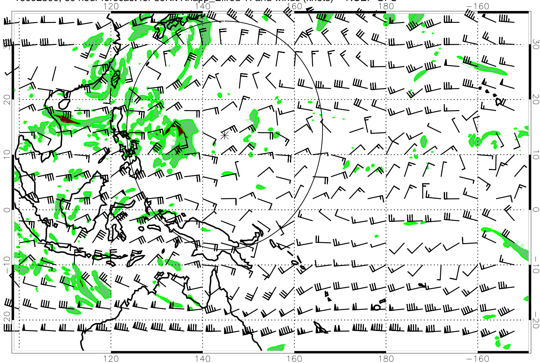
16092800, 60 hour forecast for 39Kft Knapp_Ellrod TI and winds (knots) -- NCEP GFS
