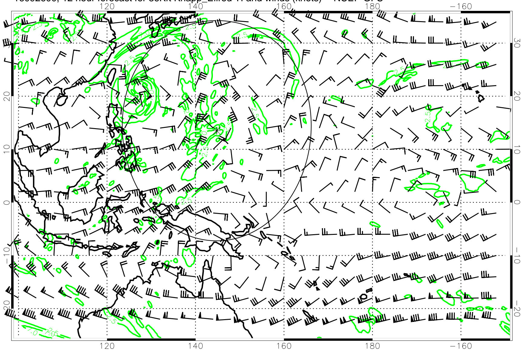
16092600, 12 hour forecast for 36Kft Knapp_Ellrod TI and winds (knots) -- NCEP GFS
