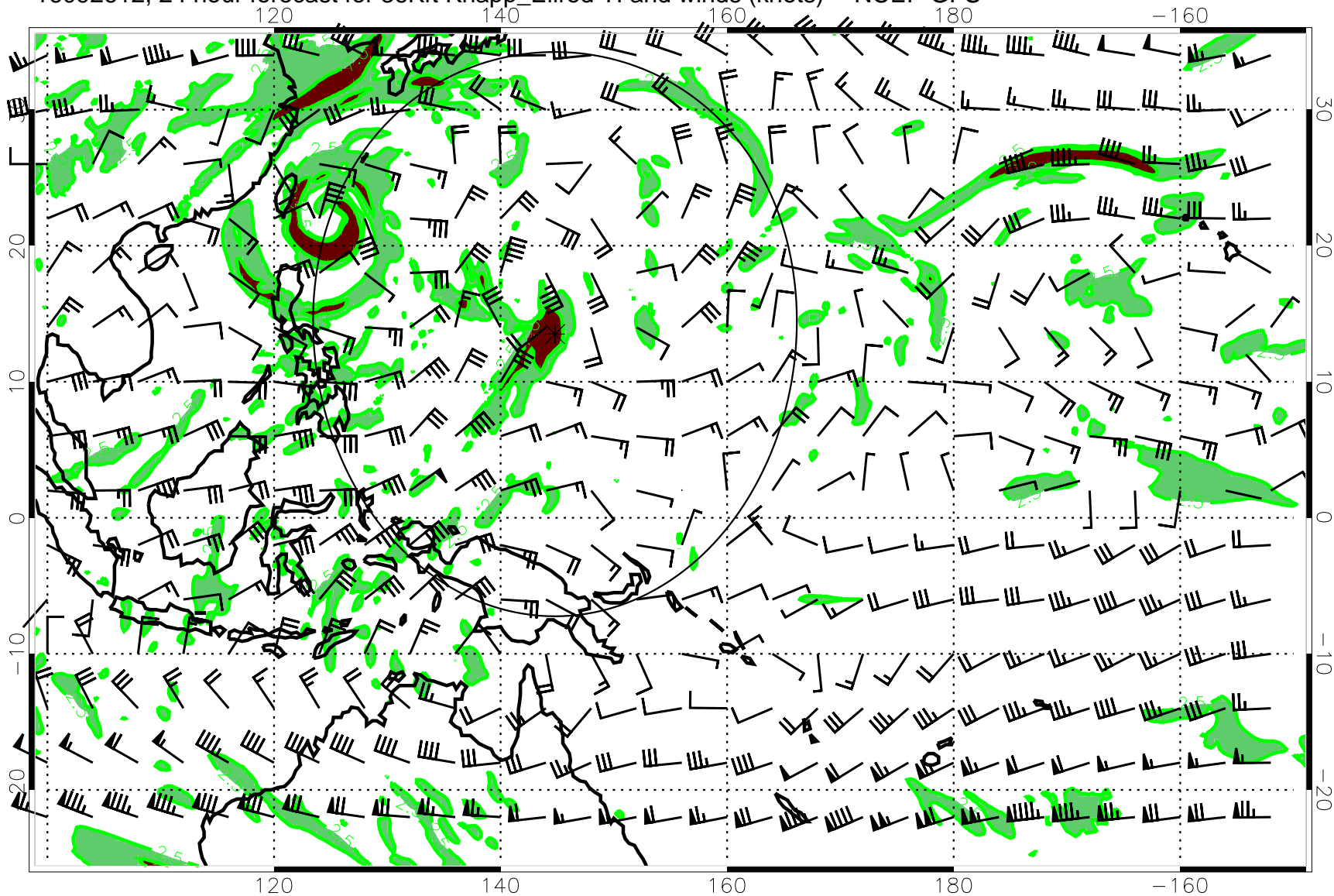
16092612, 24 hour forecast for 36Kft Knapp_Ellrod TI and winds (knots) -- NCEP GFS
