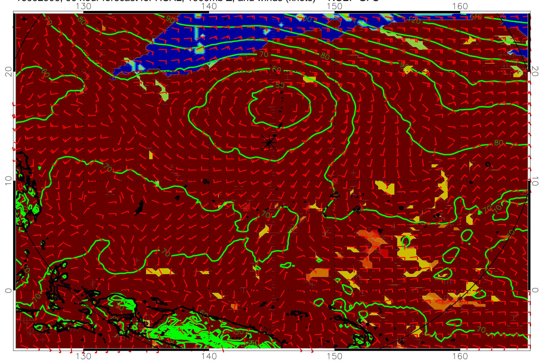
16092906, 90 hour forecast for HCAL, 1000mb Z, and winds (knots) -- NCEP GFS
