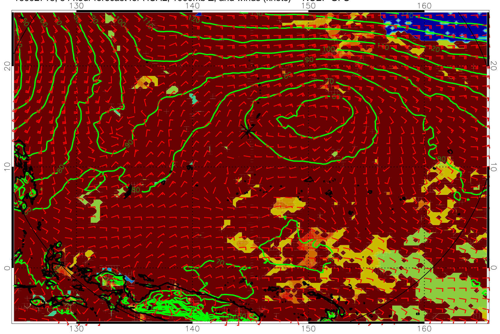
16092718, 54 hour forecast for HCAL, 1000mb Z, and winds (knots) -- NCEP GFS
