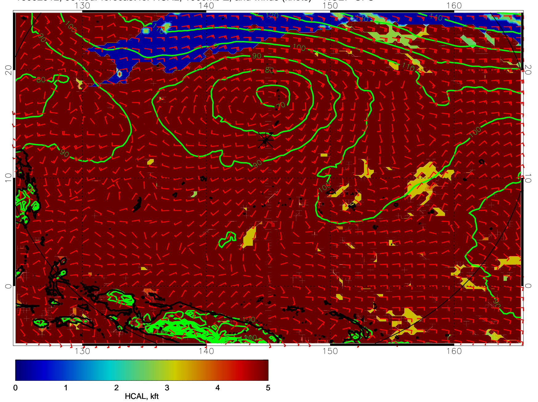
16092912, 96 hour forecast for HCAL, 1000mb Z, and winds (knots) -- NCEP GFS
