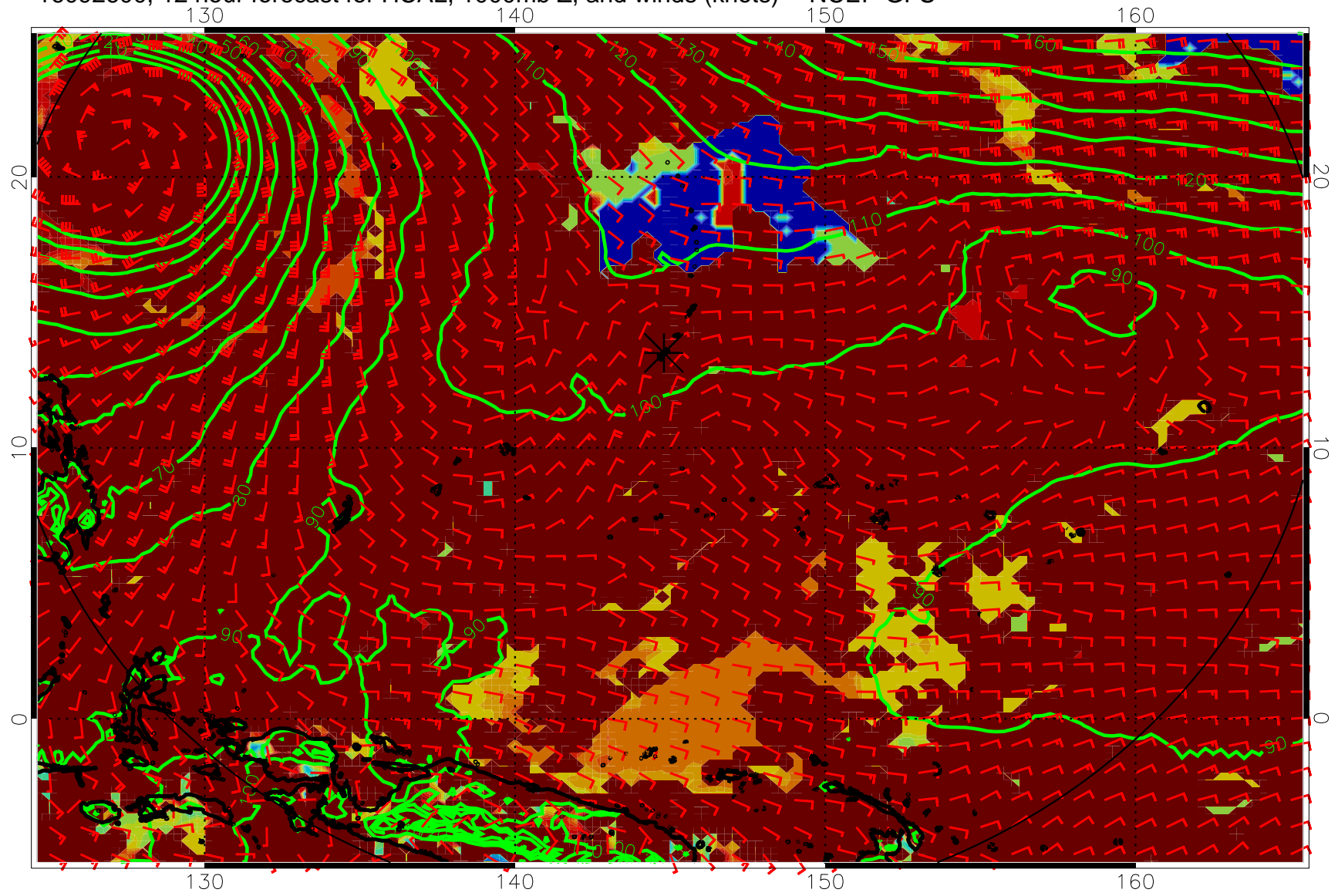
16092600, 12 hour forecast for HCAL, 1000mb Z, and winds (knots) -- NCEP GFS
