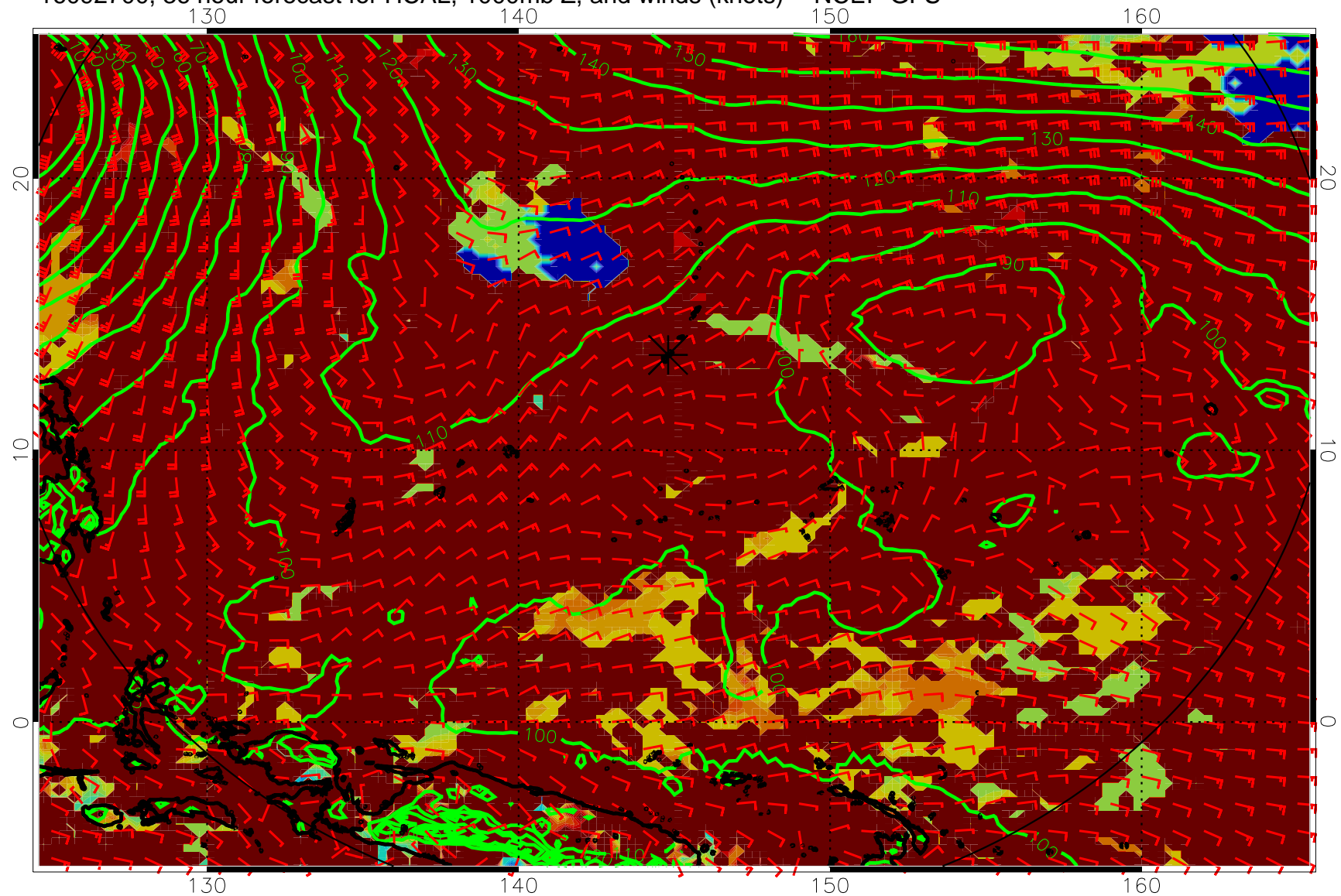
16092700, 36 hour forecast for HCAL, 1000mb Z, and winds (knots) -- NCEP GFS
