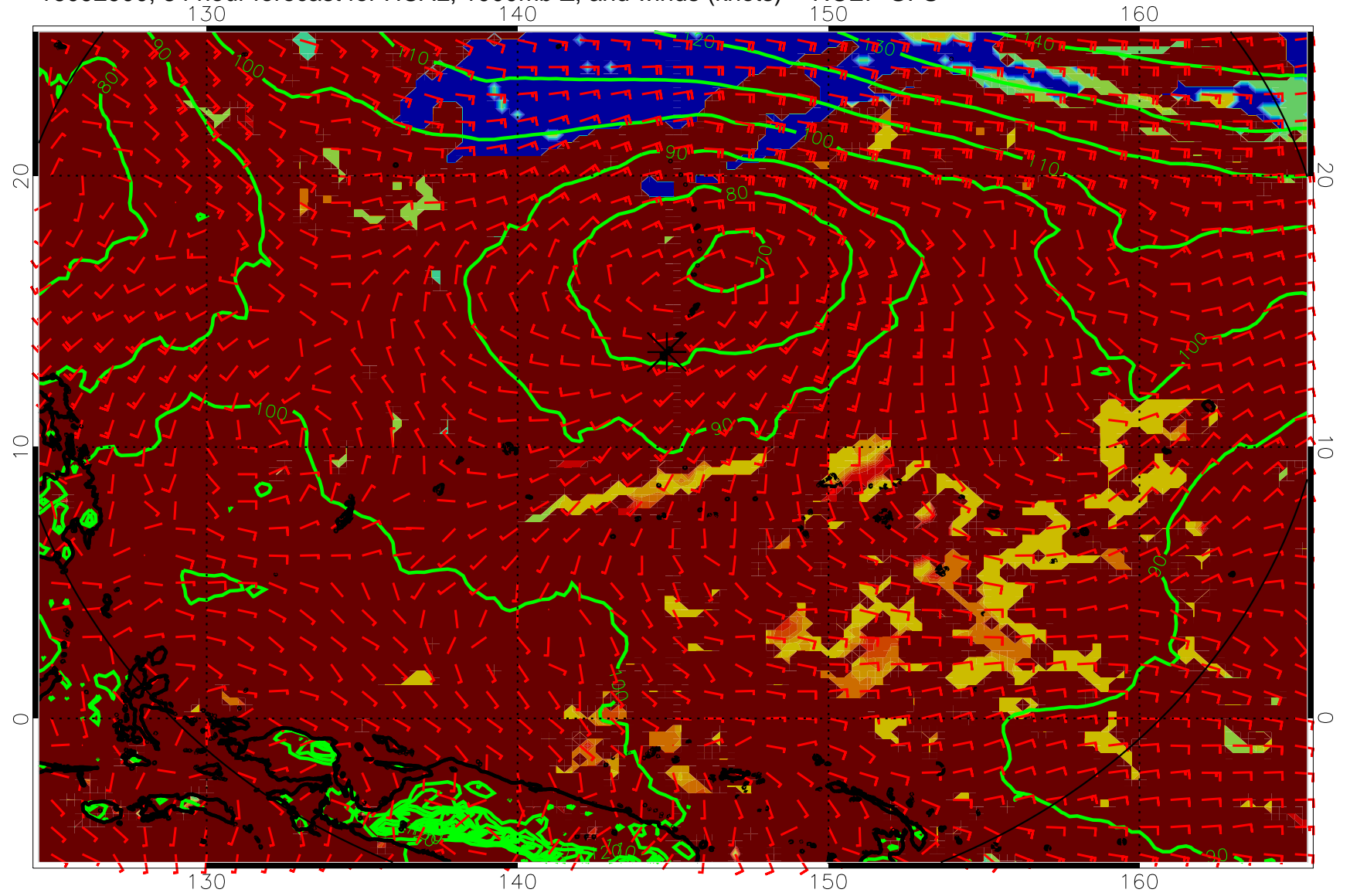
16092900, 84 hour forecast for HCAL, 1000mb Z, and winds (knots) -- NCEP GFS
