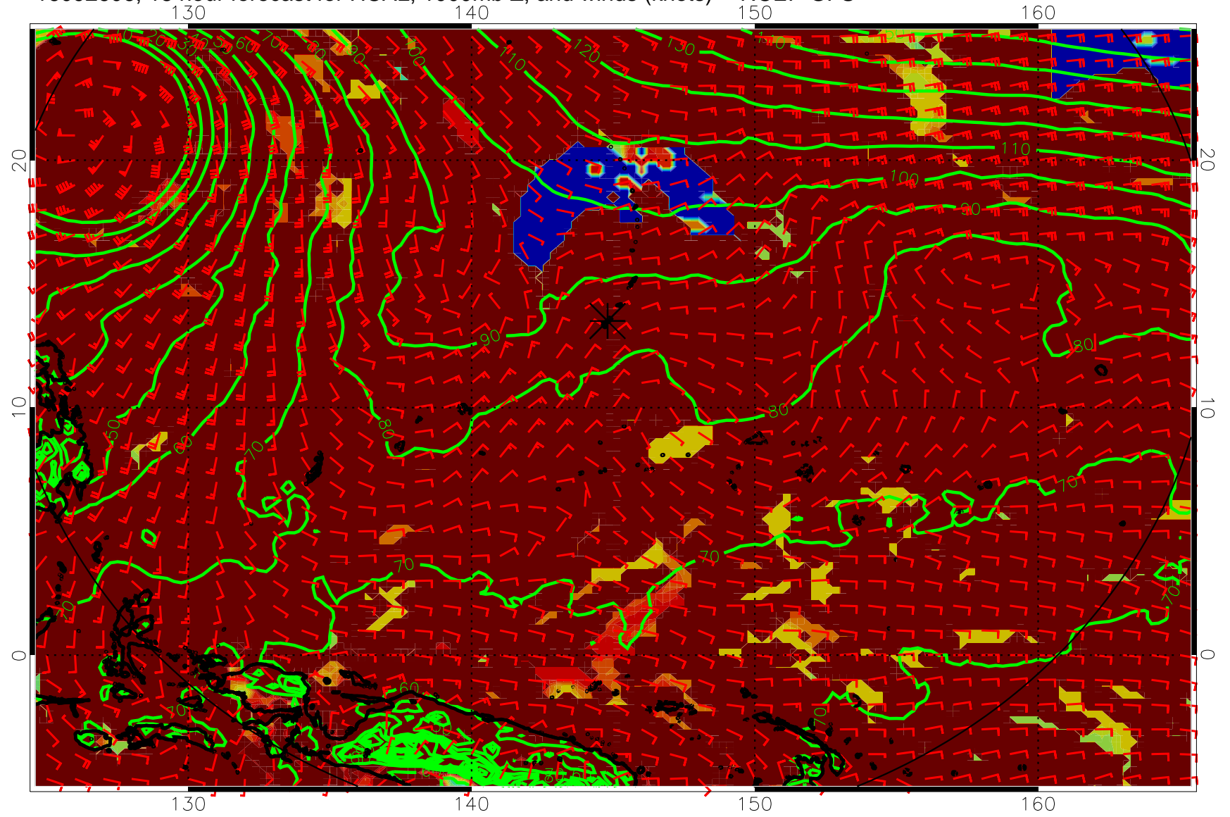
16092606, 18 hour forecast for HCAL, 1000mb Z, and winds (knots) -- NCEP GFS
