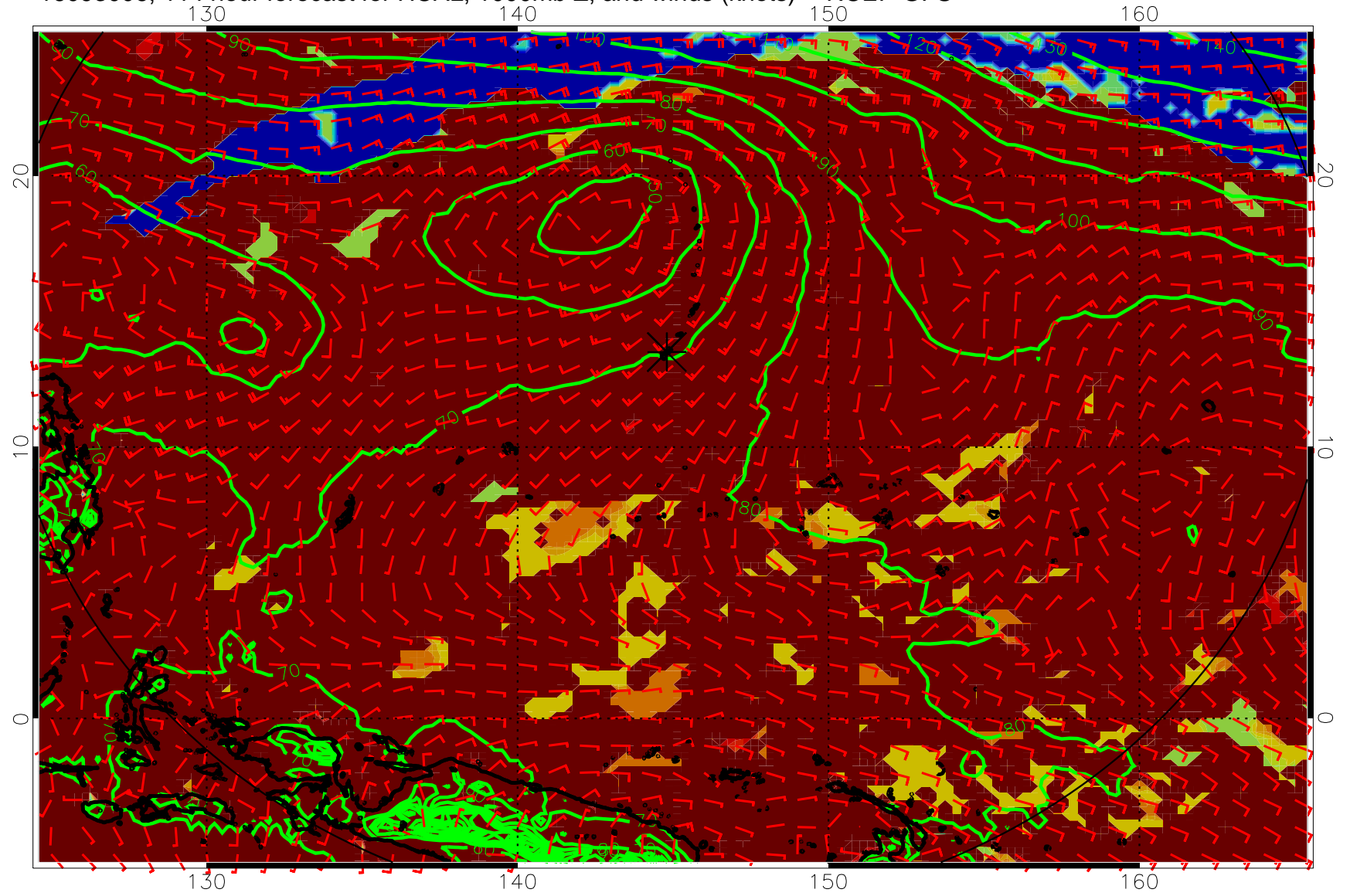
16093006, 114 hour forecast for HCAL, 1000mb Z, and winds (knots) -- NCEP GFS
