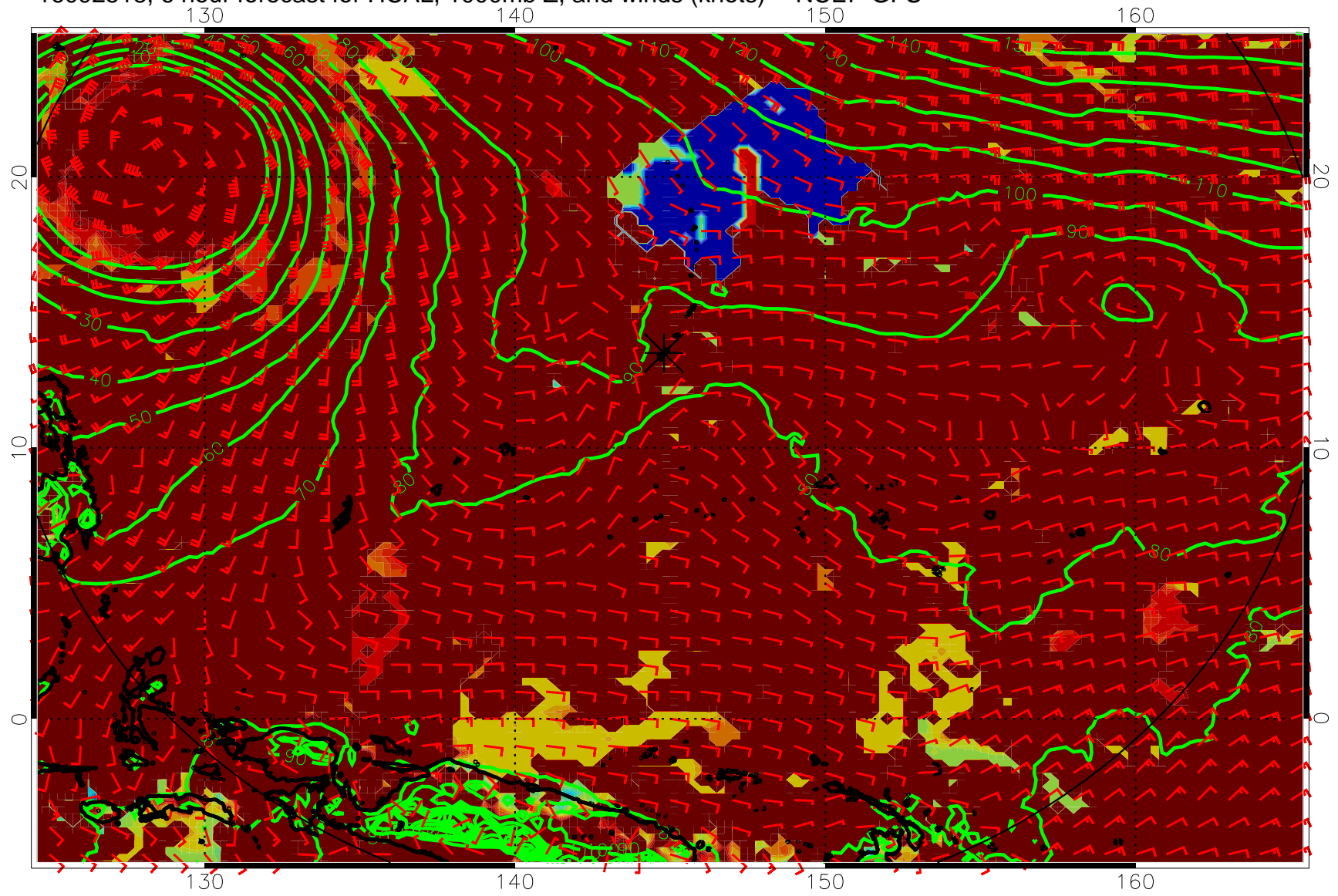
16092518, 6 hour forecast for HCAL, 1000mb Z, and winds (knots) -- NCEP GFS
