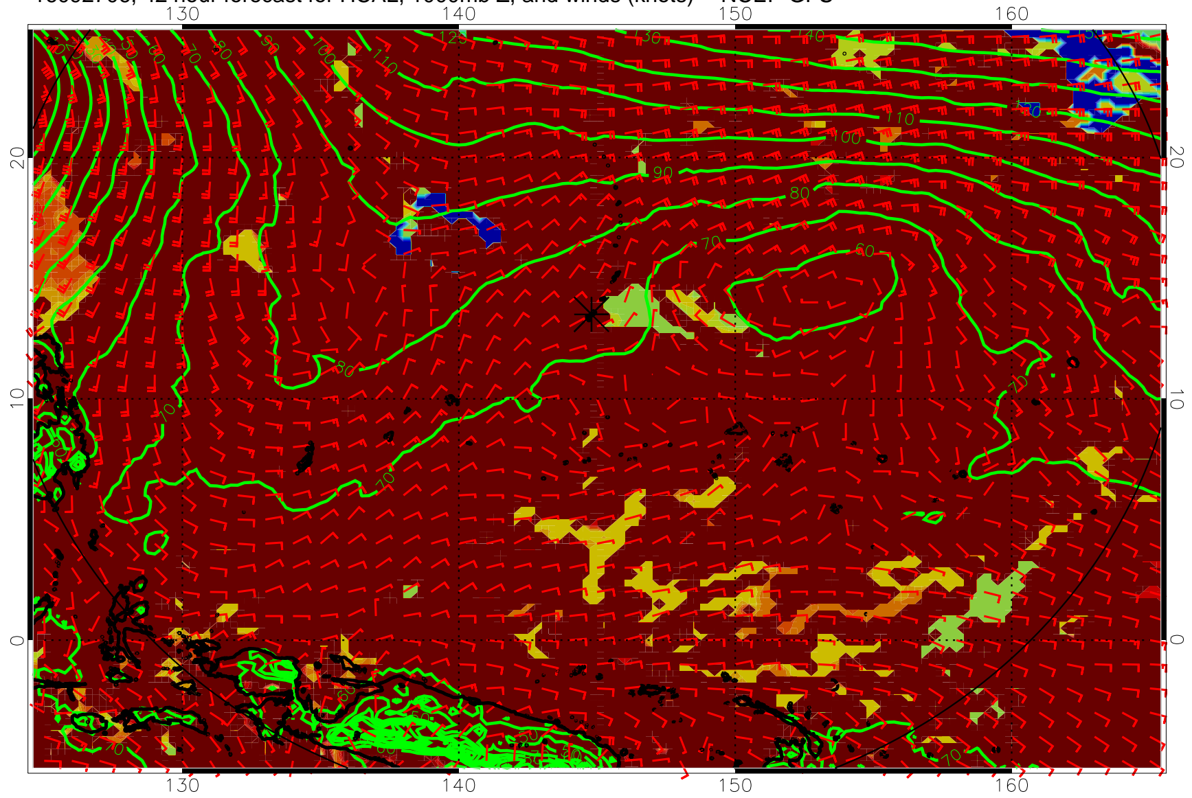
16092706, 42 hour forecast for HCAL, 1000mb Z, and winds (knots) -- NCEP GFS
