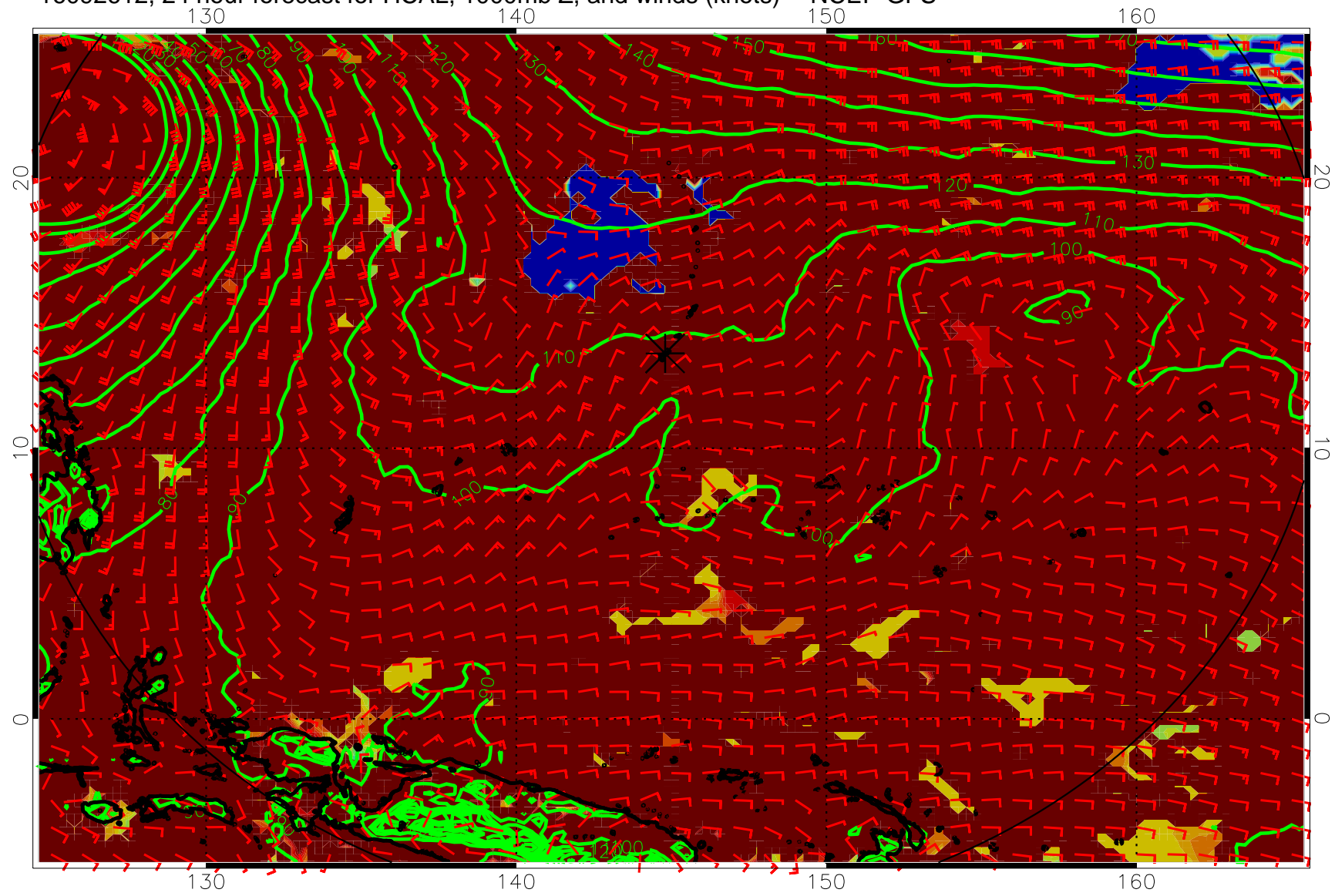
16092612, 24 hour forecast for HCAL, 1000mb Z, and winds (knots) -- NCEP GFS
