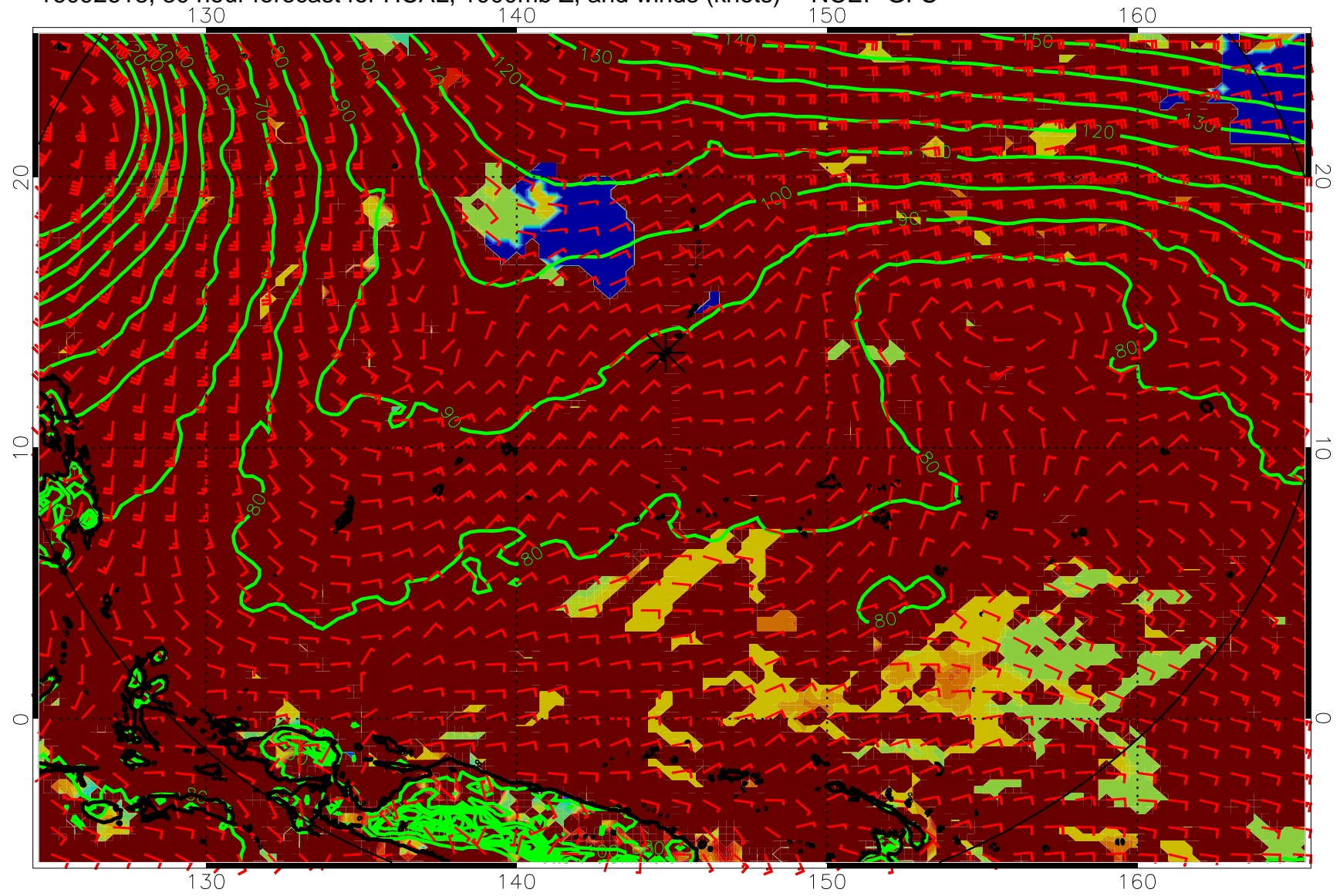
16092618, 30 hour forecast for HCAL, 1000mb Z, and winds (knots) -- NCEP GFS
