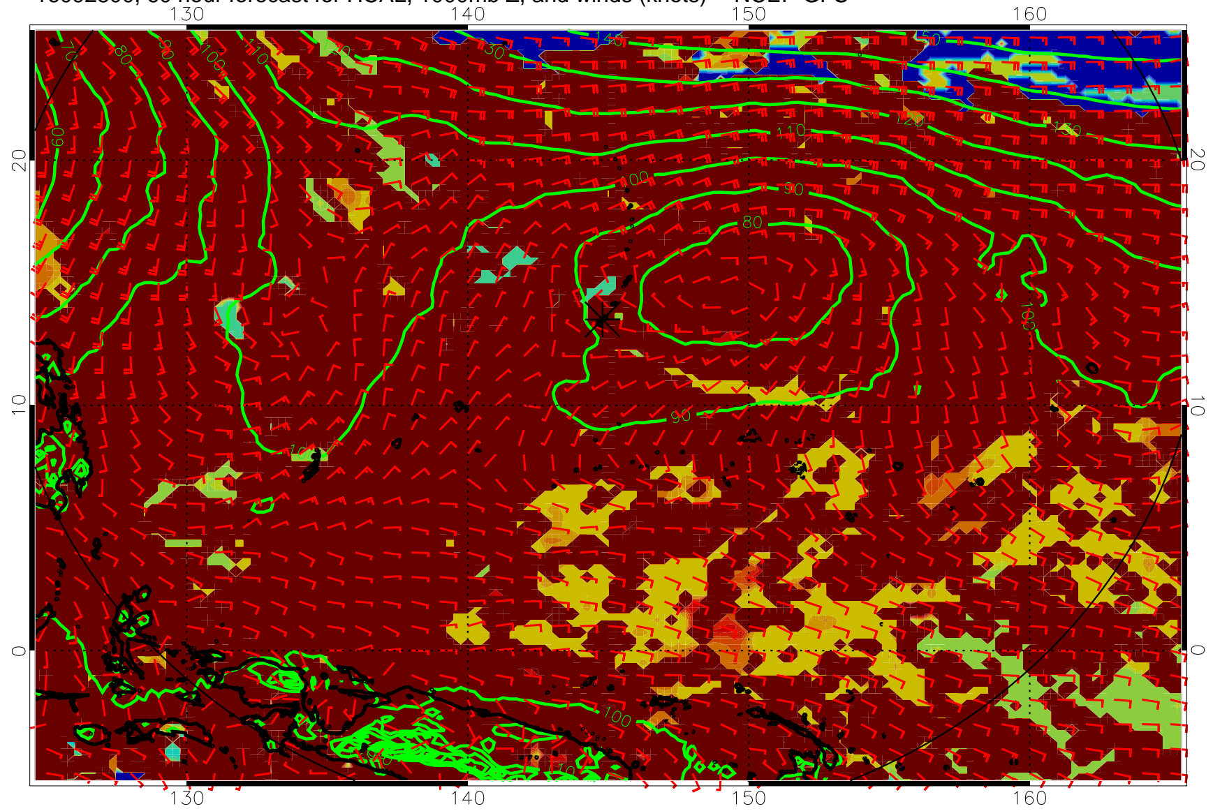
16092800, 60 hour forecast for HCAL, 1000mb Z, and winds (knots) -- NCEP GFS
