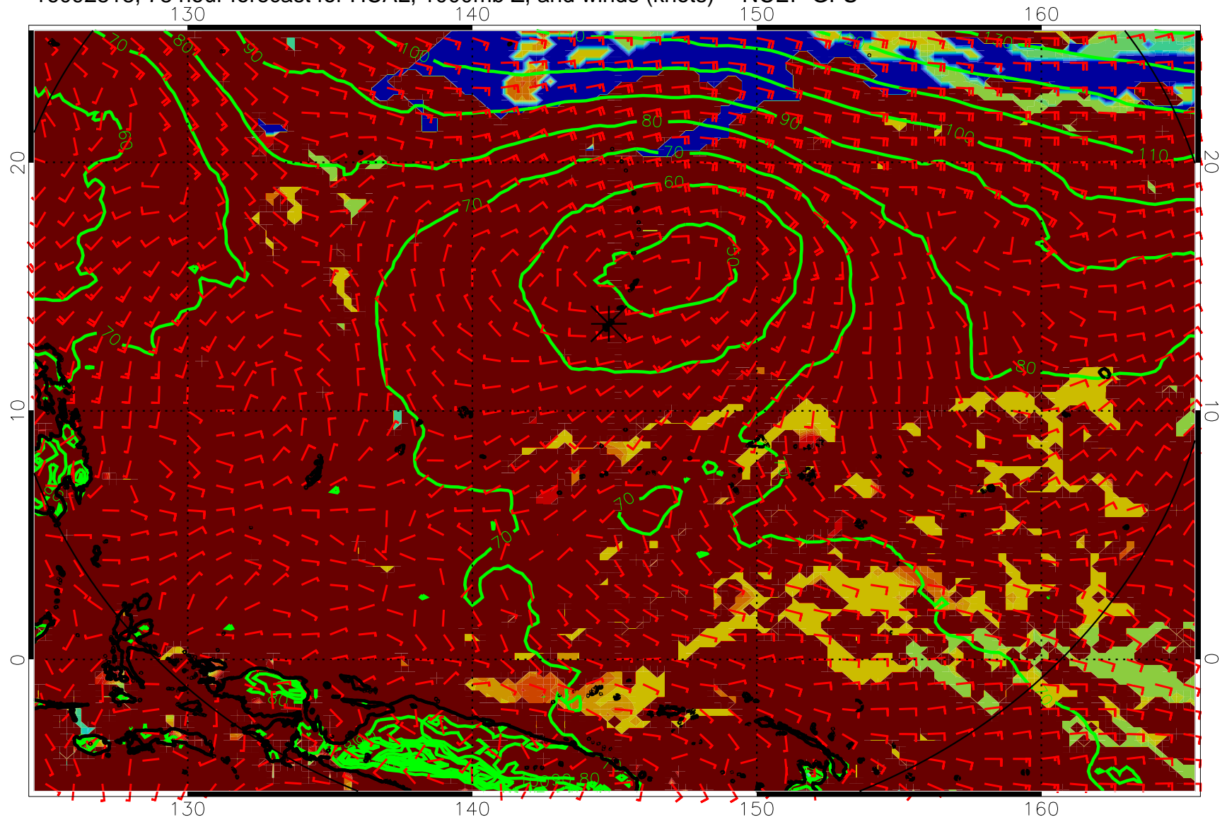
16092818, 78 hour forecast for HCAL, 1000mb Z, and winds (knots) -- NCEP GFS
