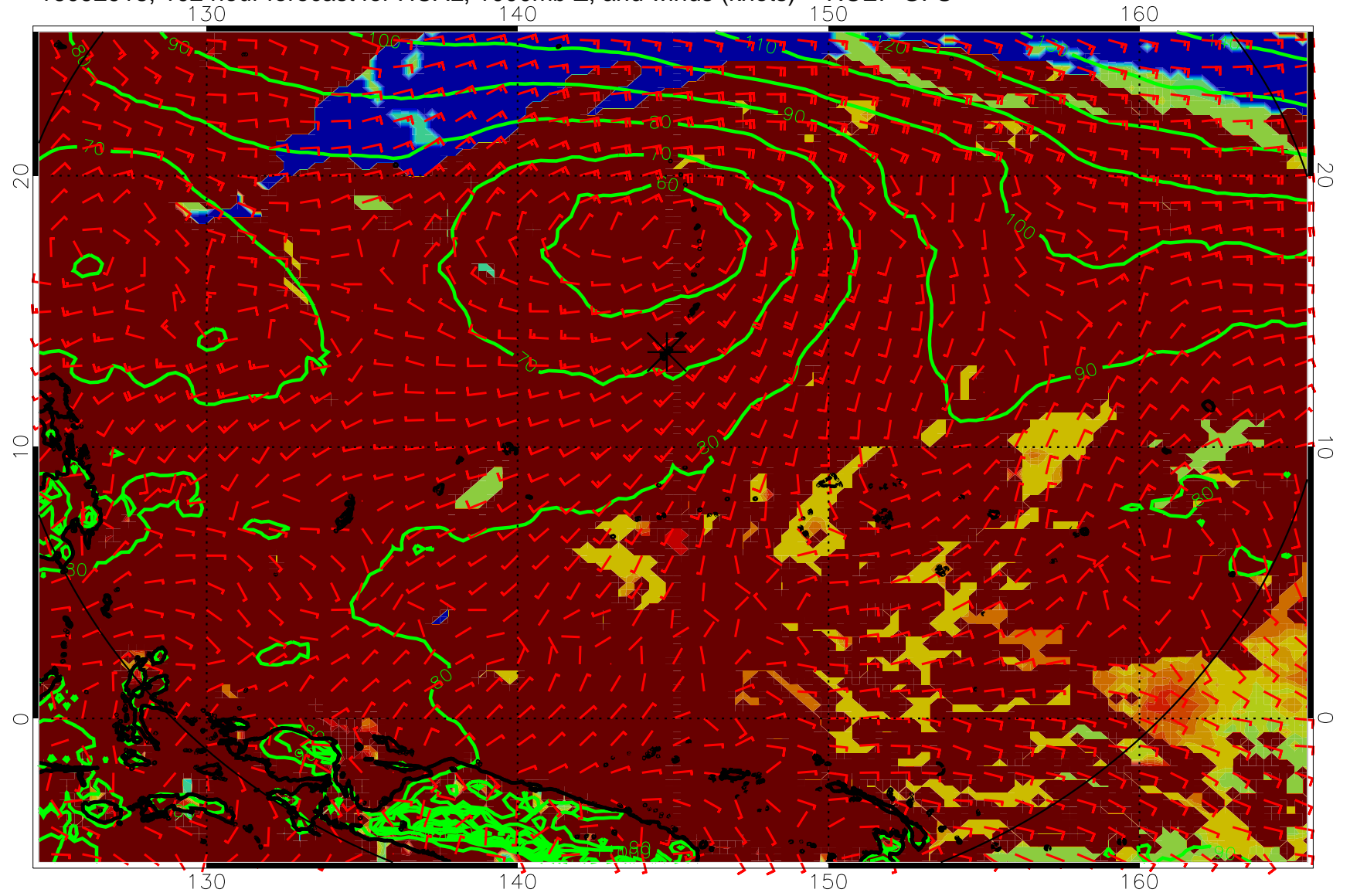
16092918, 102 hour forecast for HCAL, 1000mb Z, and winds (knots) -- NCEP GFS
