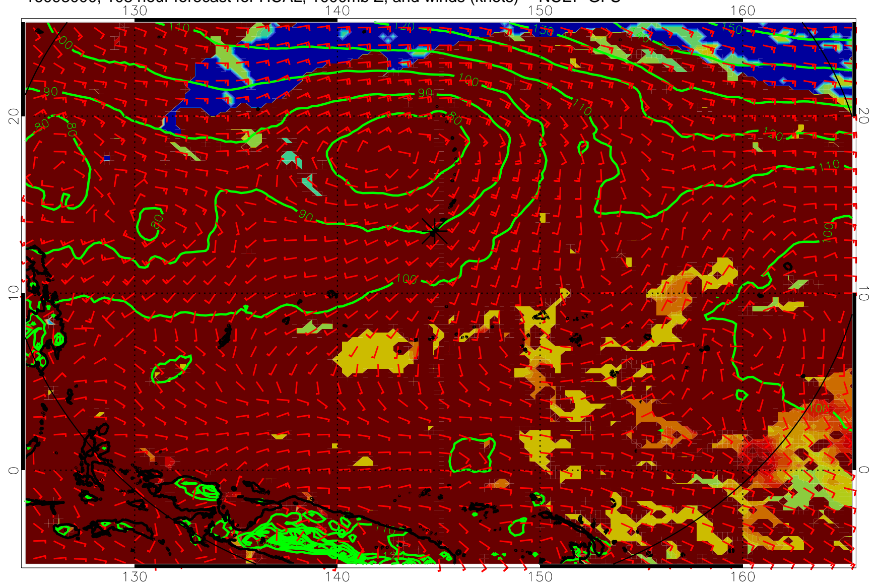
16093000, 108 hour forecast for HCAL, 1000mb Z, and winds (knots) -- NCEP GFS
