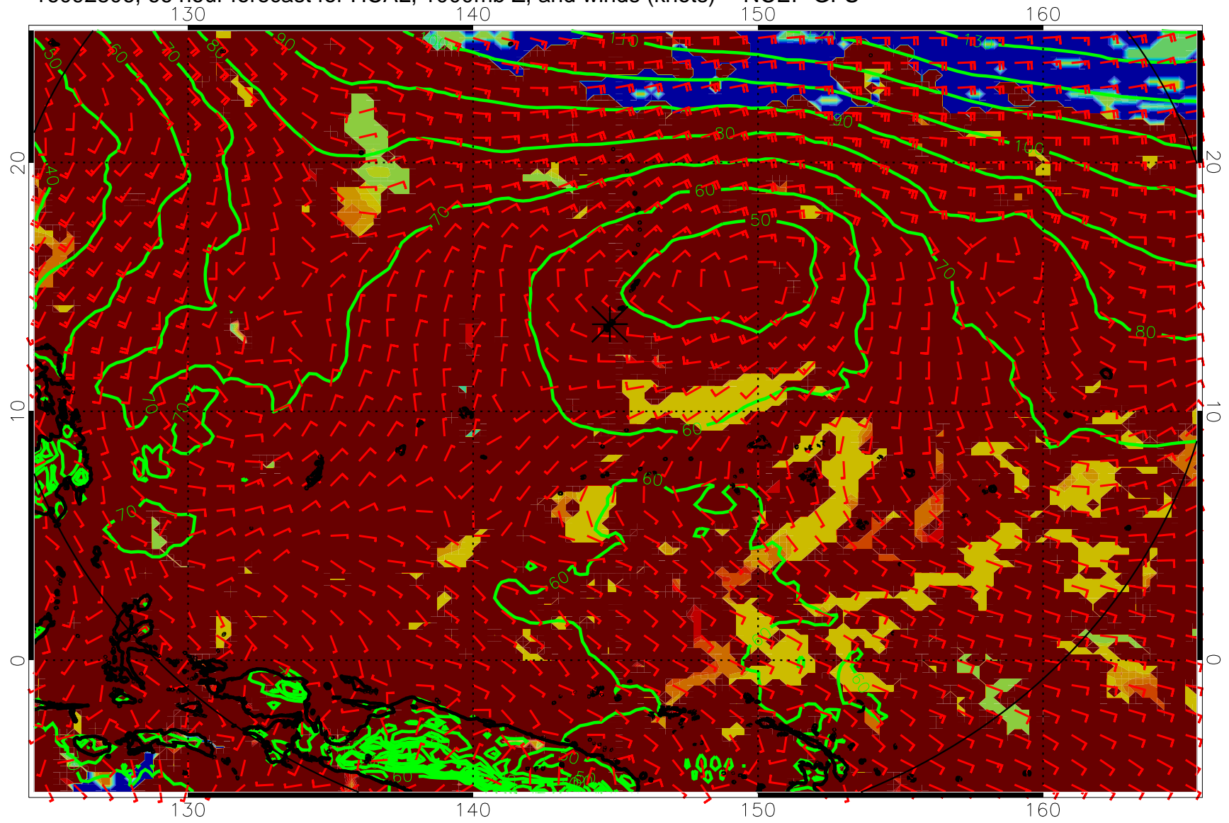
16092806, 66 hour forecast for HCAL, 1000mb Z, and winds (knots) -- NCEP GFS
