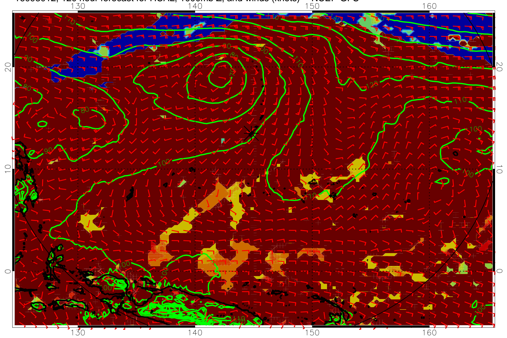
16093012, 120 hour forecast for HCAL, 1000mb Z, and winds (knots) -- NCEP GFS
