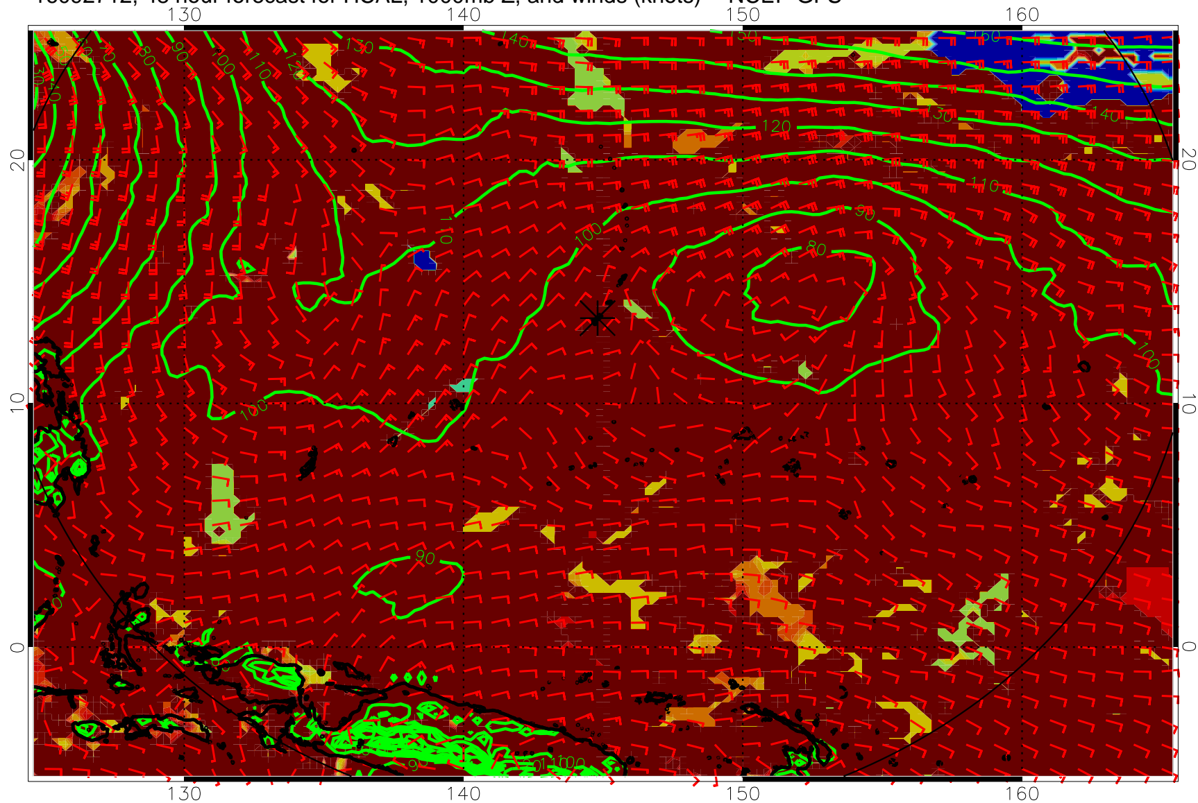
16092712, 48 hour forecast for HCAL, 1000mb Z, and winds (knots) -- NCEP GFS
