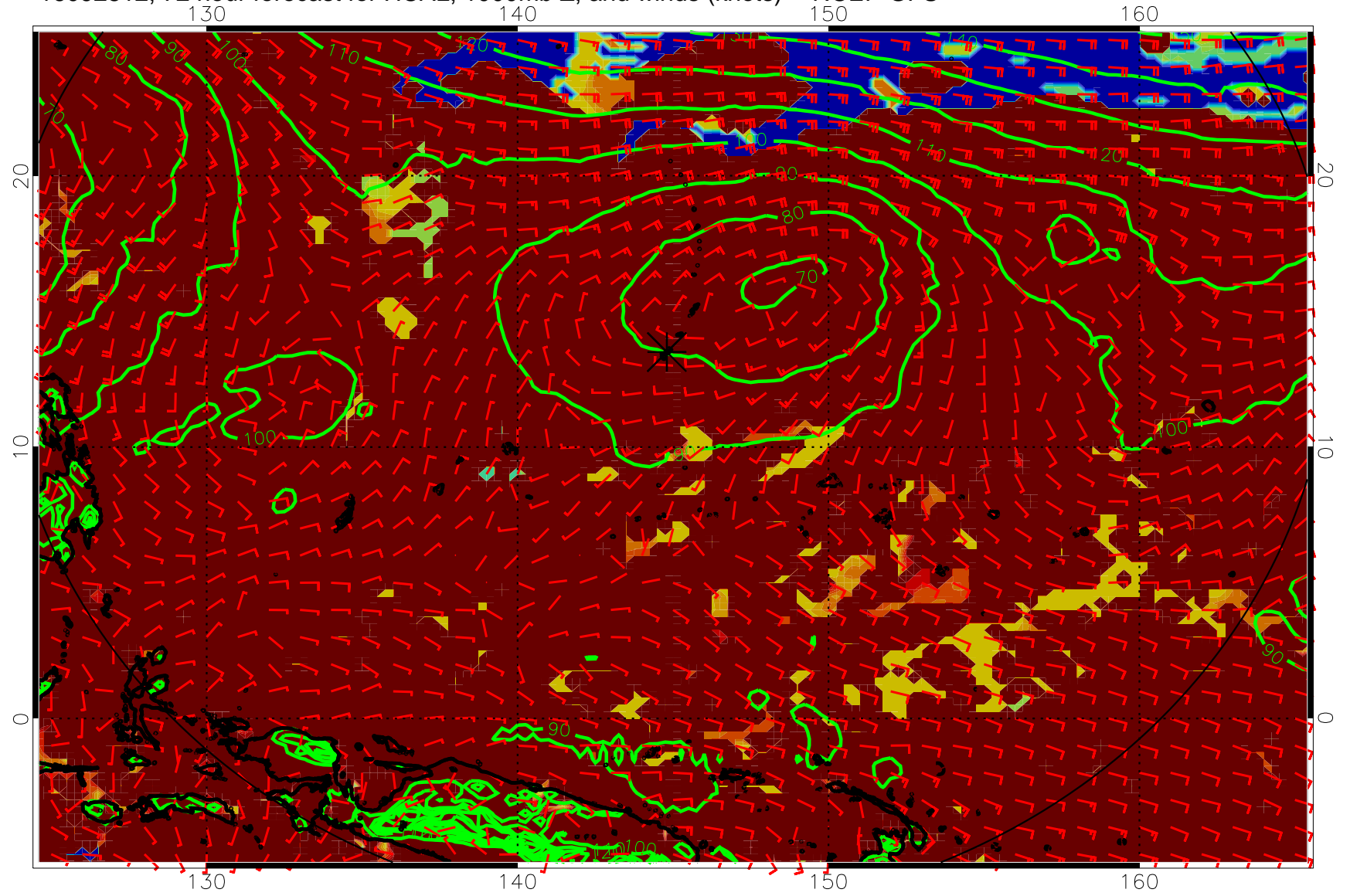
16092812, 72 hour forecast for HCAL, 1000mb Z, and winds (knots) -- NCEP GFS
